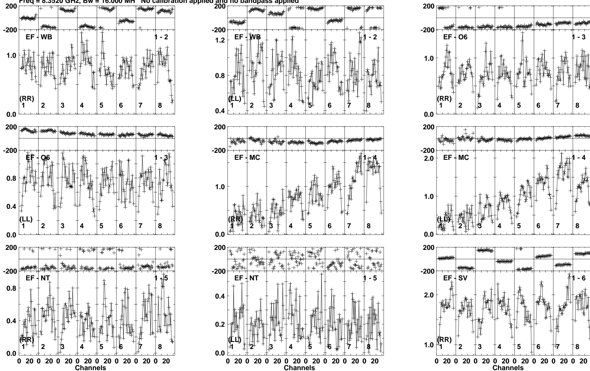
Lower frame: Milli Ampl Jy Top frame: Phas deg Vector averaged cross-power spectrum Baseline: EF (01) - WB (02) Timerange: 00/13:07:51 to 00/13:08:49
