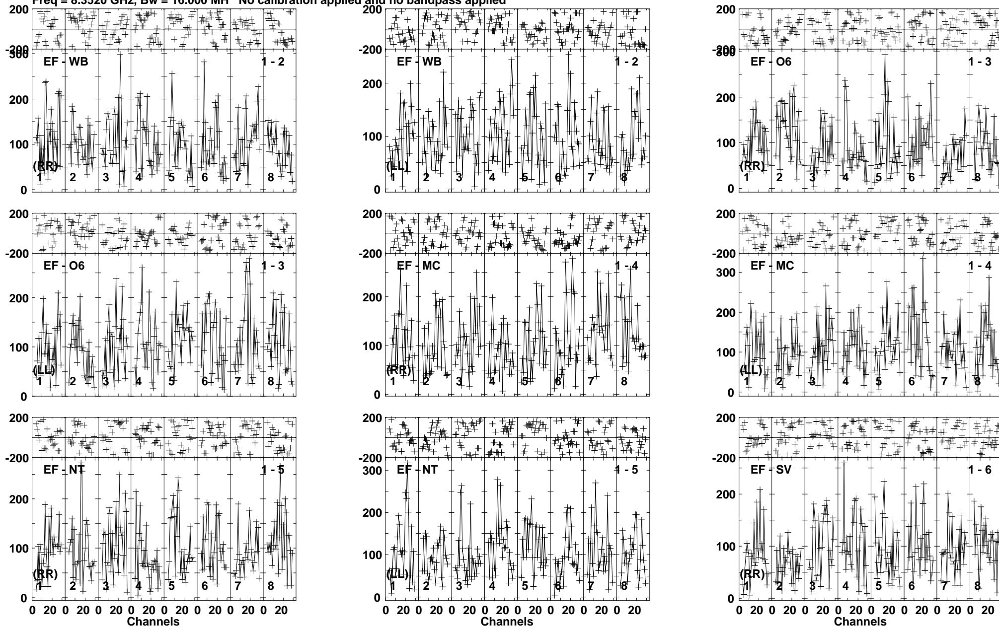
Lower frame: Micro Ampl Jy Top frame: Phas deg Vector averaged cross-power spectrum Baseline: EF (01) - WB (02) Timerange: 00/13:05:01 to 00/13:07:43
