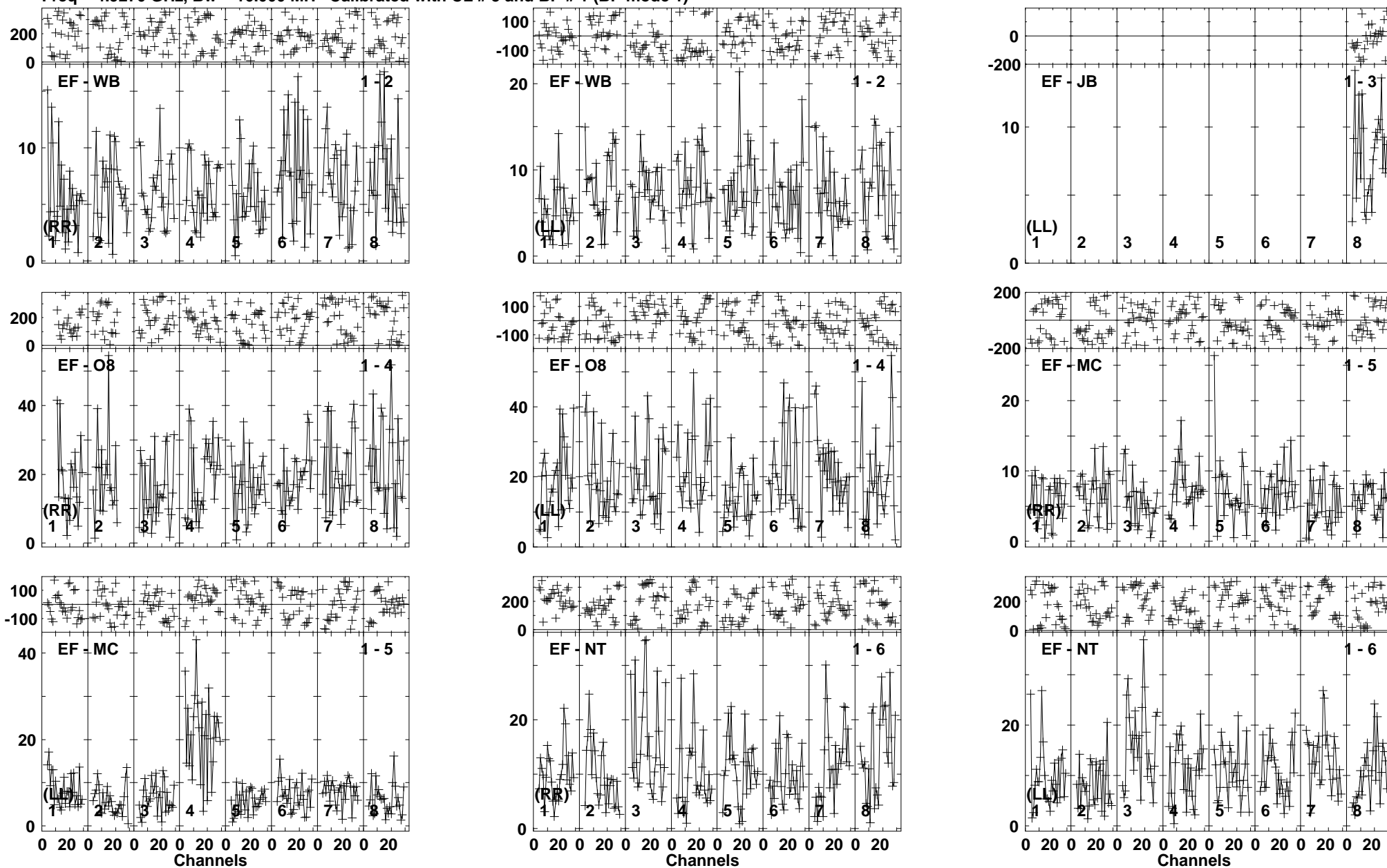
Lower frame: Milli Ampl Jy Top frame: Phas deg Vector averaged cross-power spectrum Baseline: EF (01) - WB (02) Timerange: 00/09:05:47 to 00/09:09:21
