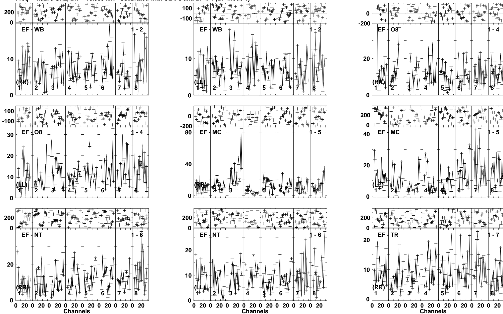
Lower frame: Milli Ampl Jy Top frame: Phas deg Vector averaged cross-power spectrum Baseline: EF (01) - WB (02) Timerange: 00/11:32:17 to 00/11:35:51
