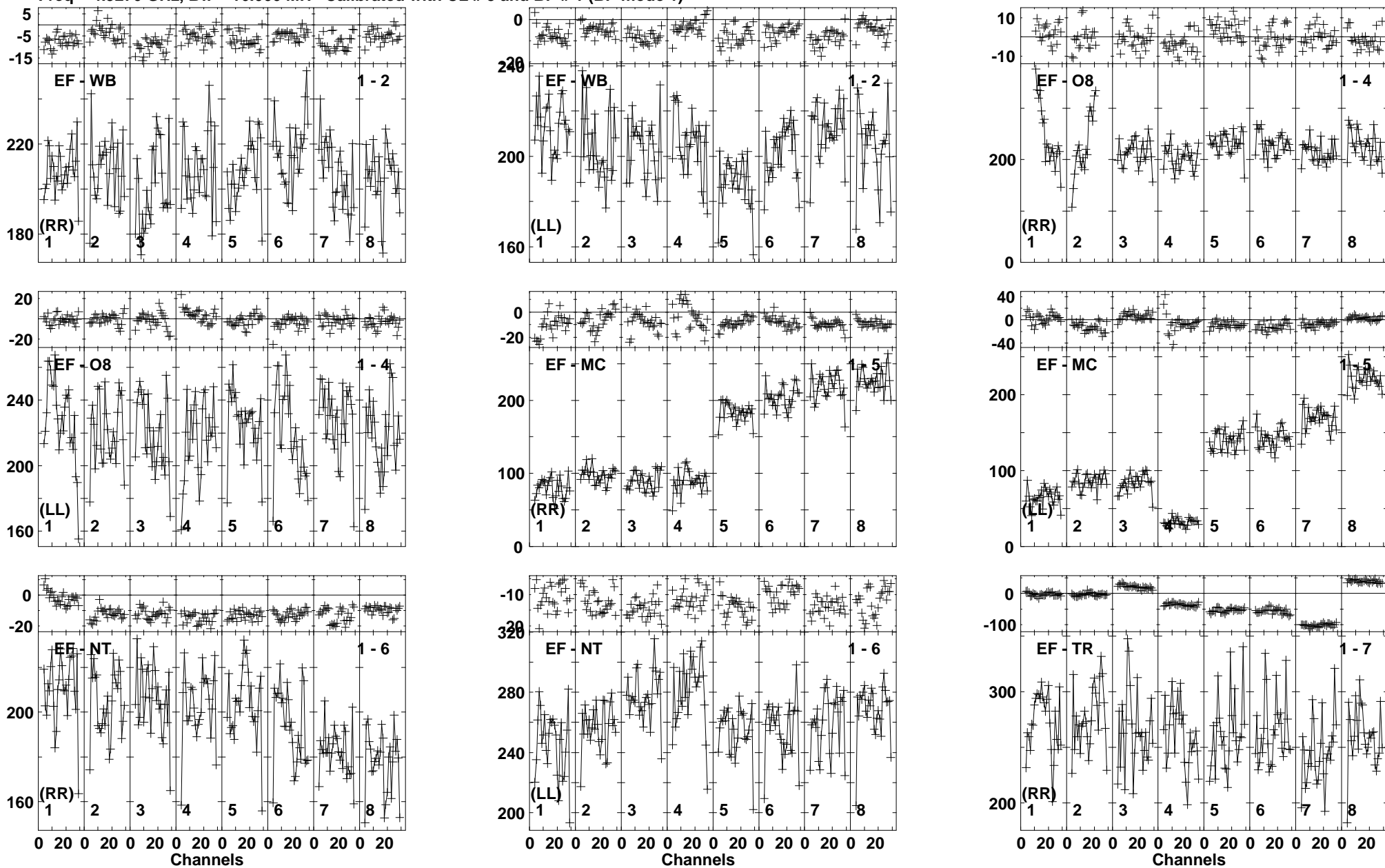
Lower frame: Milli Ampl Jy Top frame: Phas deg Vector averaged cross-power spectrum Baseline: EF (01) - WB (02) Timerange: 00/11:01:53 to 00/11:02:55
