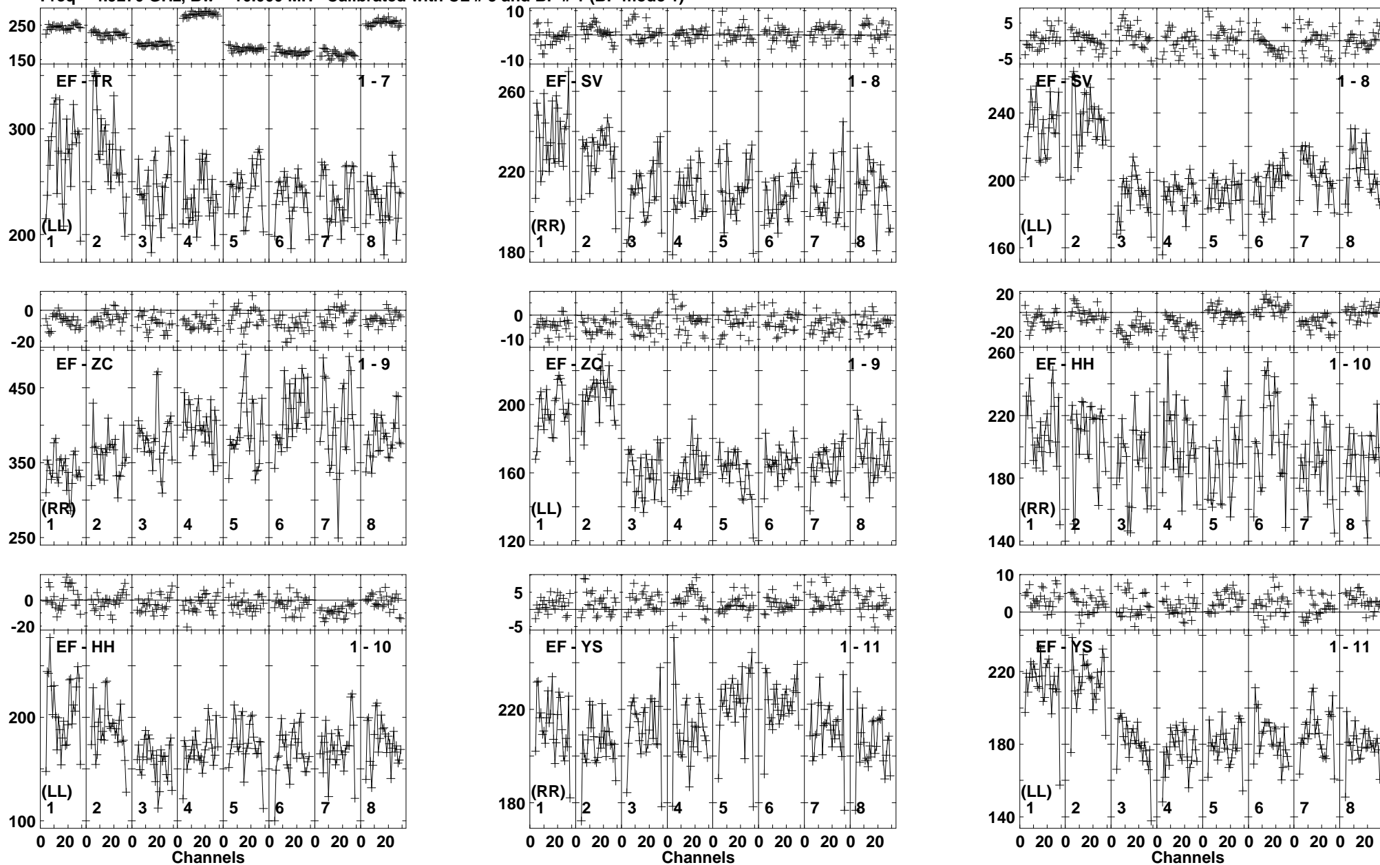
Lower frame: Milli Ampl Jy Top frame: Phas deg Vector averaged cross-power spectrum Baseline: EF (01) - TR (07) Timerange: 00/10/03:17 to 00/10/04:19
