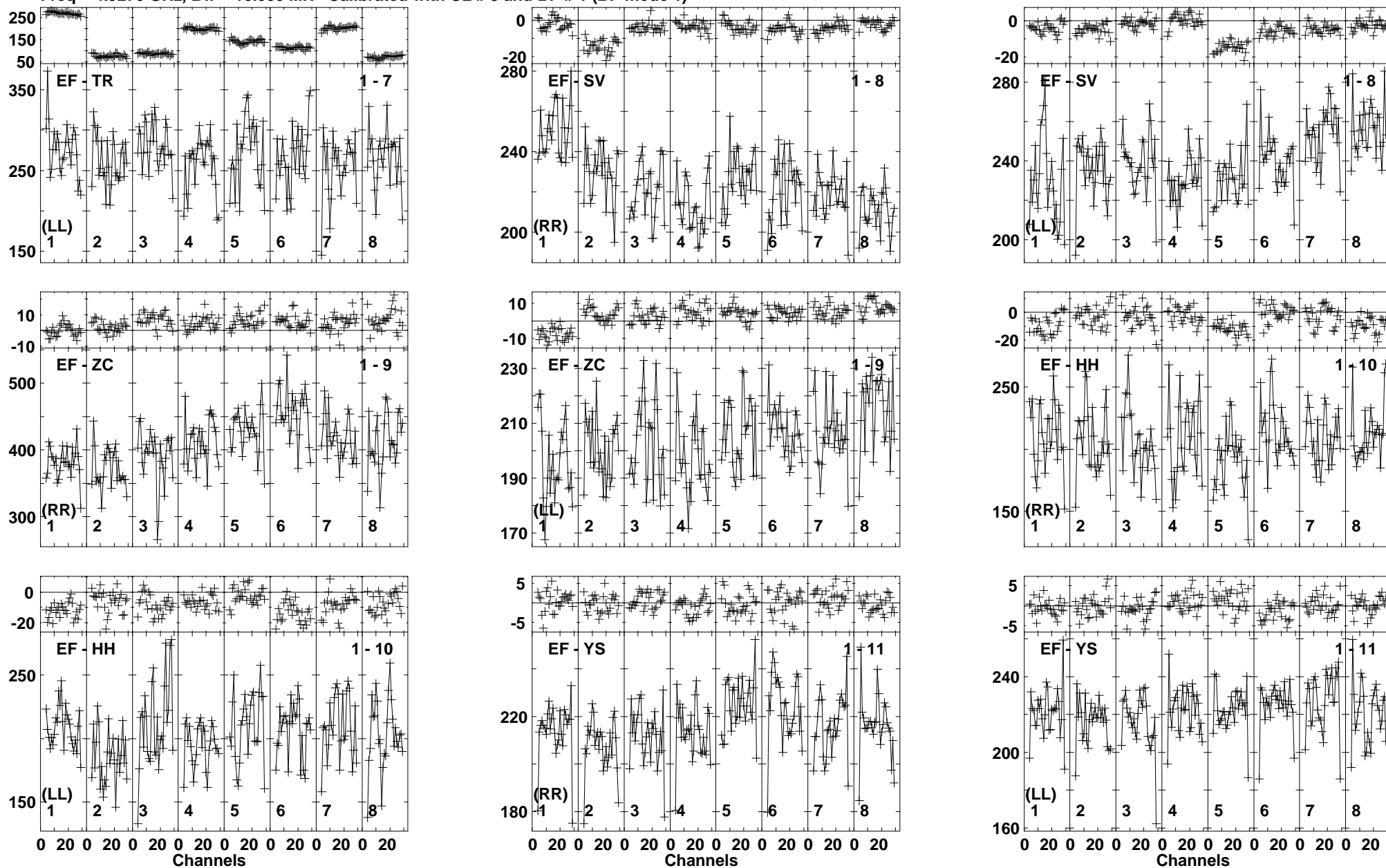
Lower frame: Milli Ampl Jy Top frame: Phas deg Vector averaged cross-power spectrum Baseline: EF (01) - TR (07) Timerange: 00/11:21:25 to 00/11:22:27
