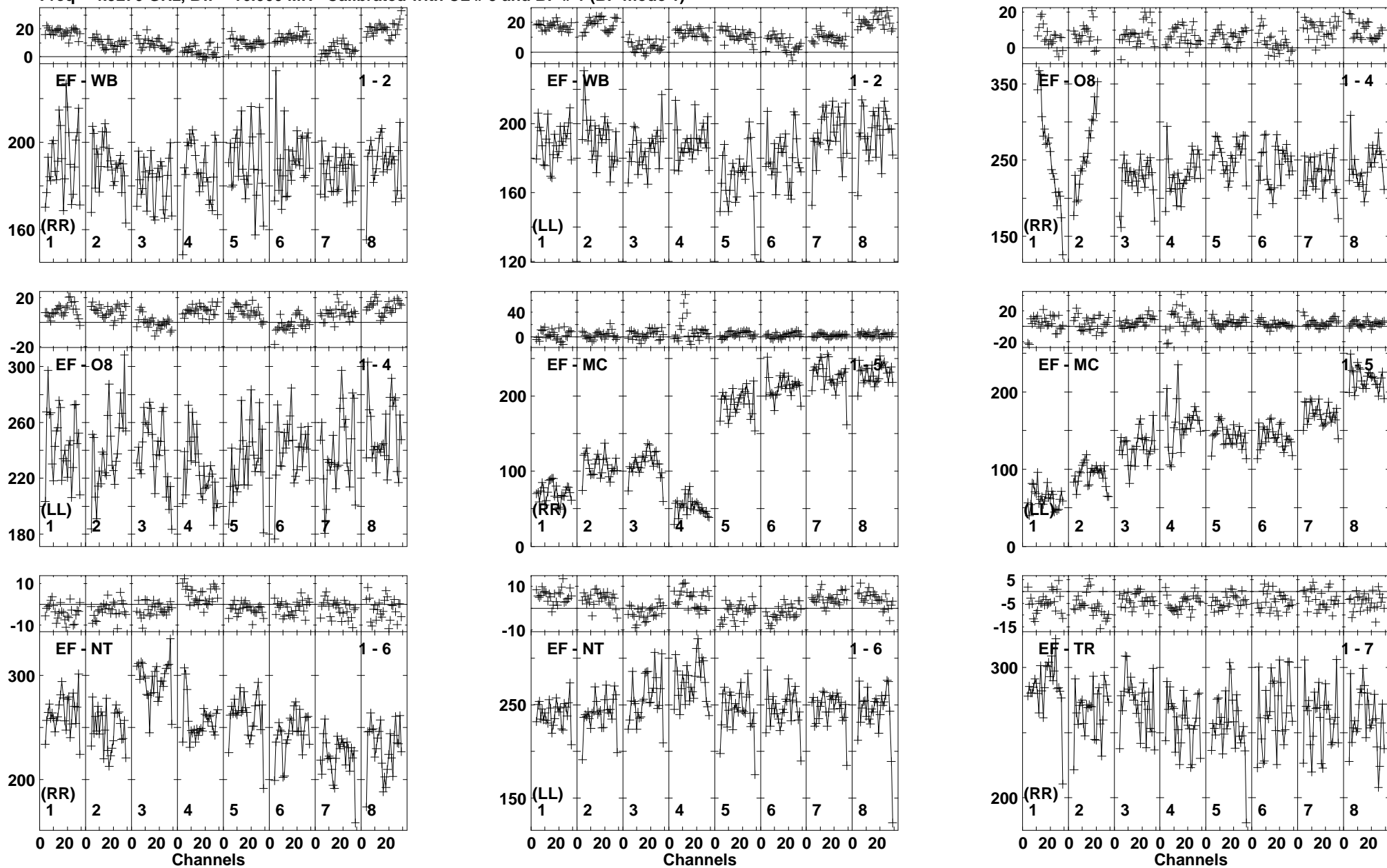
Lower frame: Milli Ampl Jy Top frame: Phas deg Vector averaged cross-power spectrum Baseline: EF (01) - WB (02) Timerange: 00/12:15:39 to 00/12:16:15
