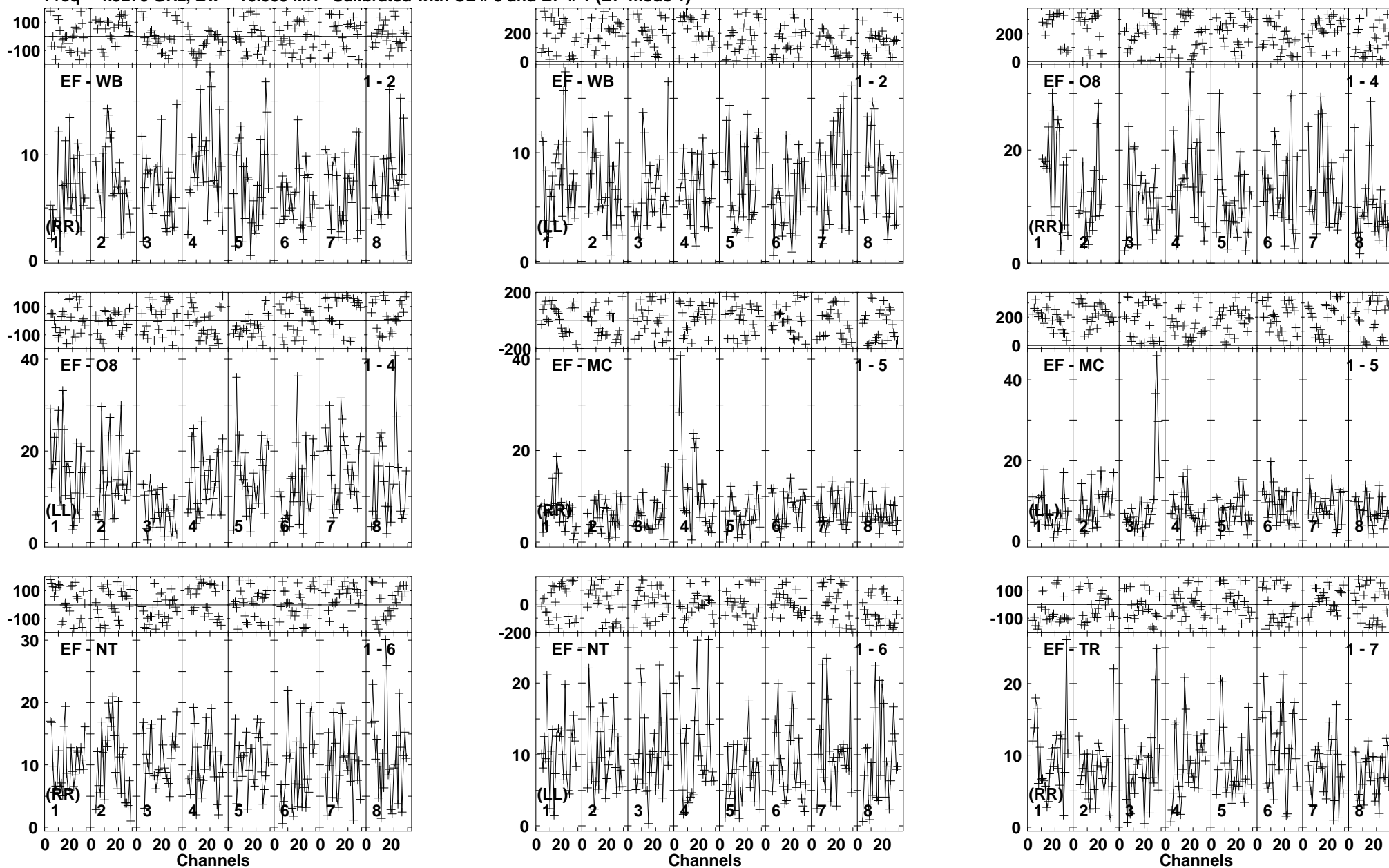
Lower frame: Milli Ampl Jy Top frame: Phas deg Vector averaged cross-power spectrum Baseline: EF (01) - WB (02) Timerange: 00:12:55:37 to 00:12:58:49
