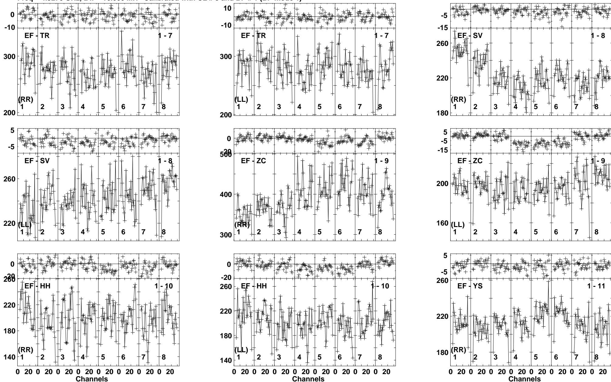
Lower frame: Milli Ampl Jy Top frame: Phas deg Vector averaged cross-power spectrum Baseline: EF (01) - TR (07) Timerange: 00/09:58:55 to 00/09:59:31
