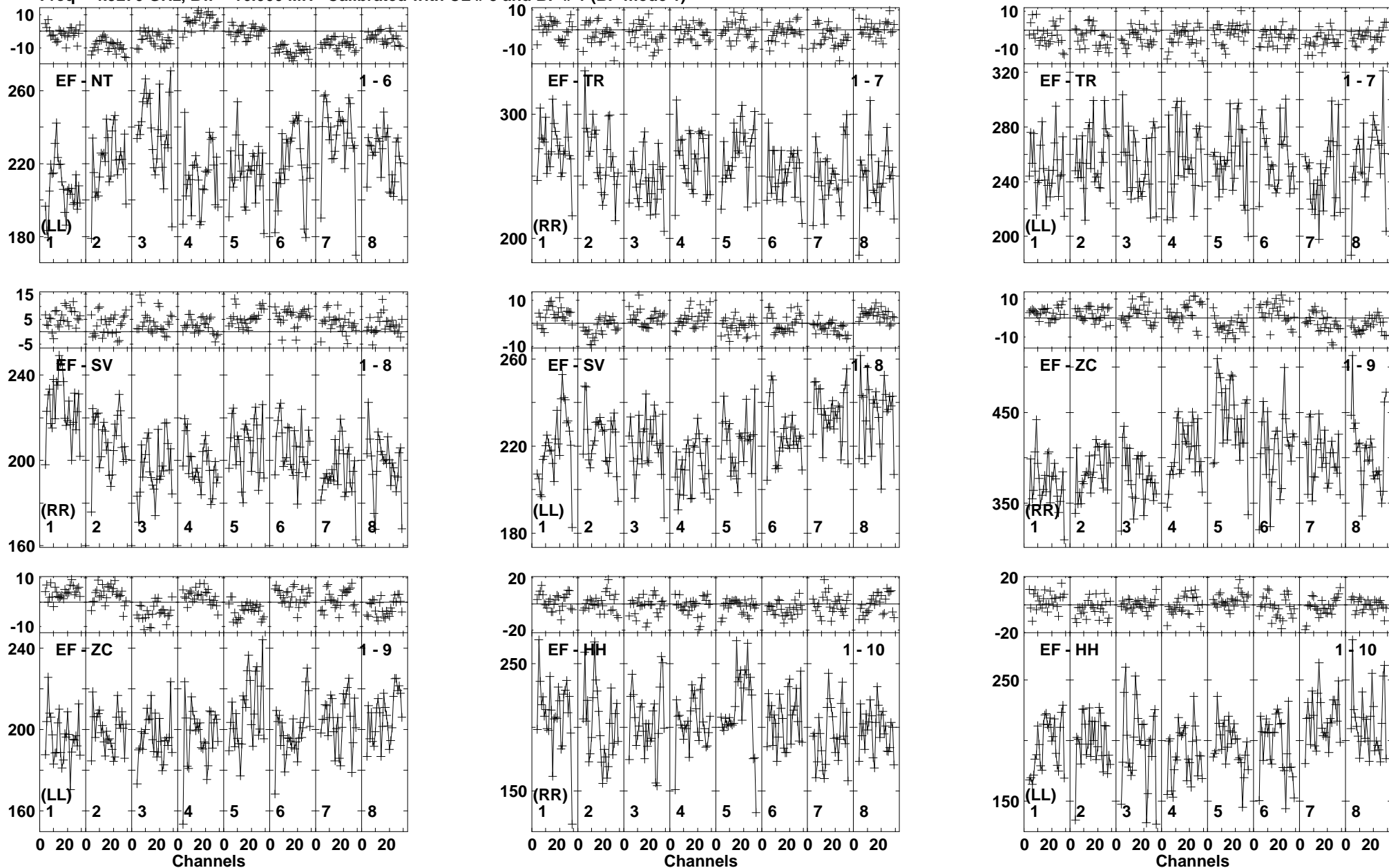
Lower frame: Milli Ampl Jy Top frame: Phas deg Vector averaged cross-power spectrum Baseline: EF (01) - NT (06) Timerange: 00/08:21:13 to 00/08:21:51
