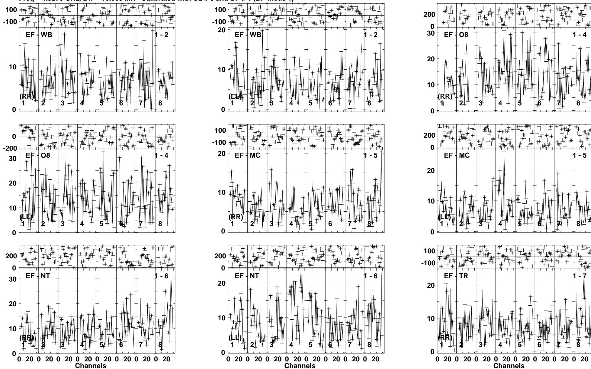
Lower frame: Milli Ampl Jy Top frame: Phas deg Vector averaged cross-power spectrum Baseline: EF (01) - WB (02) Timerange: 00/10:19:10 to 00/10:22:40
