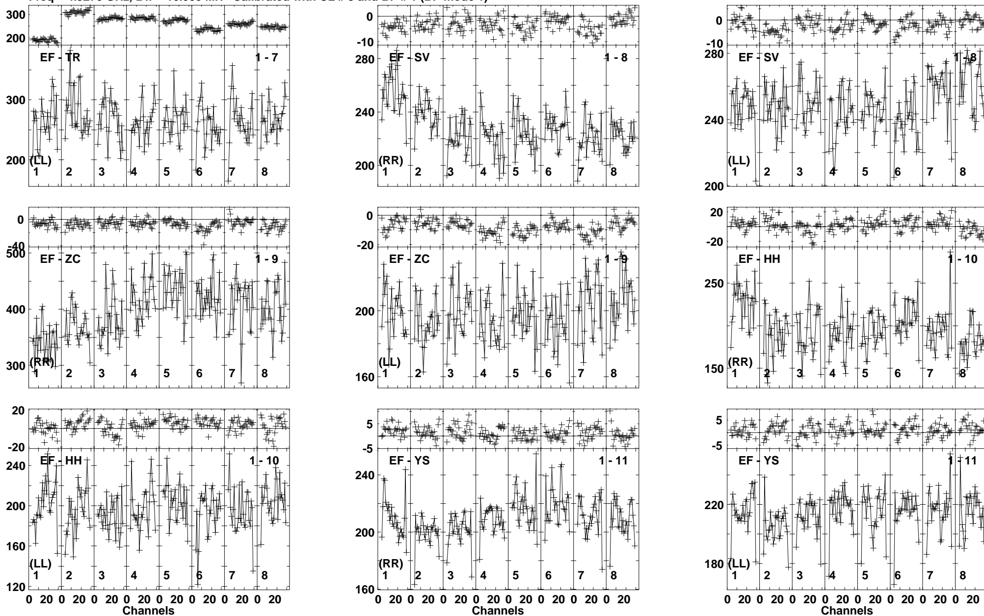
Lower frame: Milli Ampl Jy Top frame: Phas deg Vector averaged cross-power spectrum Baseline: EF (01) - TR (07) Timerange: 00/11:40:57 to 00/11:41:59
