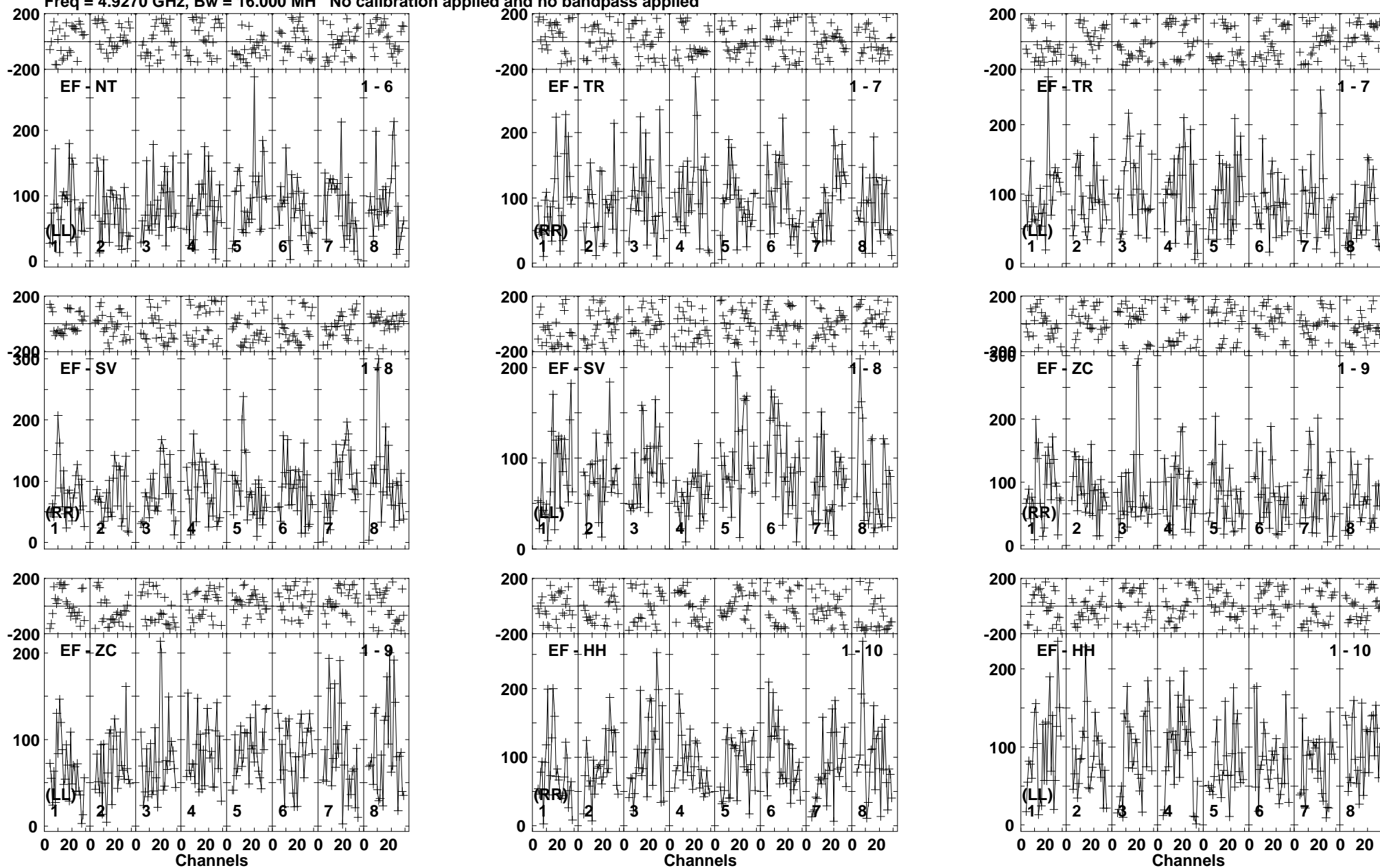
Lower frame: Micro Ampl Jy Top frame: Phas deg Vector averaged cross-power spectrum Baseline: EF (01) - NT (06) Timerange: 00/09:44:51 to 00/09:48:25
