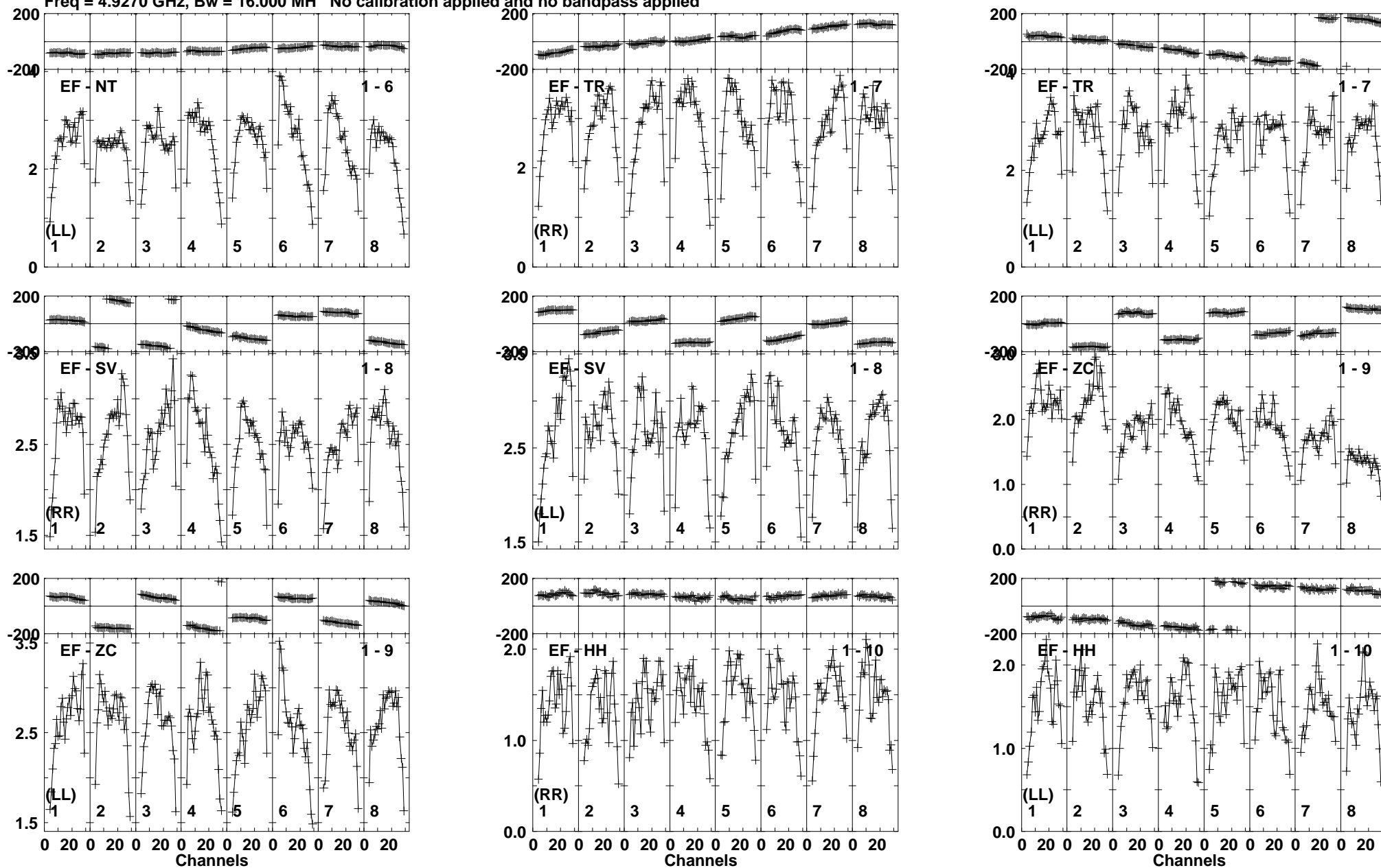
Lower frame: Milli Ampl Jy Top frame: Phas deg Vector averaged cross-power spectrum Baseline: EF (01) - NT (06) Timerange: 00/08:31:01 to 00/08:31:37
