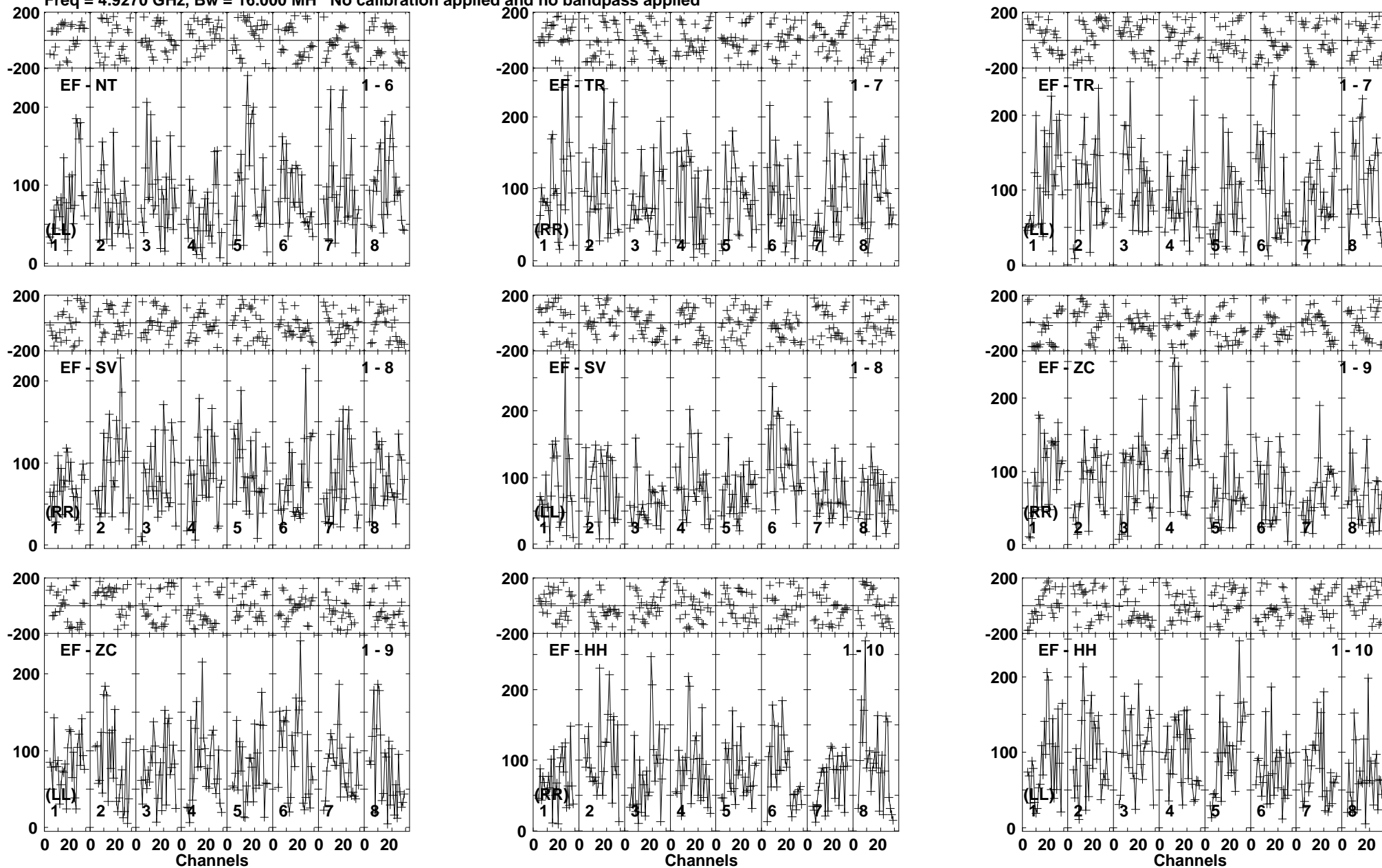
Lower frame: Micro Ampl Jy Top frame: Phas deg Vector averaged cross-power spectrum Baseline: EF (01) - NT (06) Timerange: 00/11:47:05 to 00/11:50:35
