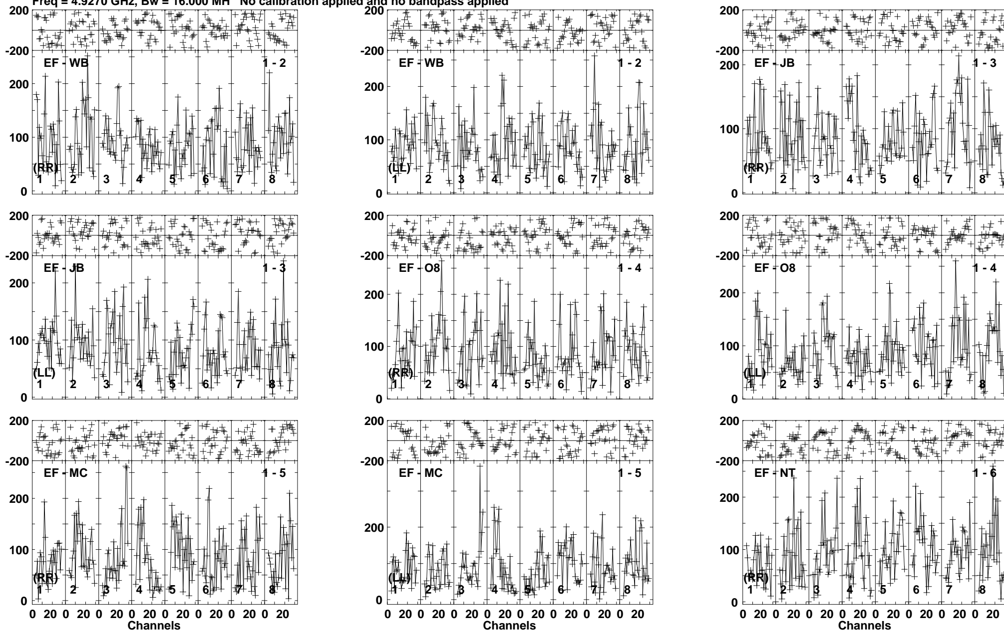
Lower frame: Micro Ampl Jy Top frame: Phas deg Vector averaged cross-power spectrum Baseline: EF (01) - WB (02) Timerange: 00/11:32:17 to 00/11:35:51
