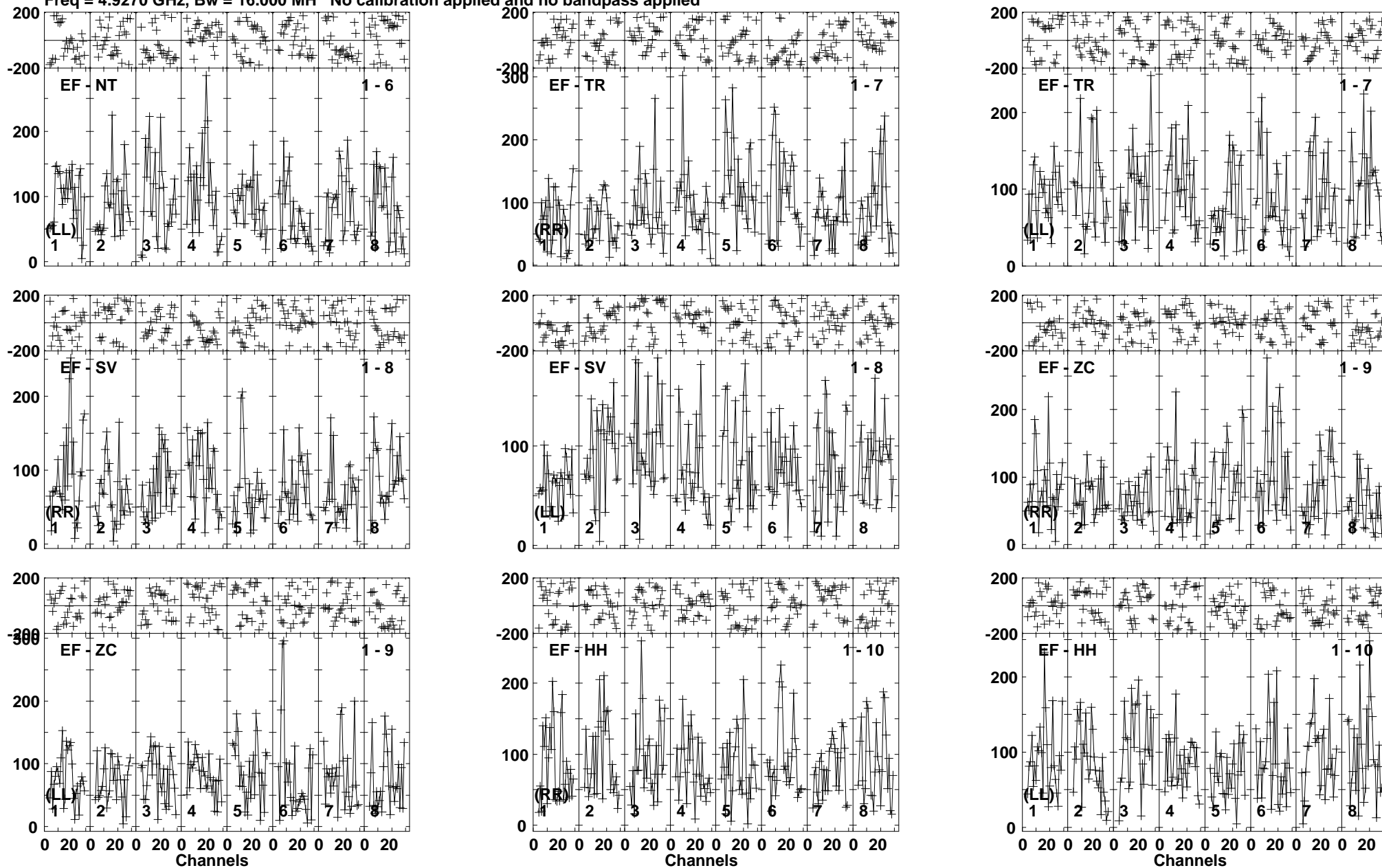
Lower frame: Micro Ampl Jy Top frame: Phas deg Vector averaged cross-power spectrum Baseline: EF (01) - NT (06) Timerange: 00/10:38:42 to 00/10:42:12
