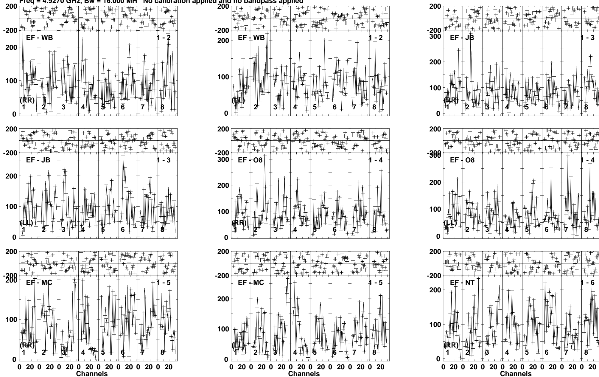
Lower frame: Micro Ampl Jy Top frame: Phas deg Vector averaged cross-power spectrum Baseline: EF (01) - WB (02) Timerange: 00/10:04:23 to 00/10:07:57
