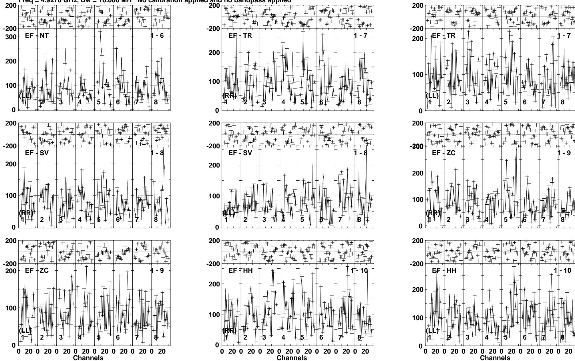
Lower frame: Micro Ampl Jy Top frame: Phas deg Vector averaged cross-power spectrum Baseline: EF (01) - NT (06) Timerange: 00/08:56:01 to 00/08:59:35
