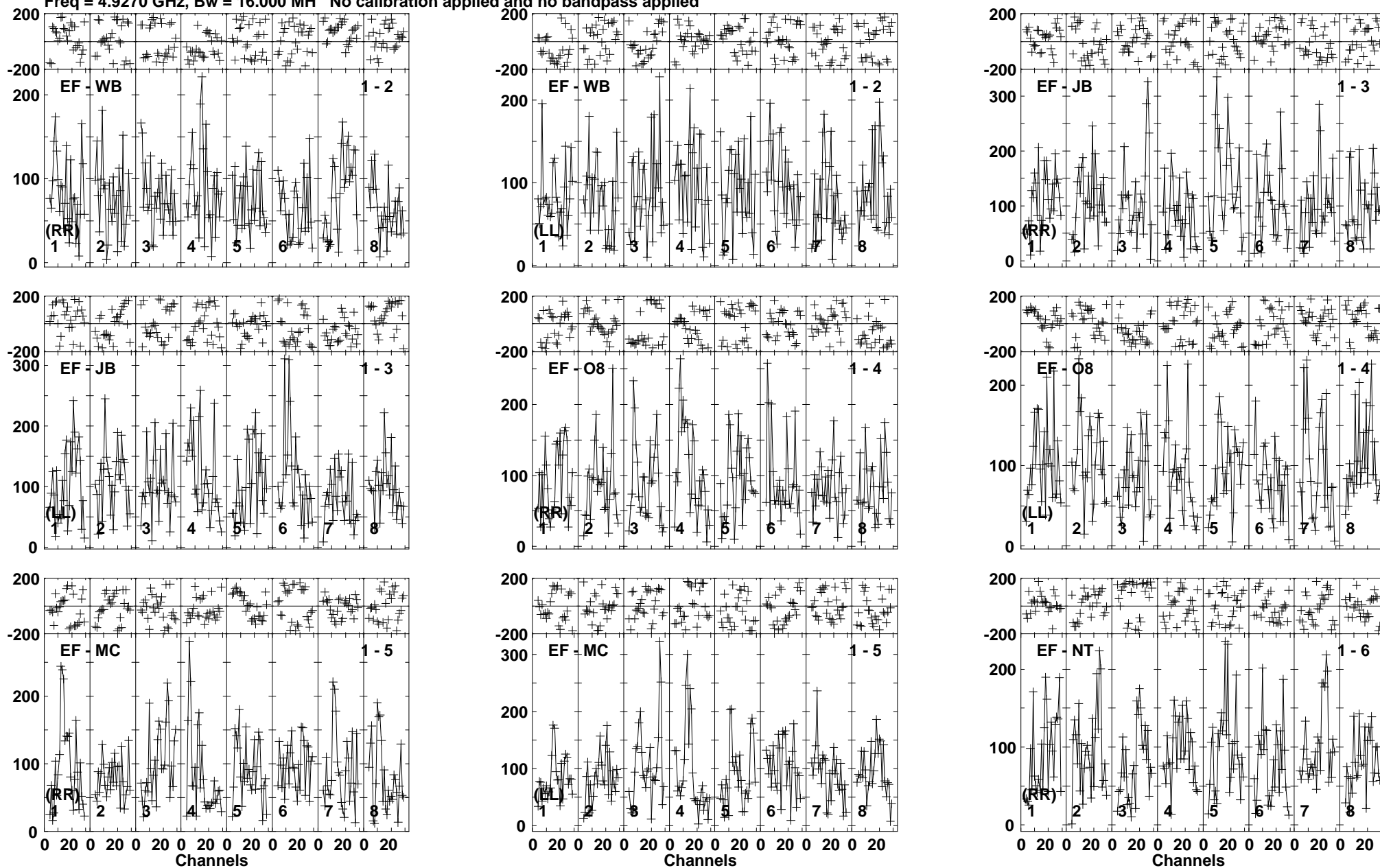
Lower frame: Micro Ampl Jy Top frame: Phas deg Vector averaged cross-power spectrum Baseline: EF (01) - WB (02) Timerange: 00:12:30:53 to 00:12:34:27
