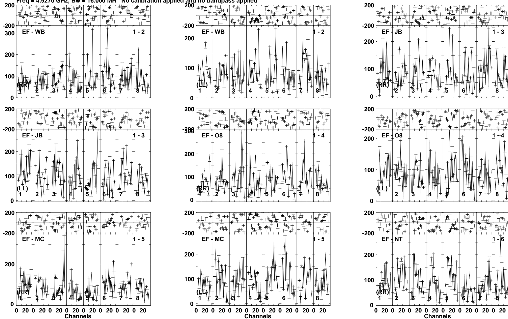
Lower frame: Micro Ampl Jy Top frame: Phas deg Vector averaged cross-power spectrum Baseline: EF (01) - WB (02) Timerange: 00/12:26:09 to 00/12:29:39
