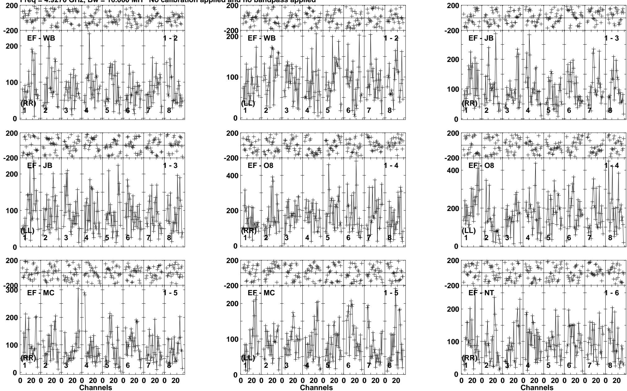
Lower frame: Micro Ampl Jy Top frame: Phas deg Vector averaged cross-power spectrum Baseline: EF (01) - WB (02) Timerange: 00/08:31:45 to 00/08:35:15
