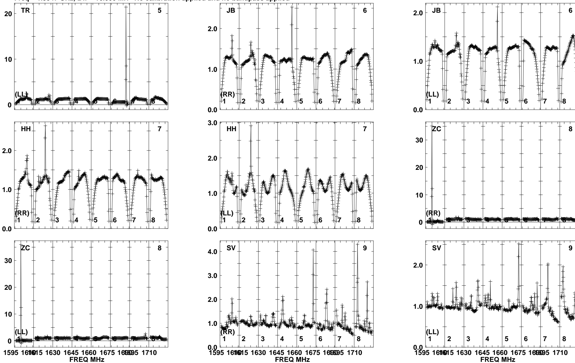
Lower frame: Real Jy Total-power spectrum Antenna: TR (05) Timerange: 00/20:25:06 to 00/20:26:34
