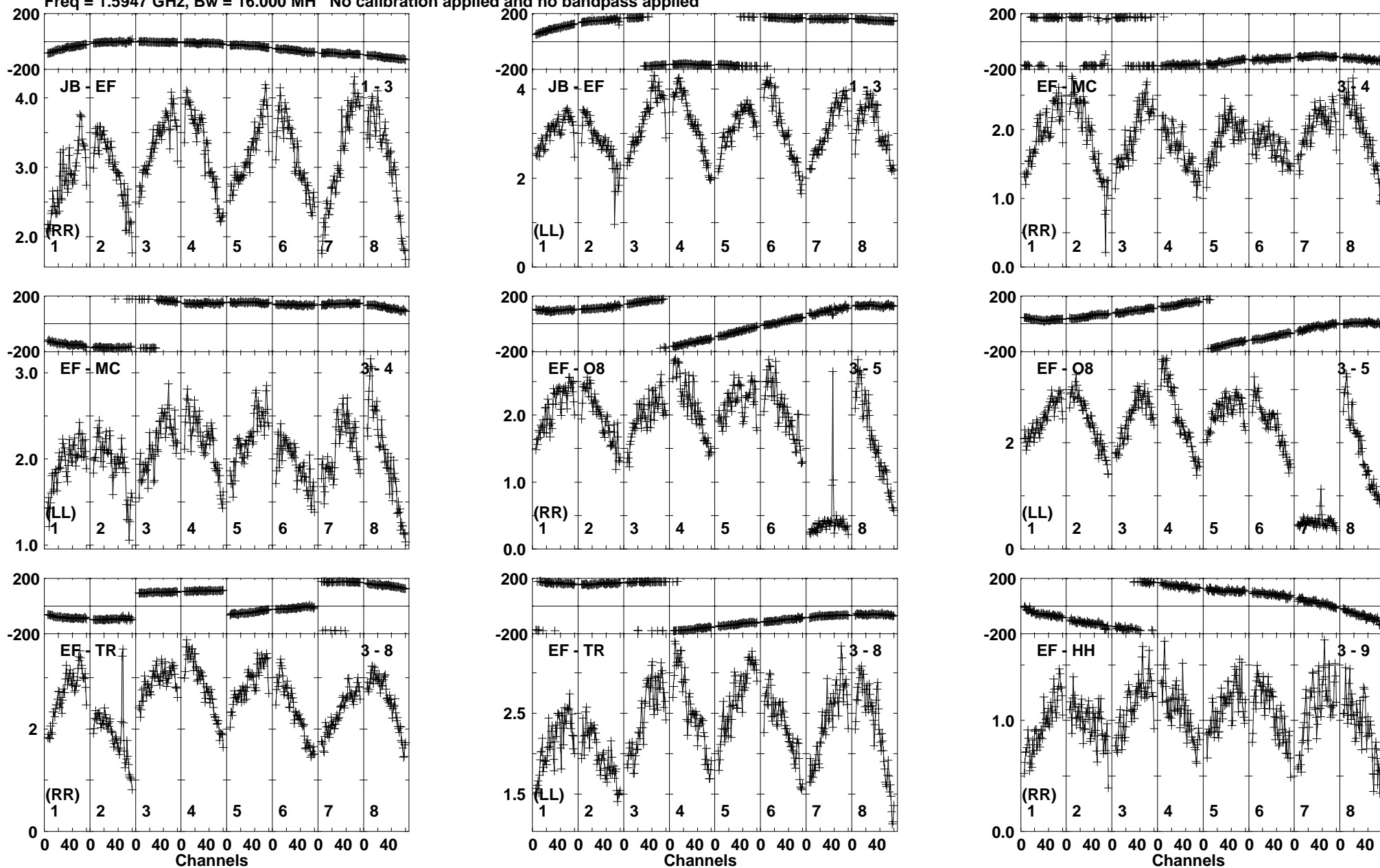
Lower frame: Milli Ampl Jy Top frame: Phas deg Vector averaged cross-power spectrum Baseline: JB (01) - EF (03) Timerange: 00:12:40:03 to 00:12:41:29
