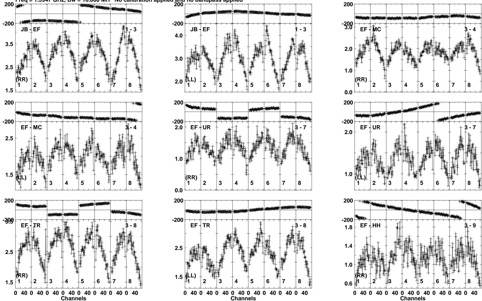
Lower frame: Milli Ampl Jy Top frame: Phas deg Vector averaged cross-power spectrum Baseline: JB (01) - EF (03) Timerange: 00/10:21:18 to 00/10:22:44
