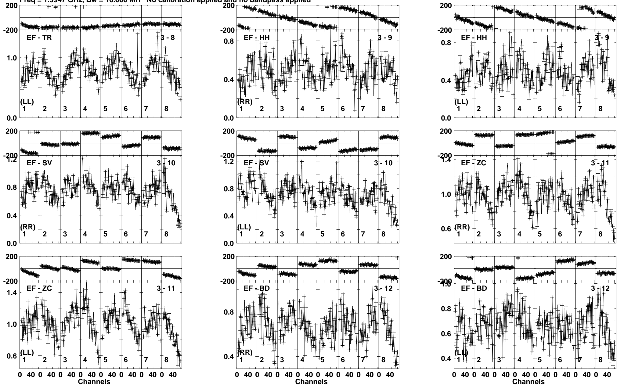
Lower frame: Milli Ampl Jy Top frame: Phas deg Vector averaged cross-power spectrum Baseline: EF (03) - TR (08) Timerange: 00/08:17:01 to 00/08:18:59
