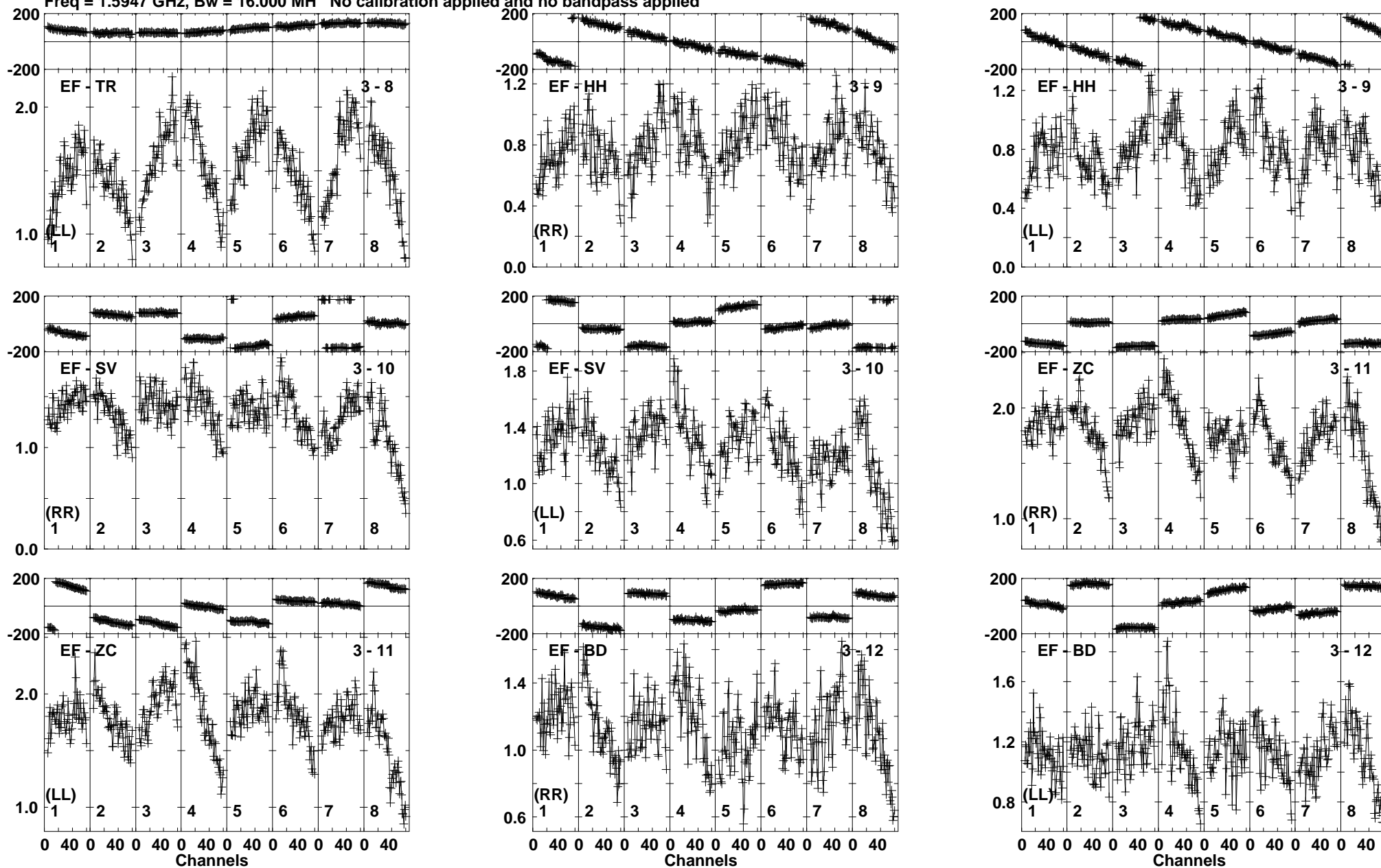
Lower frame: Milli Ampl Jy Top frame: Phas deg Vector averaged cross-power spectrum Baseline: EF (03) - TR (08) Timerange: 00/08:38:31 to 00/08:39:59
