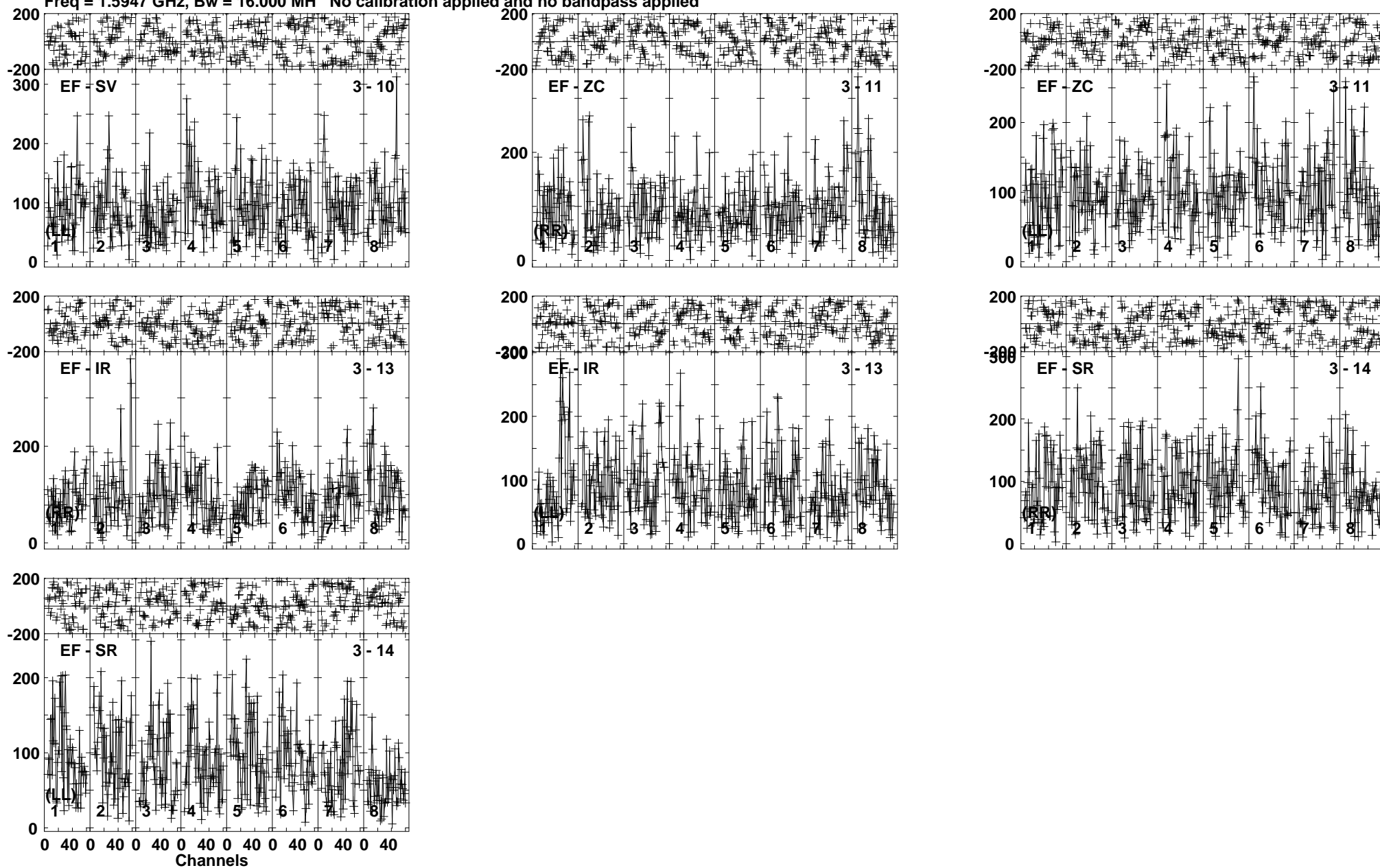
Lower frame: Micro Ampl Jy Top frame: Phas deg Vector averaged cross-power spectrum Baseline: EF (03) - SV (10) Timerange: 00/11:53:46 to 00/11:58:44
