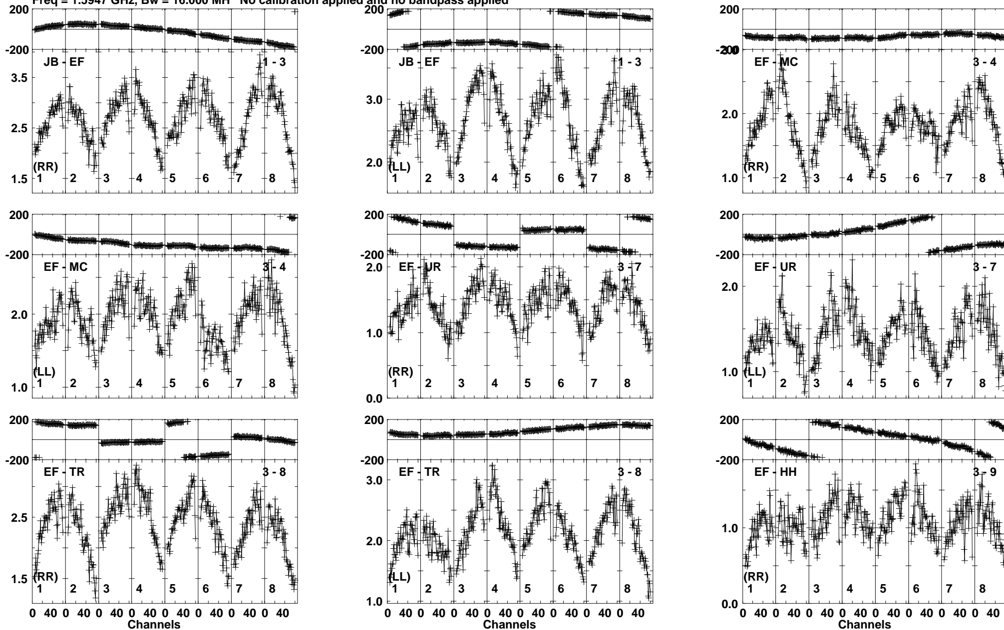
Lower frame: Milli Ampl Jy Top frame: Phas deg Vector averaged cross-power spectrum Baseline: JB (01) - EF (03) Timerange: 00/09:26:18 to 00/09:27:44
