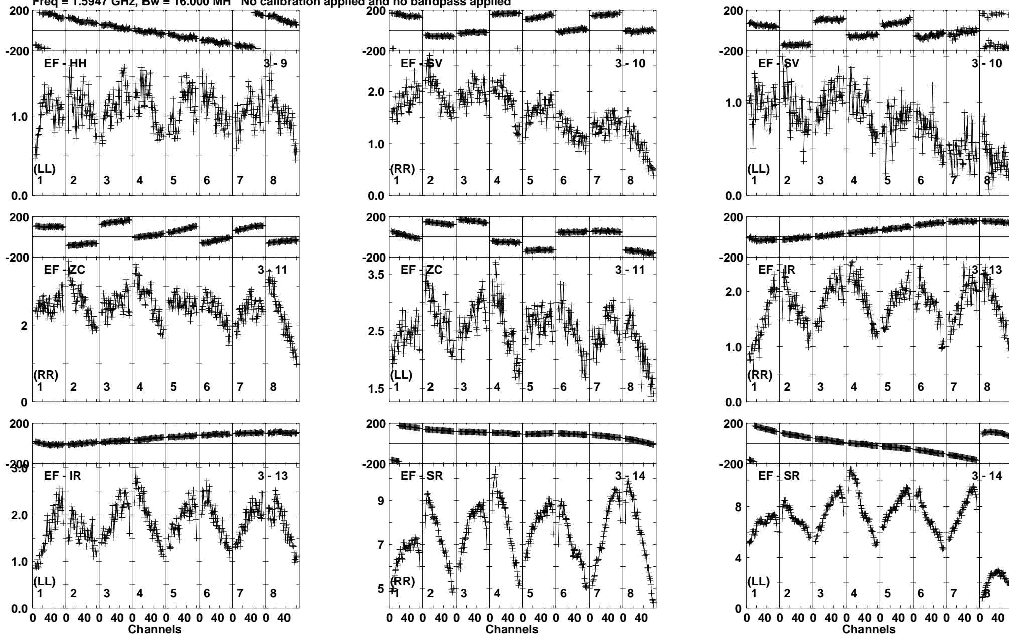
Lower frame: Milli Ampl Jy Top frame: Phas deg Vector averaged cross-power spectrum Baseline: EF (03) - HH (09) Timerange: 00:12:26:18 to 00:12:27:44
