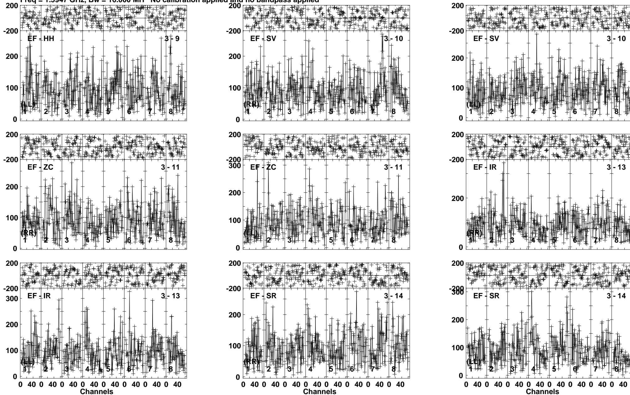
Lower frame: Micro Ampl Jy Top frame: Phas deg Vector averaged cross-power spectrum Baseline: EF (03) - HH (09) Timerange: 00/09:55:16 to 00/10:00:14
