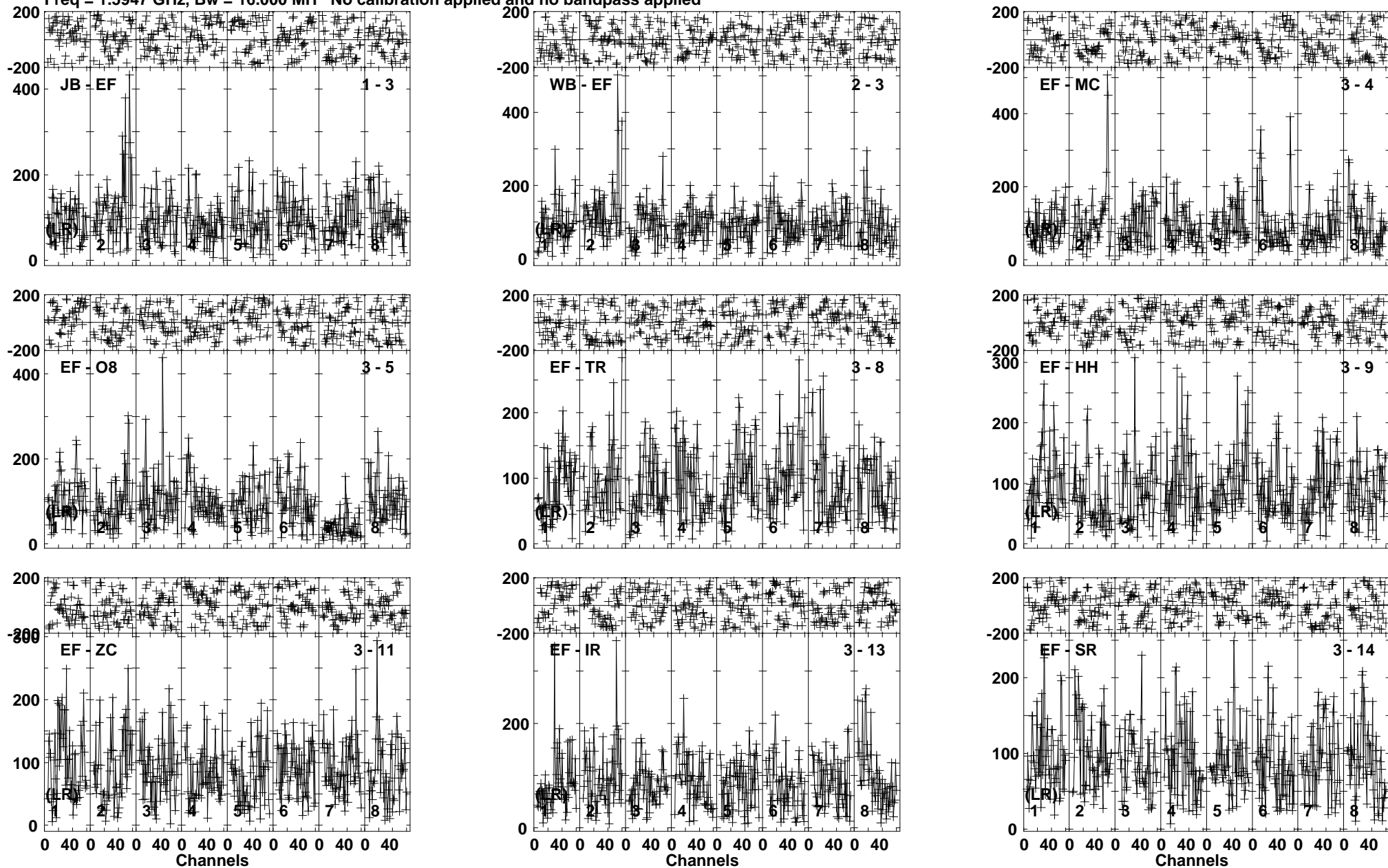
Lower frame: Micro Ampl Jy Top frame: Phas deg Vector averaged cross-power spectrum Baseline: JB (01) - EF (03) Timerange: 00:12:41:31 to 00:12:46:29
