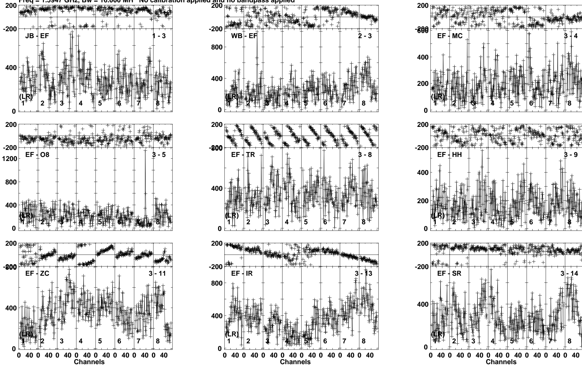
Lower frame: Micro Ampl Jy Top frame: Phas deg Vector averaged cross-power spectrum Baseline: JB (01) - EF (03) Timerange: 00/13:42:16 to 00/13:43:44
