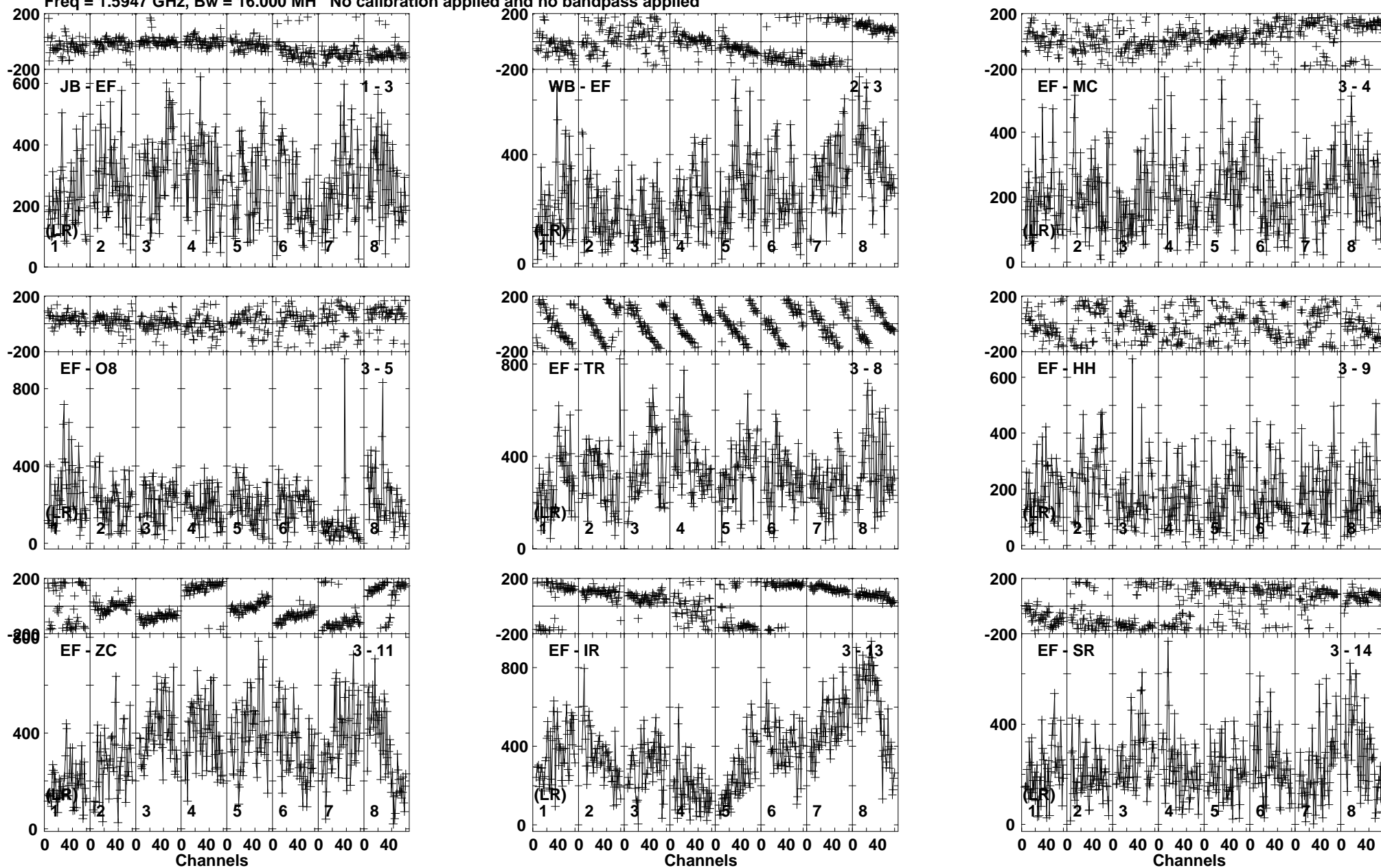
Lower frame: Micro Ampl Jy Top frame: Phas deg Vector average cross-power spectrum Baseline: JB (01) - EF (03) Timerange: 00/12:47:16 to 00/12:48:44
