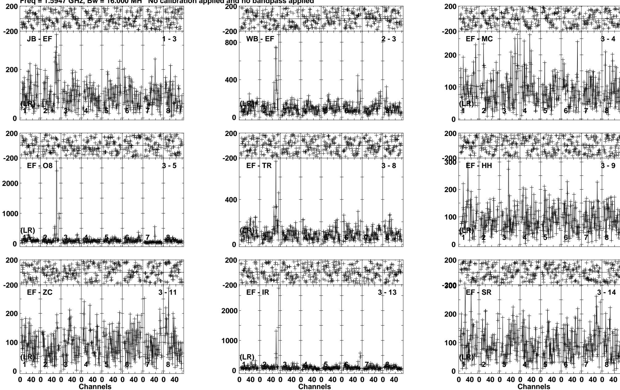
Lower frame: Micro Ampl Jy Top frame: Phas deg Vector averaged cross-power spectrum Baseline: JB (01) - EF (03) Timerange: 00/13:43:46 to 00/13:48:44
