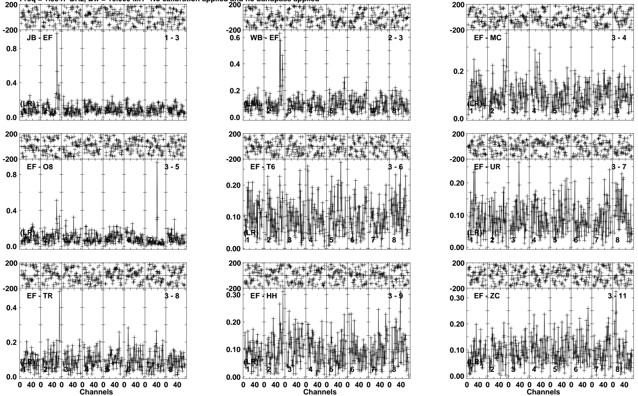
Lower frame: Milli Ampl Jy Top frame: Phas deg Vector averaged cross-power spectrum Baseline: JB (01) - EF (03) Timerange: 00/09:00:16 to 00/09:05:14
