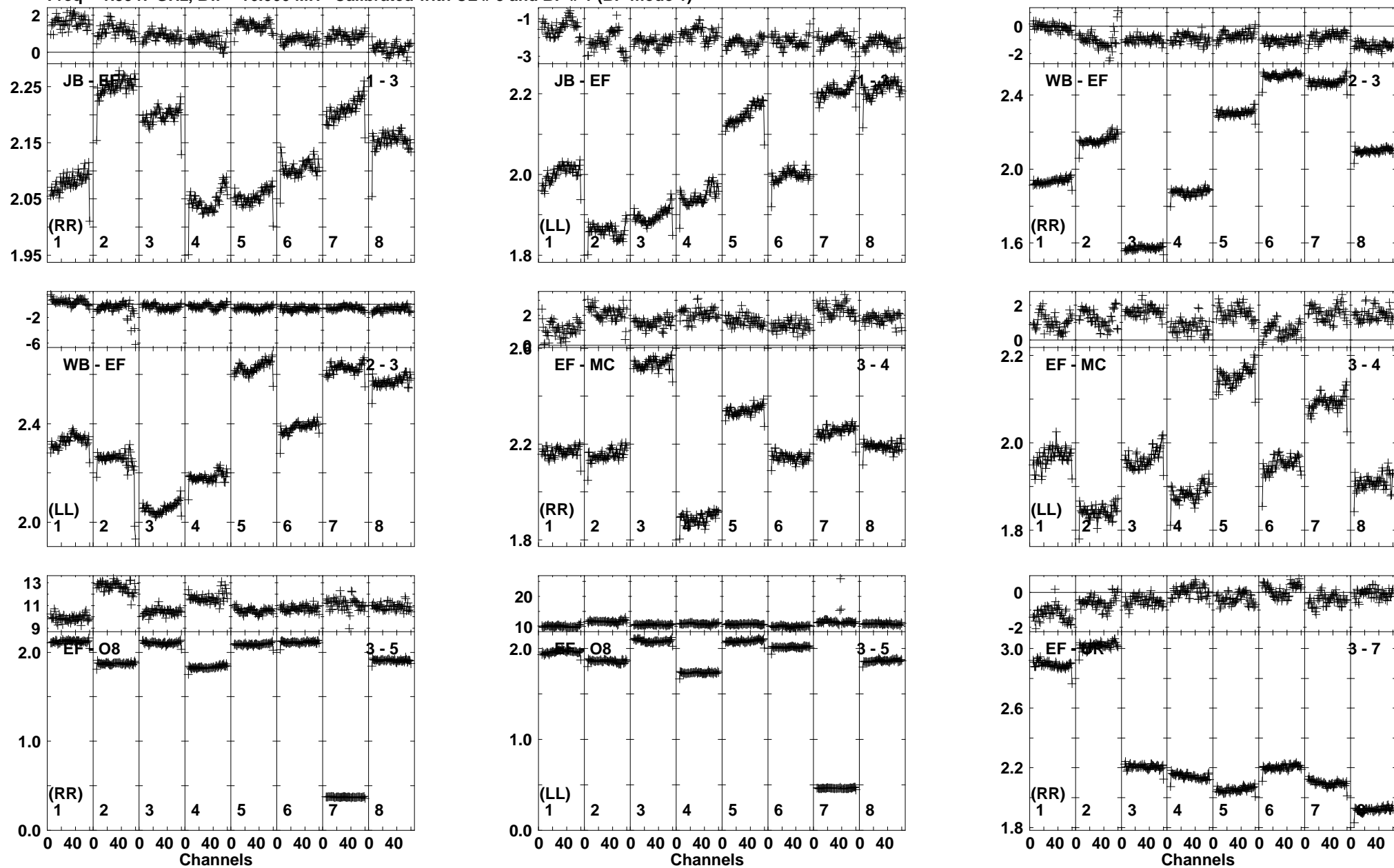
Lower frame: Ampl Jy Top frame: Phas deg Vector averaged cross-power spectrum Baseline: JB (01) - EF (03) Timerange: 00/13:53:56 to 00/13:59:54
