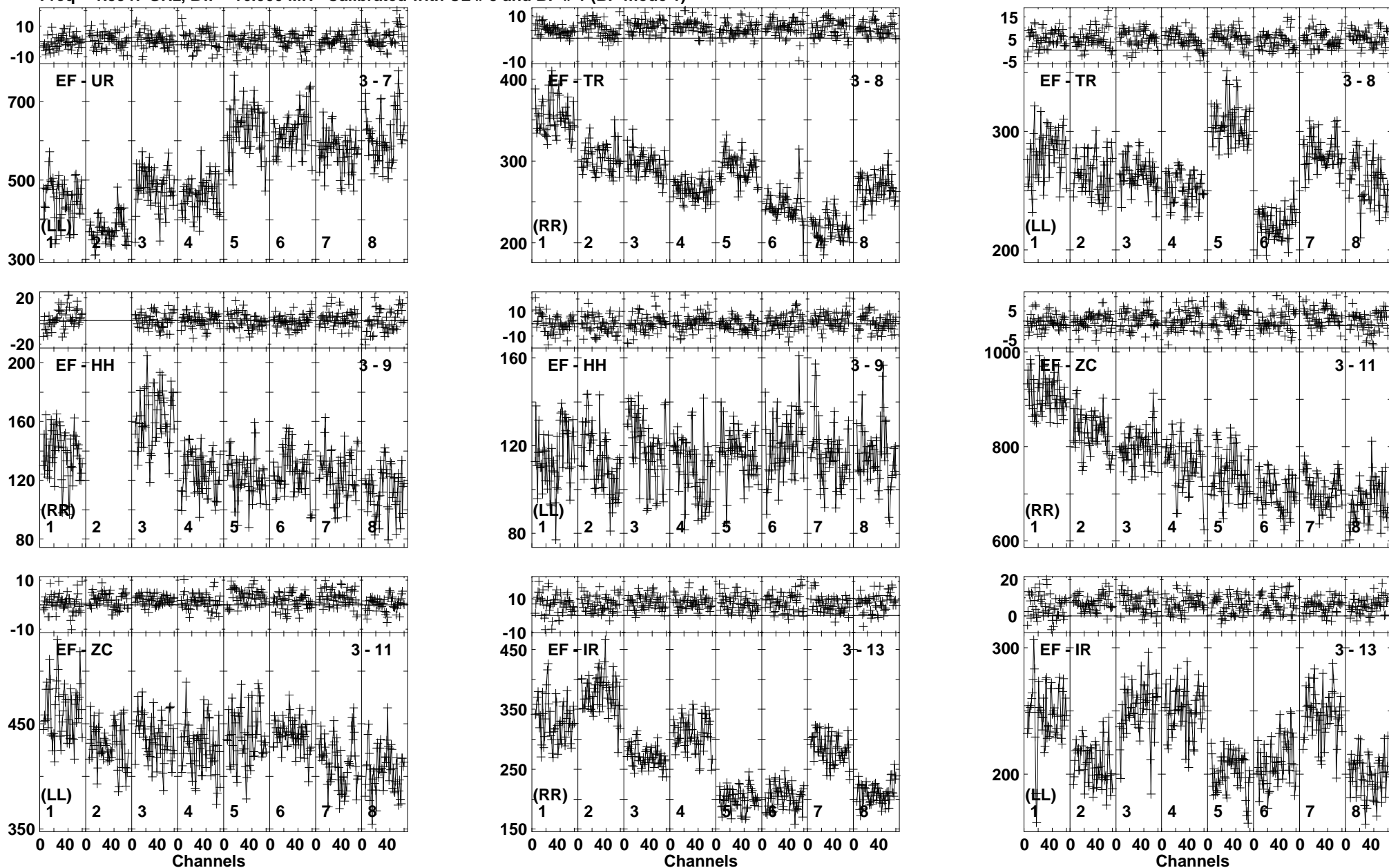
Lower frame: Milli Ampl Jy Top frame: Phas deg Vector averaged cross-power spectrum Baseline: EF (03) - UR (07) Timerange: 00/09:19:46 to 00/09:21:14
