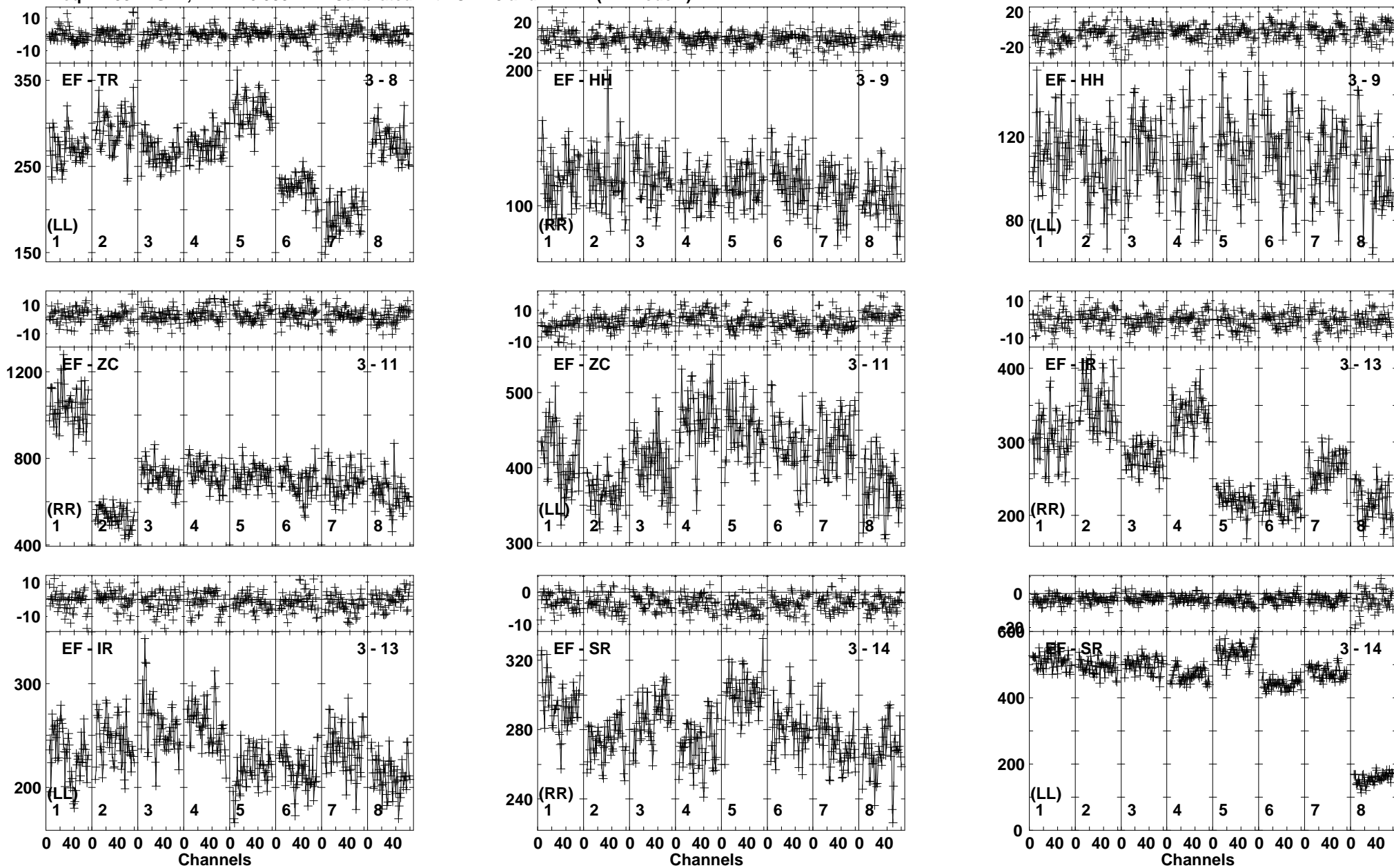
Lower frame: Milli Ampl Jy Top frame: Phas deg Vector averaged cross-power spectrum Baseline: EF (03) - TR (08) Timerange: 00/11:31:16 to 00/11:32:44
