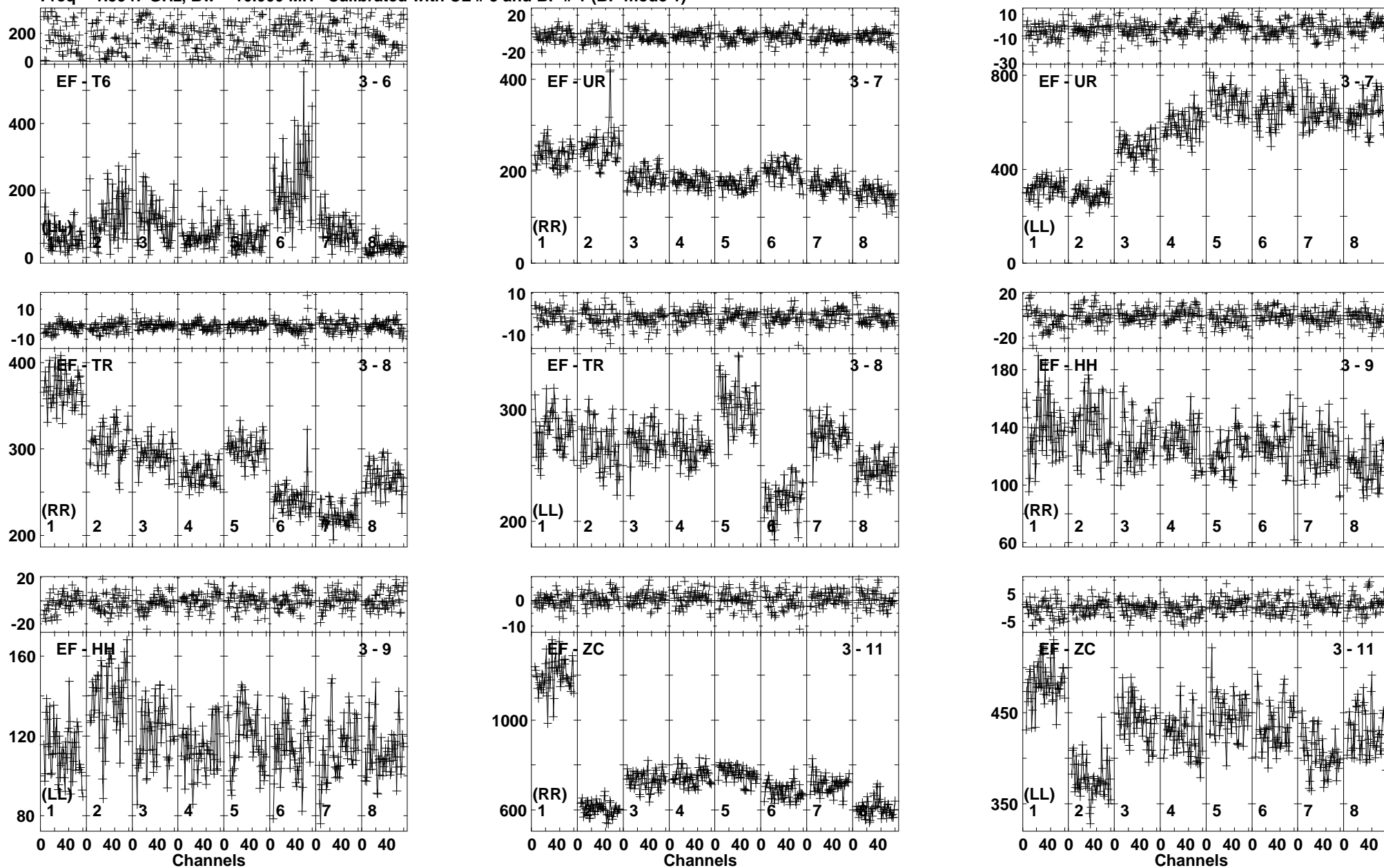
Lower frame: Milli Ampl Jy Top frame: Phas deg Vector averaged cross-power spectrum Baseline: EF (03) - T6 (06) Timerange: 00/09:06:01 to 00/09:07:29
