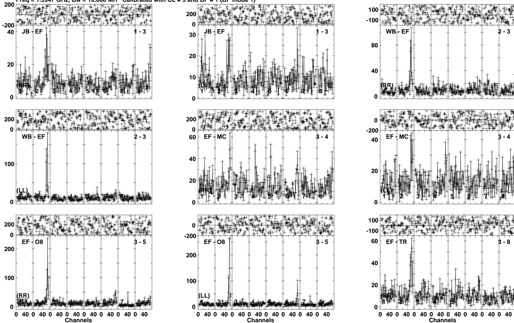
Lower frame: Milli Ampl Jy Top frame: Phas deg Vector averaged cross-power spectrum Baseline: JB (01) - EF (03) Timerange: 00/13:36:31 to 00/13:41:29
