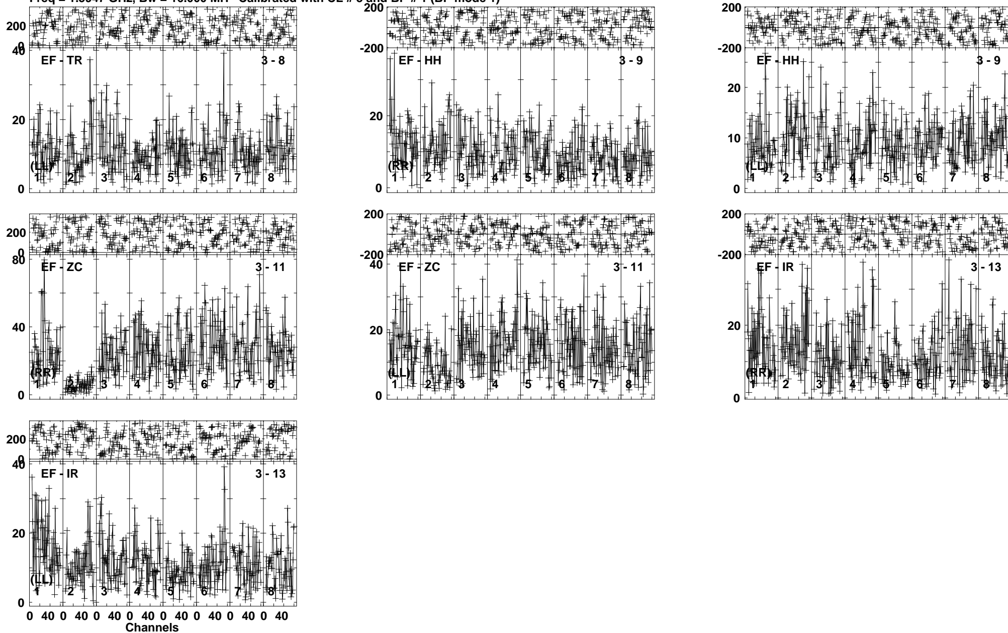
Lower frame: Milli Ampl Jy Top frame: Phas deg Vector averaged cross-power spectrum Baseline: EF (03) - TR (08) Timerange: 00:12:27:46 to 00:12:32:44
