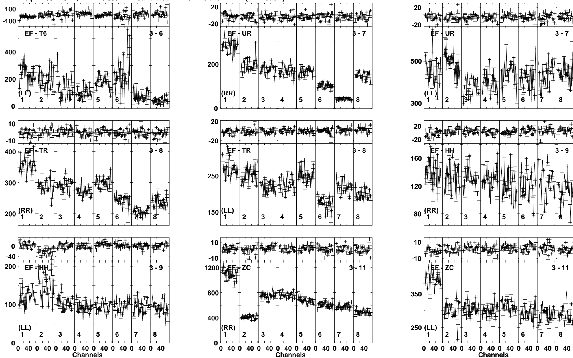
Lower frame: Milli Ampl Jy Top frame: Phas deg Vector averaged cross-power spectrum Baseline: EF (03) - T6 (06) Timerange: 00/08:58:46 to 00/09:00:14
