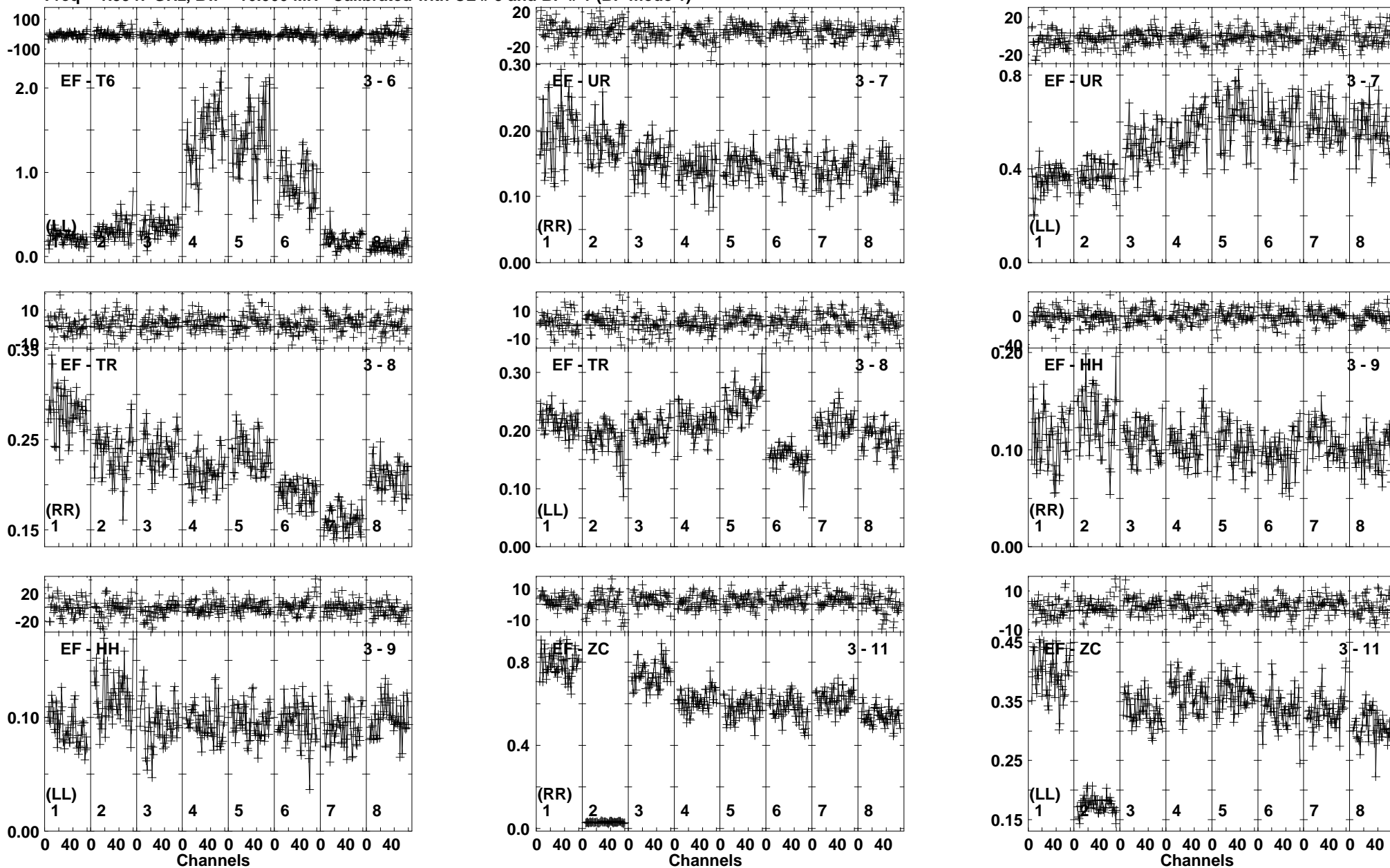
Lower frame: Ampl Jy Top frame: Phas deg Vector averaged cross-power spectrum Baseline: EF (03) - T6 (06) Timerange: 00/08:17:01 to 00/08:18:59
