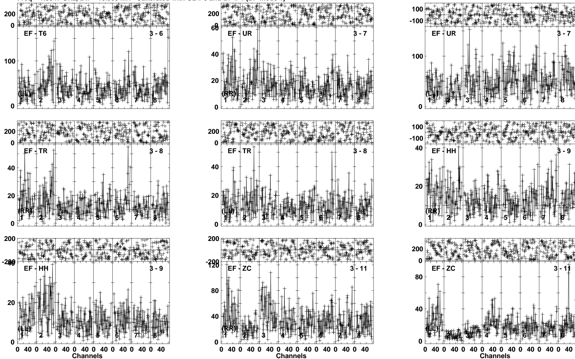
Lower frame: Milli Ampl Jy Top frame: Phas deg Vector averaged cross-power spectrum Baseline: EF (03) - T6 (06) Timerange: 00/08:26:16 to 00/08:31:14
