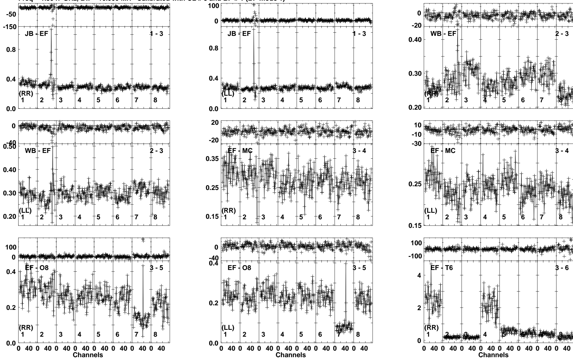
Lower frame: Ampl Jy Top frame: Phas deg Vector averaged cross-power spectrum Baseline: JB (01) - EF (03) Timerange: 00/08:31:16 to 00/08:32:44
