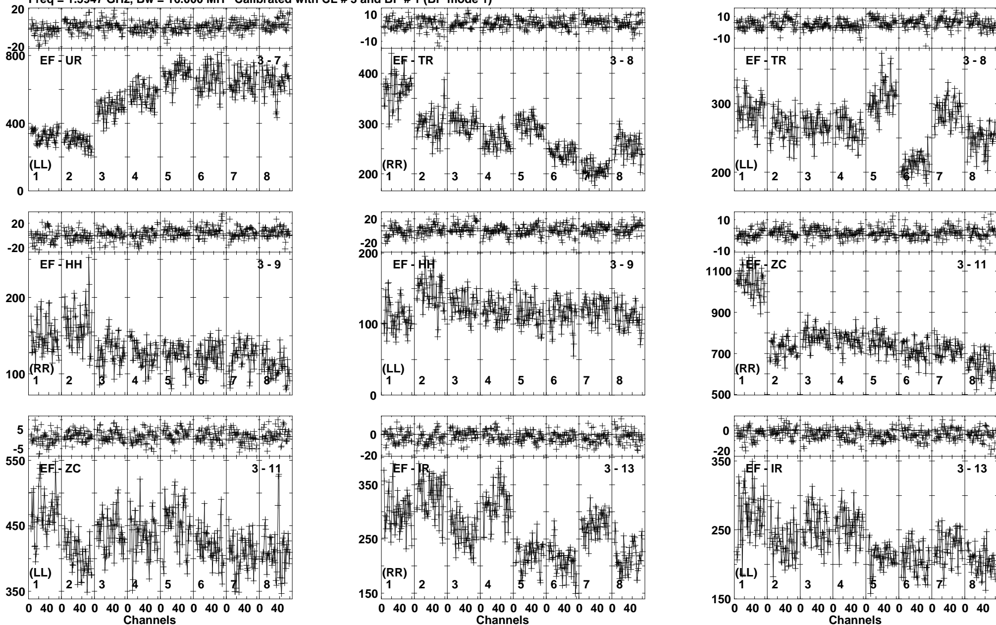
Lower frame: Milli Ampl Jy Top frame: Phas deg Vector averaged cross-power spectrum Baseline: EF (03) - UR (07) Timerange: 00/09:12:31 to 00/09:13:59
