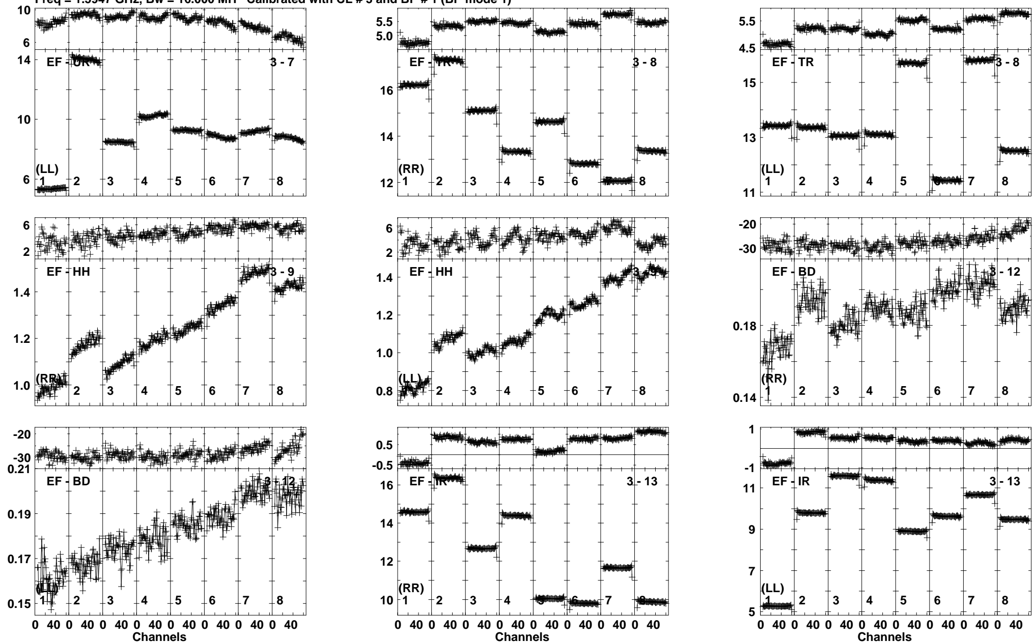
Lower frame: Ampl Jy Top frame: Phas deg Vector averaged cross-power spectrum Baseline: EF (03) - UR (07) Timerange: 00/08:08:01 to 00/08:11:59
