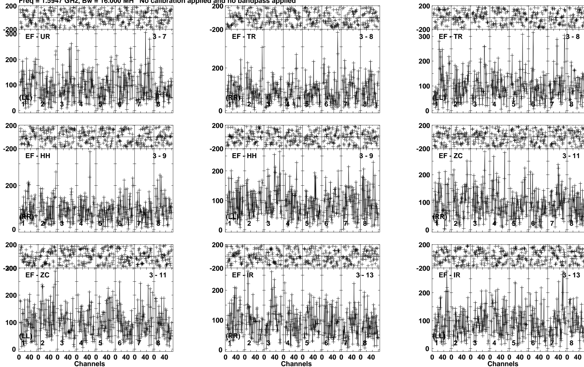
Lower frame: Micro Ampl Jy Top frame: Phas deg Vector averaged cross-power spectrum Baseline: EF (03) - UR (07) Timerange: 00/11:05:16 to 00/11:10:14
