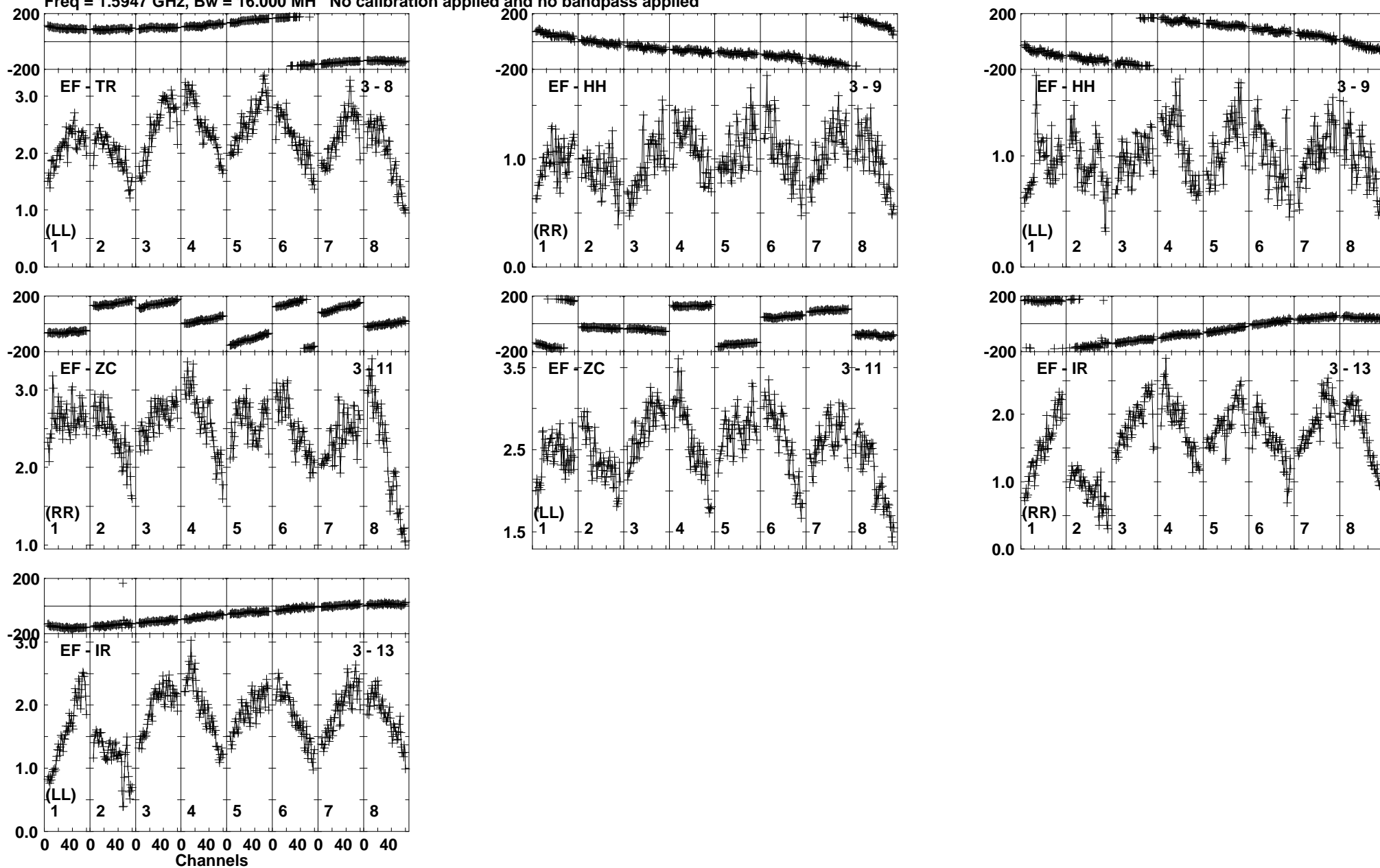
Lower frame: Milli Ampl Jy Top frame: Phas deg Vector averaged cross-power spectrum Baseline: EF (03) - TR (08) Timerange: 00/13:07:31 to 00/13:08:59
