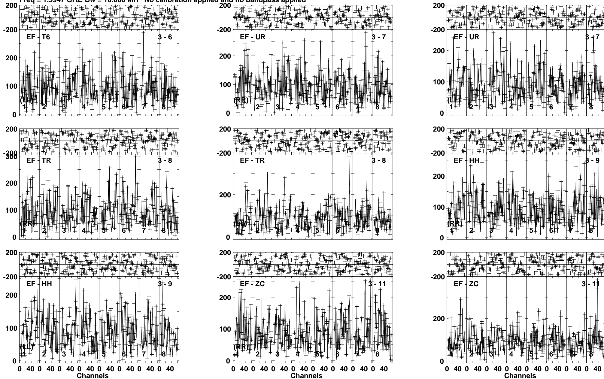
Lower frame: Micro Ampl Jy Top frame: Phas deg Vector averaged cross-power spectrum Baseline: EF (03) - T6 (06) Timerange: 00/08:26:16 to 00/08:31:14
