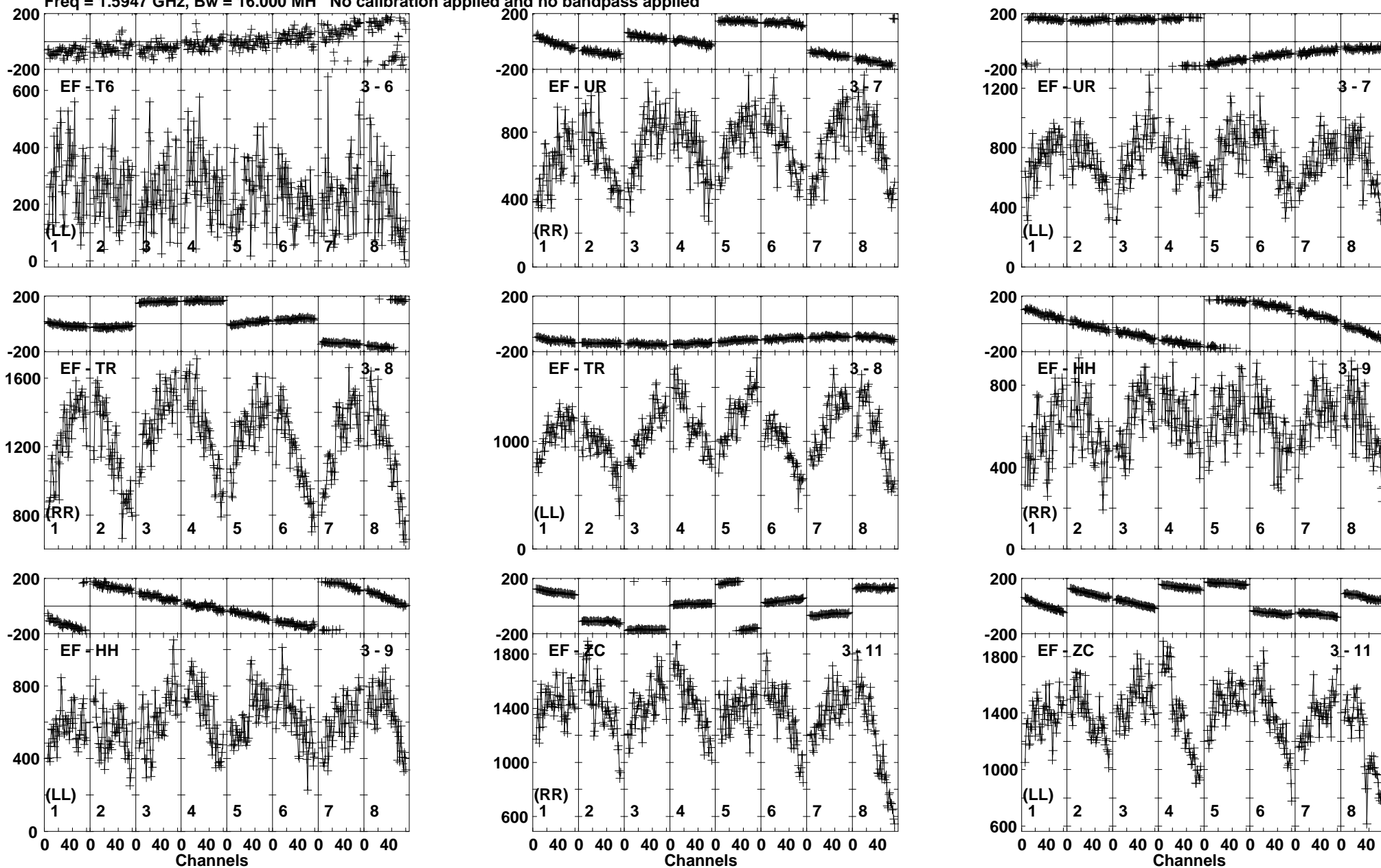
Lower frame: Micro Ampl Jy Top frame: Phas deg Vector averaged cross-power spectrum Baseline: EF (03) - T6 (06) Timerange: 00/08:17:01 to 00/08:18:59
