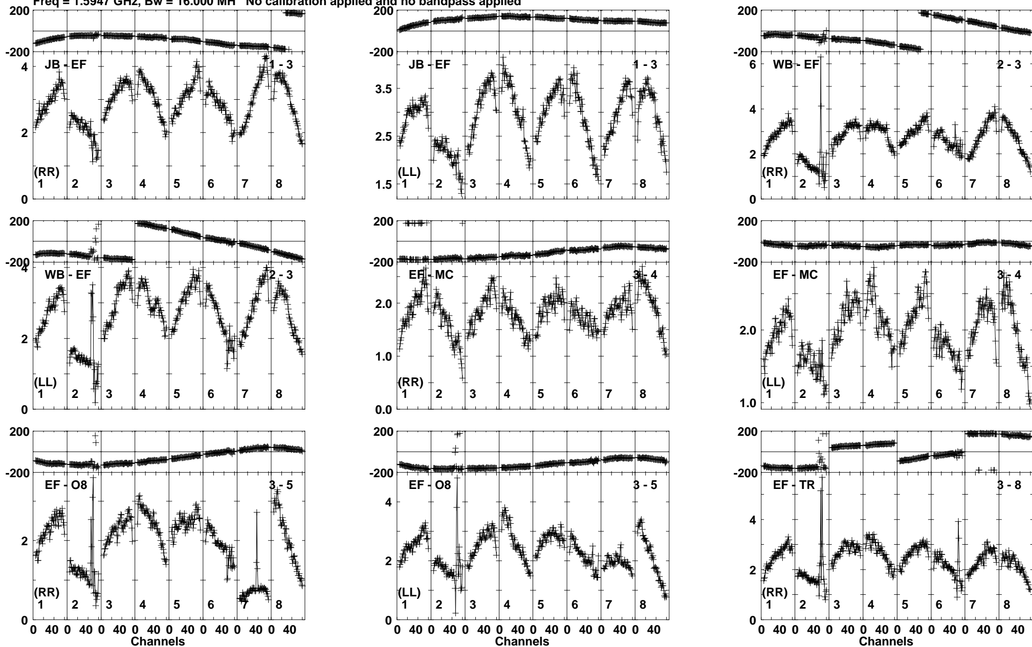
Lower frame: Milli Ampl Jy Top frame: Phas deg Vector averaged cross-power spectrum Baseline: JB (01) - EF (03) Timerange: 00/13:42:16 to 00/13:43:44
