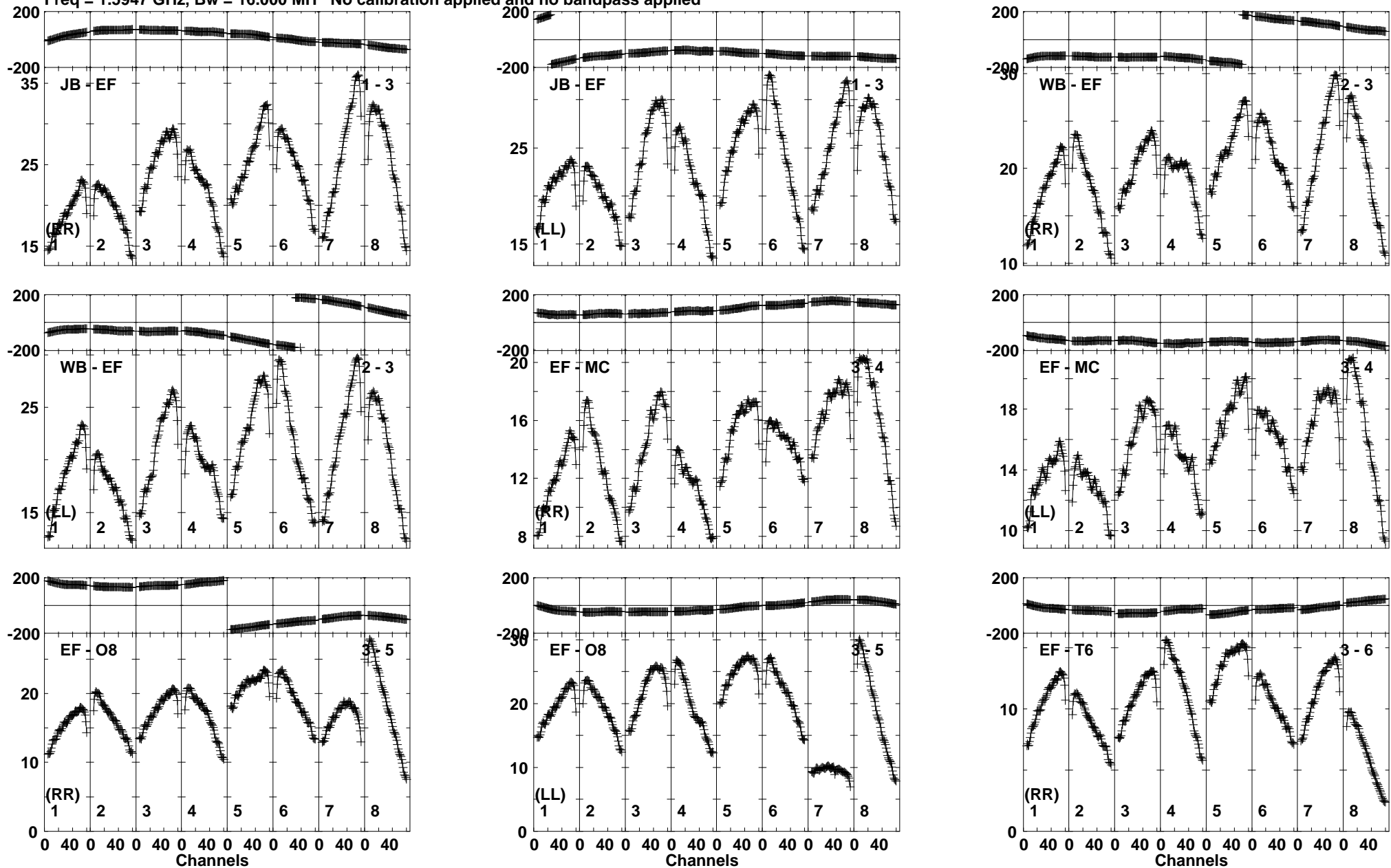
Lower frame: Milli Ampl Jy Top frame: Phas deg Vector averaged cross-power spectrum Baseline: JB (01) - EF (03) Timerange: 00/10:53:46 to 00/10:59:44
