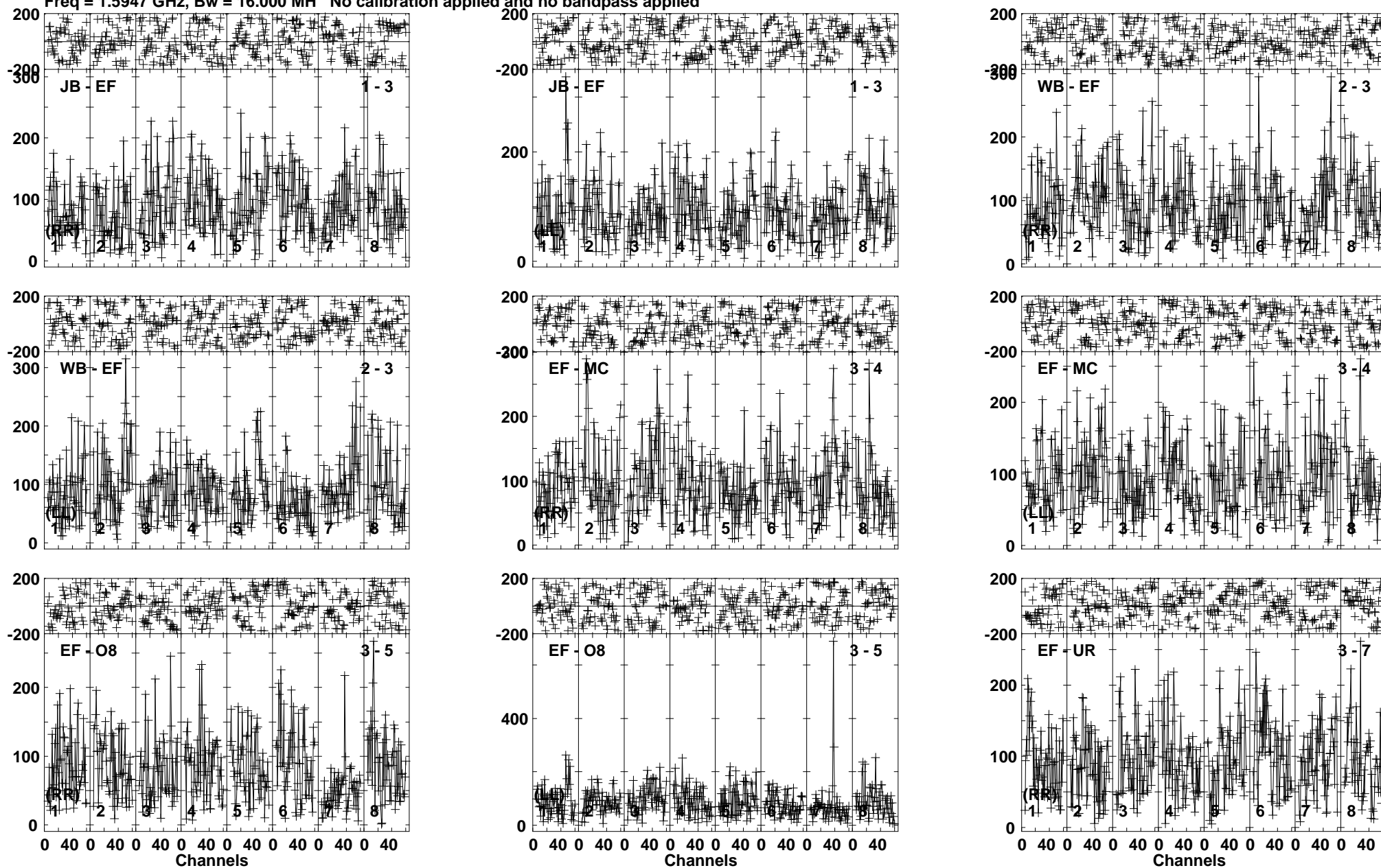
Lower frame: Micro Ampl Jy Top frame: Phas deg Vector averaged cross-power spectrum Baseline: JB (01) - EF (03) Timerange: 00/09:48:46 to 00/09:53:44
