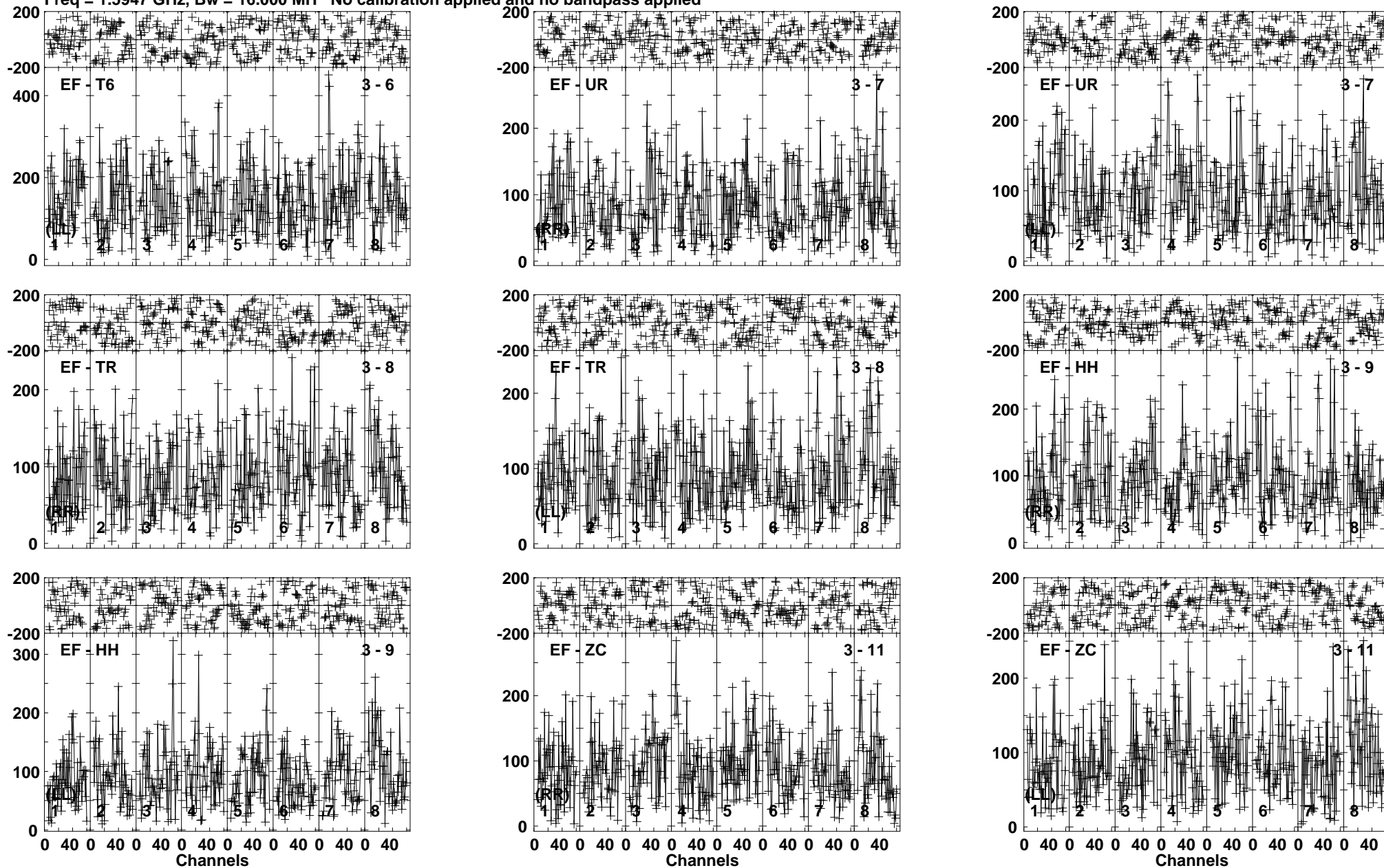
Lower frame: Micro Ampl Jy Top frame: Phas deg Vector averaged cross-power spectrum Baseline: EF (03) - T6 (06) Timerange: 00/08:19:01 to 00/08:23:59
