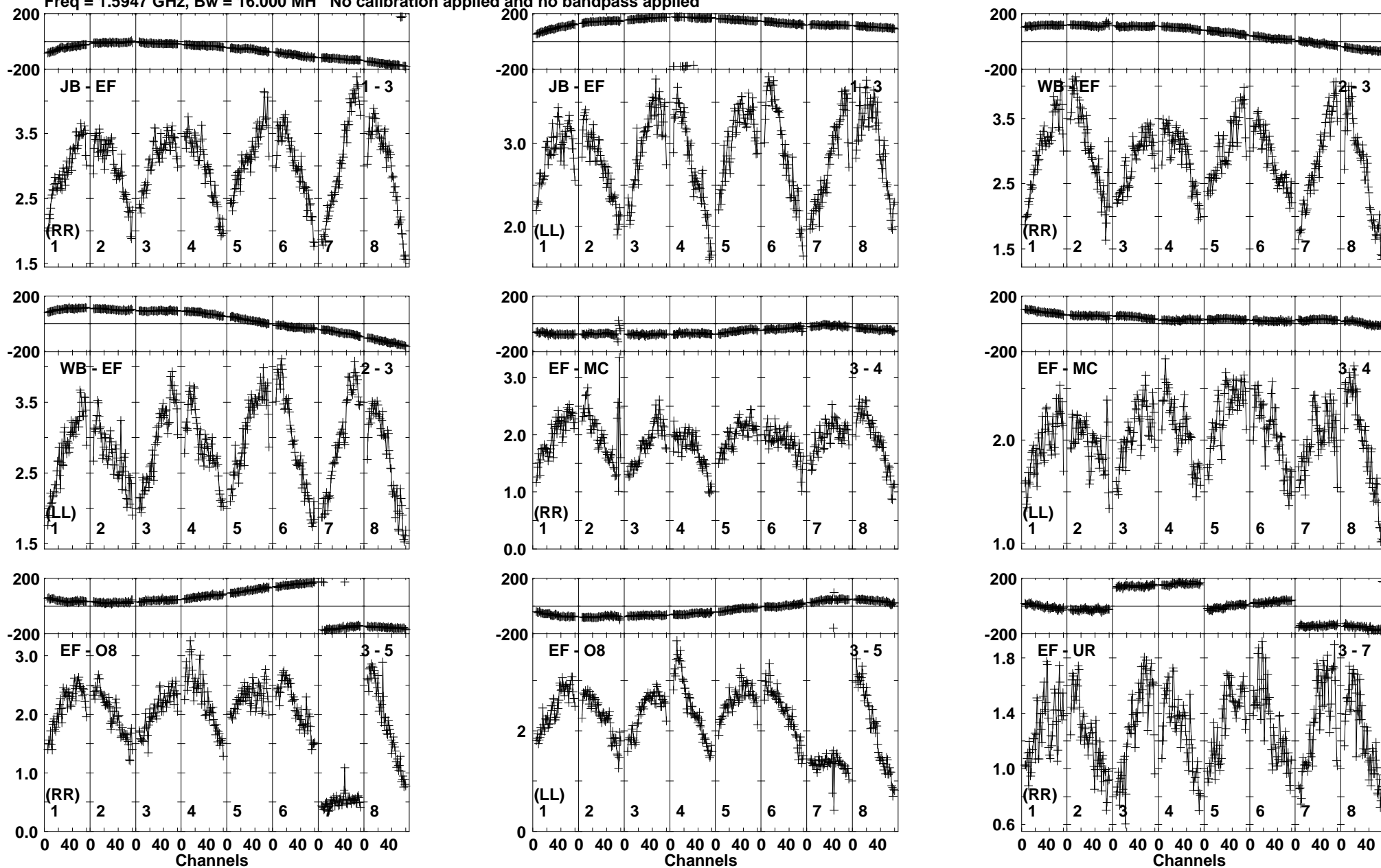
Lower frame: Milli Ampl Jy Top frame: Phas deg Vector averaged cross-power spectrum Baseline: JB (01) - EF (03) Timerange: 00/10:21:16 to 00/10:22:44
