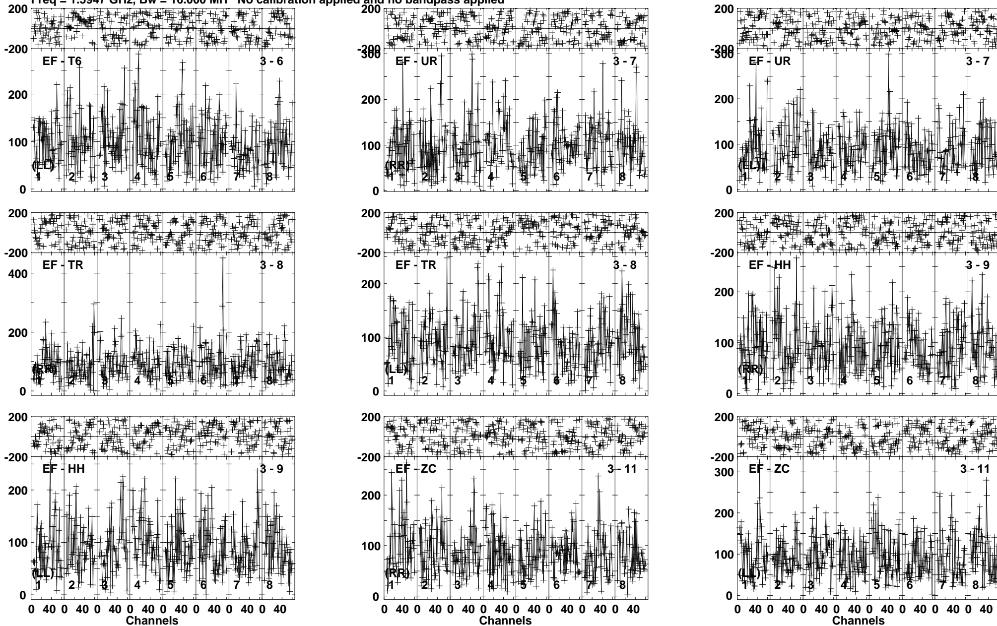
Lower frame: Micro Ampl Jy Top frame: Phas deg Vector averaged cross-power spectrum Baseline: EF (03) - T6 (06) Timerange: 00/08:32:46 to 00/08:37:44
