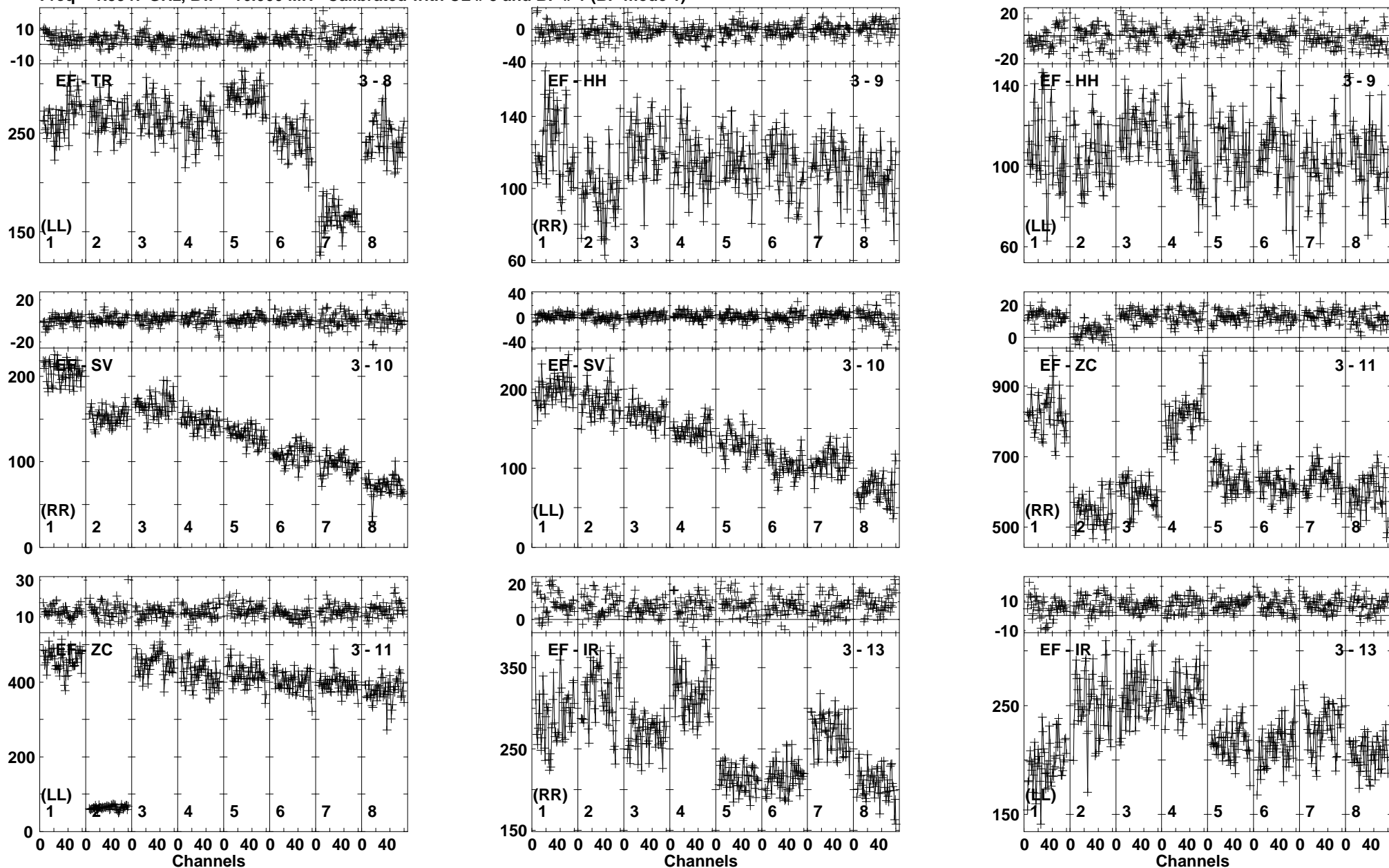
Lower frame: Milli Ampl Jy Top frame: Phas deg Vector averaged cross-power spectrum Baseline: EF (03) - TR (08) Timerange: 00/11:17:31 to 00/11:18:59
