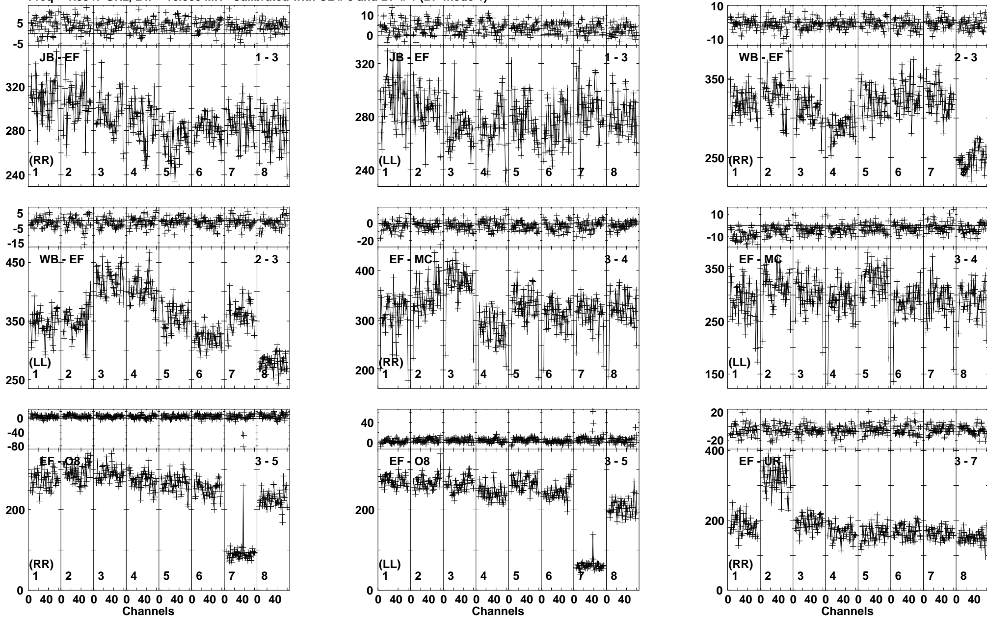
Lower frame: Milli Ampl Jy Top frame: Phas deg Vector averaged cross-power spectrum Baseline: JB (01) - EF (03) Timerange: 00/09/53:46 to 00/09/55:14
