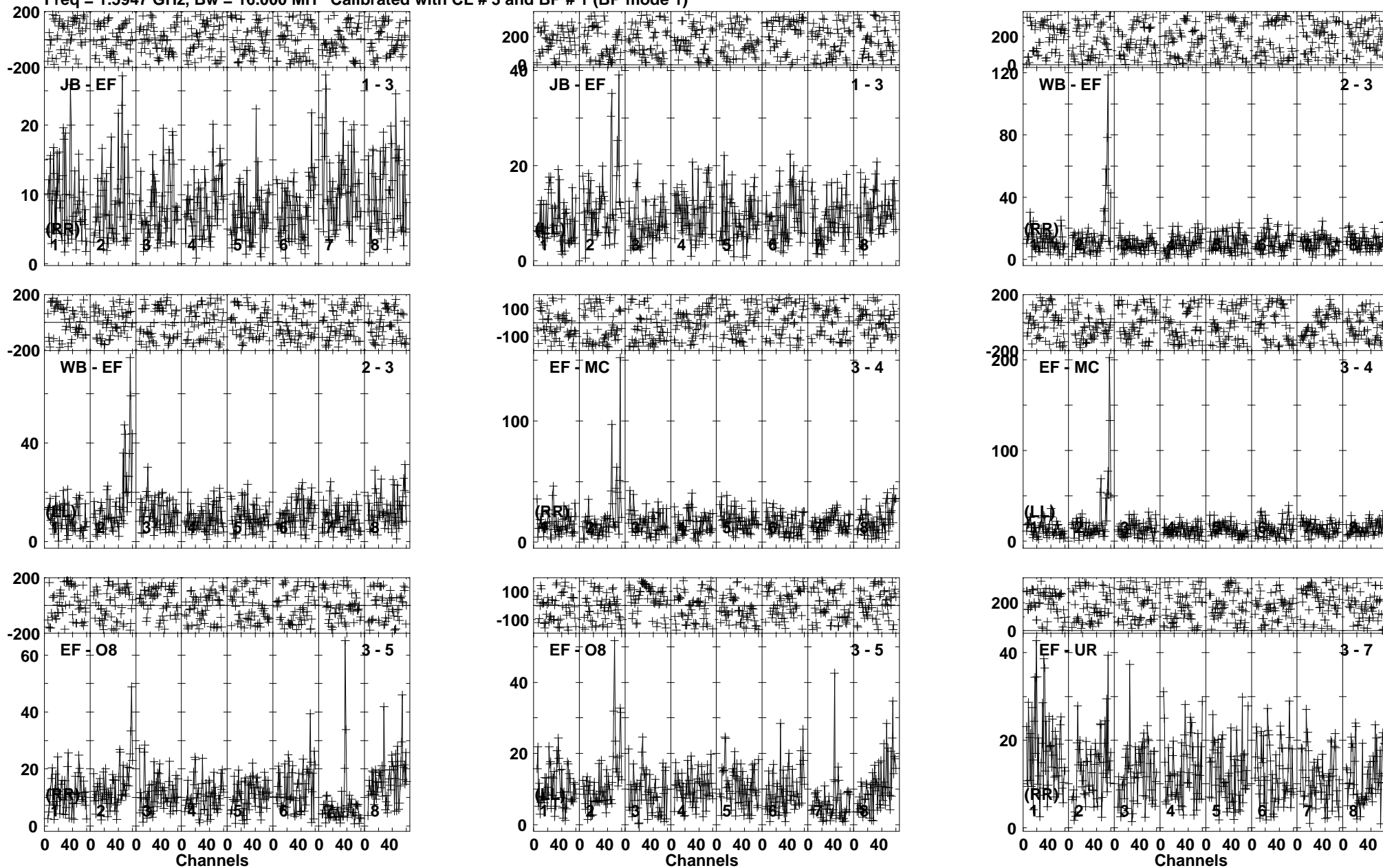
Lower frame: Milli Ampl Jy Top frame: Phas deg Vector averaged cross-power spectrum Baseline: JB (01) - EF (03) Timerange: 00/10:22:46 to 00/10:27:44
