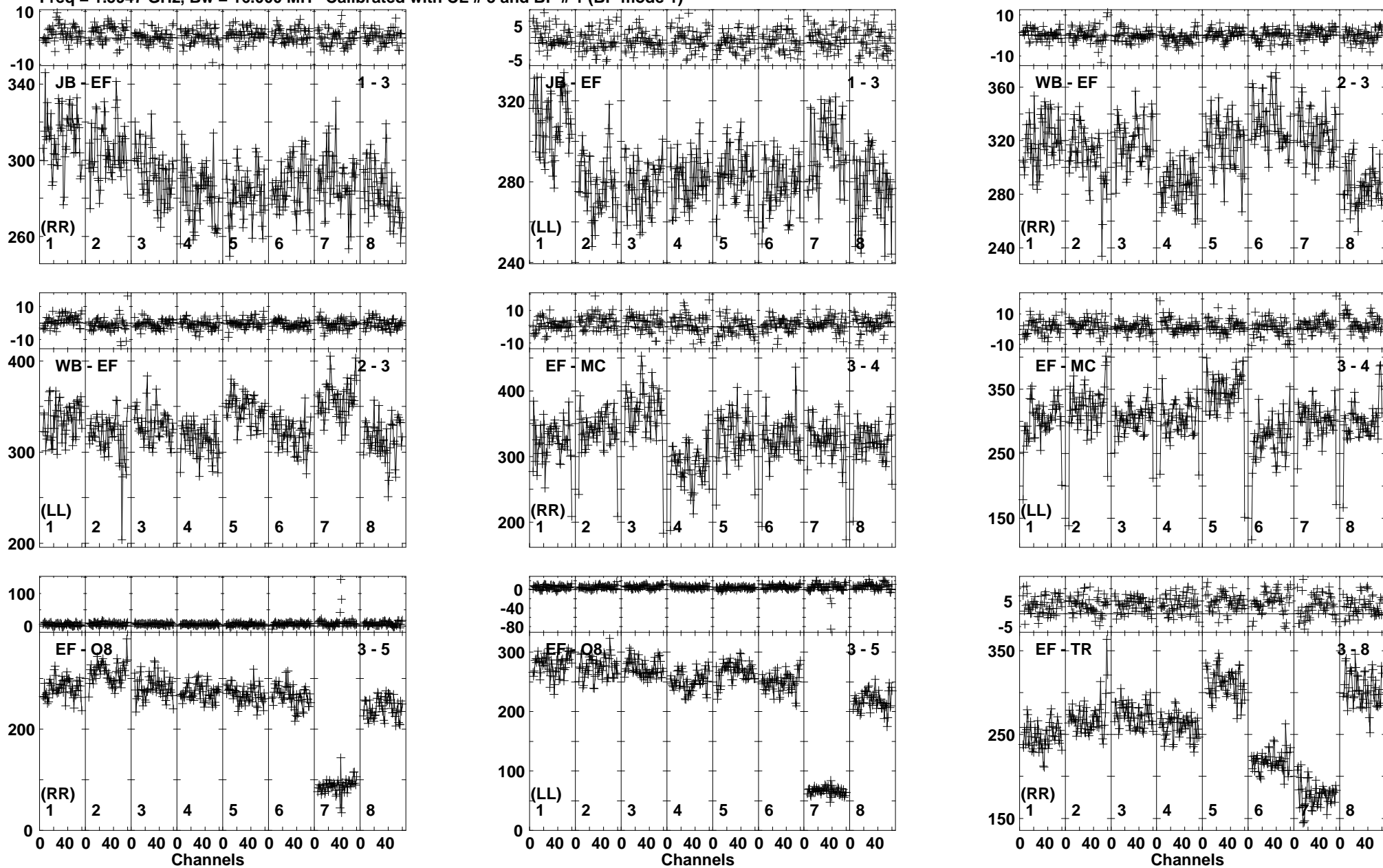
Lower frame: Milli Ampl Jy Top frame: Phas deg Vector averaged cross-power spectrum Baseline: JB (01) - EF (03) Timerange: 00/11:17:31 to 00/11:18:59
