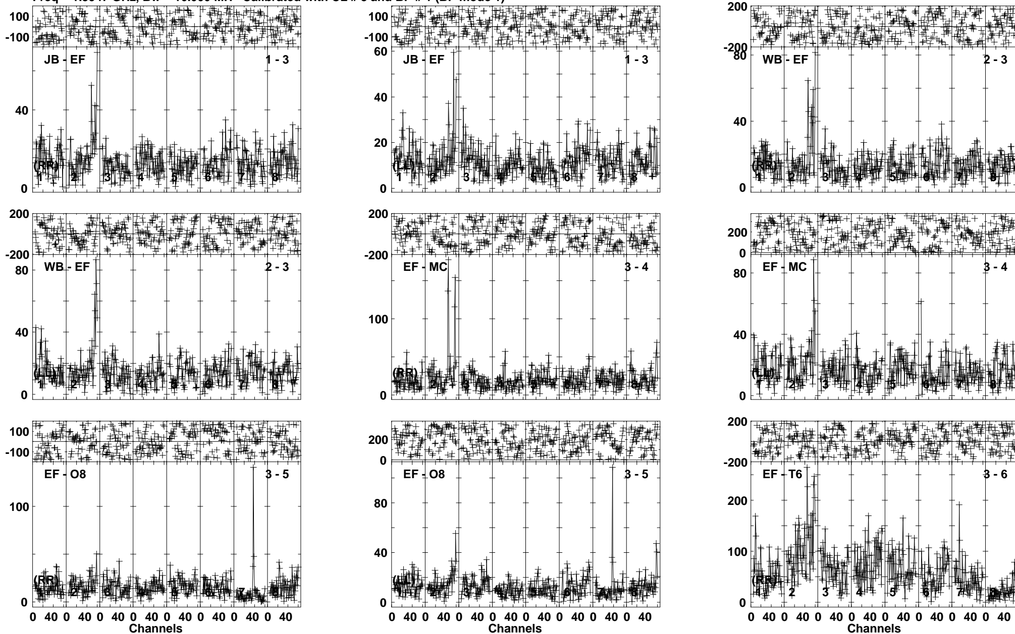
Lower frame: Milli Ampl Jy Top frame: Phas deg Vector averaged cross-power spectrum Baseline: JB (01) - EF (03) Timerange: 00/08:26:16 to 00/08:31:14
