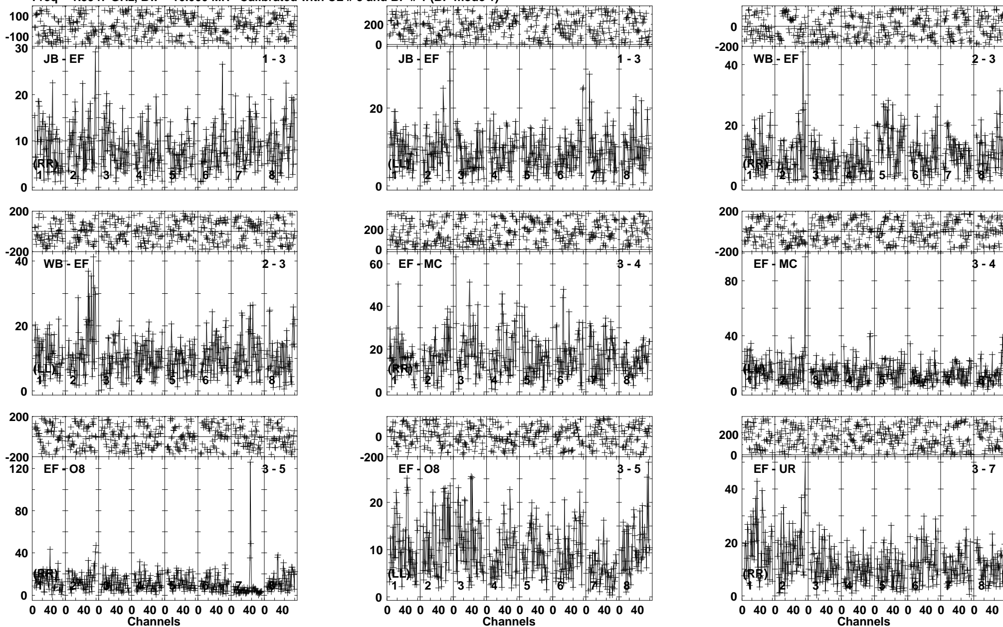
Lower frame: Milli Ampl Jy Top frame: Phas deg Vector averaged cross-power spectrum Baseline: JB (01) - EF (03) Timerange: 00/10:30:01 to 00/10:34:59
