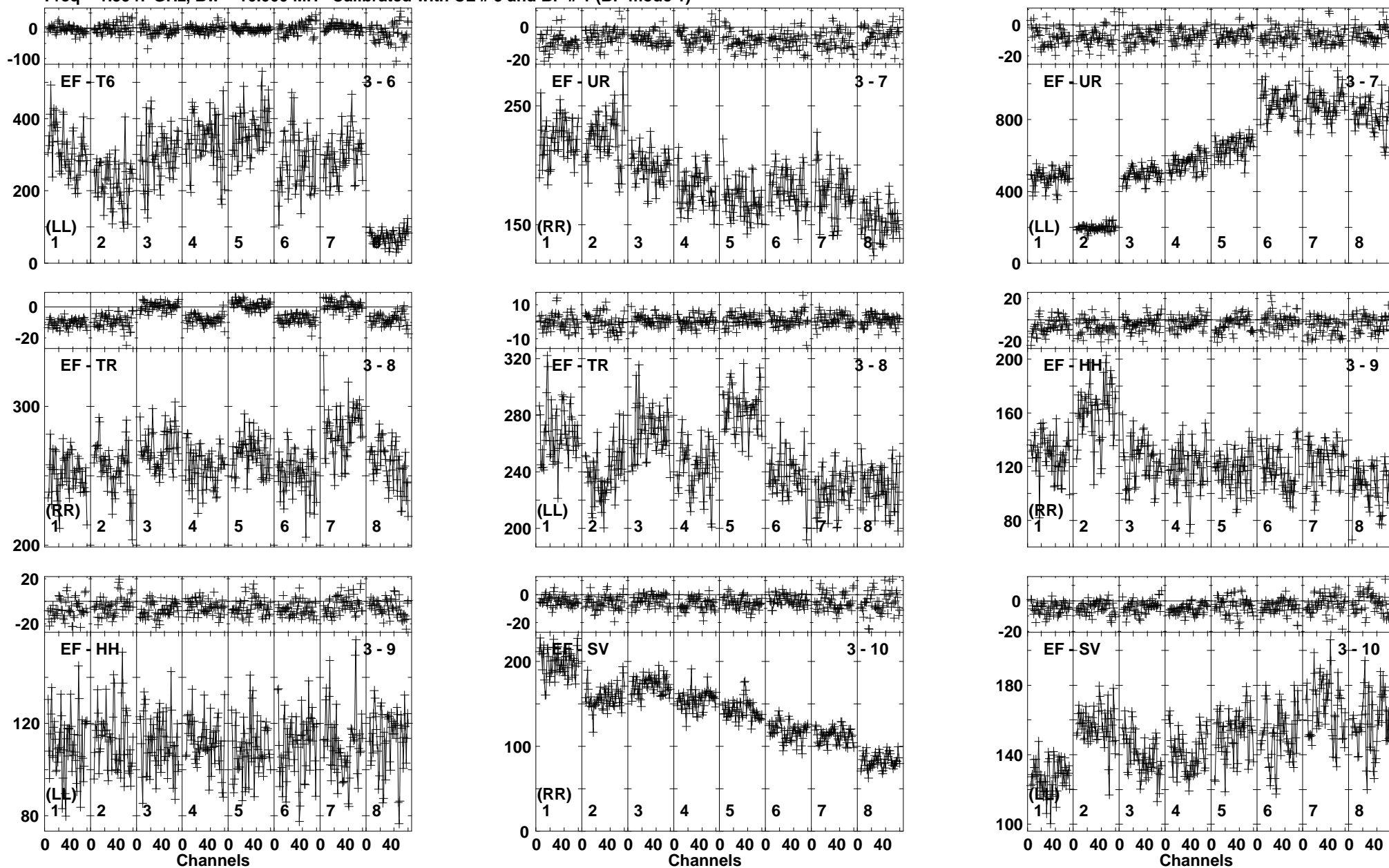
Lower frame: Milli Ampl Jy Top frame: Phas deg Vector averaged cross-power spectrum Baseline: EF (03) - T6 (06) Timerange: 00/08:52:16 to 00/08:53:44
