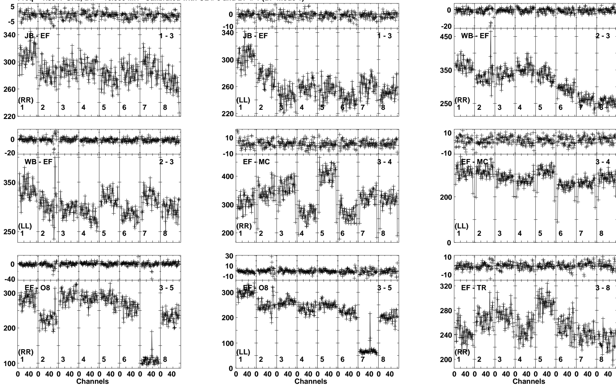
Lower frame: Milli Amp Jy Top frame: Phas deg Vector averaged cross-power spectrum Baseline: JB (01) - EF (03) Timerange: 00/13:28:31 to 00/13:29:59
