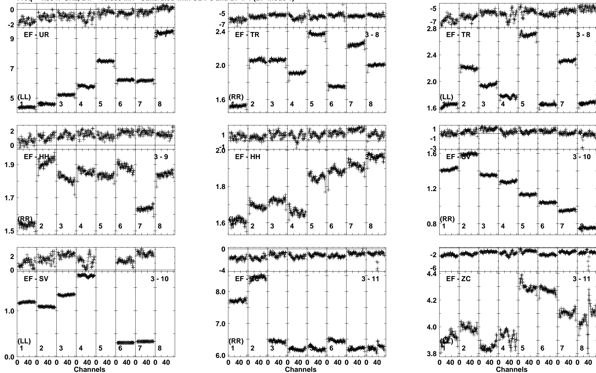
Lower frame: Ampl Jy Top frame: Phas deg Vector averaged cross-power spectrum Baseline: EF (03) - UR (07) Timerange: 00/13:53:56 to 00/13:59:54
