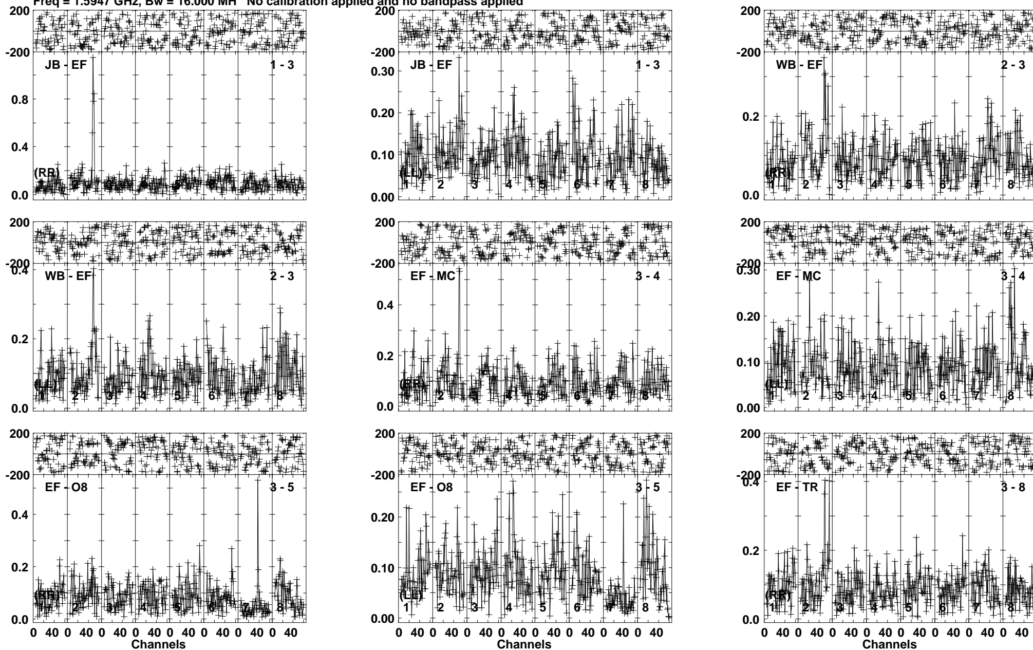
Lower frame: Milli Ampl Jy Top frame: Phas deg Vector averaged cross-power spectrum Baseline: JB (01) - EF (03) Timerange: 00:12:21:16 to 00:12:26:14
