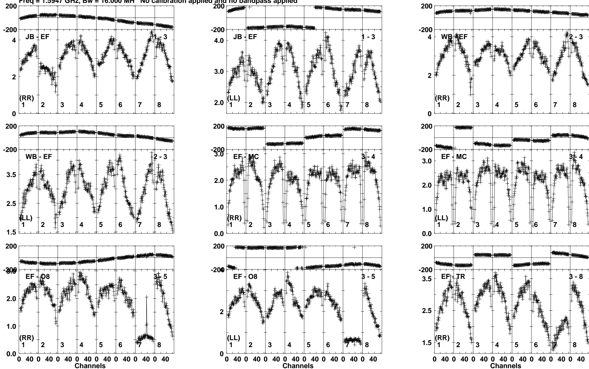
Lower frame: Milli Ampl Jy Top frame: Phas deg Vector averaged cross-power spectrum Baseline: JB (01) - EF (03) Timerange: 00/11:24:46 to 00/11:26:14
