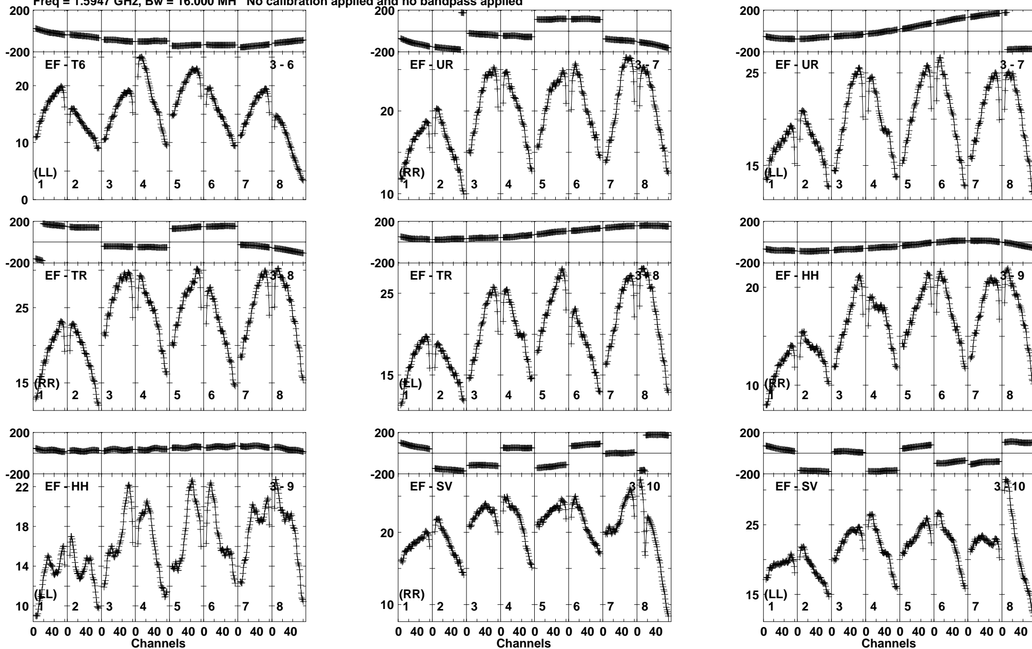
Lower frame: Milli Ampl Jy Top frame: Phas deg Vector averaged cross-power spectrum Baseline: EF (03) - T6 (06) Timerange: 00/10:53:46 to 00/10:59:44
