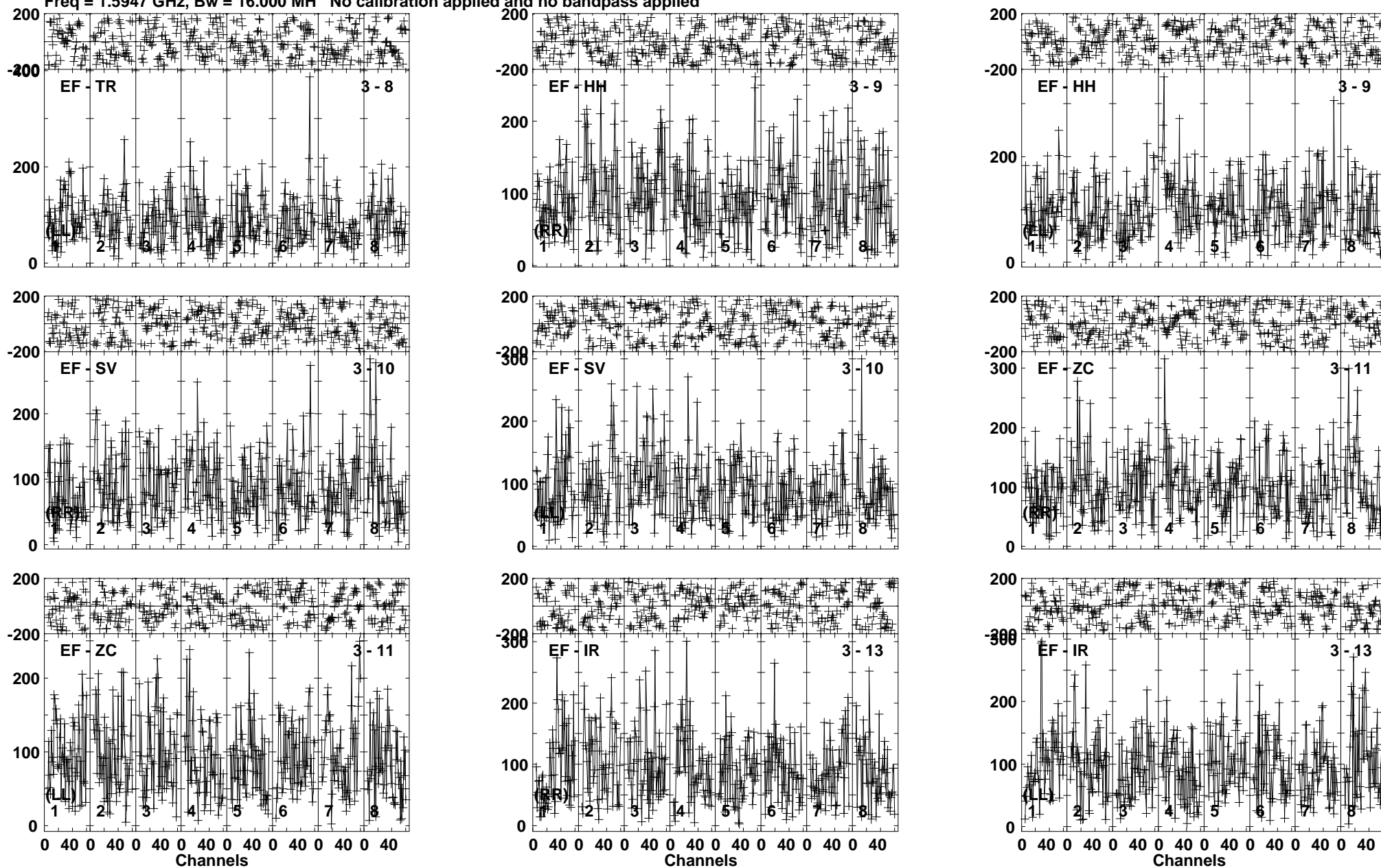
Lower frame: Micro Ampl Jy Top frame: Phas deg Vector averaged cross-power spectrum Baseline: EF (03) - TR (08) Timerange: 00/11:26:16 to 00/11:31:14
