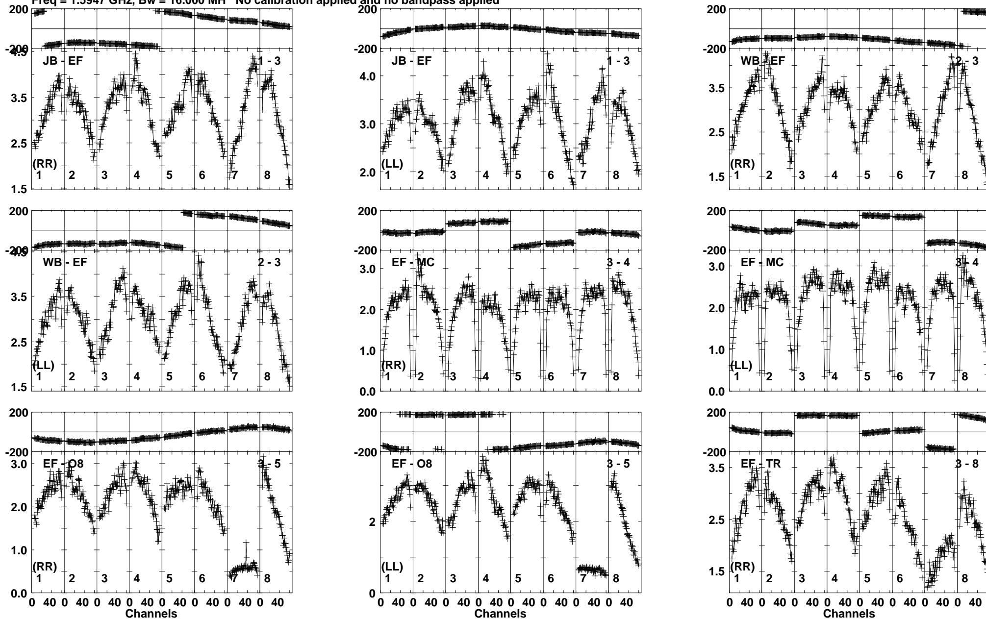
Lower frame: Milli Ampl Jy Top frame: Phas deg Vector averaged cross-power spectrum Baseline: JB (01) - EF (03) Timerange: 00/11:52:16 to 00/11:53:44
