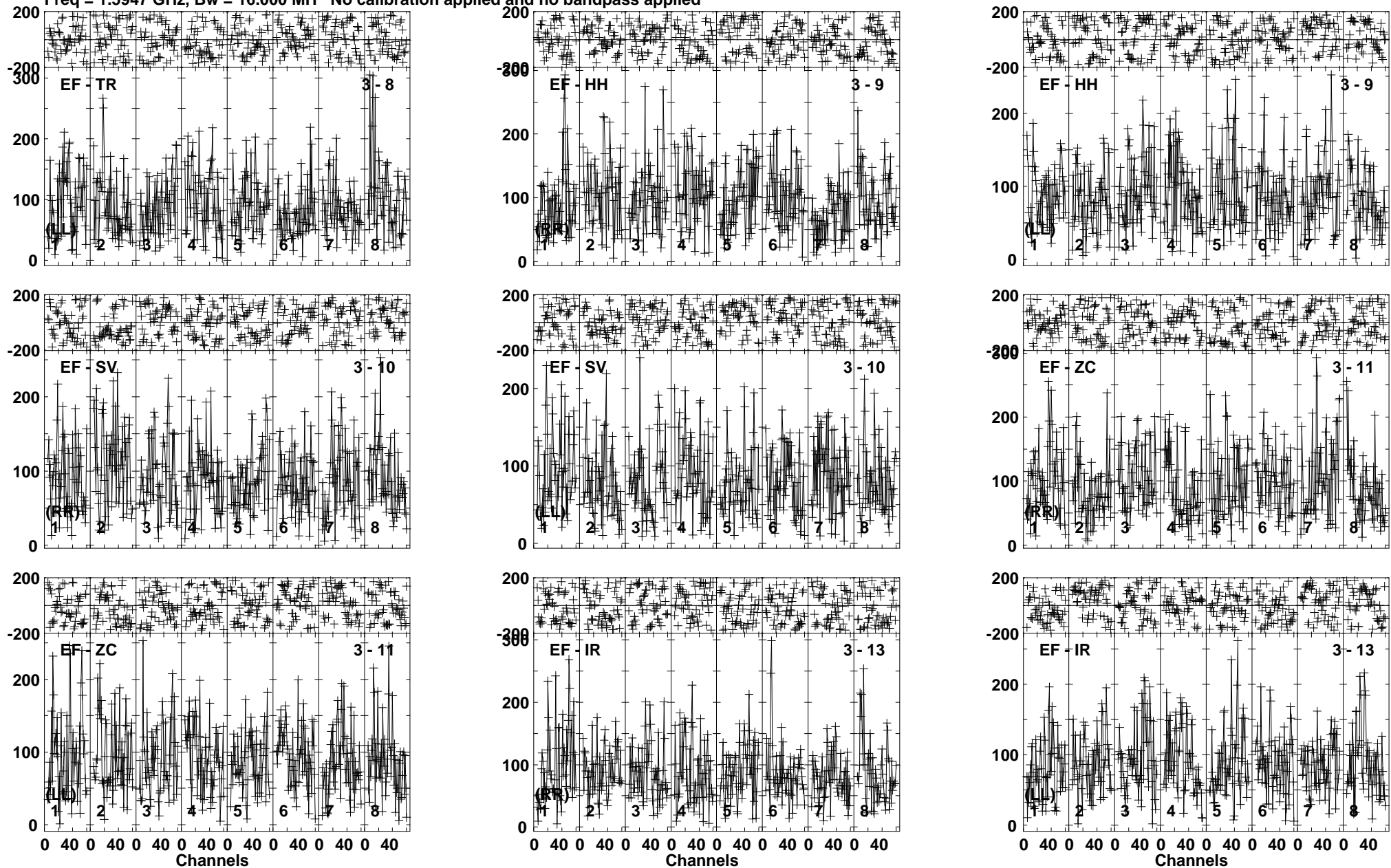
Lower frame: Micro Ampl Jy Top frame: Phas deg Vector averaged cross-power spectrum Baseline: EF (03) - TR (08) Timerange: 00/11:19:01 to 00/11:23:59
