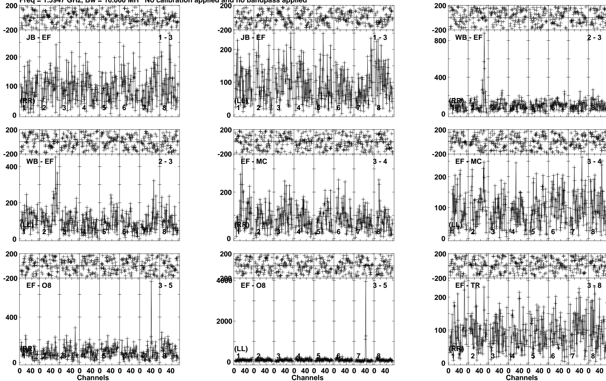
Lower frame: Micro Ampl Jy Top frame: Phas deg Vector averaged cross-power spectrum Baseline: JB (01) - EF (03) Timerange: 00/13:16:16 to 00/13:21:14
