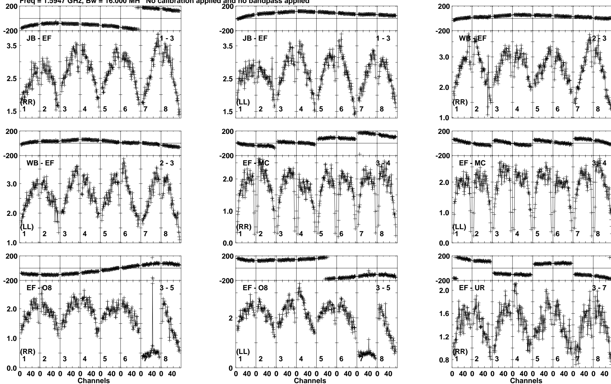
Lower frame: Milli Ampl Jy Top frame: Phas deg Vector averaged cross-power spectrum Baseline: JB (01) - EF (03) Timerange: 00/08:58:48 to 00/09:00:14
