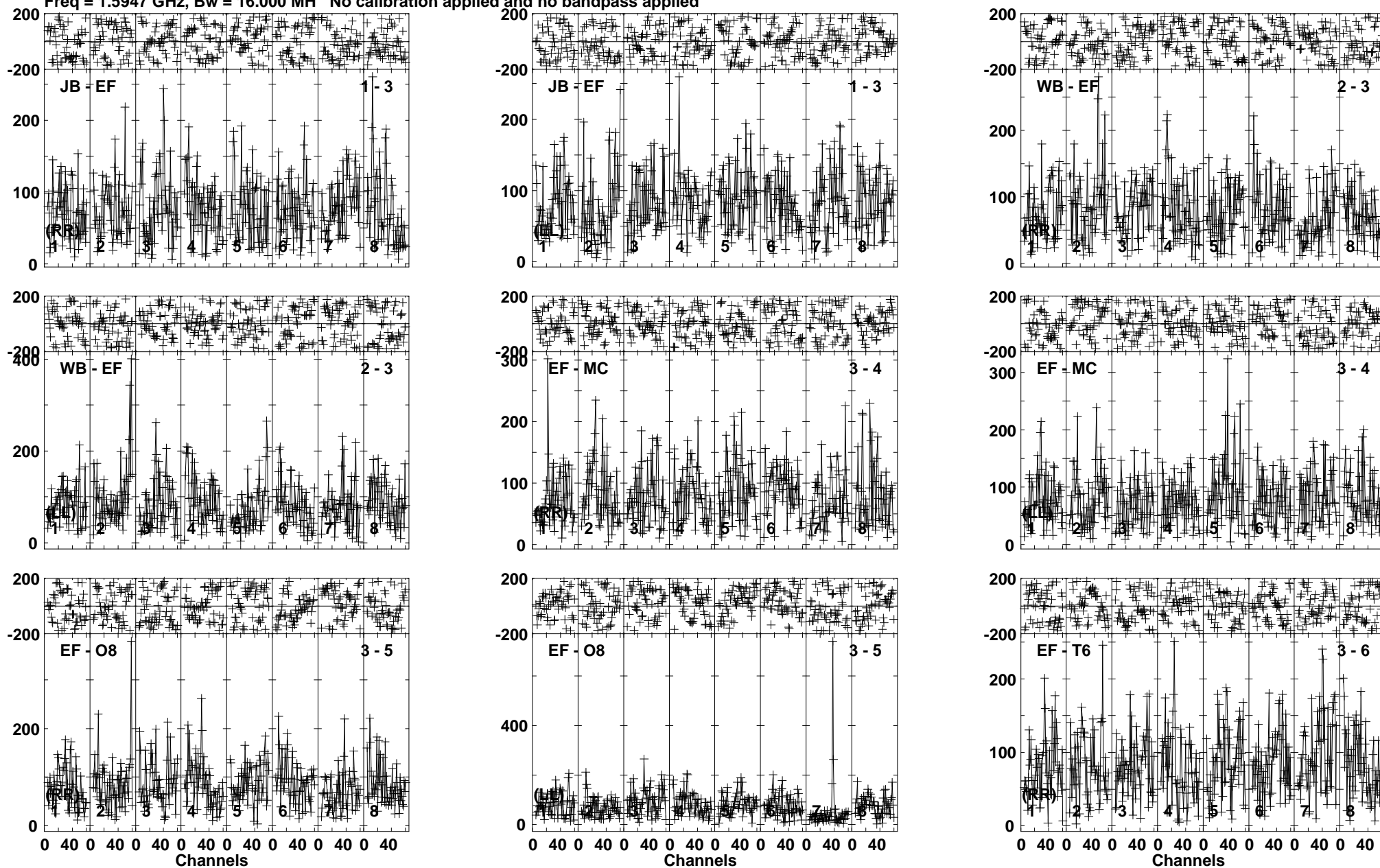
Lower frame: Micro Ampl Jy Top frame: Phas deg Vector averaged cross-power spectrum Baseline: JB (01) - EF (03) Timerange: 00/10:53:46 to 00/10:59:44
