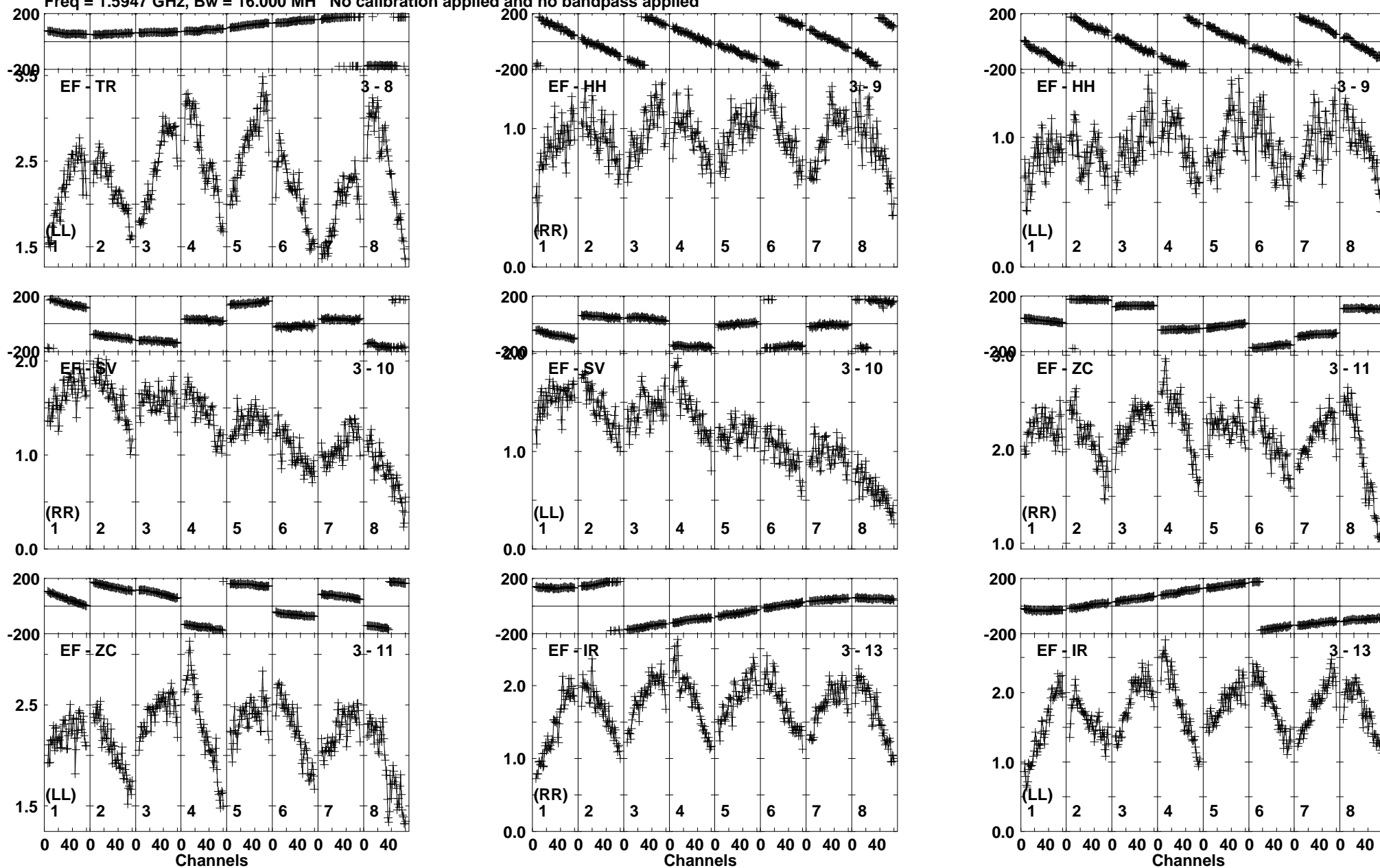
Lower frame: Milli Ampl Jy Top frame: Phas deg Vector averaged cross-power spectrum Baseline: EF (03) - TR (08) Timerange: 00/11:03:16 to 00/11:05:14
