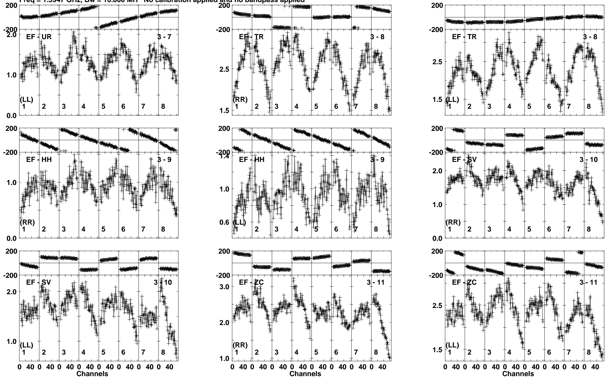
Lower frame: Milli Ampl Jy Top frame: Phas deg Vector averaged cross-power spectrum Baseline: EF (03) - UR (07) Timerange: 00/09:33:31 to 00/09:34:59
