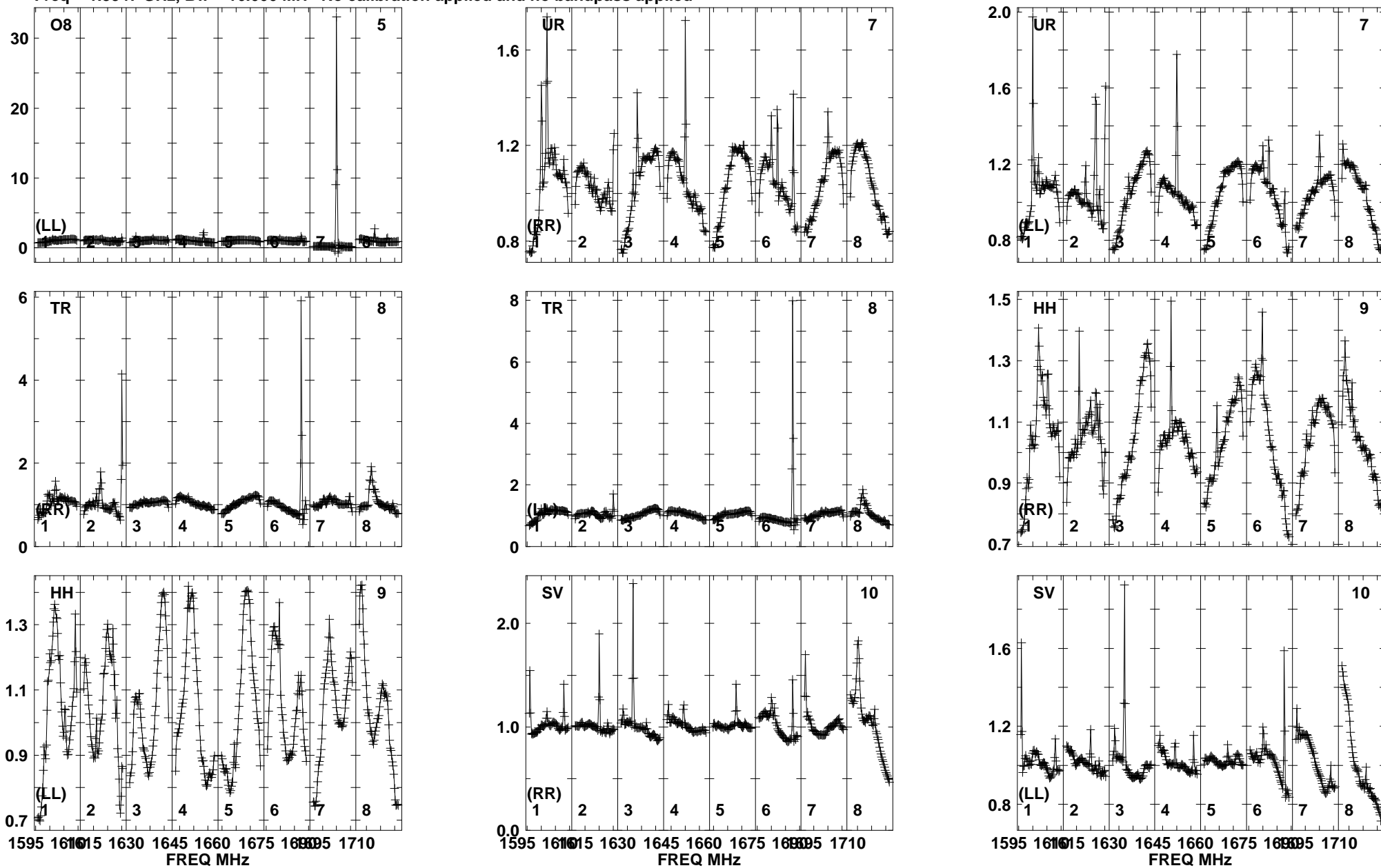
Lower frame: Real Jy Total-power spectrum Antenna: O8 (05) Timerange: 00/09:55:16 to 00/10:00:14
