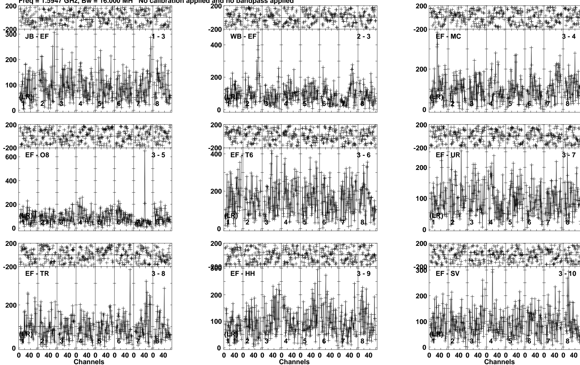
Lower frame: Micro Ampl Jy Top frame: Phas deg Vector averaged cross-power spectrum Baseline: JB (01) - EF (03) Timerange: 00/08:19:01 to 00/08:23:59
