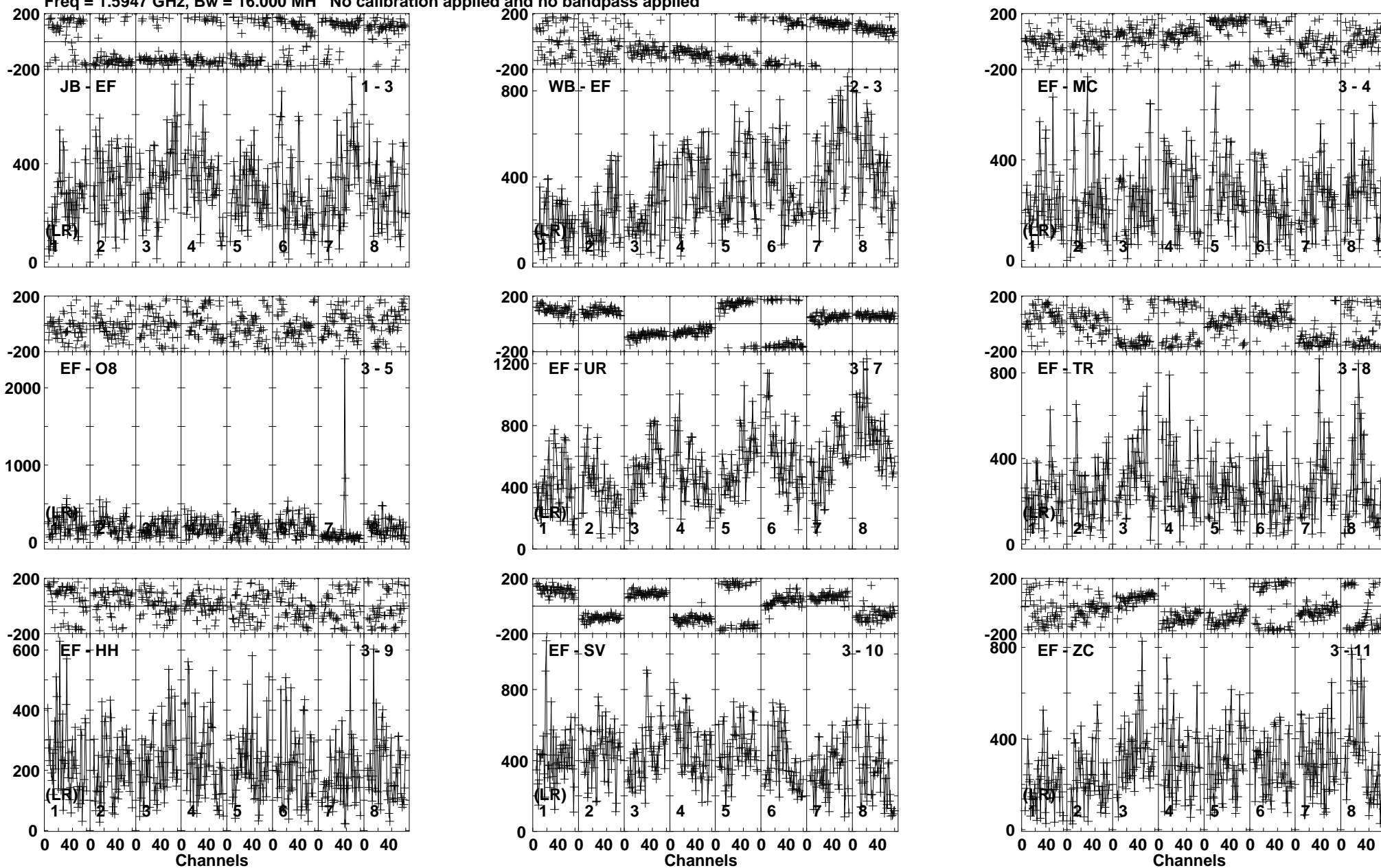
Lower frame: Micro Ampl Jy Top frame: Phas deg Vector averaged cross-power spectrum Baseline: JB (01) - EF (03) Timerange: 00/09:40:01 to 00/09:41:29
