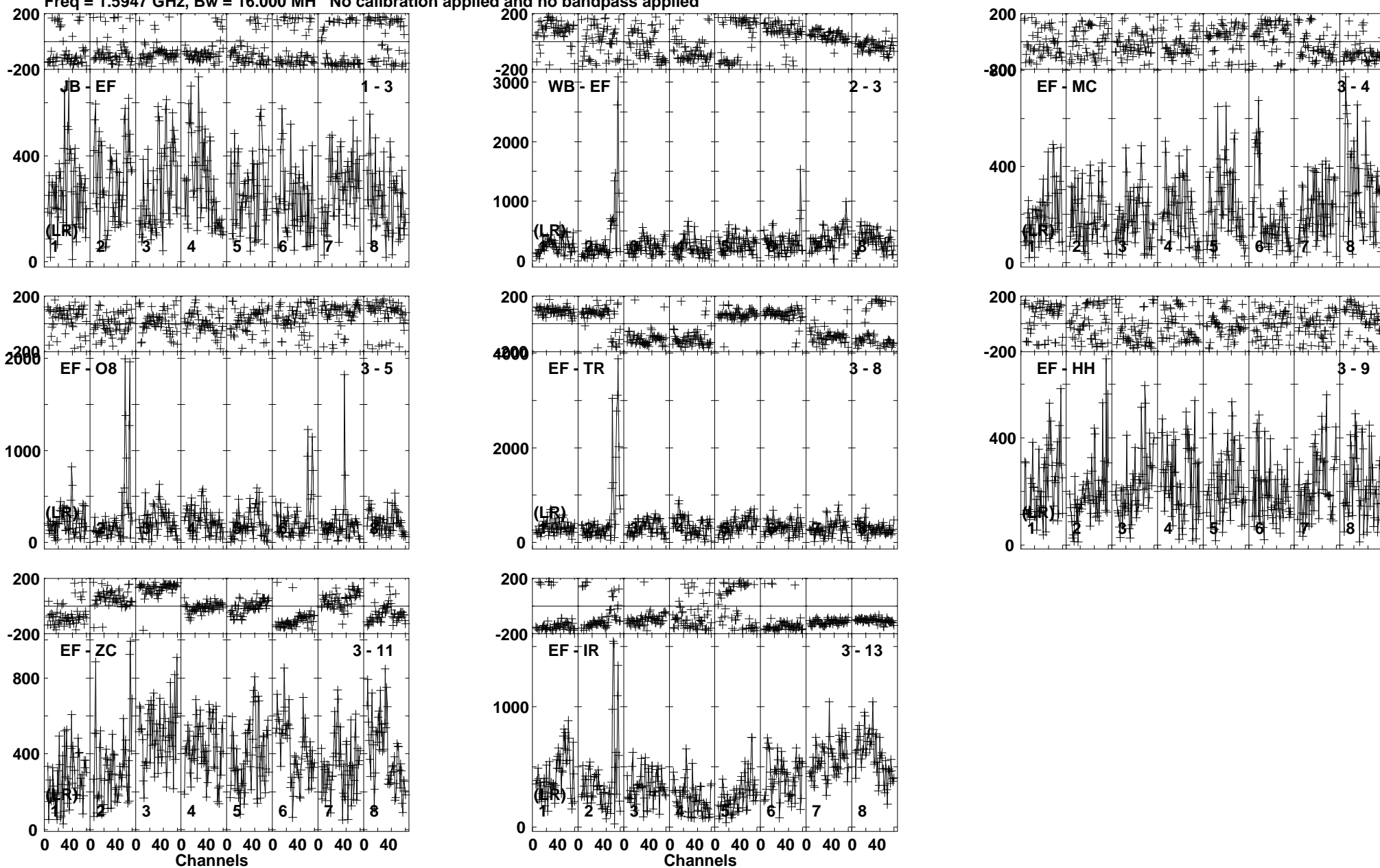
Lower frame: Micro Ampl Jy Top frame: Phas deg Vector averaged cross-power spectrum Baseline: JB (01) - EF (03) Timerange: 00:12:53:46 to 00:12:55:14
