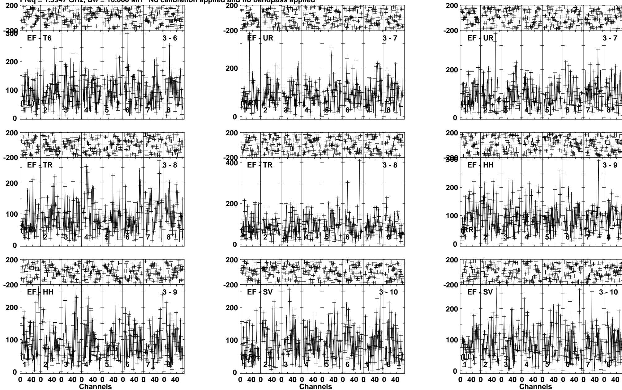
Lower frame: Micro Ampl Jy Top frame: Phas deg Vector averaged cross-power spectrum Baseline: EF (03) - T6 (06) Timerange: 00/08:46:31 to 00/08:51:29
