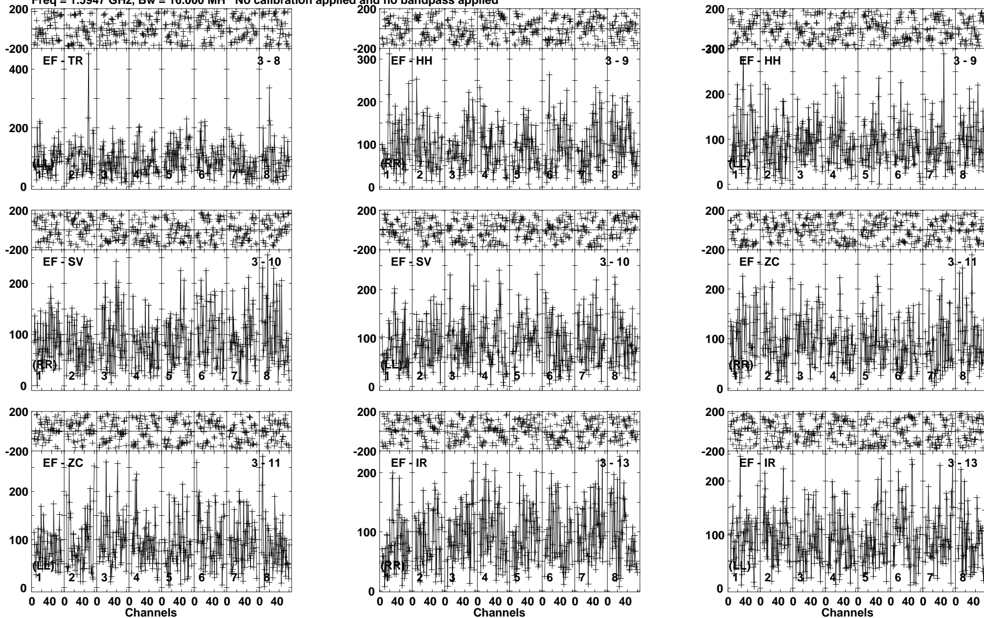
Lower frame: Micro Ampl Jy Top frame: Phas deg Vector averaged cross-power spectrum Baseline: EF (03) - TR (08) Timerange: 00:12:00:16 to 00:12:05:14
