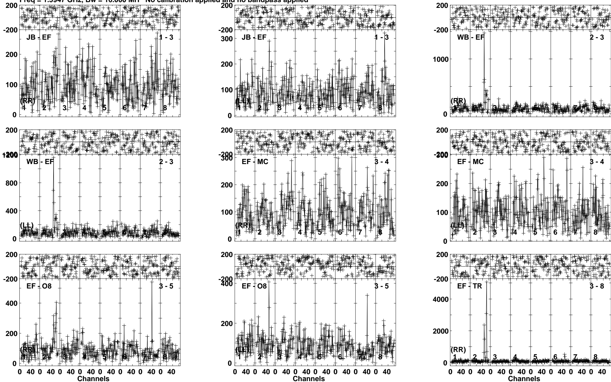
Lower frame: Micro Ampl Jy Top frame: Phas deg Vector averaged cross-power spectrum Baseline: JB (01) - EF (03) Timerange: 00/13:36:31 to 00/13:41:29
