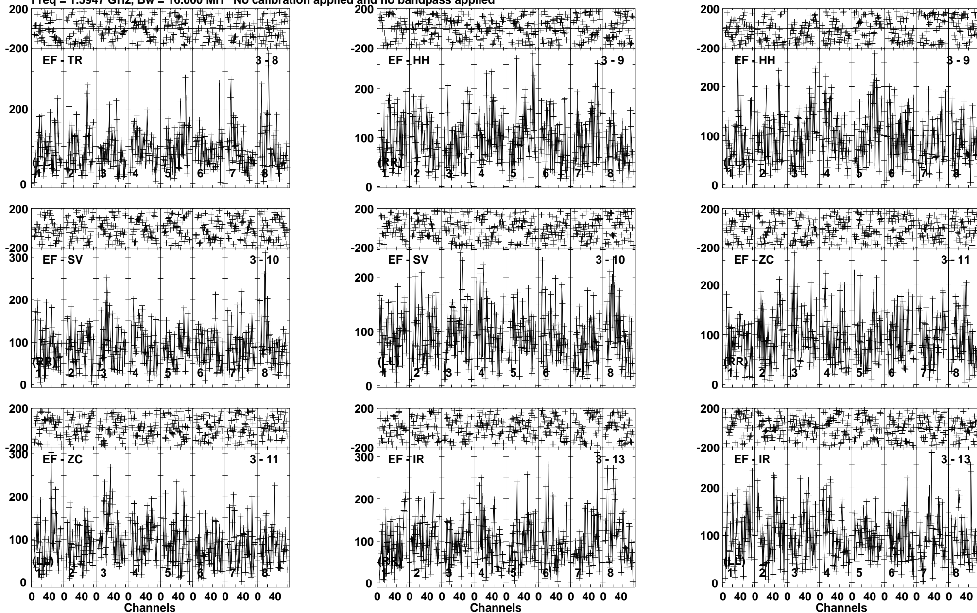
Lower frame: Micro Ampl Jy Top frame: Phas deg Vector averaged cross-power spectrum Baseline: EF (03) - TR (08) Timerange: 00/11:05:16 to 00/11:10:14
