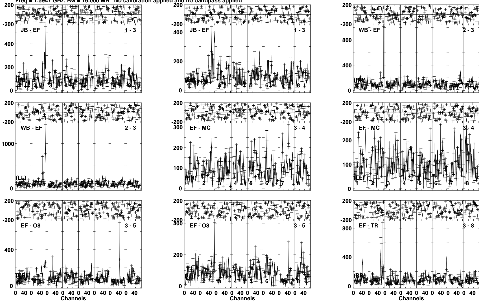
Lower frame: Micro Ampl Jy Top frame: Phas deg Vector averaged cross-power spectrum Baseline: JB (01) - EF (03) Timerange: 00/12:35:01 to 00/12:39:59
