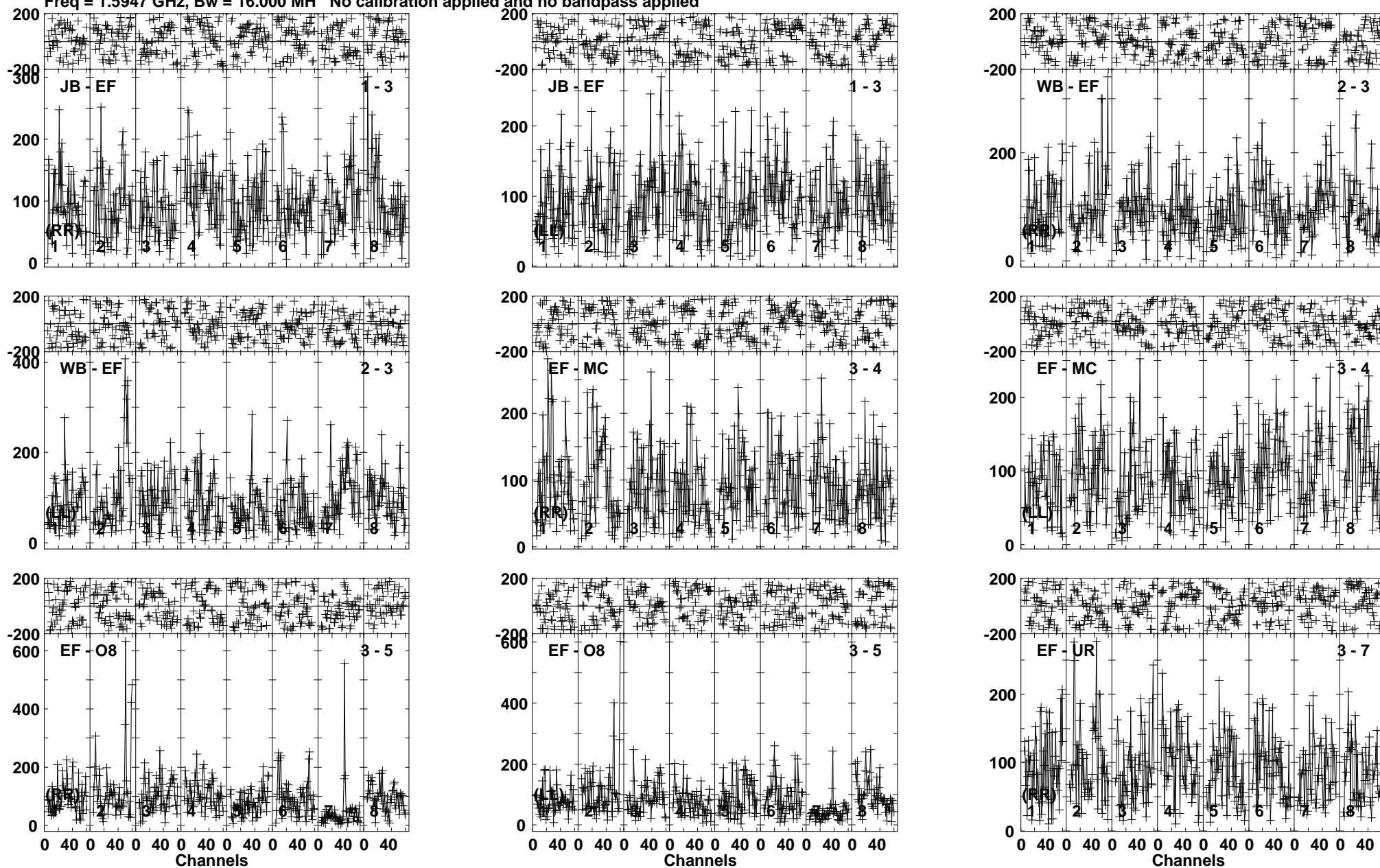
Lower frame: Micro Ampl Jy Top frame: Phas deg Vector averaged cross-power spectrum Baseline: JB (01) - EF (03) Timerange: 00/10:43:46 to 00/10:48:44
