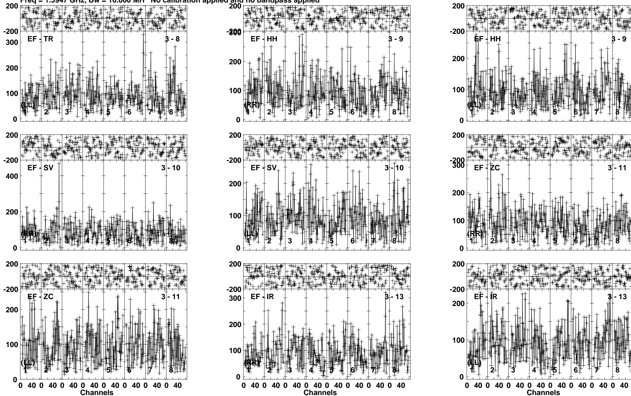
Lower frame: Micro Ampl Jy Top frame: Phas deg Vector averaged cross-power spectrum Baseline: EF (03) - TR (08) Timerange: 00/11:46:31 to 00/11:51:29
