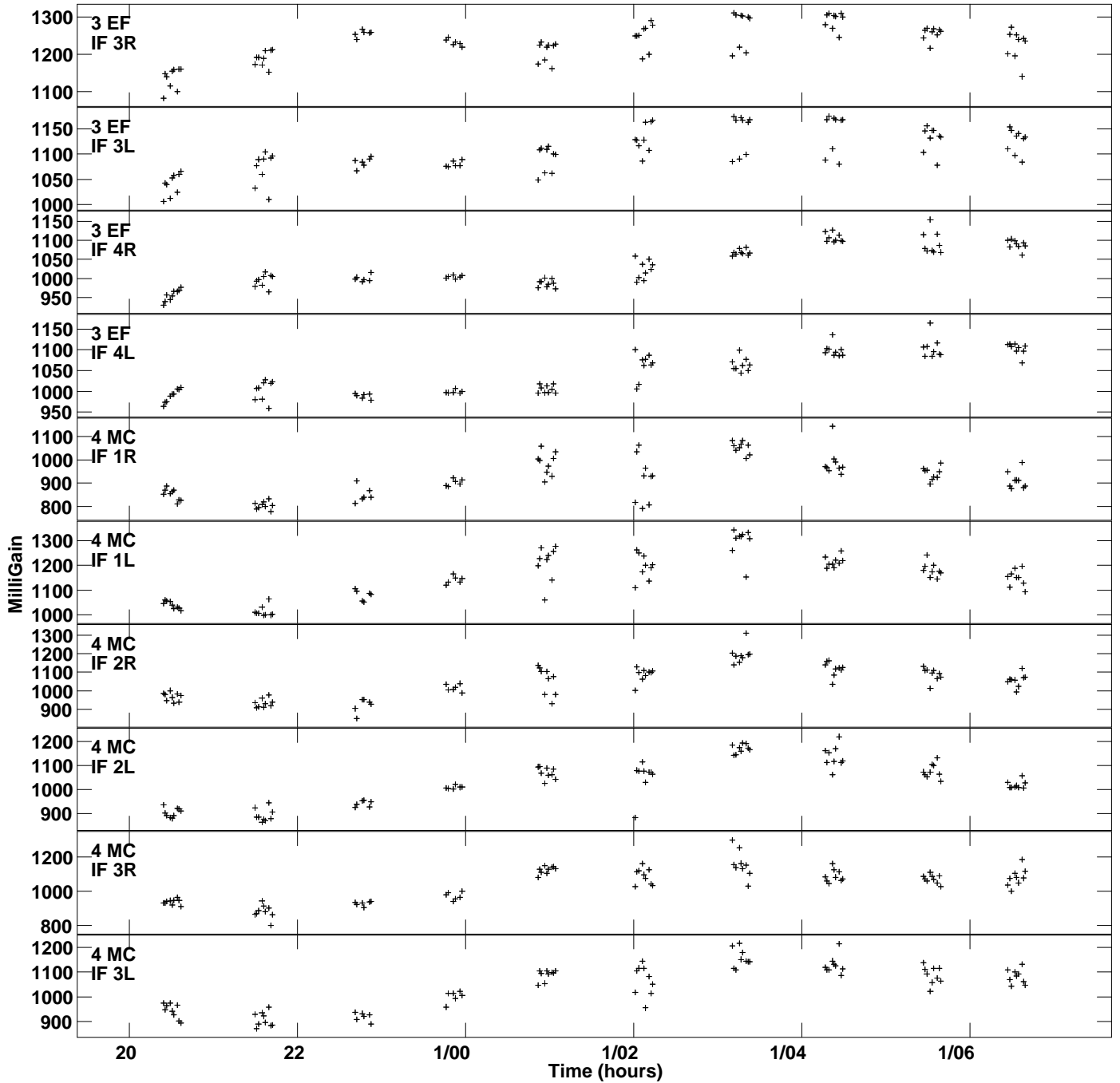
Plot file version 3 created 15-JUN-2021 11:21:52 Gain amp vs UTC time for NGC4278.MULTI.1 SN 2 Rpol & Lpol IF 1 - 4
