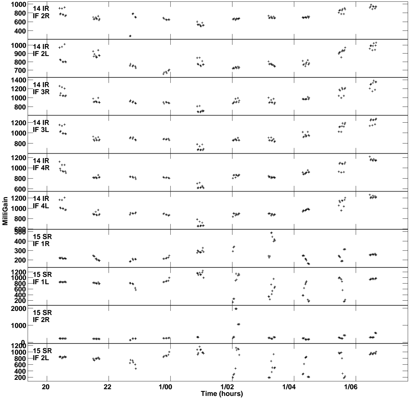
Plot file version 10 created 15-JUN-2021 11:21:52 Gain amp vs UTC time for NGC4278.MULTI.1 SN 2 Rpol & Lpol IF 1 - 4
