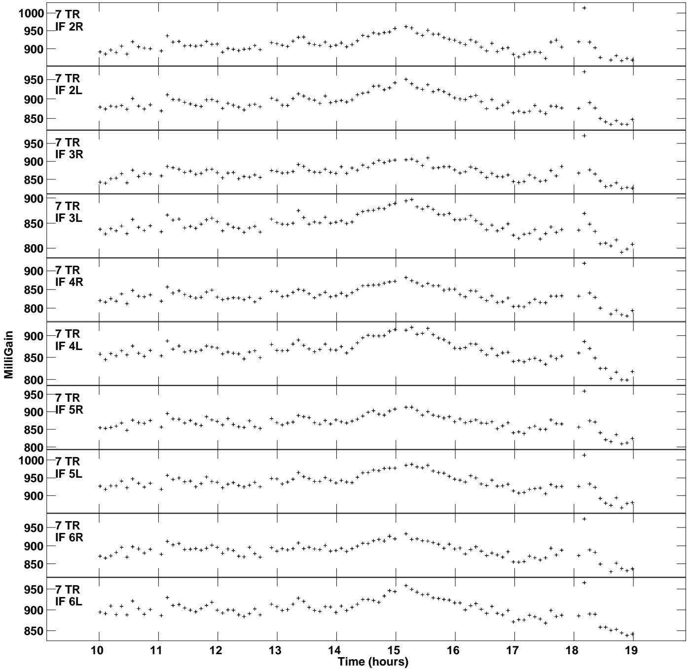
Plot file version 10 created 08-APR-2022 17:38:40 Gain amp vs UTC time for J1651+0129.MULTI.1 SN 2 Rpol & Lpol IF 1 - 8
