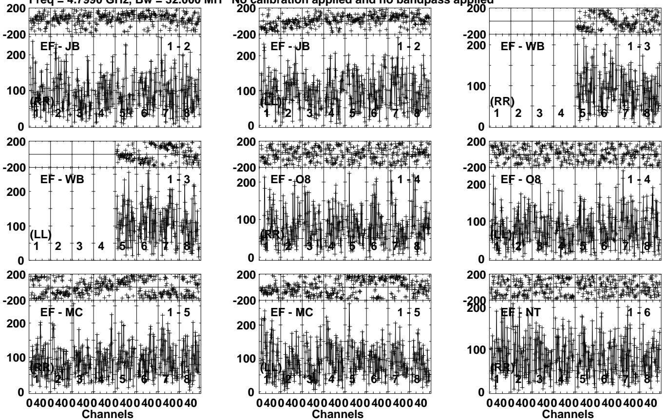
Lower frame: Micro Ampl Jy Top frame: Phas deg Vector averaged cross-power spectrum Several baselines displayed Timerange: 00/16:10:55 to 00/16:14:23
