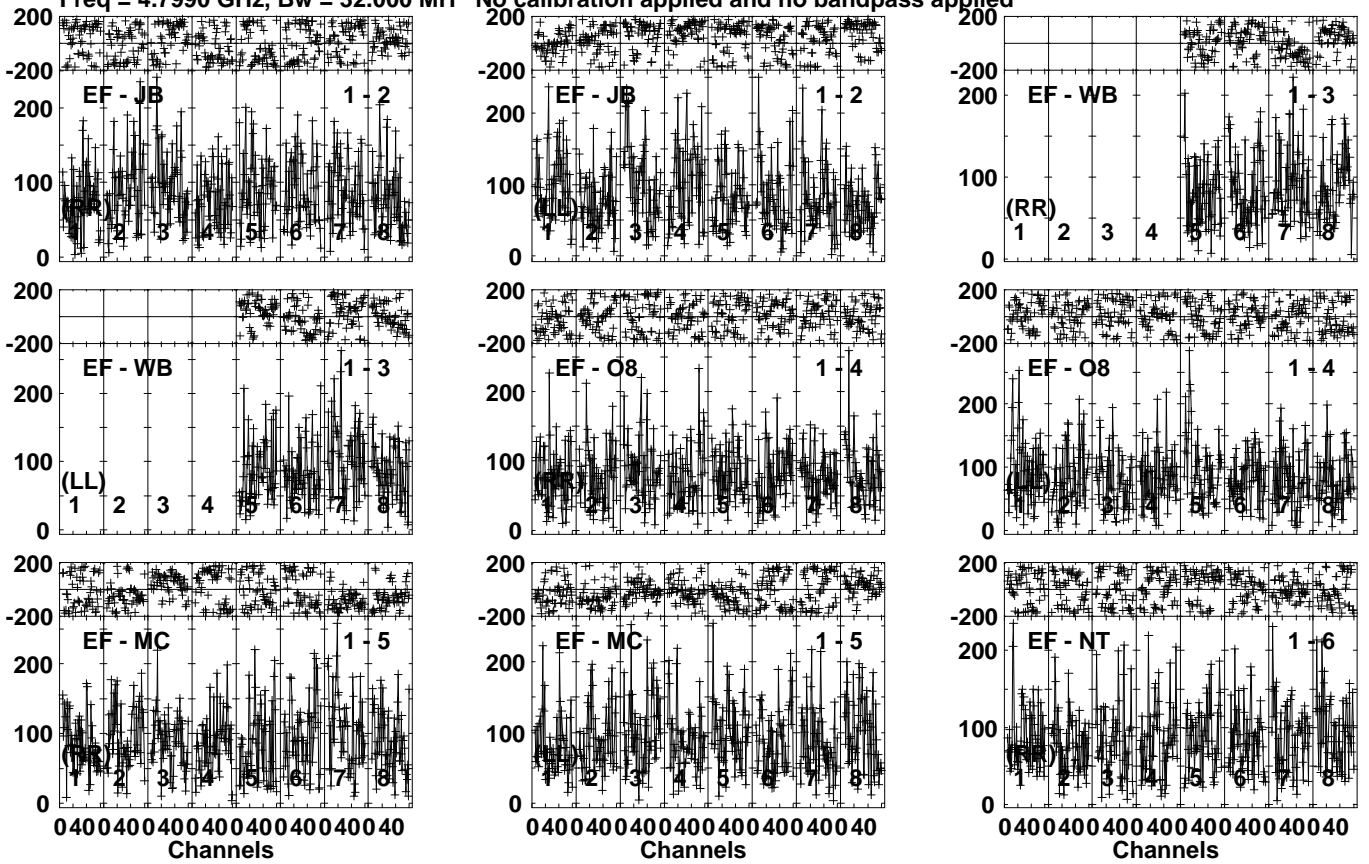
Lower frame: Micro Ampl Jy Top frame: Phas deg Vector averaged cross-power spectrum Several baselines displayed Timerange: 00/15:33:00 to 00/15:36:28
