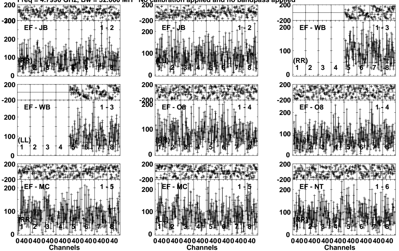
Lower frame: Micro Ampl Jy Top frame: Phas deg Vector averaged cross-power spectrum Several baselines displayed Timerange: 00/18:49:08 to 00/18:52:36
