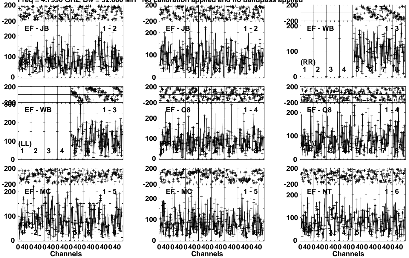
Lower frame: Micro Ampl Jy Top frame: Phas deg Vector averaged cross-power spectrum Several baselines displayed Timerange: 00/18:05:50 to 00/18:09:16
