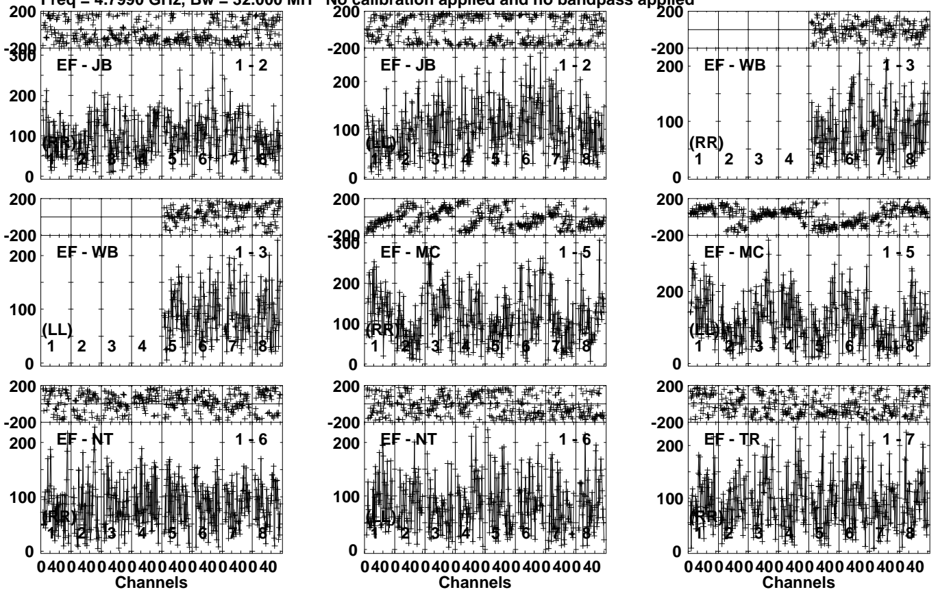
Lower frame: Micro Ampl Jy Top frame: Phas deg Vector averaged cross-power spectrum Several baselines displayed Timerange: 00/10:46:53 to 00/10:50:19
