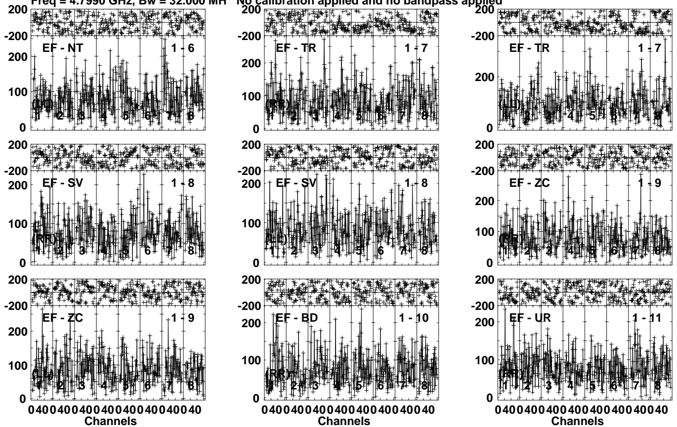
Lower frame: Micro Ampl Jy Top frame: Phas deg Vector averaged cross-power spectrum Several baselines displayed Timerange: 00/11:33:07 to 00/11:36:35
