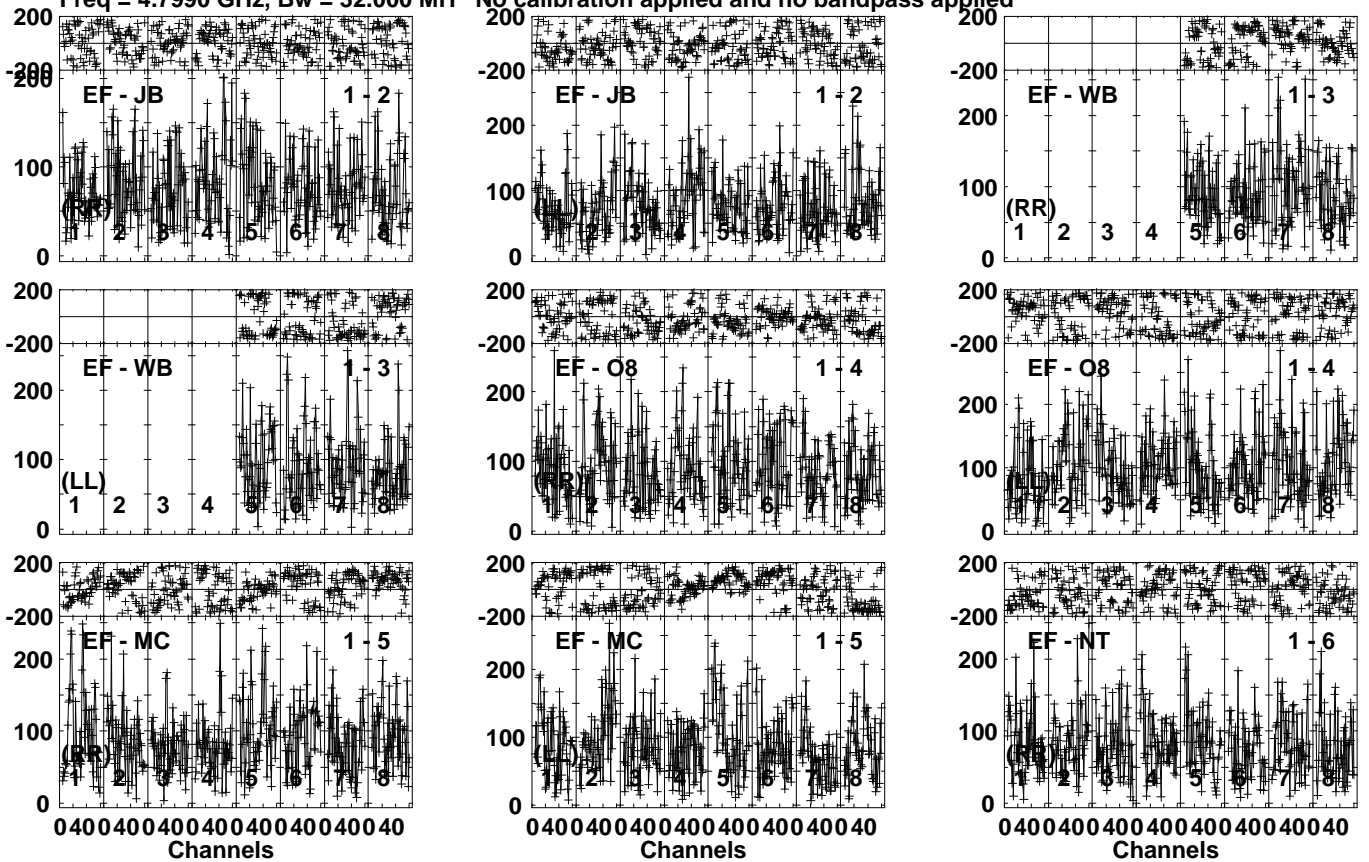
Lower frame: Micro Ampl Jy Top frame: Phas deg Vector averaged cross-power spectrum Several baselines displayed Timerange: 00/12:32:42 to 00/12:36:10
