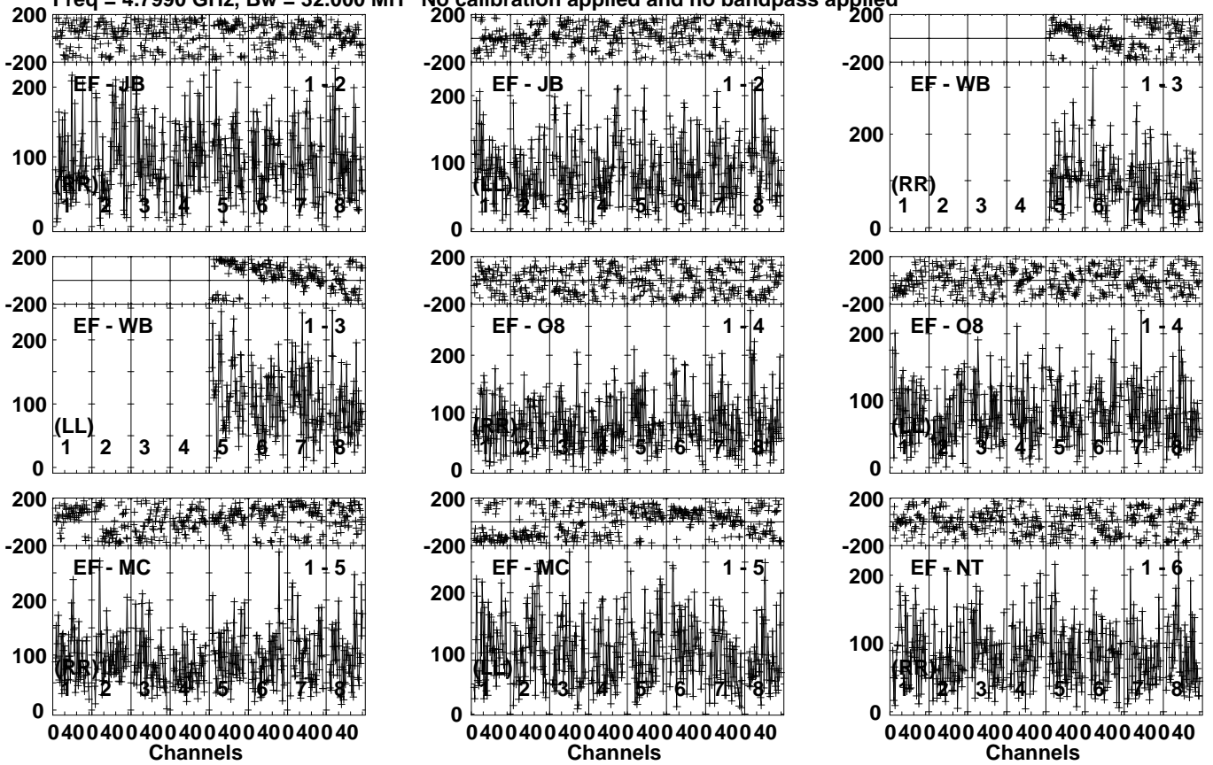
Lower frame: Micro Ampl Jy Top frame: Phas deg Vector averaged cross-power spectrum Several baselines displayed Timerange: 00/14:48:57 to 00/14:52:23
