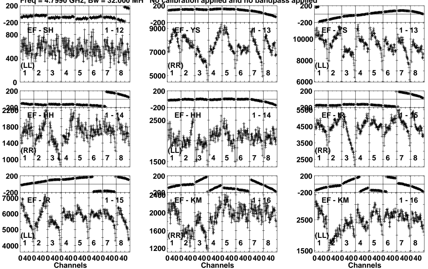
Lower frame: Micro Ampl Jy Top frame: Phas deg Vector averaged cross-power spectrum Several baselines displayed Timerange: 00/11:58:42 to 00/12:00:10
