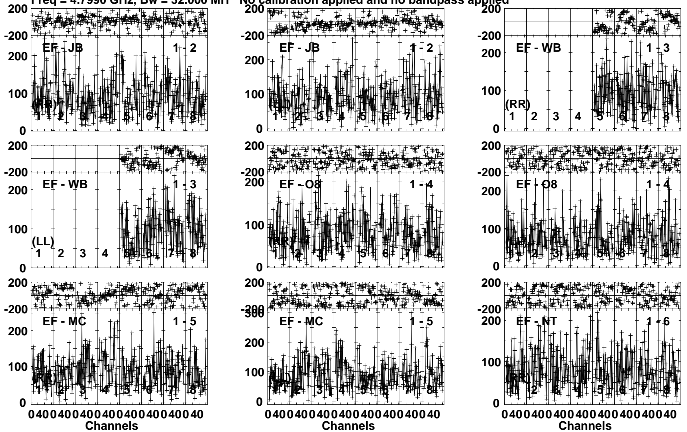
Lower frame: Micro Ampl Jy Top frame: Phas deg Vector averaged cross-power spectrum Several baselines displayed Timerange: 00/16:21:45 to 00/16:25:13
