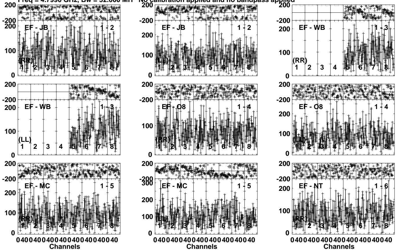
Lower frame: Micro Ampl Jy Top frame: Phas deg Vector averaged cross-power spectrum Several baselines displayed Timerange: 00/15:27:35 to 00/15:31:03
