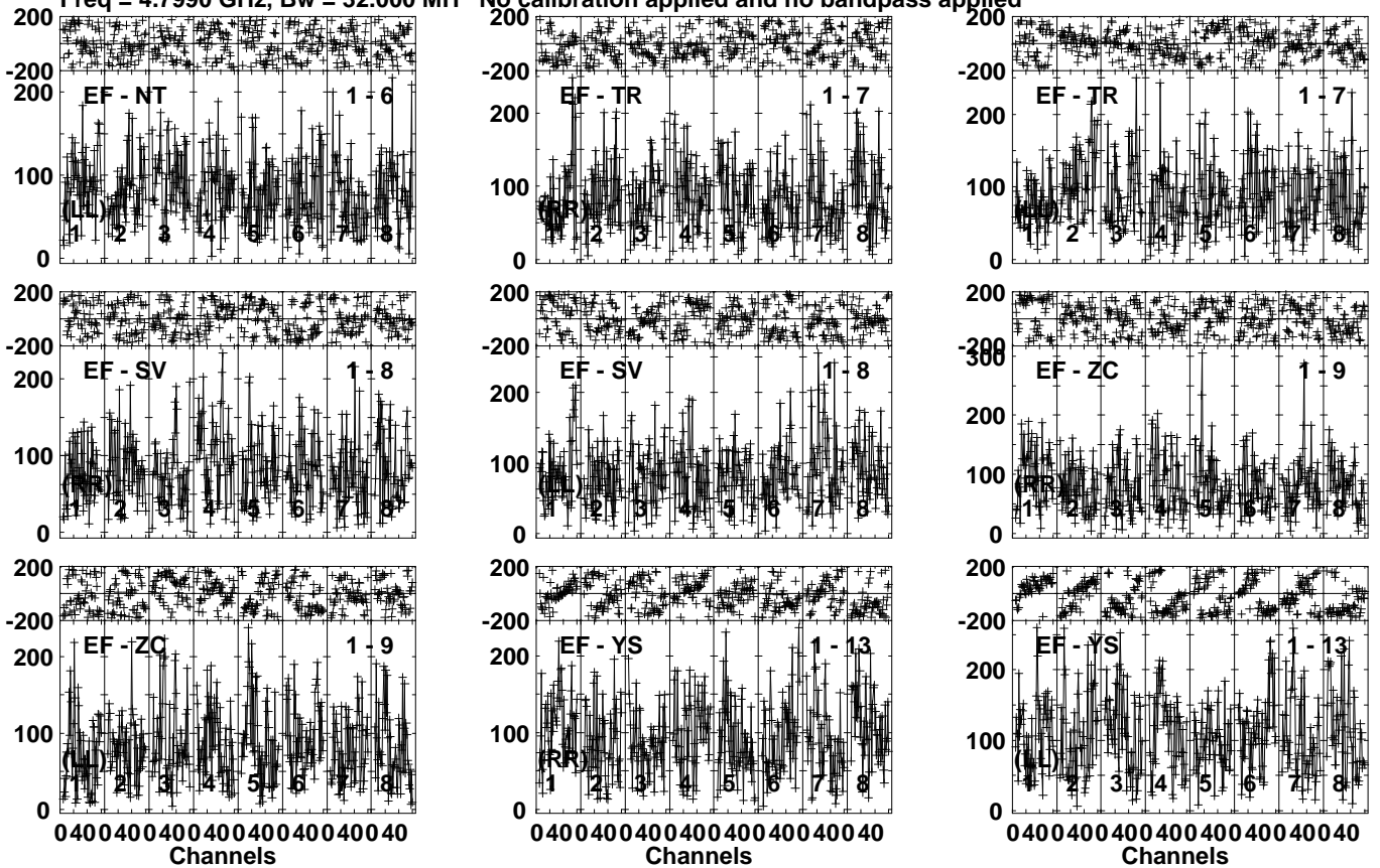
Lower frame: Micro Ampl Jy Top frame: Phas deg Vector averaged cross-power spectrum Several baselines displayed Timerange: 00/15:49:15 to 00/15:52:43
