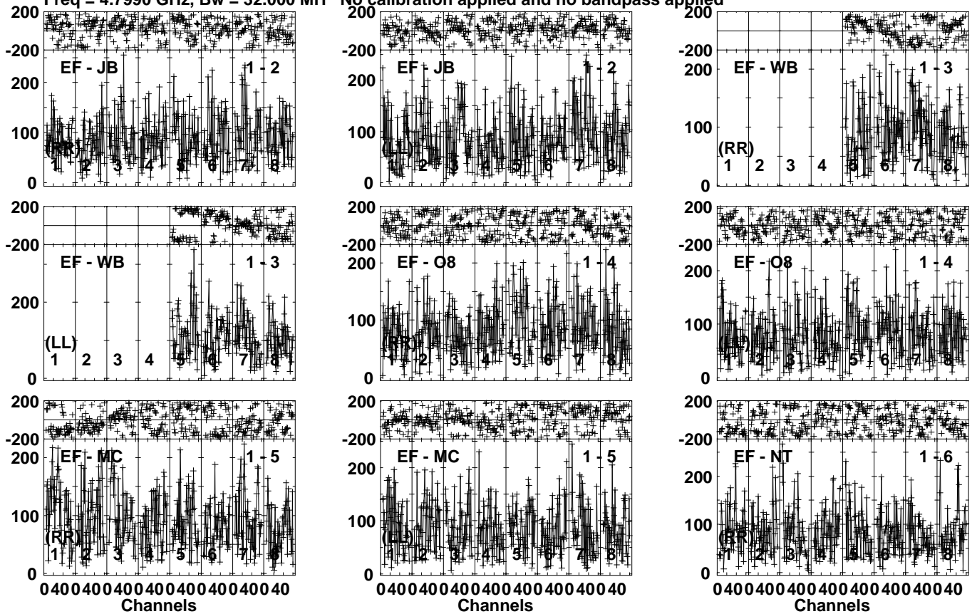
Lower frame: Micro Ampl Jy Top frame: Phas deg Vector averaged cross-power spectrum Several baselines displayed Timerange: 00/15:43:50 to 00/15:47:18
