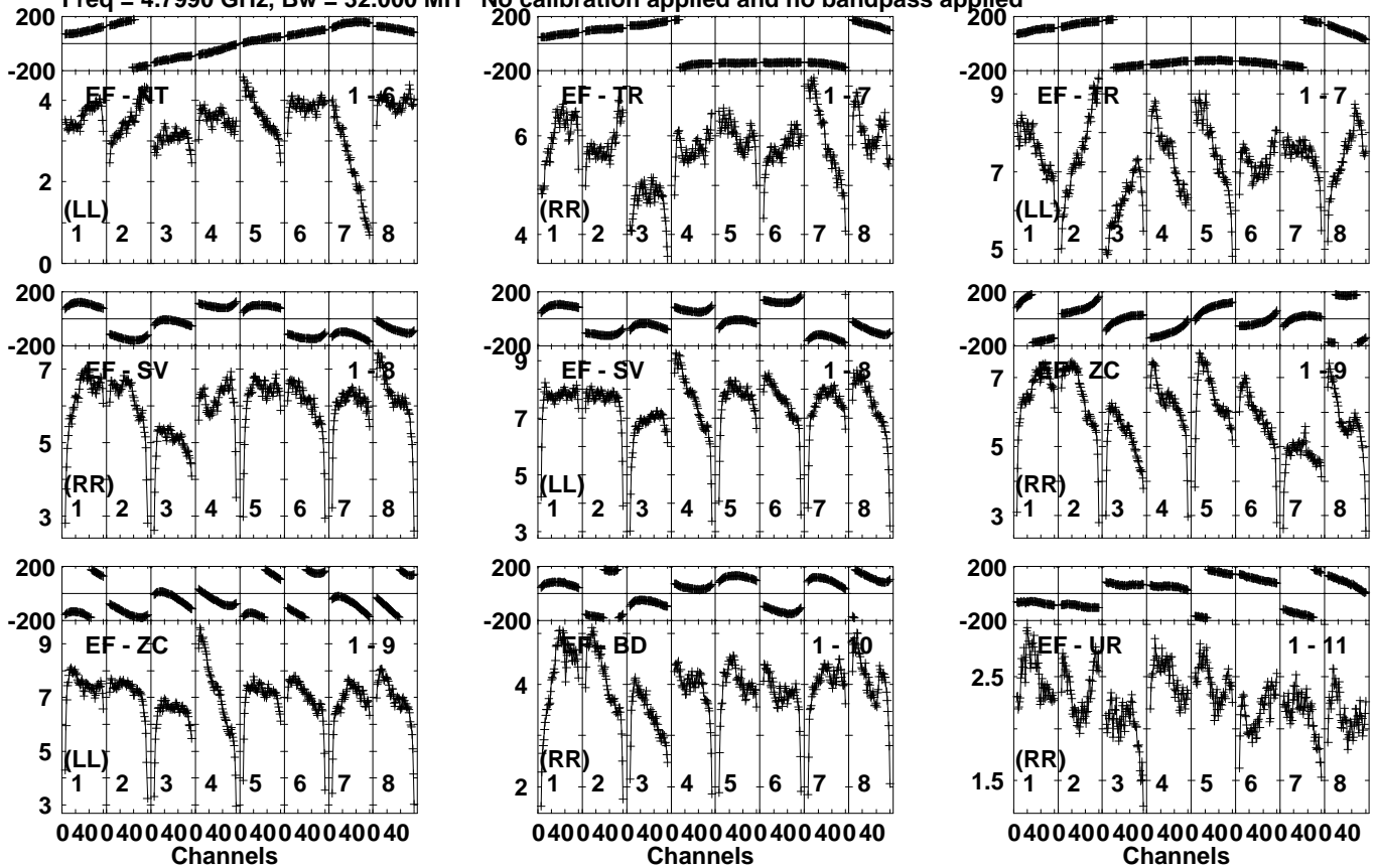
Lower frame: Milli Ampl Jy Top frame: Phas deg Vector averaged cross-power spectrum Several baselines displayed Timerange: 00/12:42:02 to 00/12:43:30
