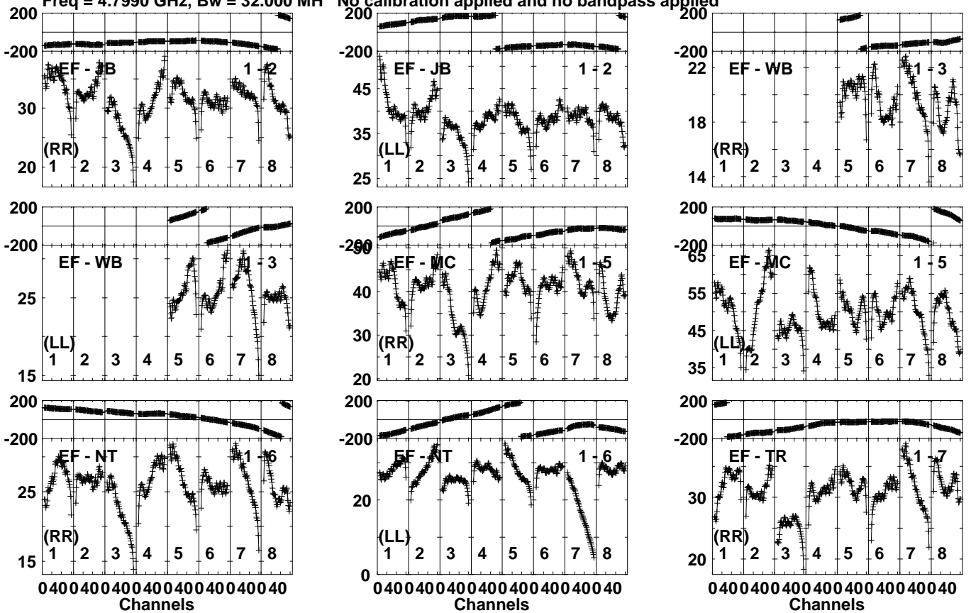
Lower frame: Milli Ampl Jy Top frame: Phas deg Vector averaged cross-power spectrum Several baselines displayed Timerange: 00/10:55:16 to 00/10:59:14
