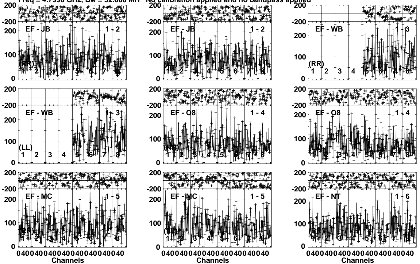
Lower frame: Micro Ampl Jy Top frame: Phas deg Vector averaged cross-power spectrum Several baselines displayed Timerange: 00/13:11:25 to 00/13:14:53
