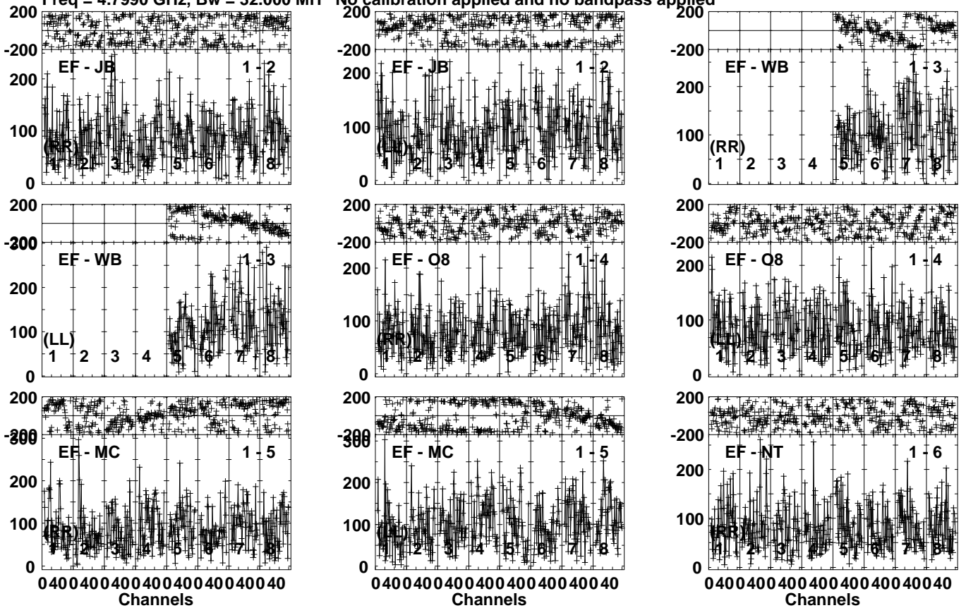
Lower frame: Micro Ampl Jy Top frame: Phas deg Vector averaged cross-power spectrum Several baselines displayed Timerange: 00/14:32:42 to 00/14:36:08
