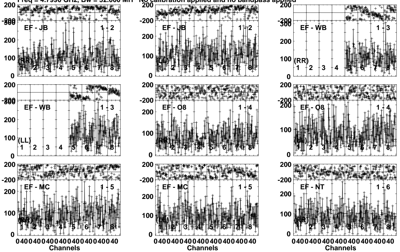
Lower frame: Micro Ampl Jy Top frame: Phas deg Vector averaged cross-power spectrum Several baselines displayed Timerange: 00/14:54:20 to 00/14:57:48
