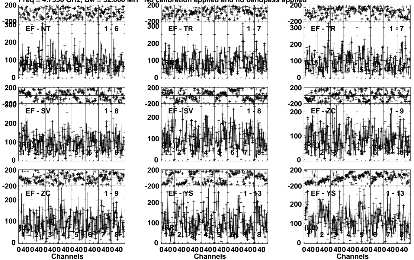
Lower frame: Micro Ampl Jy Top frame: Phas deg Vector averaged cross-power spectrum Several baselines displayed Timerange: 00/16:27:10 to 00/16:30:38
