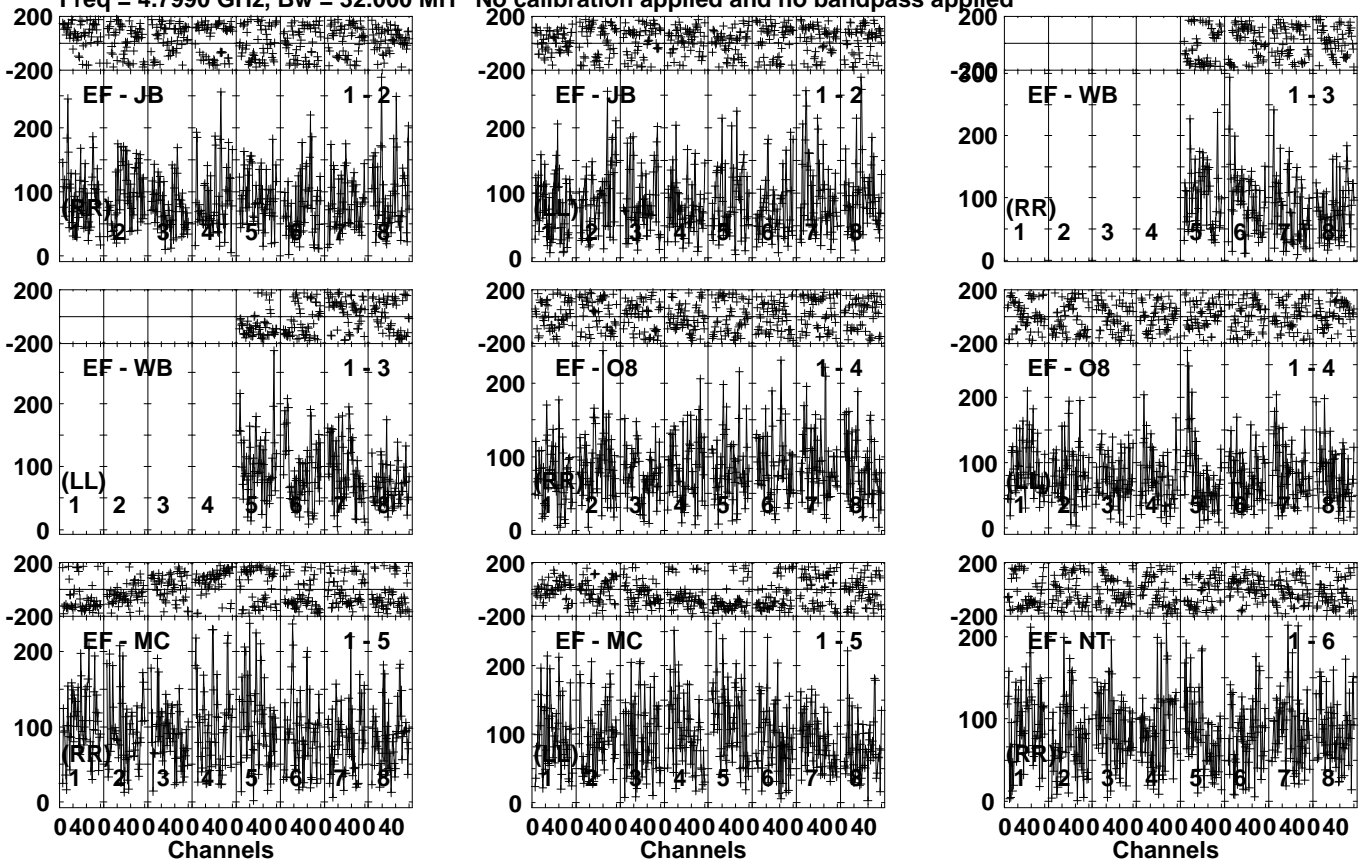
Lower frame: Micro Ampl Jy Top frame: Phas deg Vector averaged cross-power spectrum Several baselines displayed Timerange: 00/15:11:20 to 00/15:14:48
