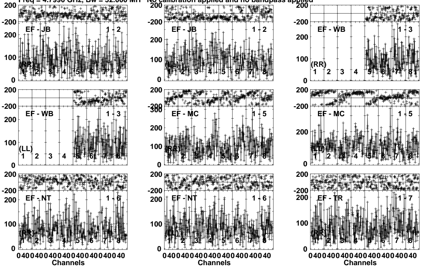
Lower frame: Micro Ampl Jy Top frame: Phas deg Vector averaged cross-power spectrum Several baselines displayed Timerange: 00/10:29:06 to 00/10:32:34
