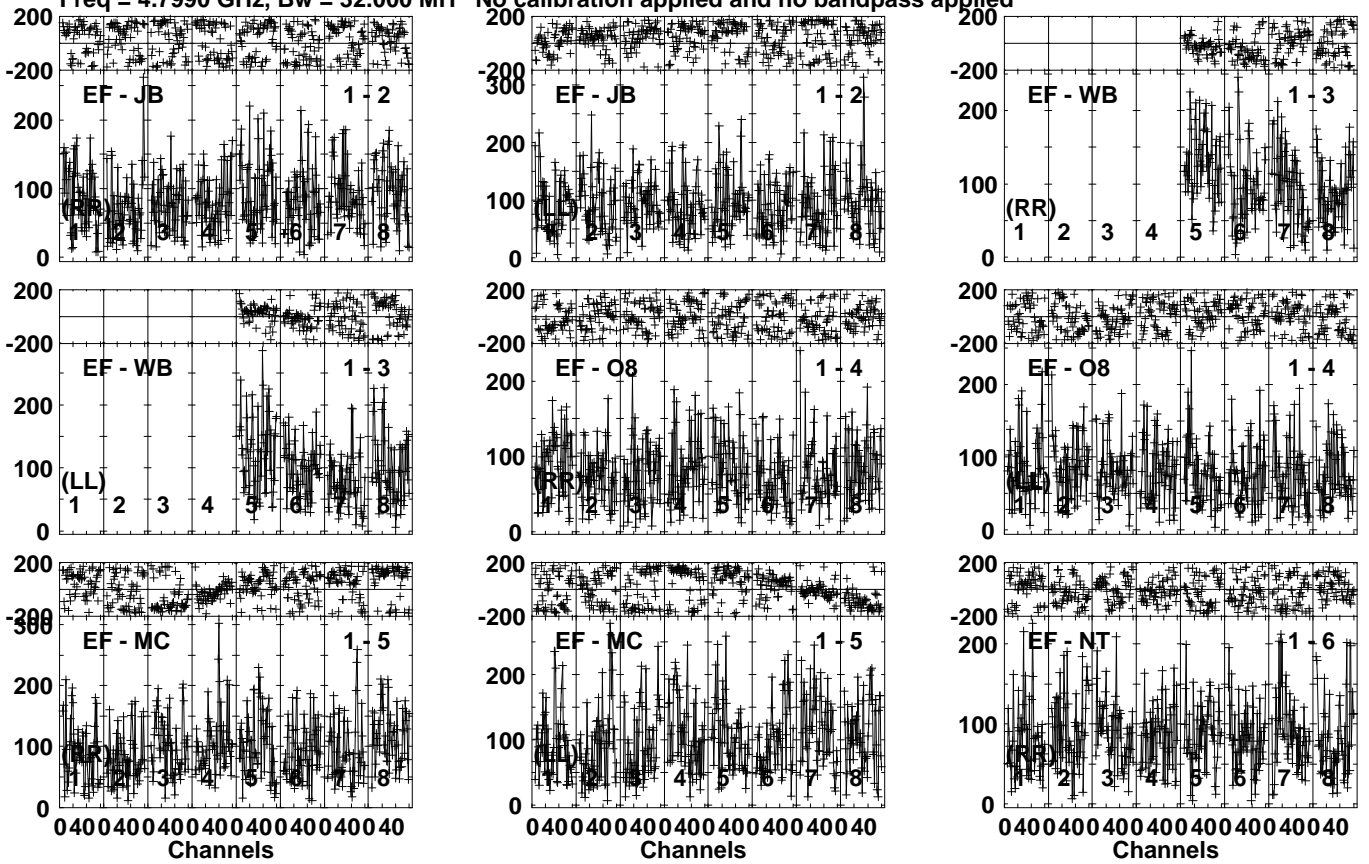
Lower frame: Micro Ampl Jy Top frame: Phas deg Vector averaged cross-power spectrum Several baselines displayed Timerange: 00/14:43:30 to 00/14:46:58
