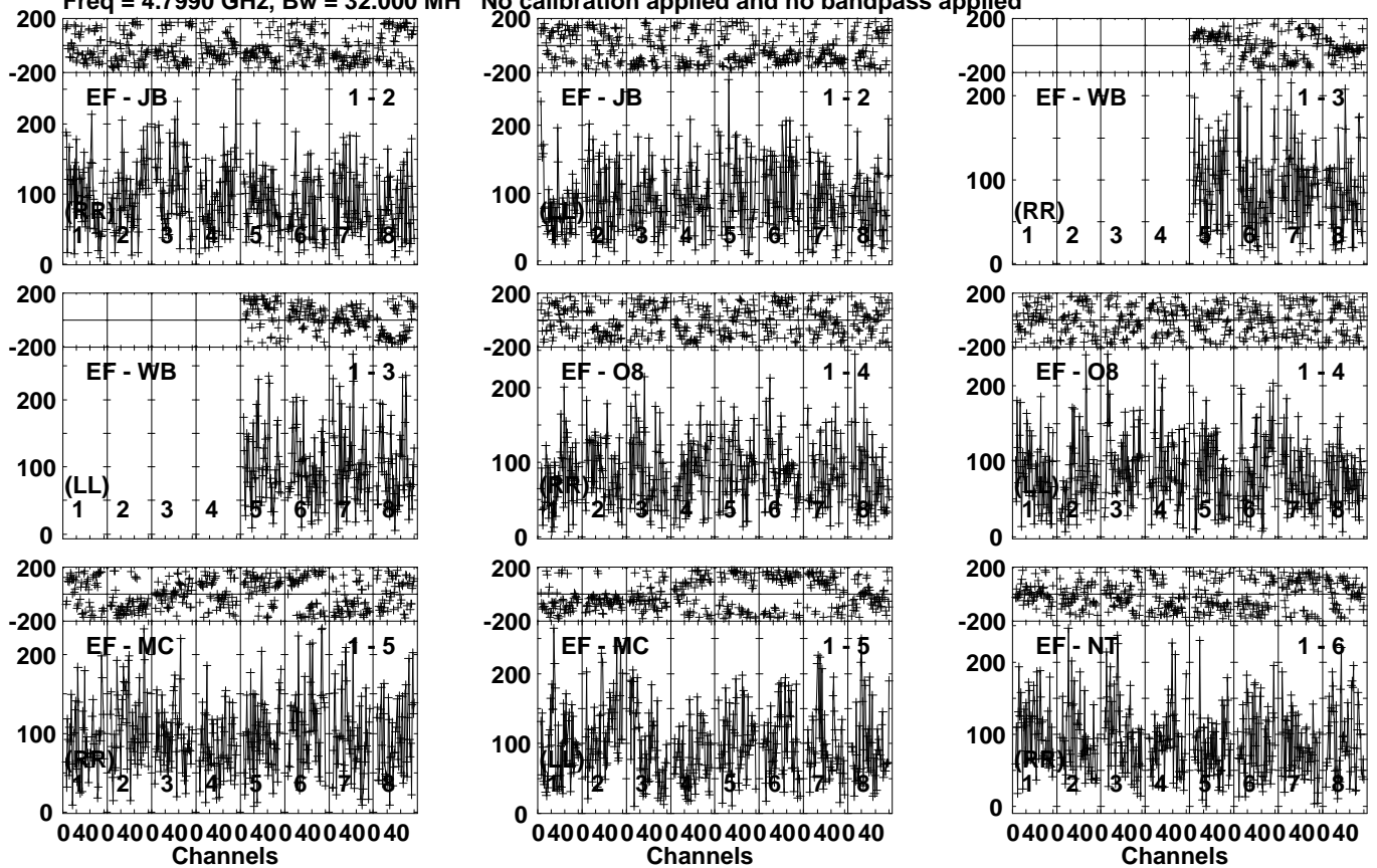
Lower frame: Micro Ampl Jy Top frame: Phas deg Vector averaged cross-power spectrum Several baselines displayed Timerange: 00/14:16:25 to 00/14:19:53
