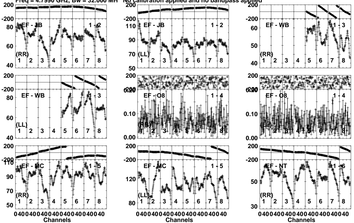
Lower frame: Milli Ampl Jy Top frame: Phas deg Vector averaged cross-power spectrum Several baselines displayed Timerange: 00/17:53:40 to 00/17:57:38
