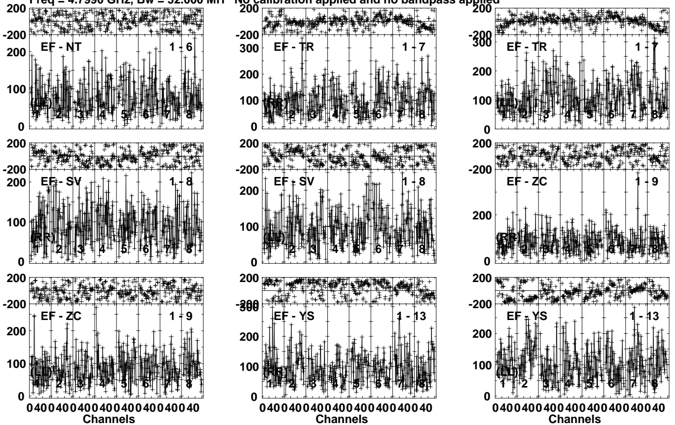
Lower frame: Micro Ampl Jy Top frame: Phas deg Vector averaged cross-power spectrum Several baselines displayed Timerange: 00/17:15:55 to 00/17:19:23
