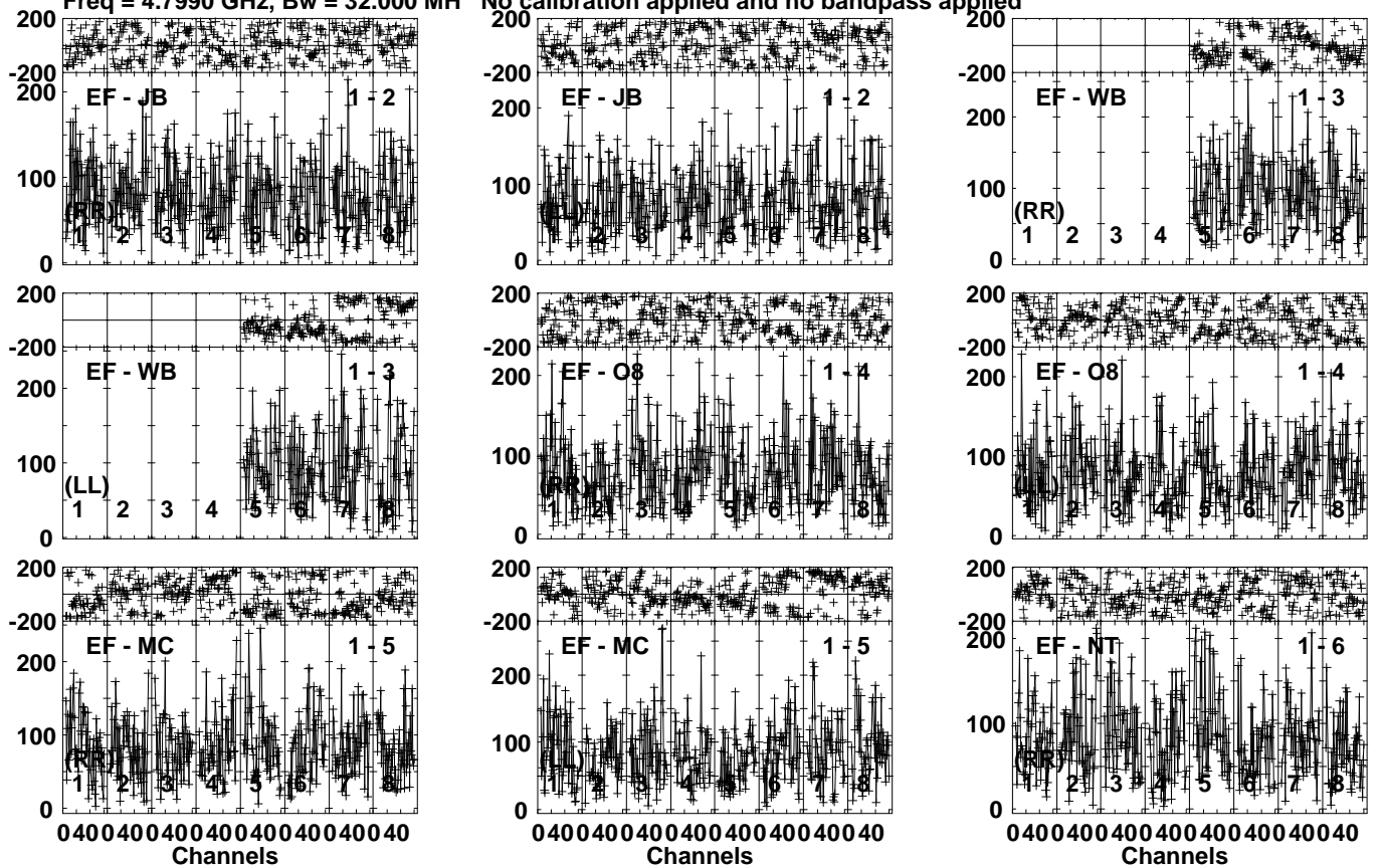
Lower frame: Micro Ampl Jy Top frame: Phas deg Vector averaged cross-power spectrum Several baselines displayed Timerange: 00/13:22:15 to 00/13:25:43
