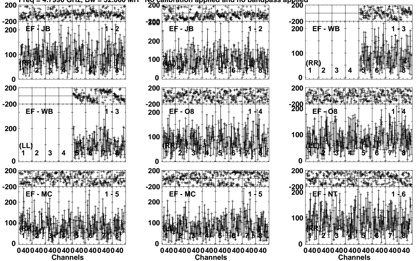
Lower frame: Micro Ampl Jy Top frame: Phas deg Vector averaged cross-power spectrum Several baselines displayed Timerange: 00/16:54:15 to 00/16:57:43
