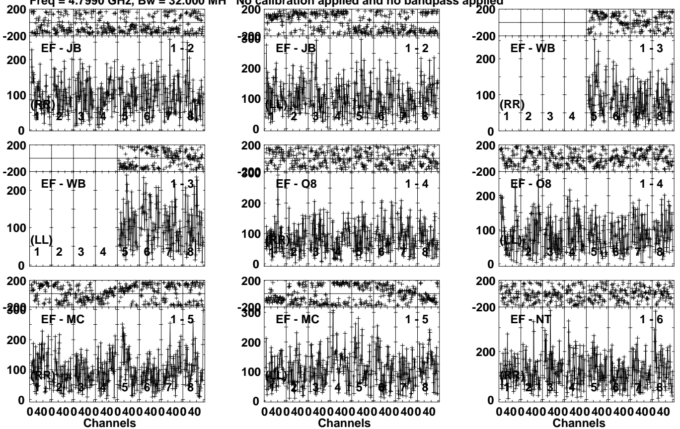
Lower frame: Micro Ampl Jy Top frame: Phas deg Vector averaged cross-power spectrum Several baselines displayed Timerange: 00/14:21:50 to 00/14:25:18
