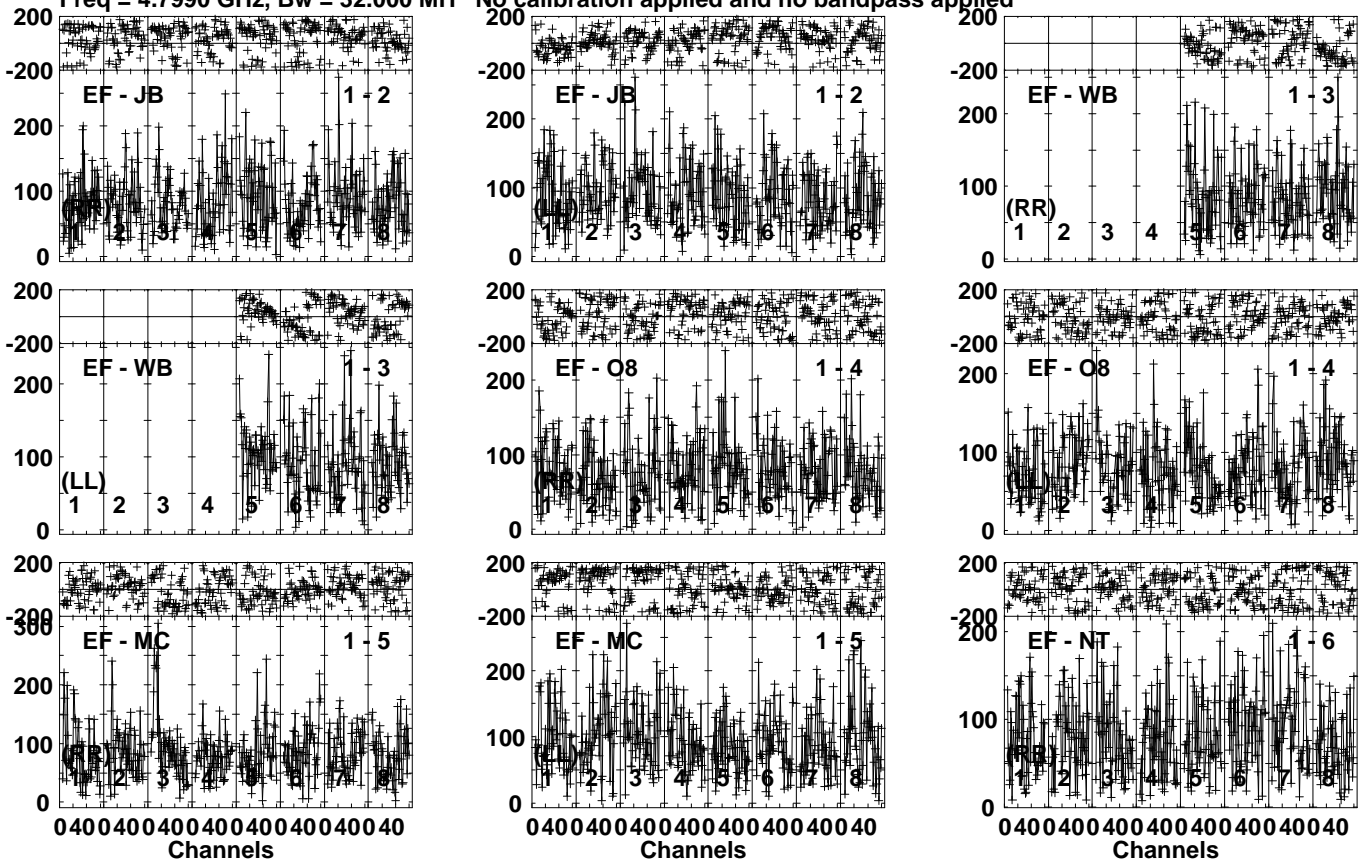
Lower frame: Micro Ampl Jy Top frame: Phas deg Vector averaged cross-power spectrum Several baselines displayed Timerange: 00/18:43:45 to 00/18:47:11
