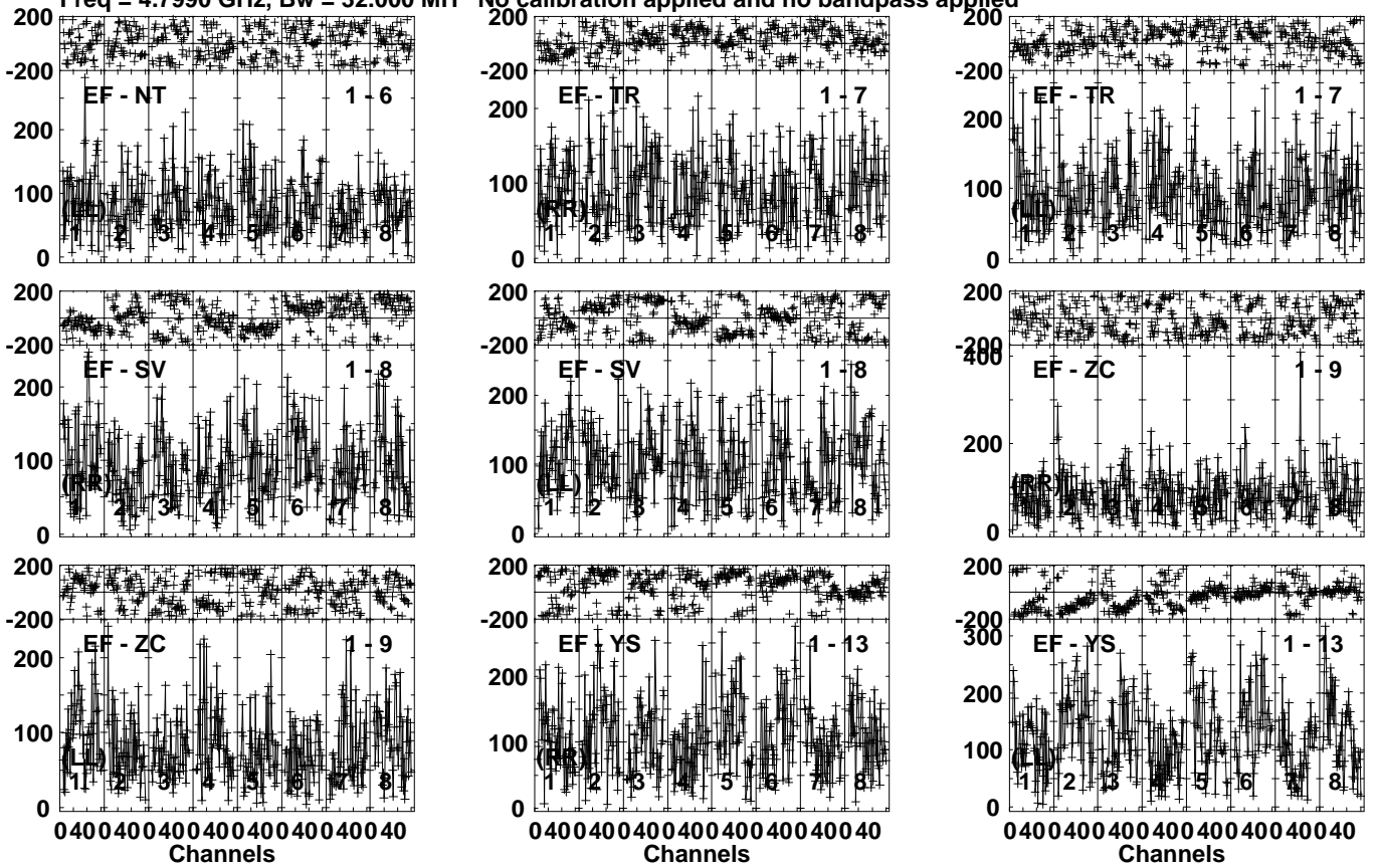
Lower frame: Micro Ampl Jy Top frame: Phas deg Vector averaged cross-power spectrum Several baselines displayed Timerange: 00/16:38:00 to 00/16:41:28
