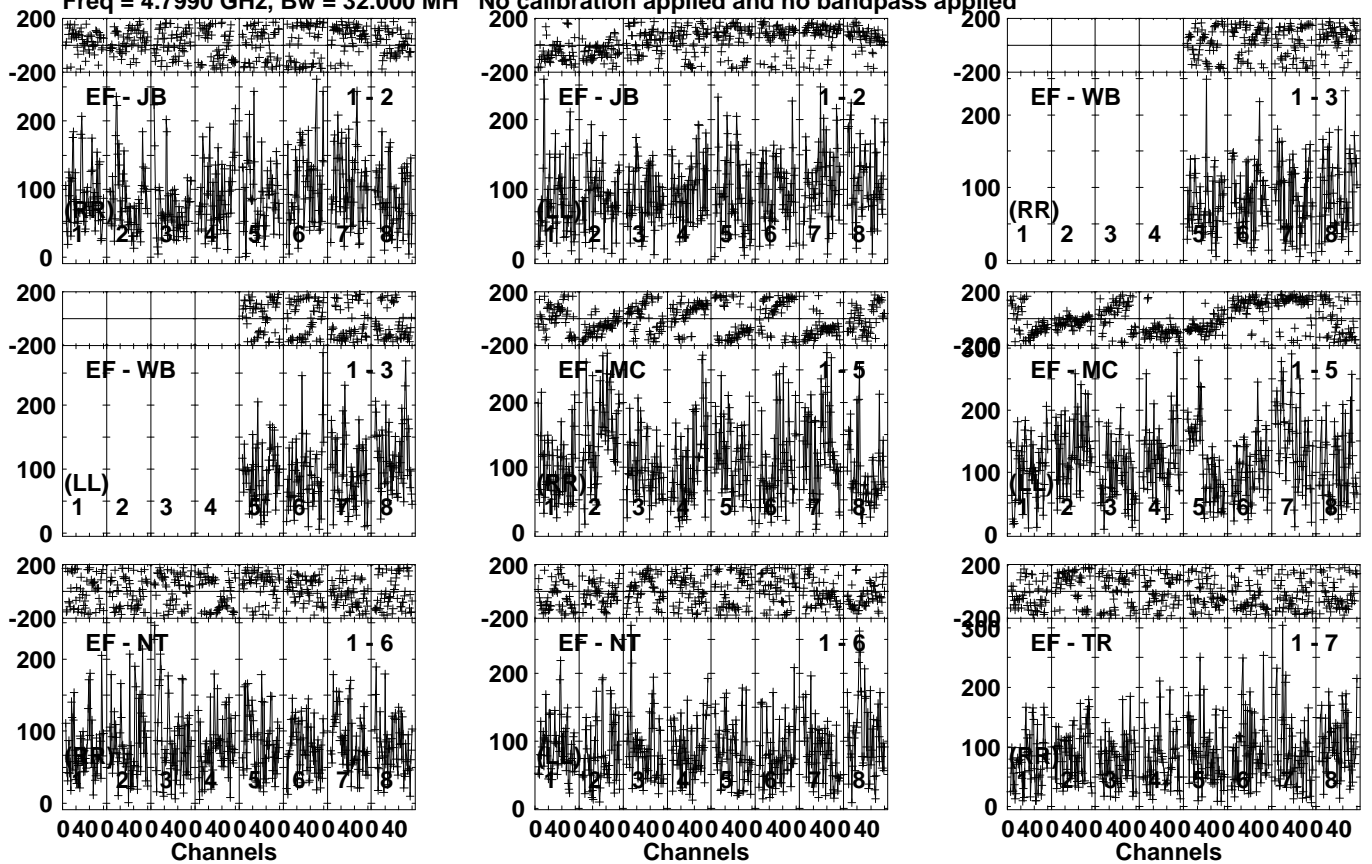
Lower frame: Micro Ampl Jy Top frame: Phas deg Vector averaged cross-power spectrum Several baselines displayed Timerange: 00/10:40:58 to 00/10:44:24
