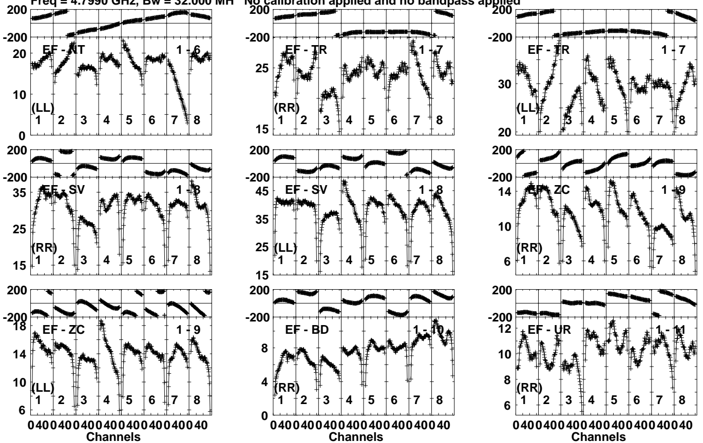
Lower frame: Milli Ampl Jy Top frame: Phas deg Vector averaged cross-power spectrum Several baselines displayed Timerange: 00/15:02:38 to 00/15:06:26
