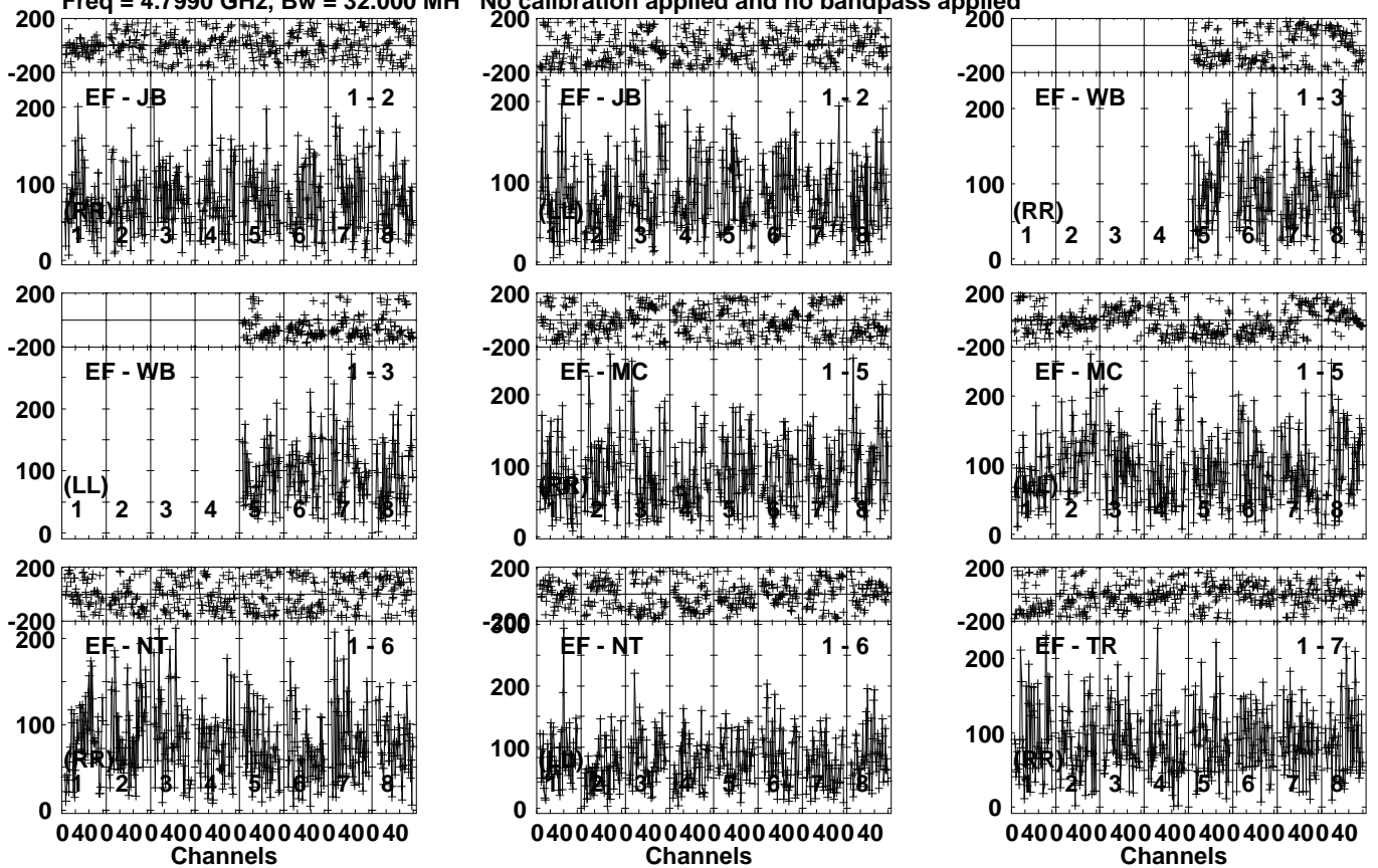
Lower frame: Micro Ampl Jy Top frame: Phas deg Vector averaged cross-power spectrum Several baselines displayed Timerange: 00/12:16:27 to 00/12:19:55
