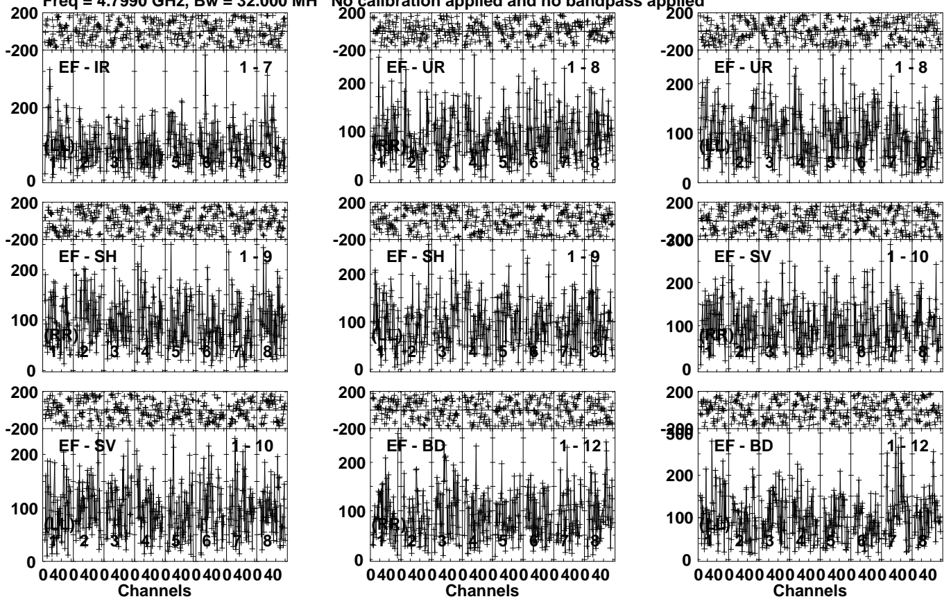
Lower frame: Micro Ampl Jy Top frame: Phas deg Vector averaged cross-power spectrum Several baselines displayed Timerange: 00/08:34:51 to 00/08:37:39
