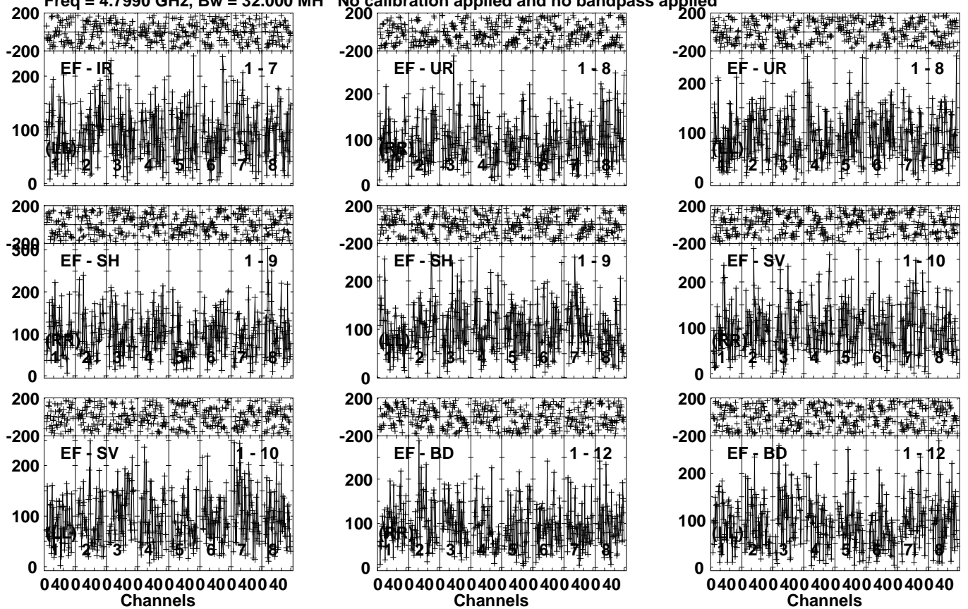
Lower frame: Micro Ampl Jy Top frame: Phas deg Vector averaged cross-power spectrum Several baselines displayed Timerange: 00/09:40:53 to 00/09:43:39
