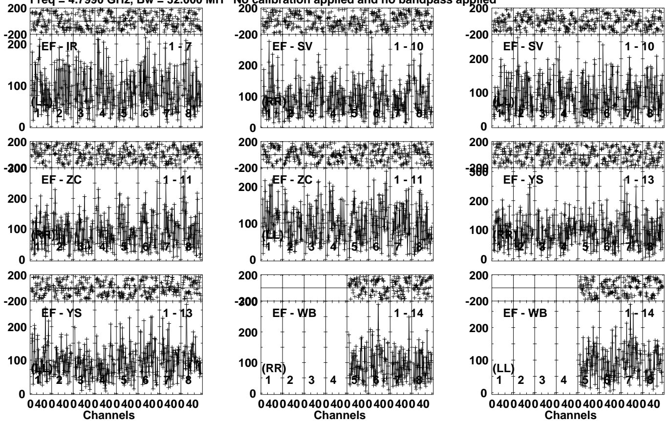
Lower frame: Micro Ampl Jy Top frame: Phas deg Vector averaged cross-power spectrum Several baselines displayed Timerange: 00/12:46:31 to 00/12:49:19
