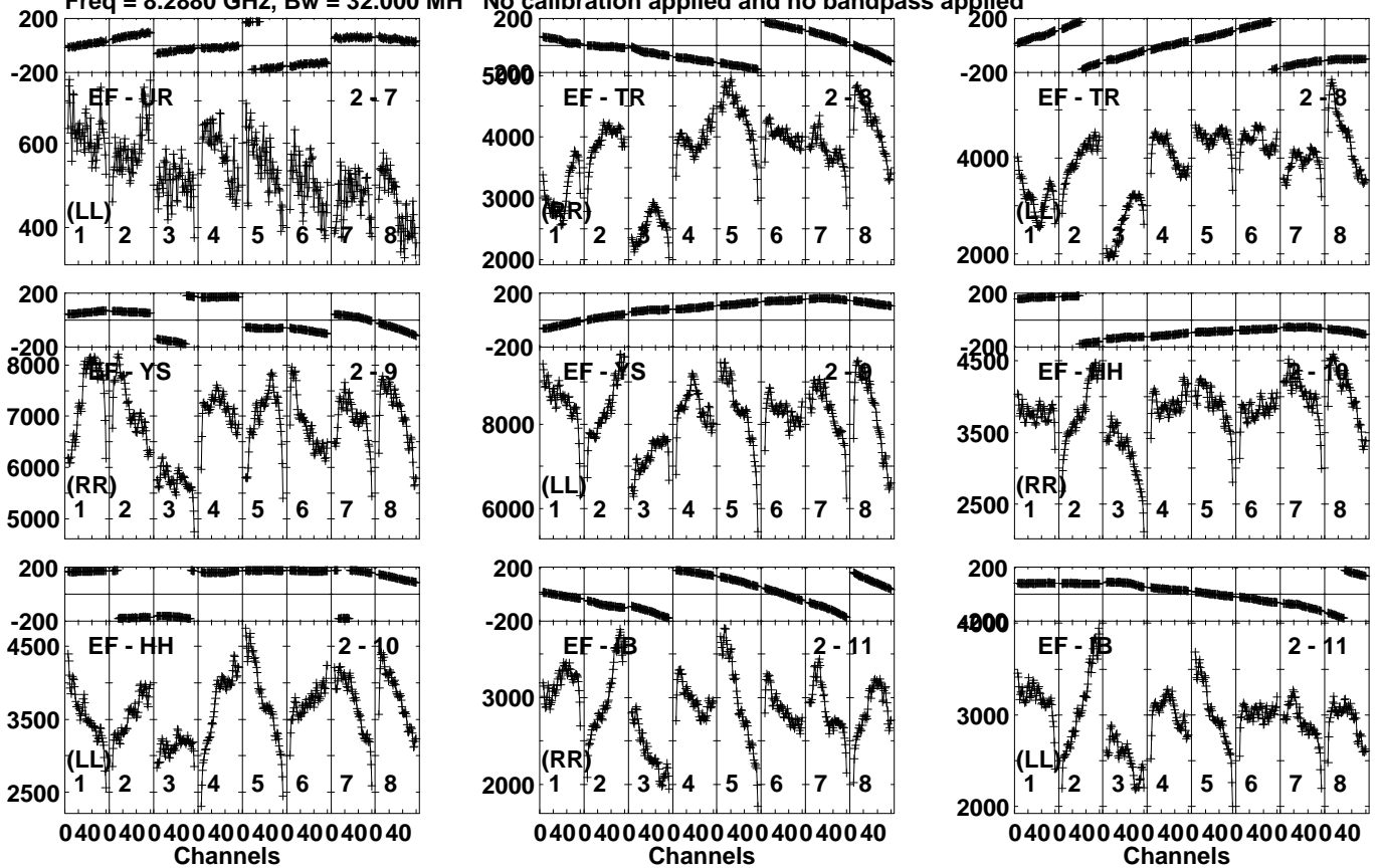
Lower frame: Micro Ampl Jy Top frame: Phas deg Vector averaged cross-power spectrum Several baselines displayed Timerange: 01/03:19:26 to 01/03:27:24
