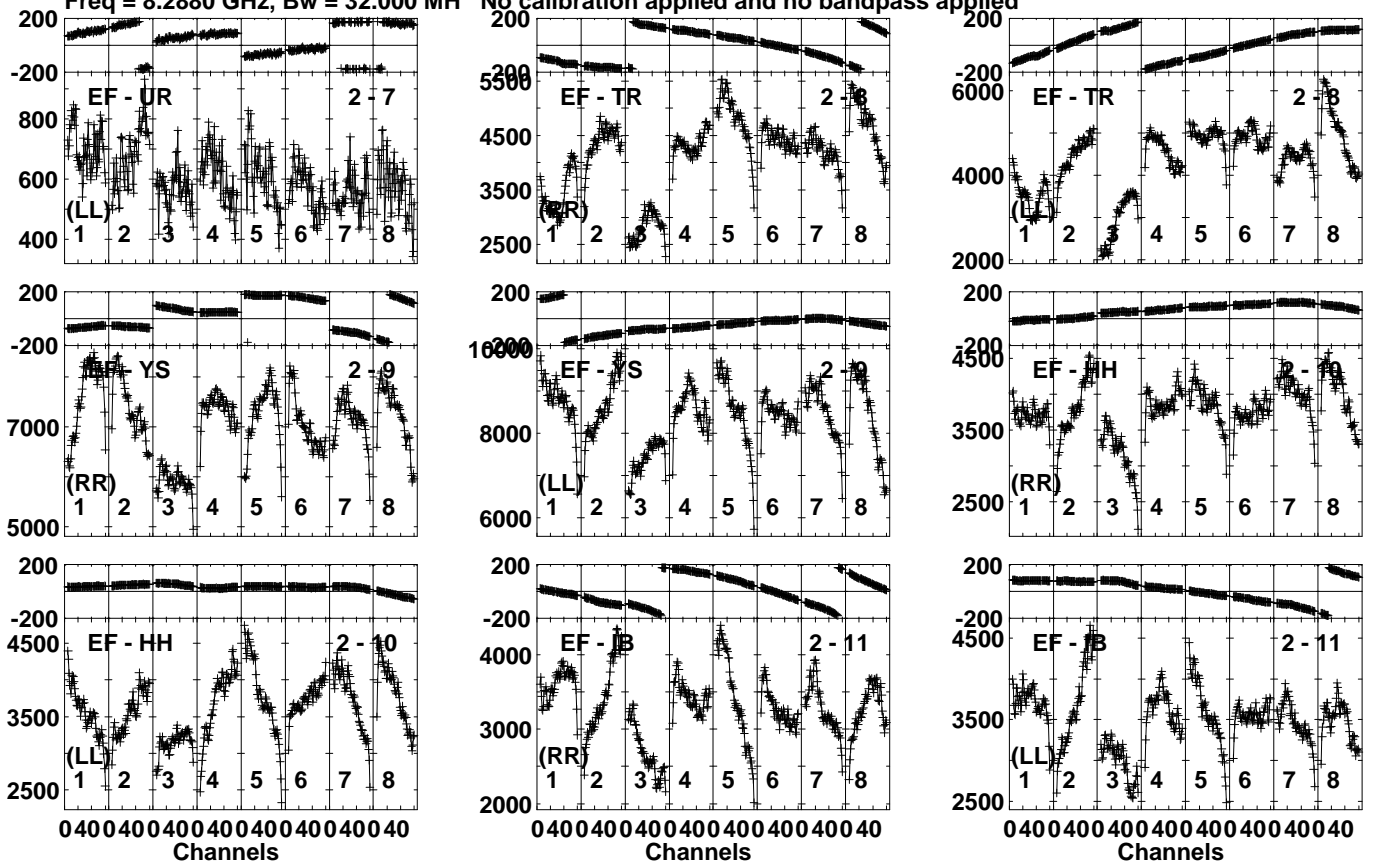
Lower frame: Micro Ampl Jy Top frame: Phas deg Vector averaged cross-power spectrum Several baselines displayed Timerange: 01/04:42:36 to 01/04:45:34
