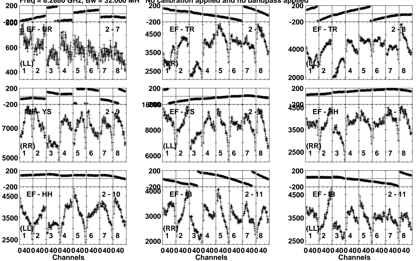
Lower frame: Micro Ampl Jy Top frame: Phas deg Vector averaged cross-power spectrum Several baselines displayed Timerange: 01/04:25:36 to 01/04:33:34
