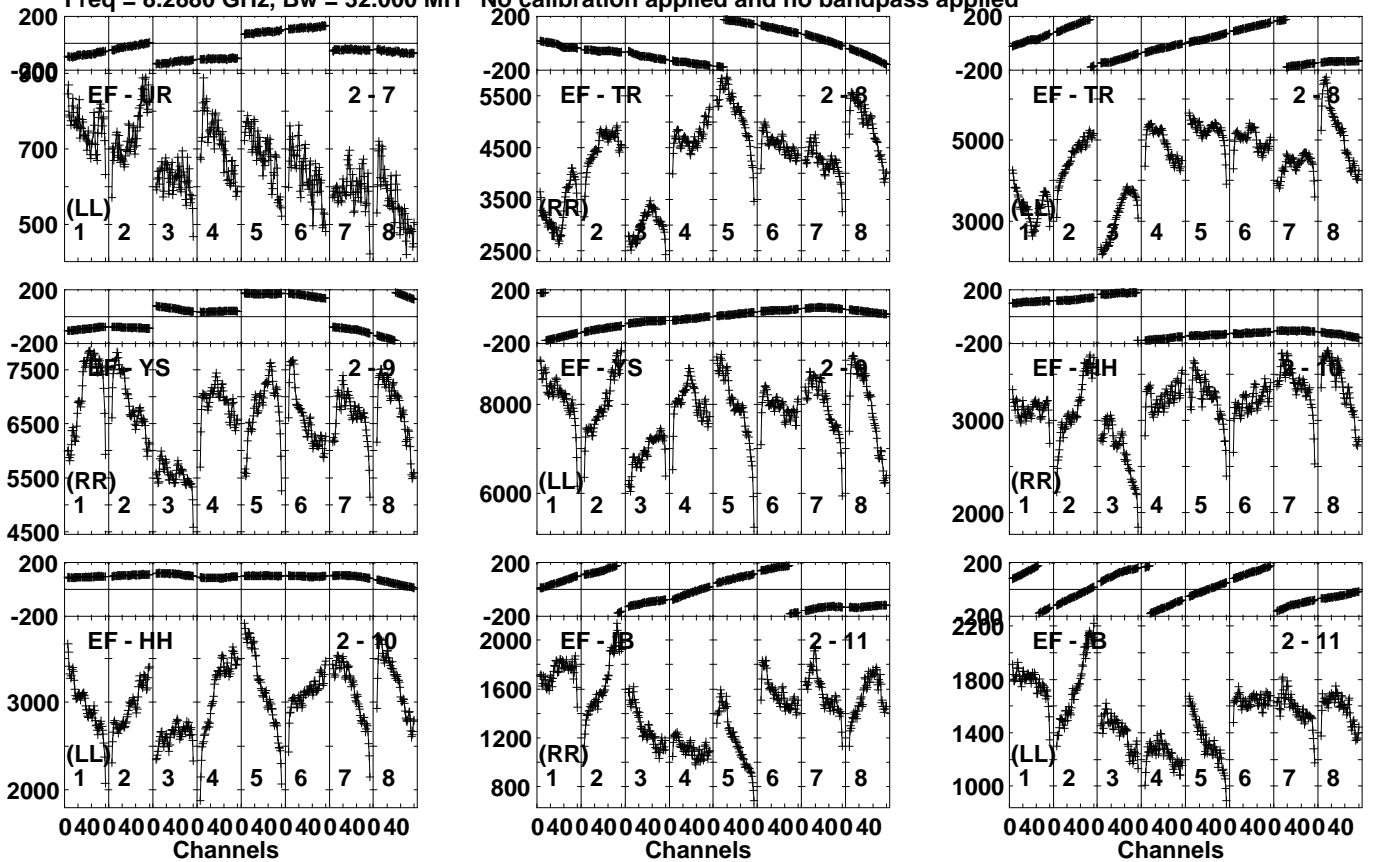
Lower frame: Micro Ampl Jy Top frame: Phas deg Vector averaged cross-power spectrum Several baselines displayed Timerange: 00/22:20:46 to 00/22:28:44
