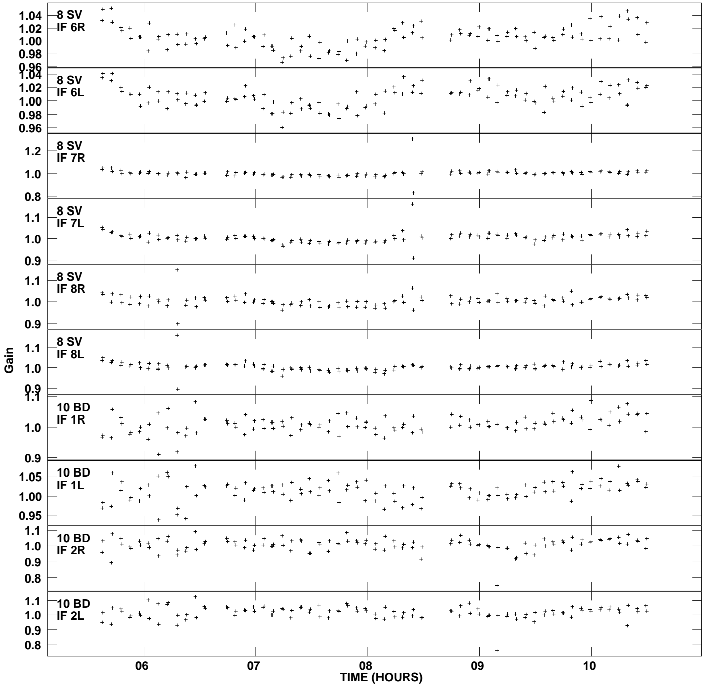
Plot file version 11 created 19-MAR-2014 11:10:21 Gain amp vs UTC time for J1426+3625.MULTI.1 SN 4 Rpol & Lpol IF 1 - 8
