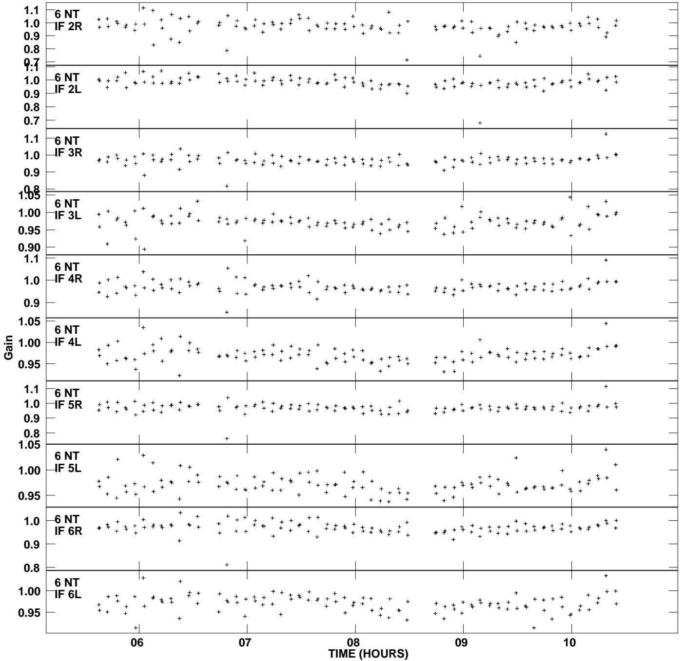
Plot file version 7 created 19-MAR-2014 11:10:21 Gain amp vs UTC time for J1426+3625.MULTI.1 SN 4 Rpol & Lpol IF 1 - 8
