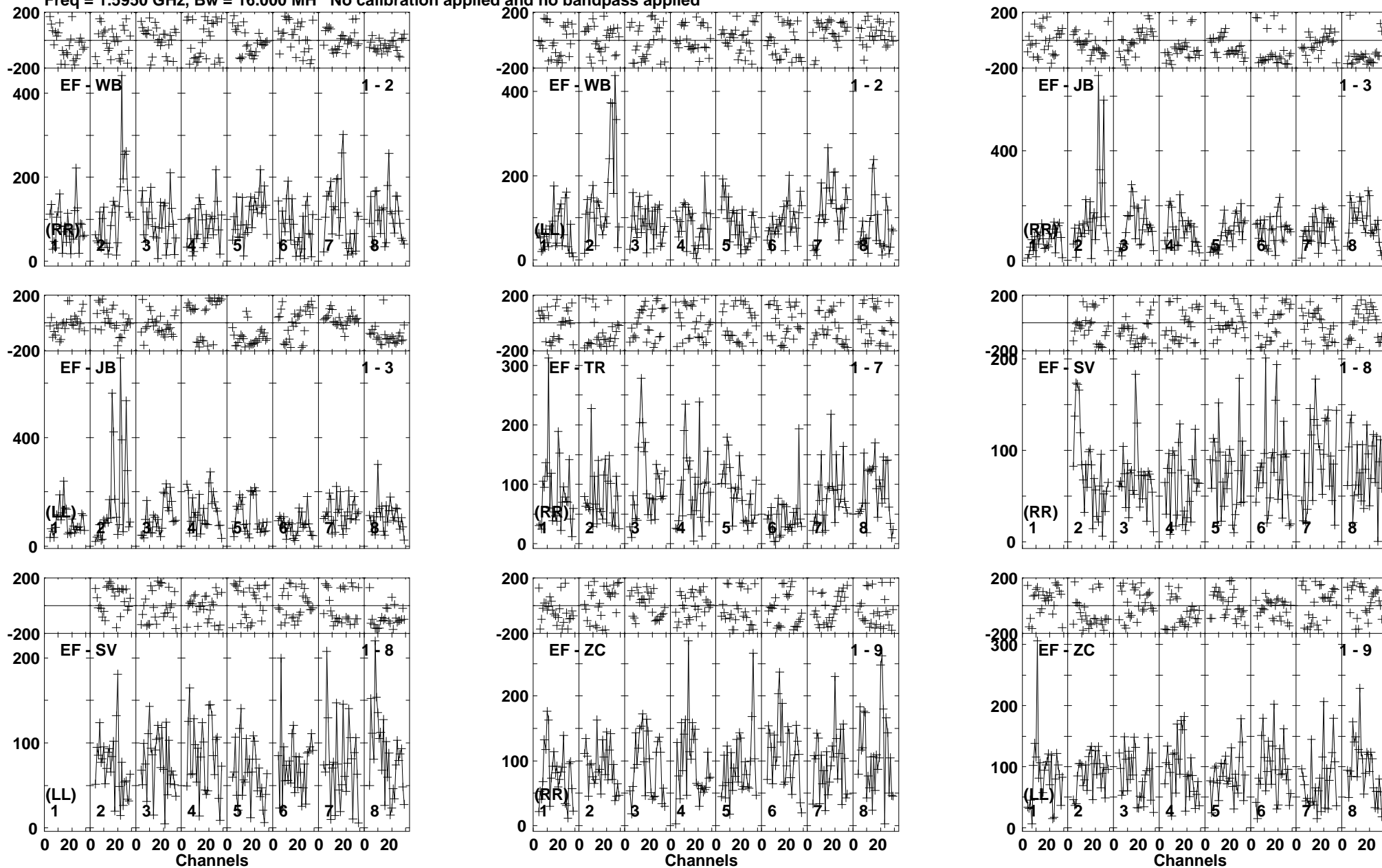
Lower frame: Micro Ampl Jy Top frame: Phas deg Vector averaged cross-power spectrum Baseline: EF (01) - WB (02) Timerange: 01/01:50:03 to 01/01:53:29
