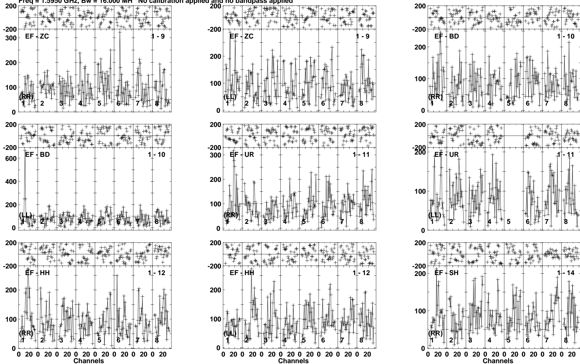
Lower frame: Micro Ampl Jy Top frame: Phas deg Vector averaged cross-power spectrum Baseline: EF (01) - ZC (09) Timerange: 01/00:14:47 to 01/00:18:09
