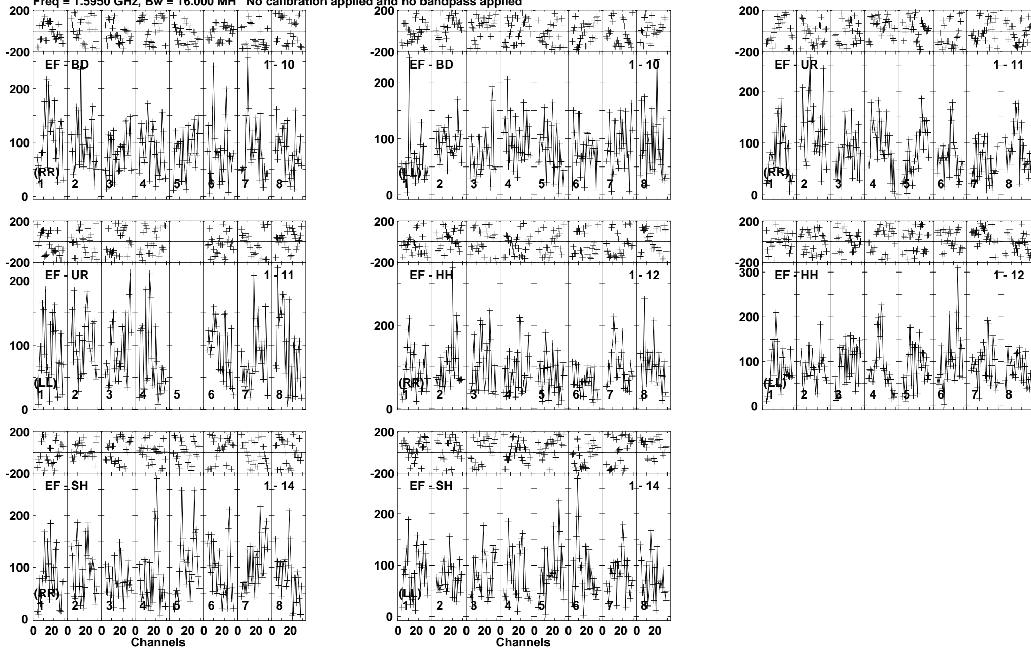
Lower frame: Micro Ampl Jy Top frame: Phas deg Vector averaged cross-power spectrum Baseline: EF (01) - BD (10) Timerange: 01/01:55:17 to 01/01:58:39
