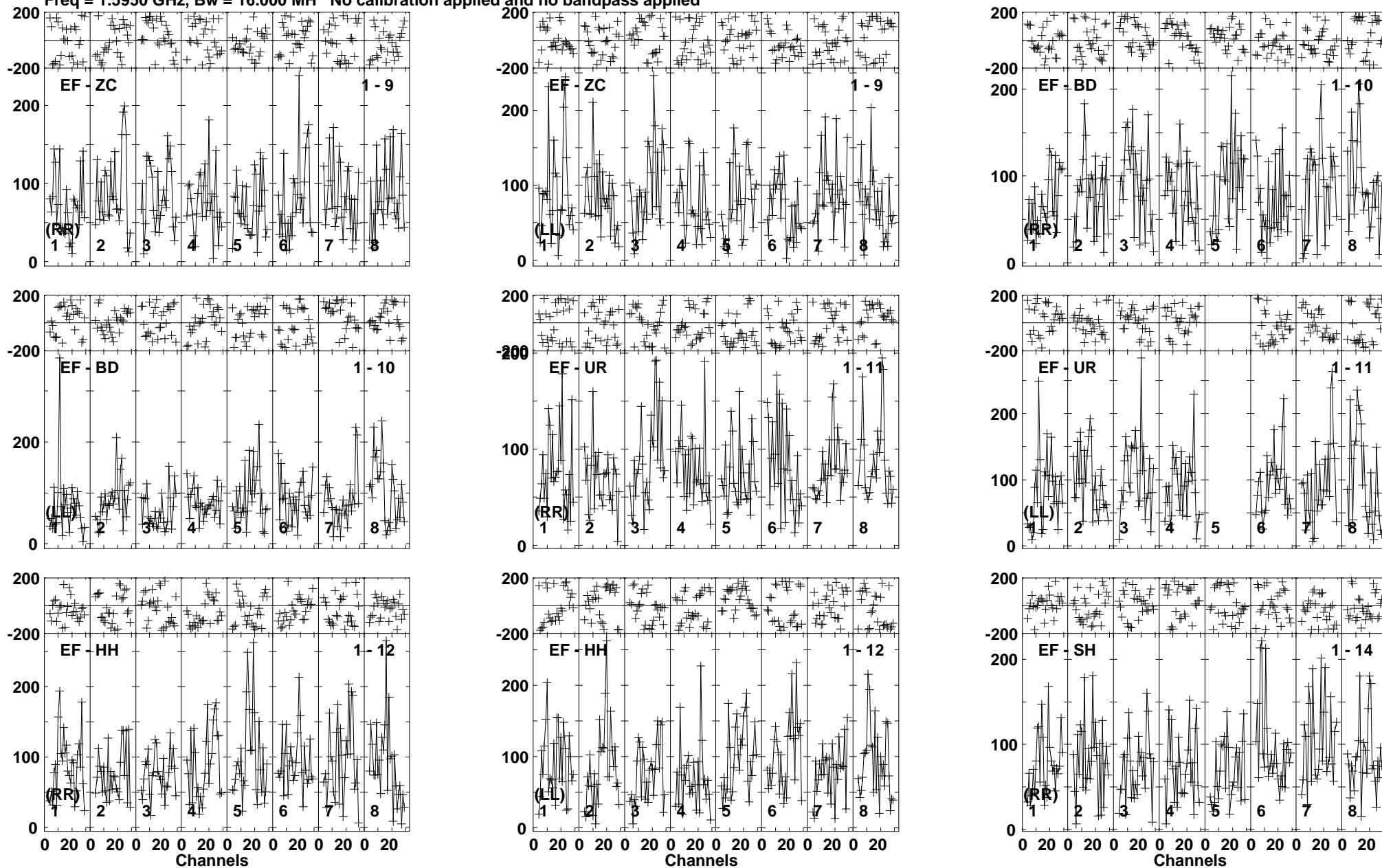
Lower frame: Micro Ampl Jy Top frame: Phas deg Vector averaged cross-power spectrum Baseline: EF (01) - ZC (09) Timerange: 00/22:28:28 to 00/22:31:48
