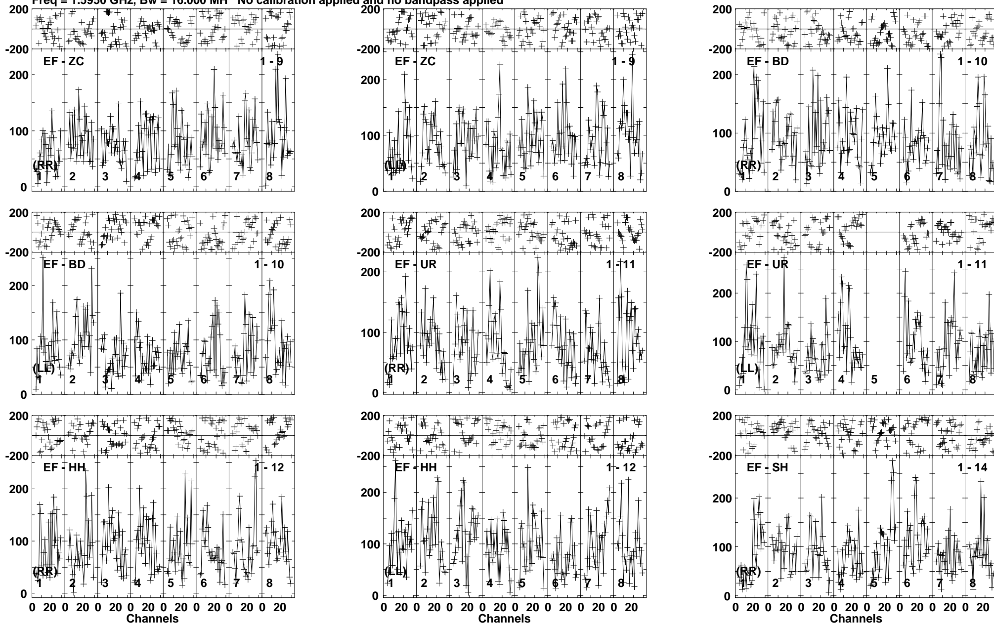
Lower frame: Micro Ampl Jy Top frame: Phas deg Vector averaged cross-power spectrum Baseline: EF (01) - ZC (09) Timerange: 00/23:54:47 to 00/23:58:09
