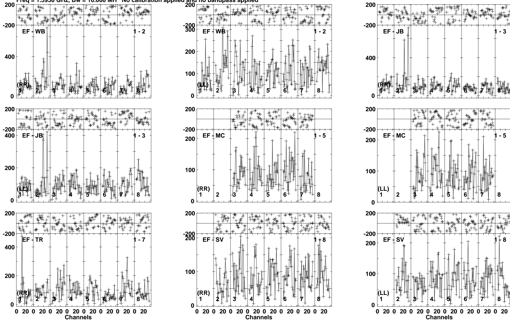
Lower frame: Micro Ampl Jy Top frame: Phas deg Vector averaged cross-power spectrum Baseline: EF (01) - WB (02) Timerange: 00/22:49:33 to 00/22:52:59
