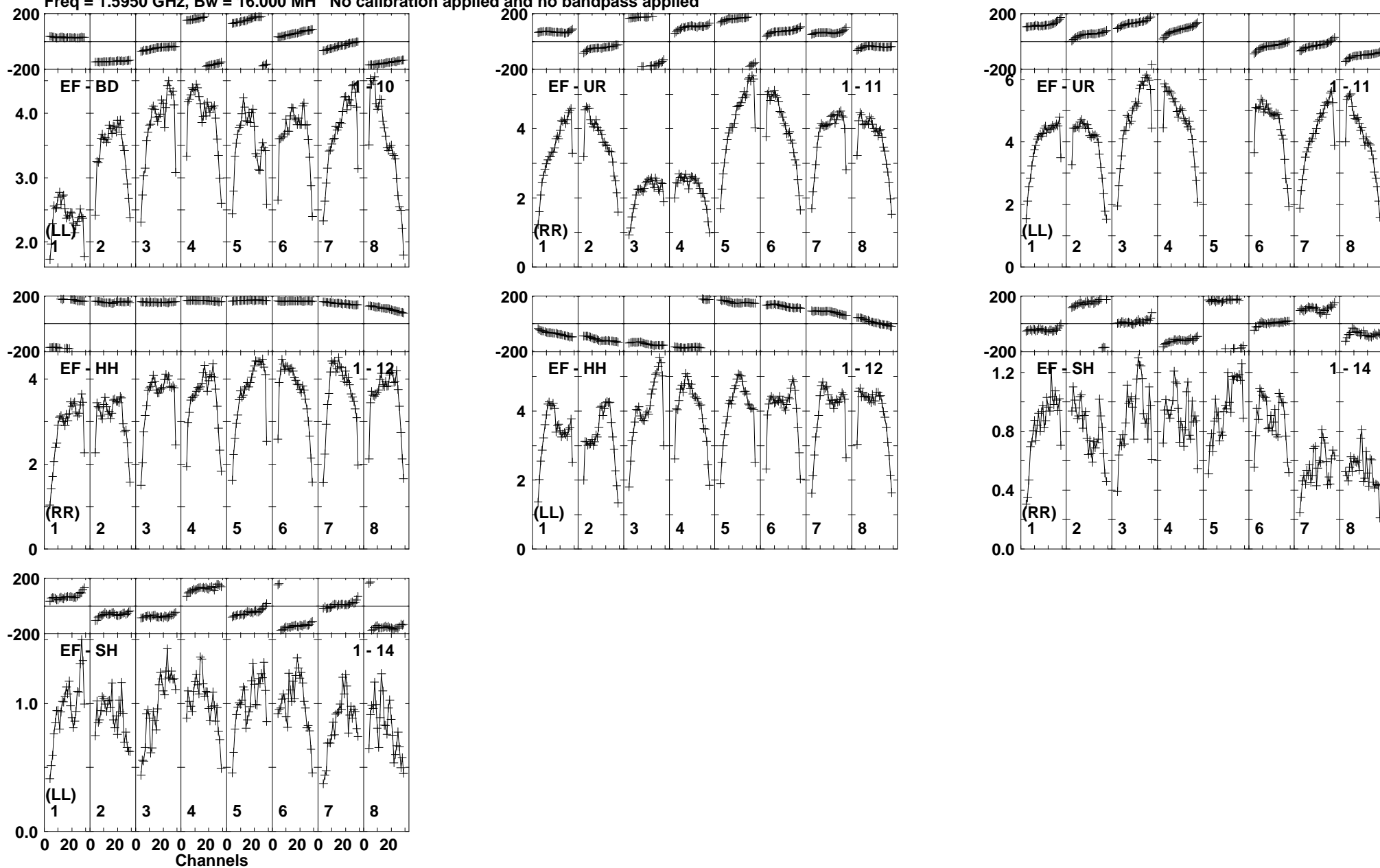
Lower frame: Milli Ampl Jy Top frame: Phas deg Vector averaged cross-power spectrum Baseline: EF (01) - BD (10) Timerange: 01/01:14:11 to 01/01:15:09
