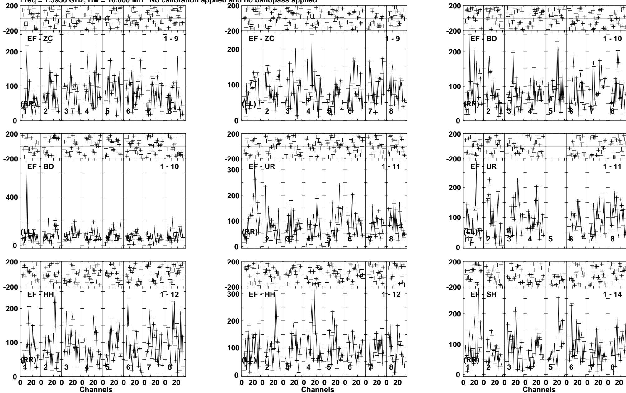
Lower frame: Micro Ampl Jy Top frame: Phas deg Vector averaged cross-power spectrum Baseline: EF (01) - ZC (09) Timerange: 00/23:49:33 to 00/23:52:59
