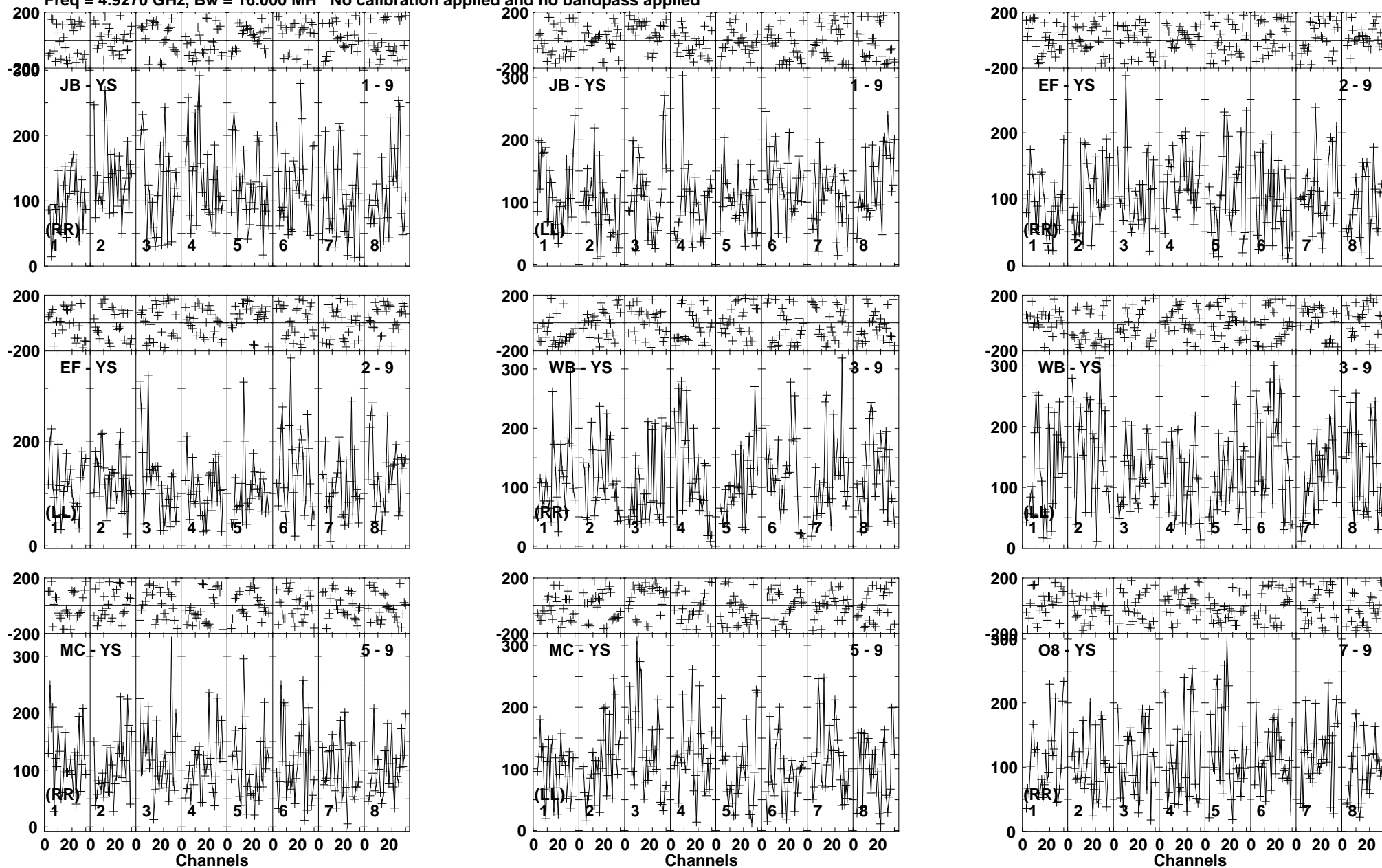
Lower frame: Micro Ampl Jy Top frame: Phas deg Vector averaged cross-power spectrum Baseline: JB (01) - YS (09) Timerange: 00/01:29:58 to 00/01:31:26
