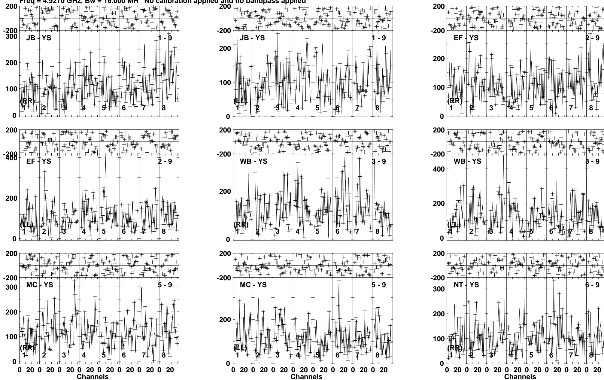
Lower frame: Micro Ampl Jy Top frame: Phas deg Vector averaged cross-power spectrum Baseline: JB (01) - YS (09) Timerange: 00/01:13:40 to 00/01:15:08
