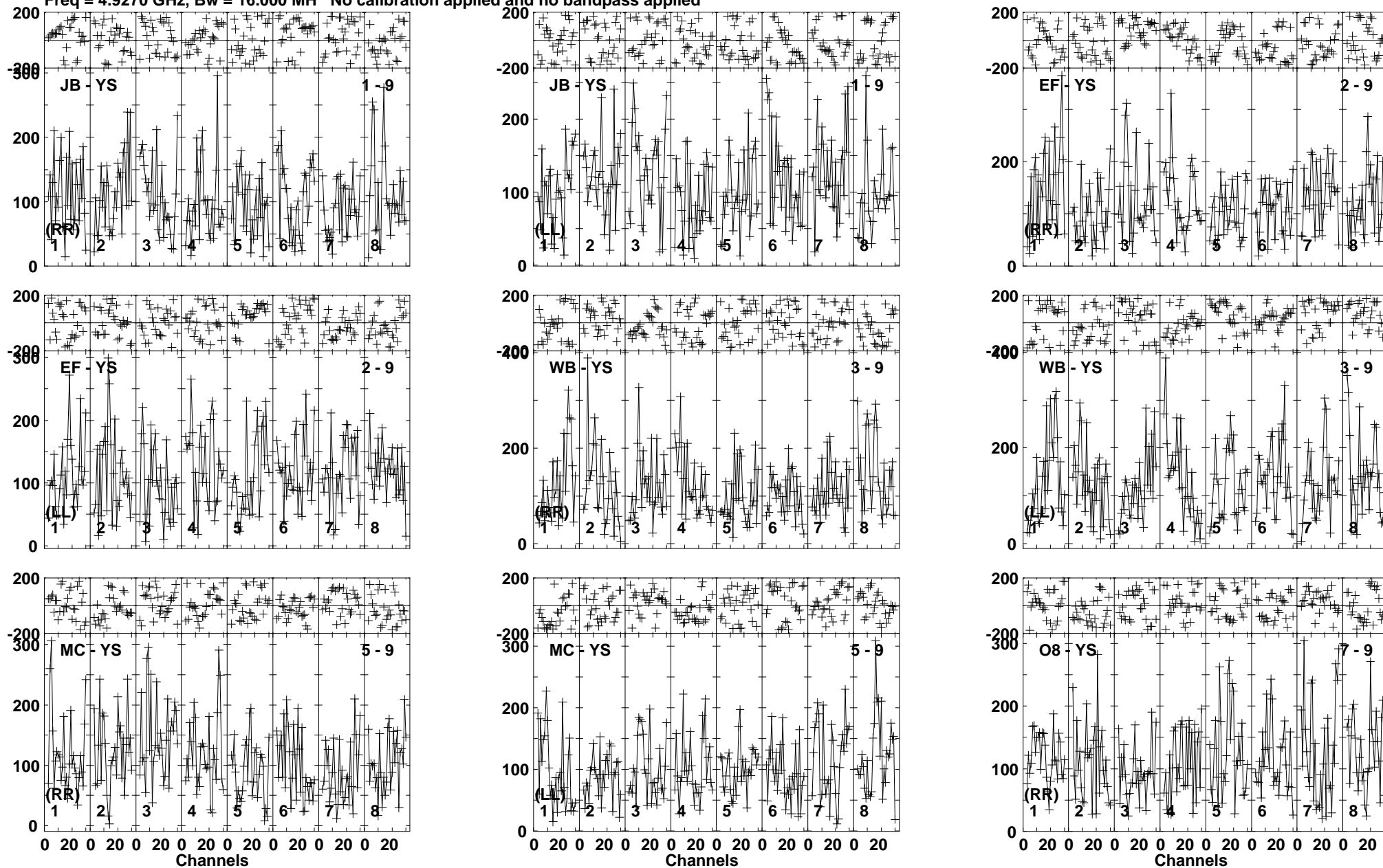
Lower frame: Micro Ampl Jy Top frame: Phas deg Vector averaged cross-power spectrum Baseline: JB (01) - YS (09) Timerange: 00/01:58:58 to 00/02:00:26
