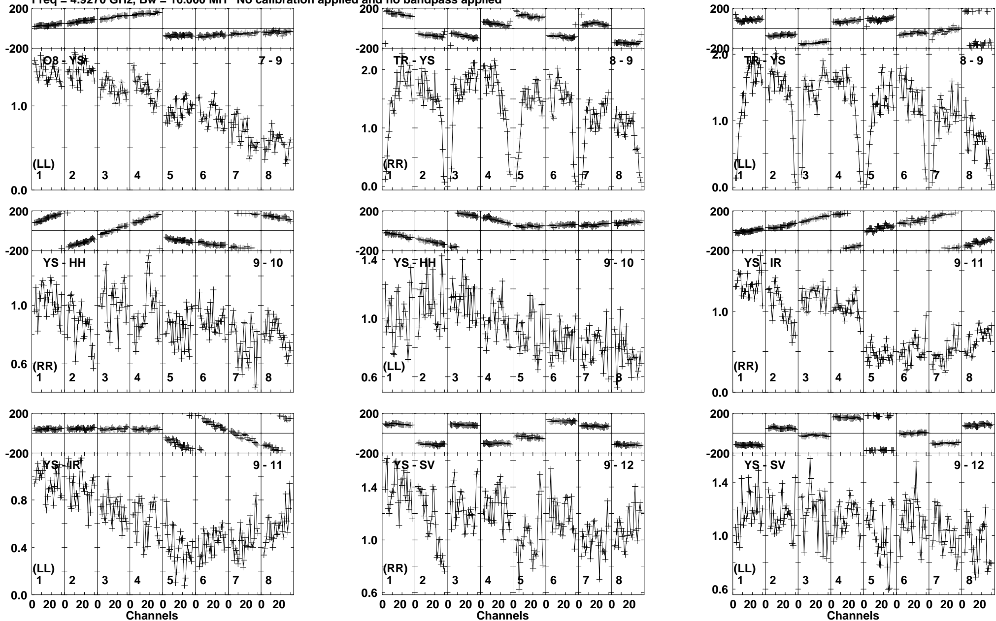
Lower frame: Milli Ampl Jy Top frame: Phas deg Vector averaged cross-power spectrum Baseline: O8 (07) - YS (09) Timerange: 00/01:48:07 to 00/01:48:49
