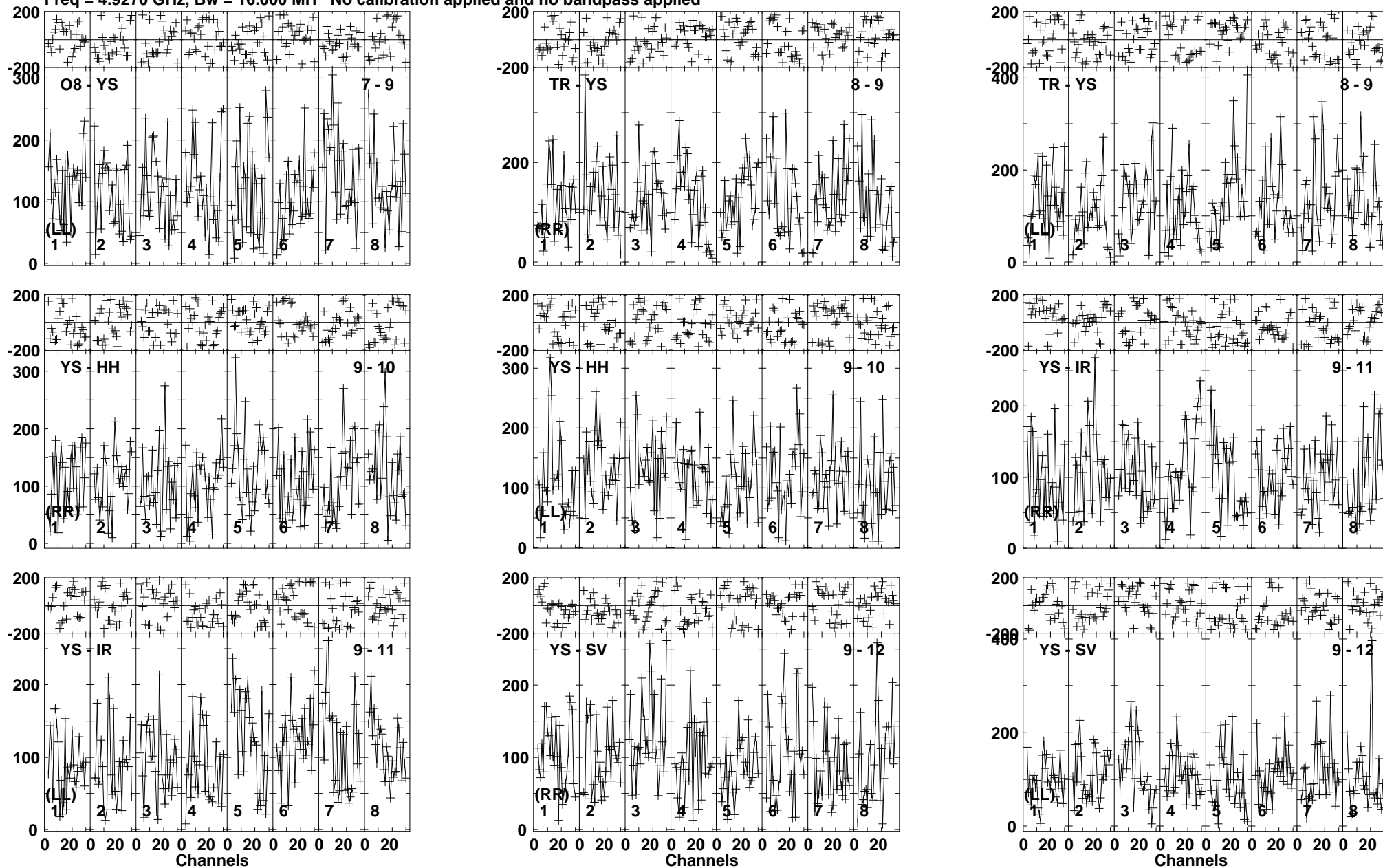
Lower frame: Micro Ampl Jy Top frame: Phas deg Vector averaged cross-power spectrum Baseline: O8 (07) - YS (09) Timerange: 00/01:58:58 to 00/02:00:26
