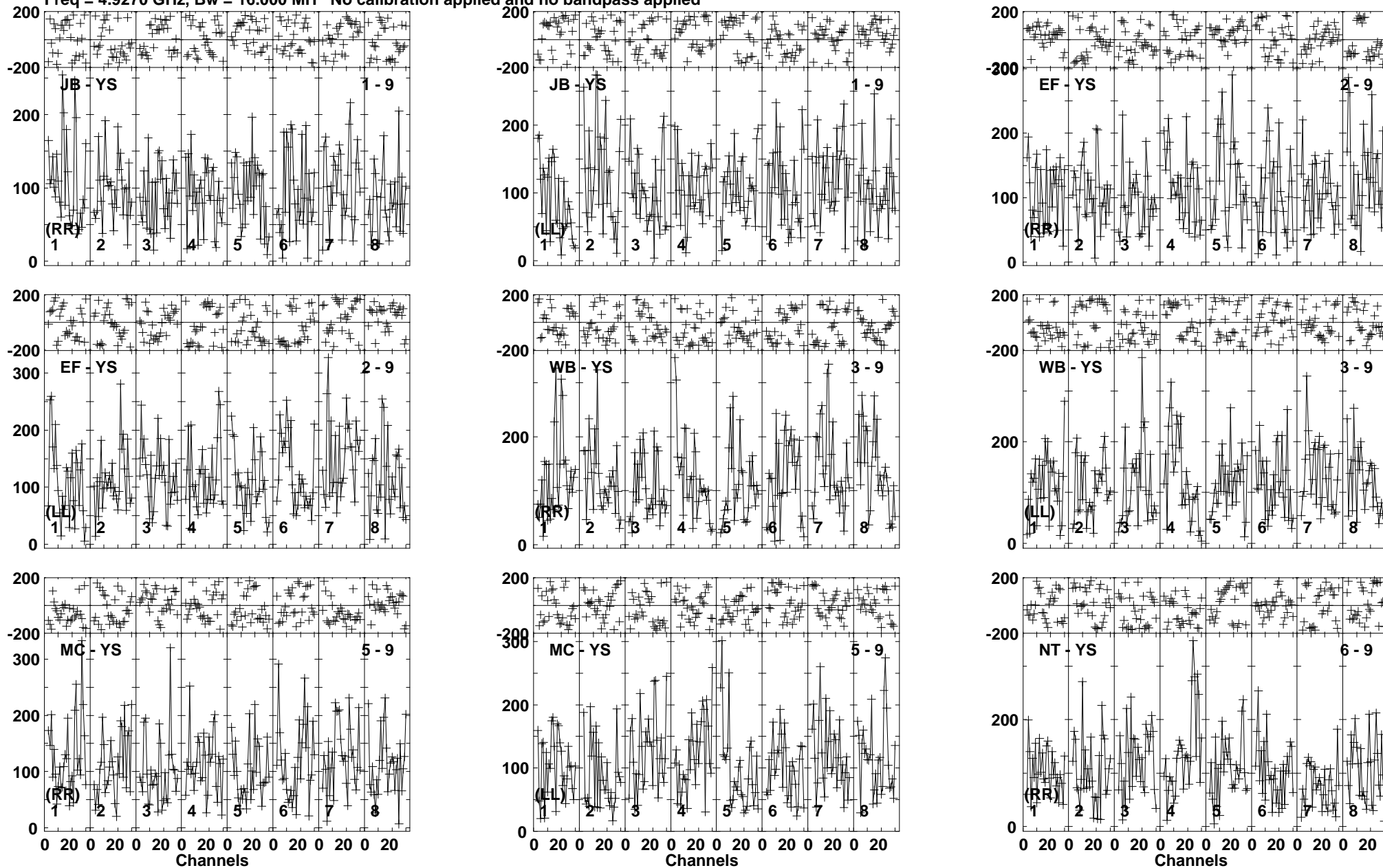
Lower frame: Micro Ampl Jy Top frame: Phas deg Vector averaged cross-power spectrum Baseline: JB (01) - YS (09) Timerange: 00/01:20:01 to 00/01:21:29
