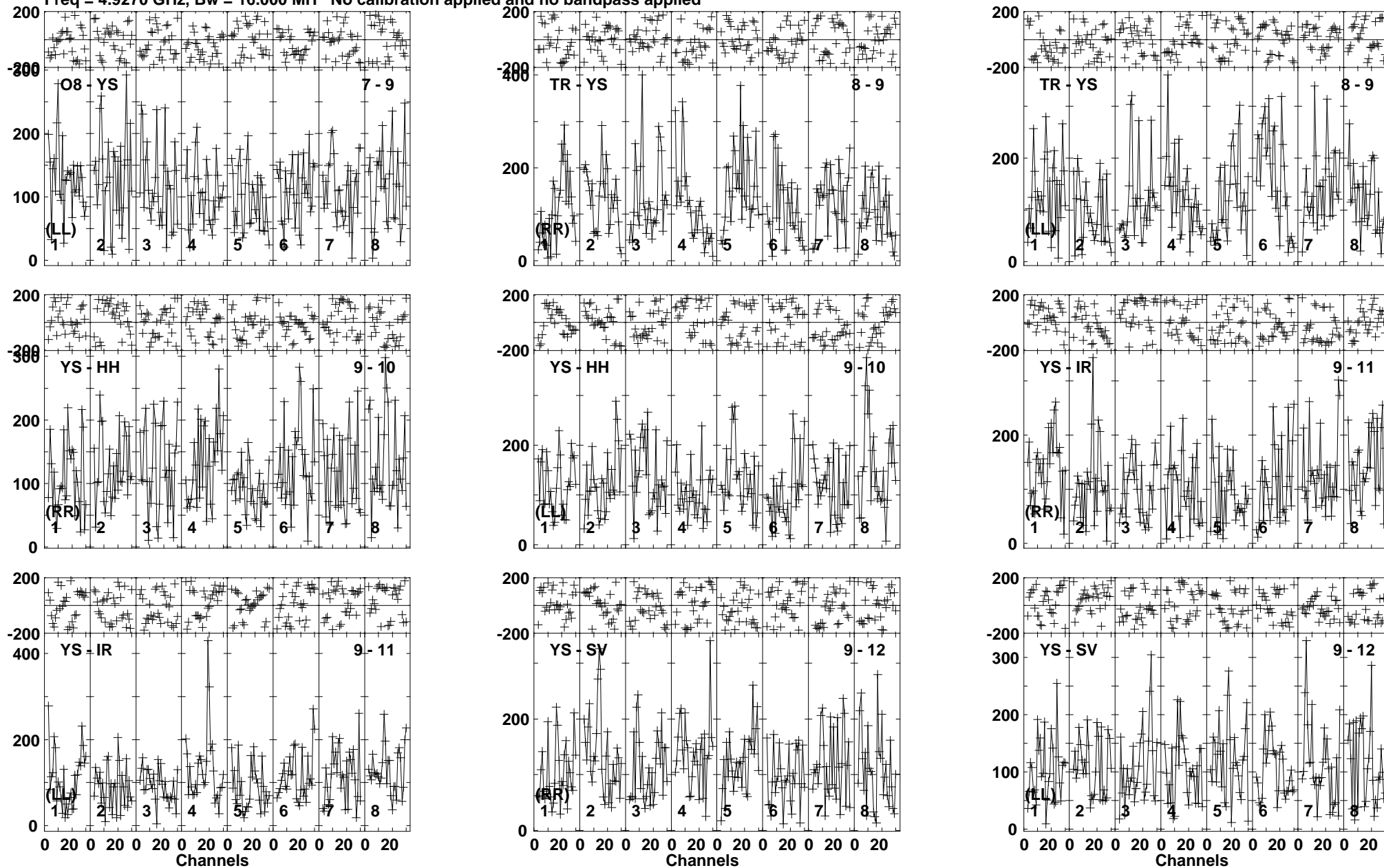
Lower frame: Micro Ampl Jy Top frame: Phas deg Vector averaged cross-power spectrum Baseline: O8 (07) - YS (09) Timerange: 00/02:37:56 to 00/02:39:24
