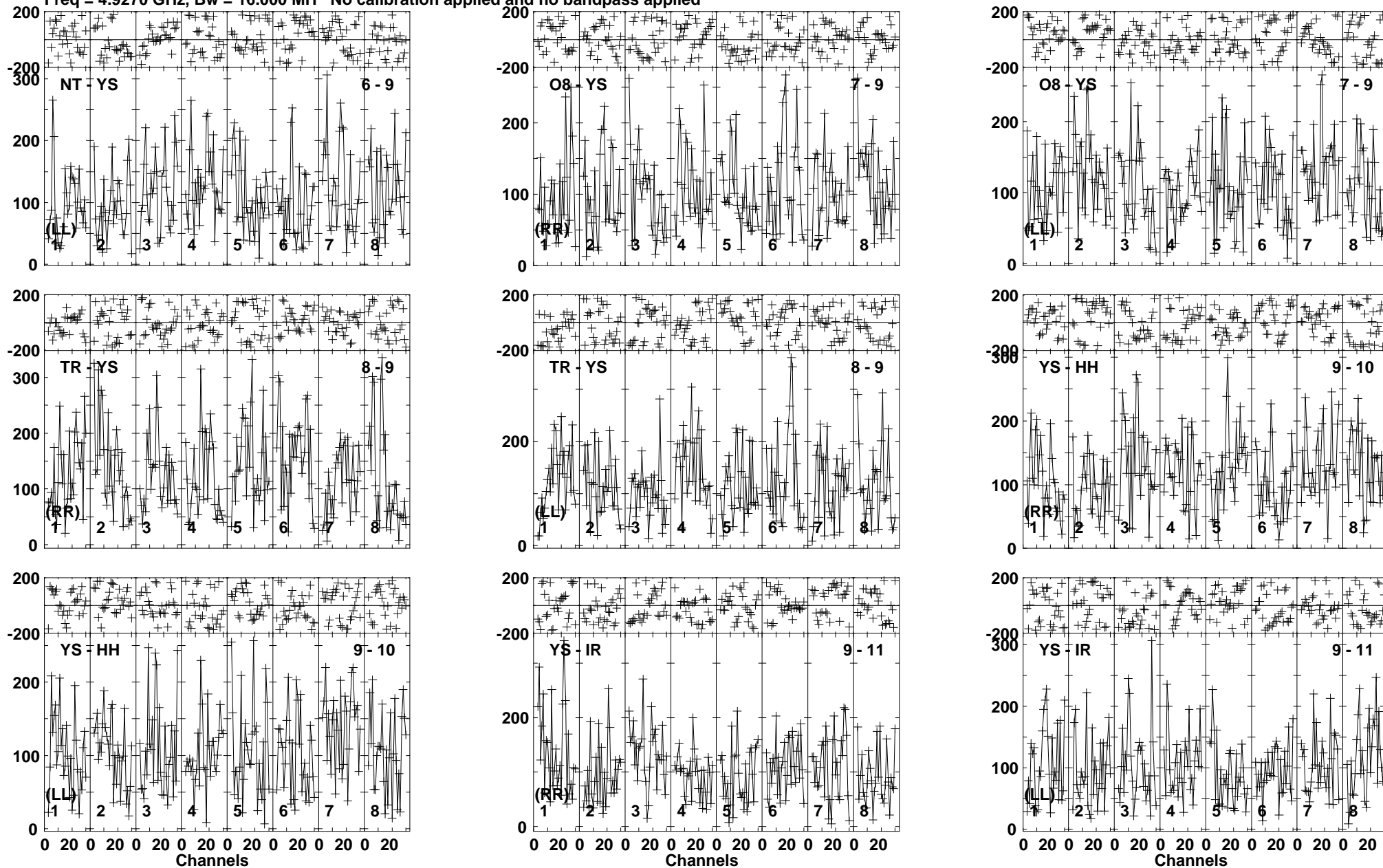
Lower frame: Micro Ampl Jy Top frame: Phas deg Vector averaged cross-power spectrum Baseline: NT (06) - YS (09) Timerange: 00/01:23:24 to 00/01:24:52
