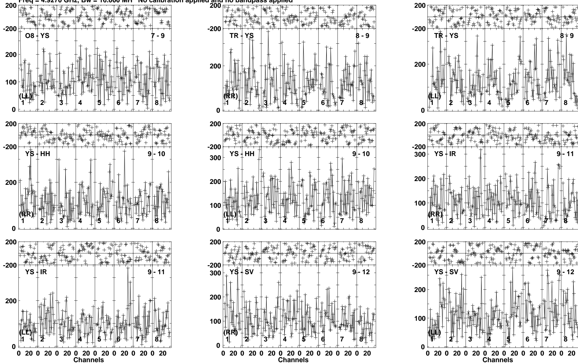
Lower frame: Micro Ampl Jy Top frame: Phas deg Vector averaged cross-power spectrum Baseline: O8 (07) - YS (09) Timerange: 00/01:33:09 to 00/01:34:37
