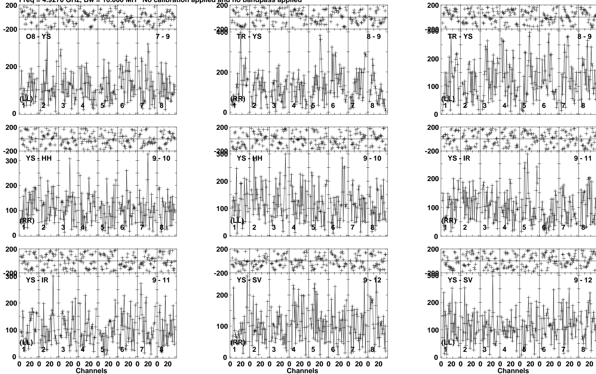
Lower frame: Micro Ampl Jy Top frame: Phas deg Vector averaged cross-power spectrum Baseline: O8 (07) - YS (09) Timerange: 00/01:39:30 to 00/01:40:58
