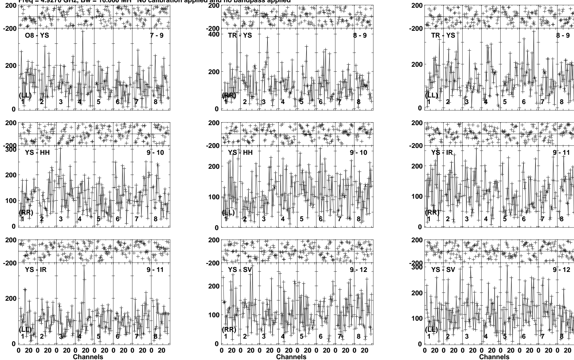
Lower frame: Micro Ampl Jy Top frame: Phas deg Vector average cross-power spectrum Baseline: O8 (07) - YS (09) Timerange: 00/01:49:27 to 00/01:50:55
