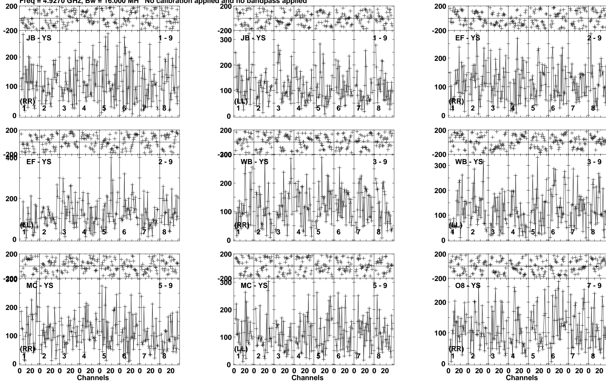
Lower frame: Micro Ampl Jy Top frame: Phas deg Vector averaged cross-power spectrum Baseline: JB (01) - YS (09) Timerange: 00/01:33:09 to 00/01:34:37
