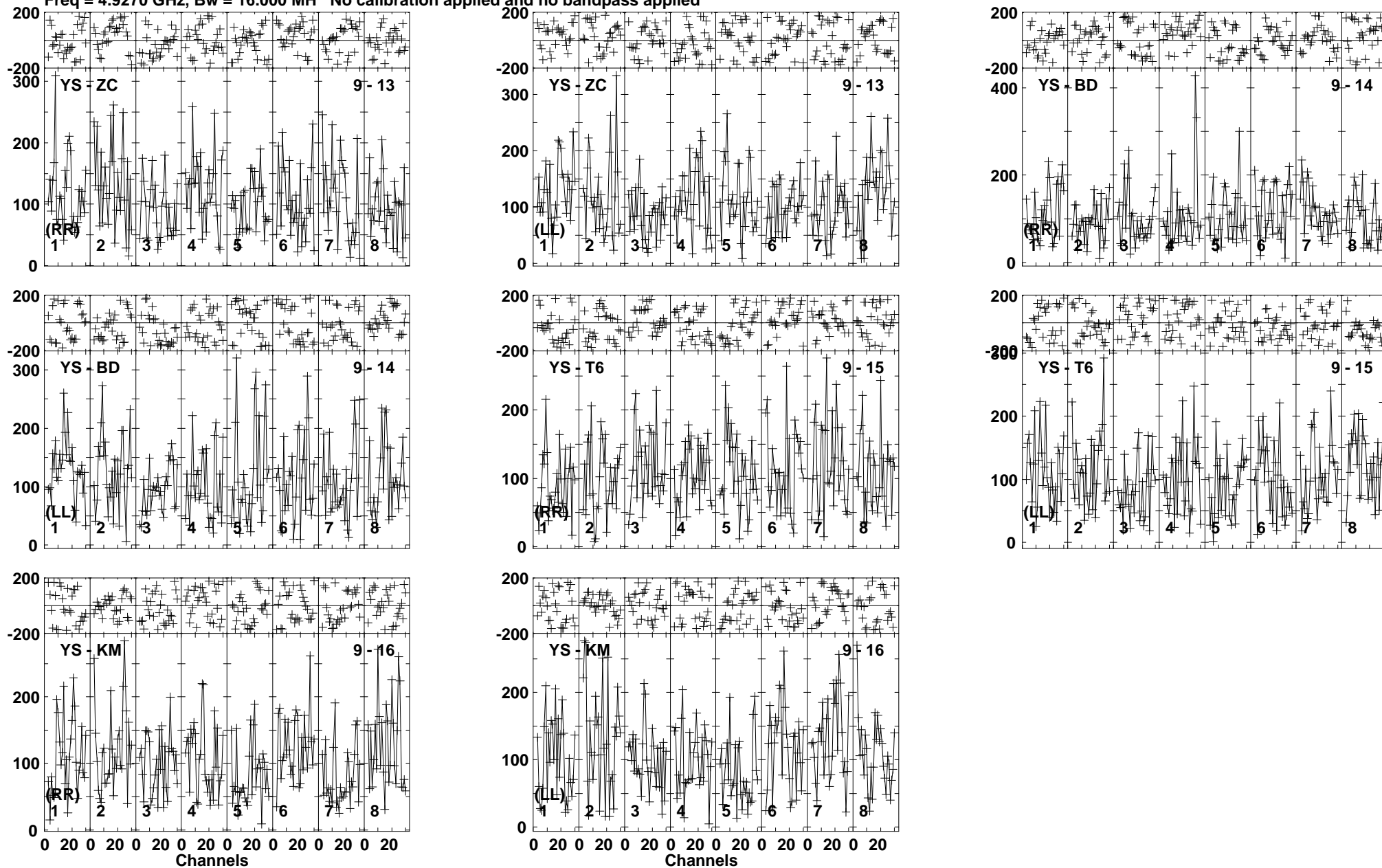
Lower frame: Micro Ampl Jy Top frame: Phas deg Vector averaged cross-power spectrum Baseline: YS (09) - ZC (13) Timerange: 00/01:39:30 to 00/01:40:58
