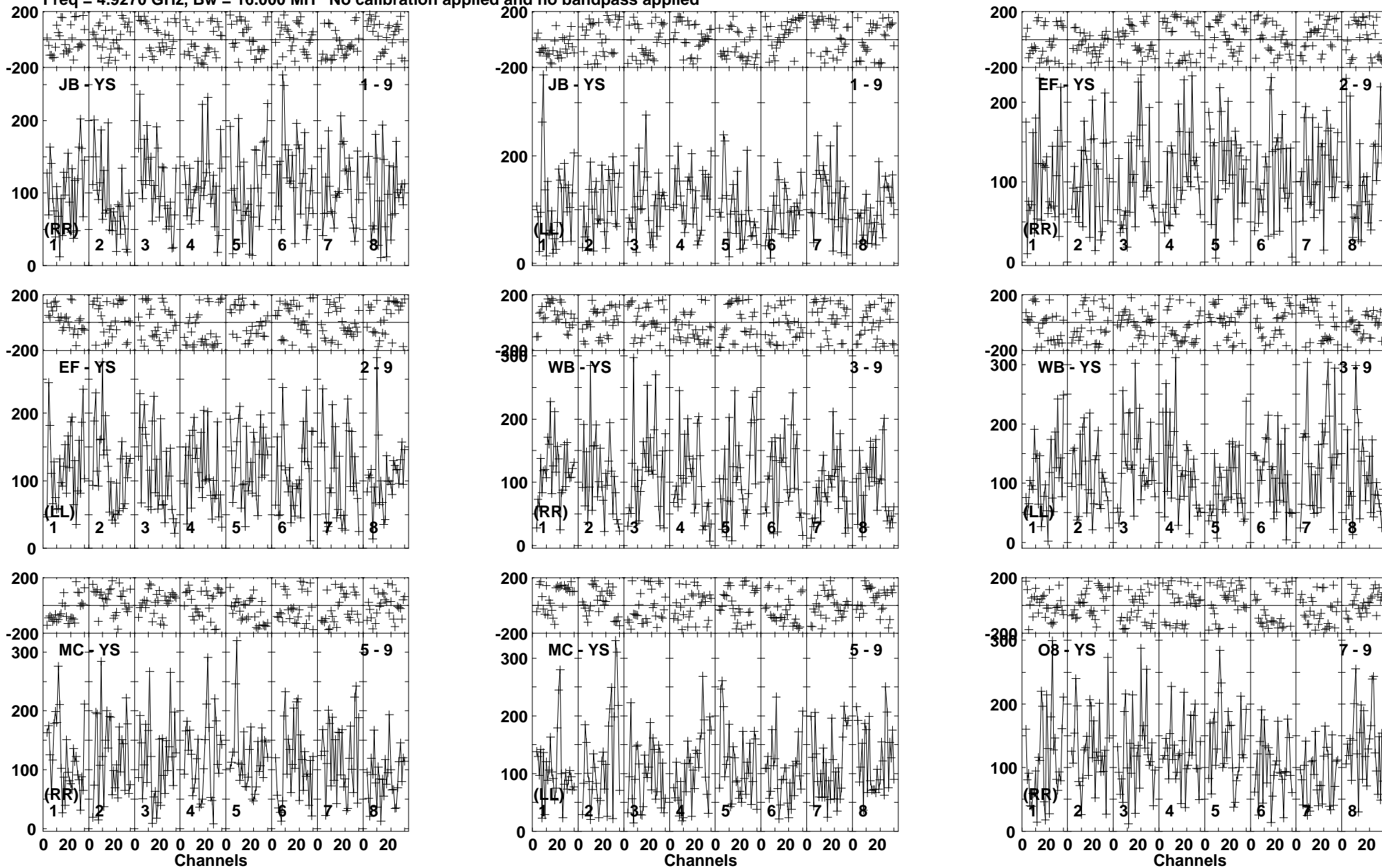
Lower frame: Micro Ampl Jy Top frame: Phas deg Vector averaged cross-power spectrum Baseline: JB (01) - YS (09) Timerange: 00/01:42:40 to 00/01:44:08
