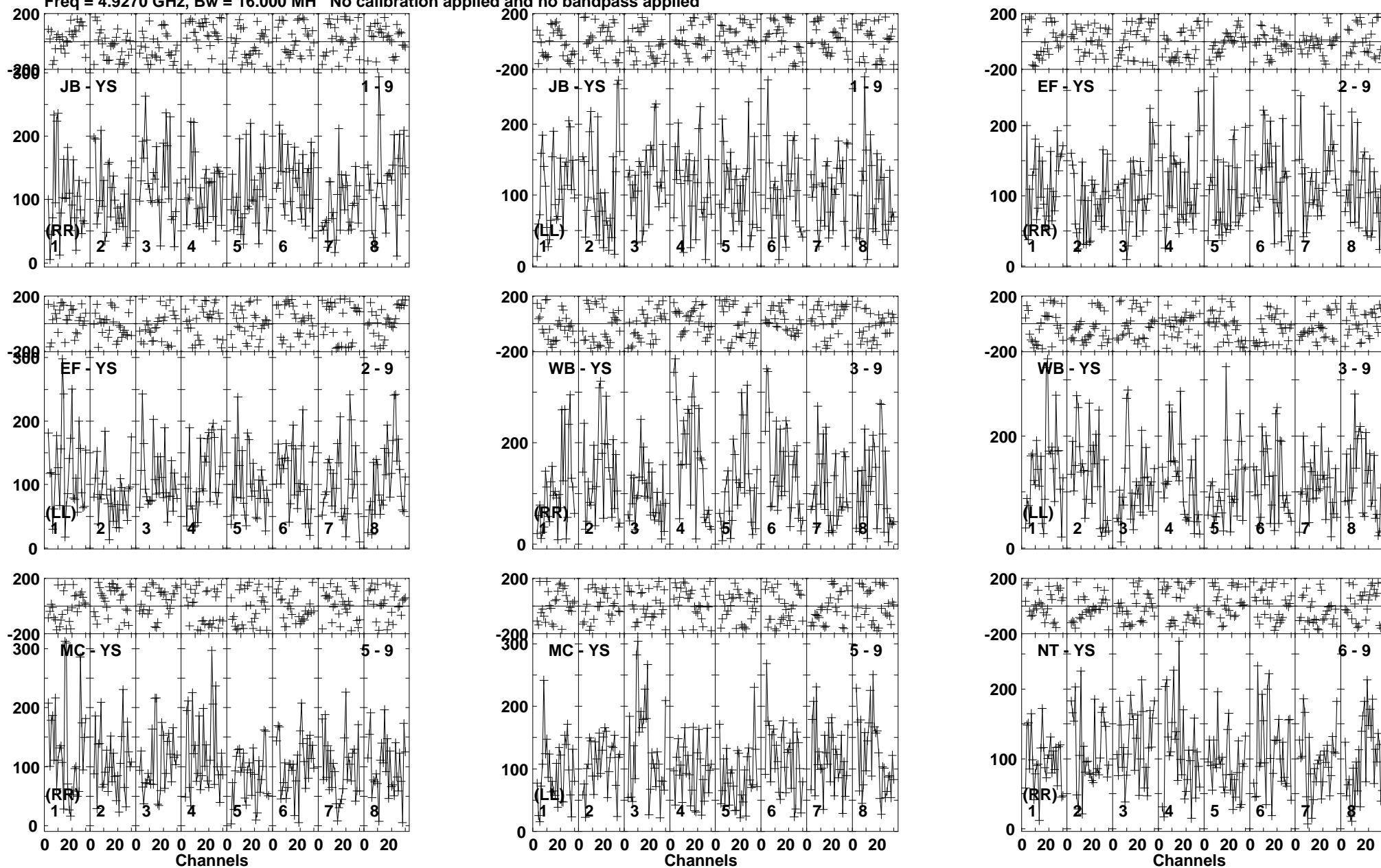
Lower frame: Micro Ampl Jy Top frame: Phas deg Vector averaged cross-power spectrum Baseline: JB (01) - YS (09) Timerange: 00/01:10:29 to 00/01:11:57
