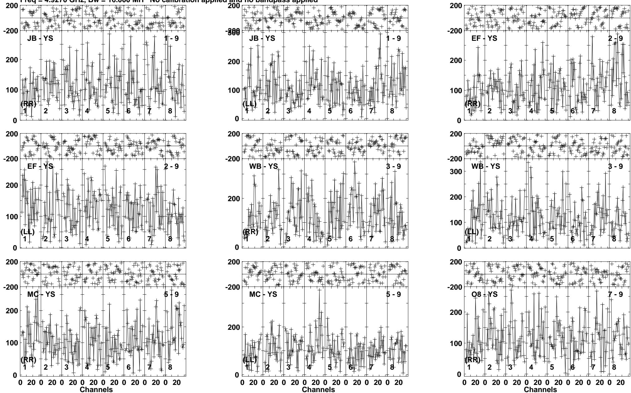
Lower frame: Micro Ampl Jy Top frame: Phas deg Vector averaged cross-power spectrum Baseline: JB (01) - YS (09) Timerange: 00/01:39:30 to 00/01:40:58
