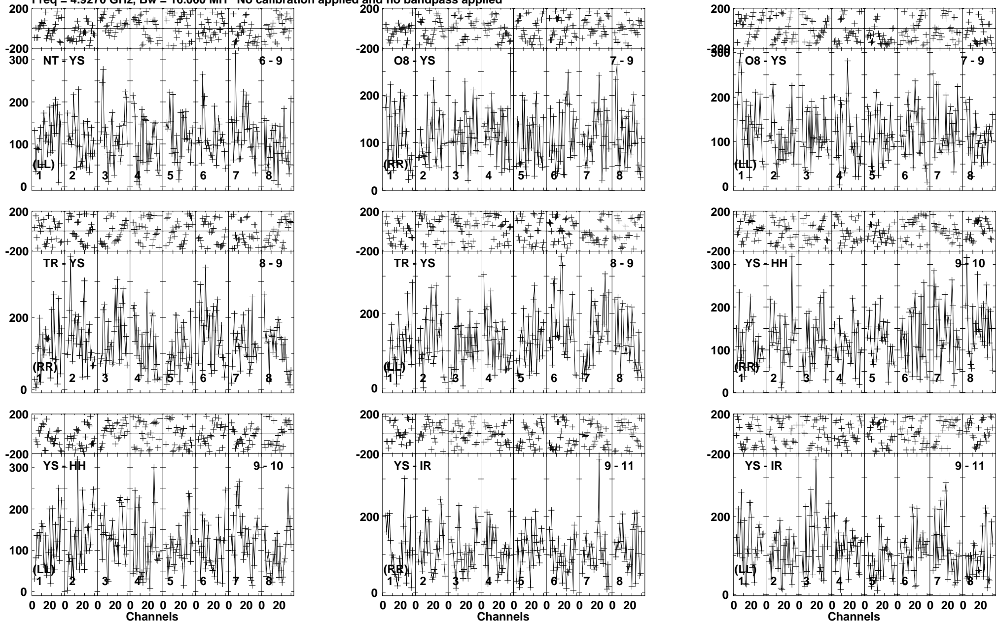
Lower frame: Micro Ampl Jy Top frame: Phas deg Vector averaged cross-power spectrum Baseline: NT (06) - YS (09) Timerange: 00/01:20:01 to 00/01:21:29
