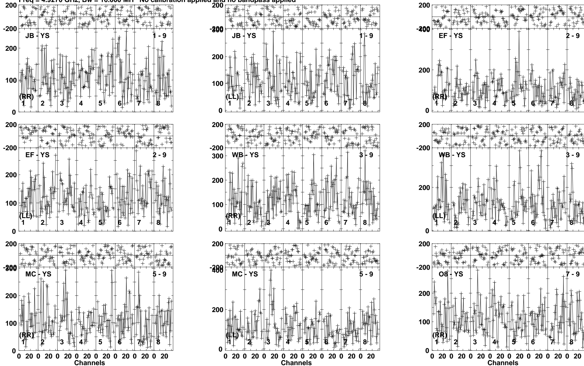
Lower frame: Micro Ampl Jy Top frame: Phas deg Vector averaged cross-power spectrum Baseline: JB (01) - YS (09) Timerange: 00/02:02:09 to 00/02:03:37
