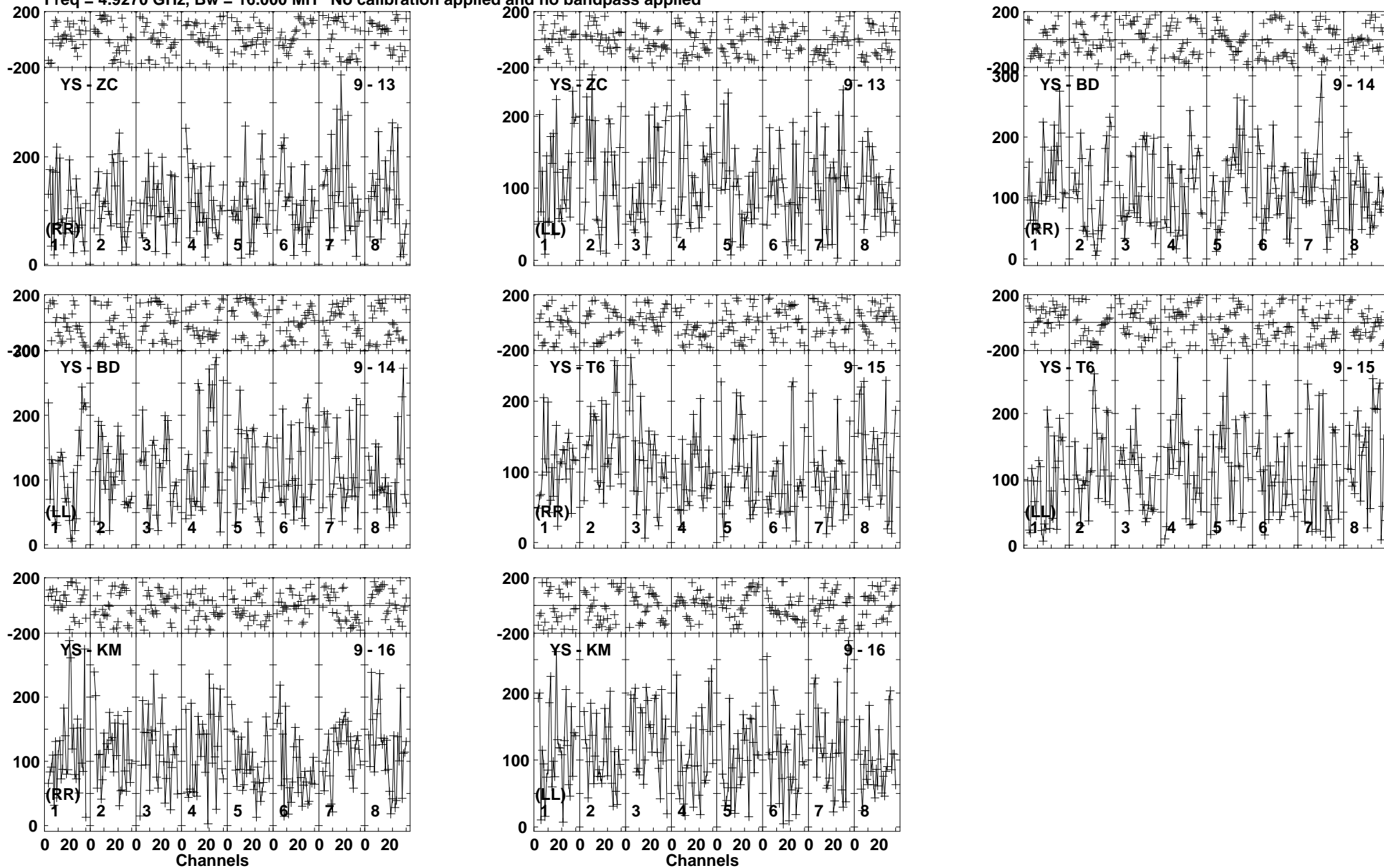
Lower frame: Micro Ampl Jy Top frame: Phas deg Vector averaged cross-power spectrum Baseline: YS (09) - ZC (13) Timerange: 00/02:47:28 to 00/02:48:56
