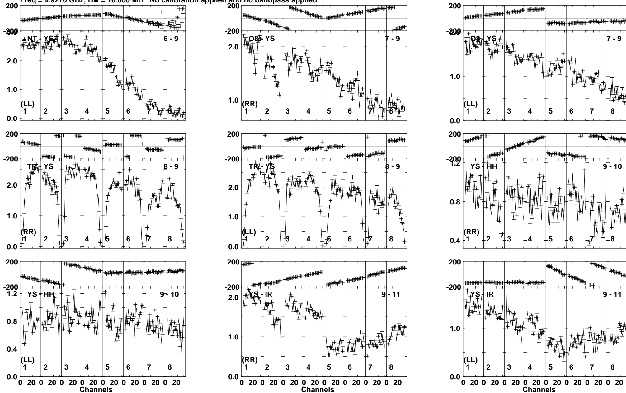
Lower frame: Milli Ampl Jy Top frame: Phas deg Vector averaged cross-power spectrum Baseline: NT (06) - YS (09) Timerange: 00/01:15:38 to 00/01:16:20
