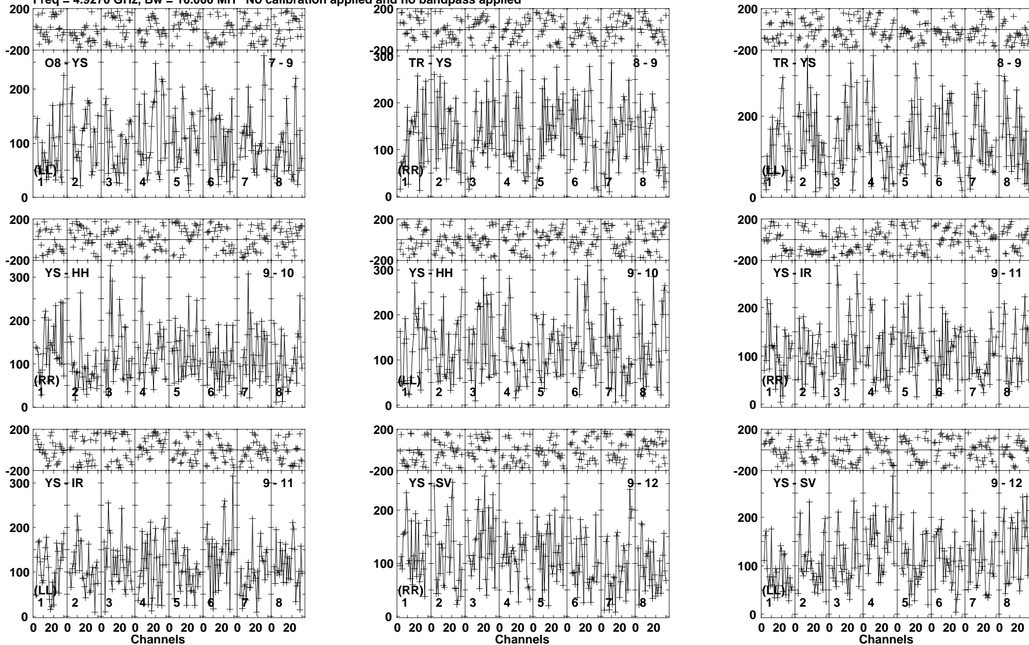
Lower frame: Micro Ampl Jy Top frame: Phas deg Vector averaged cross-power spectrum Baseline: O8 (07) - YS (09) Timerange: 00/01:52:37 to 00/01:54:05
