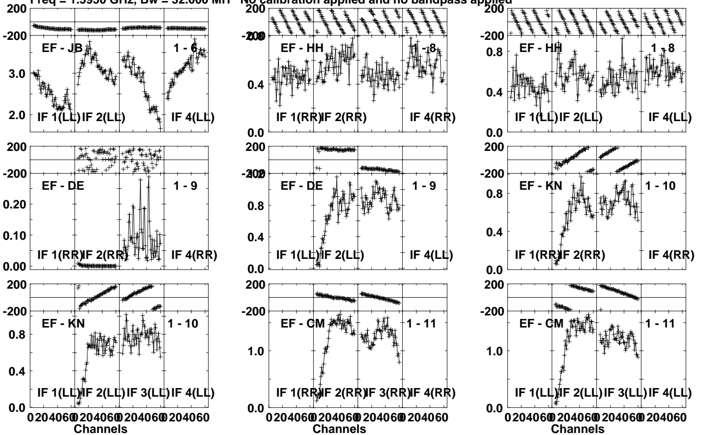
Lower frame: Milli Ampl Jy Top frame: Phas deg Vector averaged cross-power spectrum Several baselines displayed Timerange: 00/22:44:31 to 00/22:45:59
