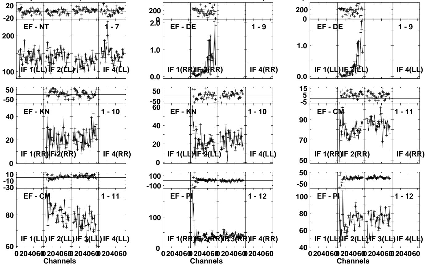
Lower frame: Milli Ampl Jy Top frame: Phas deg Vector averaged cross-power spectrum Several baselines displayed Timerange: 00/14:21:21 to 00/14:22:49
