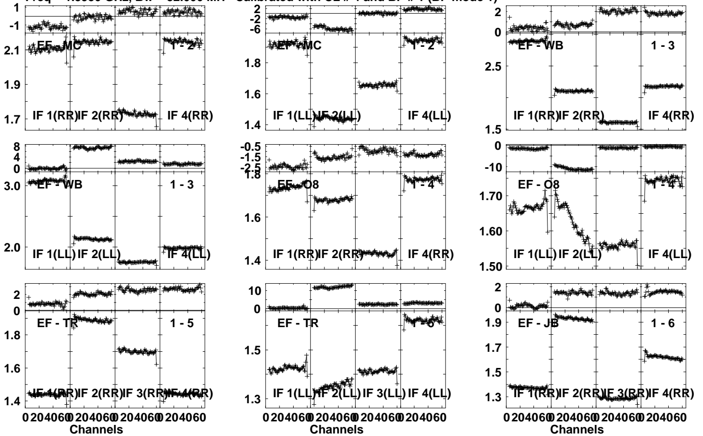
Lower frame: Ampl Jy Top frame: Phas deg Vector averaged cross-power spectrum Several baselines displayed Timerange: 00/15:53:21 to 00/15:59:19
