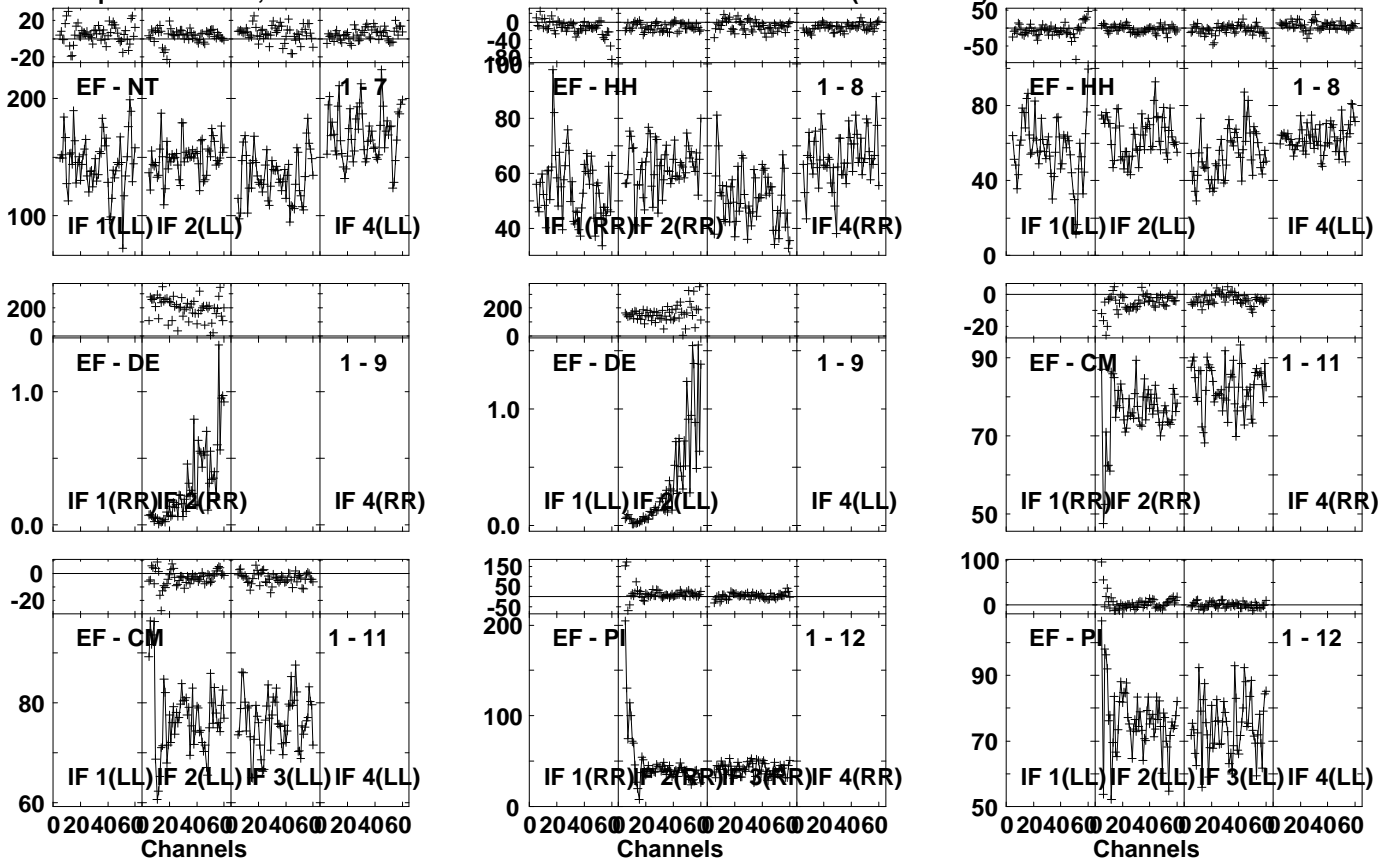
Lower frame: Milli Ampl Jy Top frame: Phas deg Vector averaged cross-power spectrum Several baselines displayed Timerange: 00/13:18:41 to 00/13:20:09
