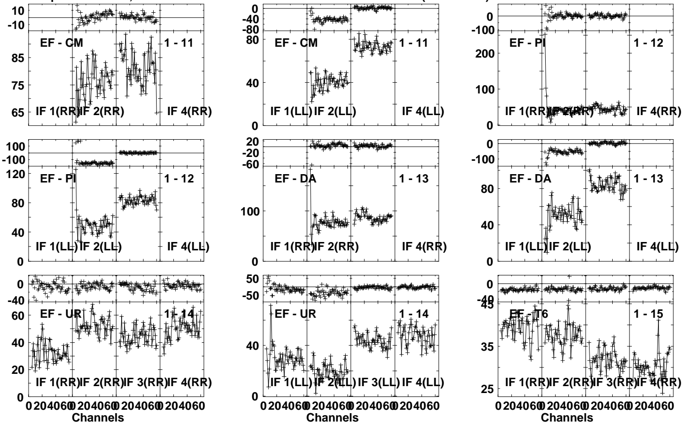
Lower frame: Milli Ampl Jy Top frame: Phas deg Vector averaged cross-power spectrum Several baselines displayed Timerange: 00/07:48:21 to 00/07:49:49
