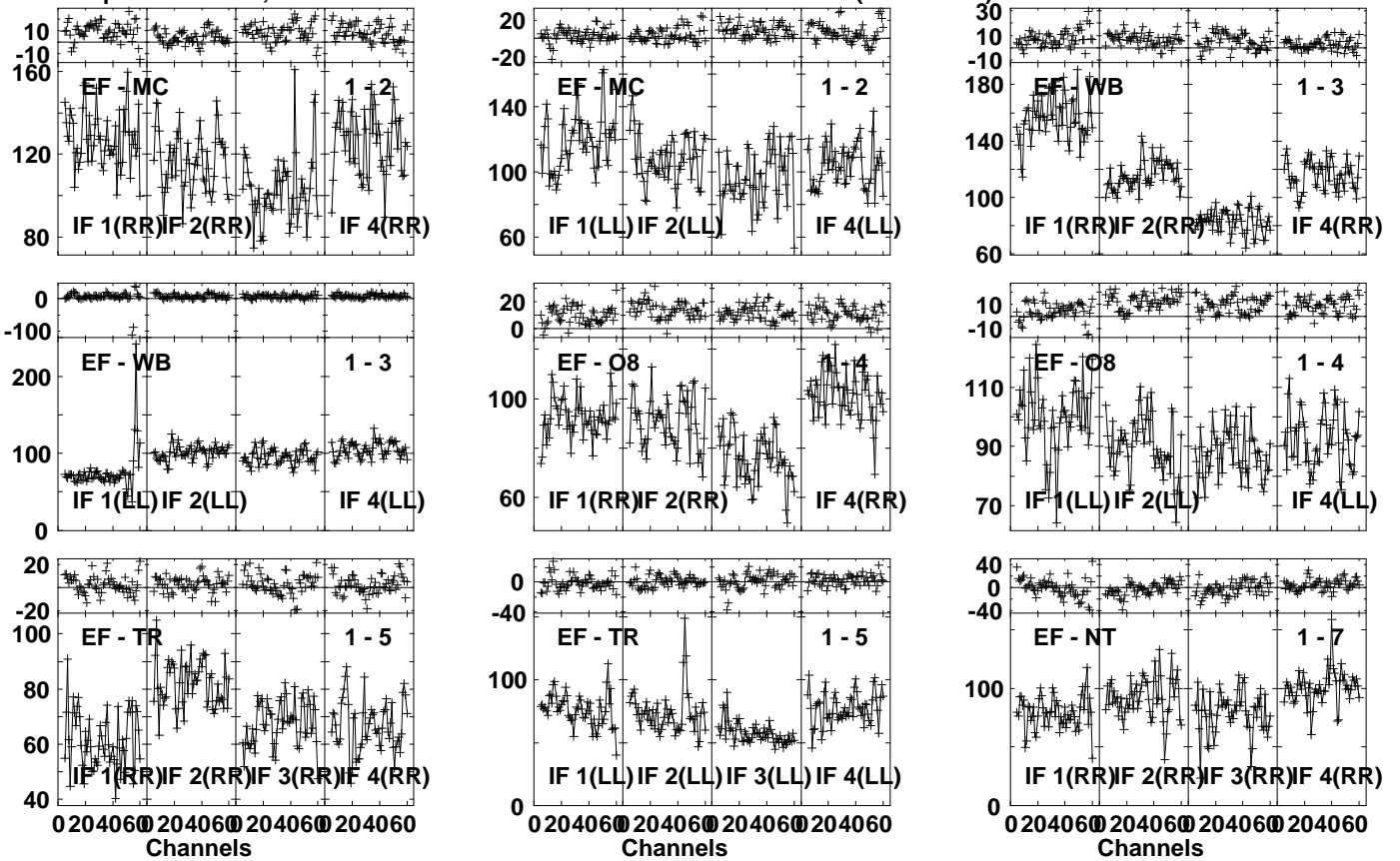
Lower frame: Milli Ampl Jy Top frame: Phas deg Vector averaged cross-power spectrum Several baselines displayed Timerange: 00/09:11:11 to 00/09:12:39
