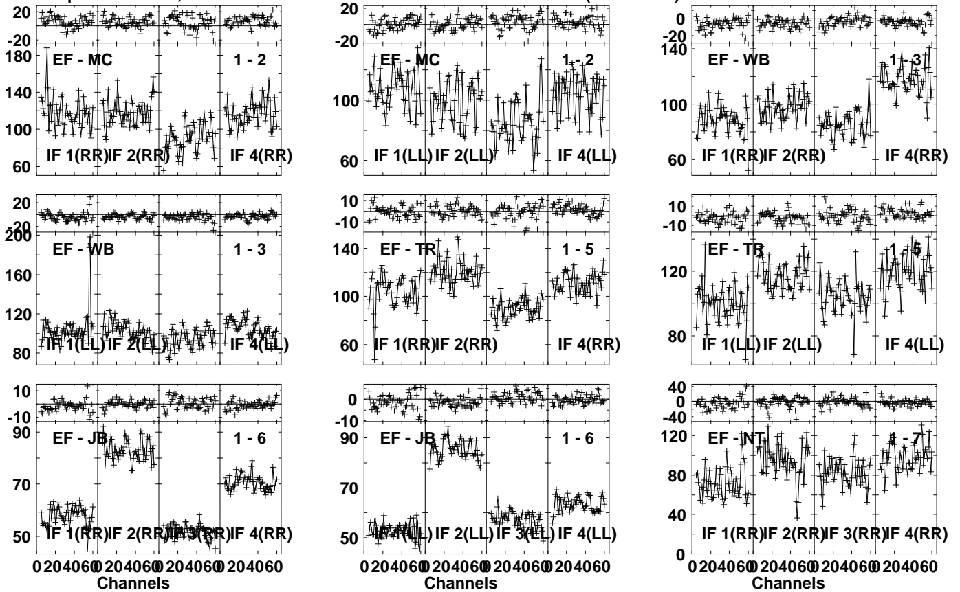
Lower frame: Milli Ampl Jy Top frame: Phas deg Vector averaged cross-power spectrum Several baselines displayed Timerange: 00:15:29:41 to 00:15:31:09
