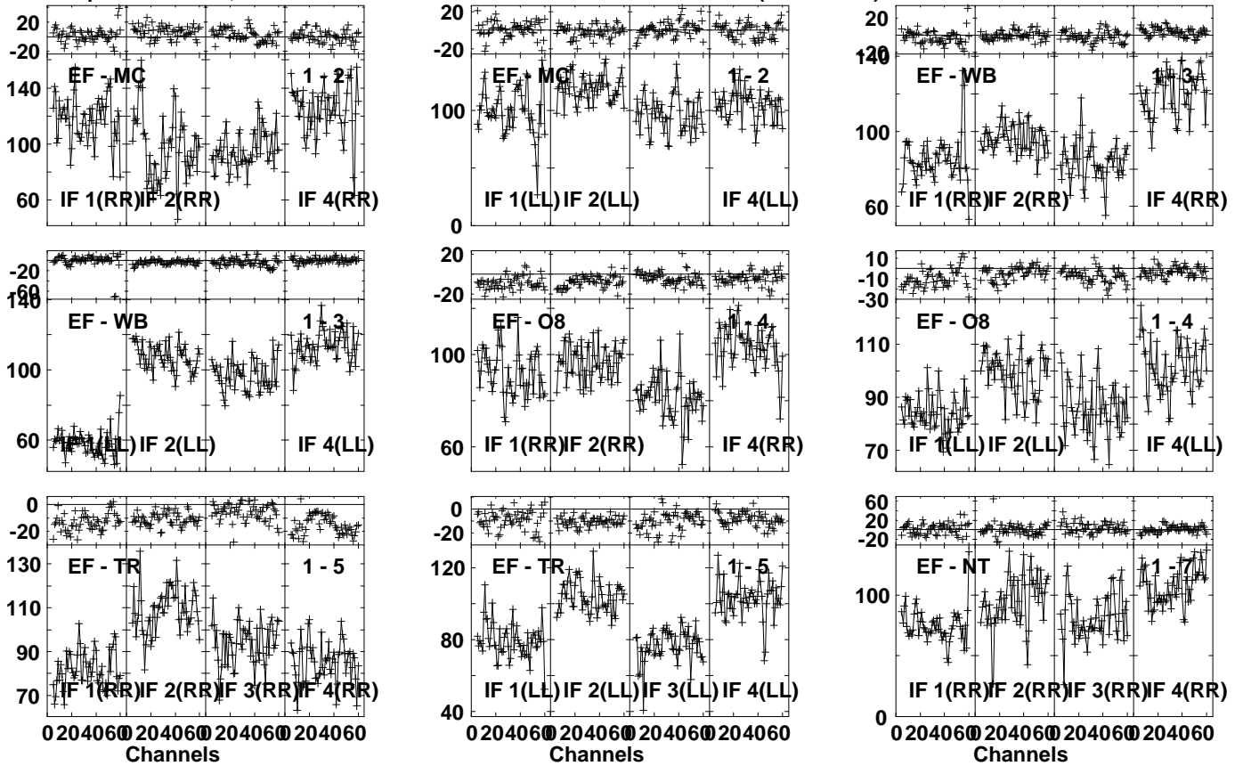
Lower frame: Milli Ampl Jy Top frame: Phas deg Vector averaged cross-power spectrum Several baselines displayed Timerange: 00/10:19:31 to 00/10:20:59
