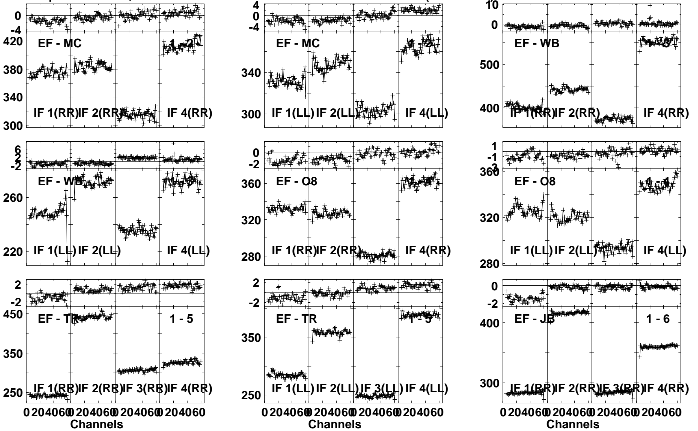
Lower frame: Milli Ampl Jy Top frame: Phas deg Vector averaged cross-power spectrum Several baselines displayed Timerange: 00/06:00:01 to 00/06:05:59
