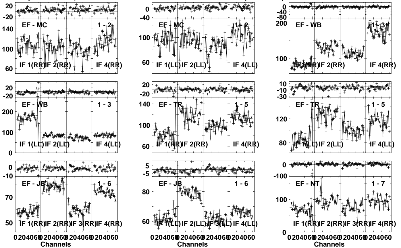
Lower frame: Milli Ampl Jy Top frame: Phas deg Vector averaged cross-power spectrum Several baselines displayed Timerange: 00:15:43:21 to 00:15:44:49
