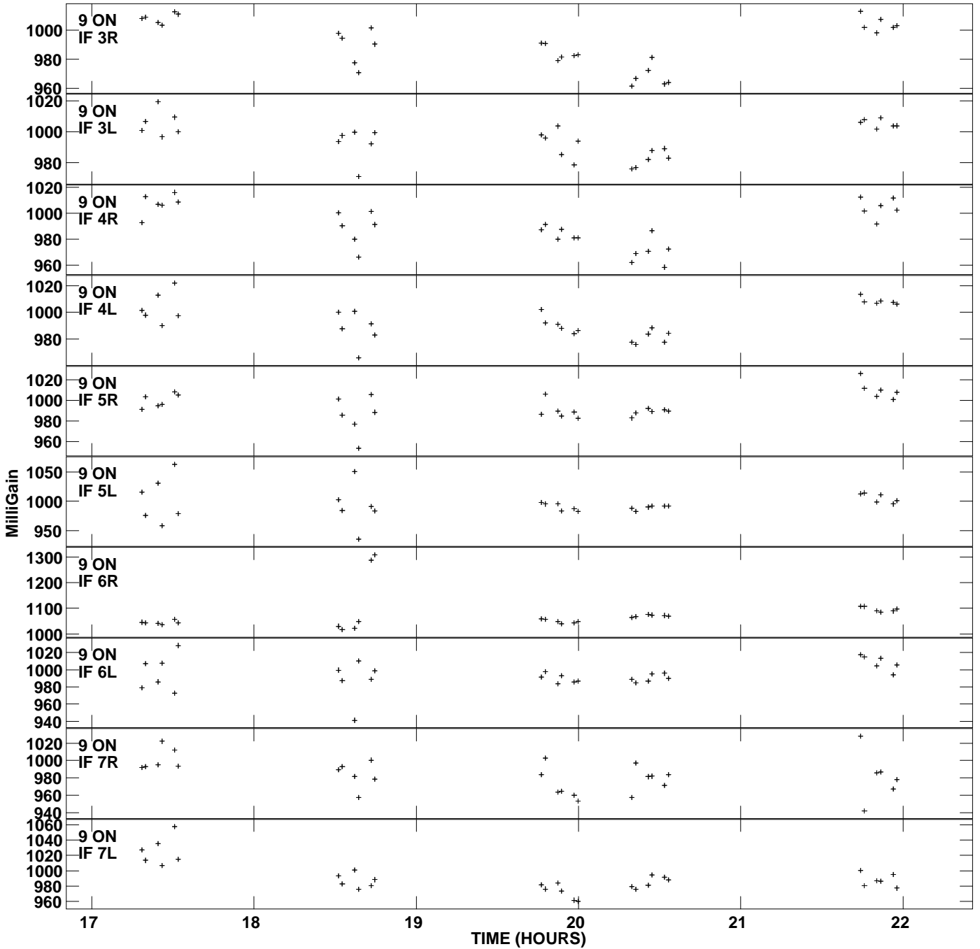
Plot file version 14 created 24-MAR-2009 12:01:20 Gain amp vs UTC time for 0202+319.MULTI.1 SN 4 Rpol & Lpol IF 1 - 8
