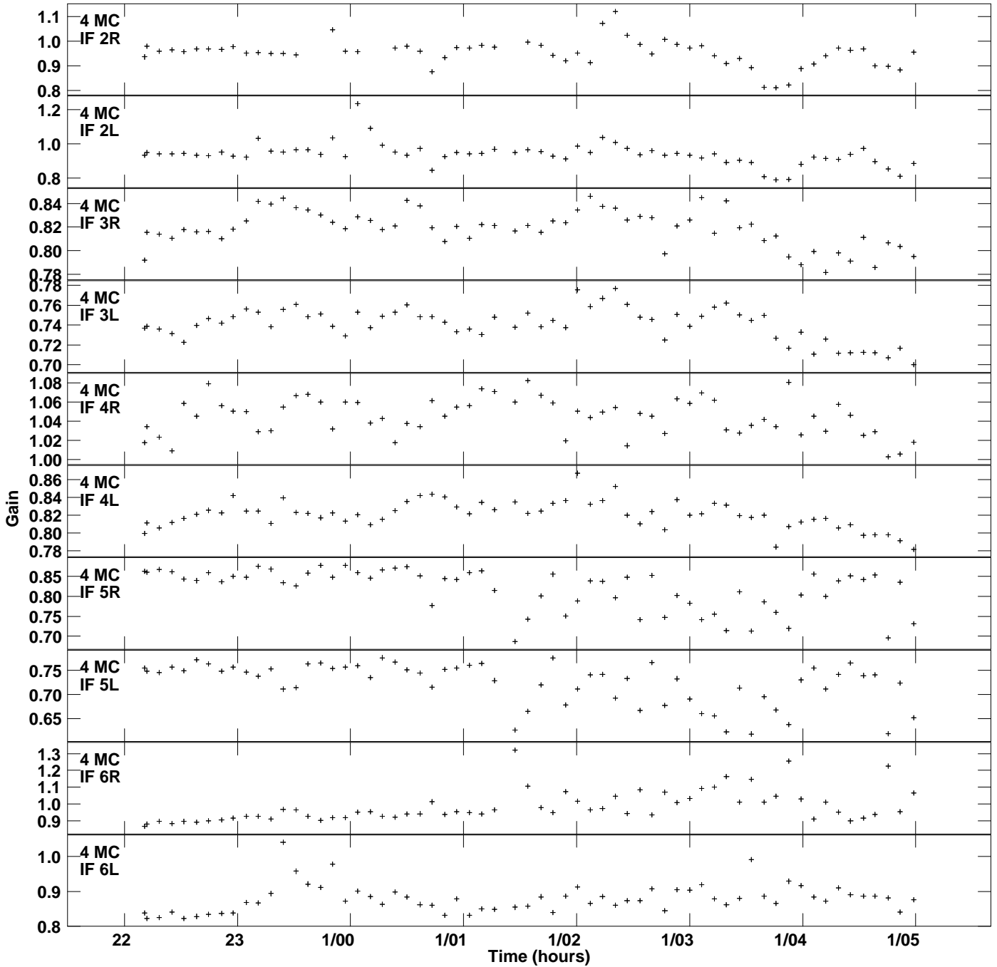
Plot file version 6 created 11-NOV-2019 14:09:42 Gain amp vs UTC time for J1826+0149.MULTI.1 SN 2 Rpol & Lpol IF 1 - 8
