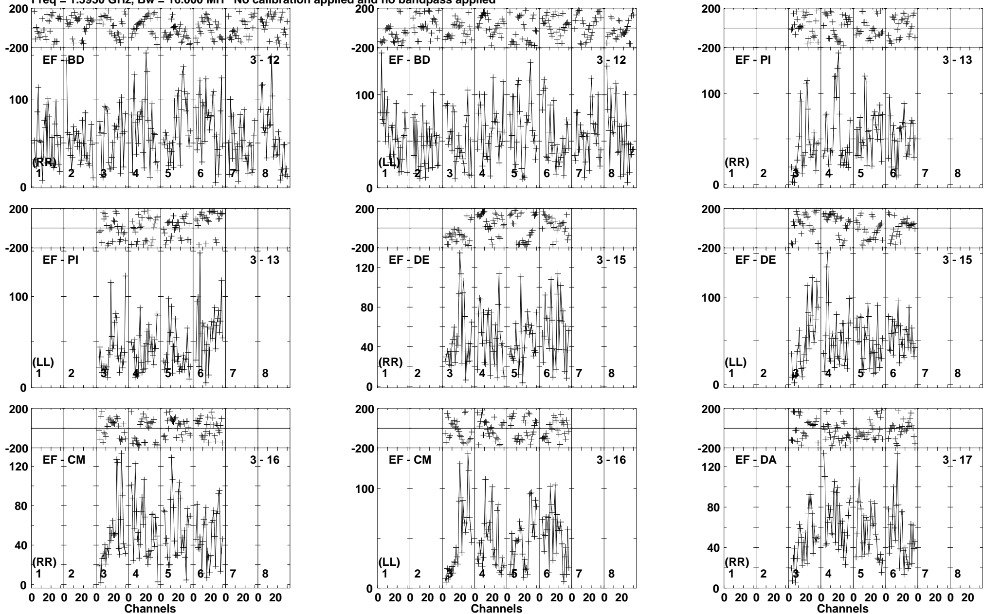
Lower frame: Micro Ampl Jy Top frame: Phas deg Vector averaged cross-power spectrum Baseline: EF (03) - BD (12) Timerange: 00/23:05:11 to 00/23:10:09
