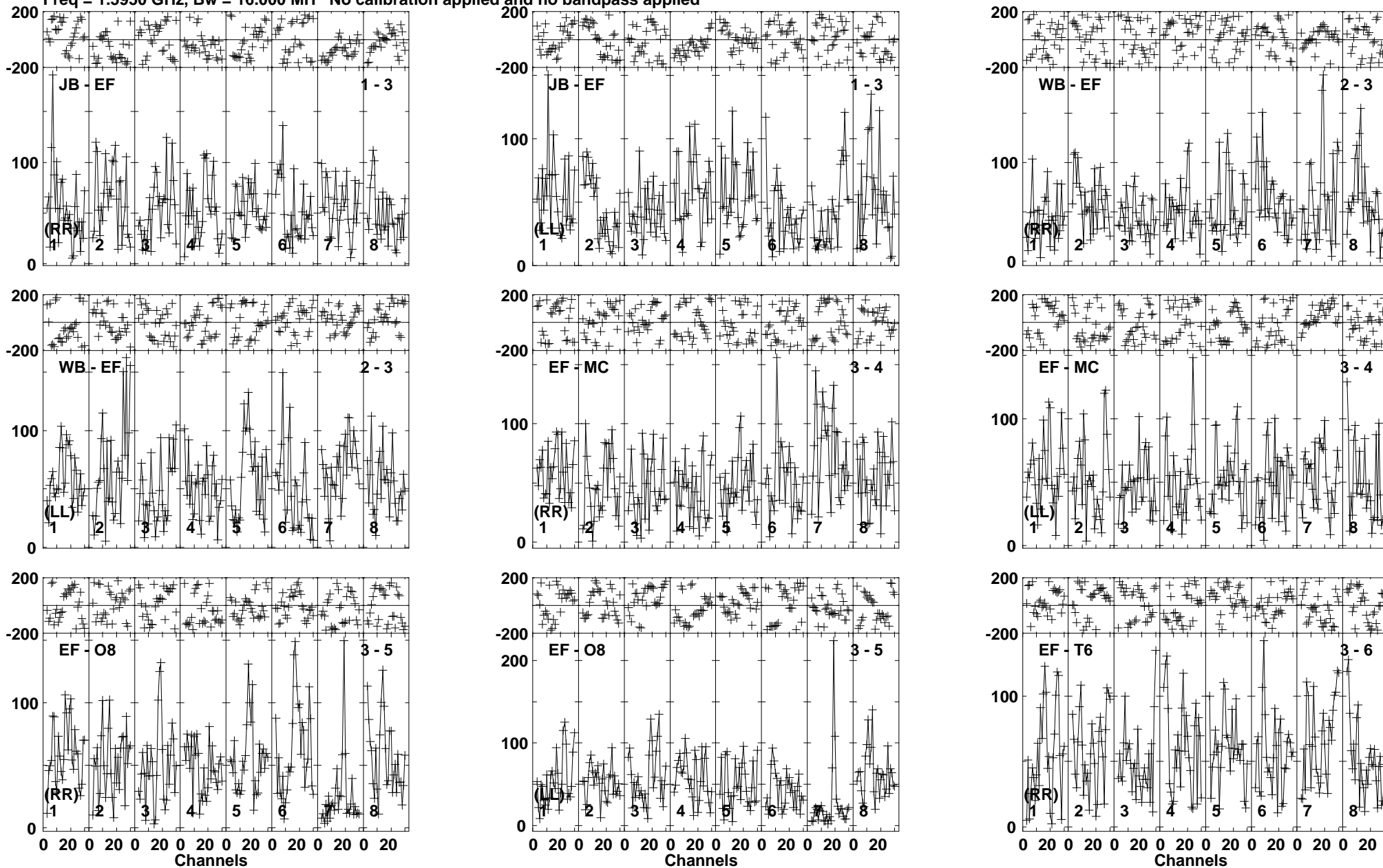
Lower frame: Micro Ampl Jy Top frame: Phas deg Vector averaged cross-power spectrum Baseline: JB (01) - EF (03) Timerange: 00:22:45:21 to 00:22:50:19
