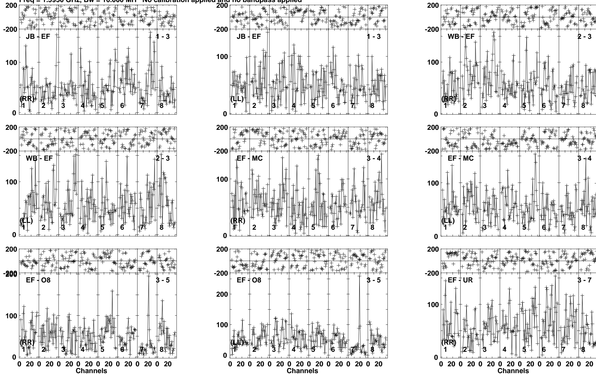
Lower frame: Micro Ampl Jy Top frame: Phas deg Vector averaged cross-power spectrum Baseline: JB (01) - EF (03) Timerange: 00/23:38:01 to 00/23:42:59
