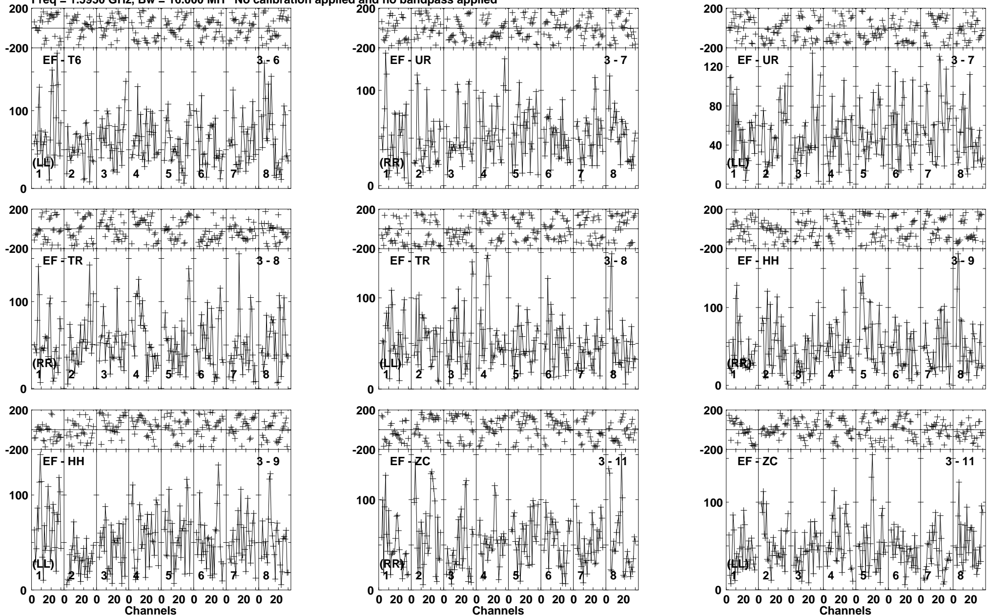
Lower frame: Micro Ampl Jy Top frame: Phas deg Vector averaged cross-power spectrum Baseline: EF (03) - T6 (06) Timerange: 00/22:58:31 to 00/23:03:29
