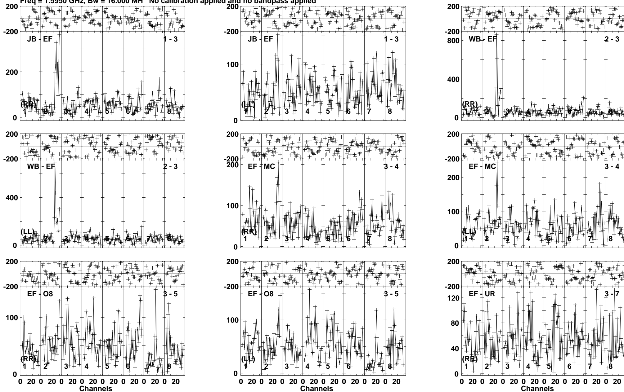
Lower frame: Micro Ampl Jy Top frame: Phas deg Vector averaged cross-power spectrum Baseline: JB (01) - EF (03) Timerange: 01/00:04:21 to 01/00:09:19
