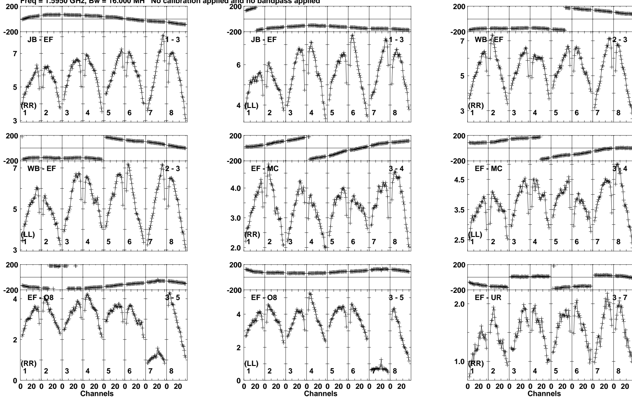
Lower frame: Milli Ampl Jy Top frame: Phas deg Vector averaged cross-power spectrum Baseline: JB (01) - EF (03) Timerange: 01/00:02:51 to 01/00:04:19
