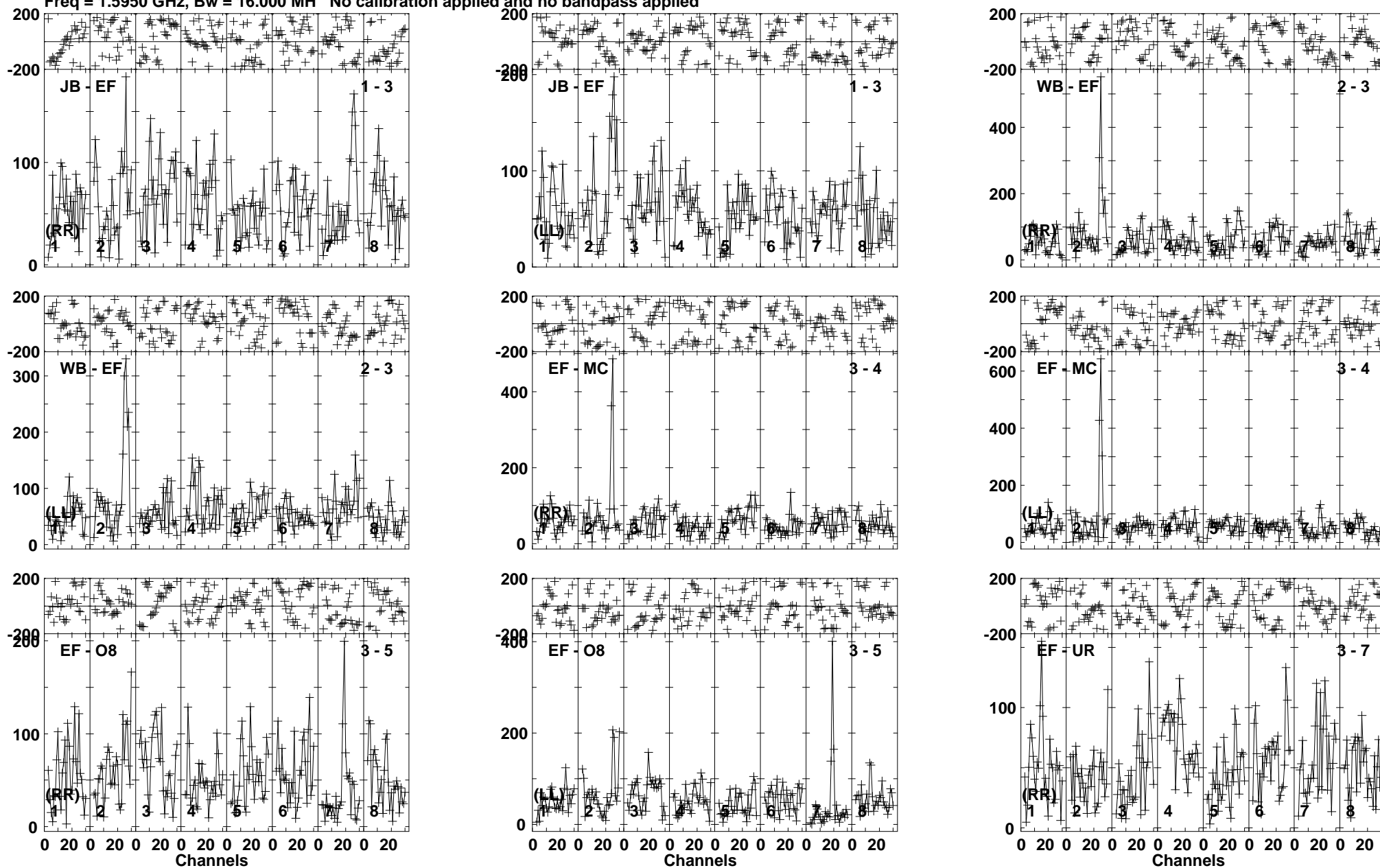
Lower frame: Micro Ampl Jy Top frame: Phas deg Vector averaged cross-power spectrum Baseline: JB (01) - EF (03) Timerange: 00/23:57:51 to 01/00:02:49
