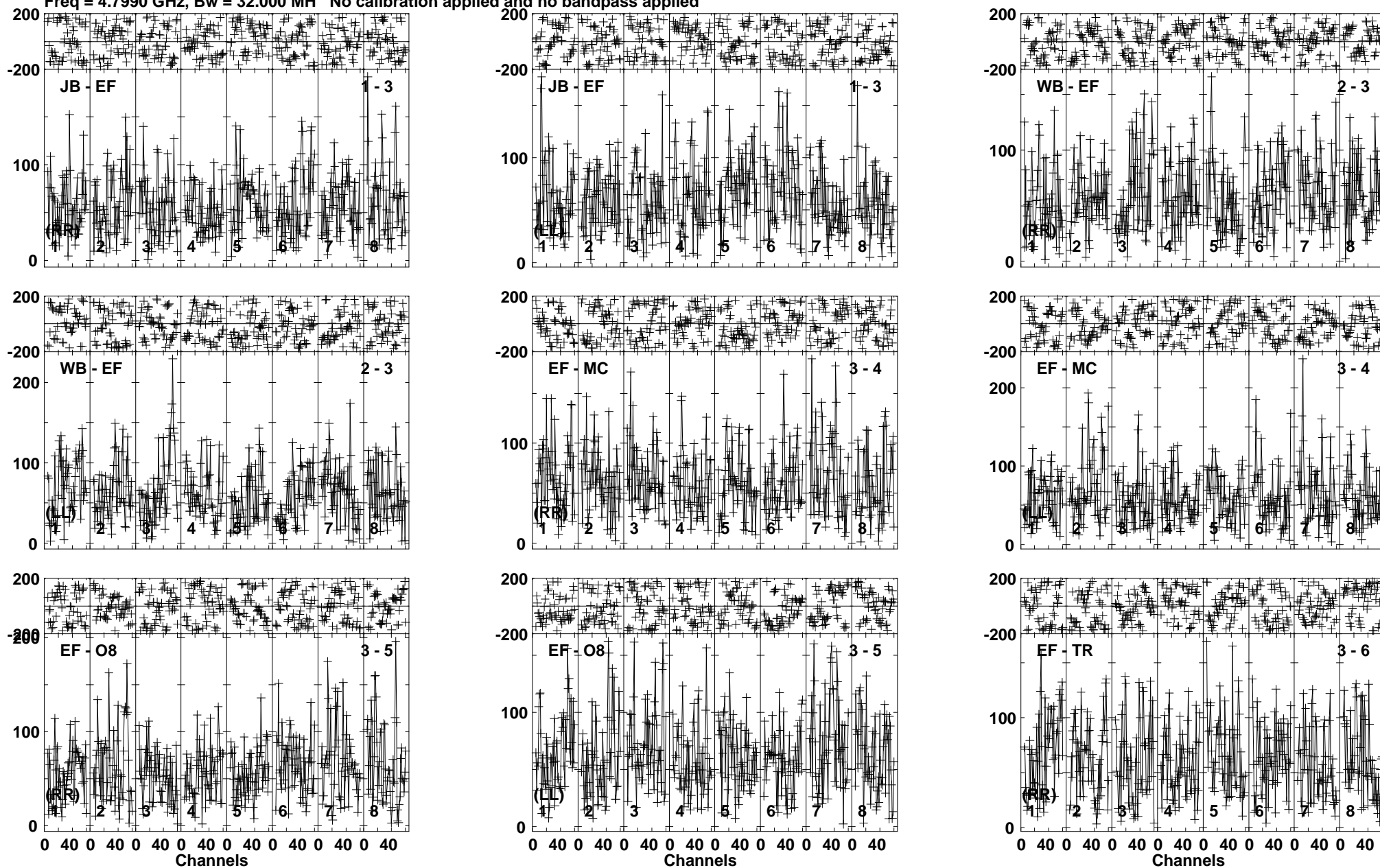
Lower frame: Micro Ampl Jy Top frame: Phas deg Vector averaged cross-power spectrum Baseline: JB (01) - EF (03) Timerange: 00/23:07:03 to 00/23:10:59
