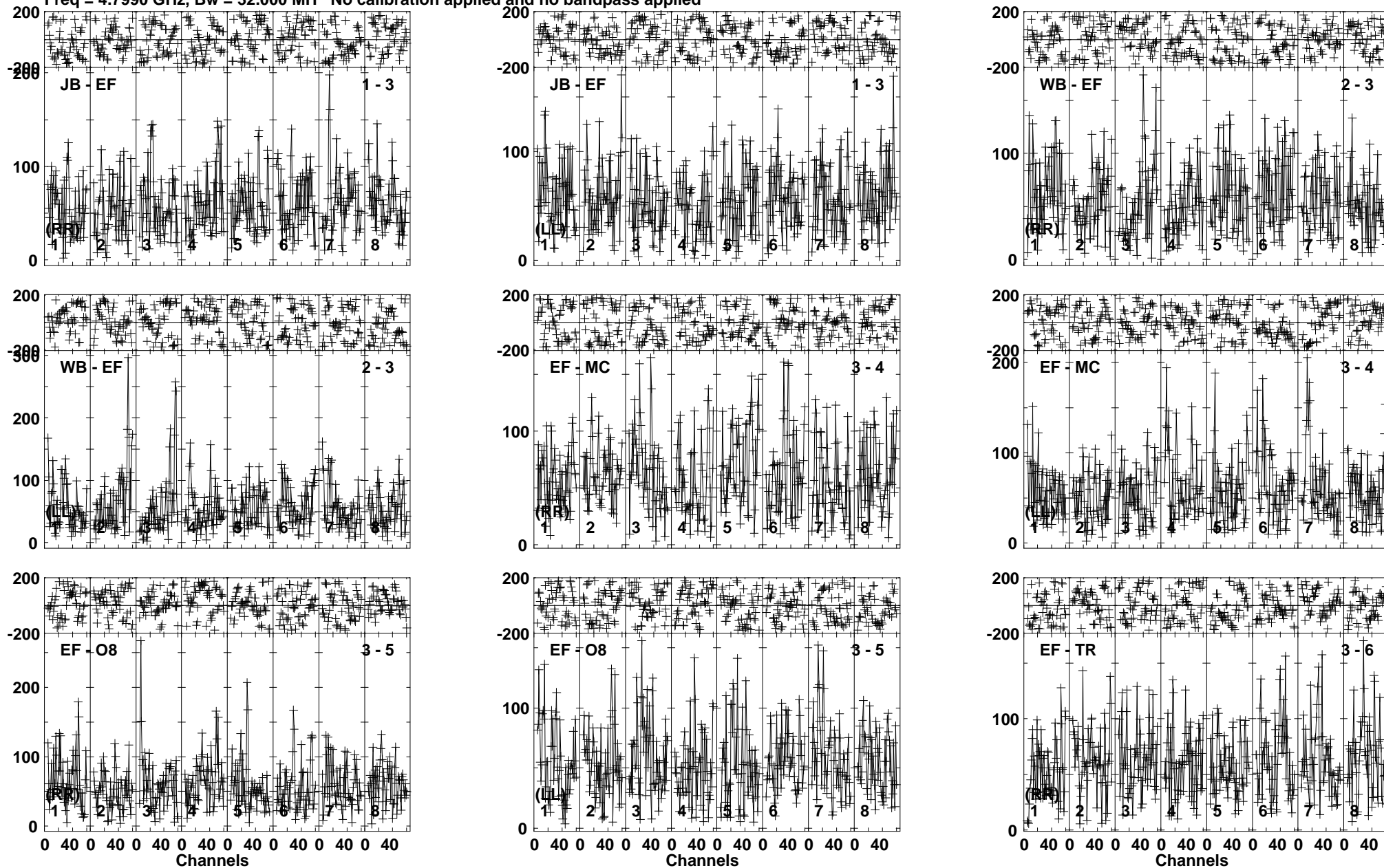
Lower frame: Micro Ampl Jy Top frame: Phas deg Vector averaged cross-power spectrum Baseline: JB (01) - EF (03) Timerange: 00:22:27:53 to 00:22:31:49
