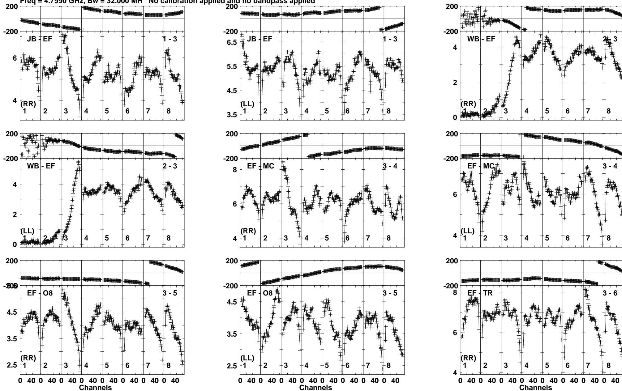
Lower frame: Milli Ampl Jy Top frame: Phas deg Vector averaged cross-power spectrum Baseline: JB (01) - EF (03) Timerange: 01/01:18:51 to 01/01:19:49
