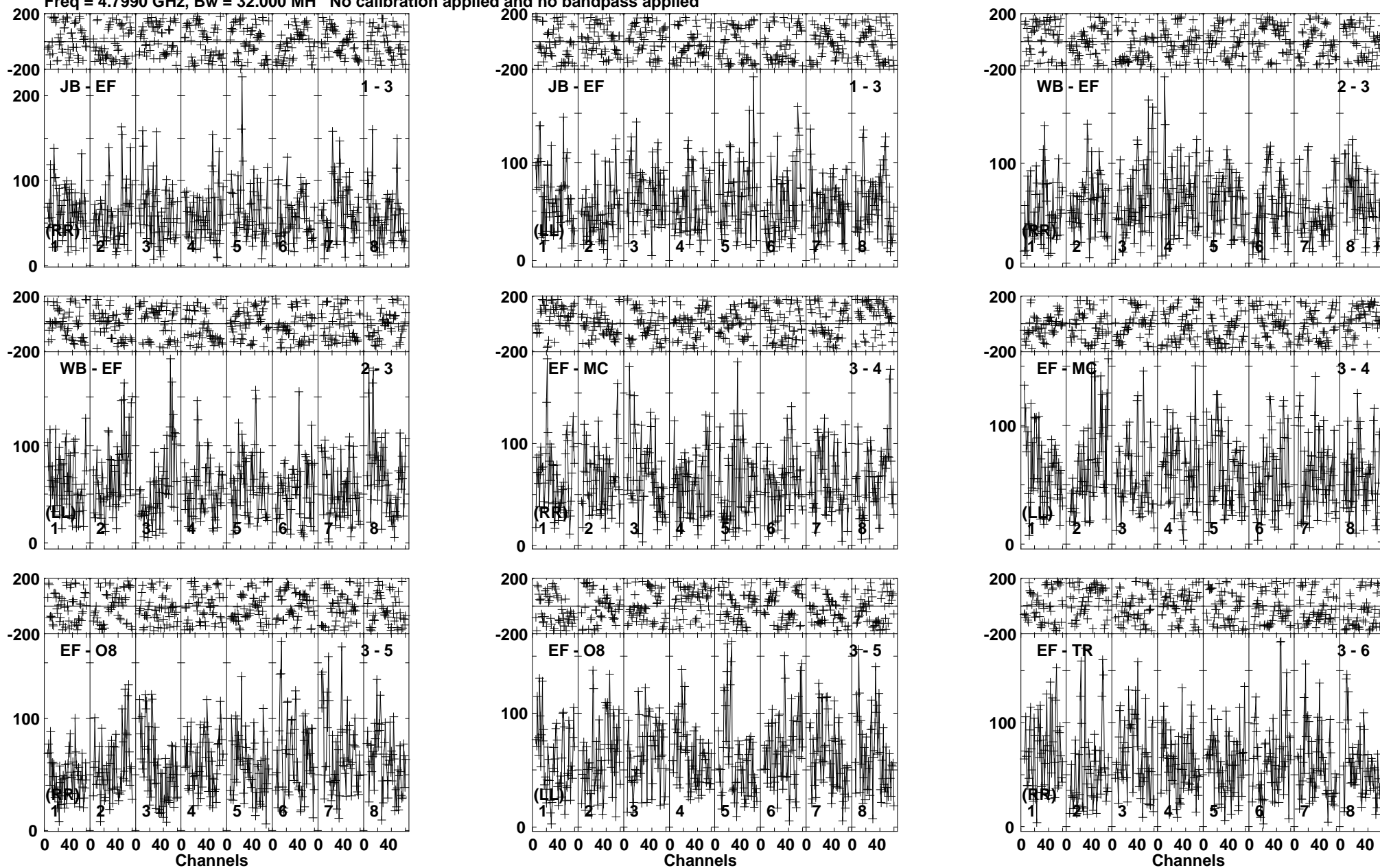
Lower frame: Micro Ampl Jy Top frame: Phas deg Vector averaged cross-power spectrum Baseline: JB (01) - EF (03) Timerange: 01/03:27:33 to 01/03:31:29
