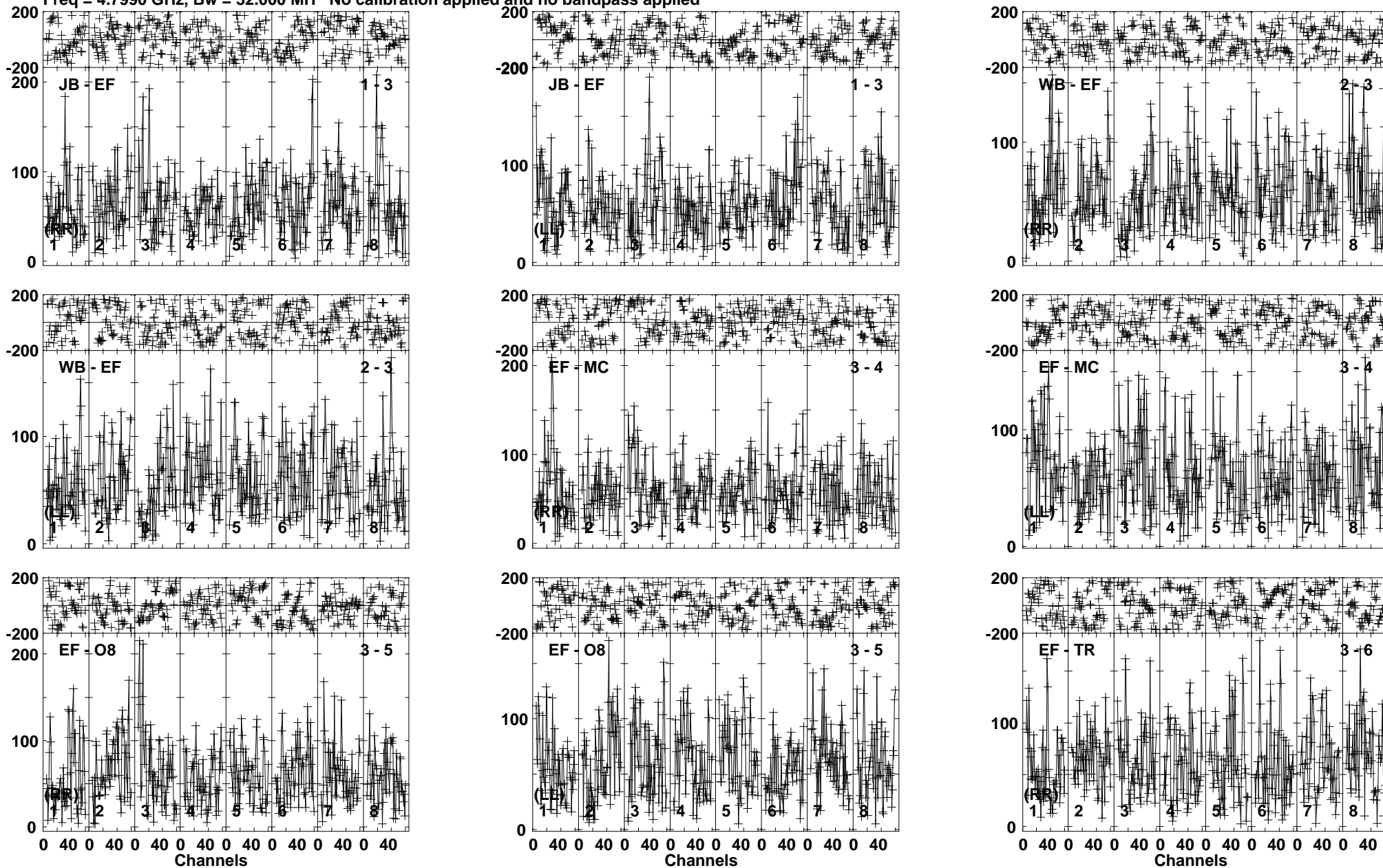
Lower frame: Micro Ampl Jy Top frame: Phas deg Vector average cross-power spectrum Baseline: JB (01) - EF (03) Timerange: 00/22:05:31 to 00/22:09:29
