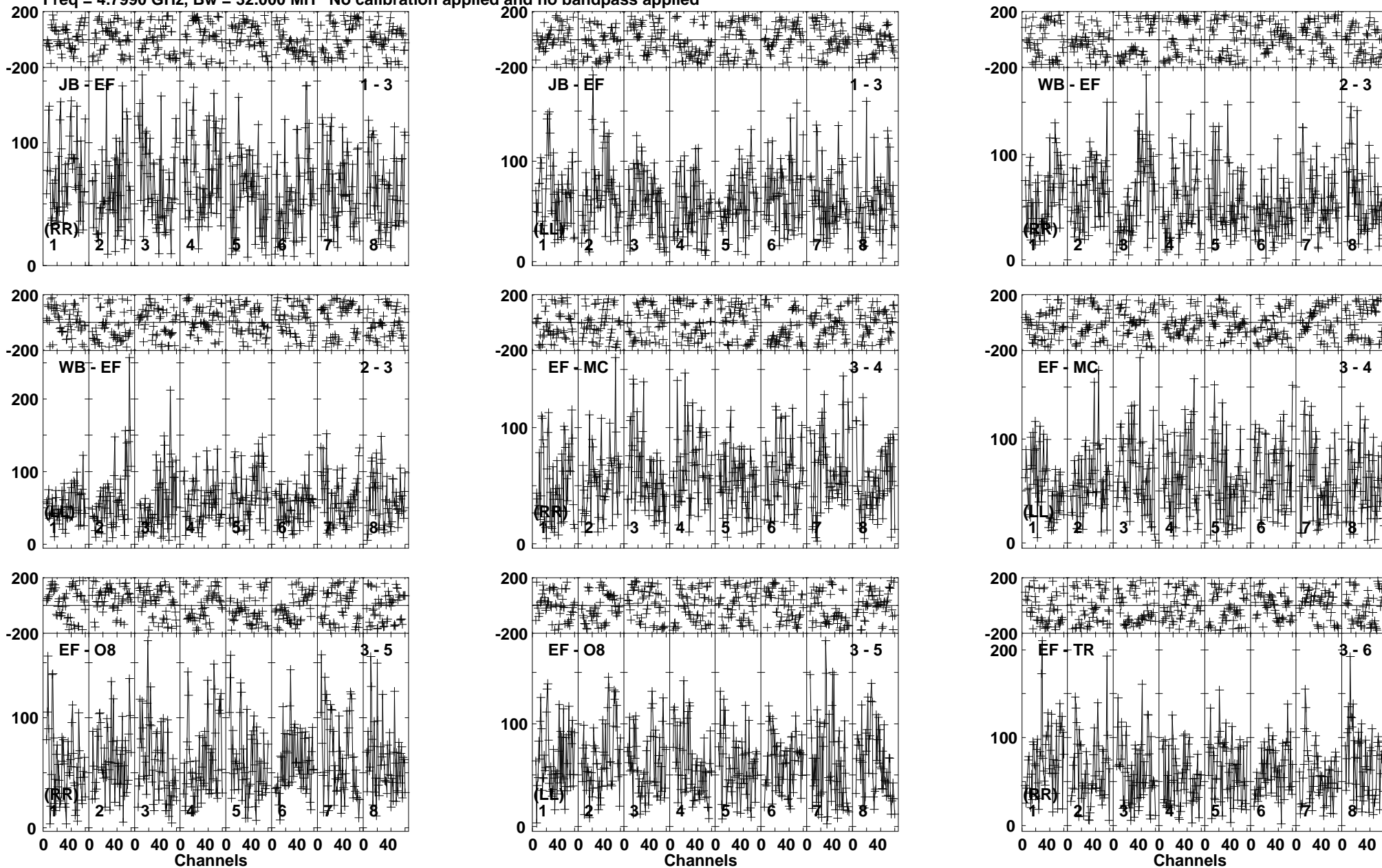
Lower frame: Micro Ampl Jy Top frame: Phas deg Vector averaged cross-power spectrum Baseline: JB (01) - EF (03) Timerange: 00/21:15:21 to 00/21:19:19
