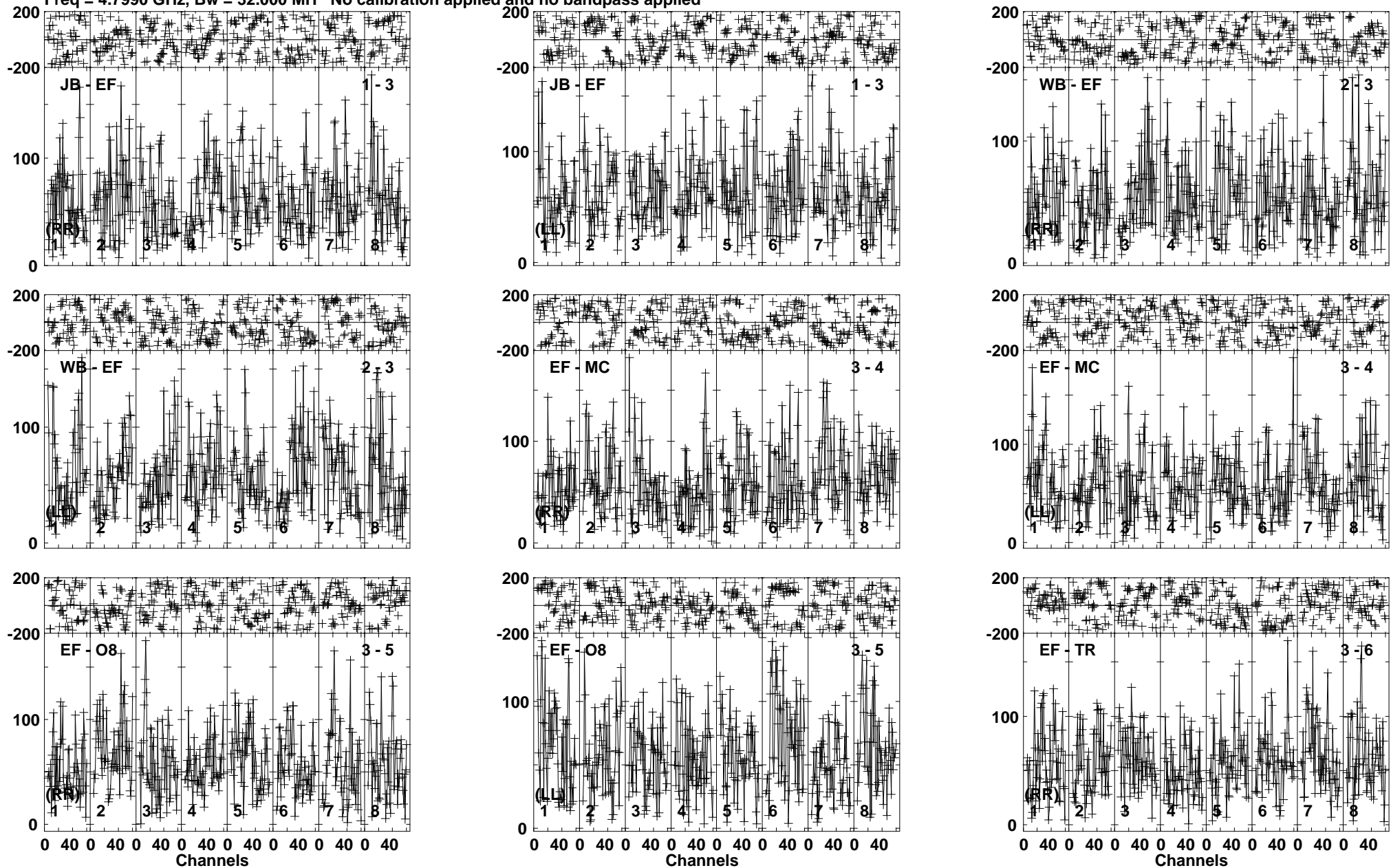
Lower frame: Micro Ampl Jy Top frame: Phas deg Vector averaged cross-power spectrum Baseline: JB (01) - EF (03) Timerange: 01/03:49:53 to 01/03:53:49
