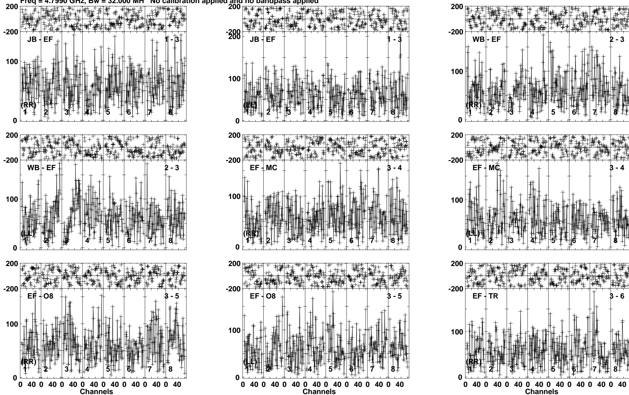
Lower frame: Micro Ampl Jy Top frame: Phas deg Vector averaged cross-power spectrum Baseline: JB (01) - EF (03) Timerange: 01/01:19:53 to 01/01:23:49
