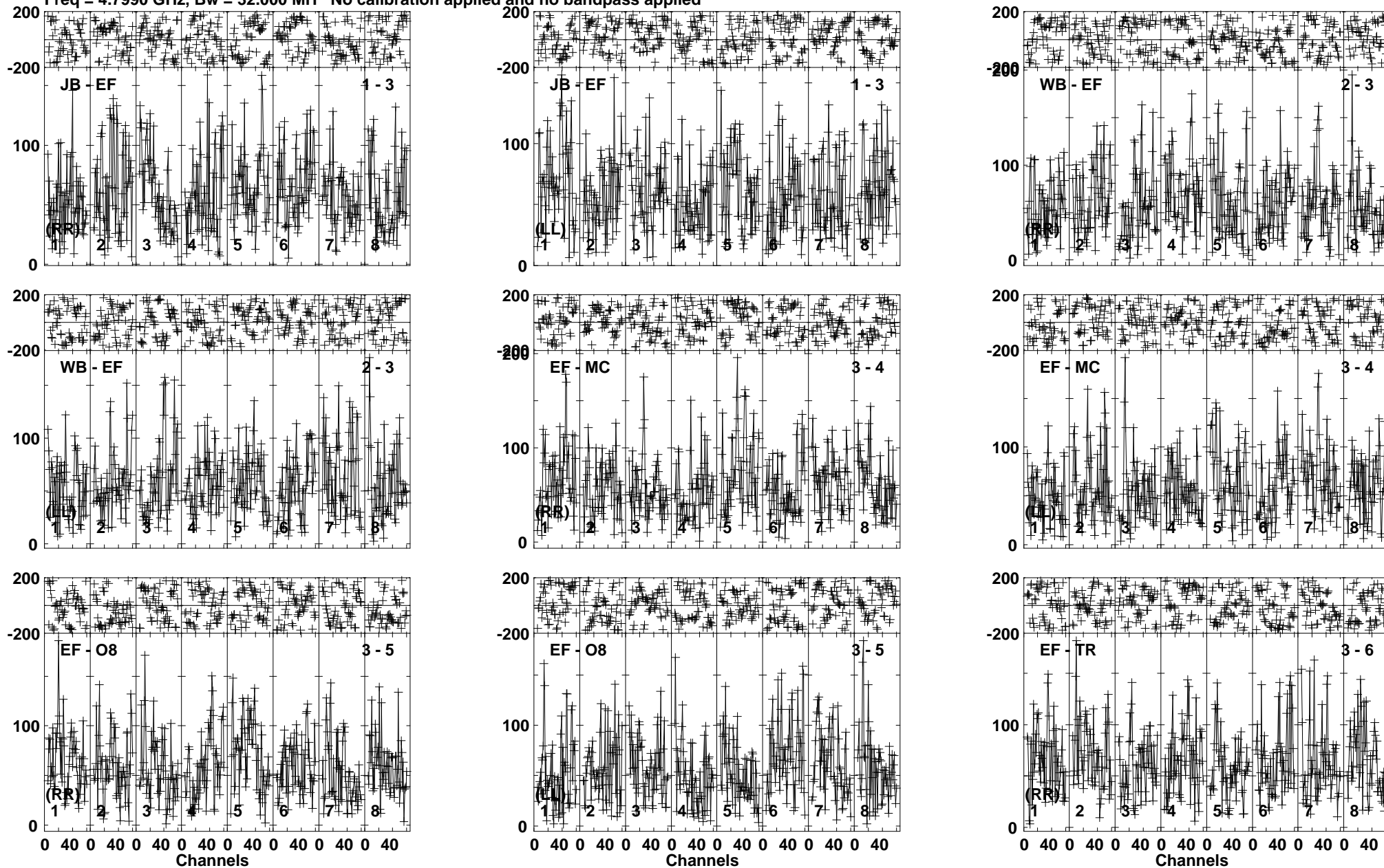
Lower frame: Micro Ampl Jy Top frame: Phas deg Vector averaged cross-power spectrum Baseline: JB (01) - EF (03) Timerange: 01/00:24:01 to 01/00:27:59
