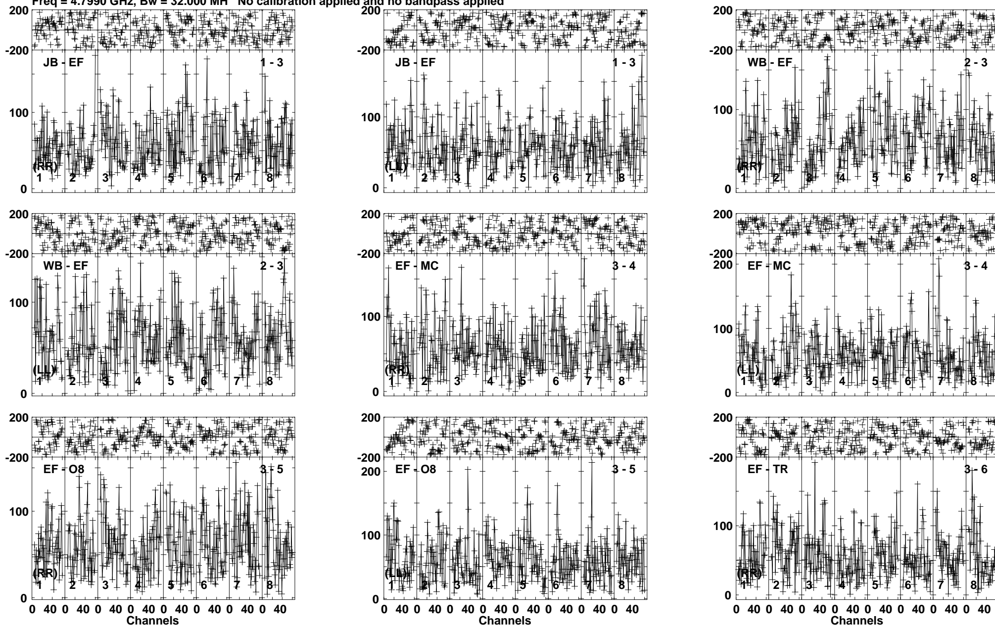
Lower frame: Micro Ampl Jy Top frame: Phas deg Vector averaged cross-power spectrum Baseline: JB (01) - EF (03) Timerange: 01/03:22:01 to 01/03:25:59
