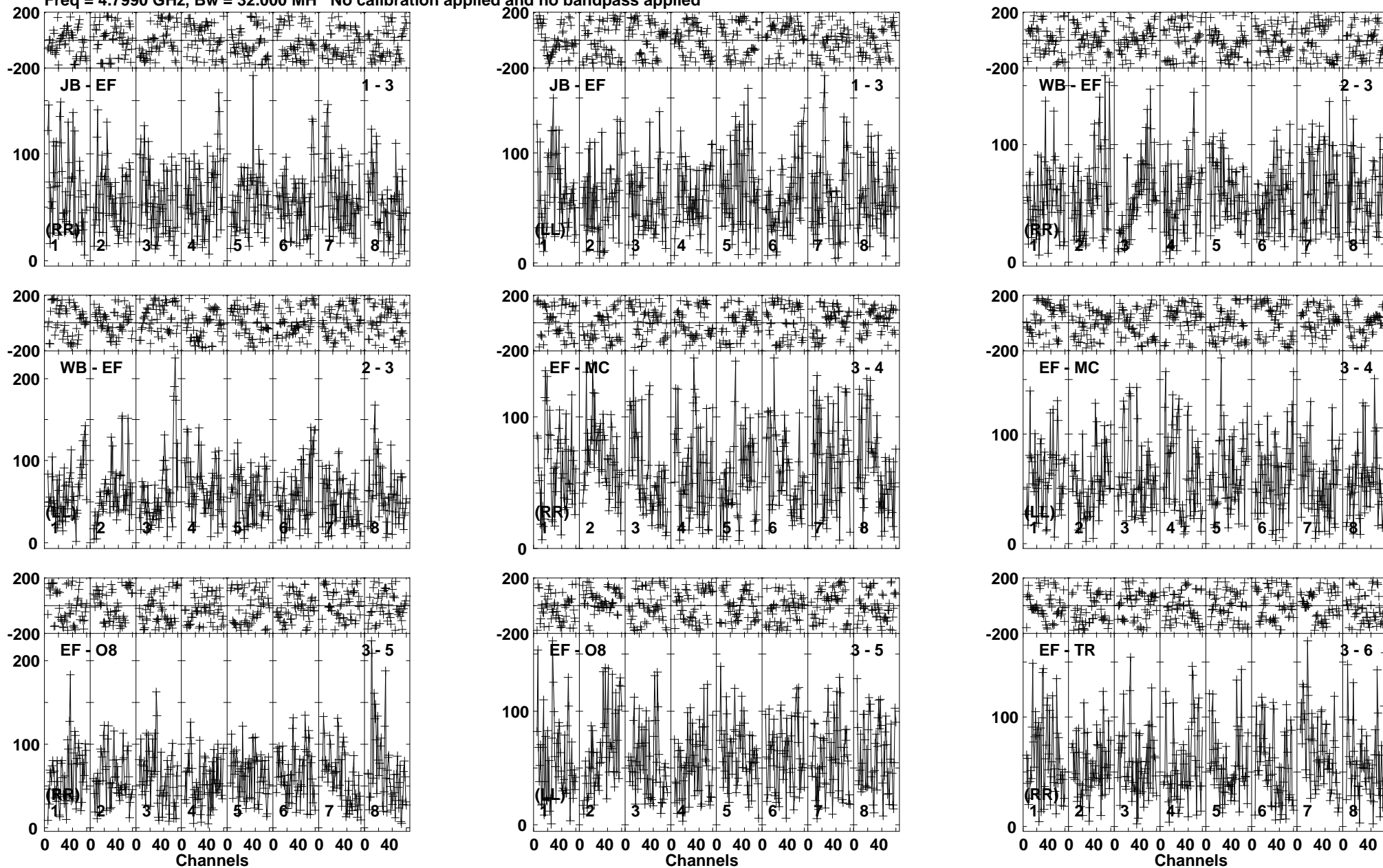
Lower frame: Micro Ampl Jy Top frame: Phas deg Vector averaged cross-power spectrum Baseline: JB (01) - EF (03) Timerange: 00:23:46:01 to 00:23:49:59
