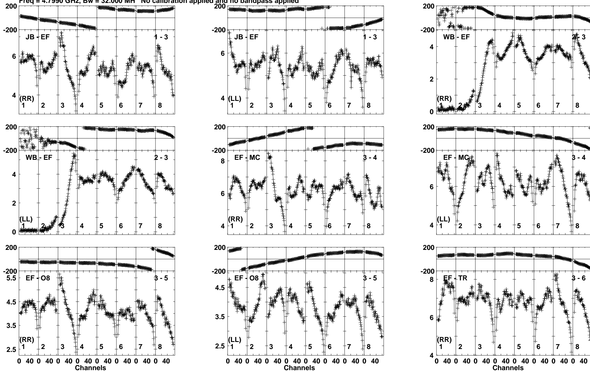
Lower frame: Milli Ampl Jy Top frame: Phas deg Vector averaged cross-power spectrum Baseline: JB (01) - EF (03) Timerange: 01/00:39:11 to 01/00:40:39
