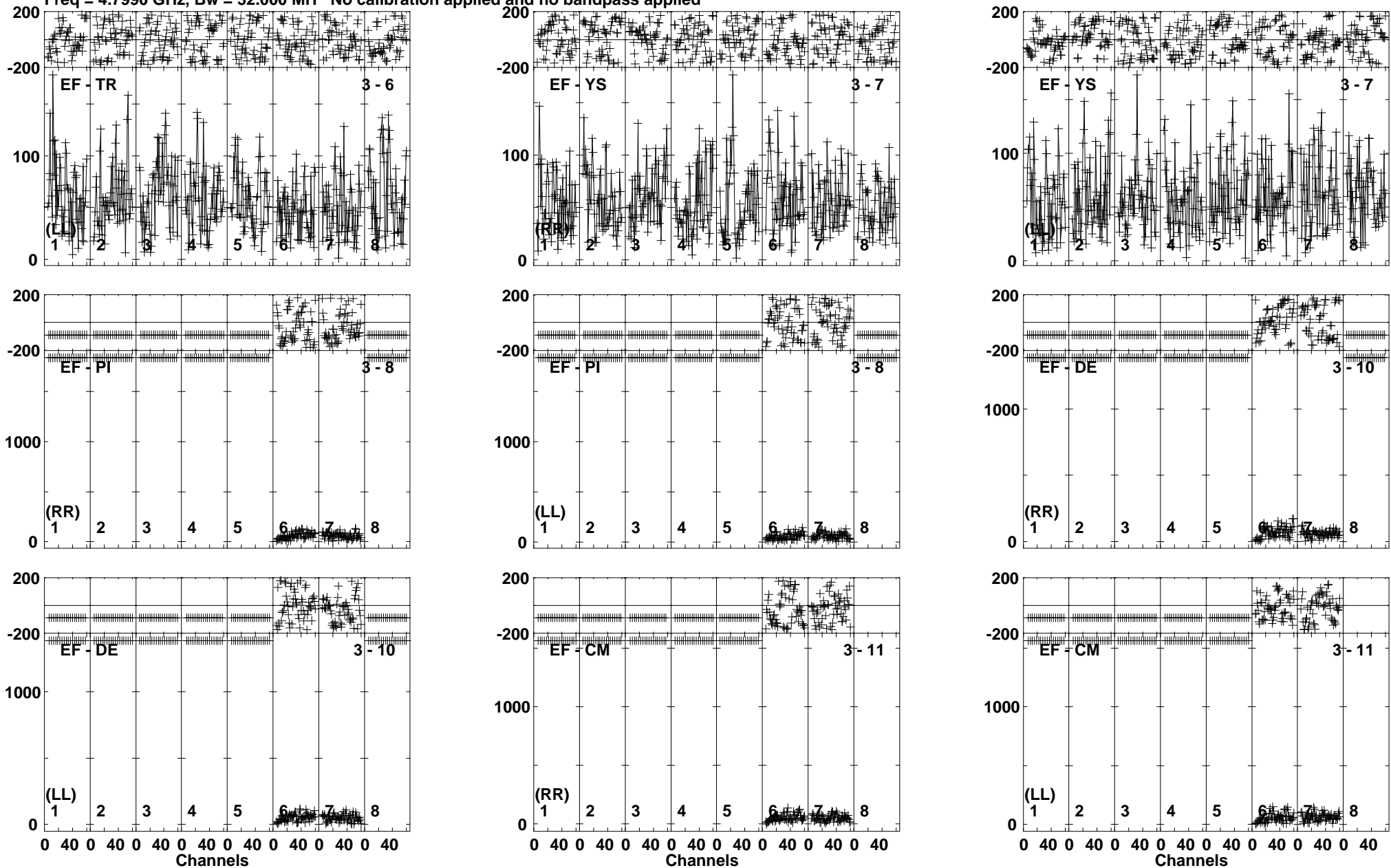
Lower frame: Micro Ampl Jy Top frame: Phas deg Vector averaged cross-power spectrum Baseline: EF (03) - TR (06) Timerange: 01/01:14:13 to 01/01:18:09
