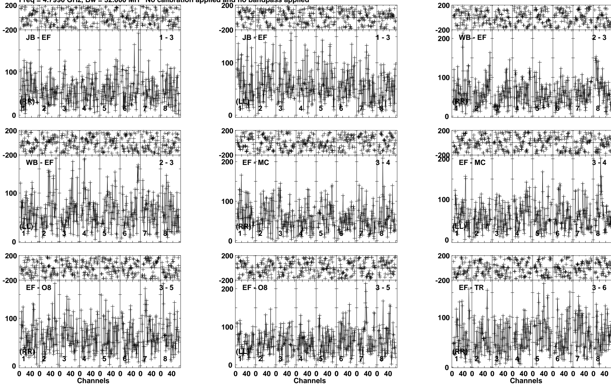
Lower frame: Micro Ampl Jy Top frame: Phas deg Vector averaged cross-power spectrum Baseline: JB (01) - EF (03) Timerange: 01/01:14:13 to 01/01:18:09
