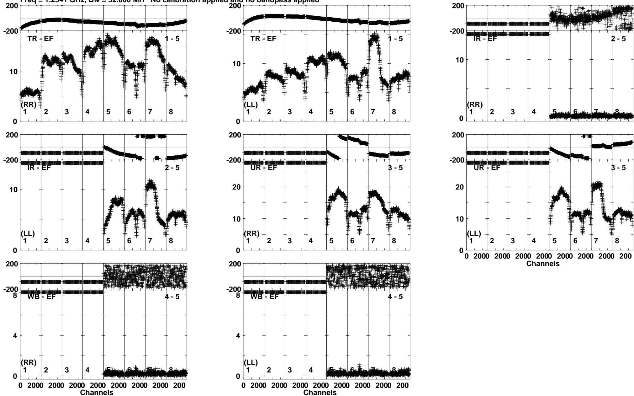
Lower frame: Milli Ampl Jy Top frame: Phas deg Vector averaged cross-power spectrum Baseline: TR (01) - EF (05) Timerange: 01/00:31:49 to 01/00:33:03
