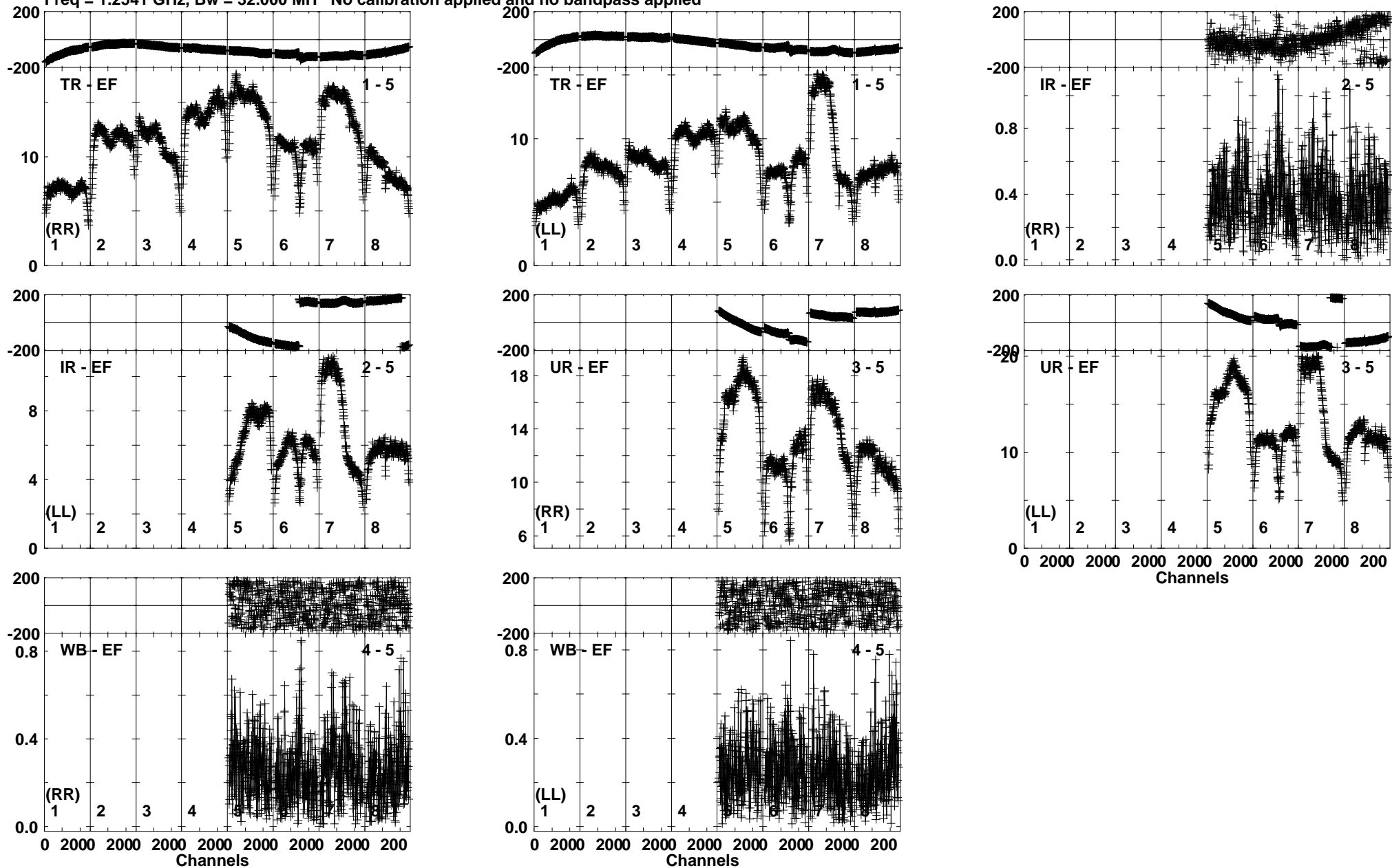
Lower frame: Milli Ampl Jy Top frame: Phas deg Vector averaged cross-power spectrum Baseline: TR (01) - EF (05) Timerange: 01/00:12:27 to 01/00:14:10
