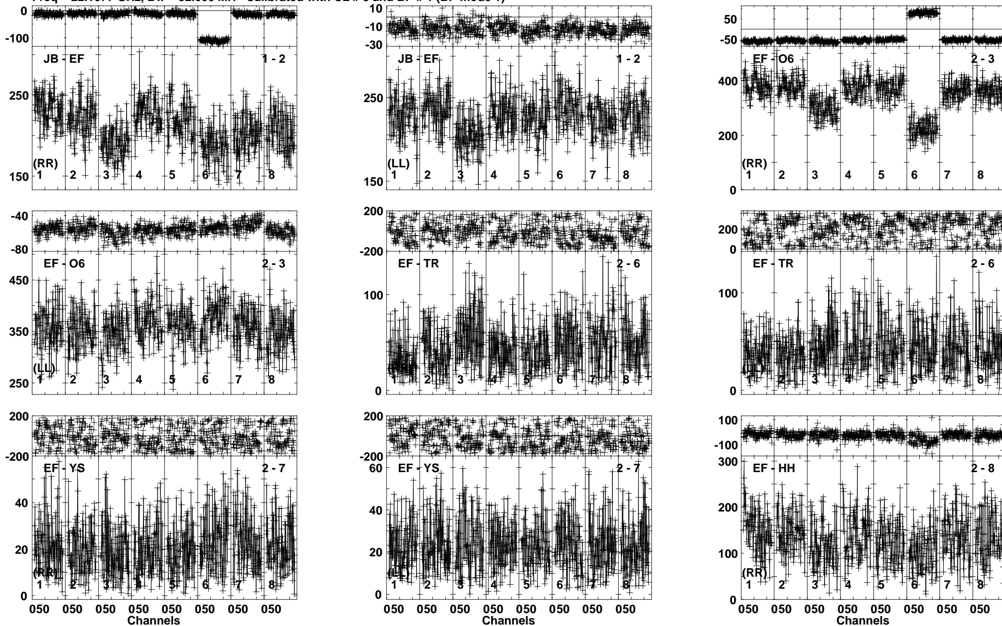
Lower frame: Milli Ampl Jy Top frame: Phas deg Vector averaged cross-power spectrum Baseline: JB (01) - EF (02) Timerange: 00:12:29:21 to 00:12:32:51
