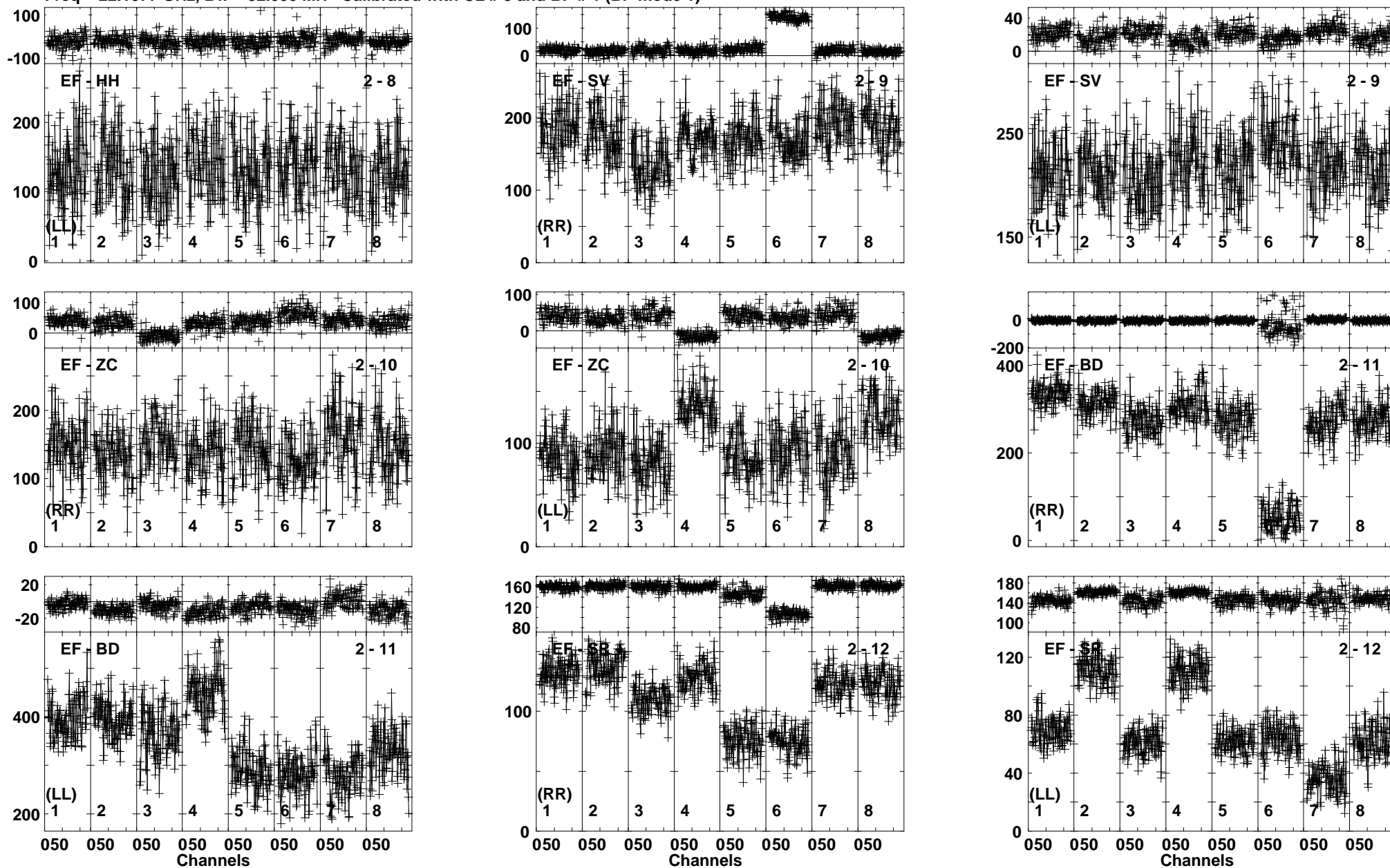
Lower frame: Milli Ampl Jy Top frame: Phas deg Vector averaged cross-power spectrum Baseline: EF (02) - HH (08) Timerange: 00:12:29:21 to 00:12:32:51
