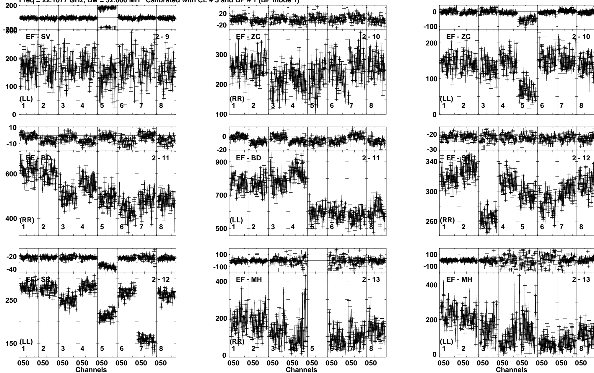
Lower frame: Milli Ampl Jy Top frame: Phas deg Vector averaged cross-power spectrum Baseline: EF (02) - SV (09) Timerange: 00/13:31:40 to 00/13:35:20
