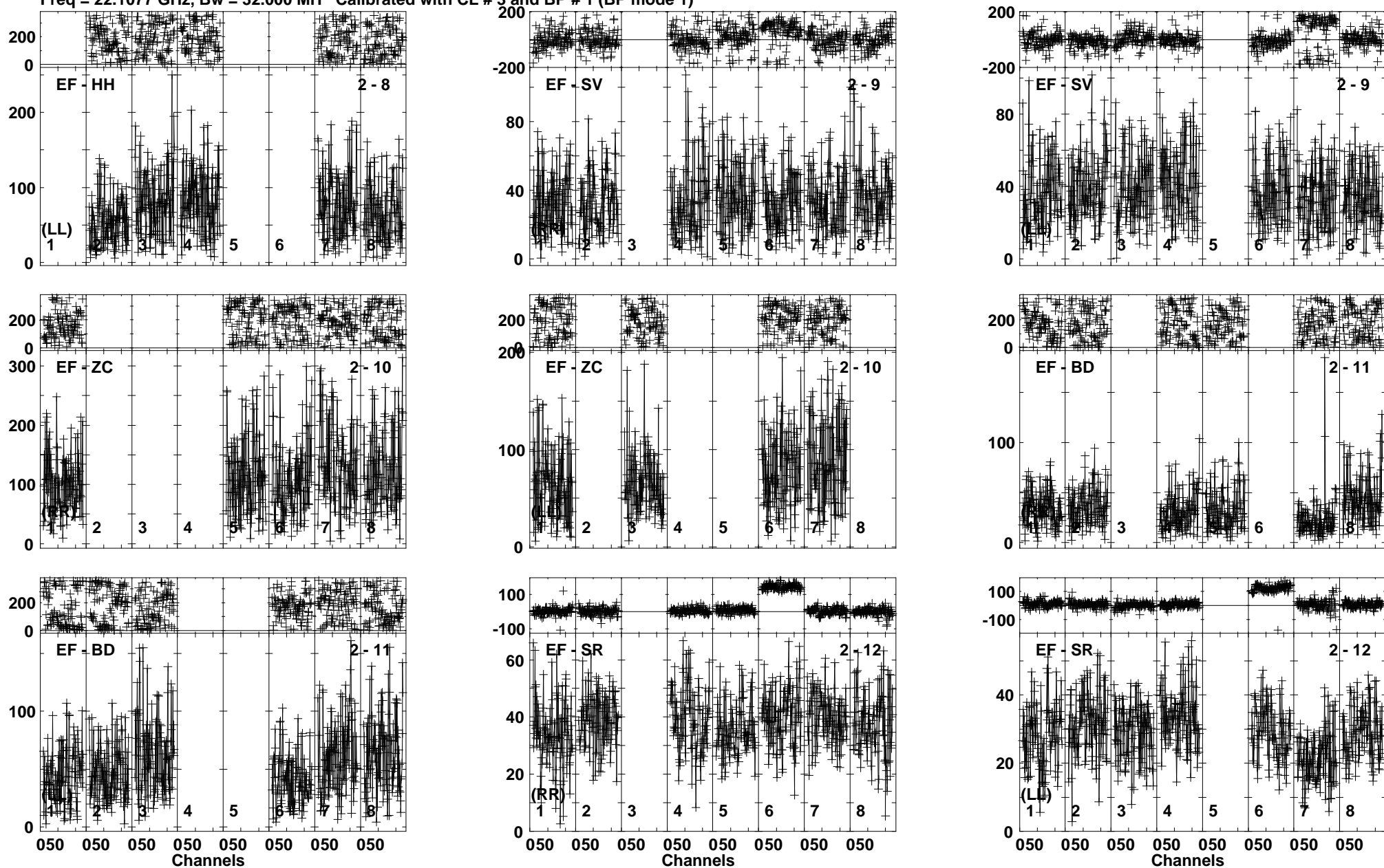
Lower frame: Milli Ampl Jy Top frame: Phas deg Vector averaged cross-power spectrum Baseline: EF (02) - HH (08) Timerange: 00/06:05:41 to 00/06:09:39
