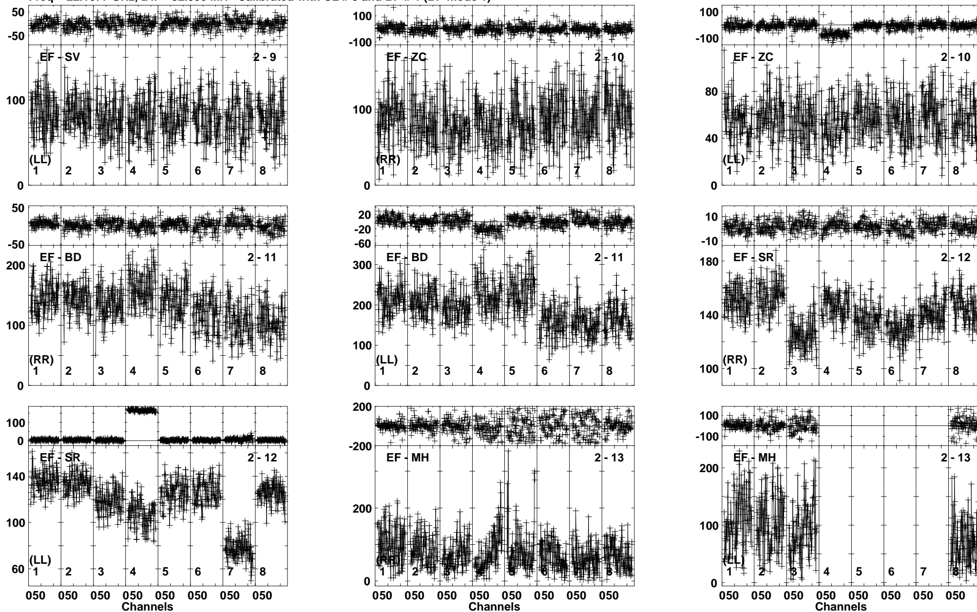
Lower frame: Milli Ampl Jy Top frame: Phas deg Vector averaged cross-power spectrum Baseline: EF (02) - SV (09) Timerange: 00/07:21:48 to 00/07:25:17
