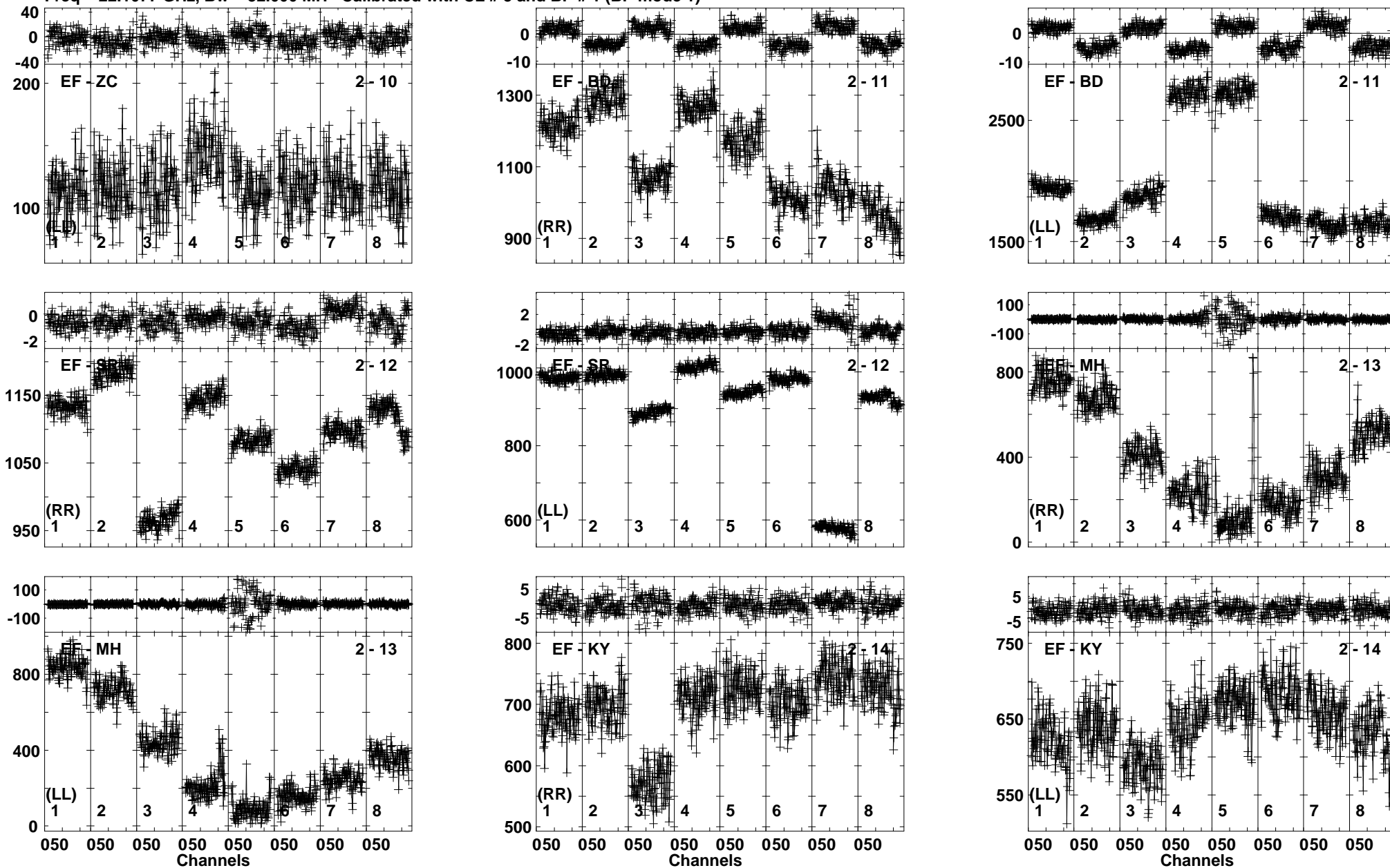
Lower frame: Milli Ampl Jy Top frame: Phas deg Vector averaged cross-power spectrum Baseline: EF (02) - ZC (10) Timerange: 00/06:33:45 to 00/06:37:15
