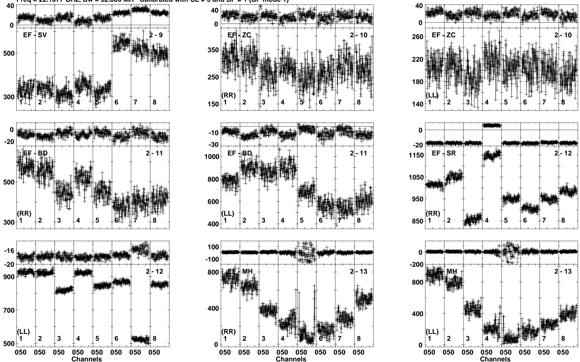
Lower frame: Milli Ampl Jy Top frame: Phas deg Vector averaged cross-power spectrum Baseline: EF (02) - SV (09) Timerange: 00/11:16:57 to 00/11:20:26
