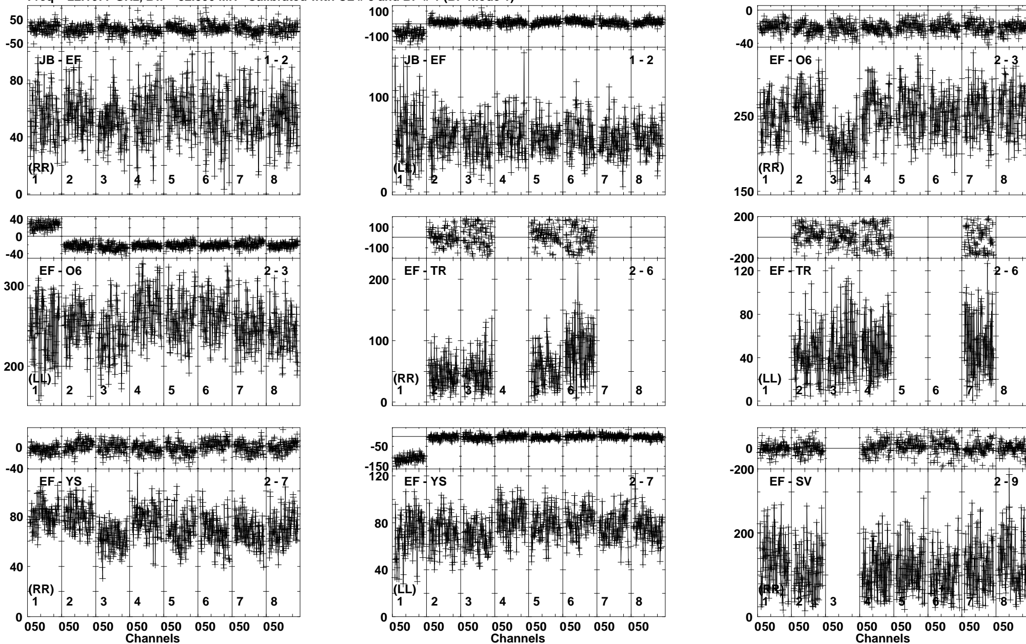
Lower frame: Milli Ampl Jy Top frame: Phas deg Vector averaged cross-power spectrum Baseline: JB (01) - EF (02) Timerange: 00/17:42:28 to 00/17:46:57
