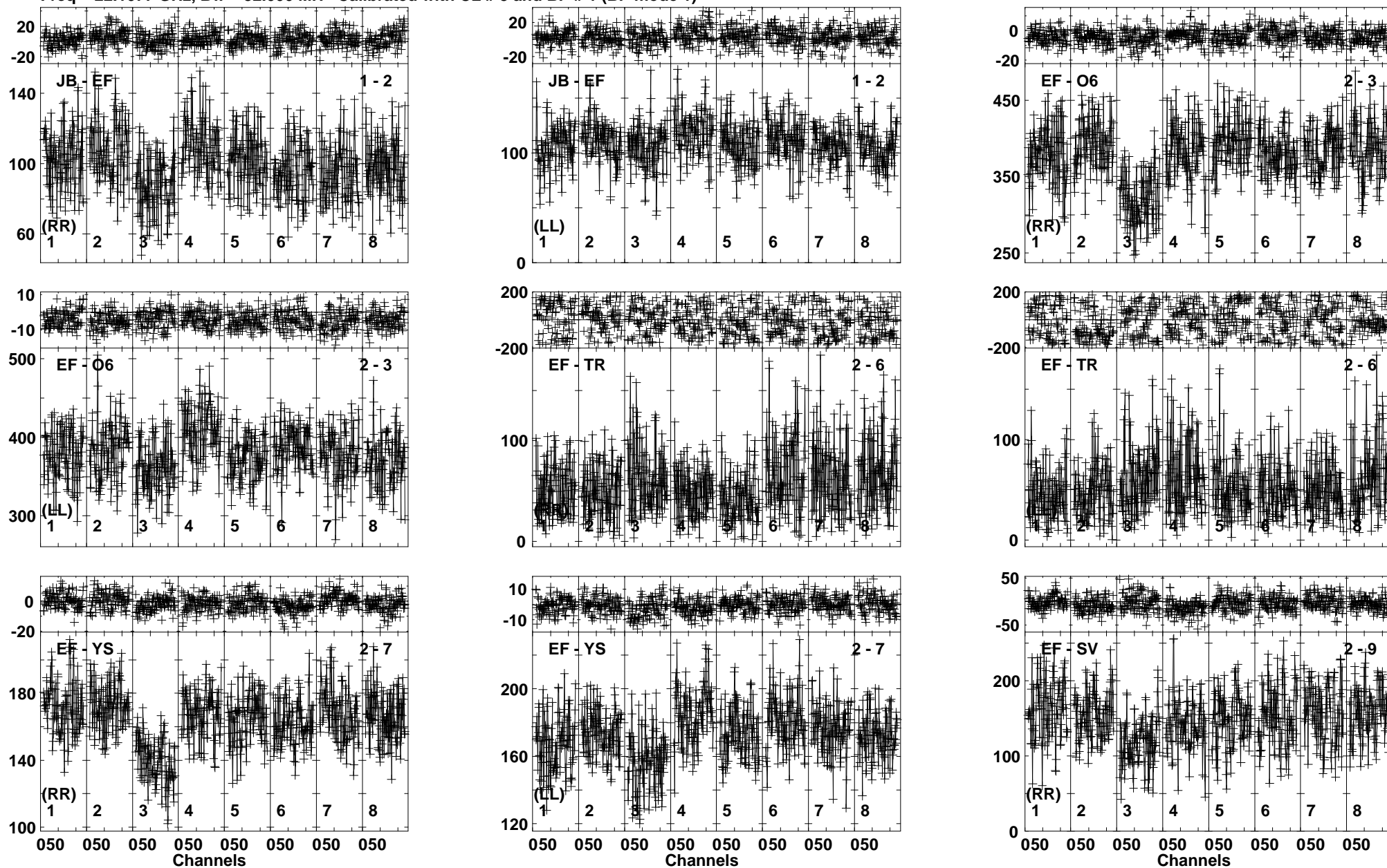
Lower frame: Milli Ampl Jy Top frame: Phas deg Vector averaged cross-power spectrum Baseline: JB (01) - EF (02) Timerange: 00/17:23:39 to 00/17:27:17
