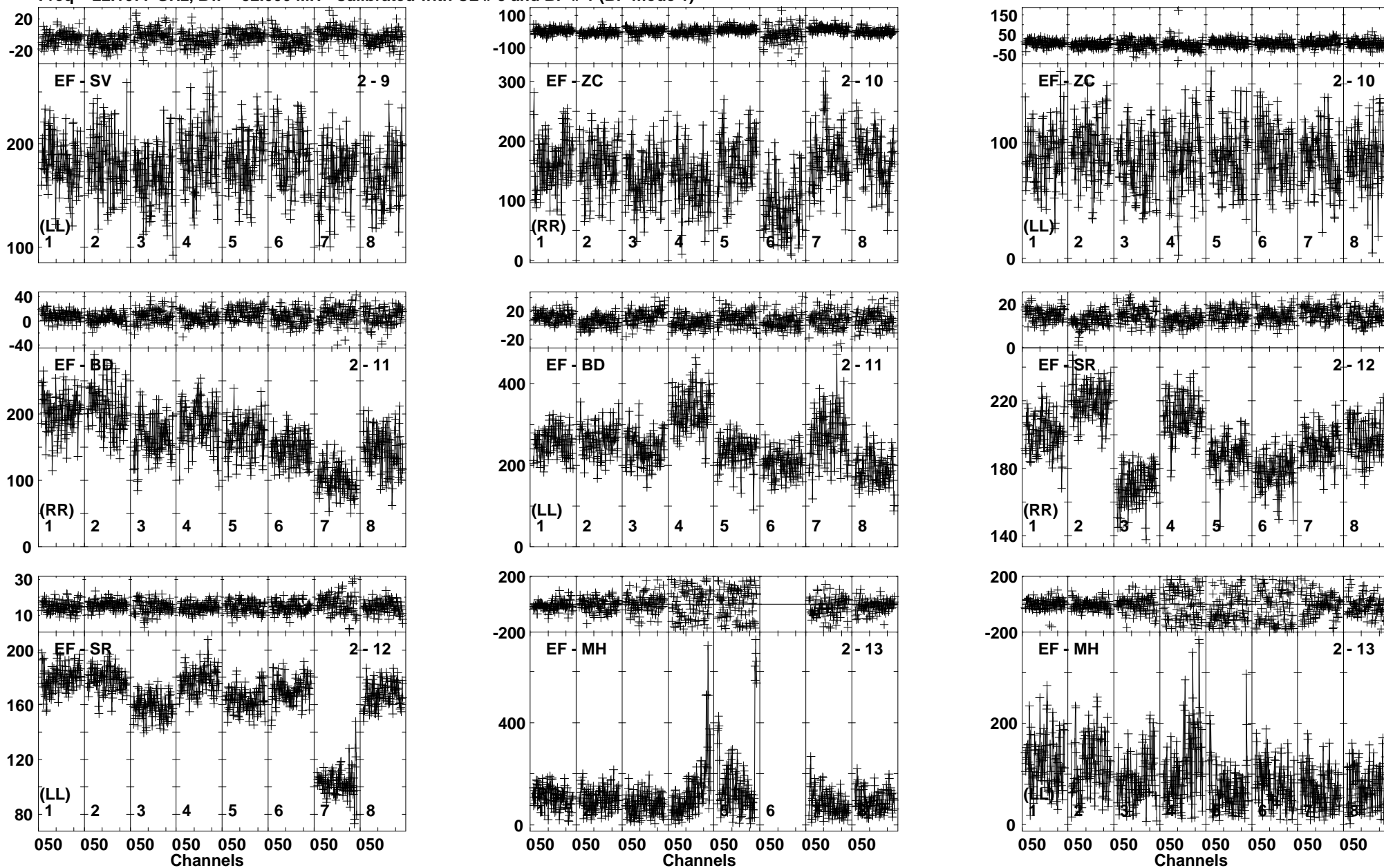
Lower frame: Milli Ampl Jy Top frame: Phas deg Vector averaged cross-power spectrum Baseline: EF (02) - SV (09) Timerange: 00/14:29:51 to 00/14:33:31
