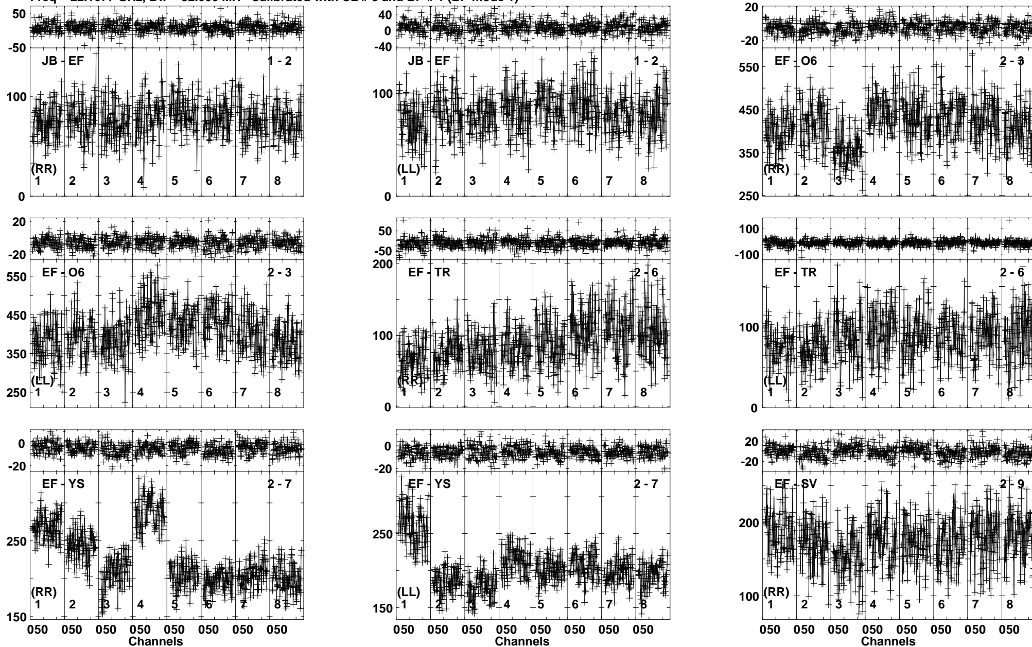
Lower frame: Milli Ampl Jy Top frame: Phas deg Vector averaged cross-power spectrum Baseline: JB (01) - EF (02) Timerange: 00/06:17:31 to 00/06:21:01
