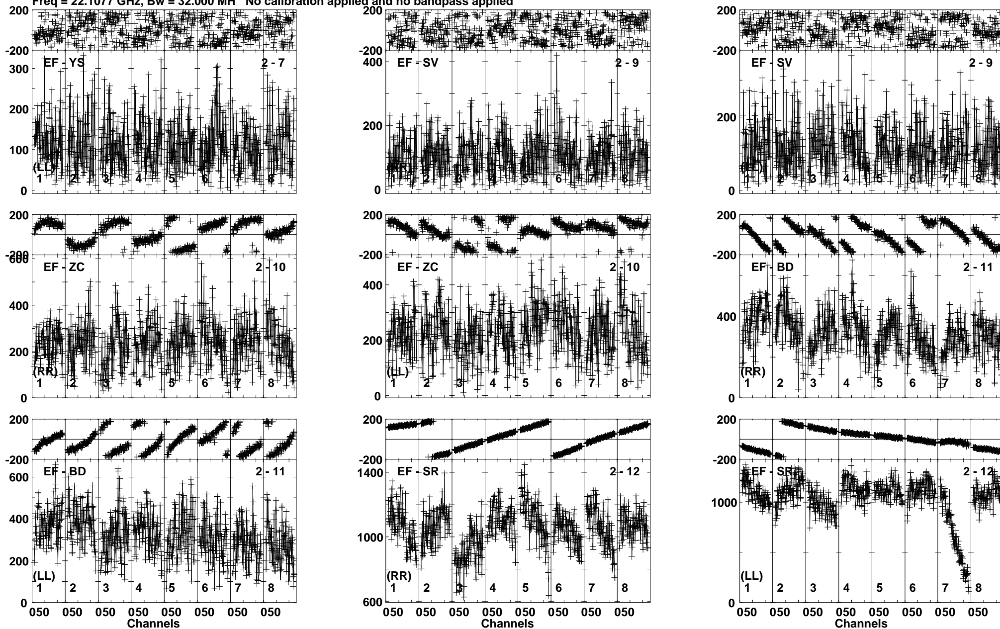
Lower frame: Micro Ampl Jy Top frame: Phas deg Vector averaged cross-power spectrum Baseline: EF (02) - YS (07) Timerange: 00/16:20:55 to 00/16:24:34
