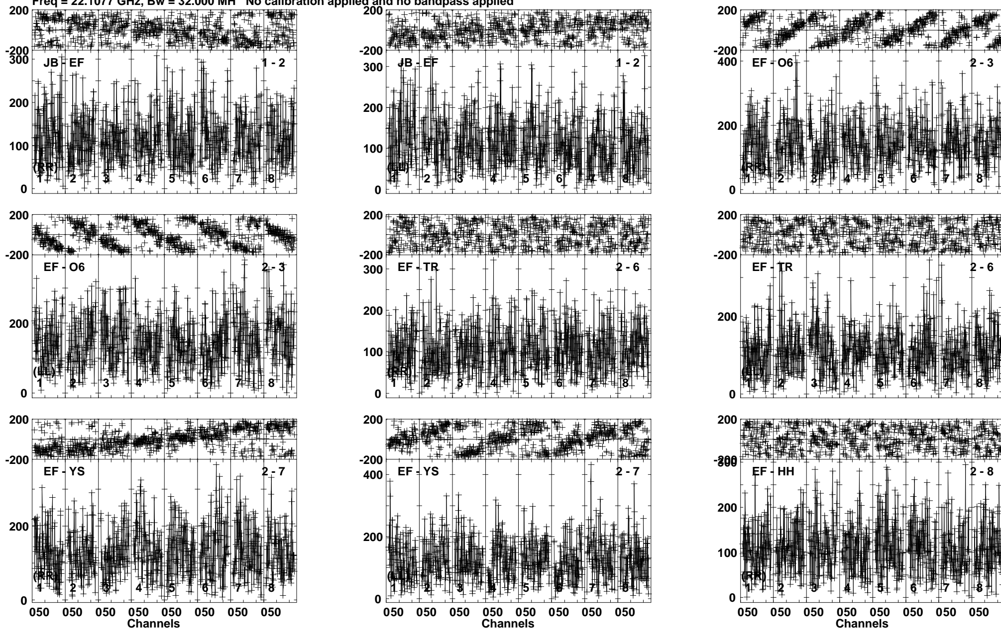
Lower frame: Micro Ampl Jy Top frame: Phas deg Vector averaged cross-power spectrum Baseline: JB (01) - EF (02) Timerange: 00/16:39:38 to 00/16:43:17
