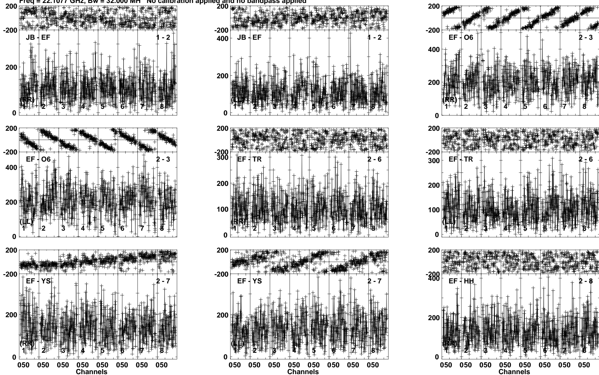
Lower frame: Micro Ampl Jy Top frame: Phas deg Vector averaged cross-power spectrum Baseline: JB (01) - EF (02) Timerange: 00/15:17:04 to 00/15:20:44
