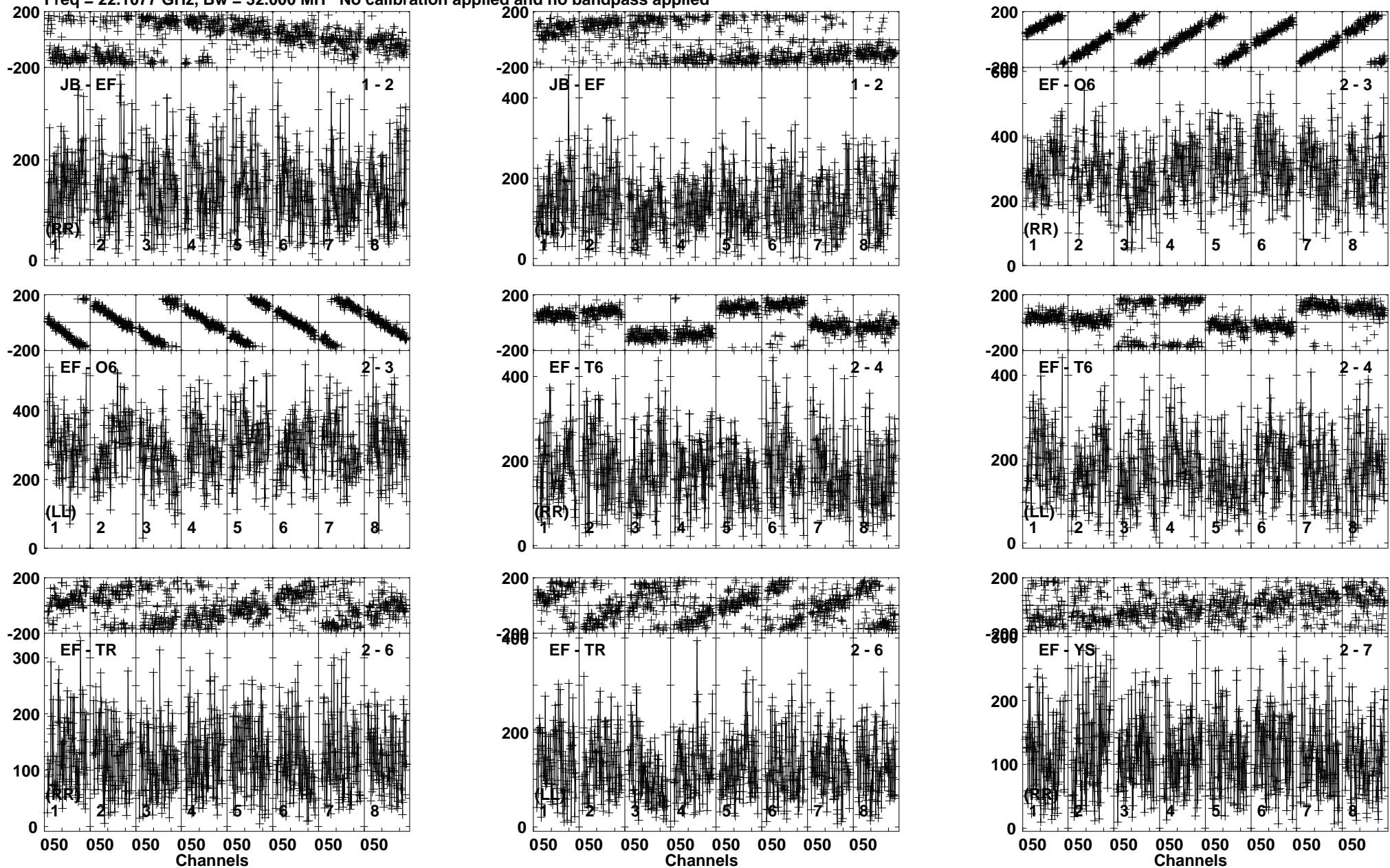
Lower frame: Micro Ampl Jy Top frame: Phas deg Vector averaged cross-power spectrum Baseline: JB (01) - EF (02) Timerange: 00/16:20:55 to 00/16:24:34
