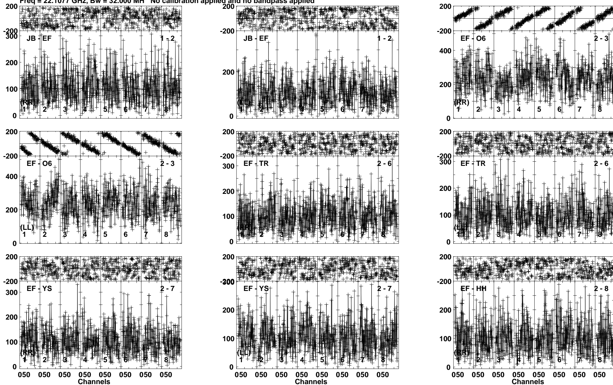
Lower frame: Micro Ampl Jy Top frame: Phas deg Vector averaged cross-power spectrum Baseline: JB (01) - EF (02) Timerange: 00/14:12:09 to 00/14:15:49
