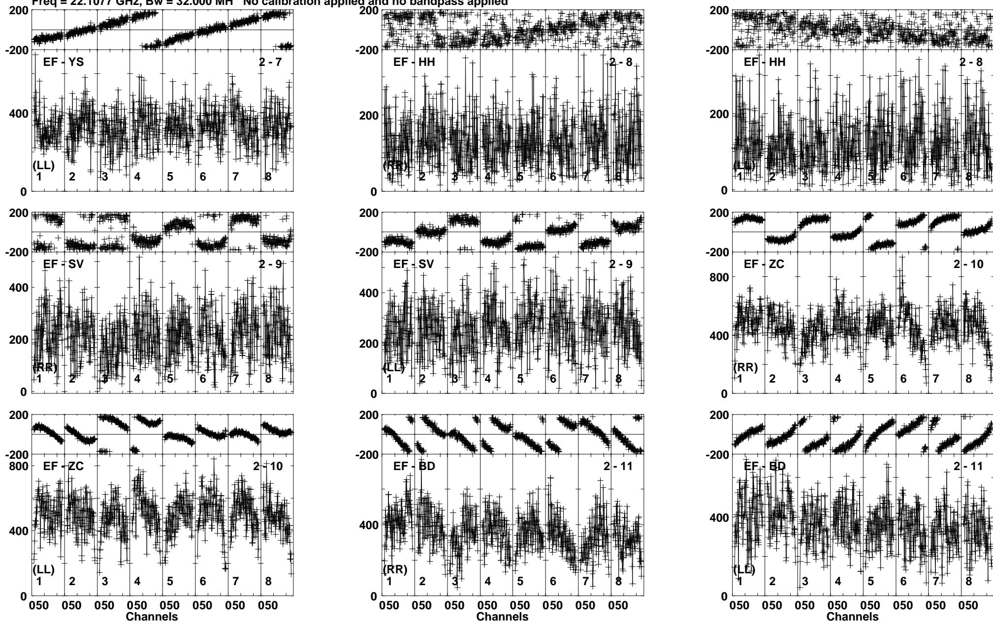
Lower frame: Micro Ampl Jy Top frame: Phas deg Vector averaged cross-power spectrum Baseline: EF (02) - YS (07) Timerange: 00/10:22:17 to 00/10:25:46
