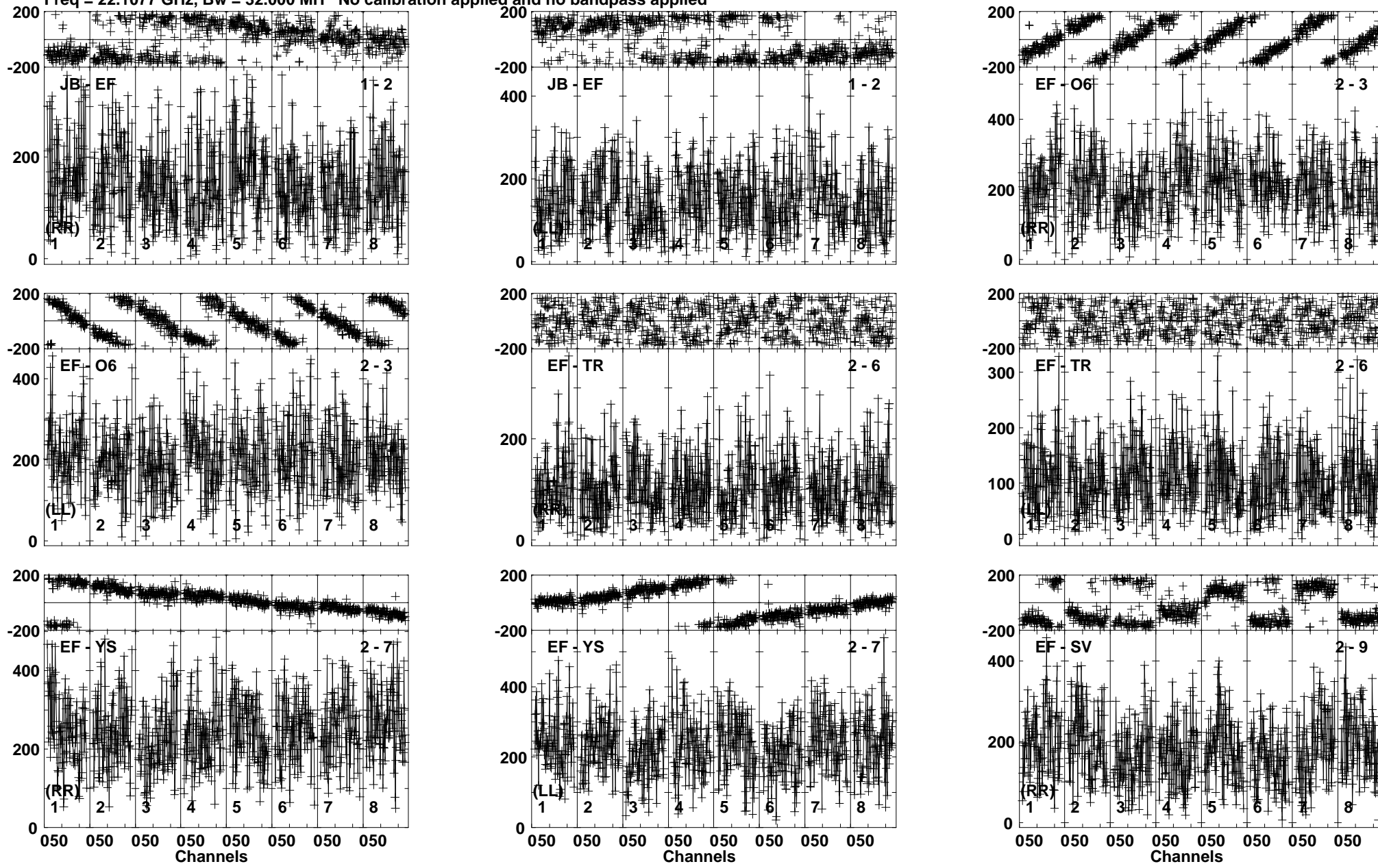
Lower frame: Micro Ampl Jy Top frame: Phas deg Vector averaged cross-power spectrum Baseline: JB (01) - EF (02) Timerange: 00/07:37:14 to 00/07:40:44
