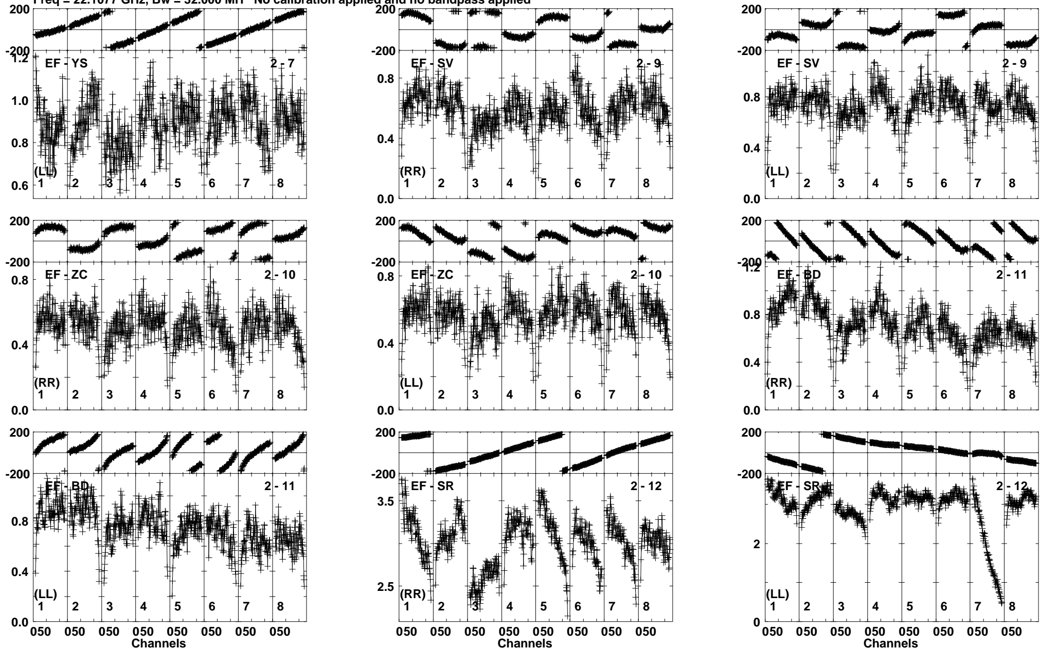
Lower frame: Milli Ampl Jy Top frame: Phas deg Vector averaged cross-power spectrum Baseline: EF (02) - YS (07) Timerange: 00/16:06:22 to 00/16:10:00
