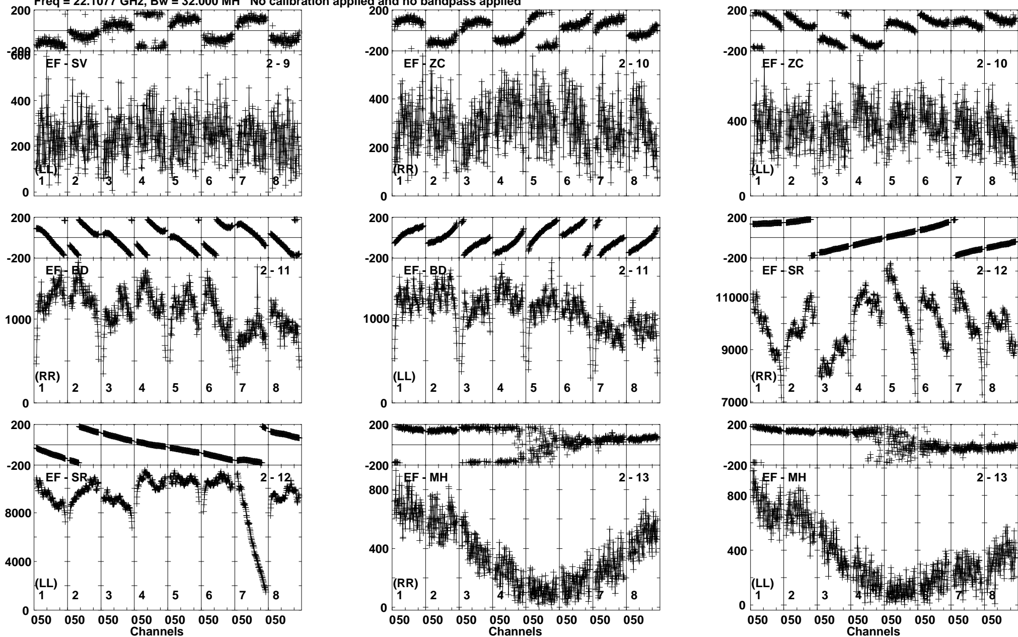
Lower frame: Micro Ampl Jy Top frame: Phas deg Vector averaged cross-power spectrum Baseline: EF (02) - SV (09) Timerange: 00/06:29:08 to 00/06:32:37
