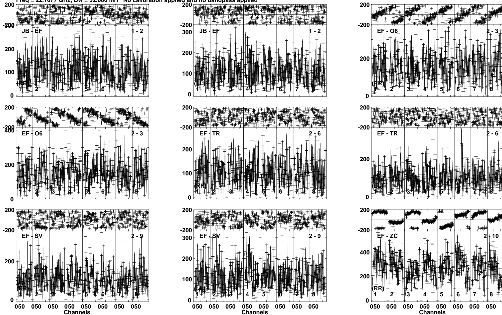
Lower frame: Micro Ampl Jy Top frame: Phas deg Vector averaged cross-power spectrum Baseline: JB (01) - EF (02) Timerange: 00/08:09:37 to 00/08:13:07
