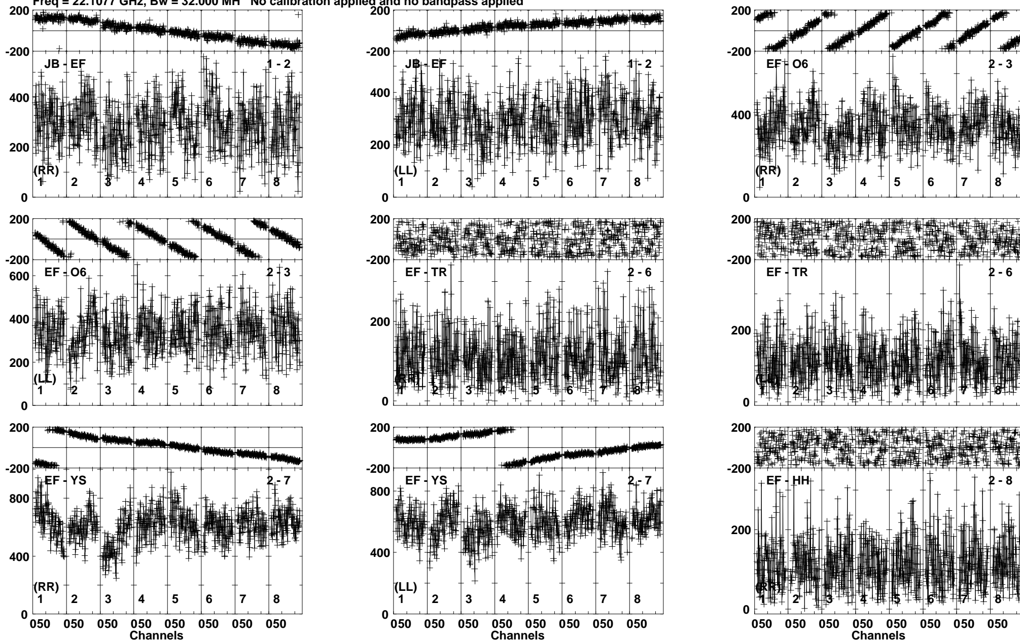
Lower frame: Micro Ampl Jy Top frame: Phas deg Vector averaged cross-power spectrum Baseline: JB (01) - EF (02) Timerange: 00/07:01:28 to 00/07:04:57
