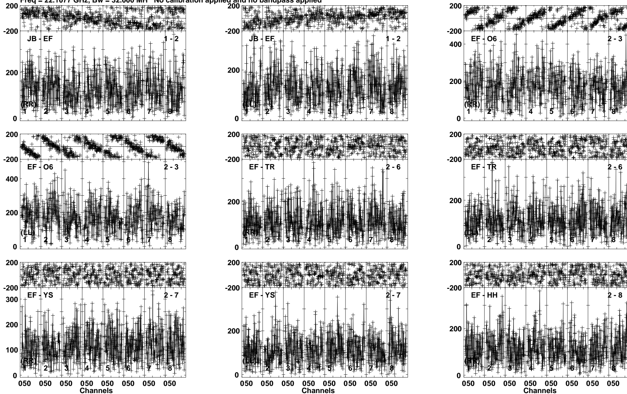
Lower frame: Micro Ampl Jy Top frame: Phas deg Vector averaged cross-power spectrum Baseline: JB (01) - EF (02) Timerange: 00/10:17:15 to 00/10:20:44
