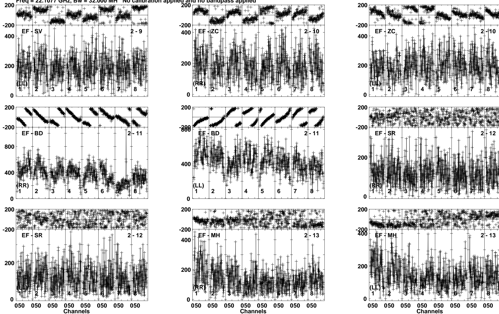
Lower frame: Micro Ampl Jy Top frame: Phas deg Vector averaged cross-power spectrum Baseline: EF (02) - SV (09) Timerange: 00/09:56:18 to 00/09:59:47
