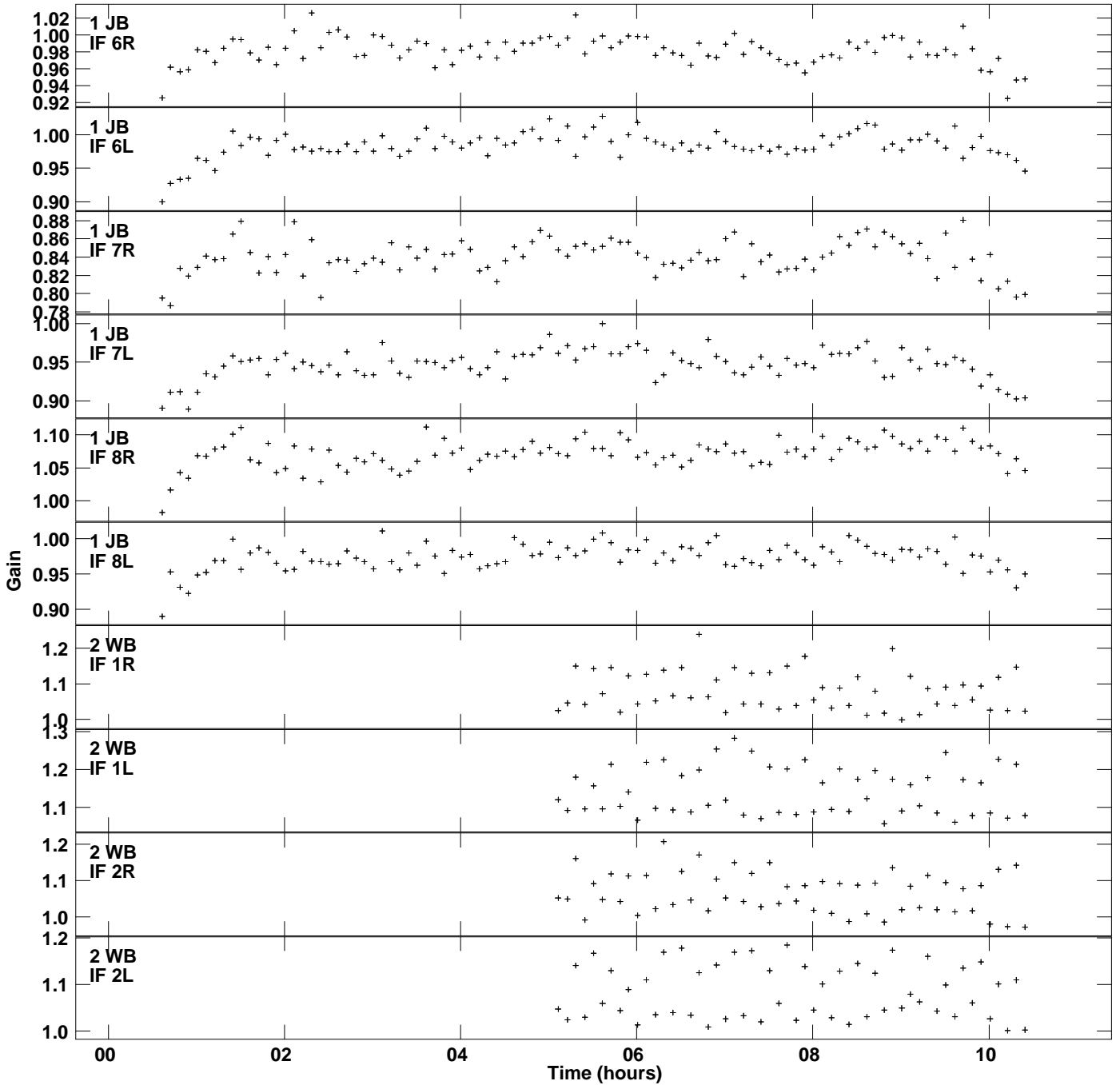
Plot file version 2 created 17-FEB-2020 16:07:19 Gain amp vs UTC time for J1359+5544.MULTI.1 SN 2 Rpol & Lpol IF 1 - 8
