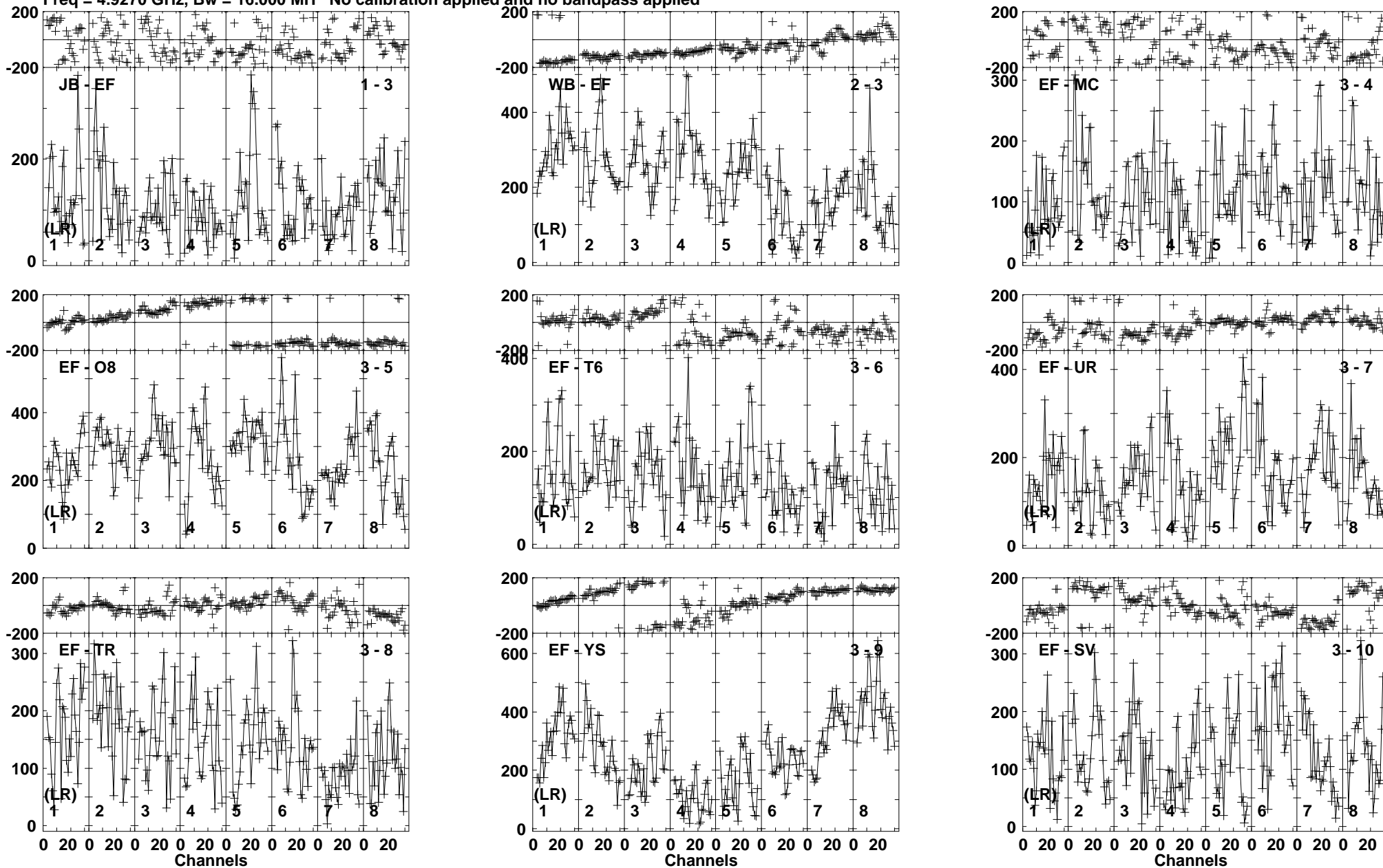
Lower frame: Micro Ampl Jy Top frame: Phas deg Vector averaged cross-power spectrum Baseline: JB (01) - EF (03) Timerange: 00/07:05:21 to 00/07:07:19
