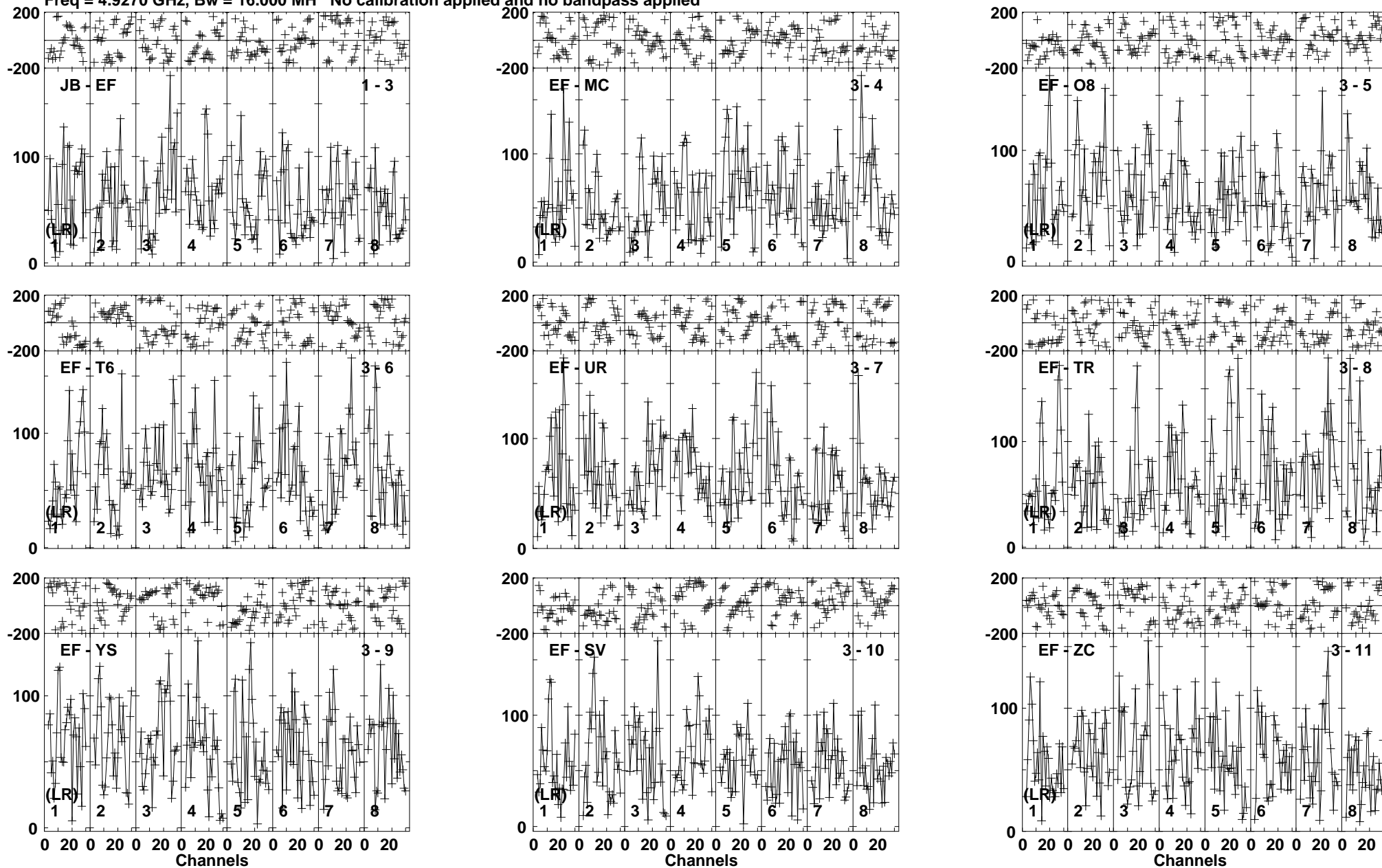
Lower frame: Micro Ampl Jy Top frame: Phas deg Vector averaged cross-power spectrum Baseline: JB (01) - EF (03) Timerange: 00/04:07:23 to 00/04:11:19
