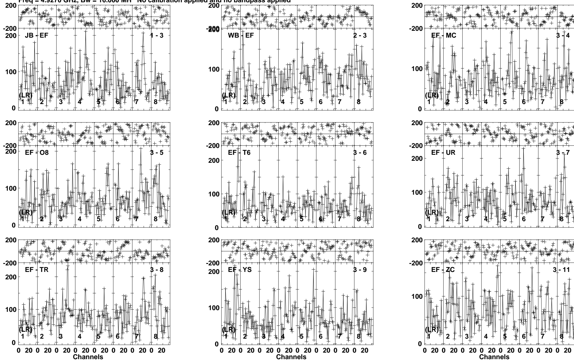
Lower frame: Micro Ampl Jy Top frame: Phas deg Vector averaged cross-power spectrum Baseline: JB (01) - EF (03) Timerange: 00/10:07:21 to 00/10:11:19
