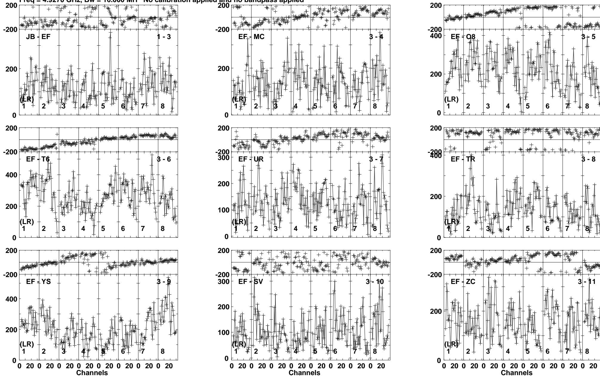
Lower frame: Micro Ampl Jy Top frame: Phas deg Vector averaged cross-power spectrum Baseline: JB (01) - EF (03) Timerange: 00/02:05:21 to 00/02:07:19
