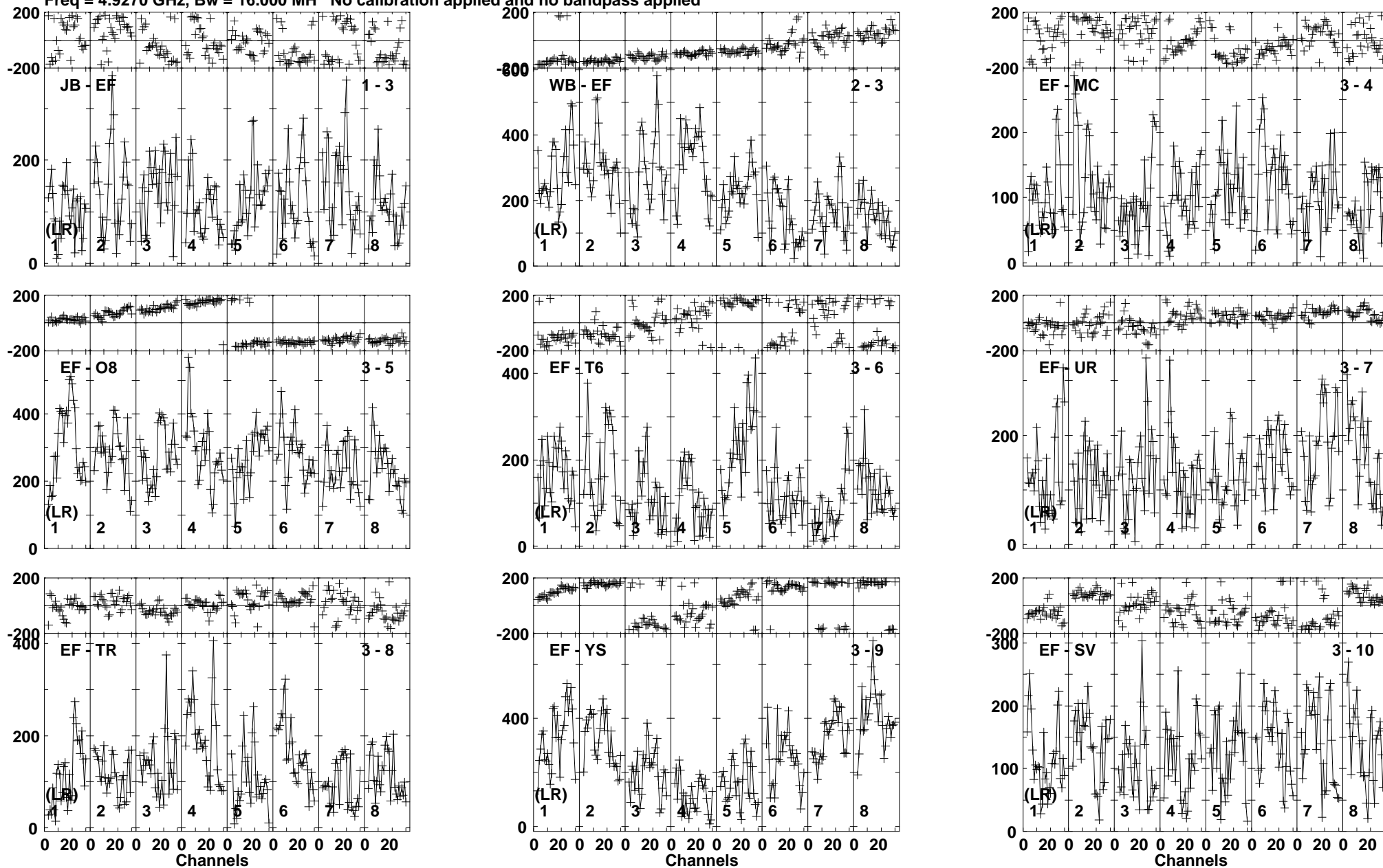
Lower frame: Micro Ampl Jy Top frame: Phas deg Vector averaged cross-power spectrum Baseline: JB (01) - EF (03) Timerange: 00/06:48:01 to 00/06:49:19
