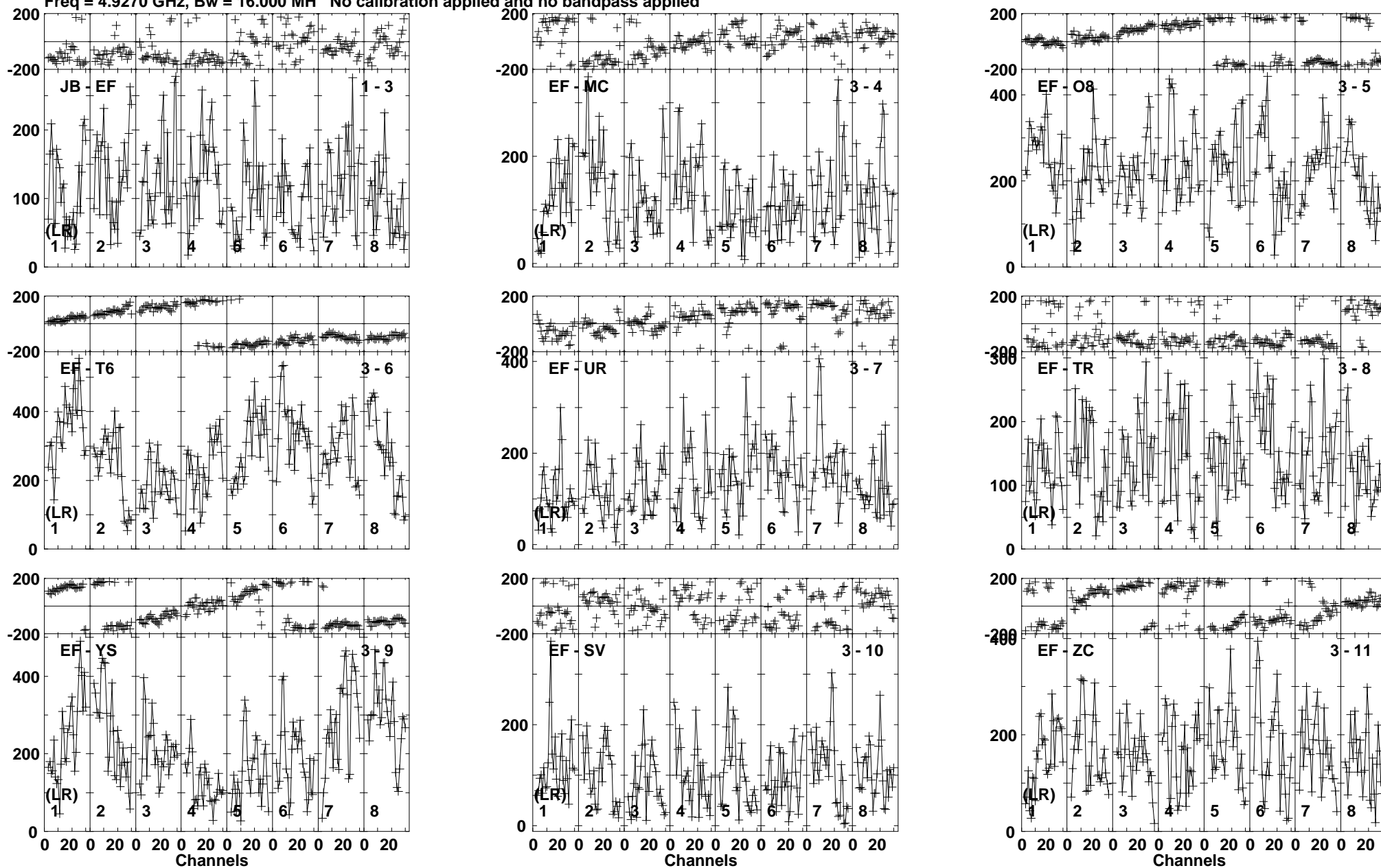
Lower frame: Micro Ampl Jy Top frame: Phas deg Vector averaged cross-power spectrum Baseline: JB (01) - EF (03) Timerange: 00/02:17:21 to 00/02:19:19
