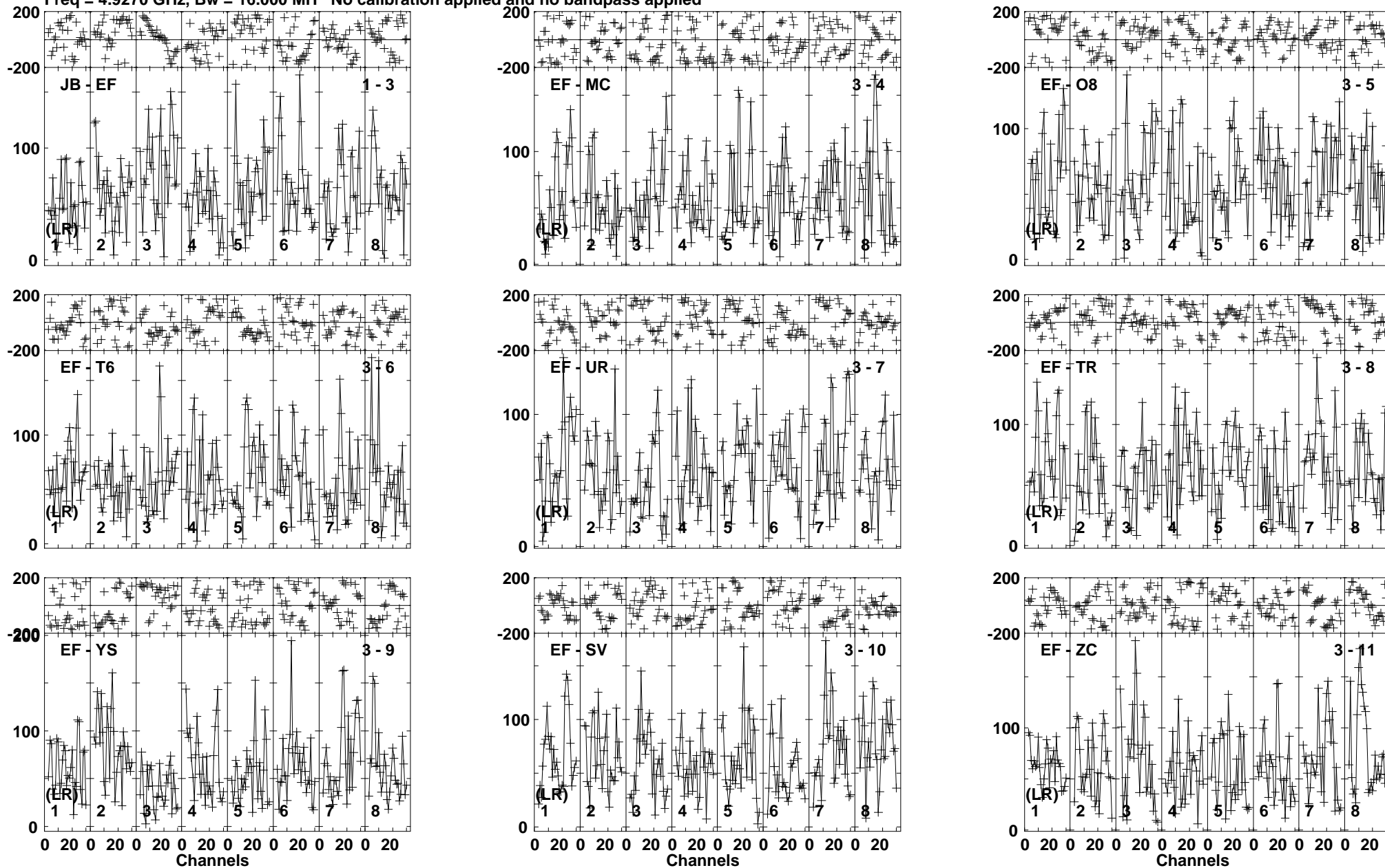
Lower frame: Micro Ampl Jy Top frame: Phas deg Vector averaged cross-power spectrum Baseline: JB (01) - EF (03) Timerange: 00/04:13:21 to 00/04:17:19
