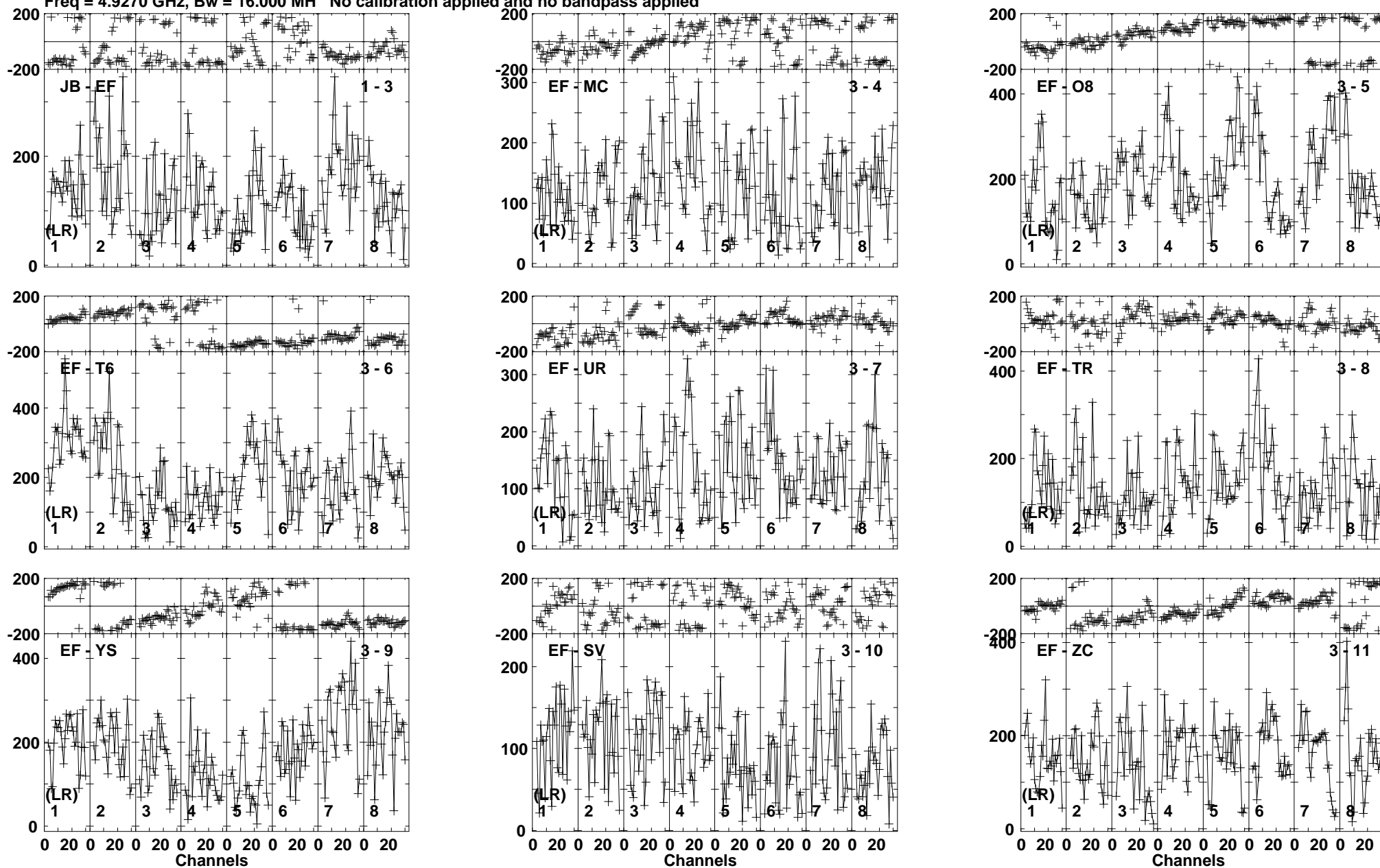
Lower frame: Micro Ampl Jy Top frame: Phas deg Vector averaged cross-power spectrum Baseline: JB (01) - EF (03) Timerange: 00/01:17:21 to 00/01:19:19
