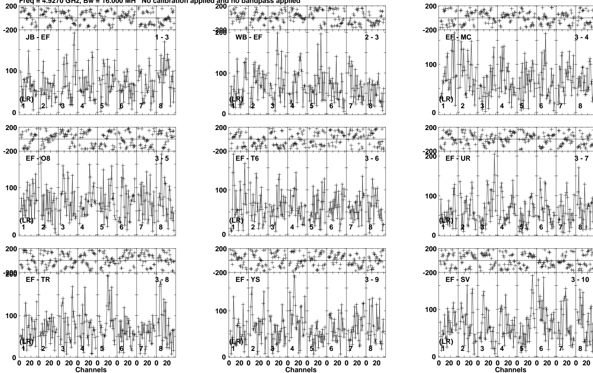
Lower frame: Micro Ampl Jy Top frame: Phas deg Vector averaged cross-power spectrum Baseline: JB (01) - EF (03) Timerange: 00/08:37:21 to 00/08:41:19
