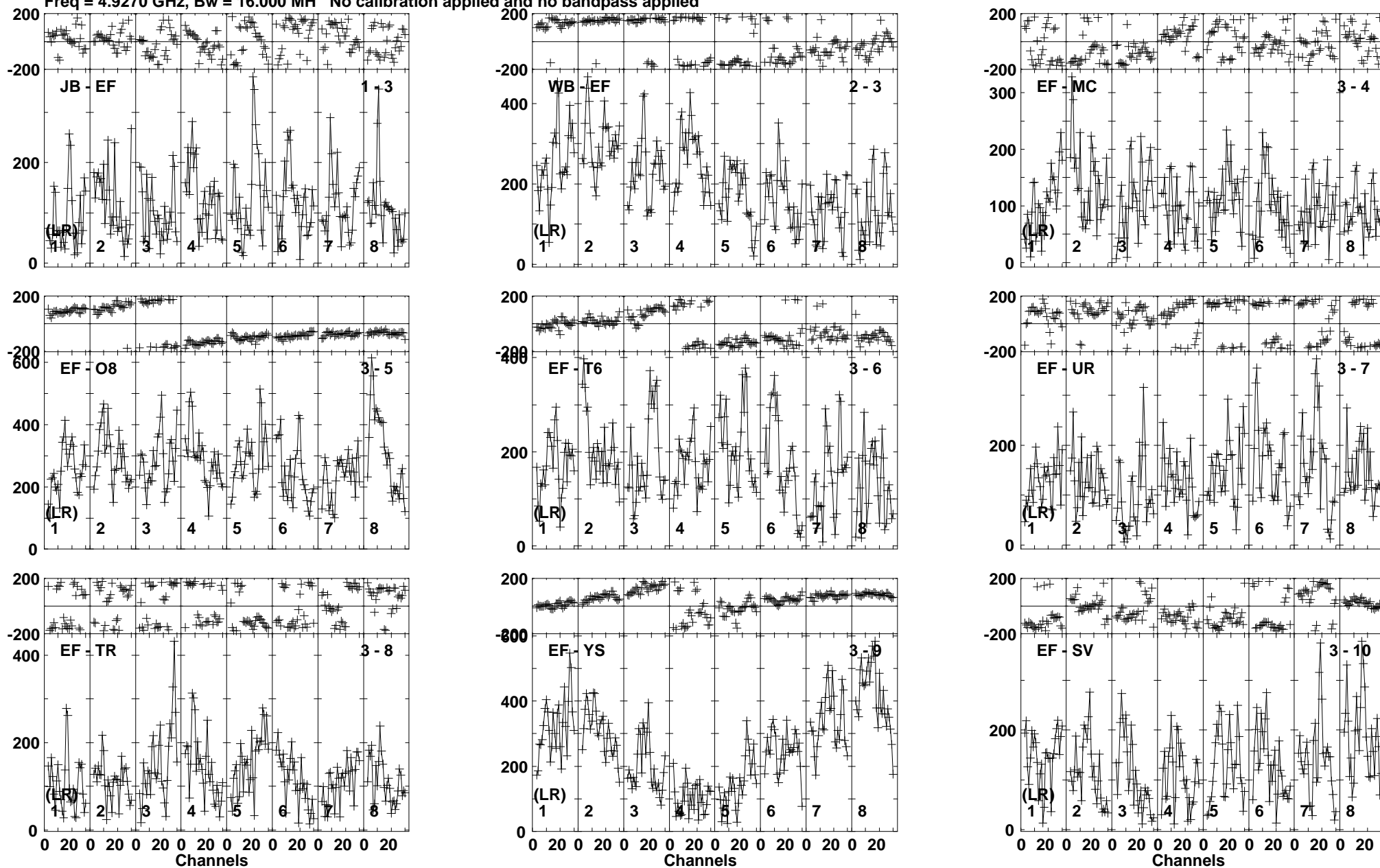
Lower frame: Micro Ampl Jy Top frame: Phas deg Vector averaged cross-power spectrum Baseline: JB (01) - EF (03) Timerange: 00/06:17:21 to 00/06:19:19
