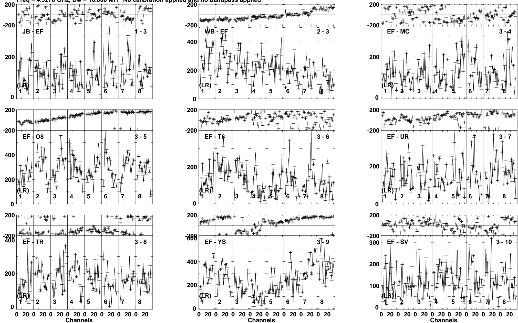
Lower frame: Micro Ampl Jy Top frame: Phas deg Vector averaged cross-power spectrum Baseline: JB (01) - EF (03) Timerange: 00/08:17:21 to 00/08:19:19
