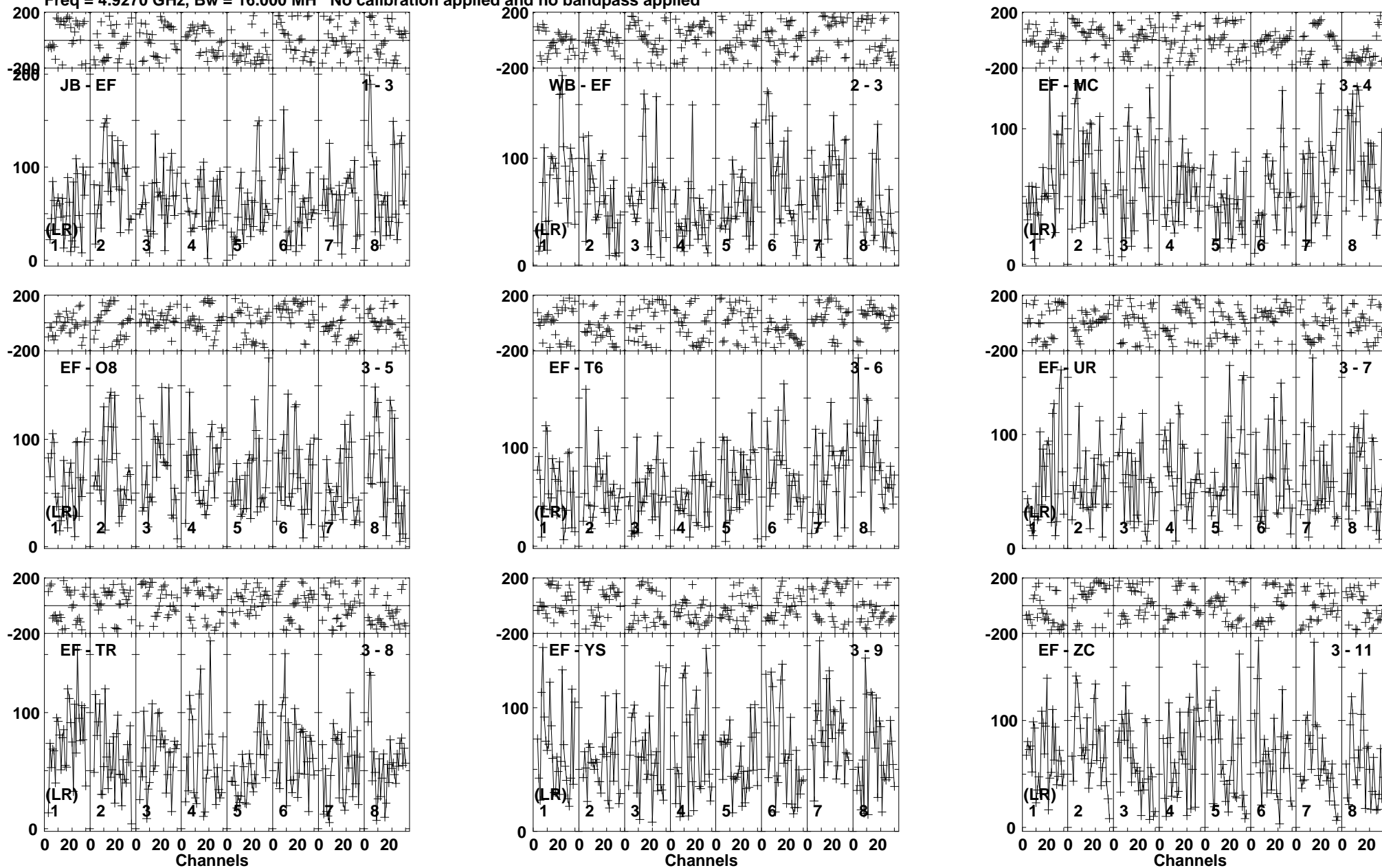
Lower frame: Micro Ampl Jy Top frame: Phas deg Vector averaged cross-power spectrum Baseline: JB (01) - EF (03) Timerange: 00/09:01:21 to 00/09:05:19
