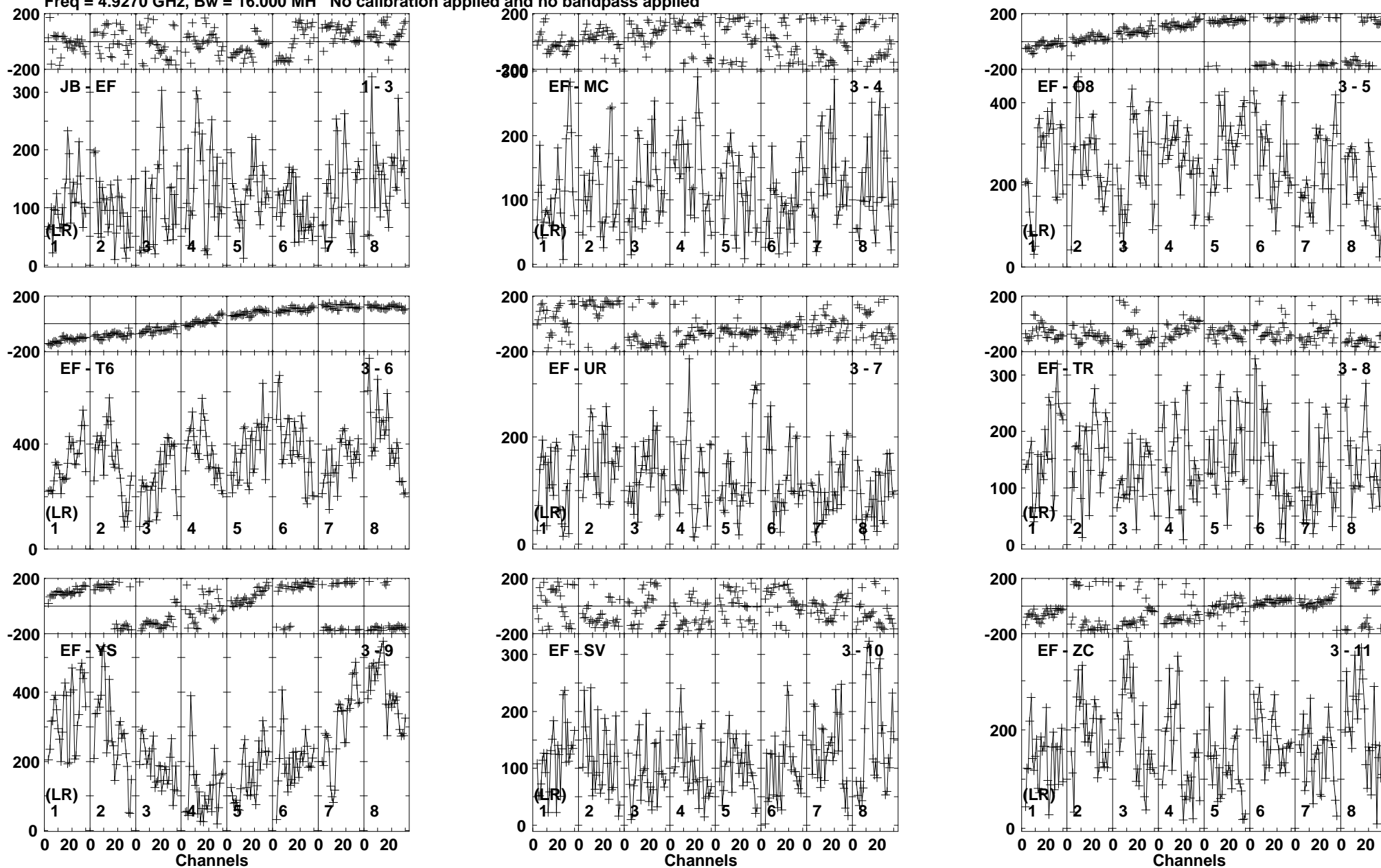
Lower frame: Micro Ampl Jy Top frame: Phas deg Vector averaged cross-power spectrum Baseline: JB (01) - EF (03) Timerange: 00/03:41:21 to 00/03:43:19
