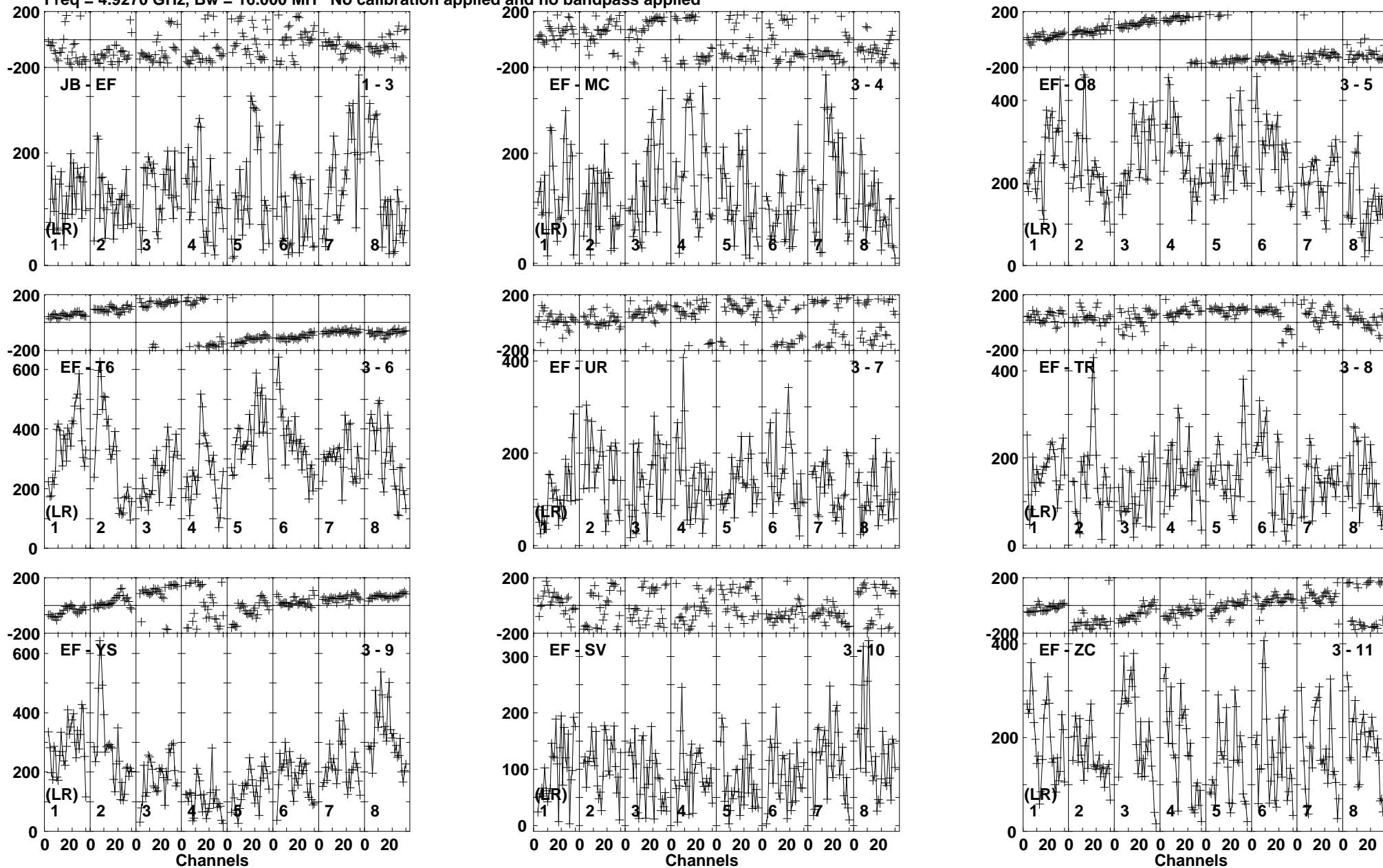
Lower frame: Micro Ampl Jy Top frame: Phas deg Vector averaged cross-power spectrum Baseline: JB (01) - EF (03) Timerange: 00/02:41:21 to 00/02:43:19
