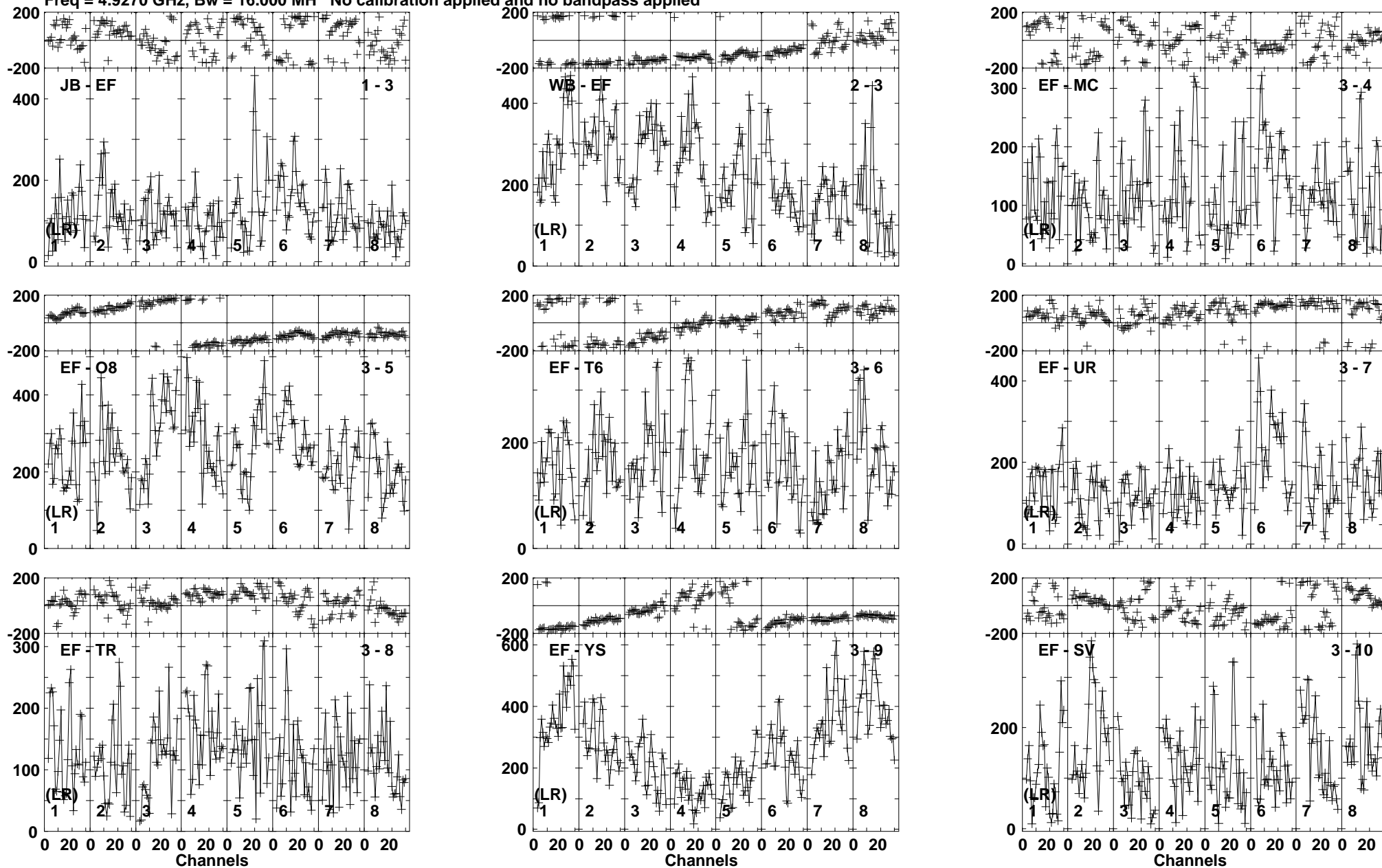
Lower frame: Micro Ampl Jy Top frame: Phas deg Vector averaged cross-power spectrum Baseline: JB (01) - EF (03) Timerange: 00/06:36:01 to 00/06:37:19
