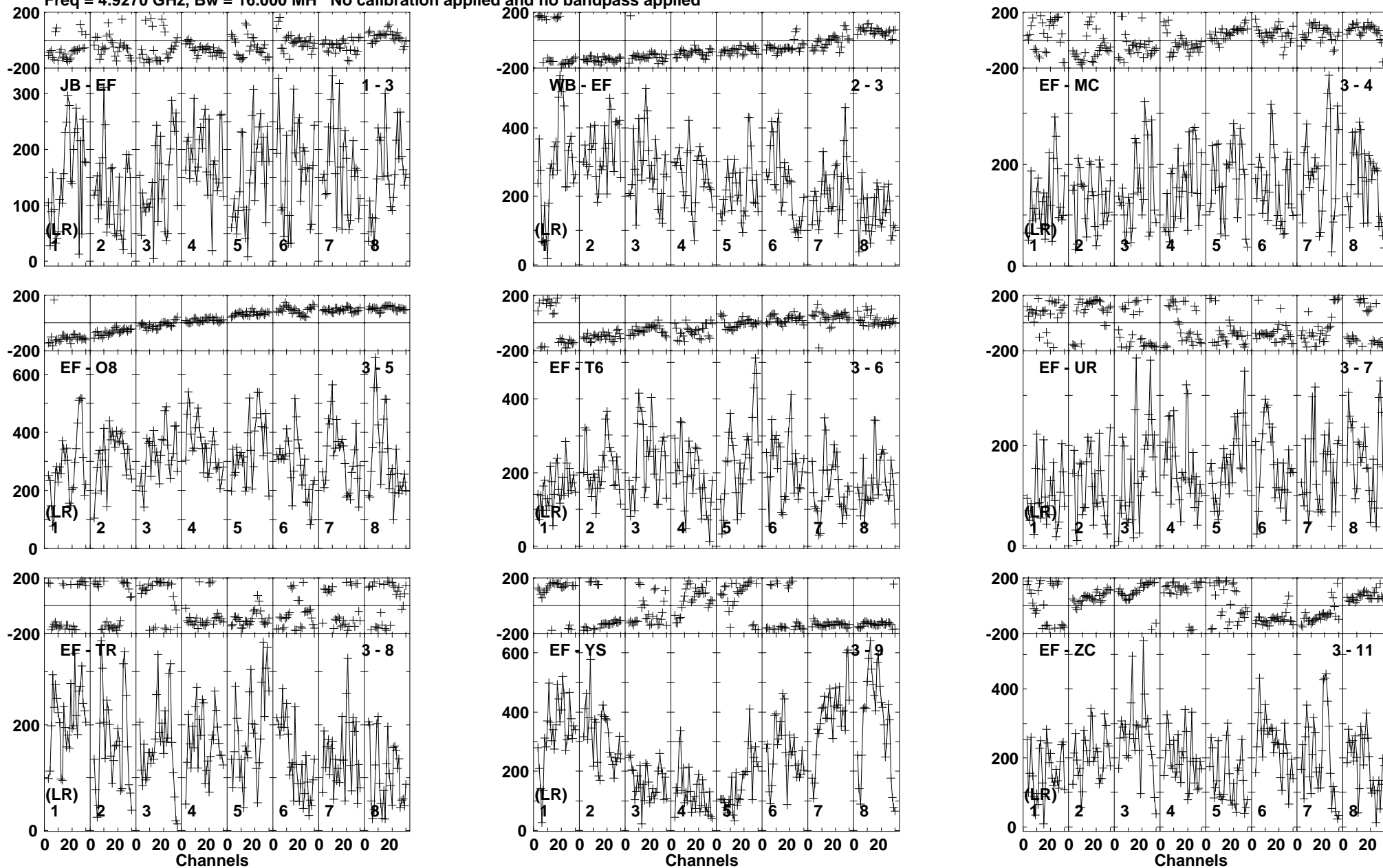
Lower frame: Micro Ampl Jy Top frame: Phas deg Vector averaged cross-power spectrum Baseline: JB (01) - EF (03) Timerange: 00/09:36:01 to 00/09:37:19
