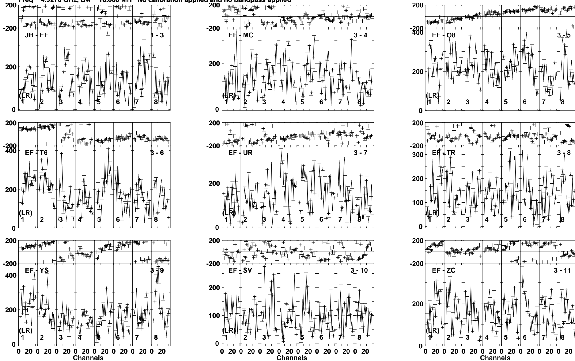
Lower frame: Micro Ampl Jy Top frame: Phas deg Vector averaged cross-power spectrum Baseline: JB (01) - EF (03) Timerange: 00/01:00:01 to 00/01:01:19
