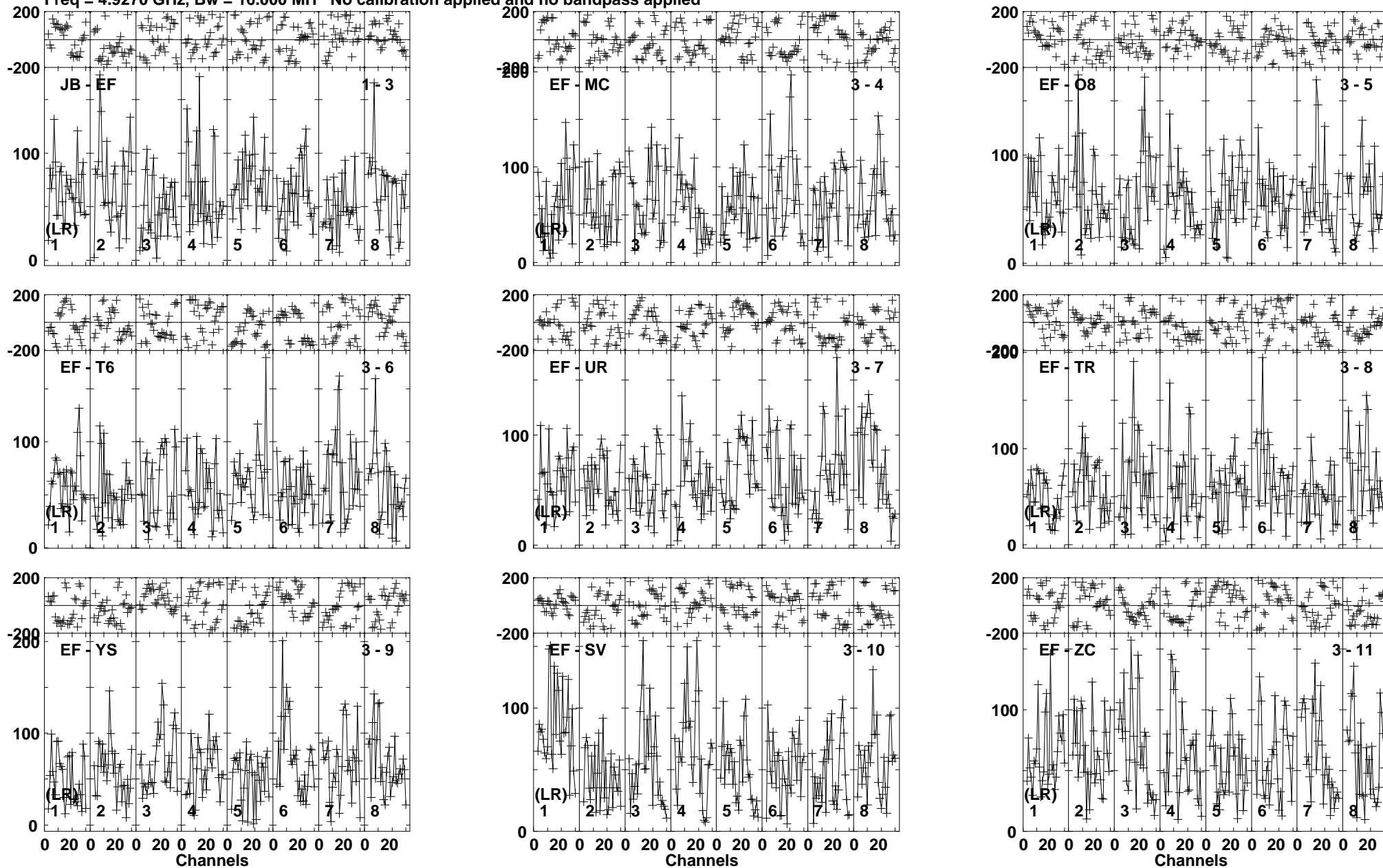
Lower frame: Micro Ampl Jy Top frame: Phas deg Vector averaged cross-power spectrum Baseline: JB (01) - EF (03) Timerange: 00/02:01:21 to 00/02:05:19
