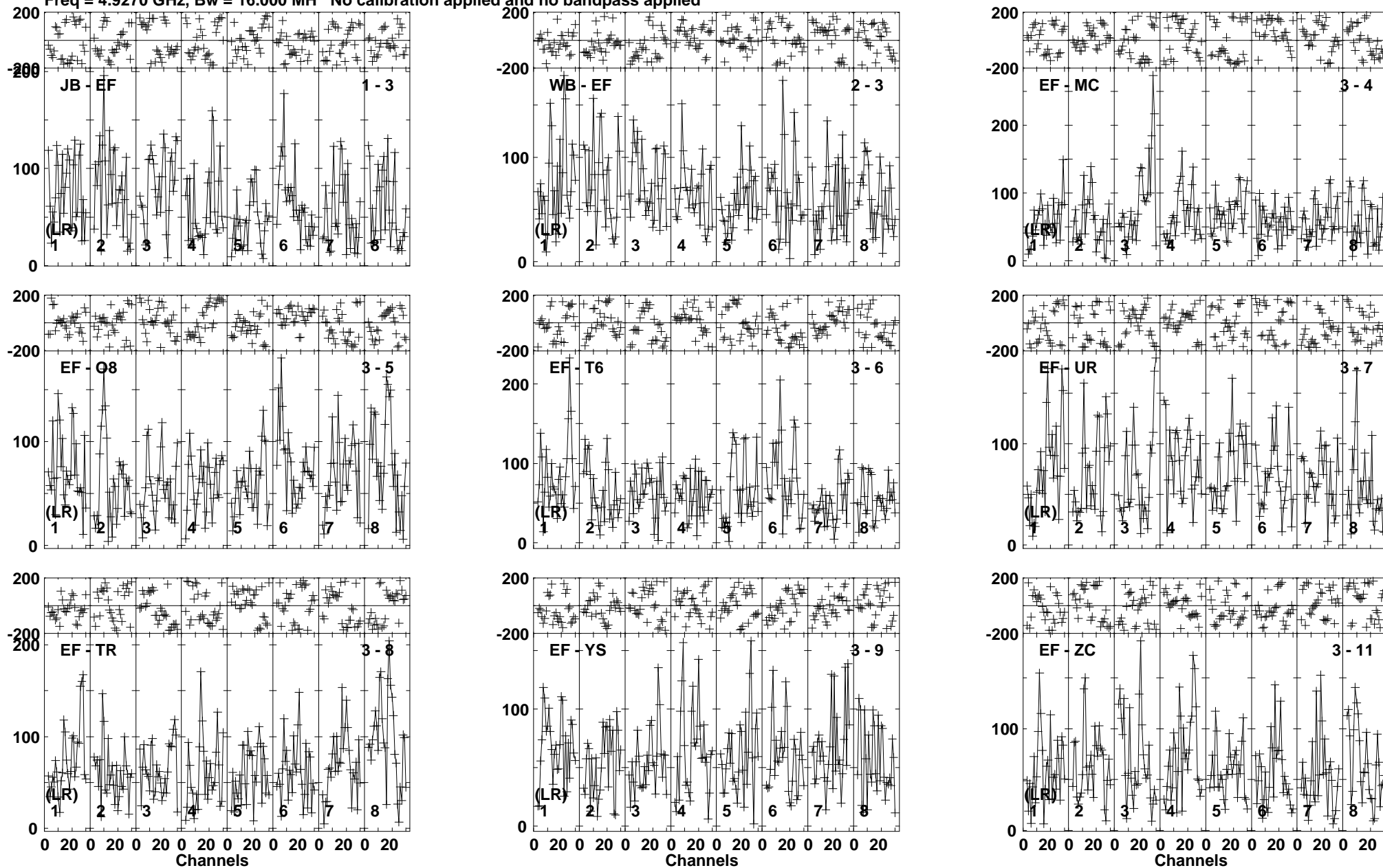
Lower frame: Micro Ampl Jy Top frame: Phas deg Vector averaged cross-power spectrum Baseline: JB (01) - EF (03) Timerange: 00/09:19:21 to 00/09:23:19
