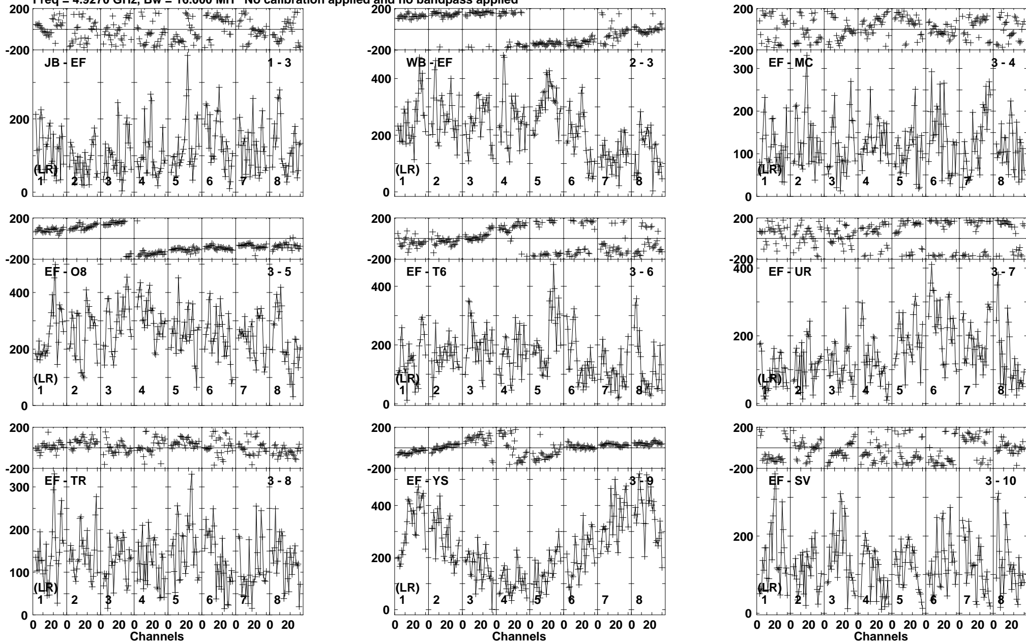
Lower frame: Micro Ampl Jy Top frame: Phas deg Vector averaged cross-power spectrum Baseline: JB (01) - EF (03) Timerange: 00/06:24:01 to 00/06:25:19
