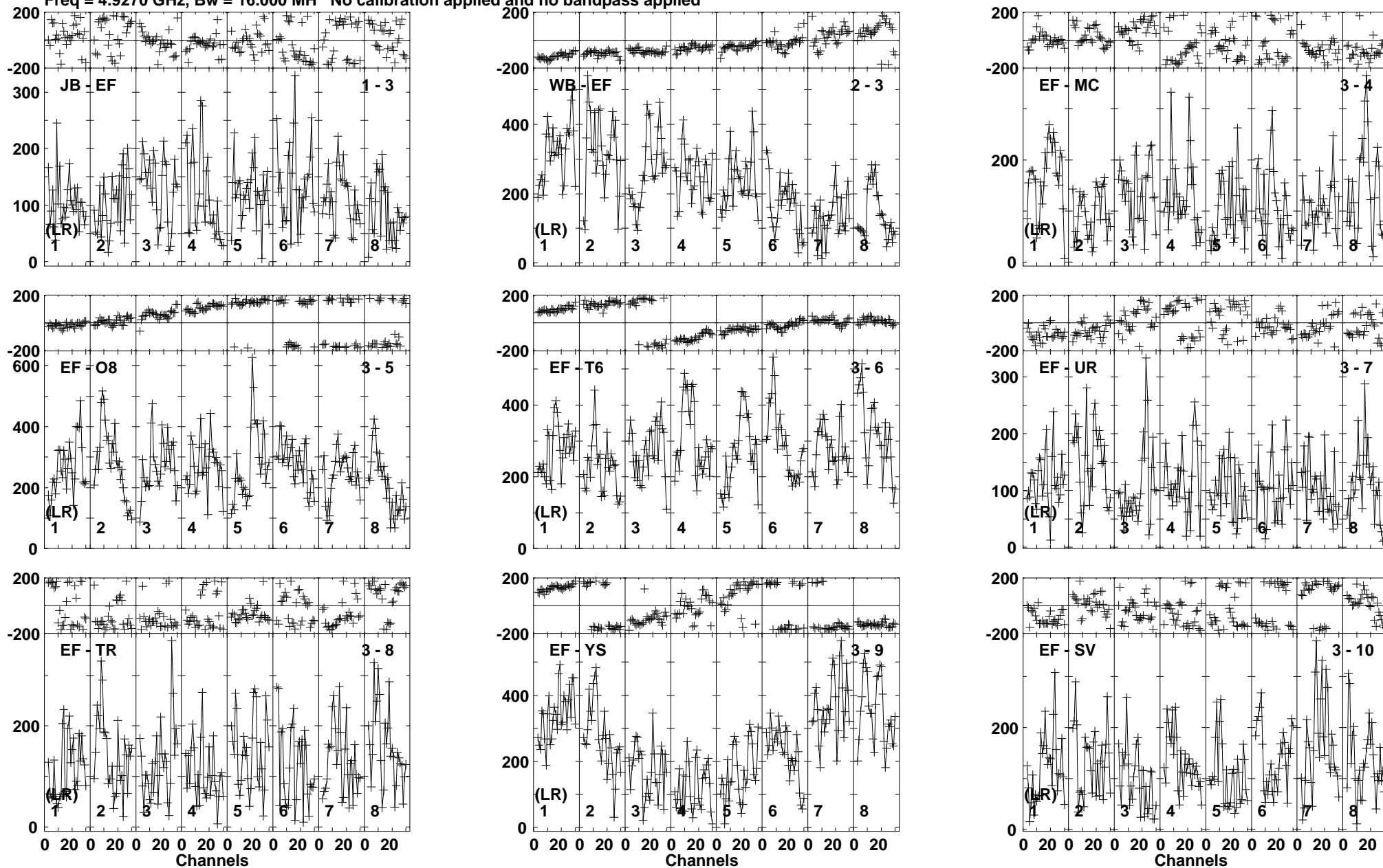
Lower frame: Micro Ampl Jy Top frame: Phas deg Vector averaged cross-power spectrum Baseline: JB (01) - EF (03) Timerange: 00/05:05:21 to 00/05:07:19
