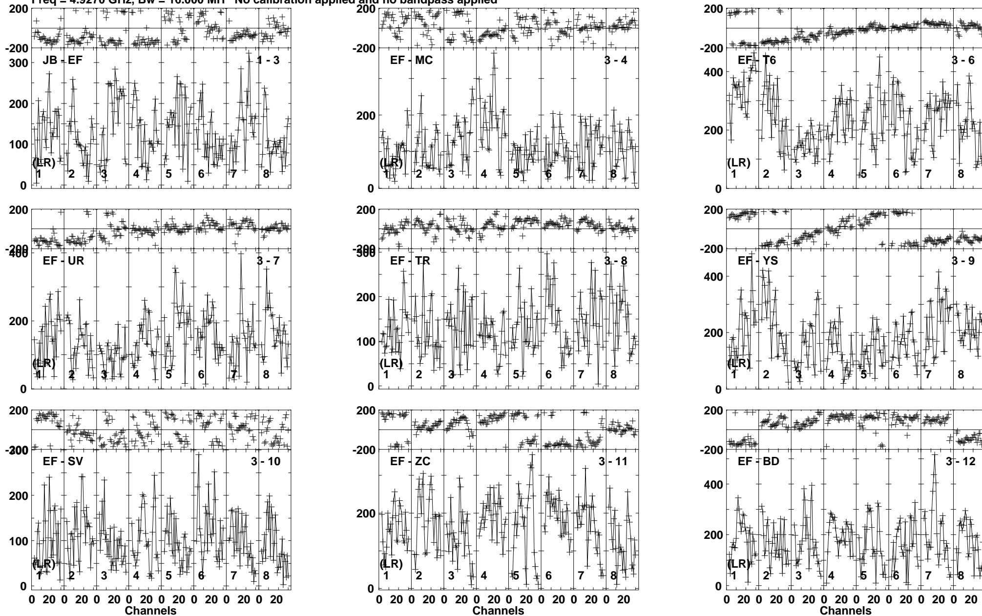
Lower frame: Micro Ampl Jy Top frame: Phas deg Vector averaged cross-power spectrum Baseline: JB (01) - EF (03) Timerange: 00/01:36:01 to 00/01:37:19
