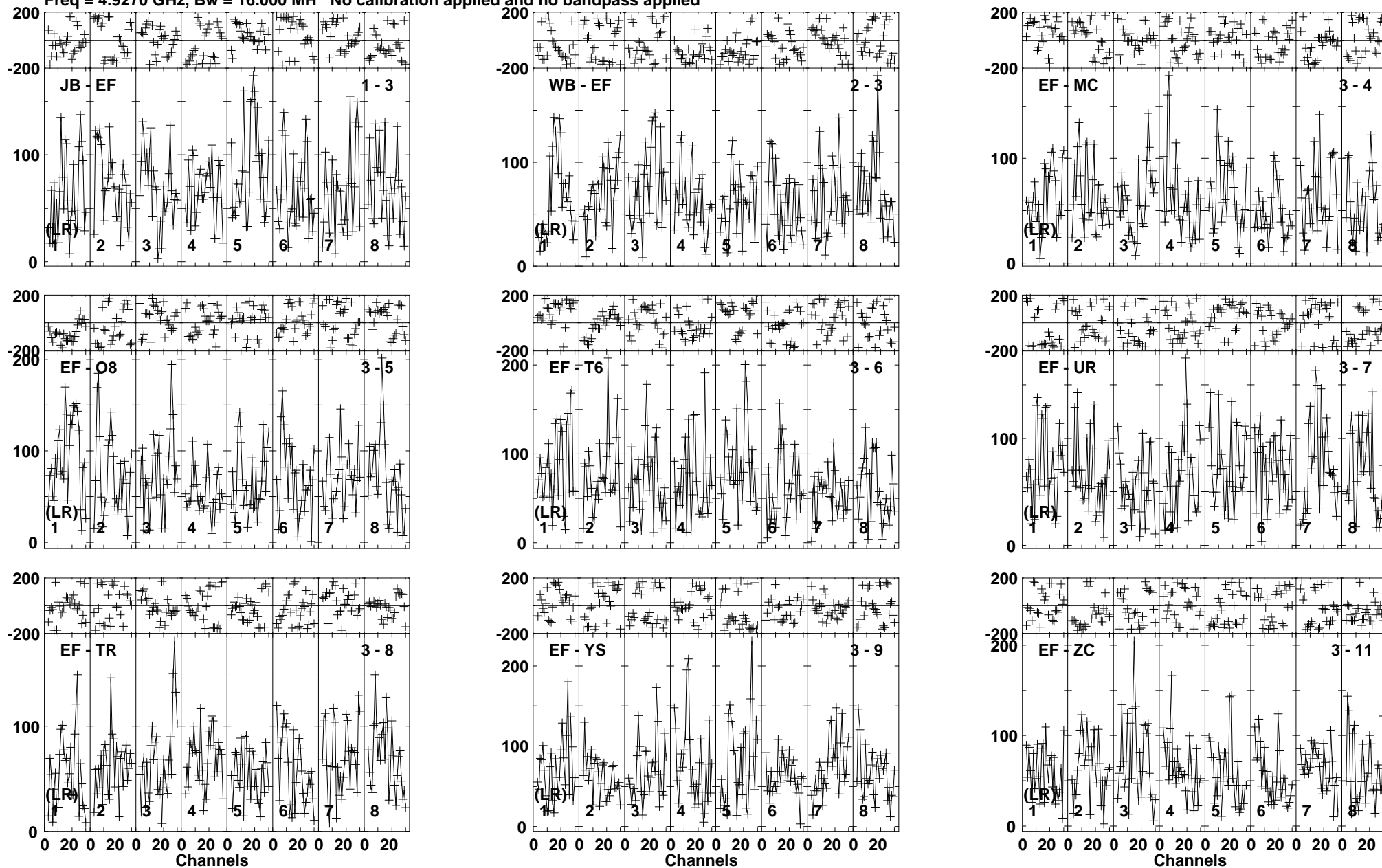
Lower frame: Micro Ampl Jy Top frame: Phas deg Vector averaged cross-power spectrum Baseline: JB (01) - EF (03) Timerange: 00/09:49:21 to 00/09:53:19
