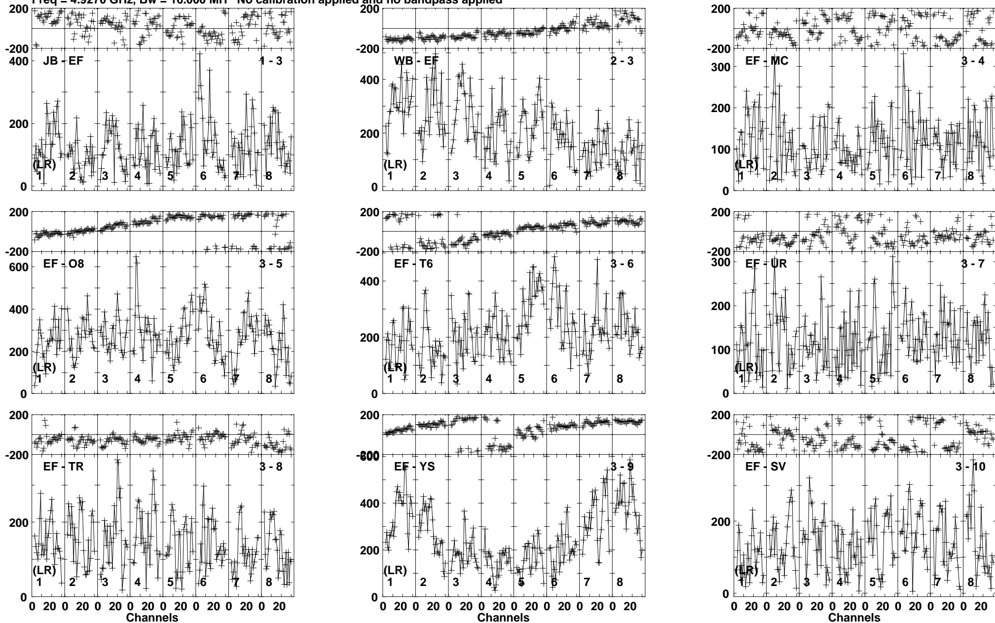
Lower frame: Micro Ampl Jy Top frame: Phas deg Vector averaged cross-power spectrum Baseline: JB (01) - EF (03) Timerange: 00/05:29:21 to 00/05:31:19
