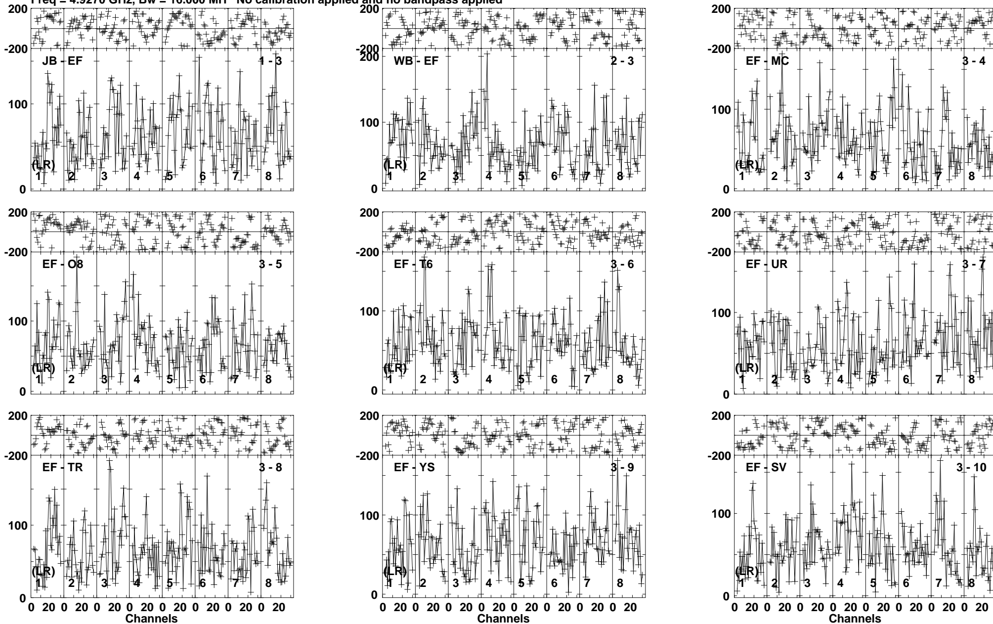
Lower frame: Micro Ampl Jy Top frame: Phas deg Vector averaged cross-power spectrum Baseline: JB (01) - EF (03) Timerange: 00/06:07:23 to 00/06:11:19
