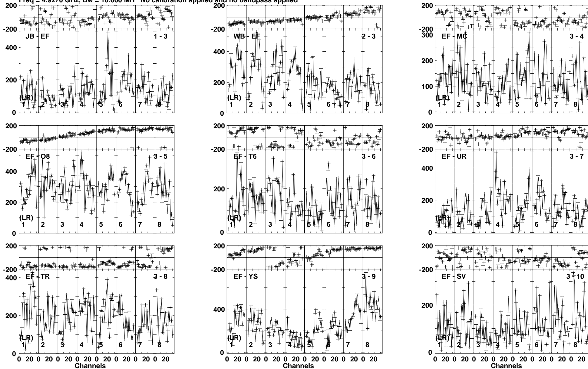
Lower frame: Micro Ampl Jy Top frame: Phas deg Vector averaged cross-power spectrum Baseline: JB (01) - EF (03) Timerange: 00/08:24:01 to 00/08:25:19
