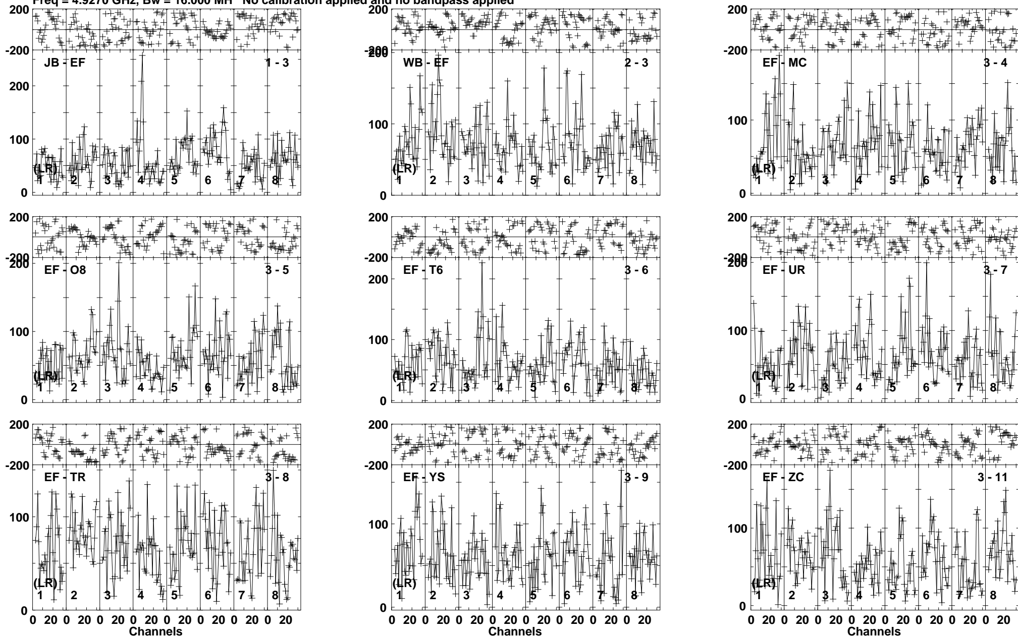
Lower frame: Micro Ampl Jy Top frame: Phas deg Vector averaged cross-power spectrum Baseline: JB (01) - EF (03) Timerange: 00/08:55:21 to 00/08:59:19
