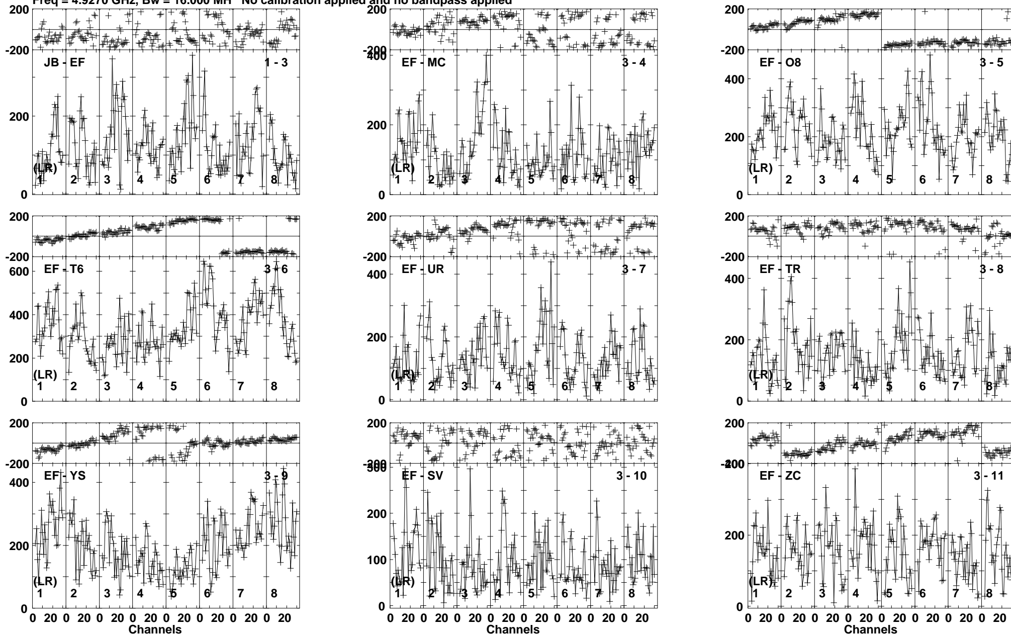
Lower frame: Micro Ampl Jy Top frame: Phas deg Vector averaged cross-power spectrum Baseline: JB (01) - EF (03) Timerange: 00/02:48:01 to 00/02:49:19
