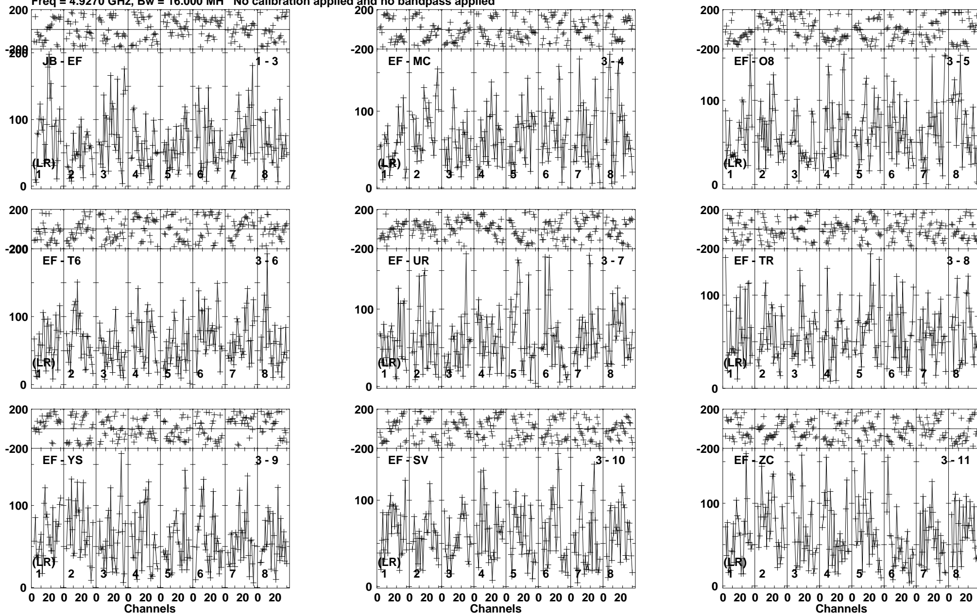
Lower frame: Micro Ampl Jy Top frame: Phas deg Vector average cross-power spectrum Baseline: JB (01) - EF (03) Timerange: 00/02:37:21 to 00/02:41:19
