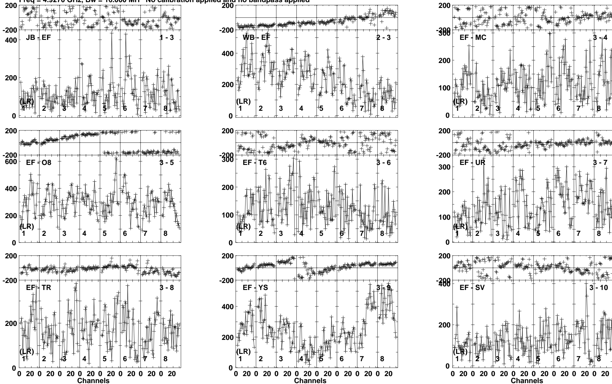
Lower frame: Micro Ampl Jy Top frame: Phas deg Vector averaged cross-power spectrum Baseline: JB (01) - EF (03) Timerange: 00/07:17:21 to 00/07:19:19
