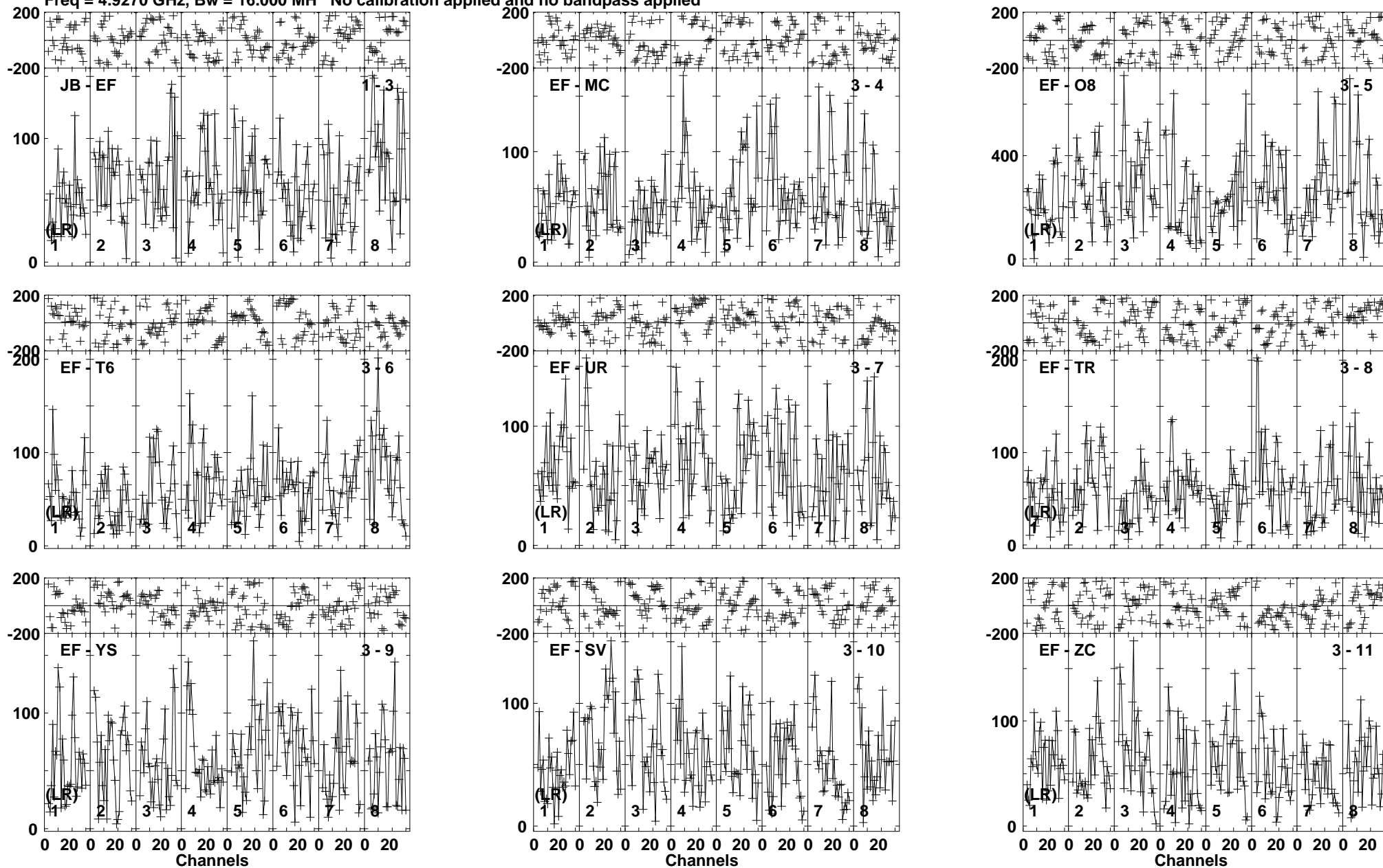
Lower frame: Micro Ampl Jy Top frame: Phas deg Vector averaged cross-power spectrum Baseline: JB (01) - EF (03) Timerange: 00/00:49:21 to 00/00:53:19
