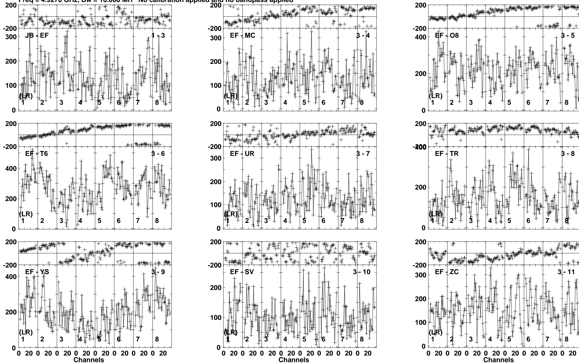
Lower frame: Micro Ampl Jy Top frame: Phas deg Vector averaged cross-power spectrum Baseline: JB (01) - EF (03) Timerange: 00/01:53:21 to 00/01:55:19
