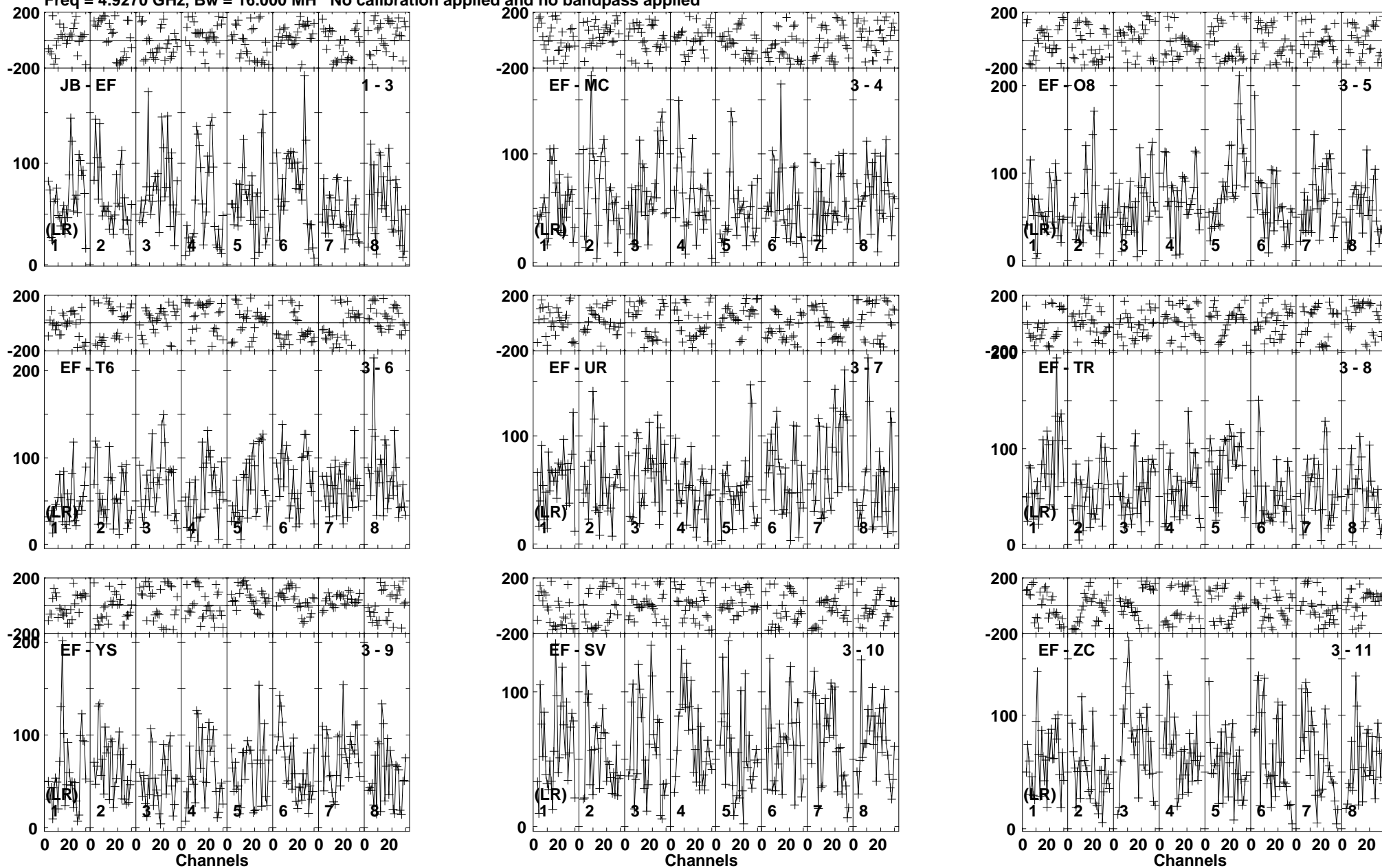
Lower frame: Micro Ampl Jy Top frame: Phas deg Vector averaged cross-power spectrum Baseline: JB (01) - EF (03) Timerange: 00/03:55:23 to 00/03:59:19
