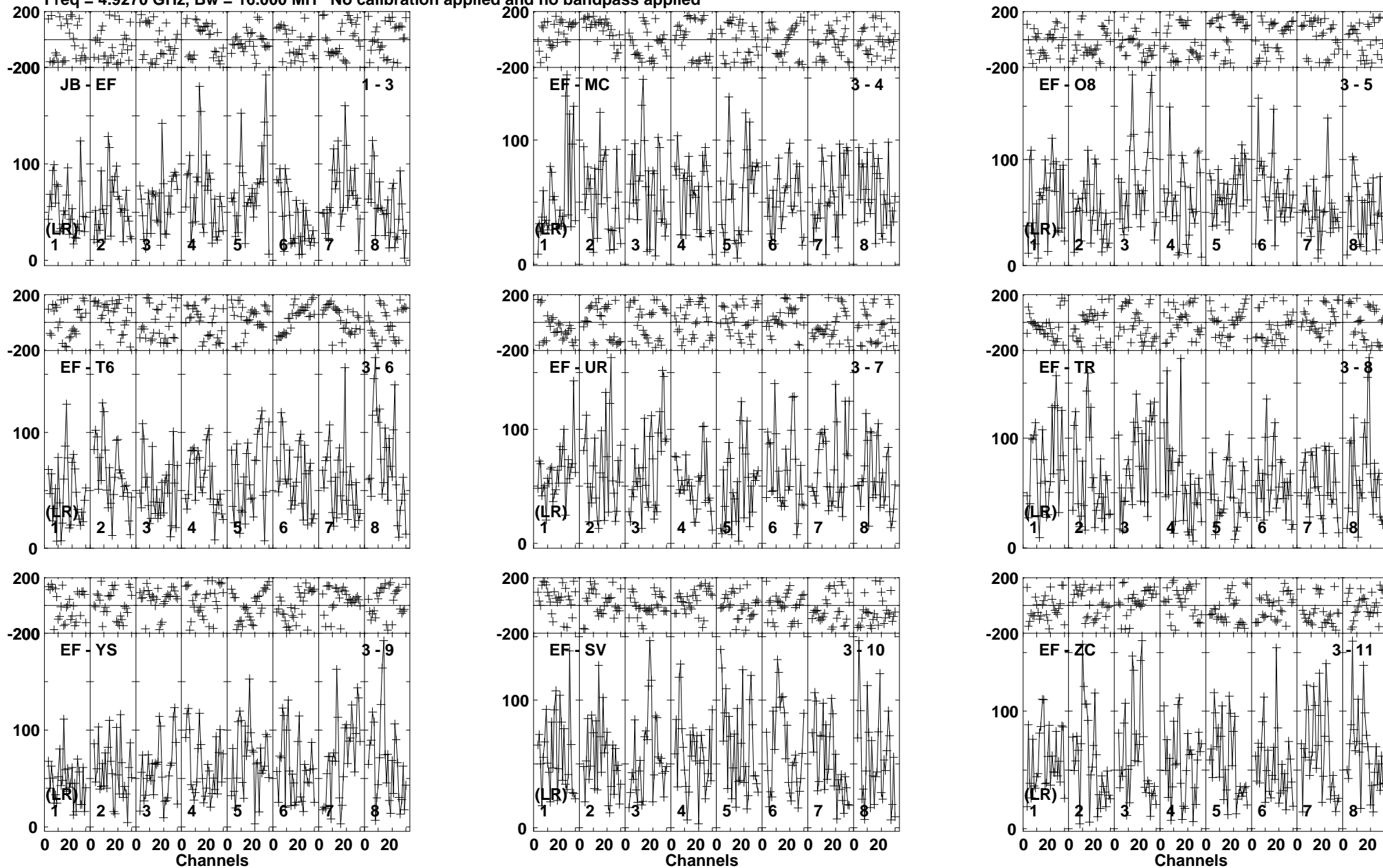
Lower frame: Micro Ampl Jy Top frame: Phas deg Vector averaged cross-power spectrum Baseline: JB (01) - EF (03) Timerange: 00/02:19:23 to 00/02:23:19
