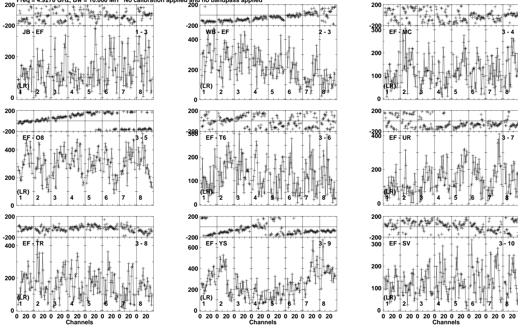
Lower frame: Micro Ampl Jy Top frame: Phas deg Vector averaged cross-power spectrum Baseline: JB (01) - EF (03) Timerange: 00/07:48:01 to 00/07:49:19
