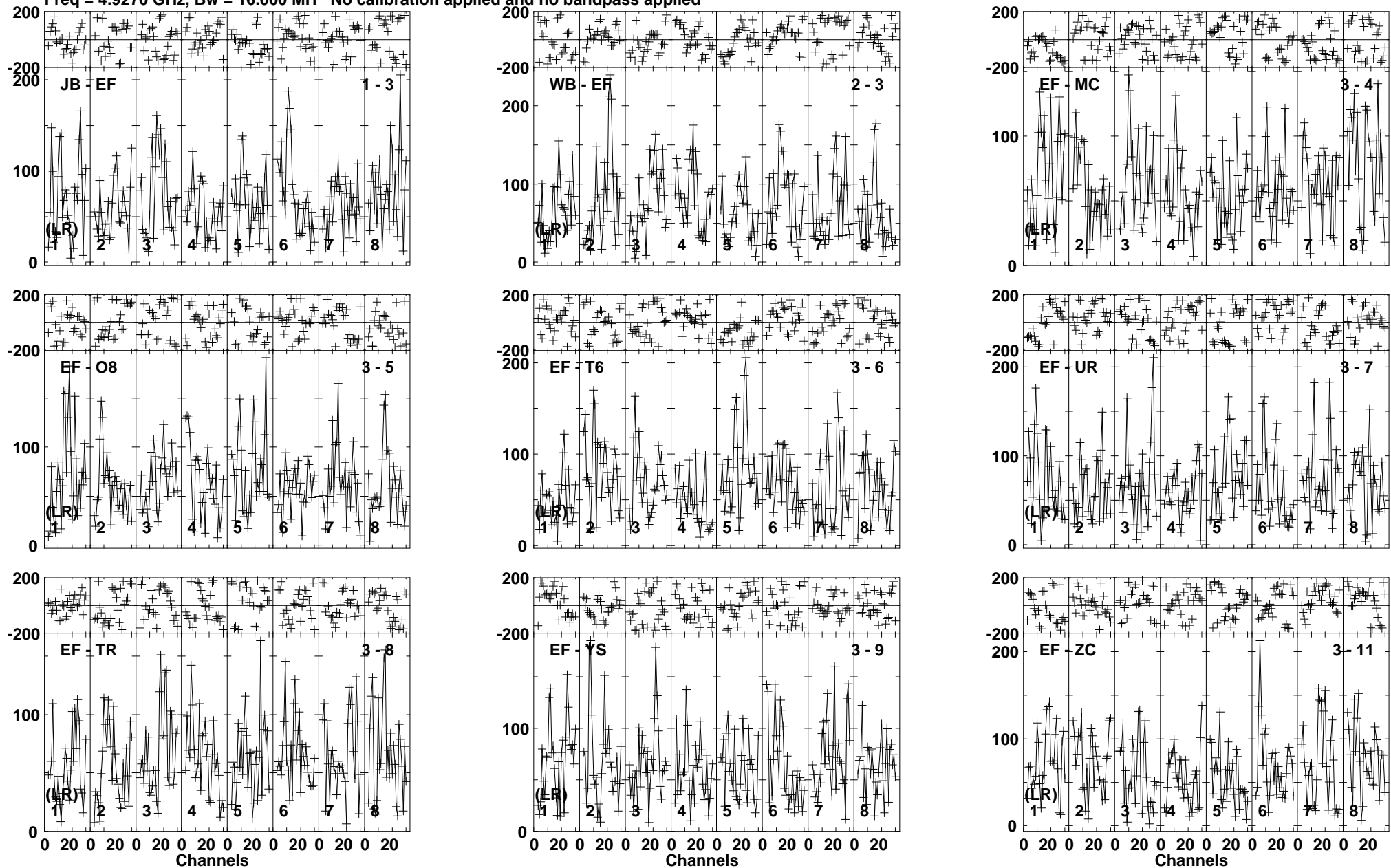
Lower frame: Micro Ampl Jy Top frame: Phas deg Vector averaged cross-power spectrum Baseline: JB (01) - EF (03) Timerange: 00/09:13:21 to 00/09:17:19
