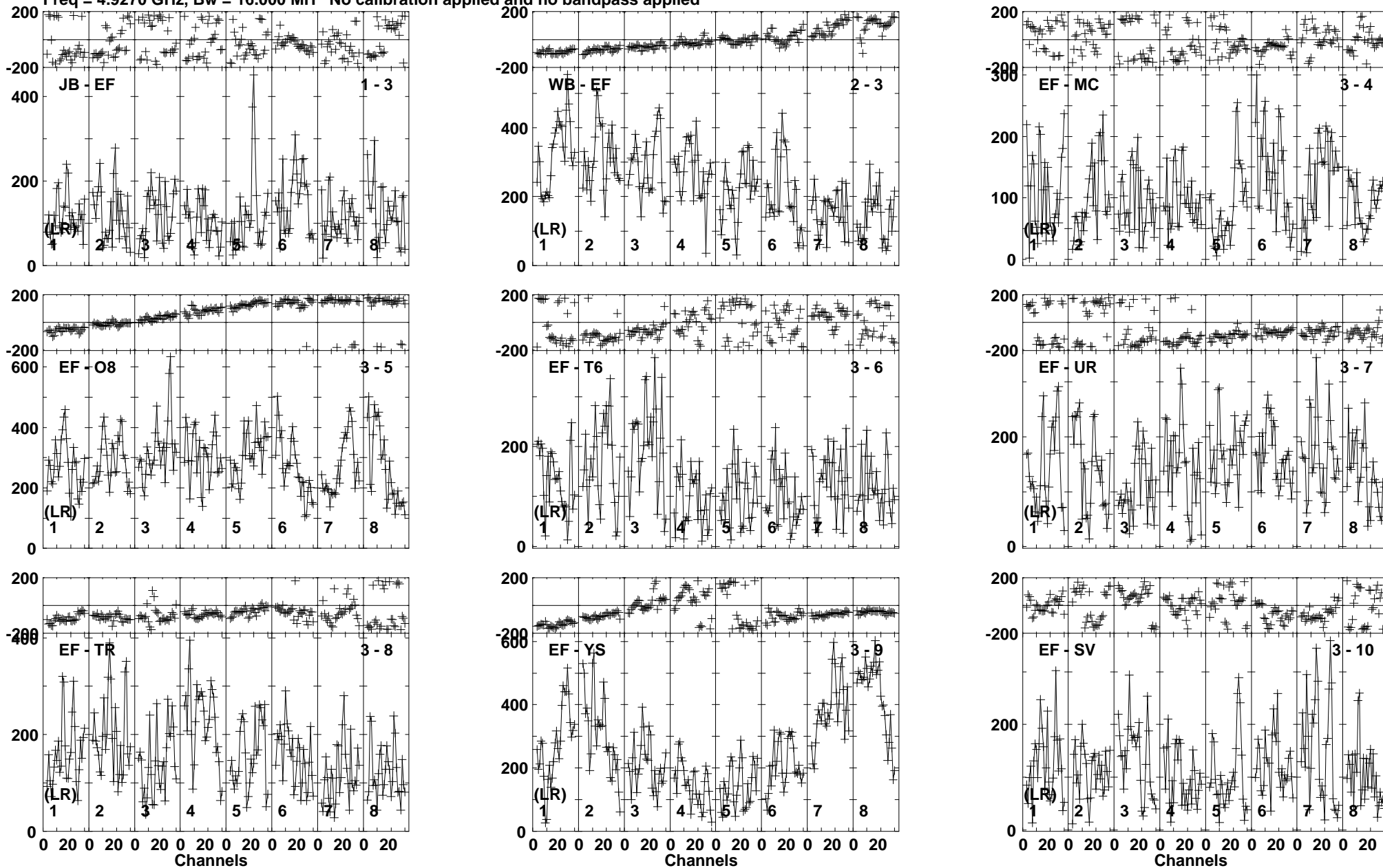
Lower frame: Micro Ampl Jy Top frame: Phas deg Vector averaged cross-power spectrum Baseline: JB (01) - EF (03) Timerange: 00/07:36:01 to 00/07:37:19
