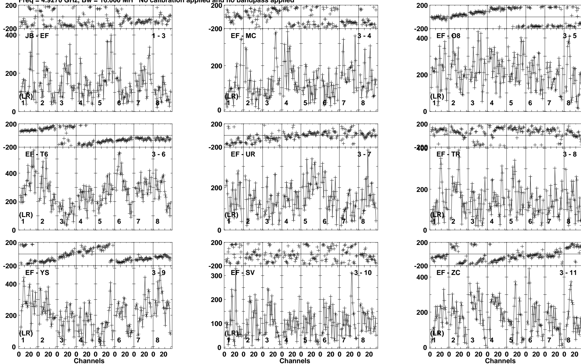
Lower frame: Micro Ampl Jy Top frame: Phas deg Vector averaged cross-power spectrum Baseline: JB (01) - EF (03) Timerange: 00/01:48:01 to 00/01:49:19
