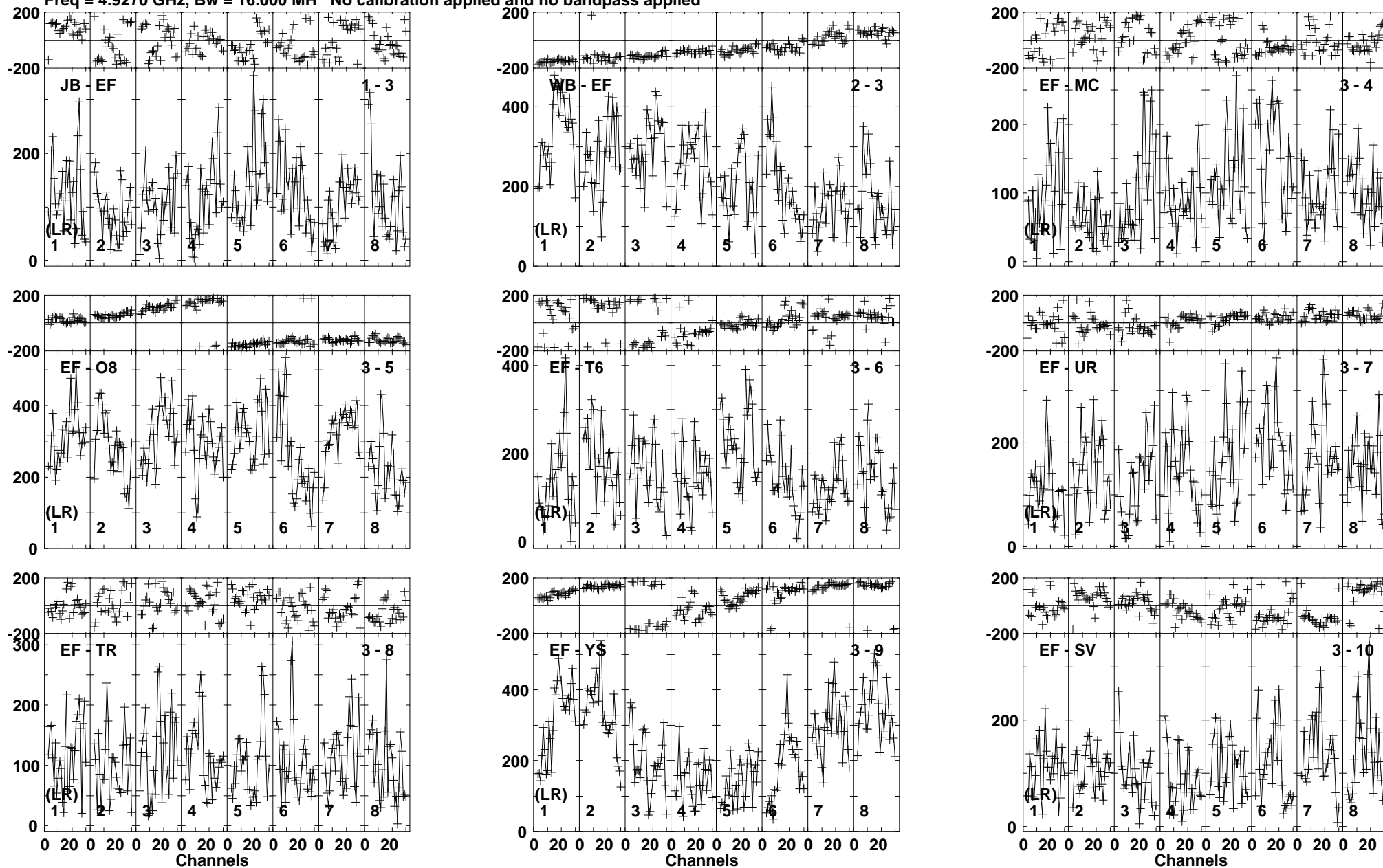
Lower frame: Micro Ampl Jy Top frame: Phas deg Vector averaged cross-power spectrum Baseline: JB (01) - EF (03) Timerange: 00/06:53:21 to 00/06:55:19
