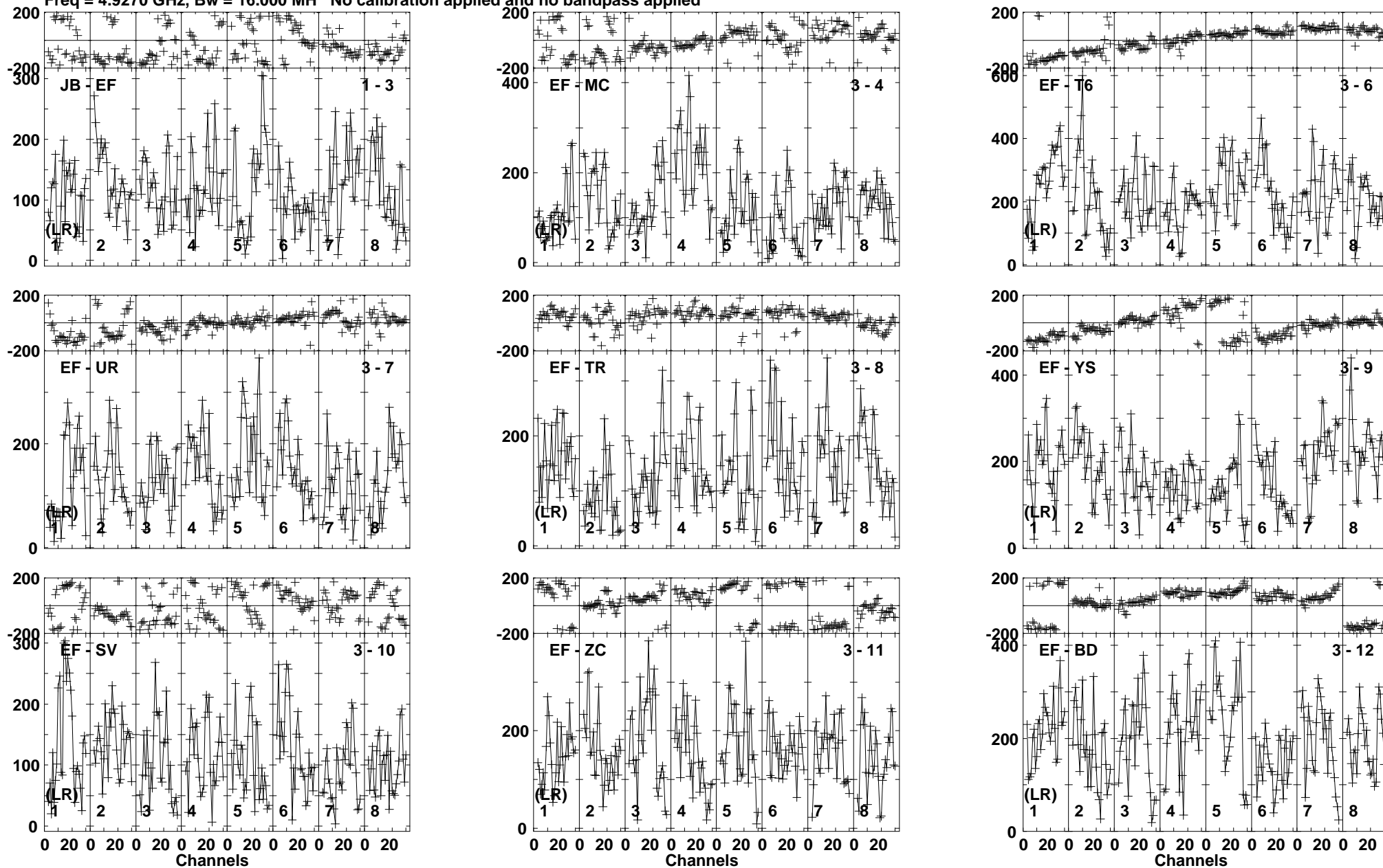
Lower frame: Micro Ampl Jy Top frame: Phas deg Vector averaged cross-power spectrum Baseline: JB (01) - EF (03) Timerange: 00/01:29:21 to 00/01:31:19
