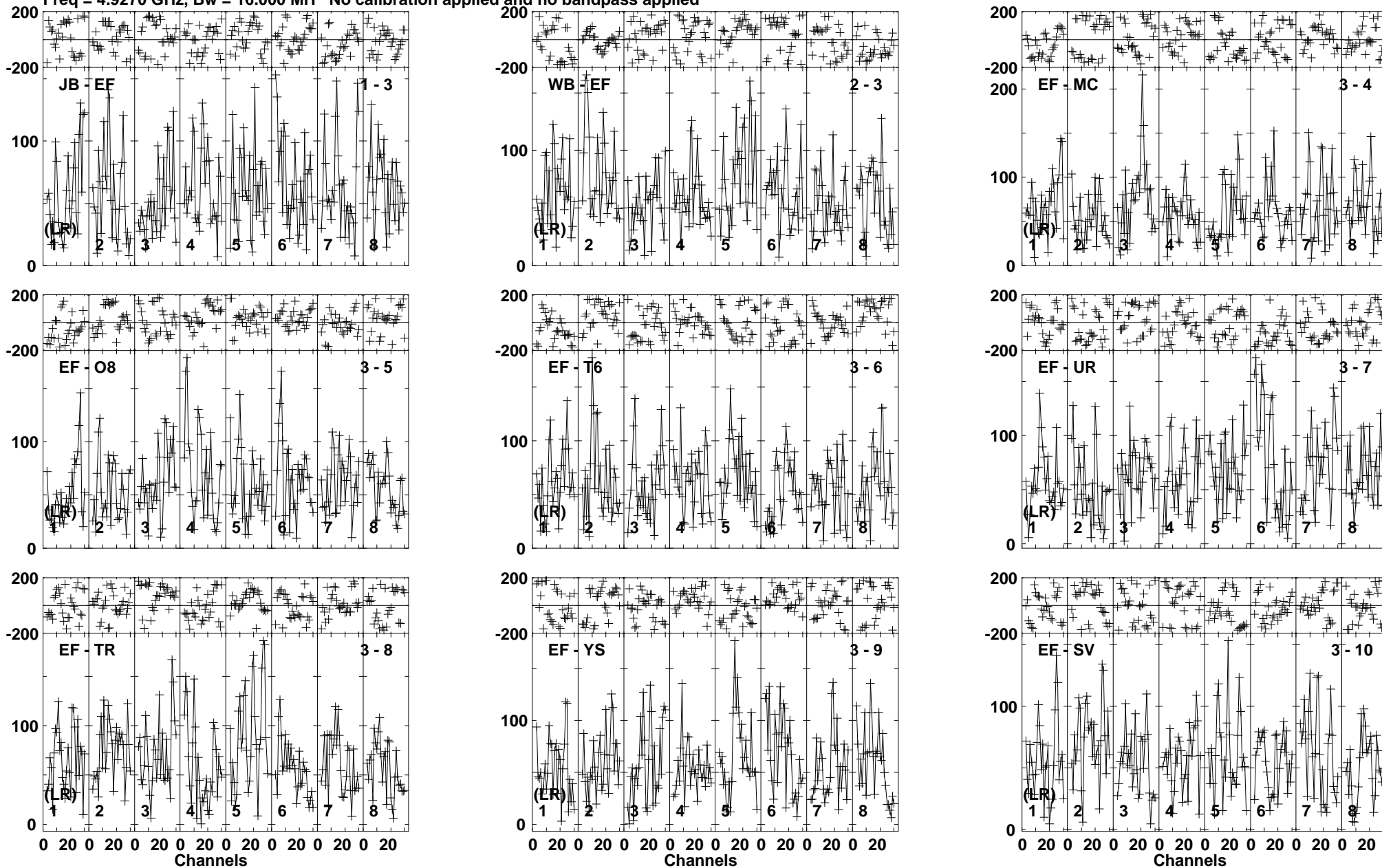
Lower frame: Micro Ampl Jy Top frame: Phas deg Vector averaged cross-power spectrum Baseline: JB (01) - EF (03) Timerange: 00/05:43:23 to 00/05:47:19
