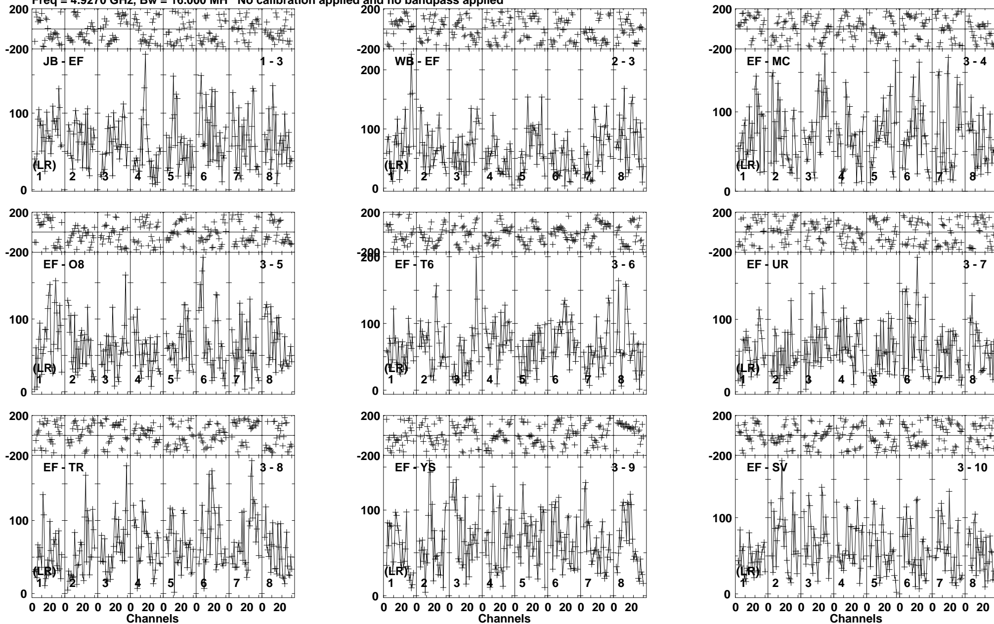
Lower frame: Micro Ampl Jy Top frame: Phas deg Vector averaged cross-power spectrum Baseline: JB (01) - EF (03) Timerange: 00/07:19:23 to 00/07:23:19
