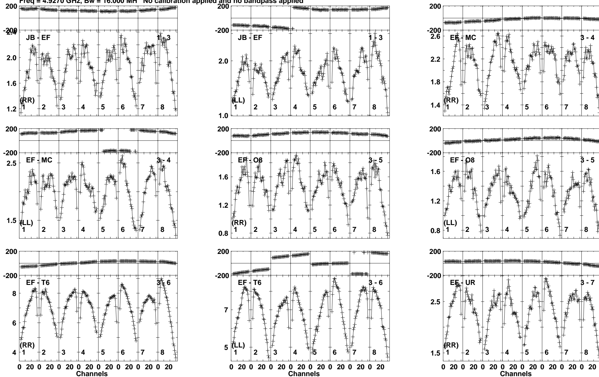
Lower frame: Milli Ampl Jy Top frame: Phas deg Vector averaged cross-power spectrum Baseline: JB (01) - EF (03) Timerange: 00/03:00:01 to 00/03:01:19
