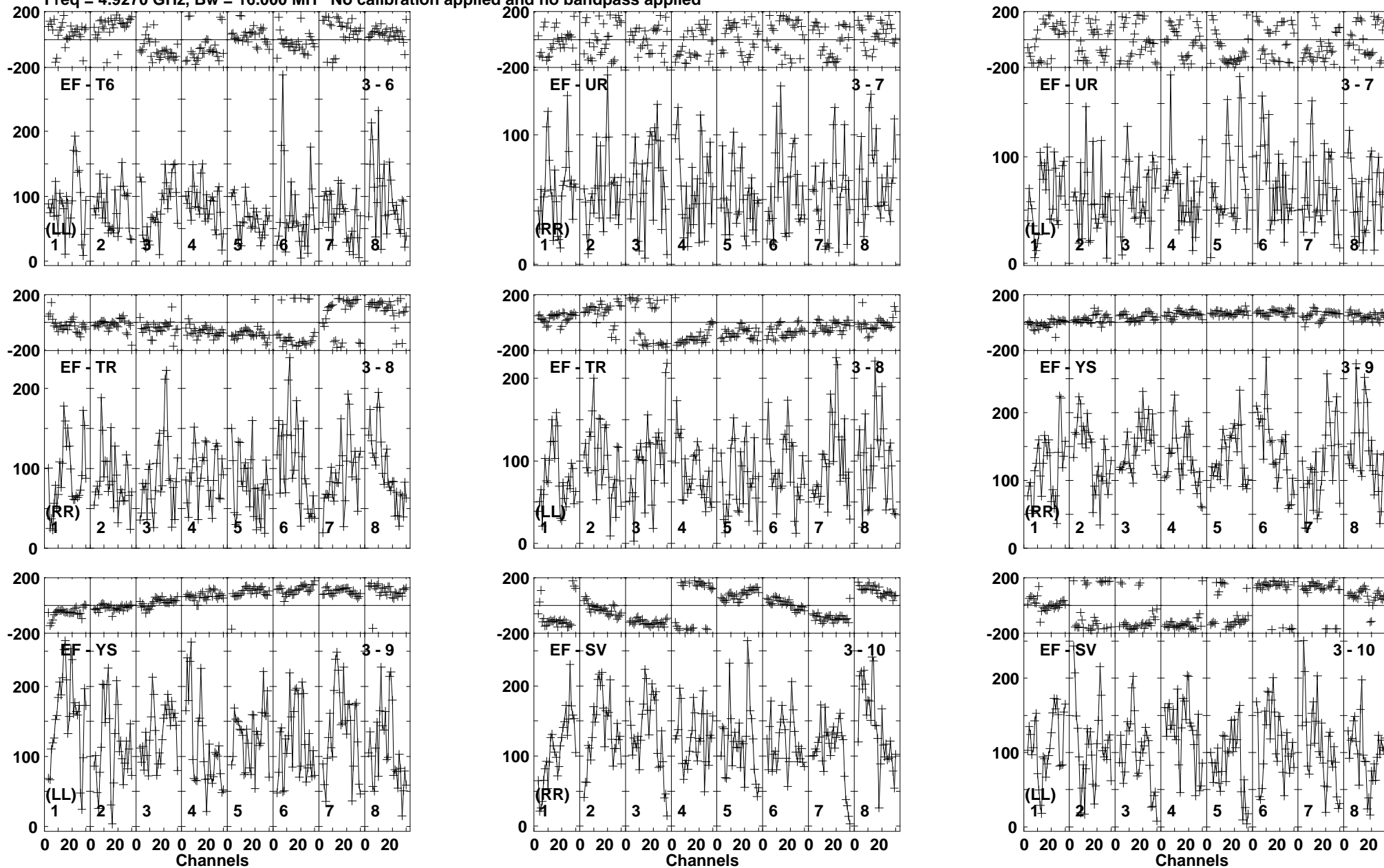
Lower frame: Micro Ampl Jy Top frame: Phas deg Vector averaged cross-power spectrum Baseline: EF (03) - T6 (06) Timerange: 00:06:49:21 to 00:06:53:19
