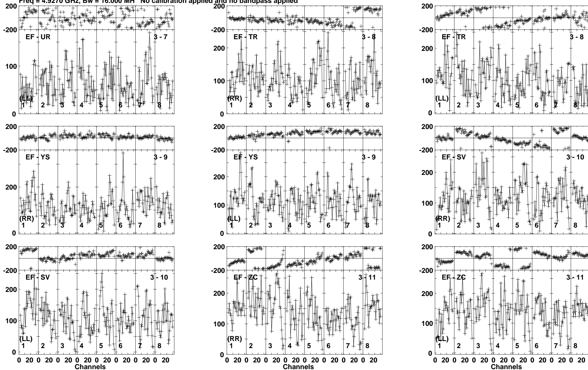
Lower frame: Micro Ampl Jy Top frame: Phas deg Vector averaged cross-power spectrum Baseline: EF (03) - UR (07) Timerange: 00/03:01:21 to 00/03:05:19
