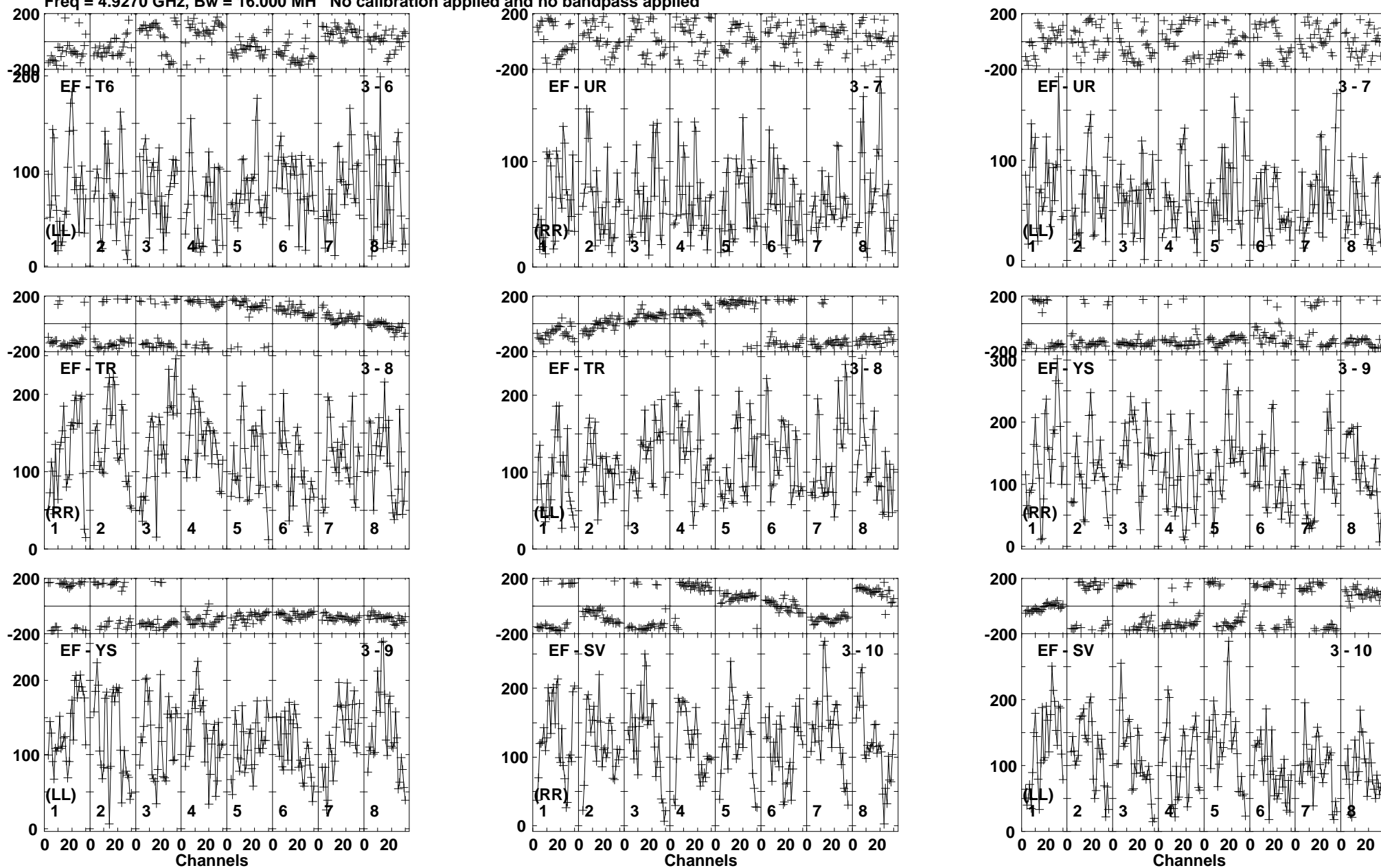
Lower frame: Micro Ampl Jy Top frame: Phas deg Vector averaged cross-power spectrum Baseline: EF (03) - T6 (06) Timerange: 00/05:49:21 to 00/05:53:19
