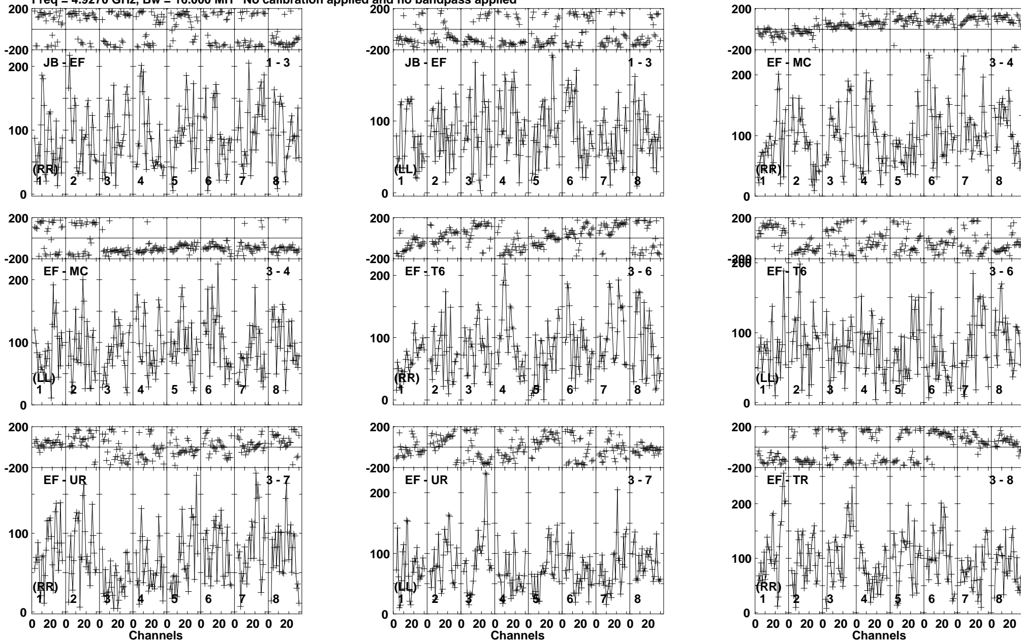
Lower frame: Micro Ampl Jy Top frame: Phas deg Vector averaged cross-power spectrum Baseline: JB (01) - EF (03) Timerange: 00/01:31:23 to 00/01:35:19
