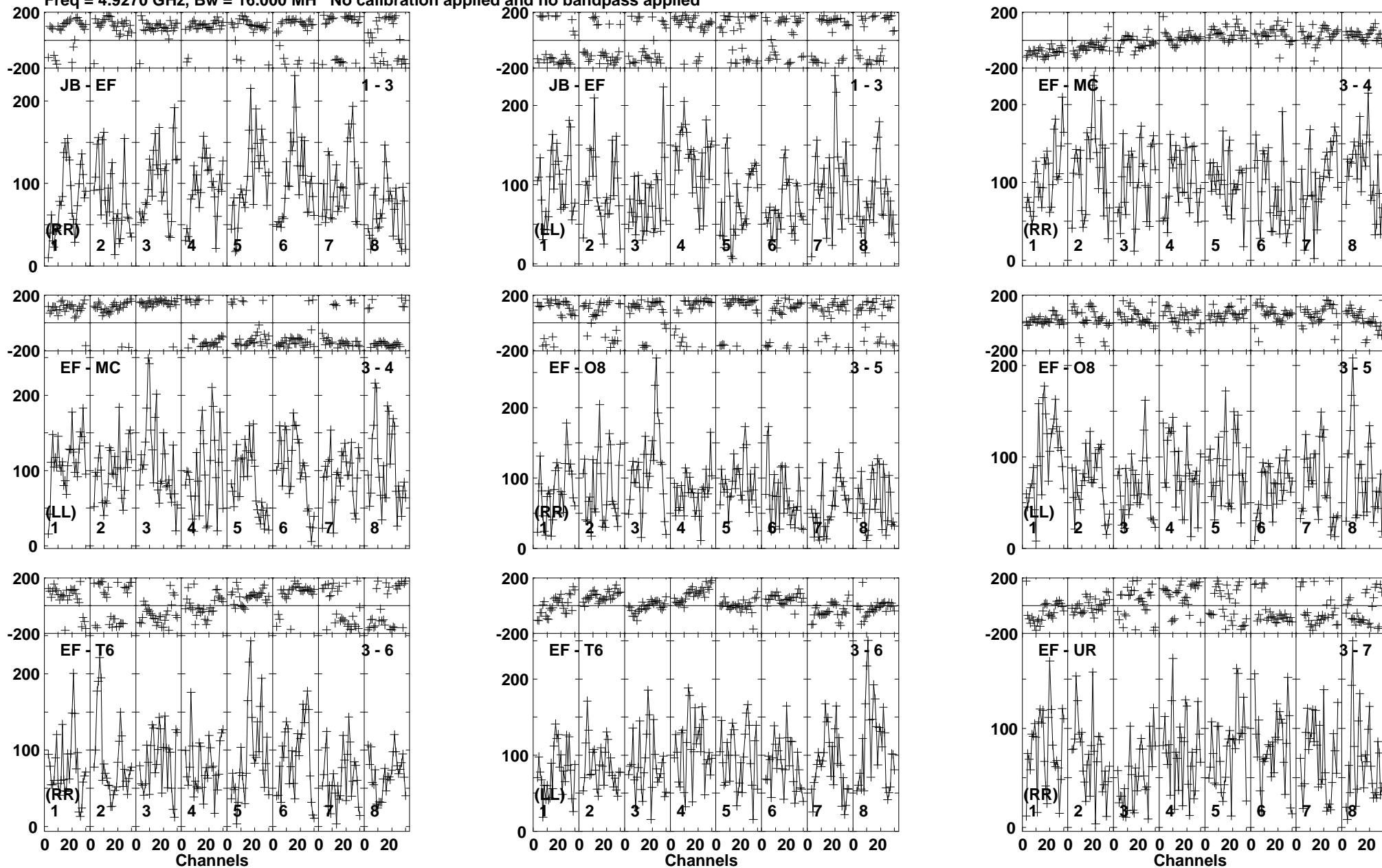
Lower frame: Micro Ampl Jy Top frame: Phas deg Vector averaged cross-power spectrum Baseline: JB (01) - EF (03) Timerange: 00/02:37:21 to 00/02:41:19
