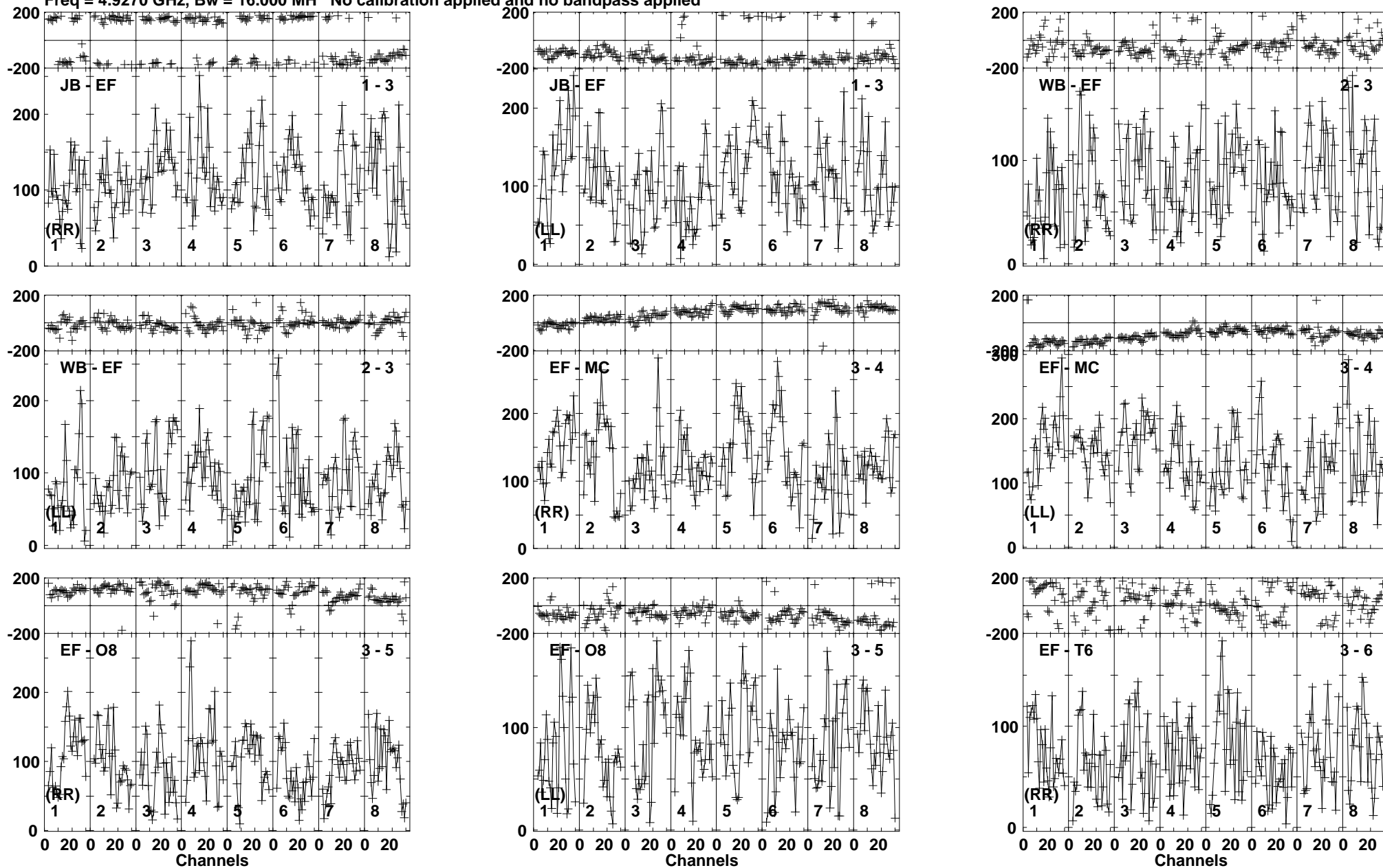
Lower frame: Micro Ampl Jy Top frame: Phas deg Vector averaged cross-power spectrum Baseline: JB (01) - EF (03) Timerange: 00/07:43:21 to 00/07:47:19
