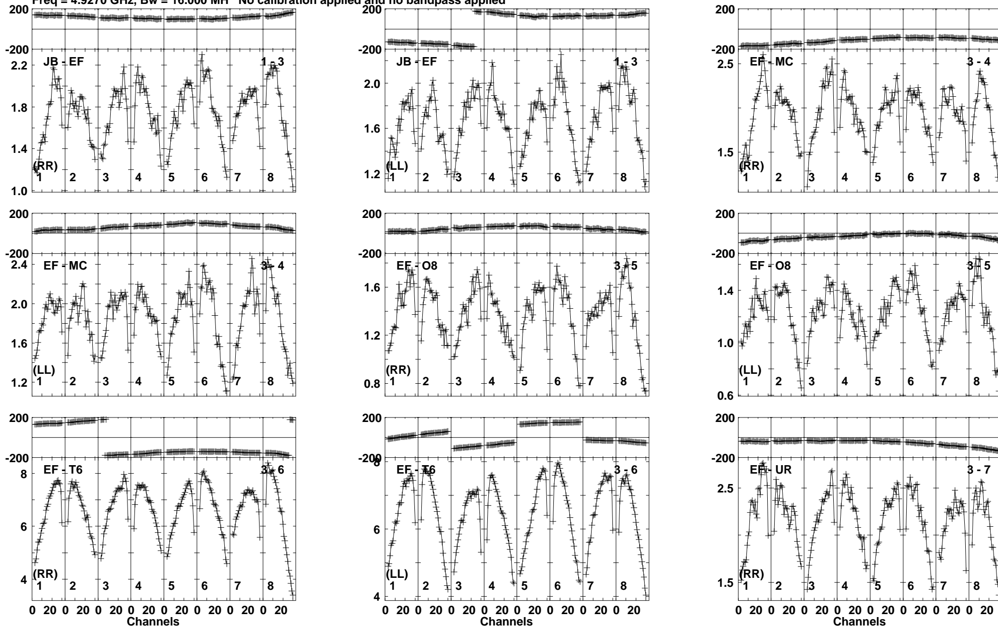
Lower frame: Milli Ampl Jy Top frame: Phas deg Vector averaged cross-power spectrum Baseline: JB (01) - EF (03) Timerange: 00/02:12:01 to 00/02:13:19
