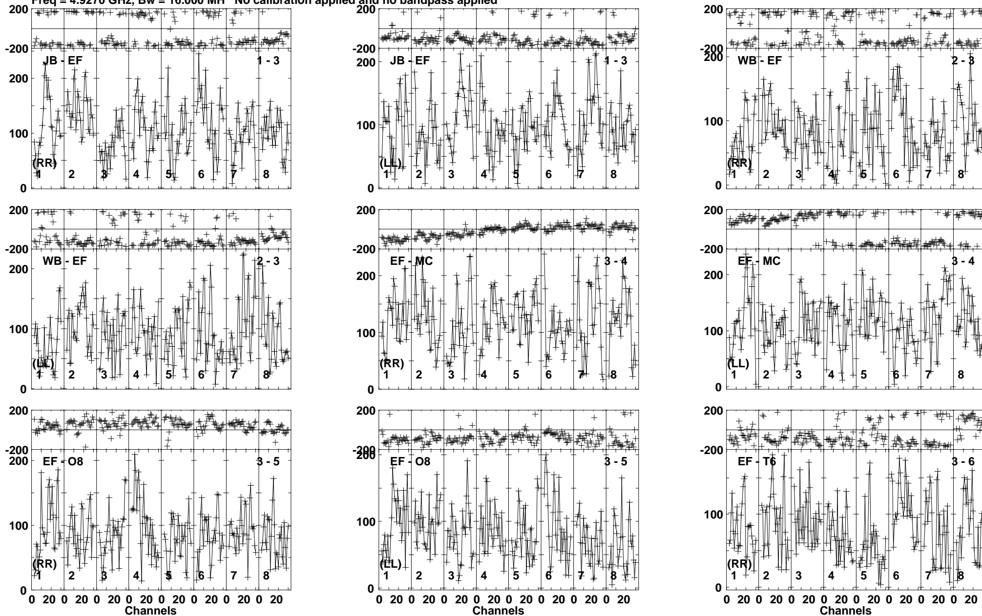
Lower frame: Micro Ampl Jy Top frame: Phas deg Vector averaged cross-power spectrum Baseline: JB (01) - EF (03) Timerange: 00/05:37:21 to 00/05:41:19
