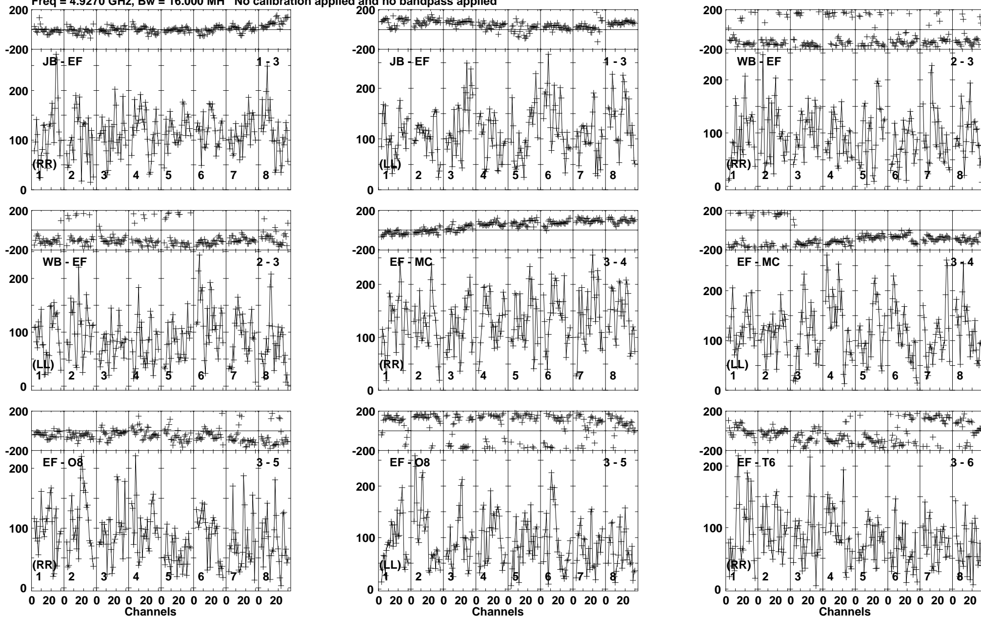
Lower frame: Micro Ampl Jy Top frame: Phas deg Vector averaged cross-power spectrum Baseline: JB (01) - EF (03) Timerange: 00/06:37:21 to 00/06:41:19
