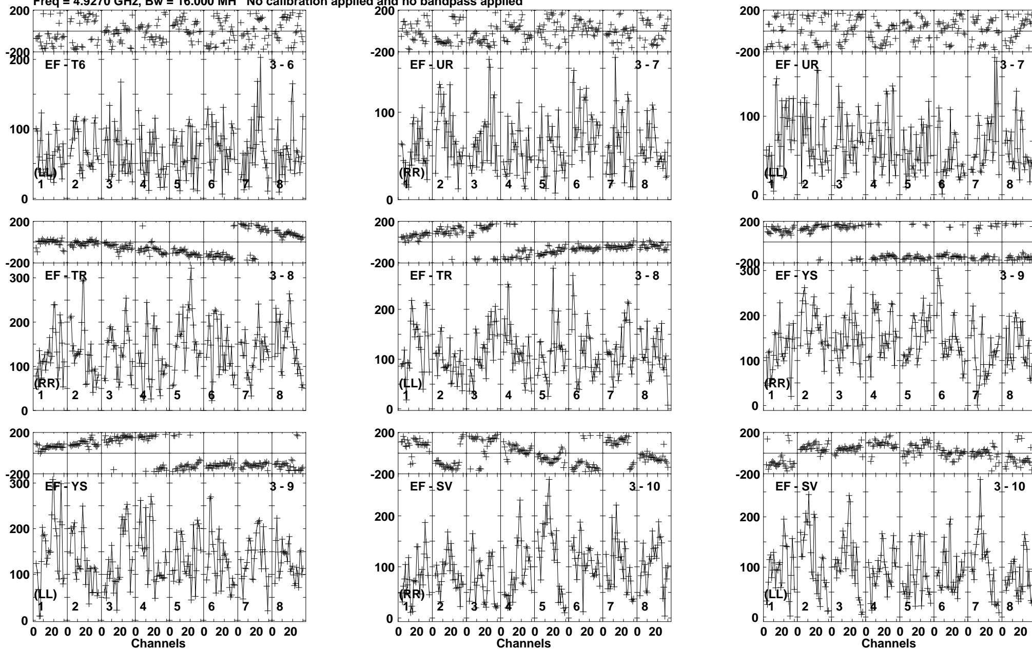
Lower frame: Micro Ampl Jy Top frame: Phas deg Vector averaged cross-power spectrum Baseline: EF (03) - T6 (06) Timerange: 00/07:55:23 to 00/07:59:19
