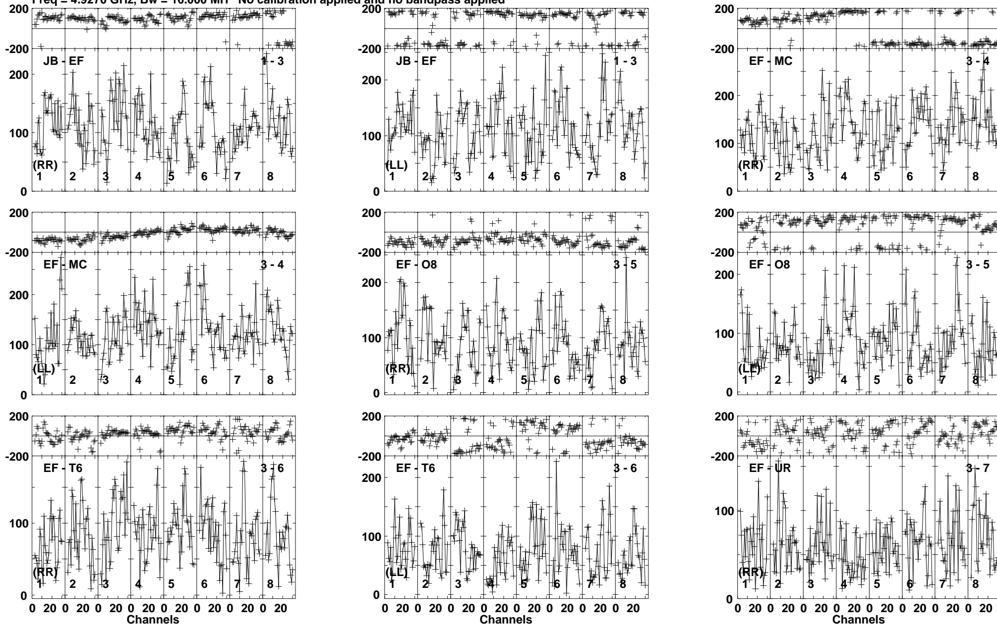
Lower frame: Micro Ampl Jy Top frame: Phas deg Vector averaged cross-power spectrum Baseline: JB (01) - EF (03) Timerange: 00/04:49:21 to 00/04:53:19
