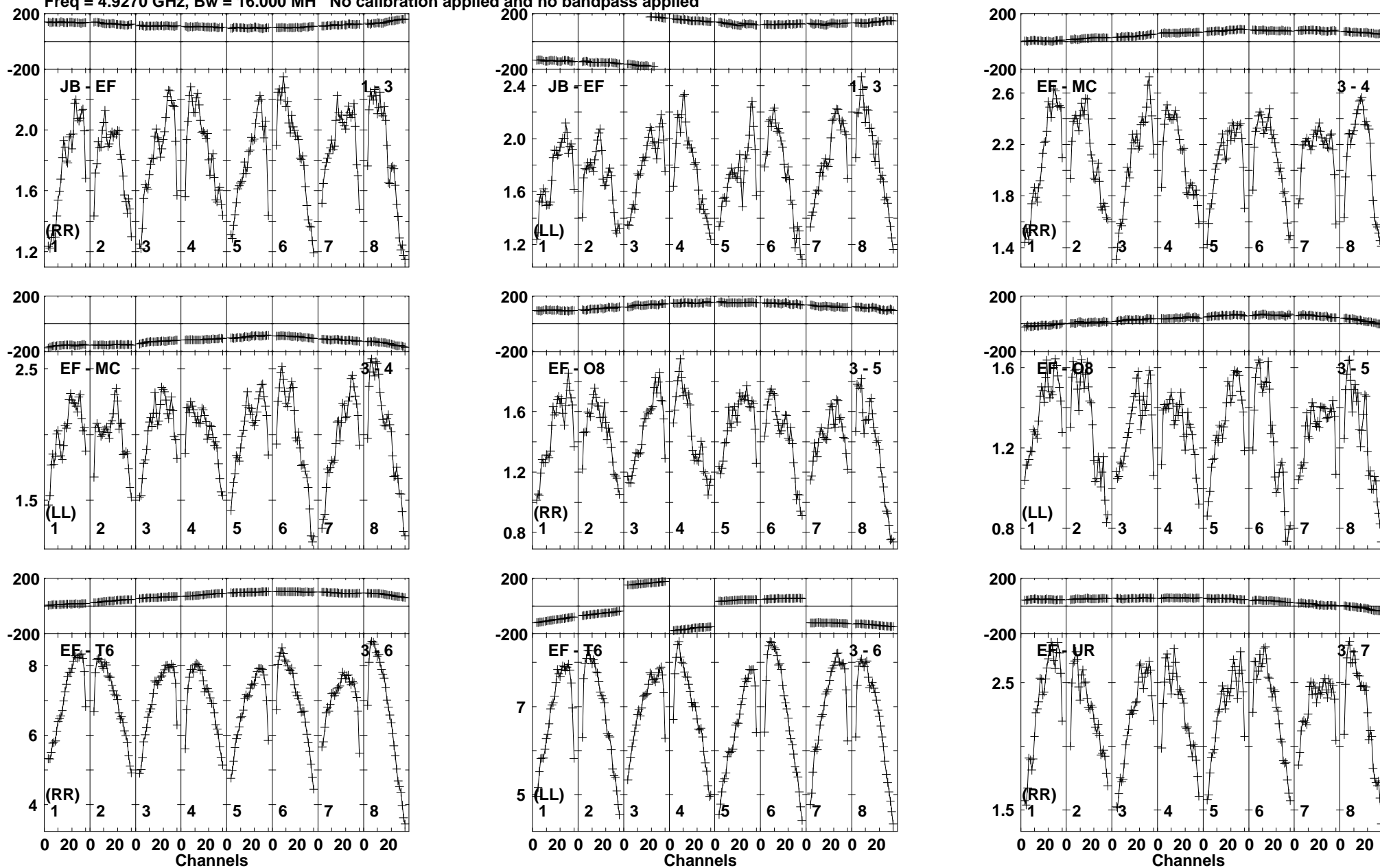
Lower frame: Milli Ampl Jy Top frame: Phas deg Vector averaged cross-power spectrum Baseline: JB (01) - EF (03) Timerange: 00/02:48:01 to 00/02:49:19
