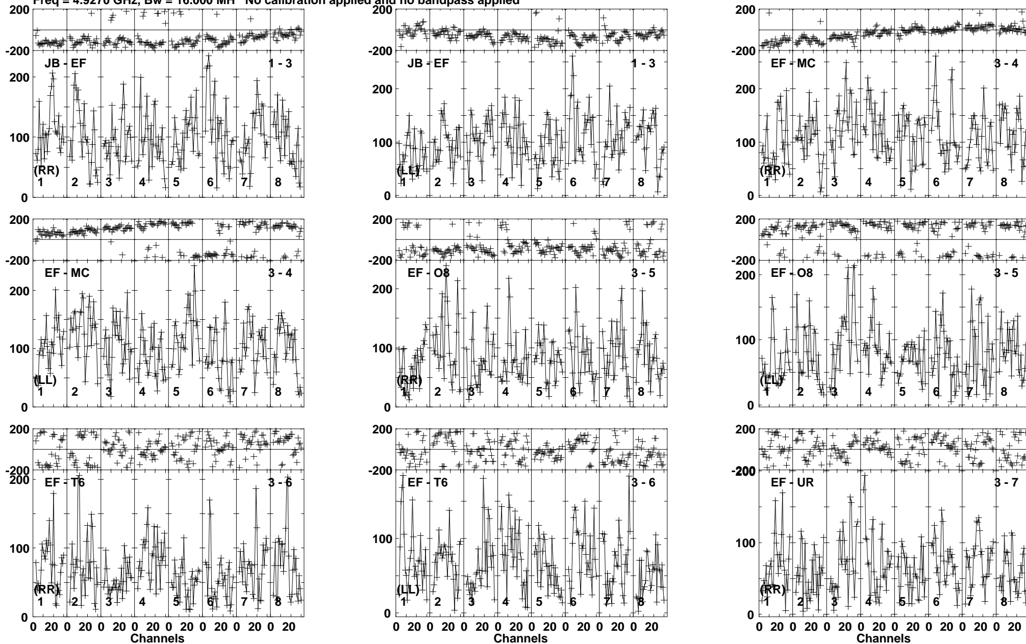
Lower frame: Micro Ampl Jy Top frame: Phas deg Vector averaged cross-power spectrum Baseline: JB (01) - EF (03) Timerange: 00/03:25:21 to 00/03:29:19
