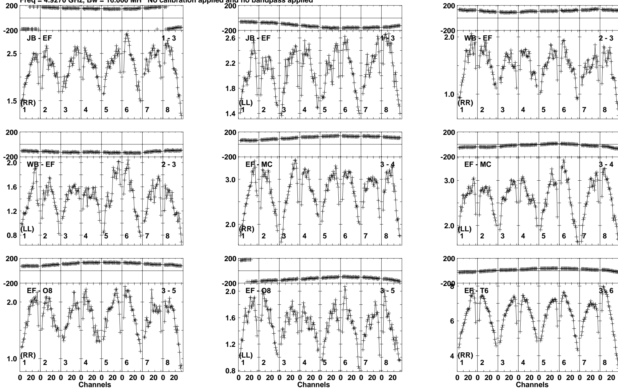
Lower frame: Milli Ampl Jy Top frame: Phas deg Vector averaged cross-power spectrum Baseline: JB (01) - EF (03) Timerange: 00/09:53:21 to 00/09:55:19
