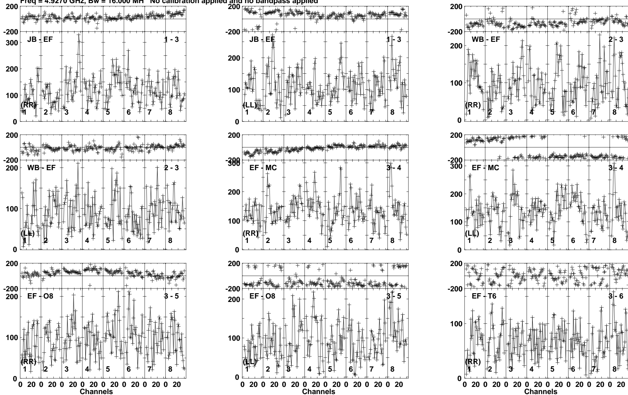
Lower frame: Micro Ampl Jy Top frame: Phas deg Vector averaged cross-power spectrum Baseline: JB (01) - EF (03) Timerange: 00/07:55:23 to 00/07:59:19
