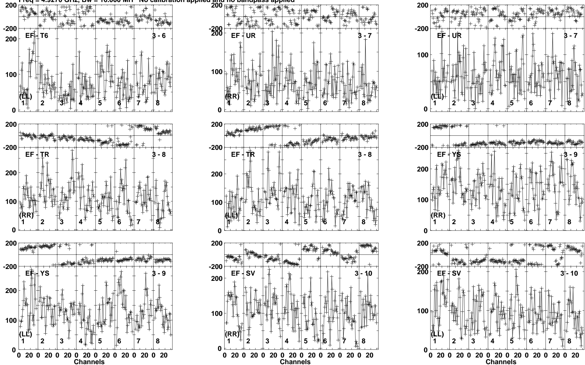
Lower frame: Micro Ampl Jy Top frame: Phas deg Vector averaged cross-power spectrum Baseline: EF (03) - T6 (06) Timerange: 00/07:31:23 to 00/07:35:19
