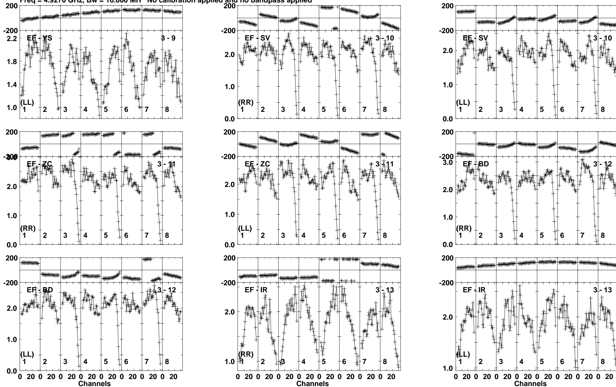
Lower frame: Milli Ampl Jy Top frame: Phas deg Vector averaged cross-power spectrum Baseline: EF (03) - YS (09) Timerange: 00/00:35:41 to 00/00:37:19
