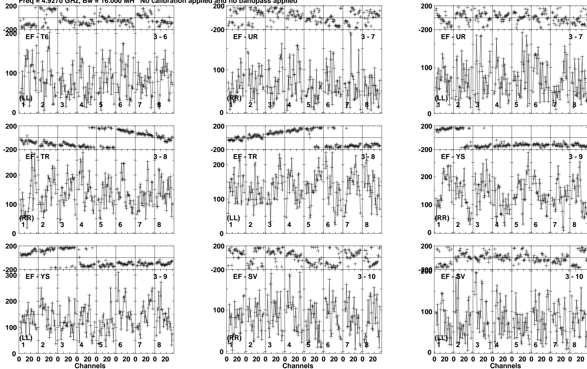
Lower frame: Micro Ampl Jy Top frame: Phas deg Vector averaged cross-power spectrum Baseline: EF (03) - T6 (06) Timerange: 00/08:31:23 to 00/08:35:19
