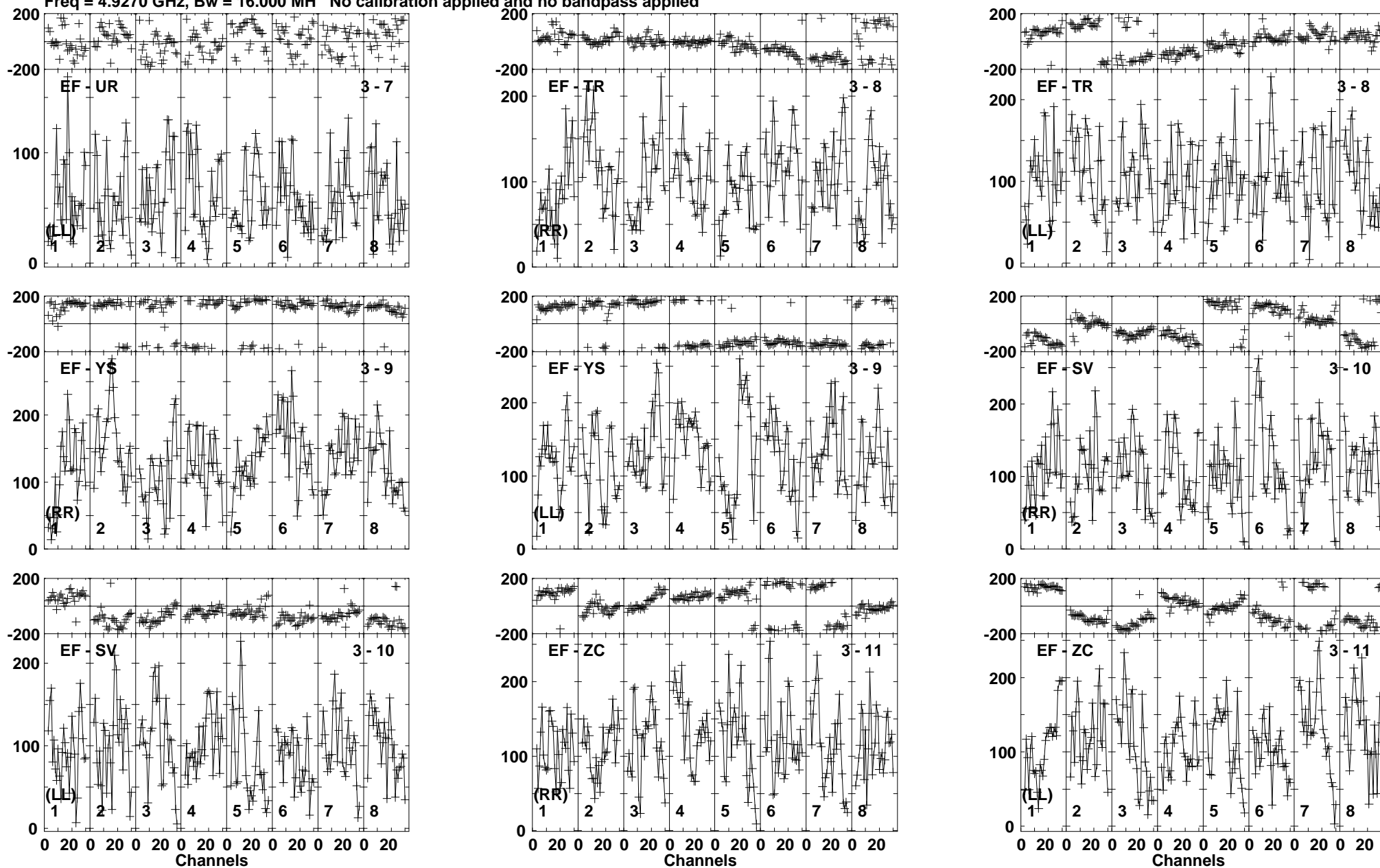
Lower frame: Micro Ampl Jy Top frame: Phas deg Vector averaged cross-power spectrum Baseline: EF (03) - UR (07) Timerange: 00/03:55:23 to 00/03:59:19
