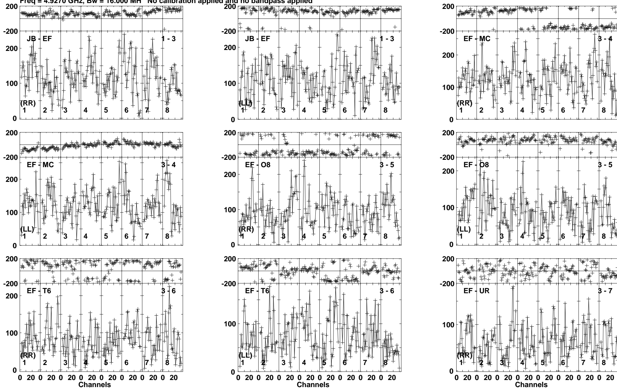
Lower frame: Micro Ampl Jy Top frame: Phas deg Vector averaged cross-power spectrum Baseline: JB (01) - EF (03) Timerange: 00/04:55:23 to 00/04:59:19
