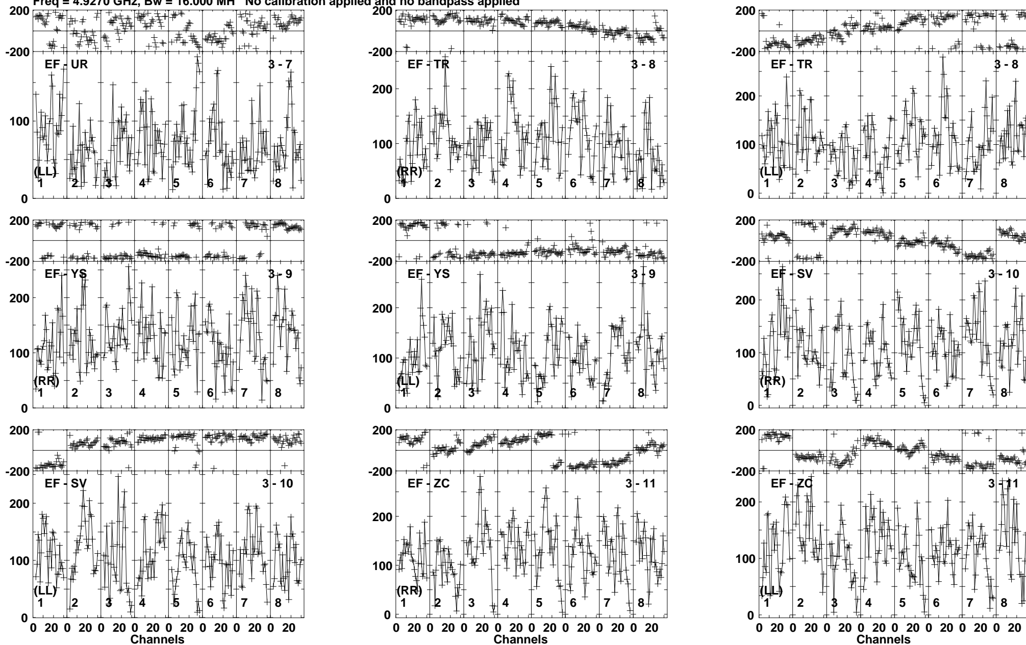
Lower frame: Micro Ampl Jy Top frame: Phas deg Vector averaged cross-power spectrum Baseline: EF (03) - UR (07) Timerange: 00/02:43:23 to 00/02:47:19
