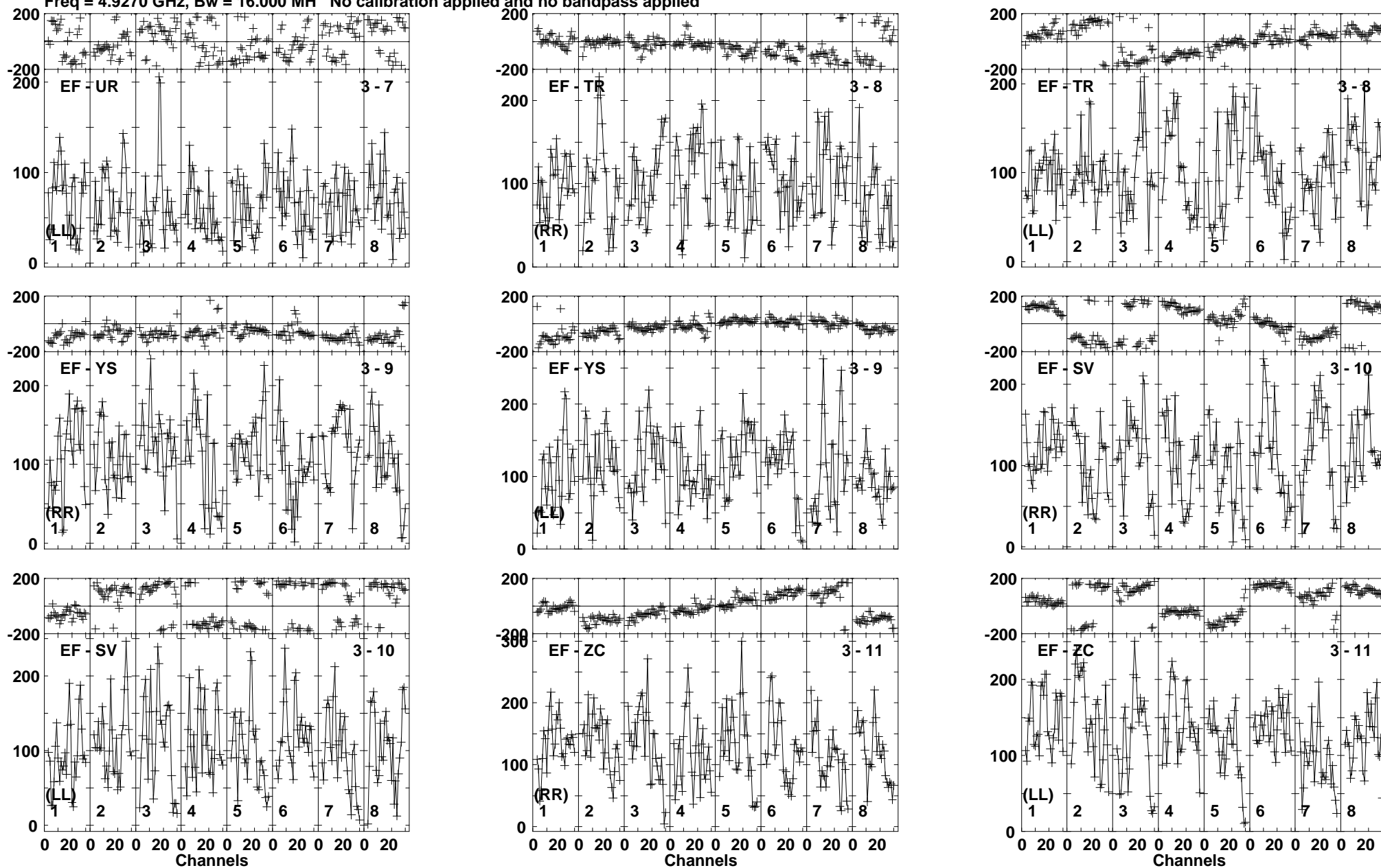
Lower frame: Micro Ampl Jy Top frame: Phas deg Vector averaged cross-power spectrum Baseline: EF (03) - UR (07) Timerange: 00/02:55:23 to 00/02:59:19
