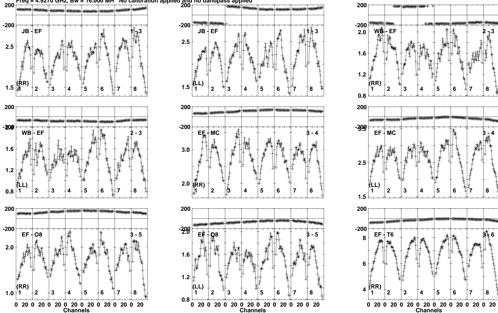
Lower frame: Milli Ampl Jy Top frame: Phas deg Vector averaged cross-power spectrum Baseline: JB (01) - EF (03) Timerange: 00/08:53:21 to 00/08:55:19
