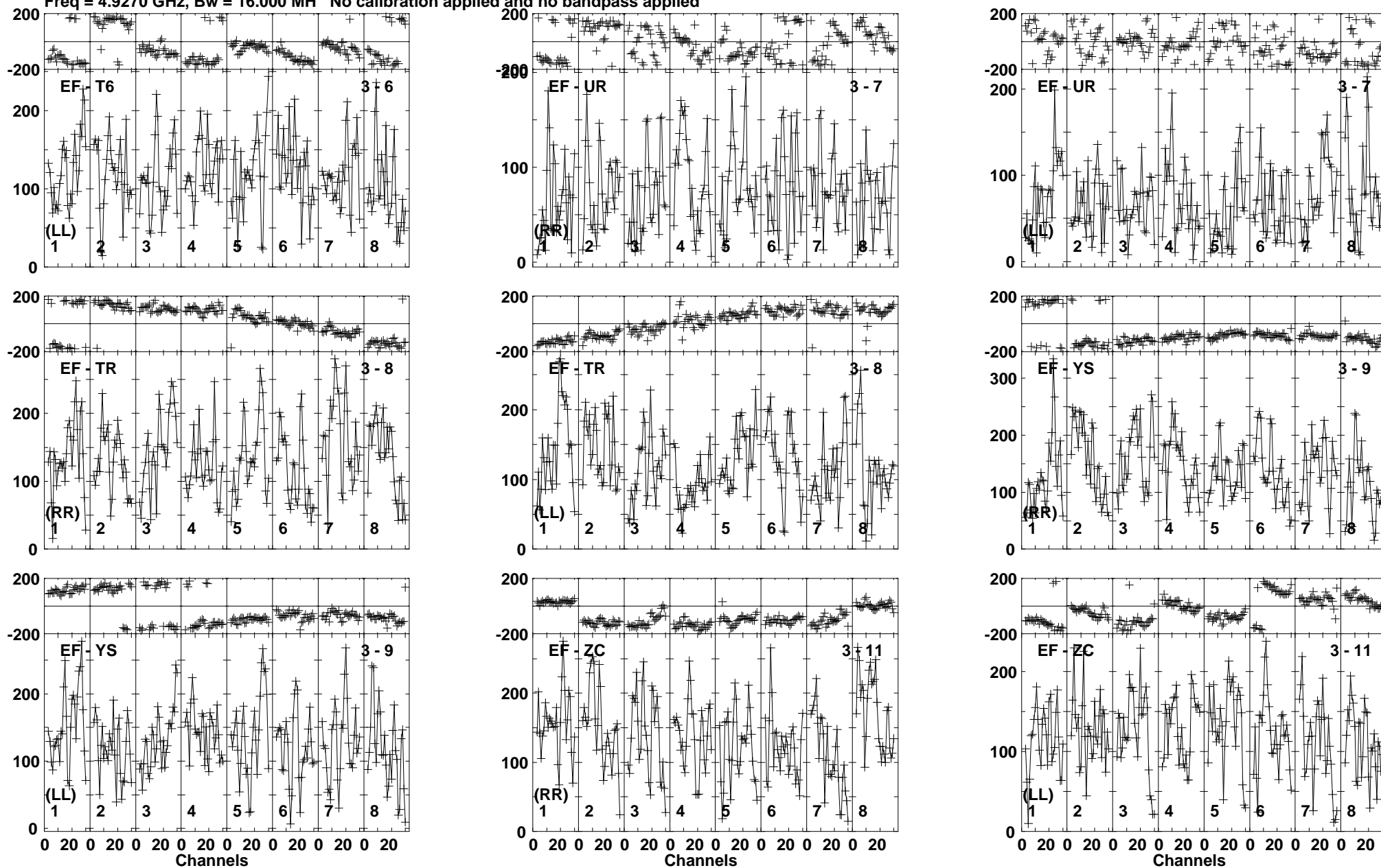
Lower frame: Micro Ampl Jy Top frame: Phas deg Vector averaged cross-power spectrum Baseline: EF (03) - T6 (06) Timerange: 00/09:01:21 to 00/09:05:19
