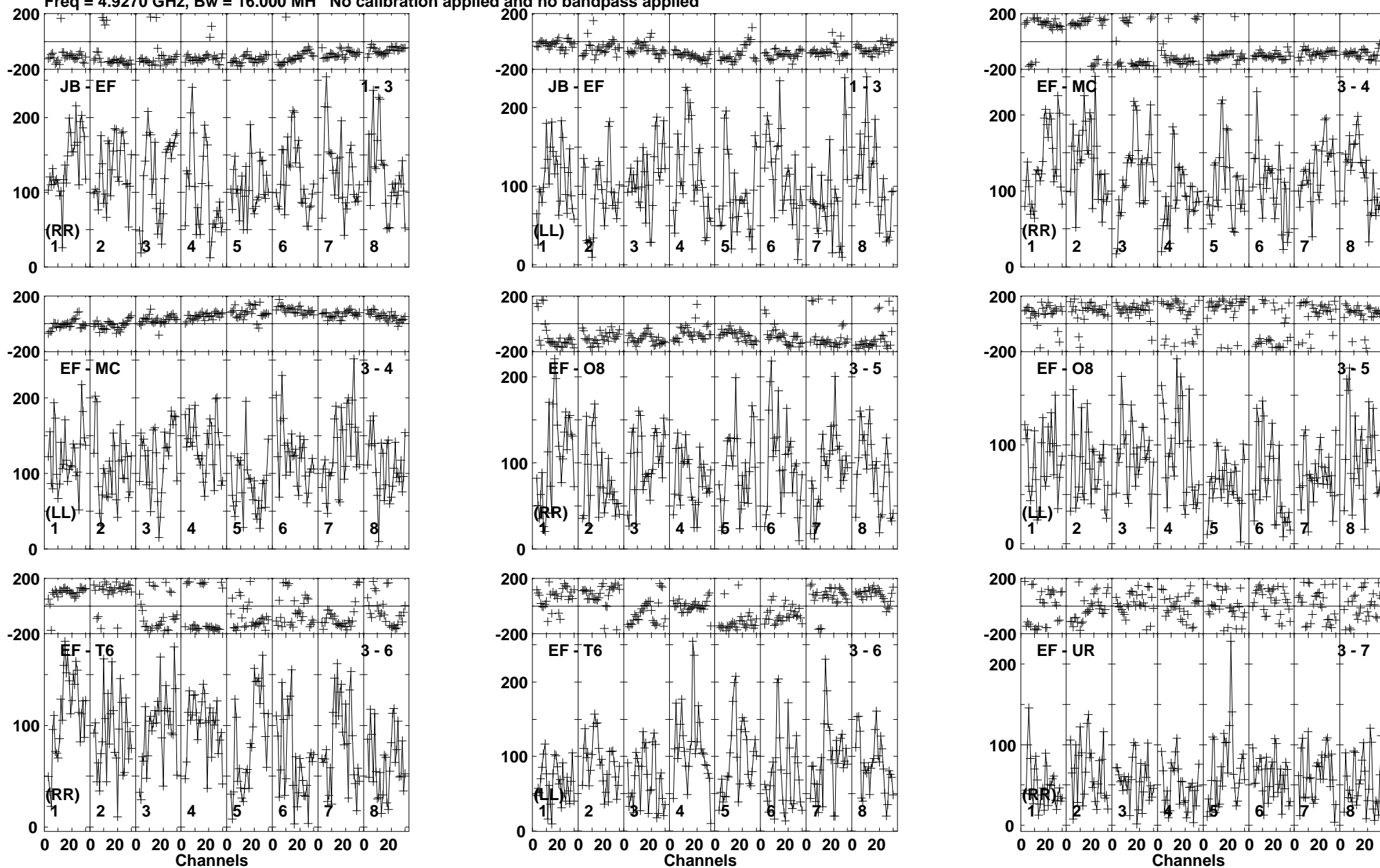
Lower frame: Micro Ampl Jy Top frame: Phas deg Vector averaged cross-power spectrum Baseline: JB (01) - EF (03) Timerange: 00/04:19:23 to 00/04:23:19
