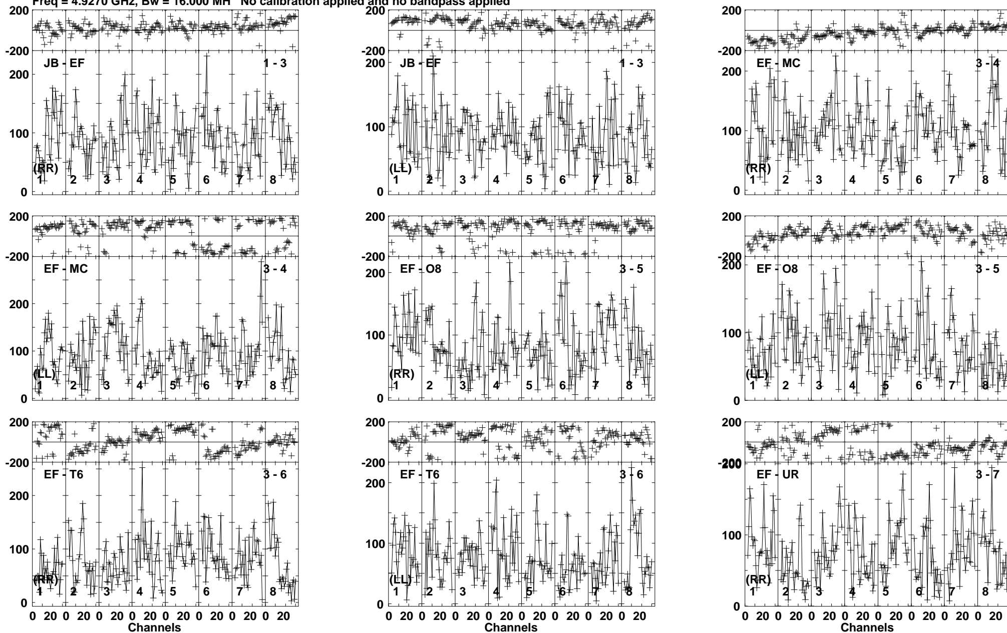
Lower frame: Micro Ampl Jy Top frame: Phas deg Vector averaged cross-power spectrum Baseline: JB (01) - EF (03) Timerange: 00/02:07:23 to 00/02:11:19
