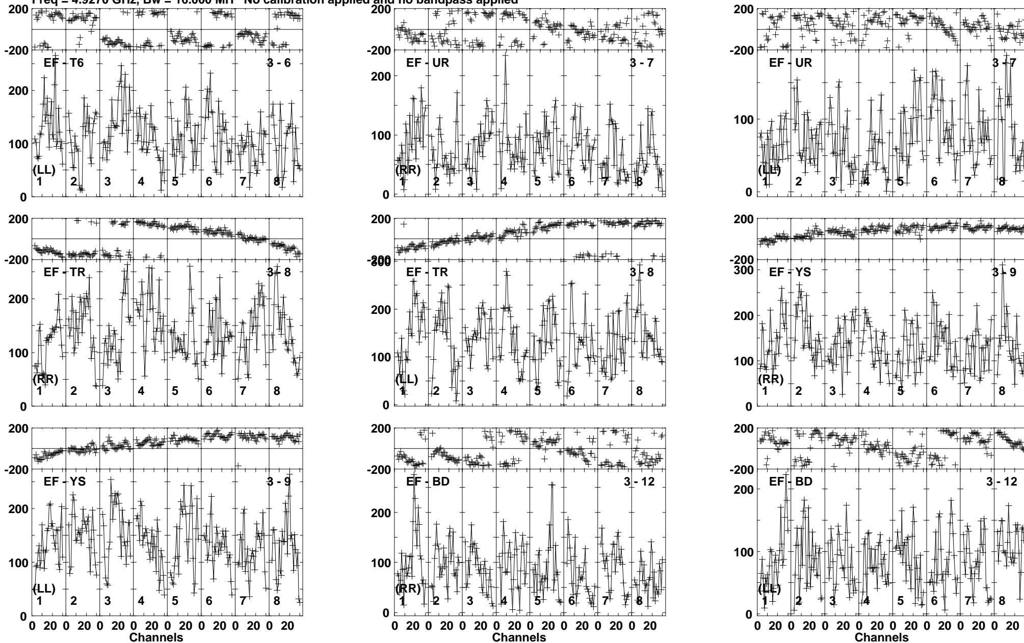
Lower frame: Micro Ampl Jy Top frame: Phas deg Vector averaged cross-power spectrum Baseline: EF (03) - T6 (06) Timerange: 00/08:49:21 to 00/08:53:19
