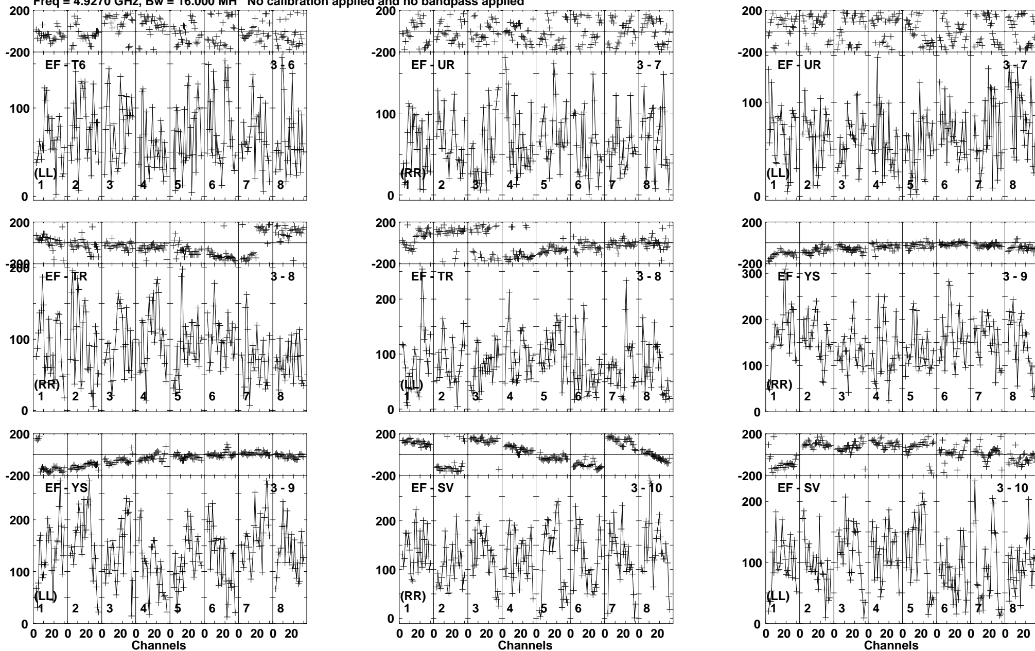
Lower frame: Micro Ampl Jy Top frame: Phas deg Vector averaged cross-power spectrum Baseline: EF (03) - T6 (06) Timerange: 00/07:07:21 to 00/07:11:19
