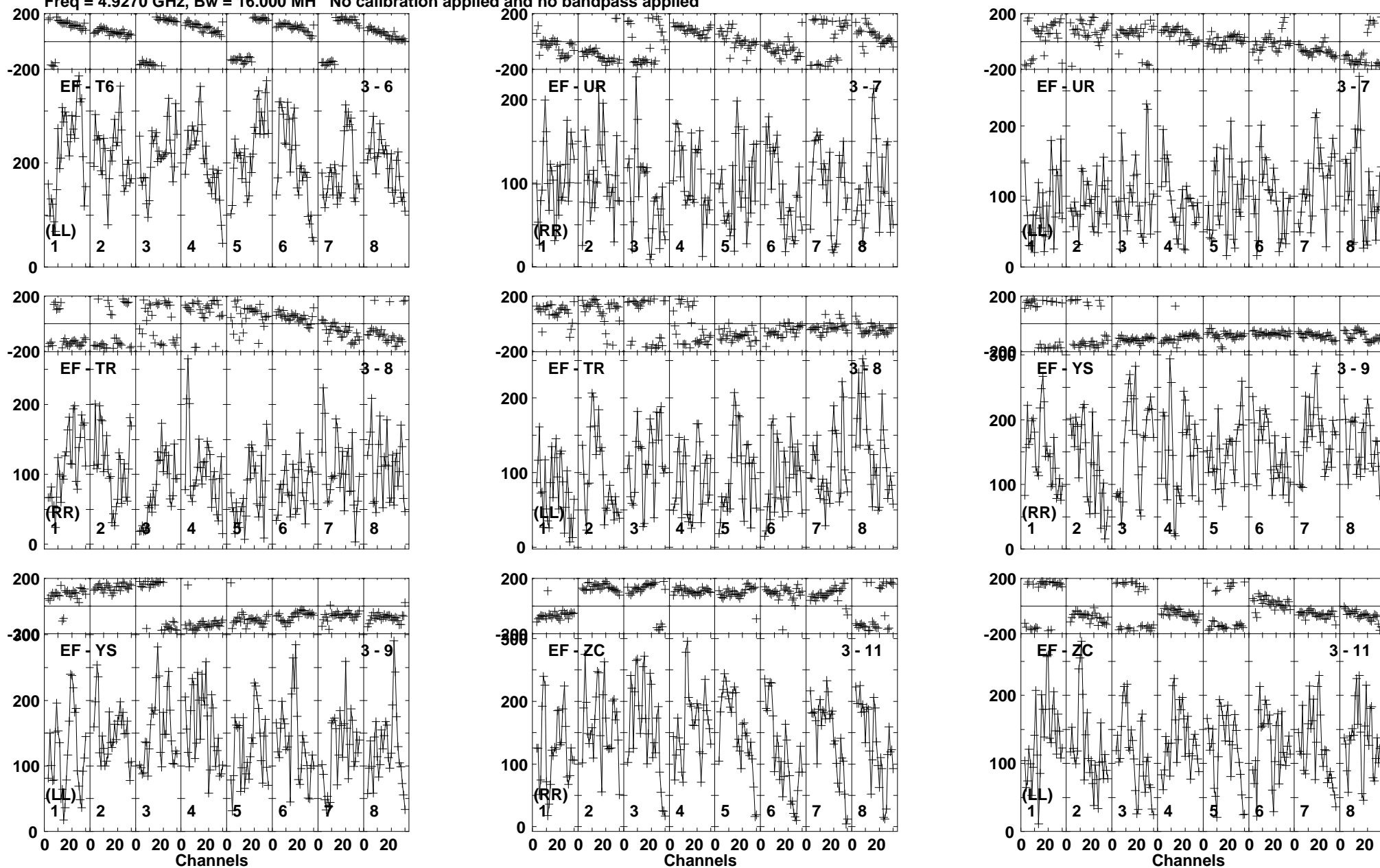
Lower frame: Micro Ampl Jy Top frame: Phas deg Vector averaged cross-power spectrum Baseline: EF (03) - T6 (06) Timerange: 00/10:19:21 to 00/10:23:19
