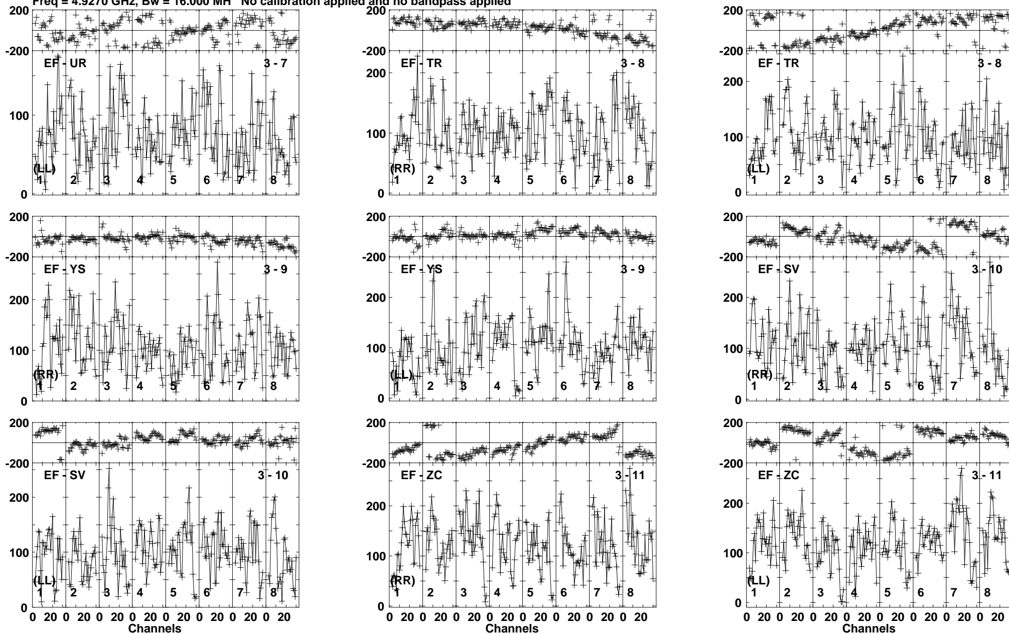
Lower frame: Micro Ampl Jy Top frame: Phas deg Vector averaged cross-power spectrum Baseline: EF (03) - UR (07) Timerange: 00/02:13:21 to 00/02:17:19
