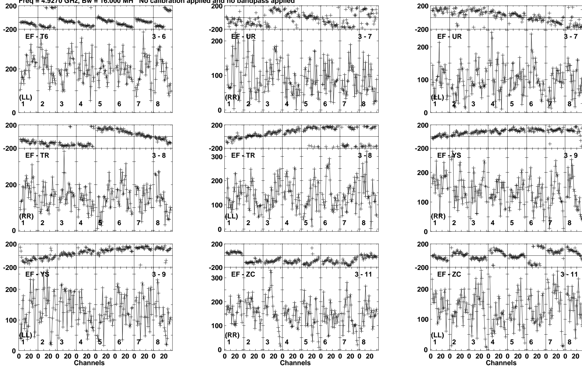
Lower frame: Micro Ampl Jy Top frame: Phas deg Vector averaged cross-power spectrum Baseline: EF (03) - T6 (06) Timerange: 00/09:55:21 to 00/09:59:19
