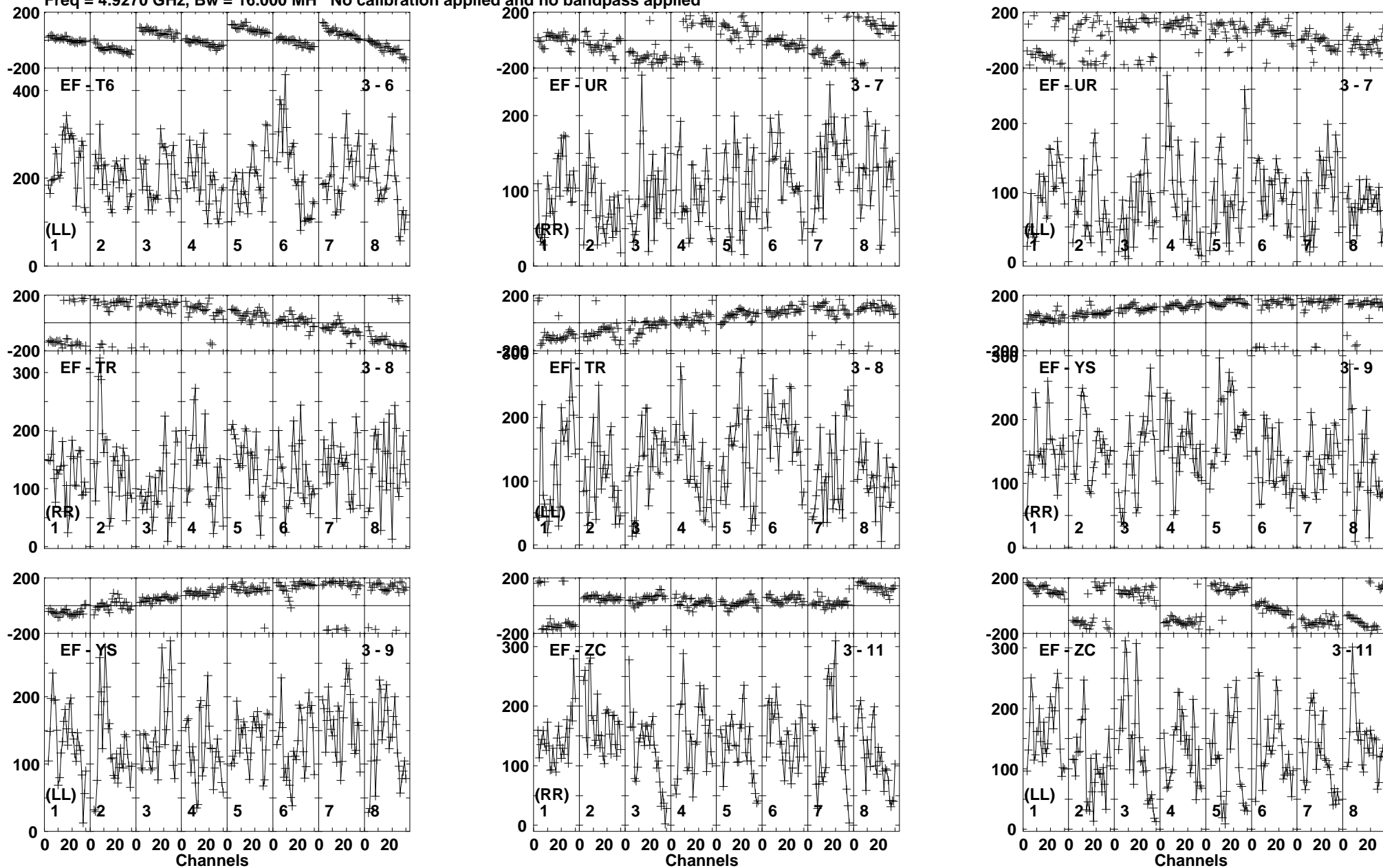
Lower frame: Micro Ampl Jy Top frame: Phas deg Vector averaged cross-power spectrum Baseline: EF (03) - T6 (06) Timerange: 00/10/01:21 to 00/10/05:19
