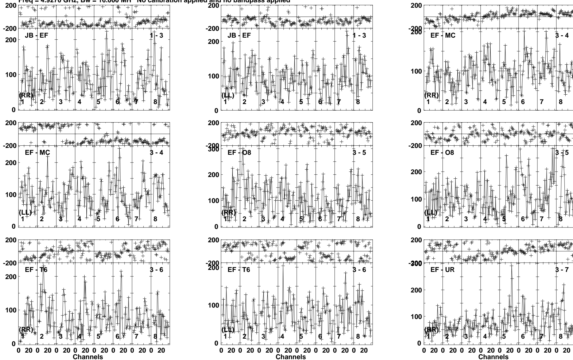
Lower frame: Micro Ampl Jy Top frame: Phas deg Vector averaged cross-power spectrum Baseline: JB (01) - EF (03) Timerange: 00/01:43:23 to 00/01:47:19
