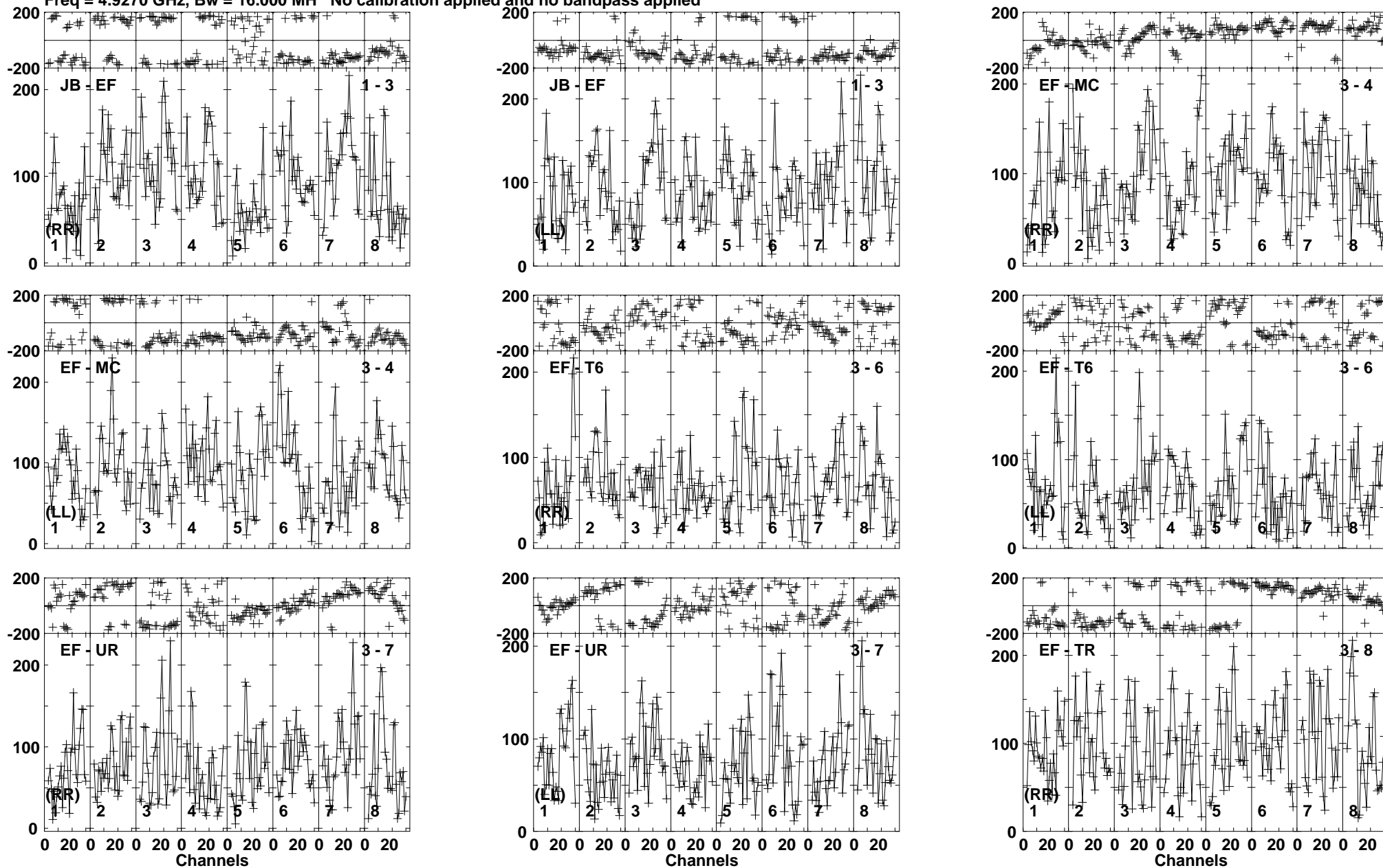
Lower frame: Micro Ampl Jy Top frame: Phas deg Vector averaged cross-power spectrum Baseline: JB (01) - EF (03) Timerange: 00/01:37:21 to 00/01:41:19
