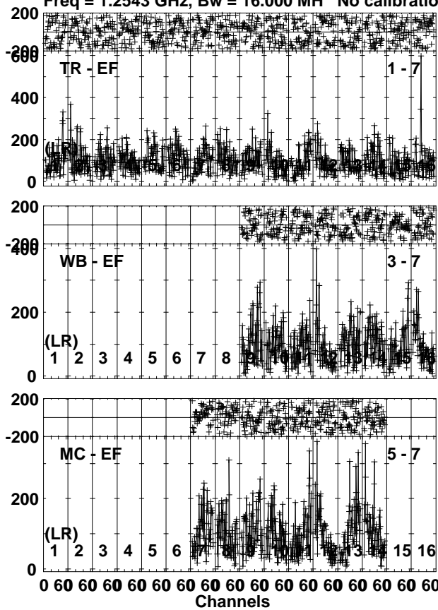
Lower frame: Micro Ampl Jy Top frame: Phas deg Vector averaged cross-power spectrum Several baselines displayed Timerange: 00/19:22:06 to 00/19:26:04
