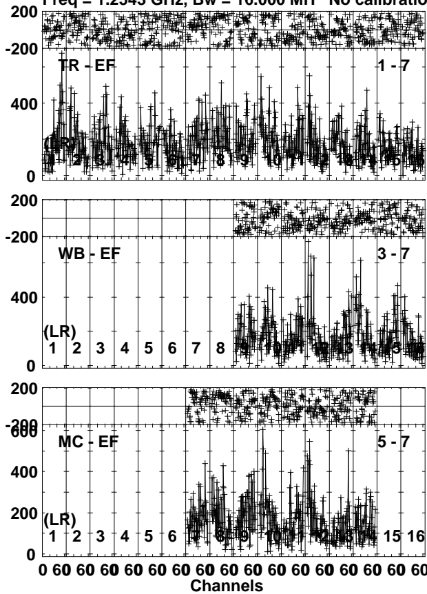
Lower frame: Micro Ampl Jy Top frame: Phas deg Vector averaged cross-power spectrum Several baselines displayed Timerange: 00/16:49:25 to 00/16:50:51
