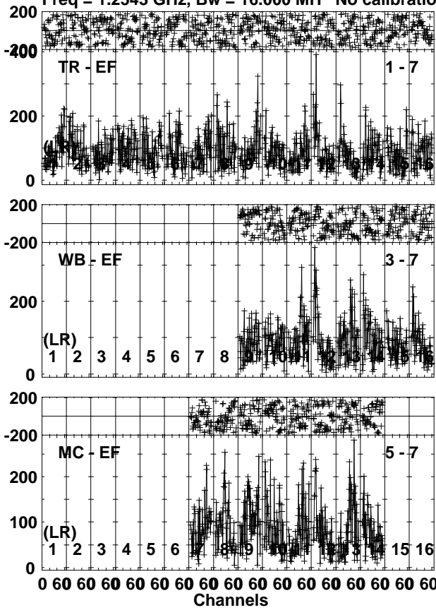
Lower frame: Micro Ampl Jy Top frame: Phas deg Vector averaged cross-power spectrum Several baselines displayed Timerange: 00/18:51:53 to 00/18:57:21
