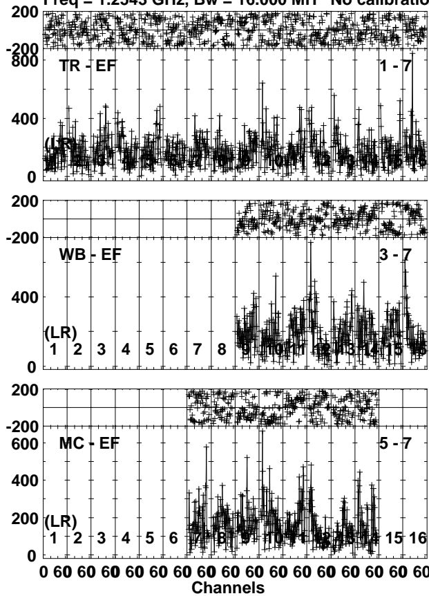
Lower frame: Micro Ampl Jy Top frame: Phas deg Vector averaged cross-power spectrum Several baselines displayed Timerange: 00/18:29:49 to 00/18:31:15
