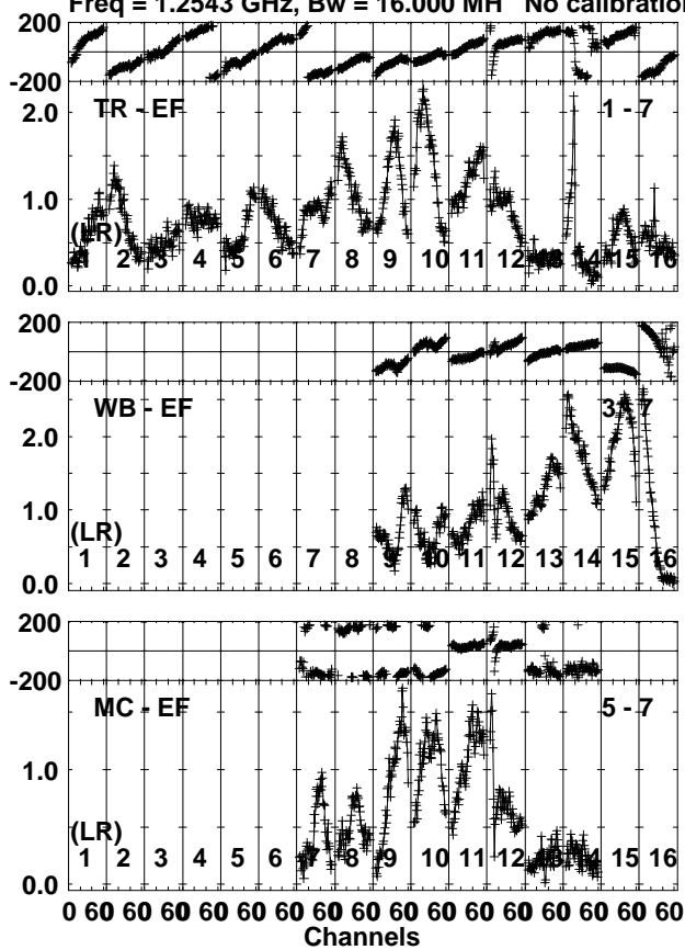
Lower frame: Milli Ampl Jy Top frame: Phas deg Vector averaged cross-power spectrum Several baselines displayed Timerange: 00/20:34:10 to 00/20:39:08
