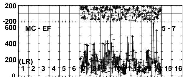
Lower frame: Micro Ampl Jy Top frame: Phas deg Vector averaged cross-power spectrum Several baselines displayed Timerange: 00/20:25:12 to 00/20:26:38
