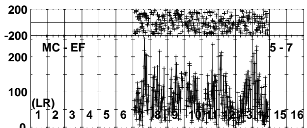
Lower frame: Micro Ampl Jy Top frame: Phas deg Vector averaged cross-power spectrum Several baselines displayed Timerange: 00/18:16:11 to 00/18:21:39
