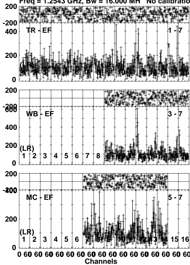
Lower frame: Micro Ampl Jy Top frame: Phas deg Vector averaged cross-power spectrum Several baselines displayed Timerange: 00/18:10:11 to 00/18:14:09
