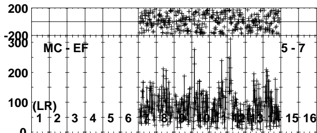
Lower frame: Micro Ampl Jy Top frame: Phas deg Vector averaged cross-power spectrum Several baselines displayed Timerange: 00/17:47:36 to 00/17:53:04
