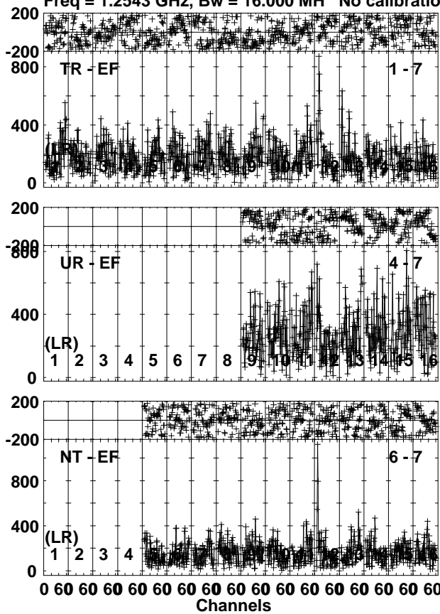
Lower frame: Micro Ampl Jy Top frame: Phas deg Vector averaged cross-power spectrum Several baselines displayed Timerange: 00/16:06:11 to 00/16:07:37
