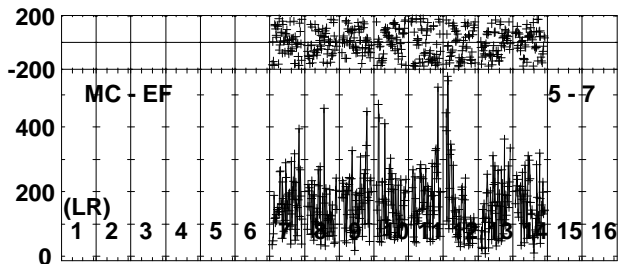
Lower frame: Micro Ampl Jy Top frame: Phas deg Vector averaged cross-power spectrum Several baselines displayed Timerange: 00/17:38:01 to 00/17:39:59
