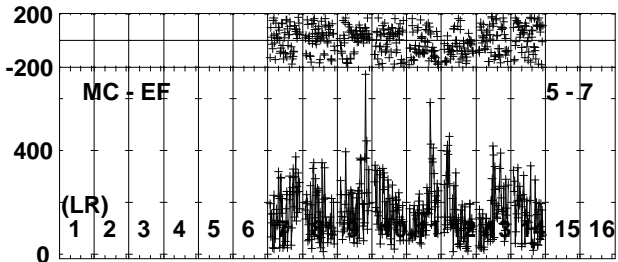
Lower frame: Micro Ampl Jy Top frame: Phas deg Vector averaged cross-power spectrum Several baselines displayed Timerange: 00/18:58:01 to 00/18:59:27
