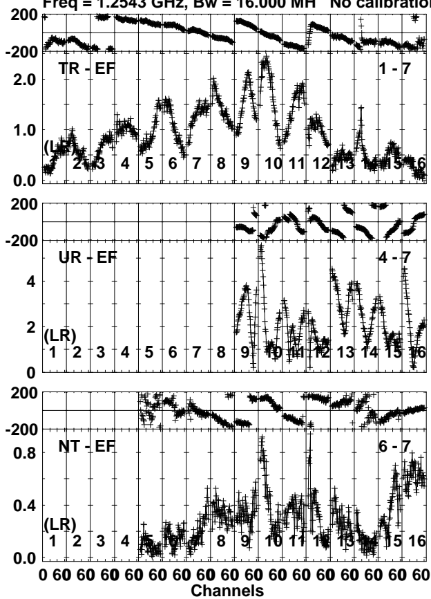
Lower frame: Milli Ampl Jy Top frame: Phas deg Vector averaged cross-power spectrum Several baselines displayed Timerange: 00/15:45:03 to 00/15:49:59
