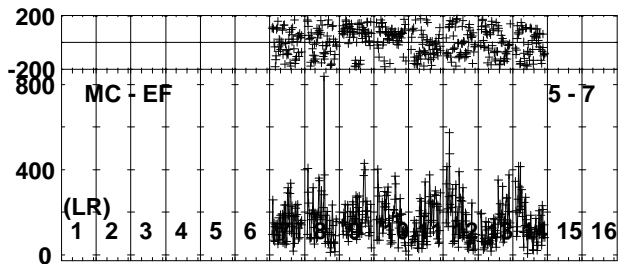
Lower frame: Micro Ampl Jy Top frame: Phas deg Vector averaged cross-power spectrum Several baselines displayed Timerange: 00/17:02:55 to 00/17:04:21
