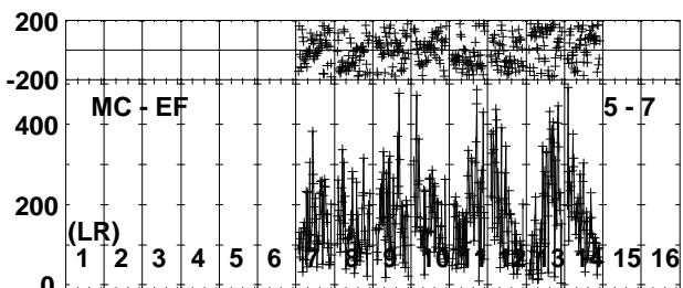
Lower frame: Micro Ampl Jy Top frame: Phas deg Vector averaged cross-power spectrum Several baselines displayed Timerange: 00/19:26:38 to 00/19:28:04
