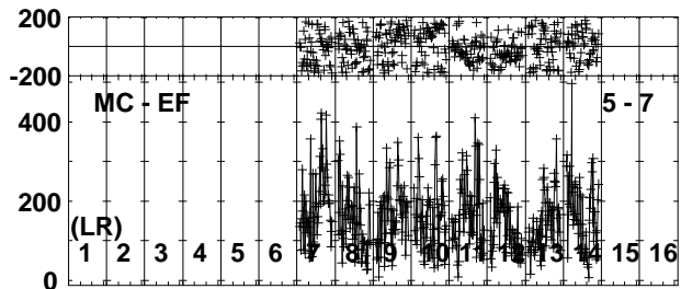
Lower frame: Micro Ampl Jy Top frame: Phas deg Vector averaged cross-power spectrum Several baselines displayed Timerange: 00/16:56:23 to 00/16:58:21
