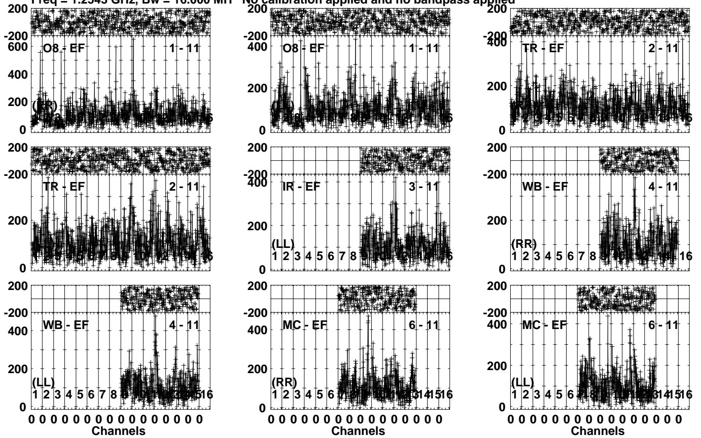
Lower frame: Micro Ampl Jy Top frame: Phas deg Vector averaged cross-power spectrum Several baselines displayed Timerange: 00/16:41:14 to 00/16:45:26
