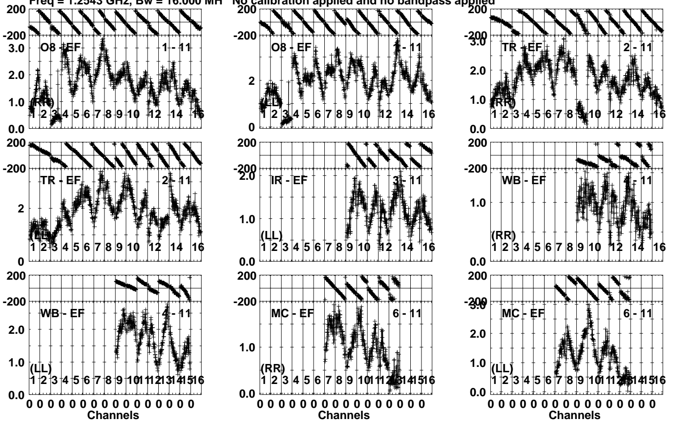
Lower frame: Milli Ampl Jy Top frame: Phas deg Vector averaged cross-power spectrum Several baselines displayed Timerange: 00/16:51:56 to 00/16:53:54
