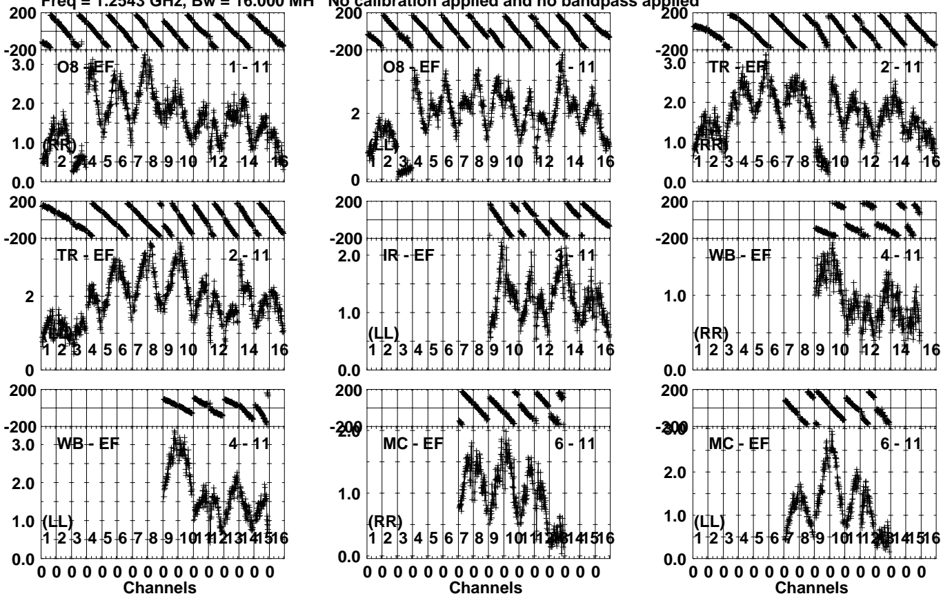
Lower frame: Milli Ampl Jy Top frame: Phas deg Vector averaged cross-power spectrum Several baselines displayed Timerange: 00/16:15:20 to 00/16:17:18
