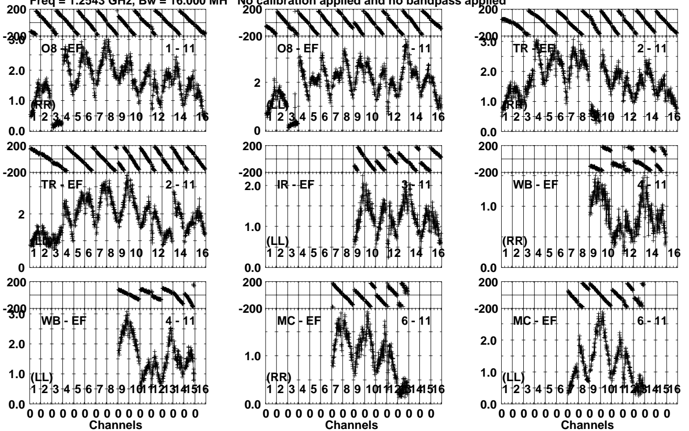
Lower frame: Milli Ampl Jy Top frame: Phas deg Vector averaged cross-power spectrum Several baselines displayed Timerange: 00/16:26:32 to 00/16:28:30
