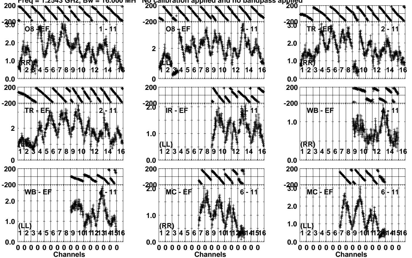
Lower frame: Milli Ampl Jy Top frame: Phas deg Vector averaged cross-power spectrum Several baselines displayed Timerange: 00/17:10:15 to 00/17:11:43
