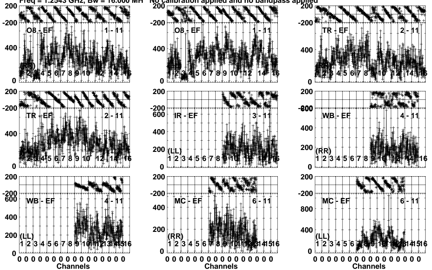
Lower frame: Micro Ampl Jy Top frame: Phas deg Vector averaged cross-power spectrum Several baselines displayed Timerange: 00/18:25:26 to 00/18:28:24
