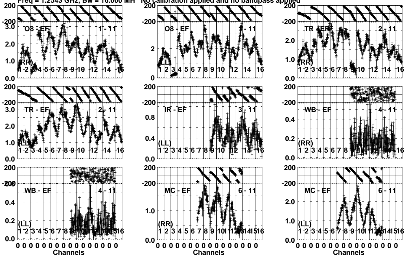
Lower frame: Milli Ampl Jy Top frame: Phas deg Vector averaged cross-power spectrum Several baselines displayed Timerange: 00/16:57:33 to 00/16:59:01
