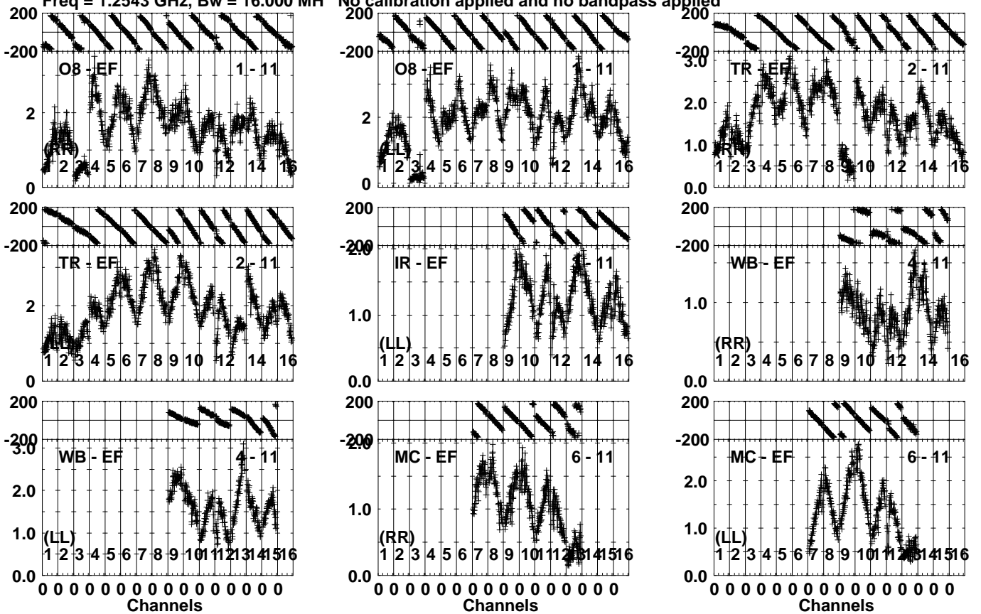
Lower frame: Milli Ampl Jy Top frame: Phas deg Vector averaged cross-power spectrum Several baselines displayed Timerange: 00/16:09:20 to 00/16:10:48
