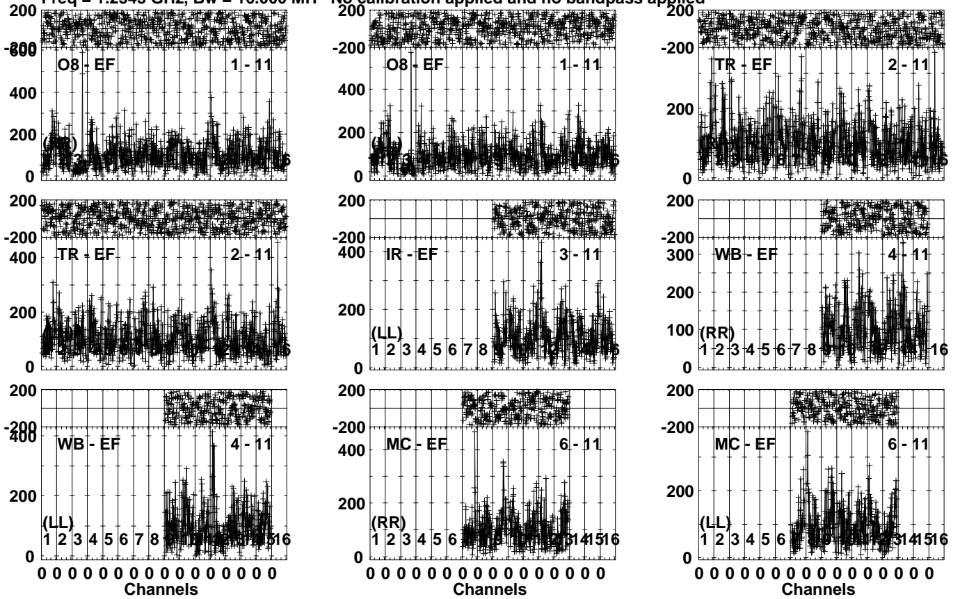
Lower frame: Micro Ampl Jy Top frame: Phas deg Vector averaged cross-power spectrum Several baselines displayed Timerange: 00/19:07:28 to 00/19:11:40
