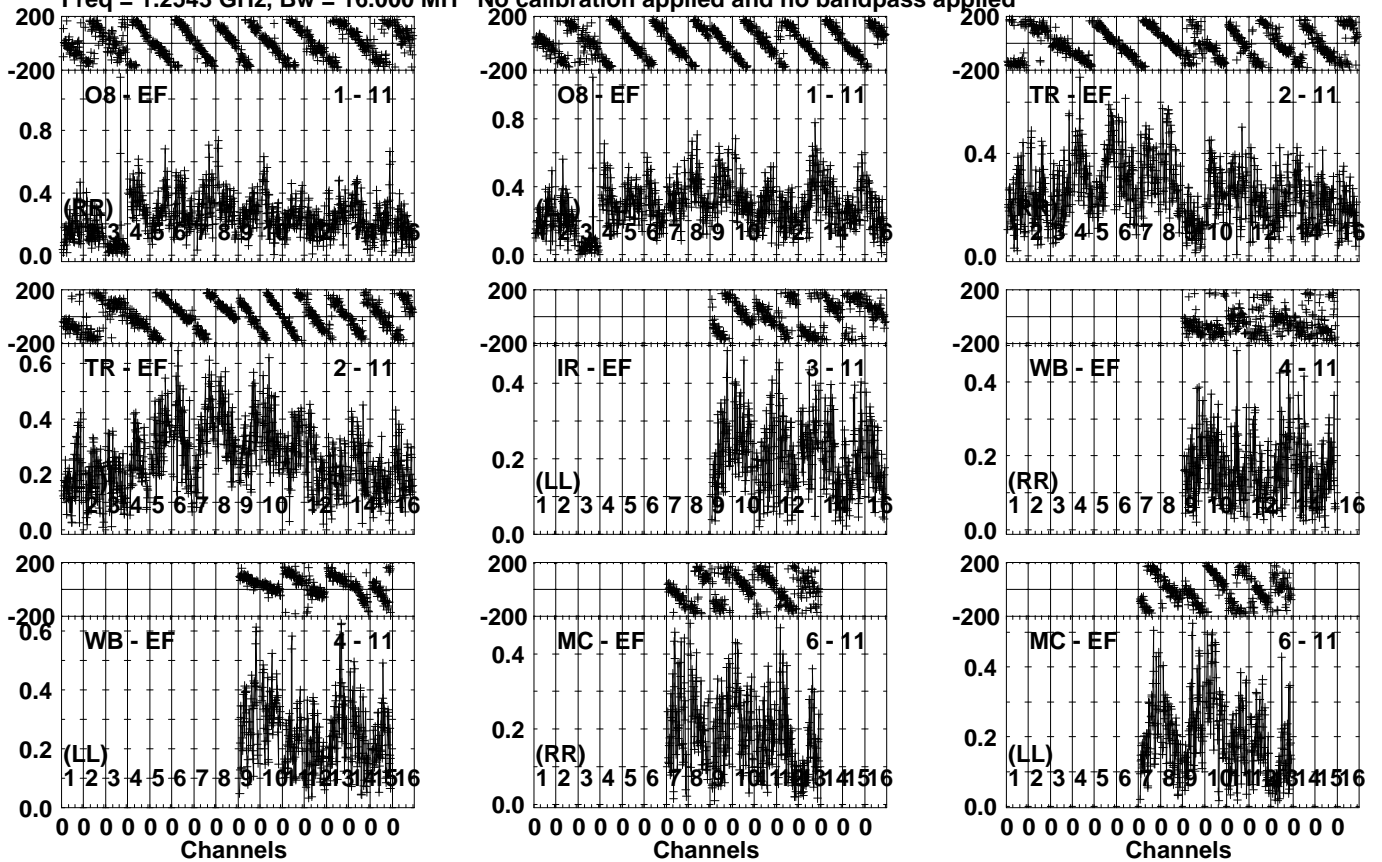
Lower frame: Milli Ampl Jy Top frame: Phas deg Vector averaged cross-power spectrum Several baselines displayed Timerange: 00/18:55:52 to 00/18:58:50
