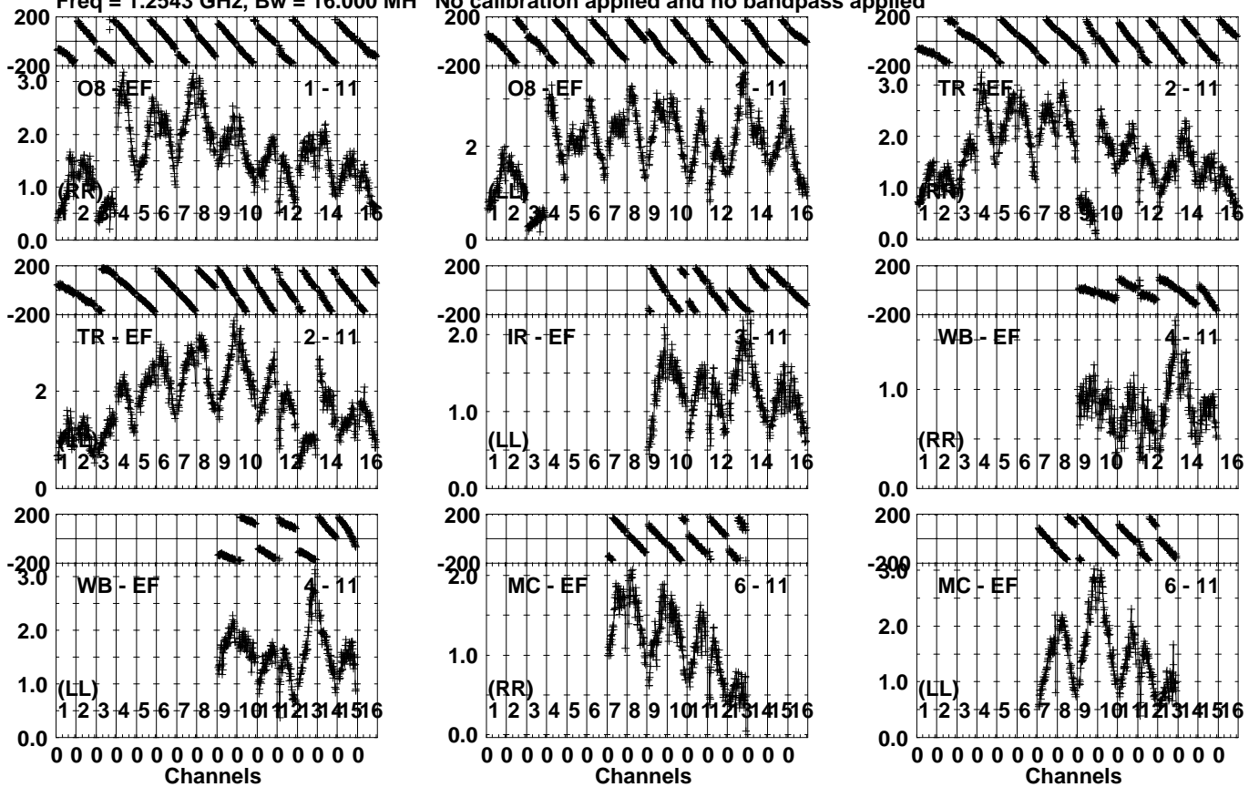
Lower frame: Milli Ampl Jy Top frame: Phas deg Vector averaged cross-power spectrum Several baselines displayed Timerange: 00/15:25:55 to 00/15:27:53
