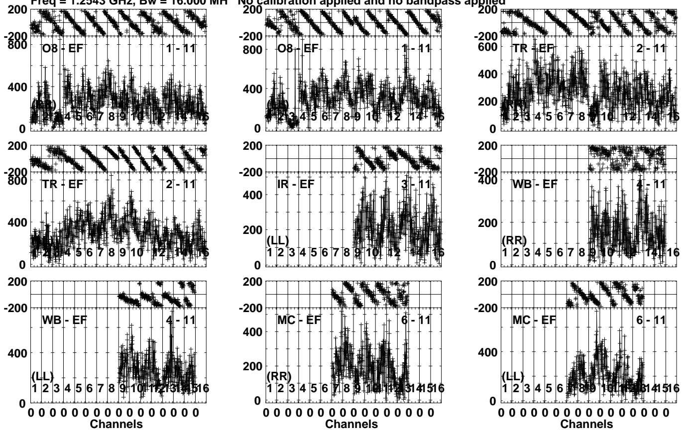
Lower frame: Micro Ampl Jy Top frame: Phas deg Vector averaged cross-power spectrum Several baselines displayed Timerange: 00/17:54:54 to 00/17:57:52
