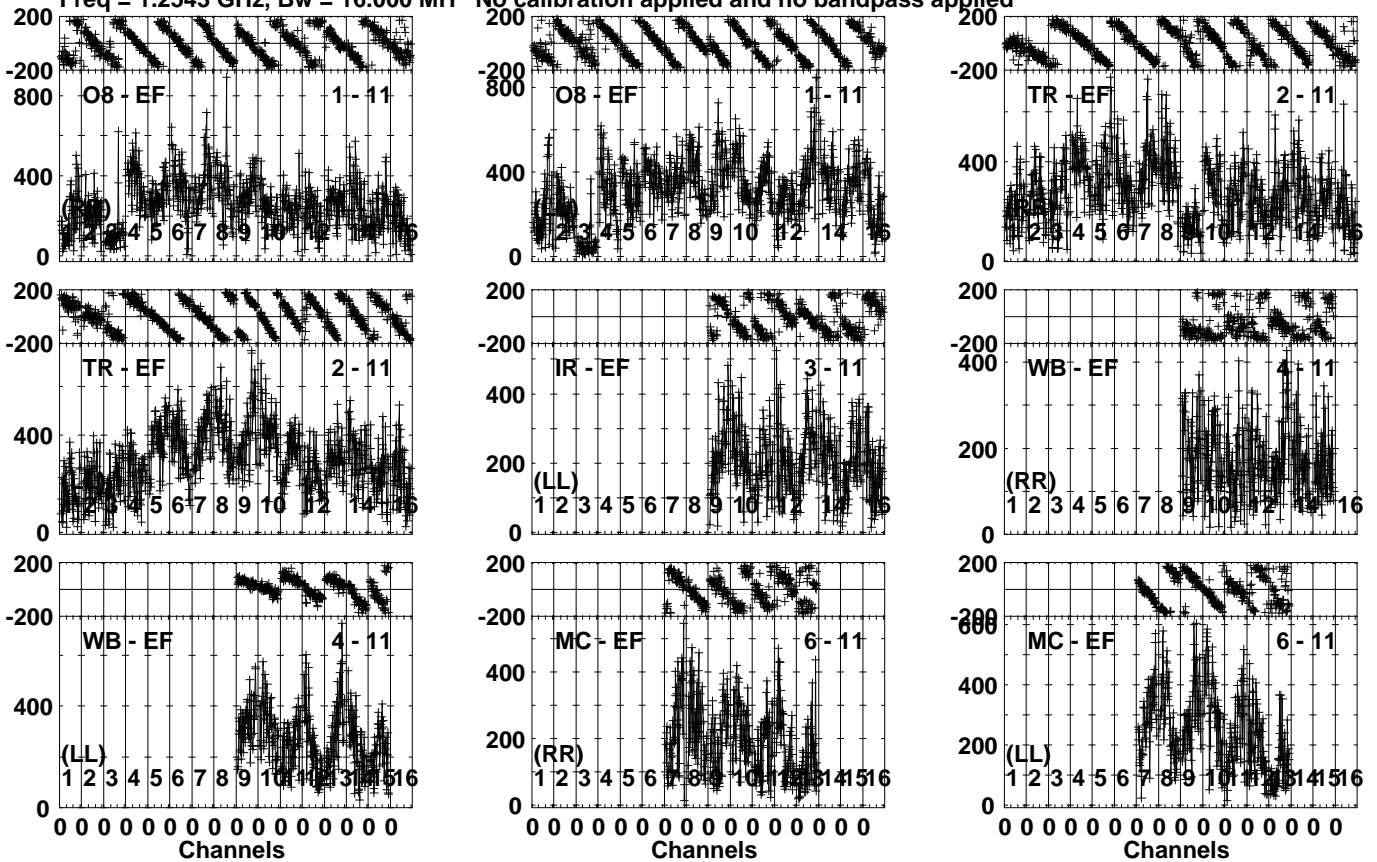
Lower frame: Micro Ampl Jy Top frame: Phas deg Vector averaged cross-power spectrum Several baselines displayed Timerange: 00/16:53:56 to 00/16:56:54
