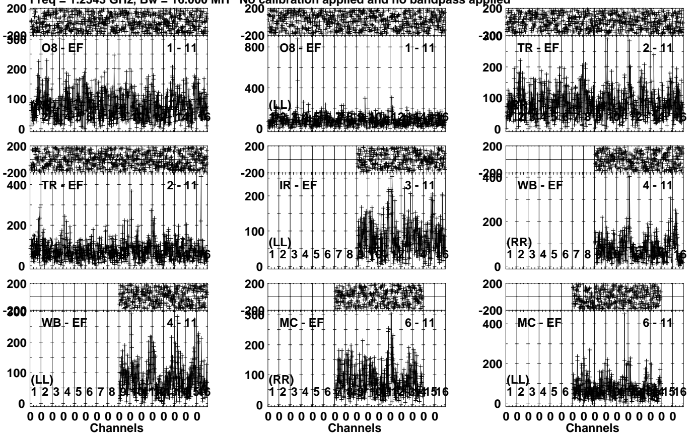
Lower frame: Micro Ampl Jy Top frame: Phas deg Vector averaged cross-power spectrum Several baselines displayed Timerange: 00/14:03:34 to 00/14:10:02
