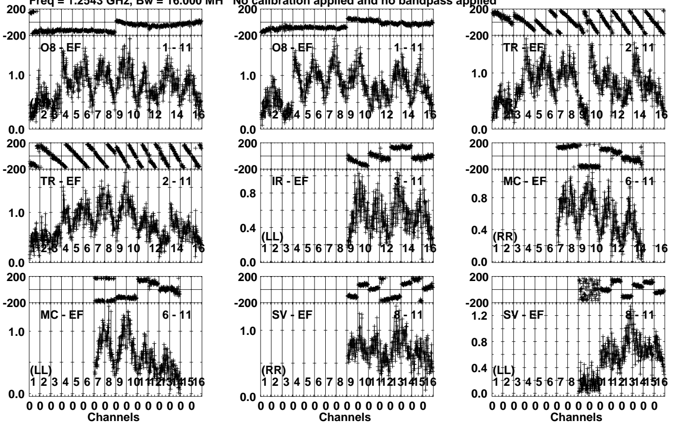
Lower frame: Milli Ampl Jy Top frame: Phas deg Vector averaged cross-power spectrum Several baselines displayed Timerange: 00/11:14:04 to 00/11:16:02
