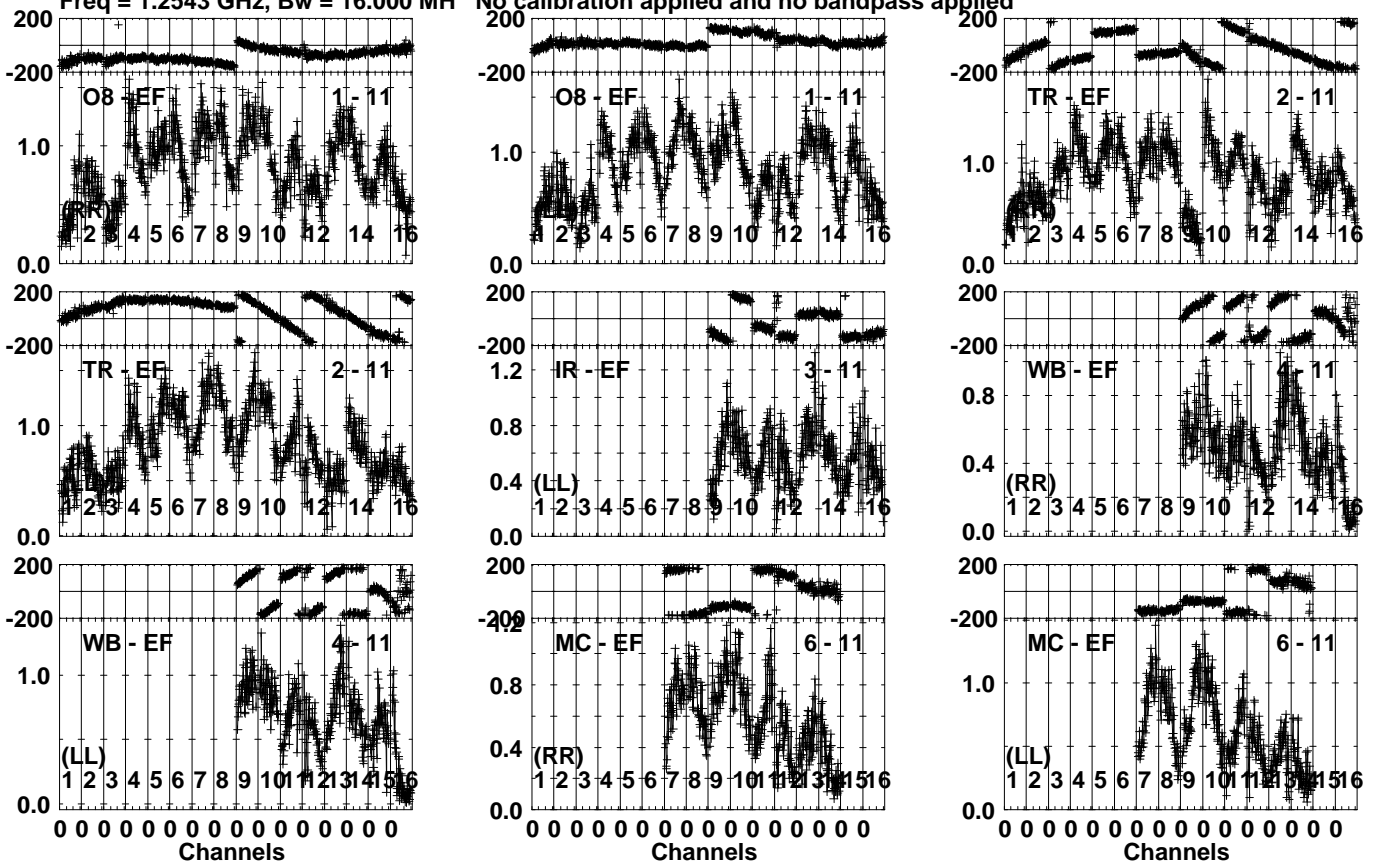
Lower frame: Milli Ampl Jy Top frame: Phas deg Vector averaged cross-power spectrum Several baselines displayed Timerange: 00/14:02:06 to 00/14:03:32
