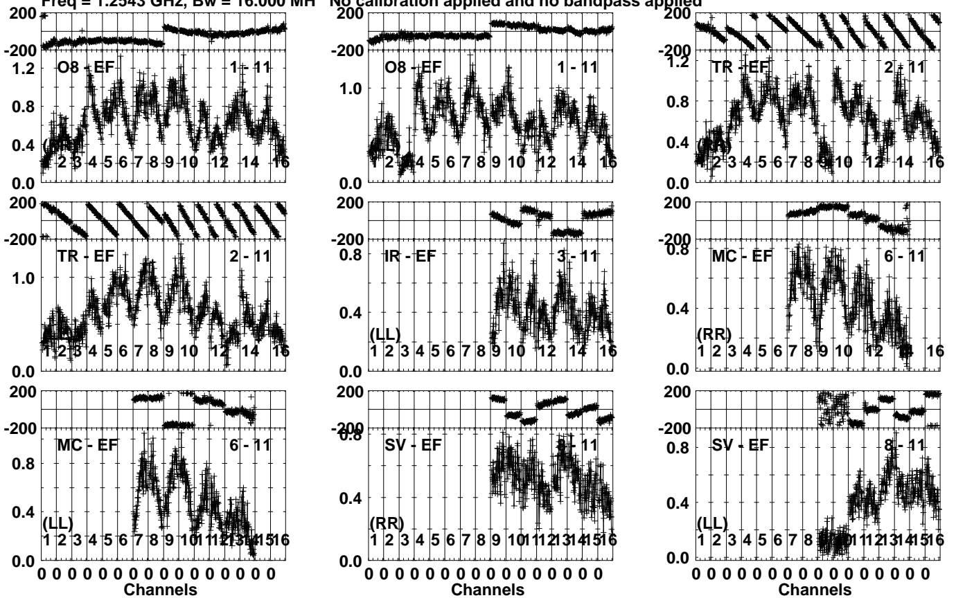
Lower frame: Milli Ampl Jy Top frame: Phas deg Vector averaged cross-power spectrum Several baselines displayed Timerange: 00/11:41:42 to 00/11:45:10
