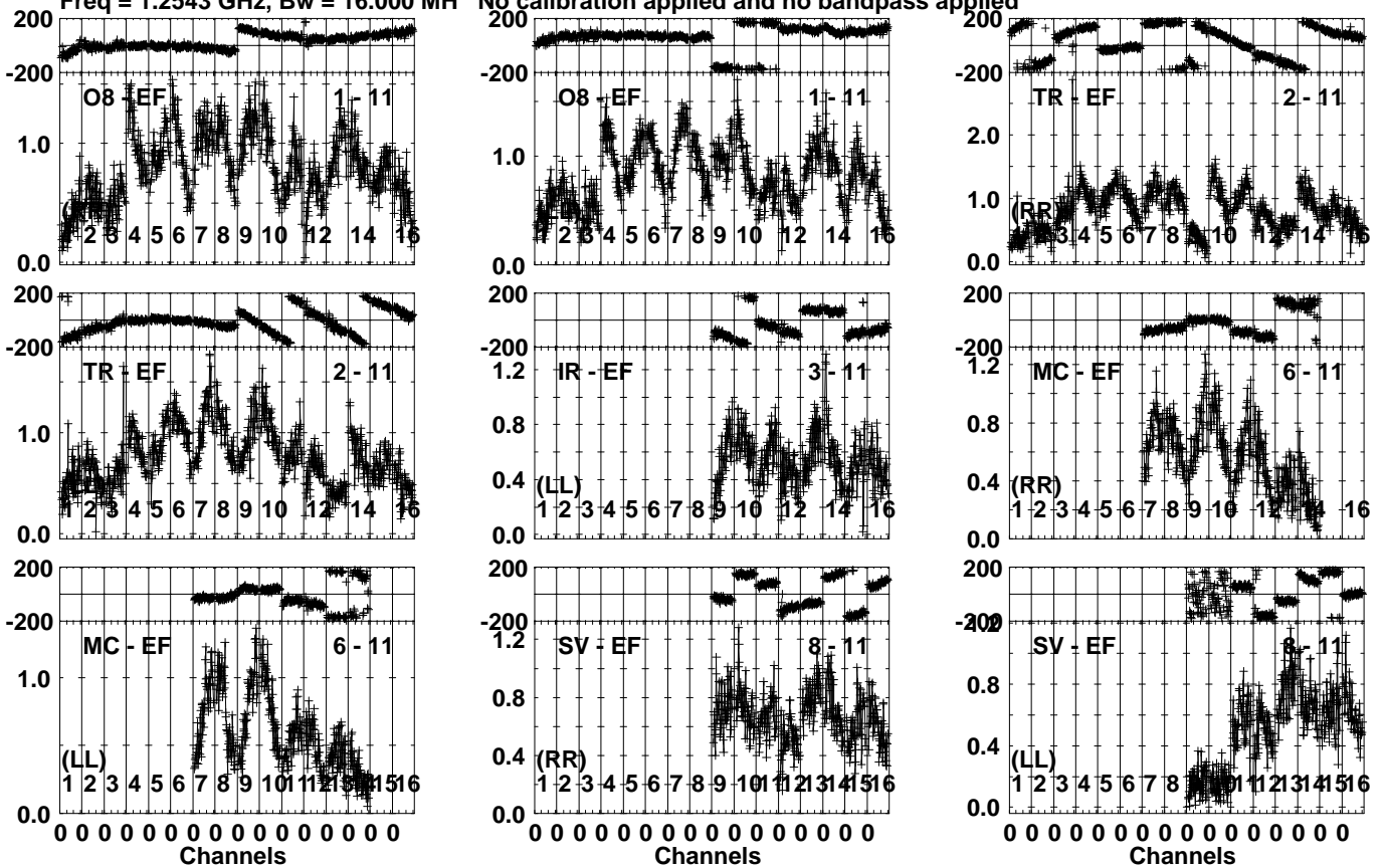
Lower frame: Milli Ampl Jy Top frame: Phas deg Vector averaged cross-power spectrum Several baselines displayed Timerange: 00/12:33:32 to 00/12:35:30
