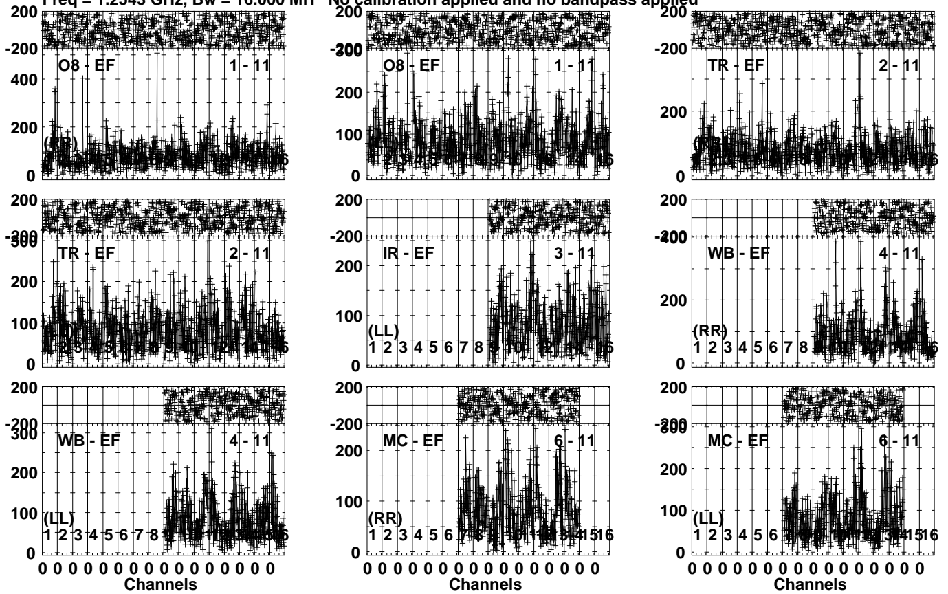
Lower frame: Micro Ampl Jy Top frame: Phas deg Vector averaged cross-power spectrum Several baselines displayed Timerange: 00/15:36:44 to 00/15:42:42
