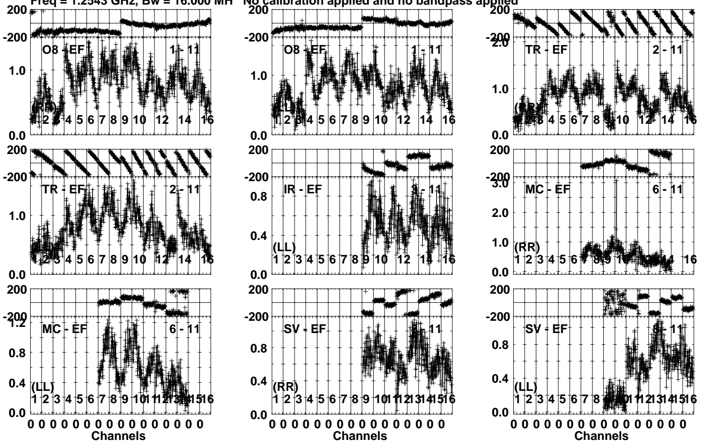
Lower frame: Milli Ampl Jy Top frame: Phas deg Vector averaged cross-power spectrum Several baselines displayed Timerange: 00/11:23:08 to 00/11:24:36
