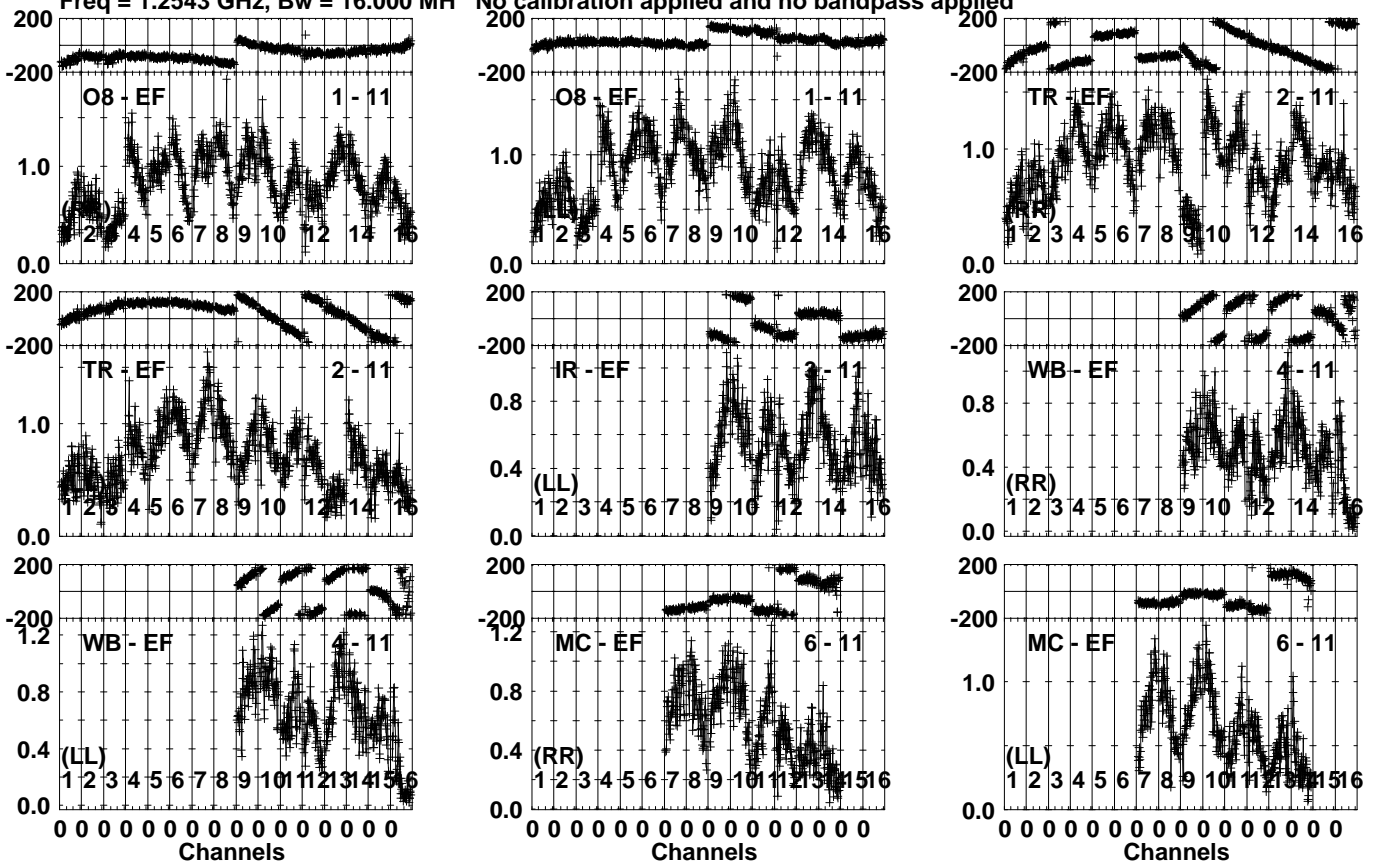
Lower frame: Milli Ampl Jy Top frame: Phas deg Vector averaged cross-power spectrum Several baselines displayed Timerange: 00/13:53:00 to 00/13:54:58
