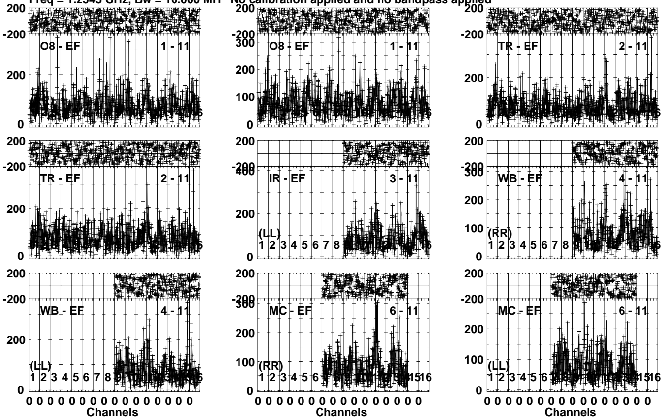
Lower frame: Micro Ampl Jy Top frame: Phas deg Vector averaged cross-power spectrum Several baselines displayed Timerange: 00/13:55:00 to 00/14:01:28
