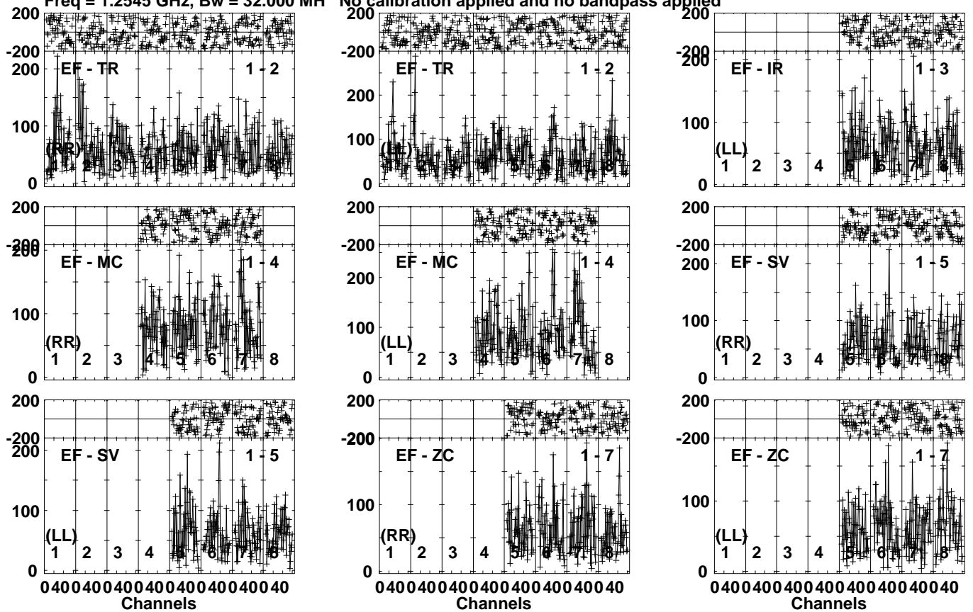
Lower frame: Micro Ampl Jy Top frame: Phas deg Vector averaged cross-power spectrum Several baselines displayed Timerange: 00/10:39:06 to 00/10:44:38
