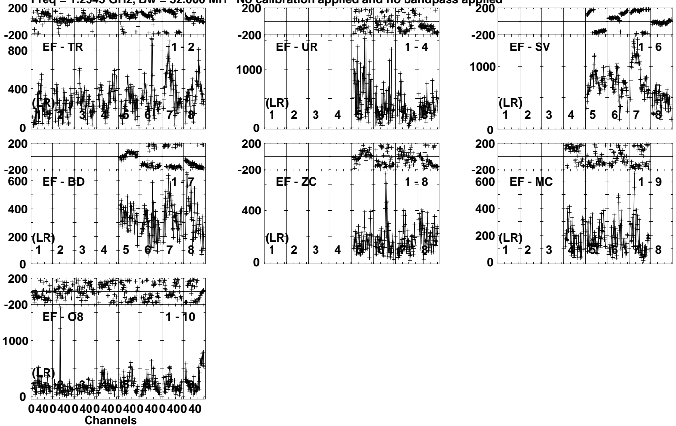
Lower frame: Micro Ampl Jy Top frame: Phas deg Vector averaged cross-power spectrum Several baselines displayed Timerange: 00/03:33:47 to 00/03:35:55
