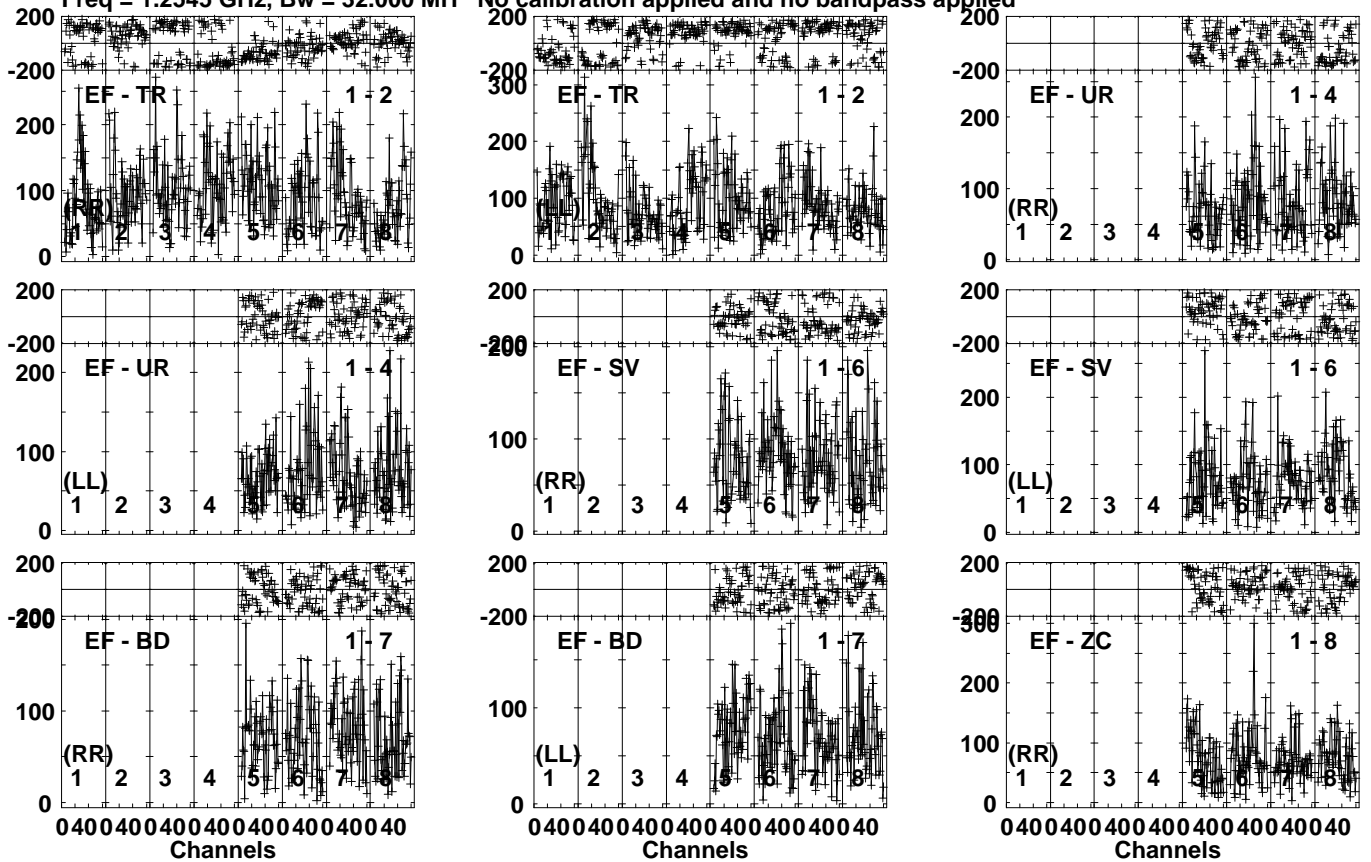
Lower frame: Micro Ampl Jy Top frame: Phas deg Vector averaged cross-power spectrum Several baselines displayed Timerange: 00/10:26:38 to 00/10:30:34
