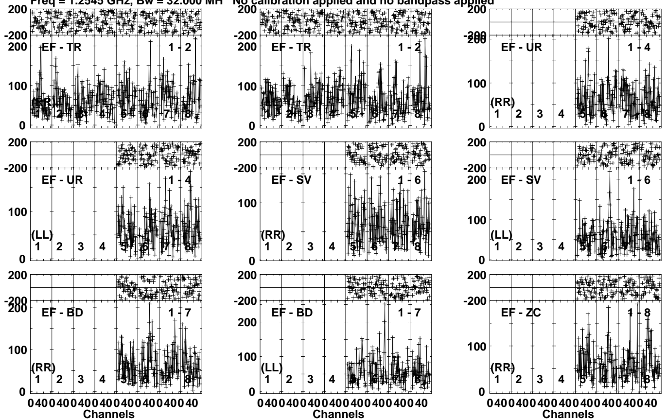
Lower frame: Micro Ampl Jy Top frame: Phas deg Vector averaged cross-power spectrum Several baselines displayed Timerange: 00/02:21:59 to 00/02:27:27
