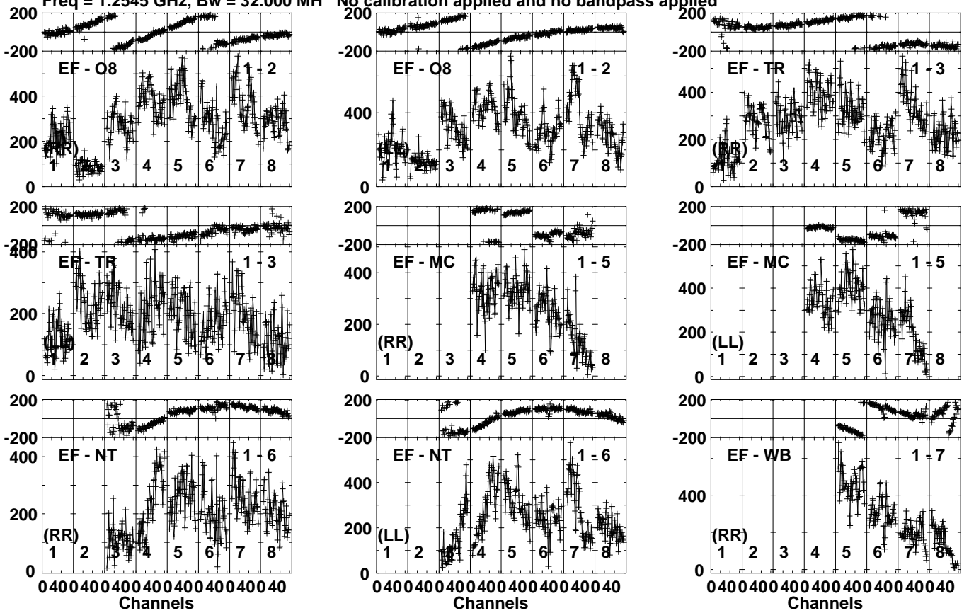
Lower frame: Micro Ampl Jy Top frame: Phas deg Vector averaged cross-power spectrum Several baselines displayed Timerange: 00/17:29:04 to 00/17:32:36
