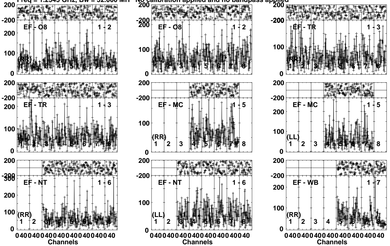
Lower frame: Micro Ampl Jy Top frame: Phas deg Vector averaged cross-power spectrum Several baselines displayed Timerange: 00/17:05:44 to 00/17:11:12
