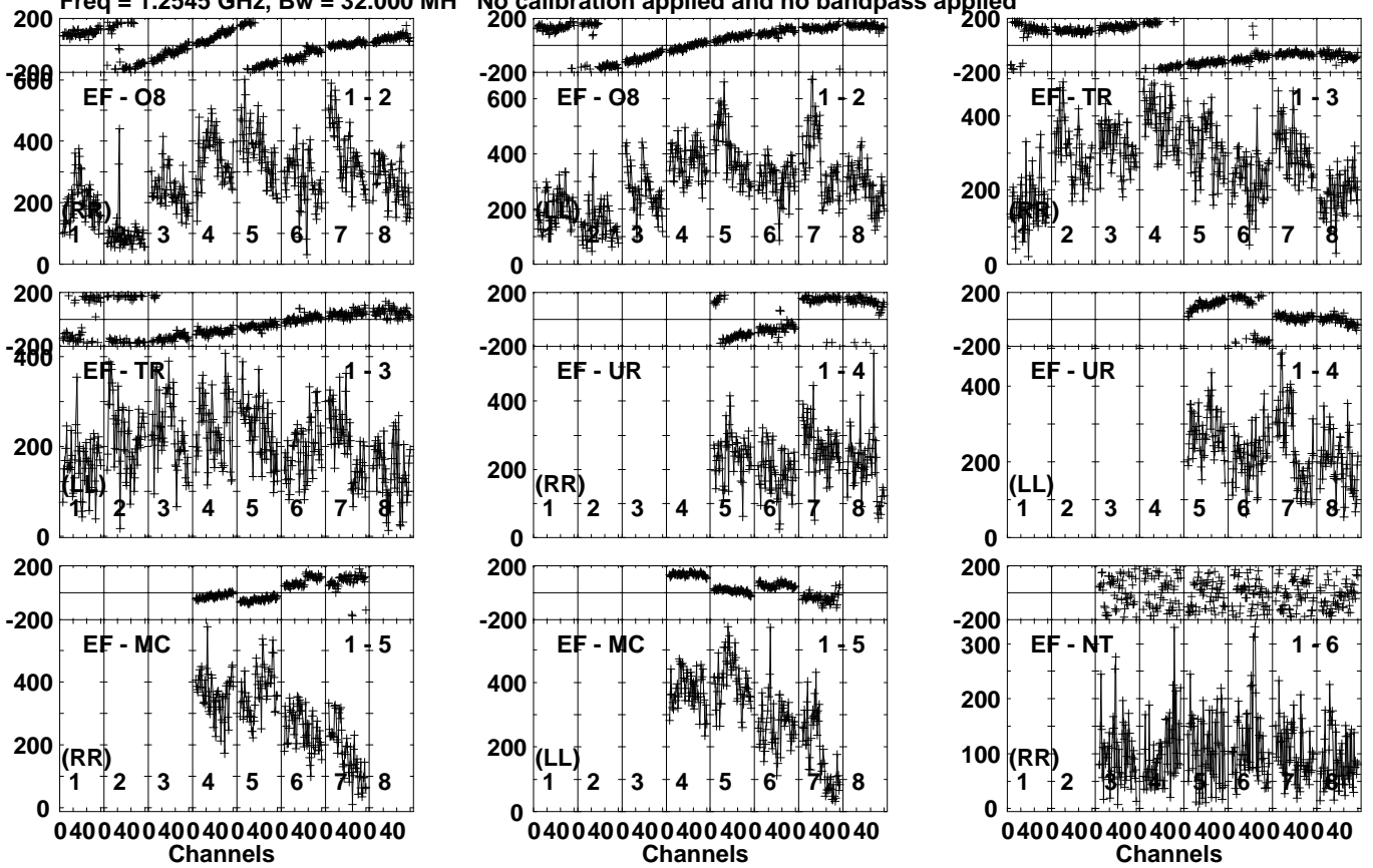
Lower frame: Micro Ampl Jy Top frame: Phas deg Vector averaged cross-power spectrum Several baselines displayed Timerange: 00/16:15:44 to 00/16:19:14
