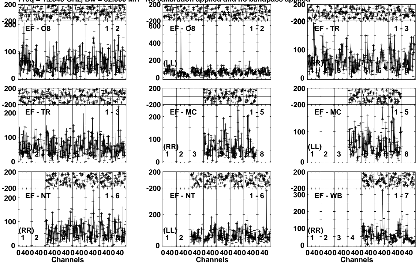
Lower frame: Micro Ampl Jy Top frame: Phas deg Vector averaged cross-power spectrum Several baselines displayed Timerange: 00/17:21:13 to 00/17:26:41
