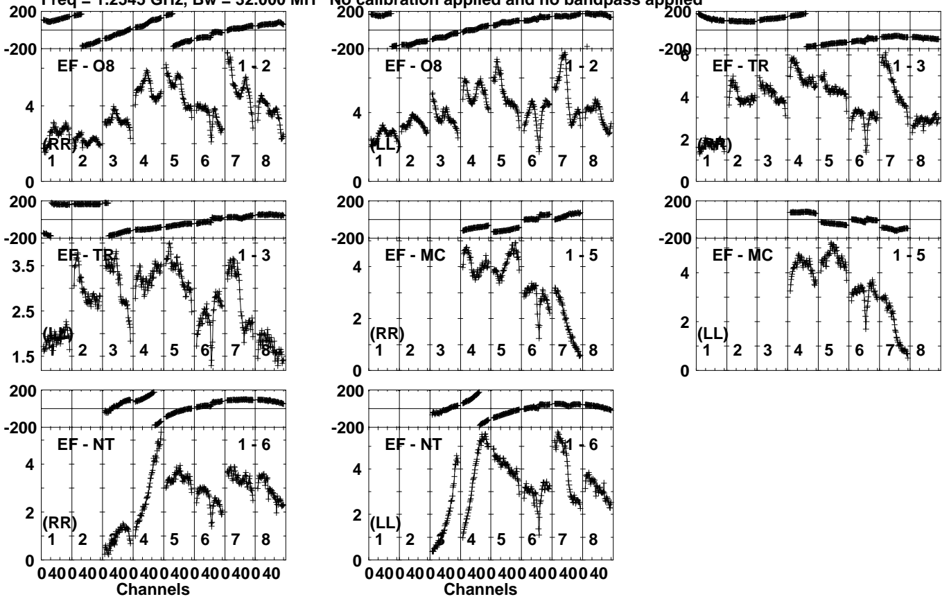
Lower frame: Milli Ampl Jy Top frame: Phas deg Vector averaged cross-power spectrum Several baselines displayed Timerange: 00/15:58:44 to 00/16:00:10
