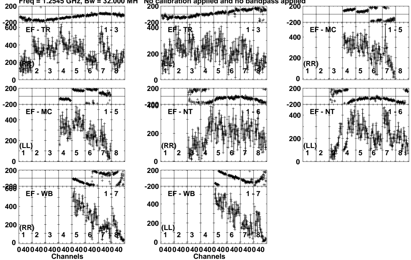
Lower frame: Micro Ampl Jy Top frame: Phas deg Vector averaged cross-power spectrum Several baselines displayed Timerange: 00/18:05:43 to 00/18:09:15
