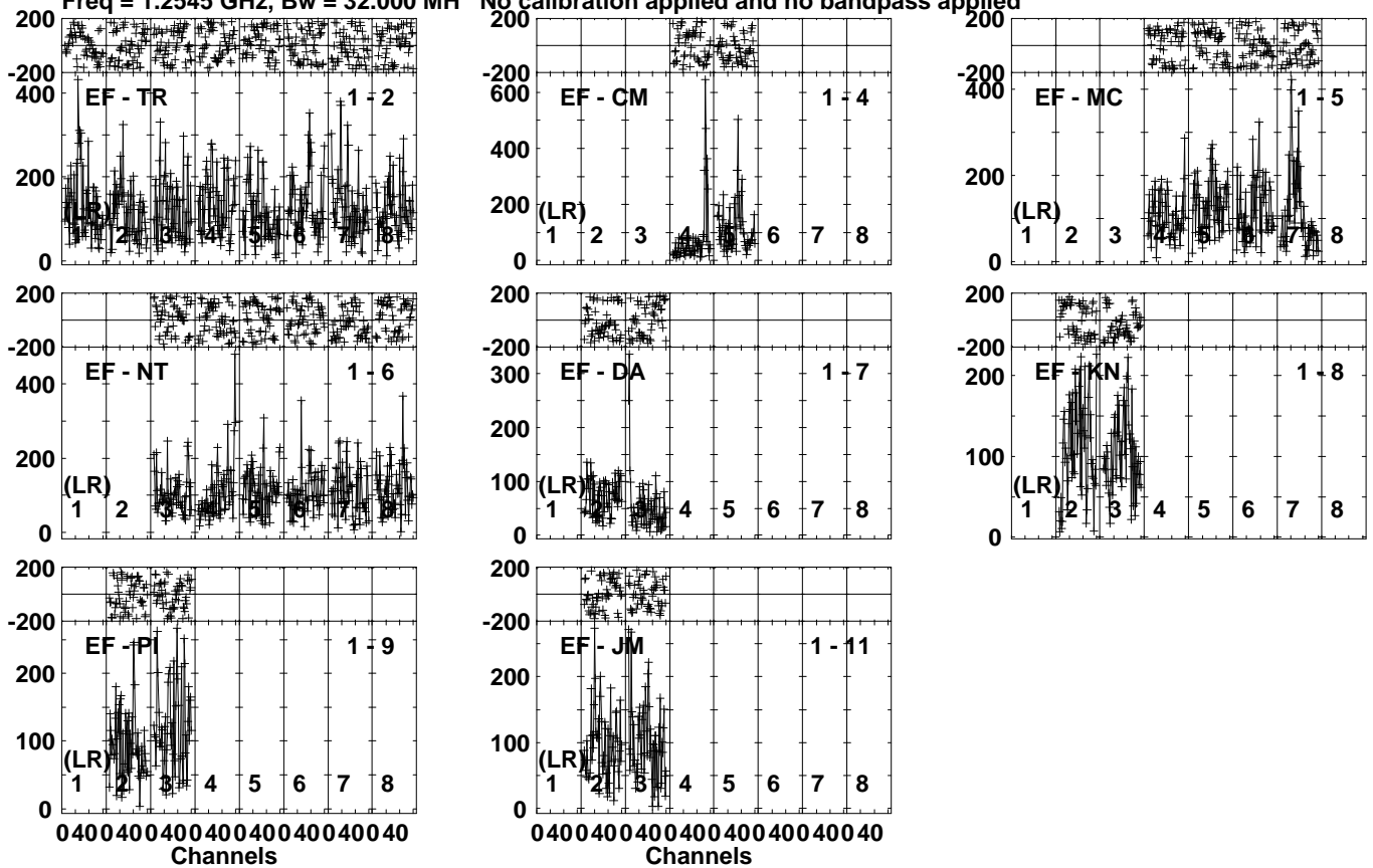
Lower frame: Micro Ampl Jy Top frame: Phas deg Vector averaged cross-power spectrum Several baselines displayed Timerange: 00/14:06:43 to 00/14:08:11
