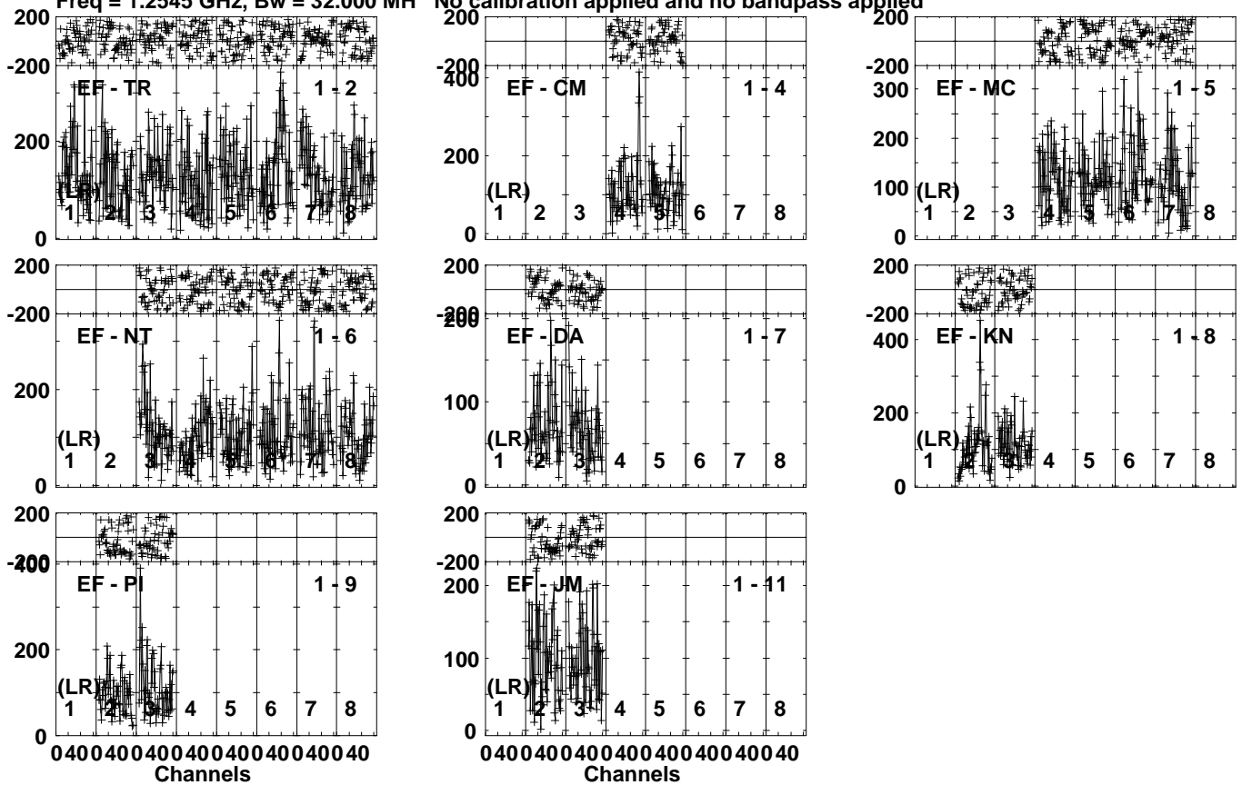
Lower frame: Micro Ampl Jy Top frame: Phas deg Vector averaged cross-power spectrum Several baselines displayed Timerange: 00/12:52:13 to 00/12:53:41
