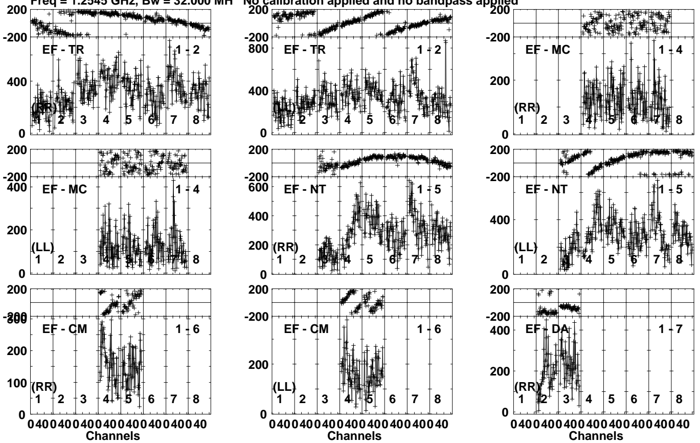
Lower frame: Micro Ampl Jy Top frame: Phas deg Vector averaged cross-power spectrum Several baselines displayed Timerange: 01/02:55:07 to 01/02:56:35
