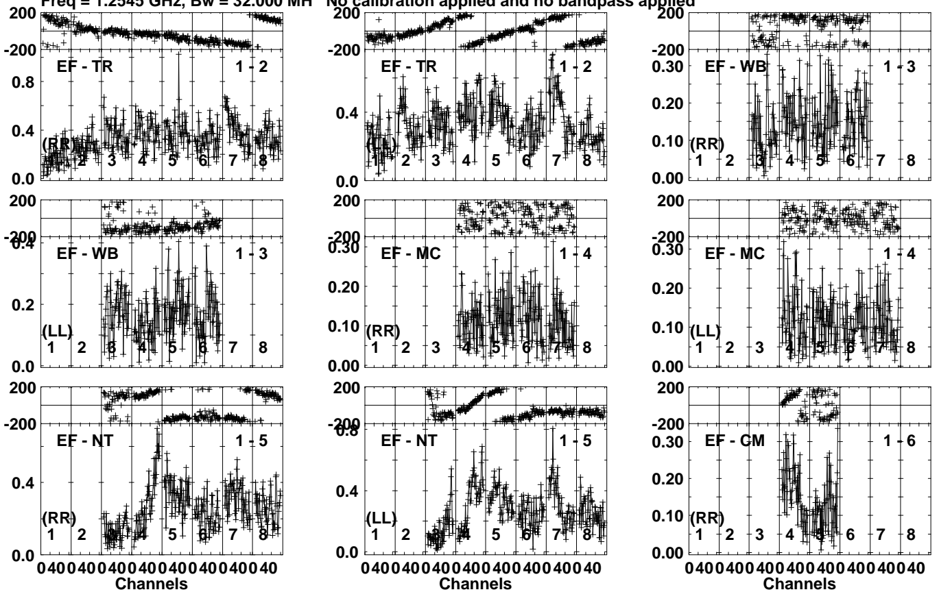
Lower frame: Milli Ampl Jy Top frame: Phas deg Vector averaged cross-power spectrum Several baselines displayed Timerange: 01/01:39:30 to 01/01:40:58
