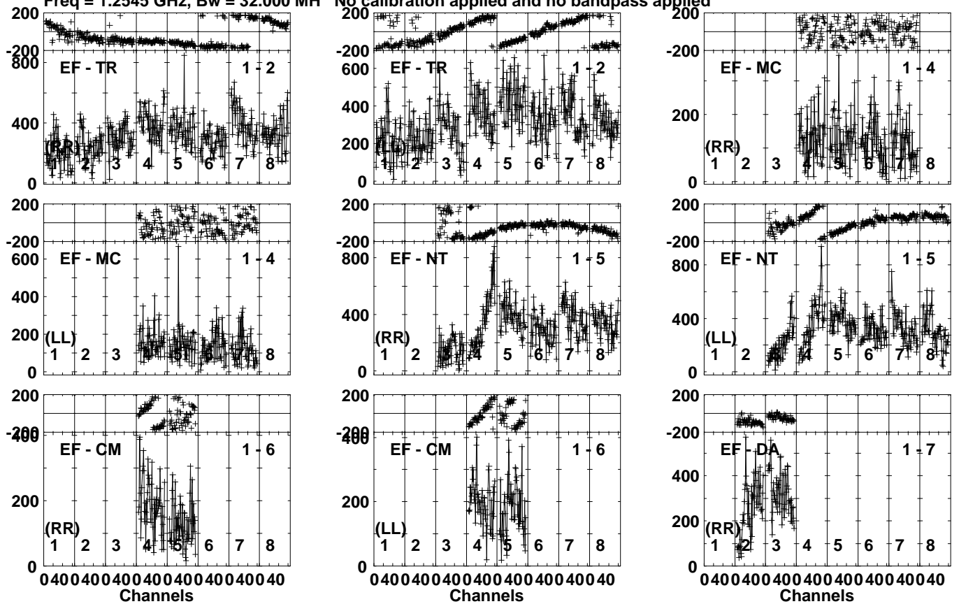
Lower frame: Micro Ampl Jy Top frame: Phas deg Vector averaged cross-power spectrum Several baselines displayed Timerange: 01/03:32:15 to 01/03:34:13
