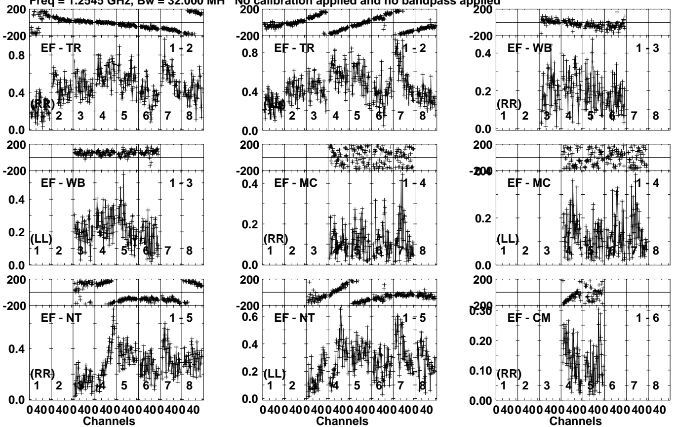
Lower frame: Milli Ampl Jy Top frame: Phas deg Vector averaged cross-power spectrum Several baselines displayed Timerange: 01/01:09:19 to 01/01:10:47
