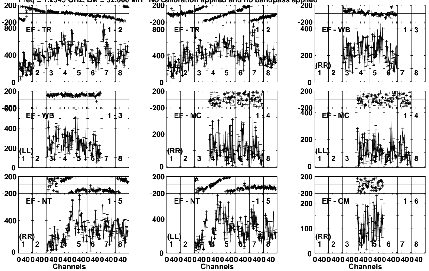
Lower frame: Micro Ampl Jy Top frame: Phas deg Vector averaged cross-power spectrum Several baselines displayed Timerange: 01/01:16:34 to 01/01:18:34
