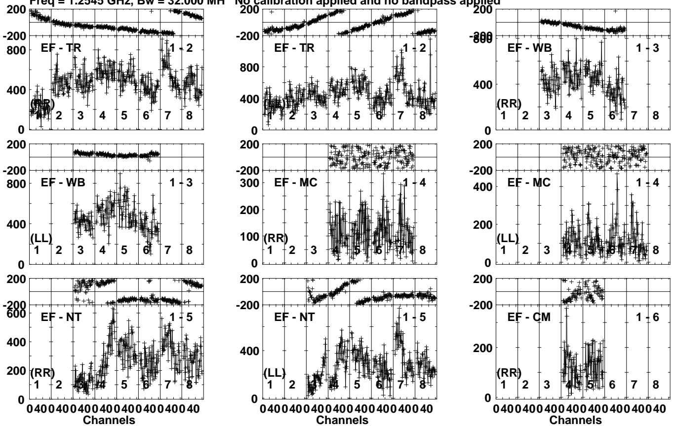
Lower frame: Micro Ampl Jy Top frame: Phas deg Vector averaged cross-power spectrum Several baselines displayed Timerange: 01/01:00:50 to 01/01:02:48
