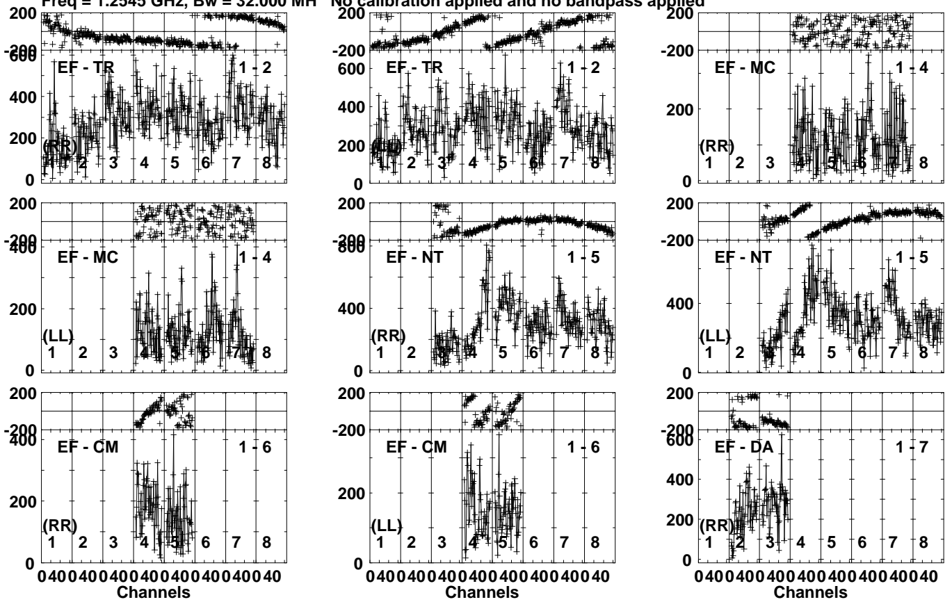
Lower frame: Micro Ampl Jy Top frame: Phas deg Vector averaged cross-power spectrum Several baselines displayed Timerange: 01/03:10:52 to 01/03:12:20
