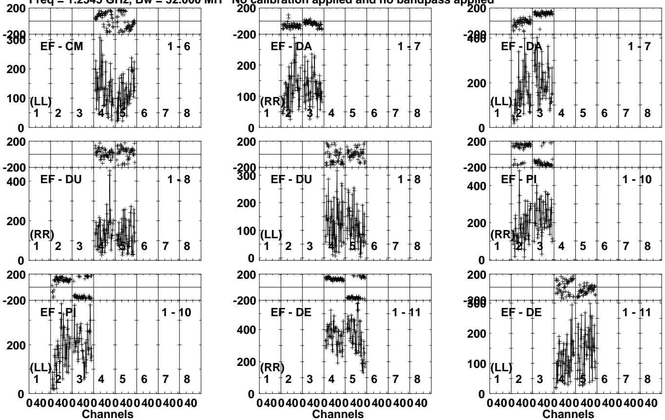
Lower frame: Micro Ampl Jy Top frame: Phas deg Vector averaged cross-power spectrum Several baselines displayed Timerange: 01/01:09:19 to 01/01:10:47
