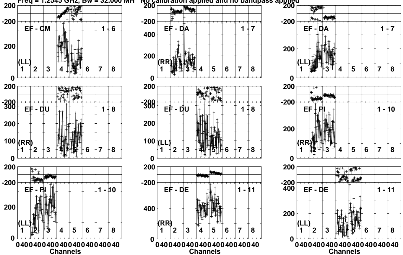
Lower frame: Micro Ampl Jy Top frame: Phas deg Vector averaged cross-power spectrum Several baselines displayed Timerange: 01/01:39:30 to 01/01:40:58
