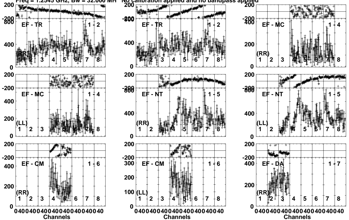
Lower frame: Micro Ampl Jy Top frame: Phas deg Vector averaged cross-power spectrum Several baselines displayed Timerange: 01/03:02:24 to 01/03:04:22
