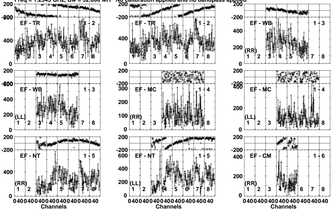
Lower frame: Micro Ampl Jy Top frame: Phas deg Vector averaged cross-power spectrum Several baselines displayed Timerange: 01/01:55:15 to 01/01:56:43
