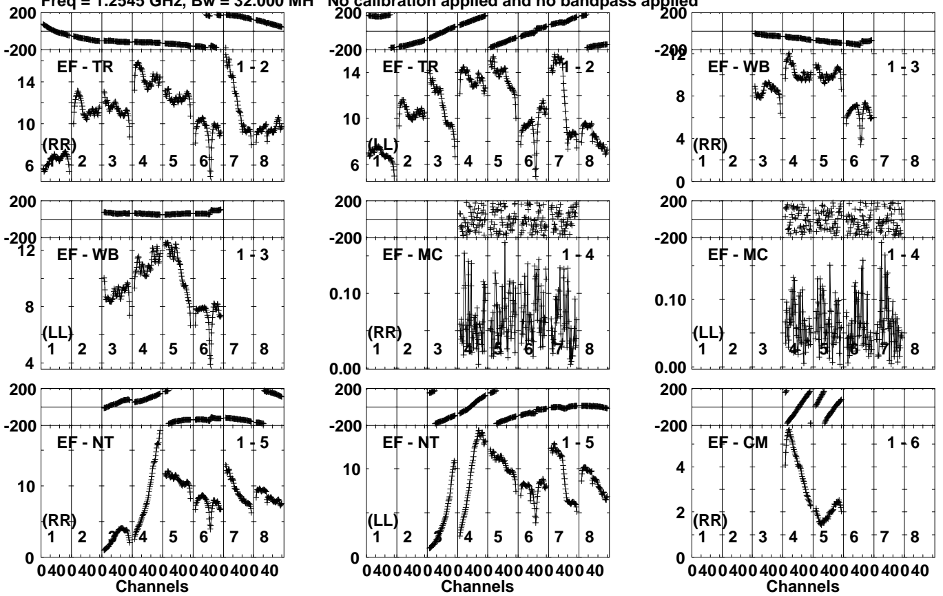
Lower frame: Milli Ampl Jy Top frame: Phas deg Vector averaged cross-power spectrum Several baselines displayed Timerange: 01/06:49:05 to 01/06:53:03
