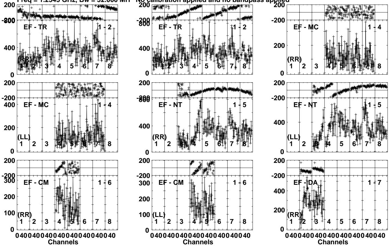
Lower frame: Micro Ampl Jy Top frame: Phas deg Vector averaged cross-power spectrum Several baselines displayed Timerange: 01/03:40:43 to 01/03:42:11
