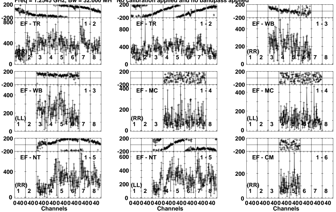
Lower frame: Micro Ampl Jy Top frame: Phas deg Vector averaged cross-power spectrum Several baselines displayed Timerange: 01/01:46:45 to 01/01:48:45
