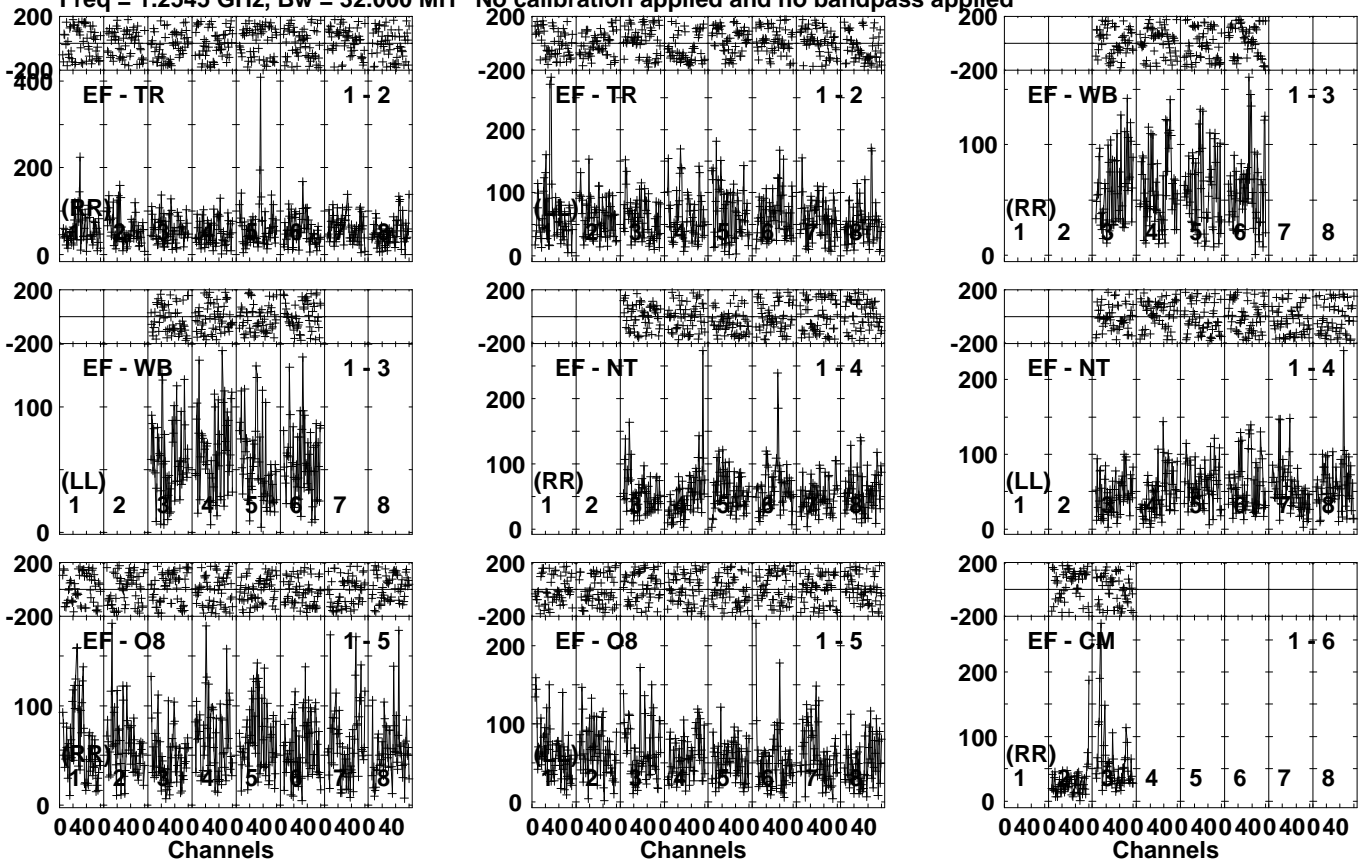
Lower frame: Micro Ampl Jy Top frame: Phas deg Vector averaged cross-power spectrum Several baselines displayed Timerange: 01/01:45:51 to 01/01:51:29
