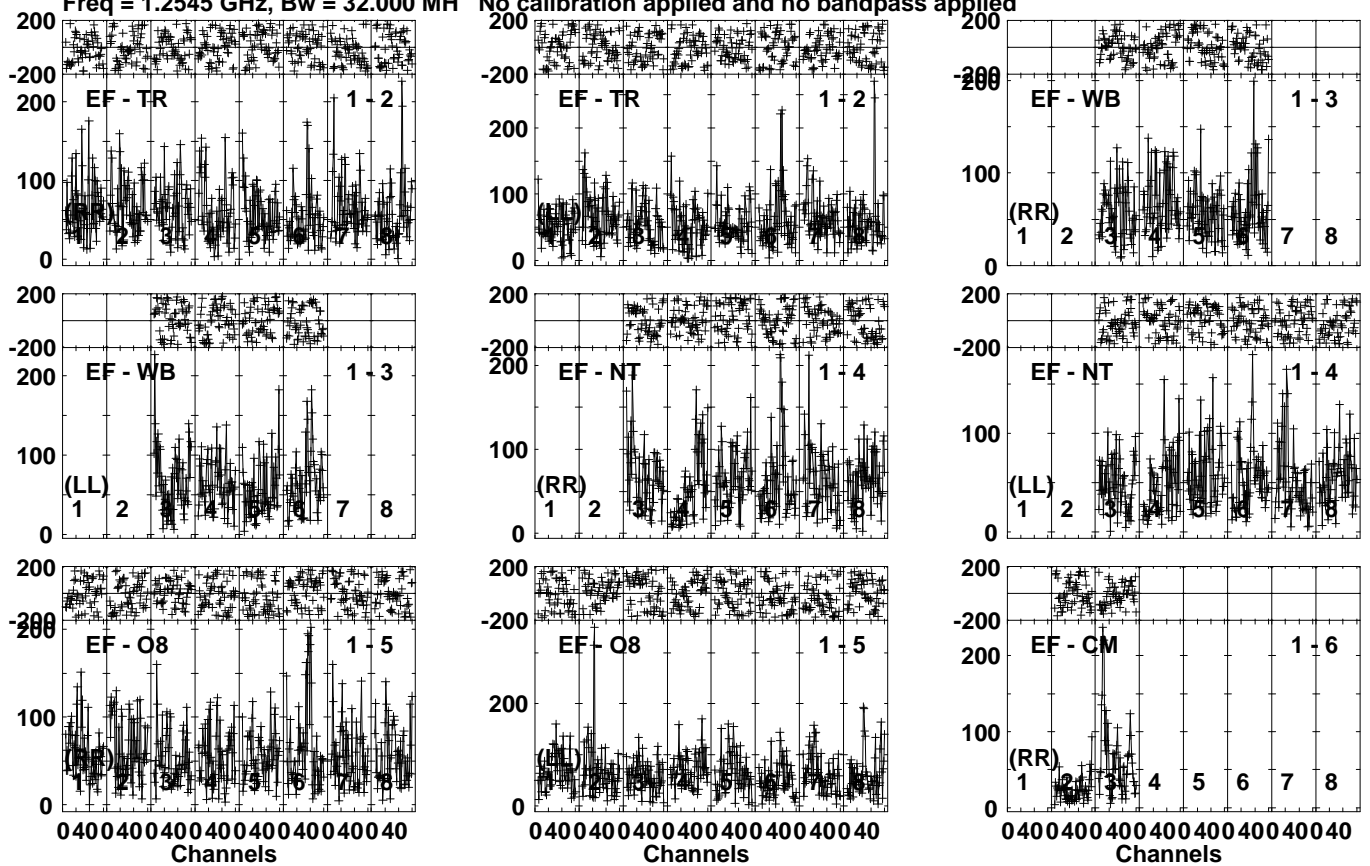
Lower frame: Micro Ampl Jy Top frame: Phas deg Vector averaged cross-power spectrum Several baselines displayed Timerange: 01/05:29:24 to 01/05:35:02
