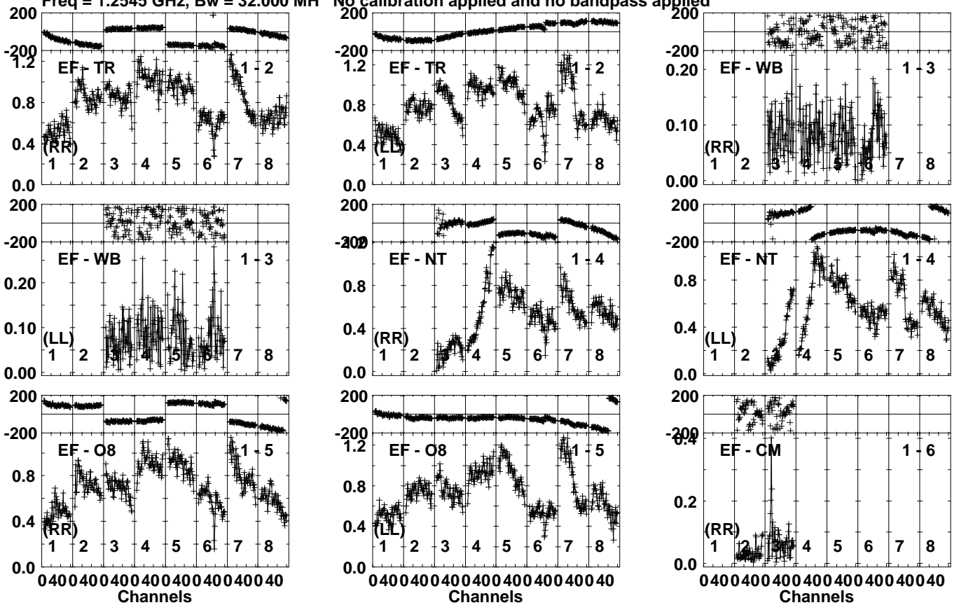
Lower frame: Milli Ampl Jy Top frame: Phas deg Vector averaged cross-power spectrum Several baselines displayed Timerange: 01/03:08:07 to 01/03:11:57
