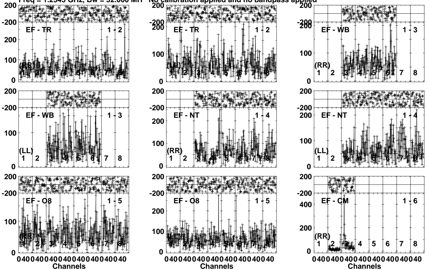
Lower frame: Micro Ampl Jy Top frame: Phas deg Vector averaged cross-power spectrum Several baselines displayed Timerange: 01/03:37:33 to 01/03:43:11
