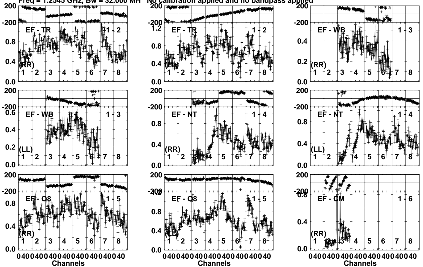
Lower frame: Milli Ampl Jy Top frame: Phas deg Vector averaged cross-power spectrum Several baselines displayed Timerange: 01/05:35:45 to 01/05:37:13
