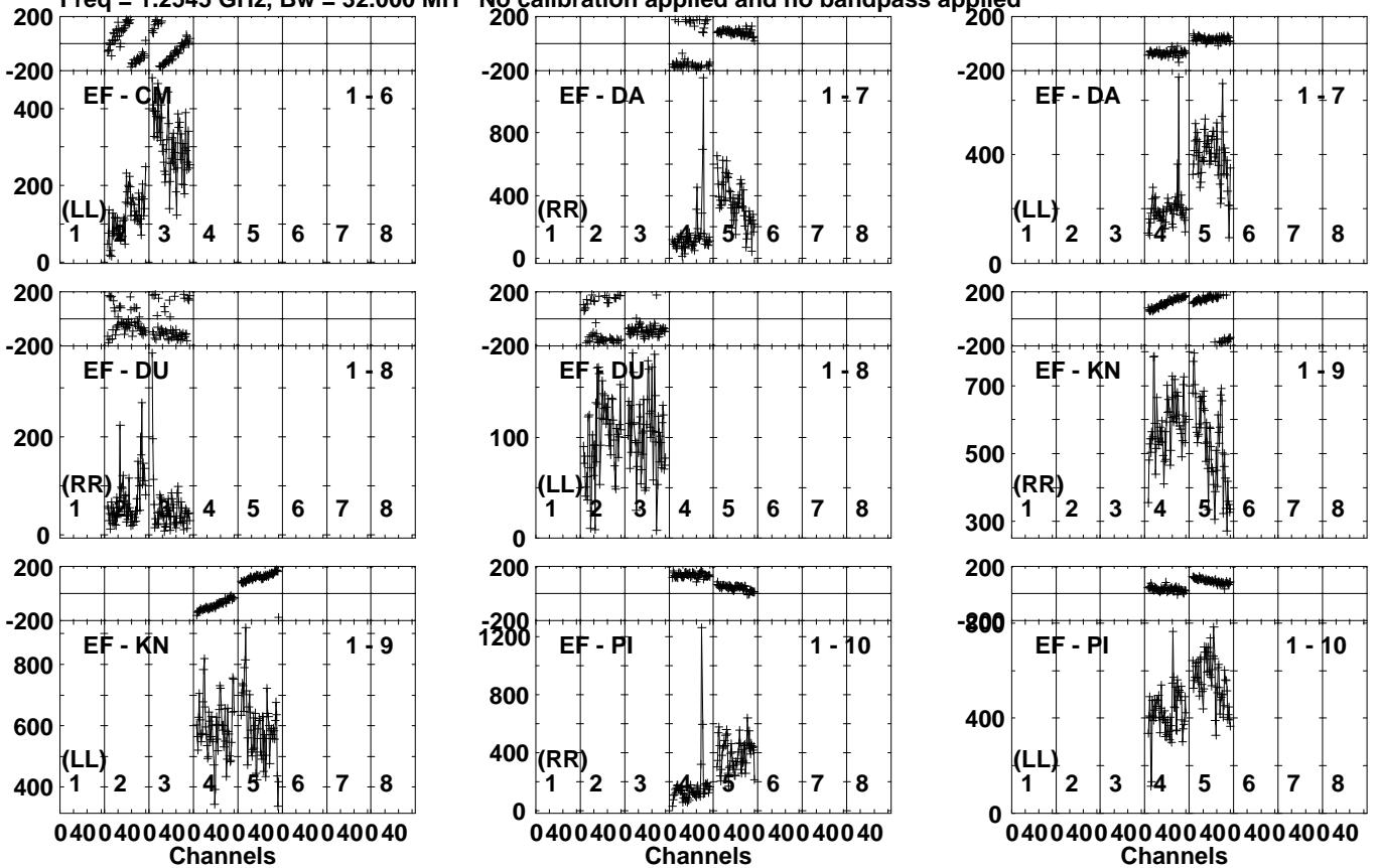
Lower frame: Micro Ampl Jy Top frame: Phas deg Vector averaged cross-power spectrum Several baselines displayed Timerange: 01/01:21:00 to 01/01:22:28
