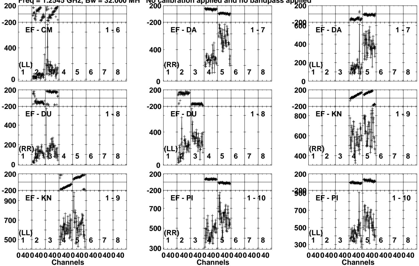
Lower frame: Micro Ampl Jy Top frame: Phas deg Vector averaged cross-power spectrum Several baselines displayed Timerange: 01/03:49:51 to 01/03:51:19
