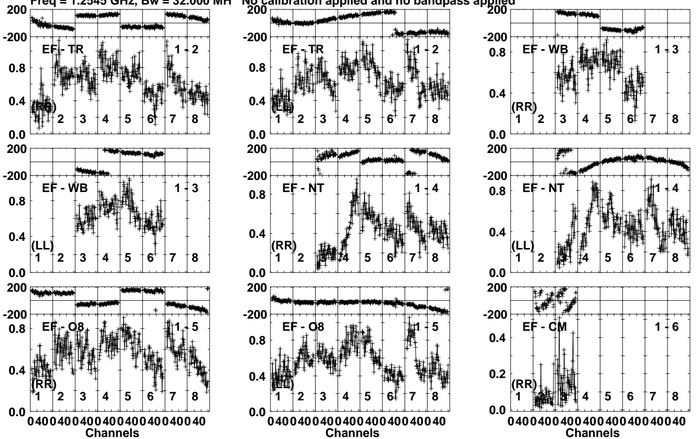
Lower frame: Milli Ampl Jy Top frame: Phas deg Vector averaged cross-power spectrum Several baselines displayed Timerange: 01/00:51:47 to 01/00:53:15
