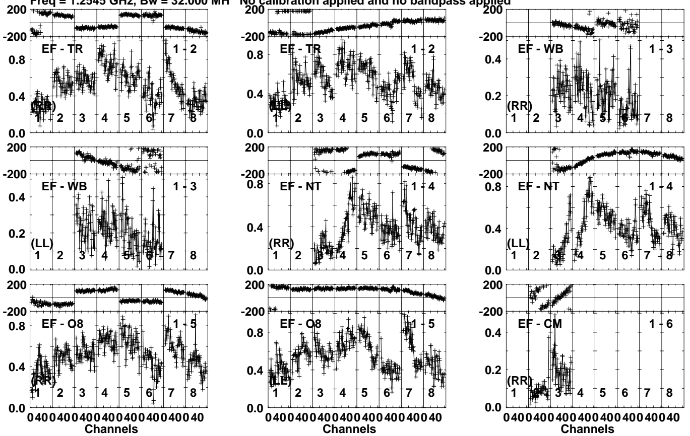
Lower frame: Milli Ampl Jy Top frame: Phas deg Vector averaged cross-power spectrum Several baselines displayed Timerange: 01/00:14:07 to 01/00:16:07
