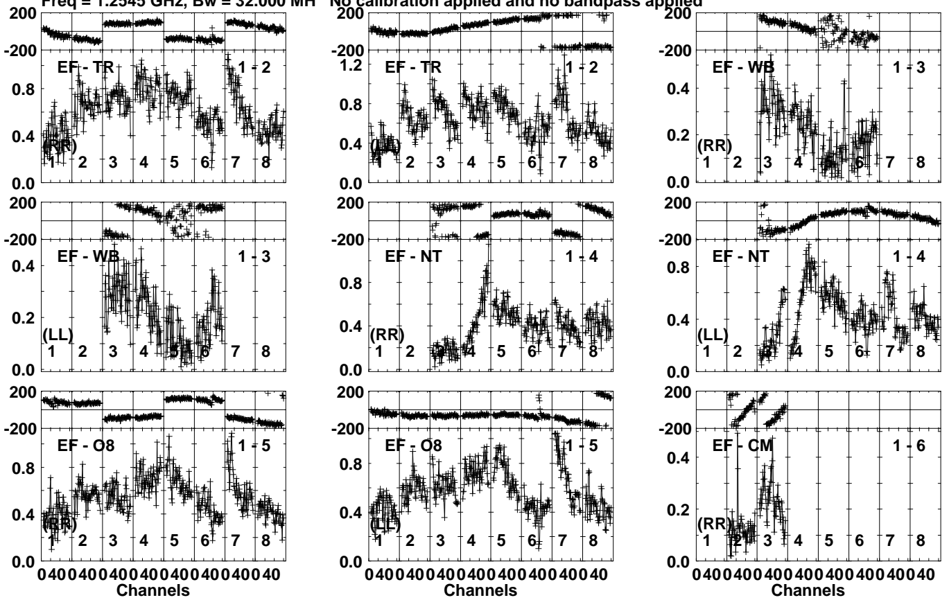
Lower frame: Milli Ampl Jy Top frame: Phas deg Vector averaged cross-power spectrum Several baselines displayed Timerange: 01/01:07:24 to 01/01:08:52
