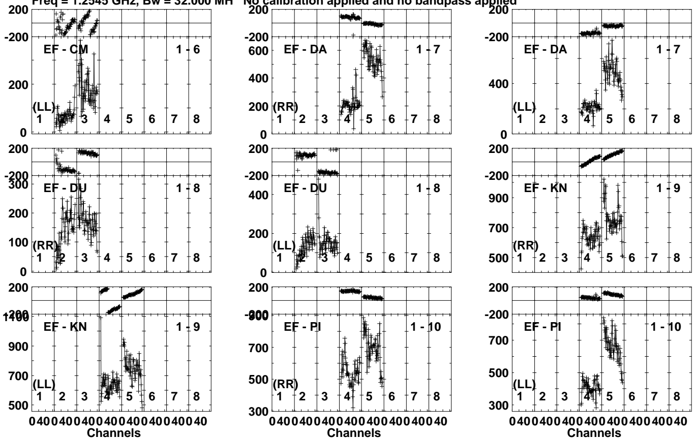
Lower frame: Micro Ampl Jy Top frame: Phas deg Vector averaged cross-power spectrum Several baselines displayed Timerange: 01/04:22:47 to 01/04:26:37
