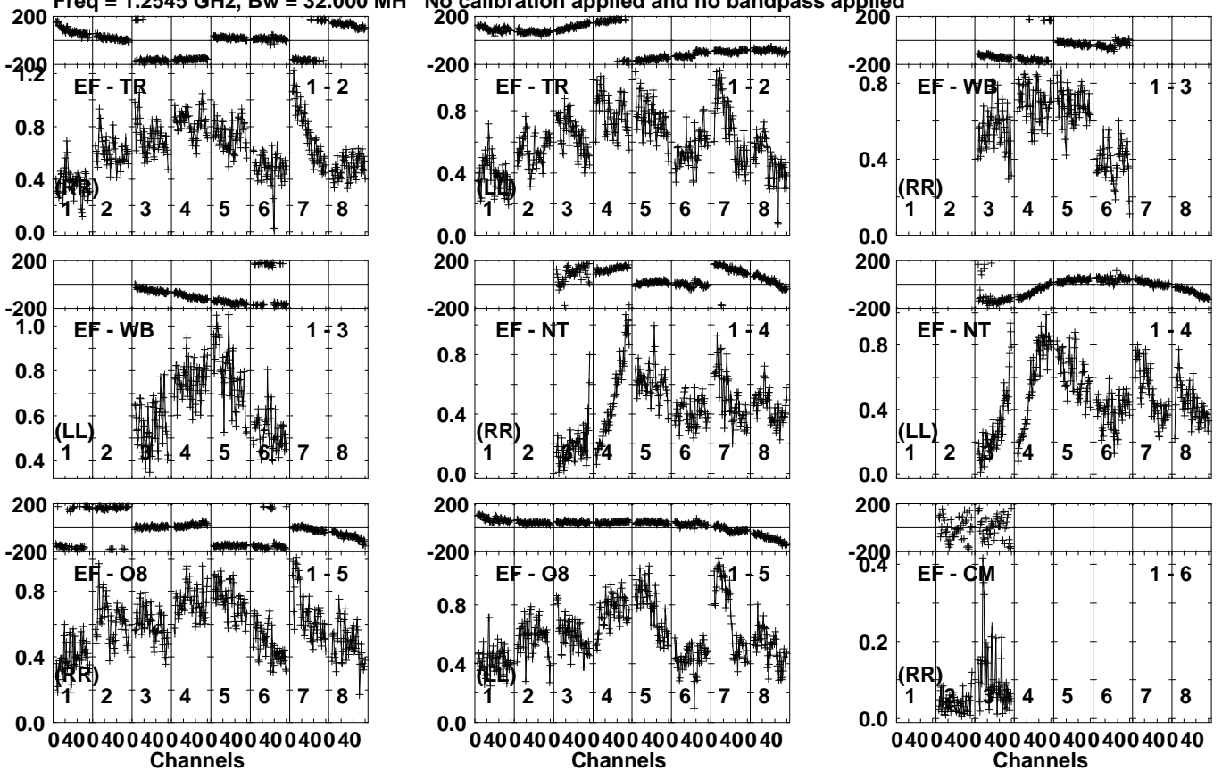
Lower frame: Milli Ampl Jy Top frame: Phas deg Vector averaged cross-power spectrum Several baselines displayed Timerange: 01/02:35:16 to 01/02:36:44
