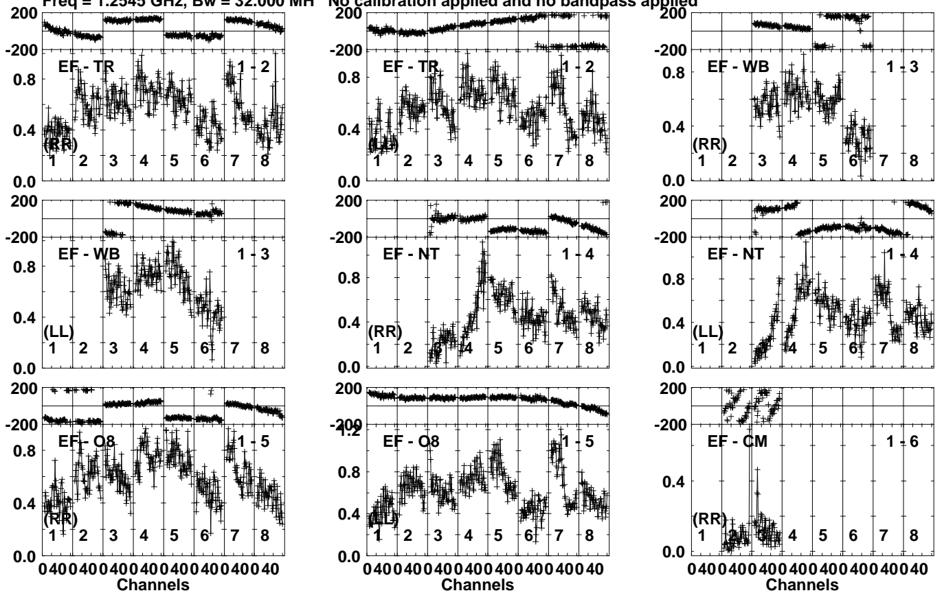
Lower frame: Milli Ampl Jy Top frame: Phas deg Vector averaged cross-power spectrum Several baselines displayed Timerange: 01/03:49:51 to 01/03:51:19
