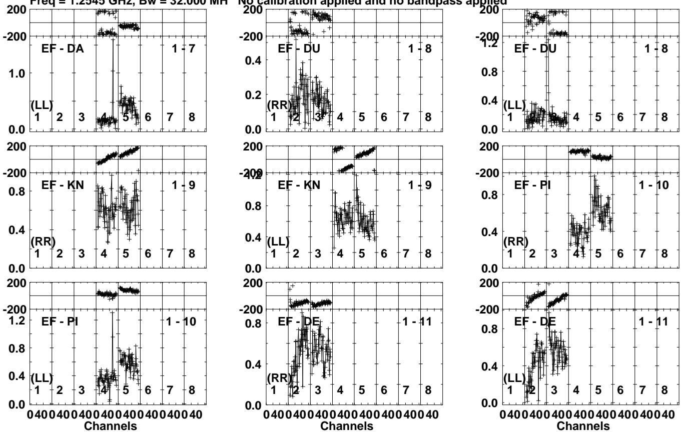
Lower frame: Milli Ampl Jy Top frame: Phas deg Vector averaged cross-power spectrum Several baselines displayed Timerange: 01/04:26:40 to 01/04:28:30
