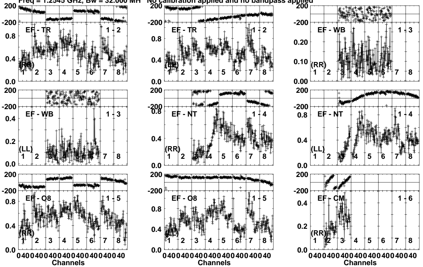
Lower frame: Milli Ampl Jy Top frame: Phas deg Vector averaged cross-power spectrum Several baselines displayed Timerange: 01/00:22:33 to 01/00:24:01
