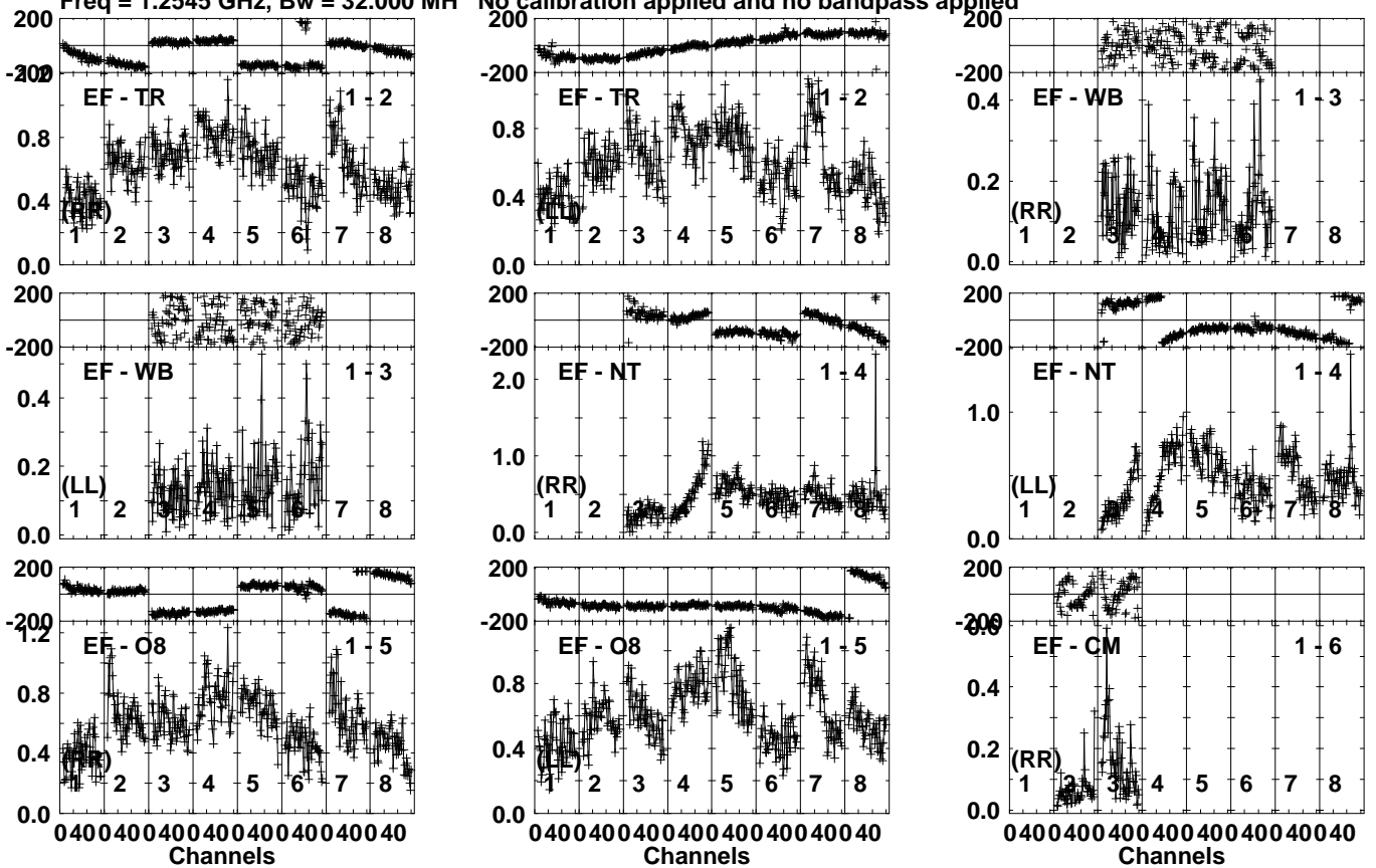
Lower frame: Milli Ampl Jy Top frame: Phas deg Vector averaged cross-power spectrum Several baselines displayed Timerange: 01/03:20:21 to 01/03:21:49
