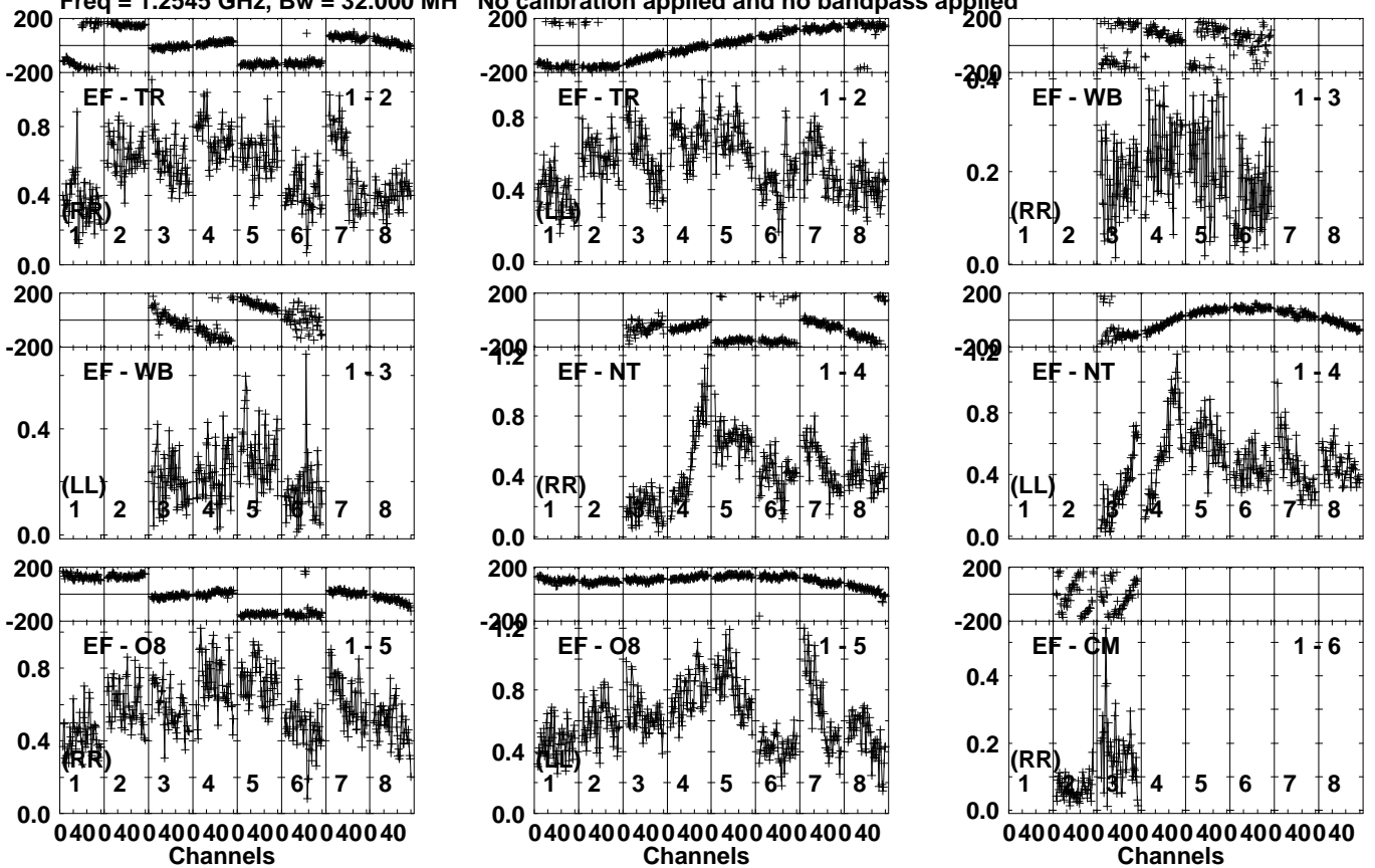
Lower frame: Milli Ampl Jy Top frame: Phas deg Vector averaged cross-power spectrum Several baselines displayed Timerange: 01/04:57:53 to 01/04:59:53
