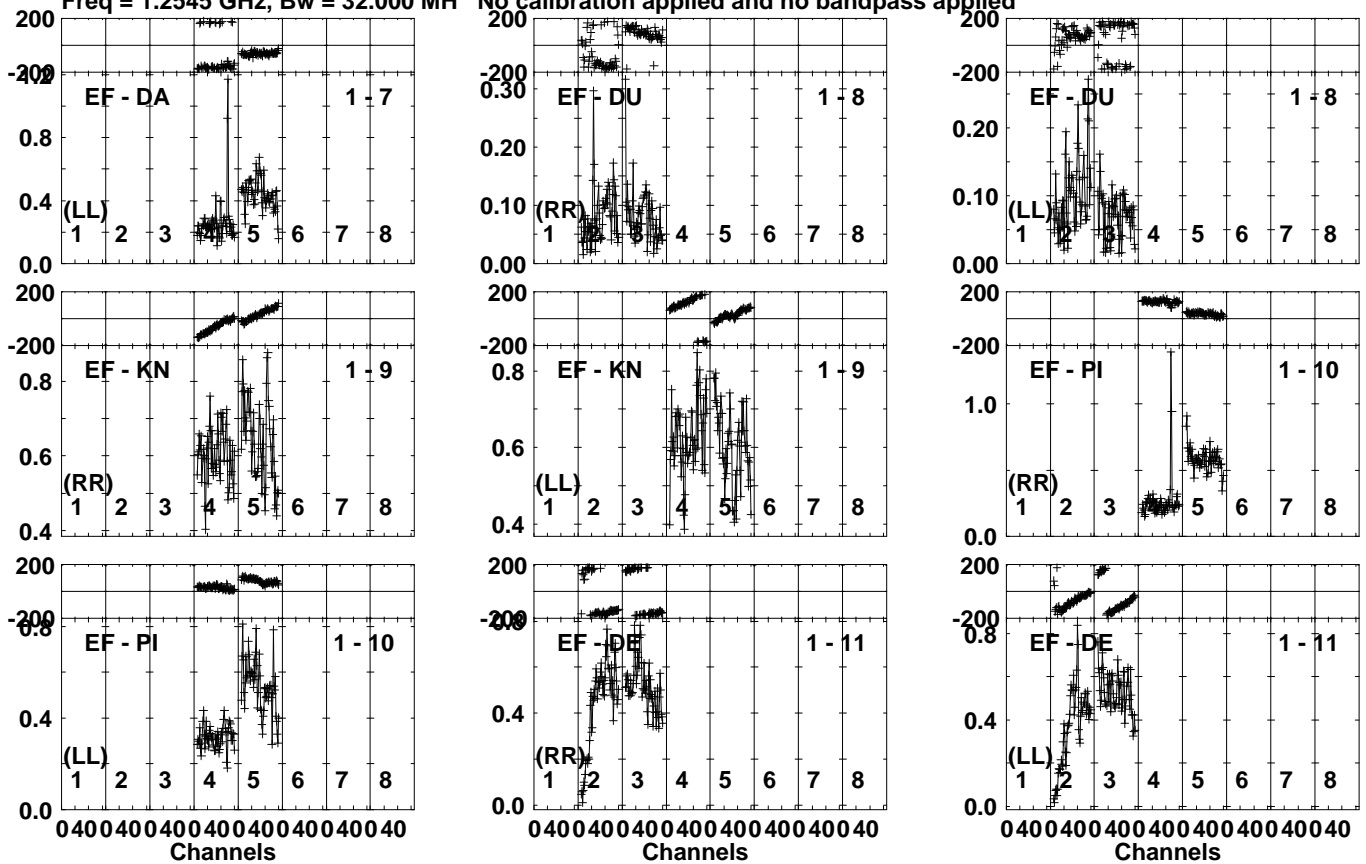
Lower frame: Milli Ampl Jy Top frame: Phas deg Vector averaged cross-power spectrum Several baselines displayed Timerange: 01/04:21:17 to 01/04:22:45
