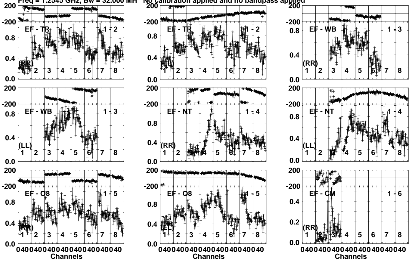
Lower frame: Milli Ampl Jy Top frame: Phas deg Vector averaged cross-power spectrum Several baselines displayed Timerange: 01/02:13:07 to 01/02:15:07
