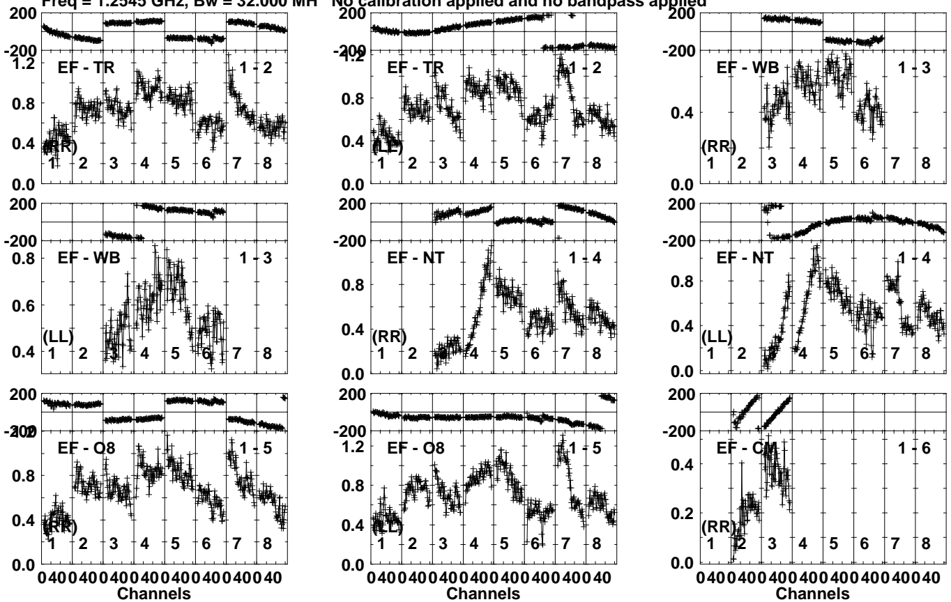
Lower frame: Milli Ampl Jy Top frame: Phas deg Vector averaged cross-power spectrum Several baselines displayed Timerange: 01/01:16:37 to 01/01:20:05
