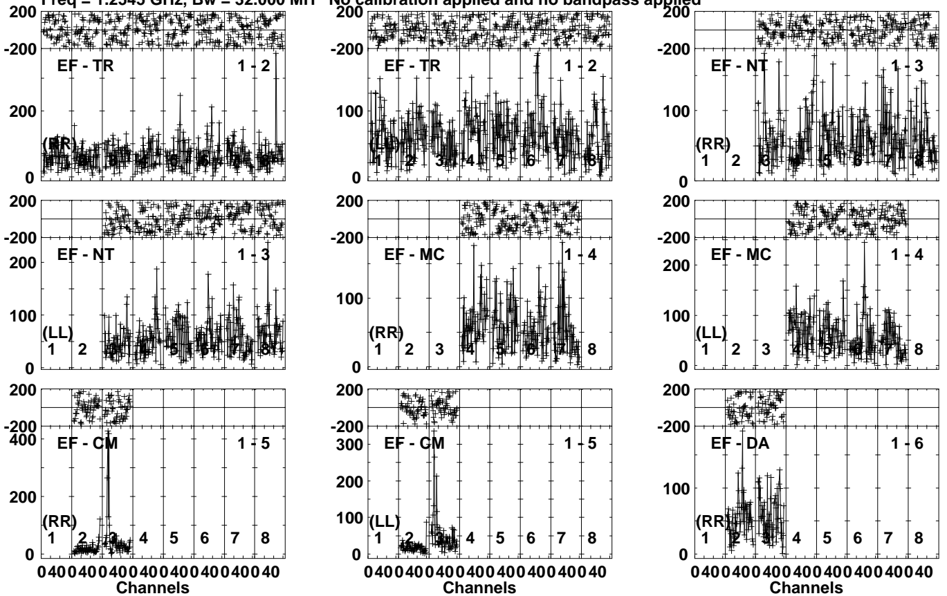
Lower frame: Micro Ampl Jy Top frame: Phas deg Vector averaged cross-power spectrum Several baselines displayed Timerange: 00/04:07:52 to 00/04:13:32
