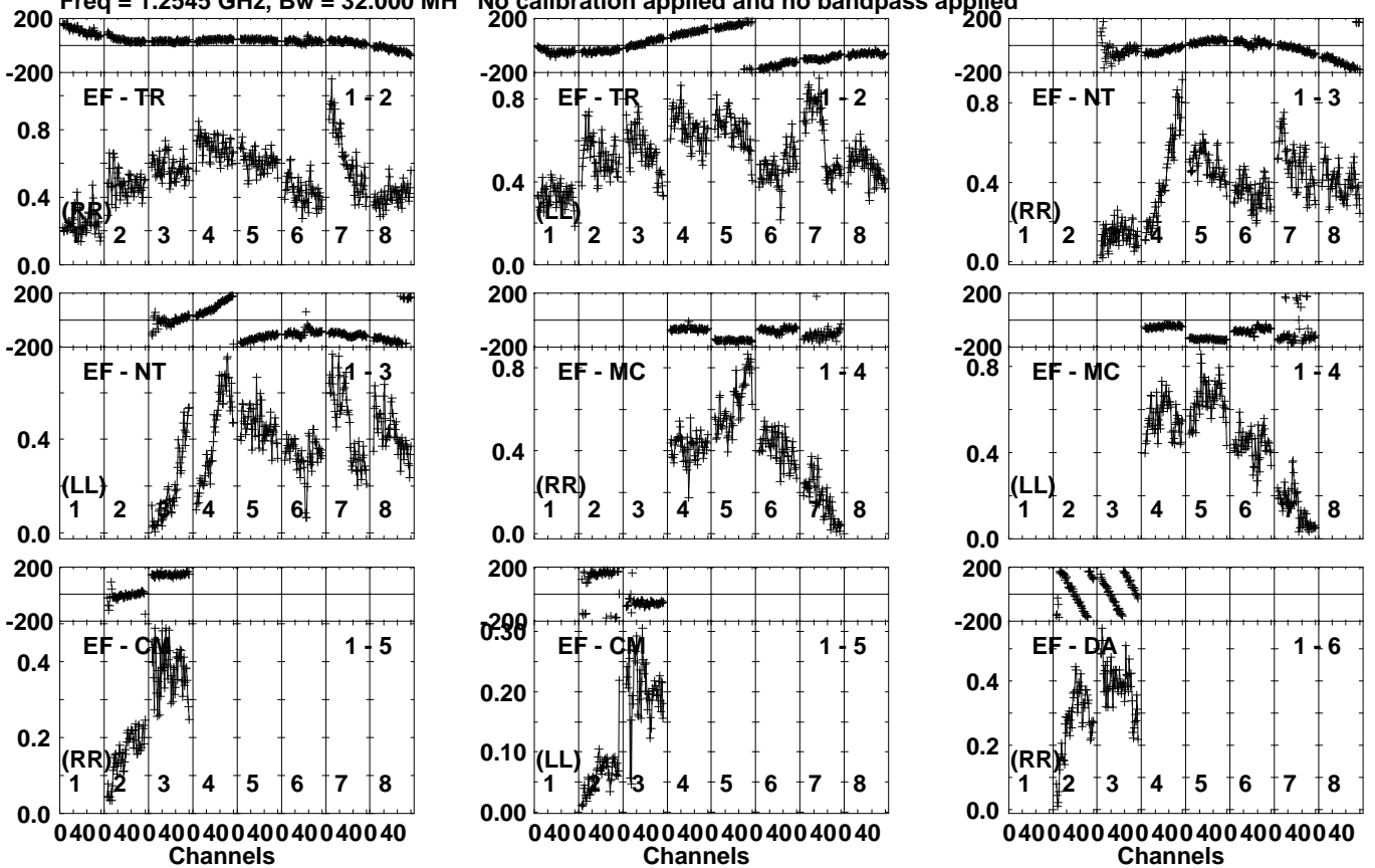
Lower frame: Milli Ampl Jy Top frame: Phas deg Vector averaged cross-power spectrum Several baselines displayed Timerange: 00/01:47:42 to 00/01:51:08
