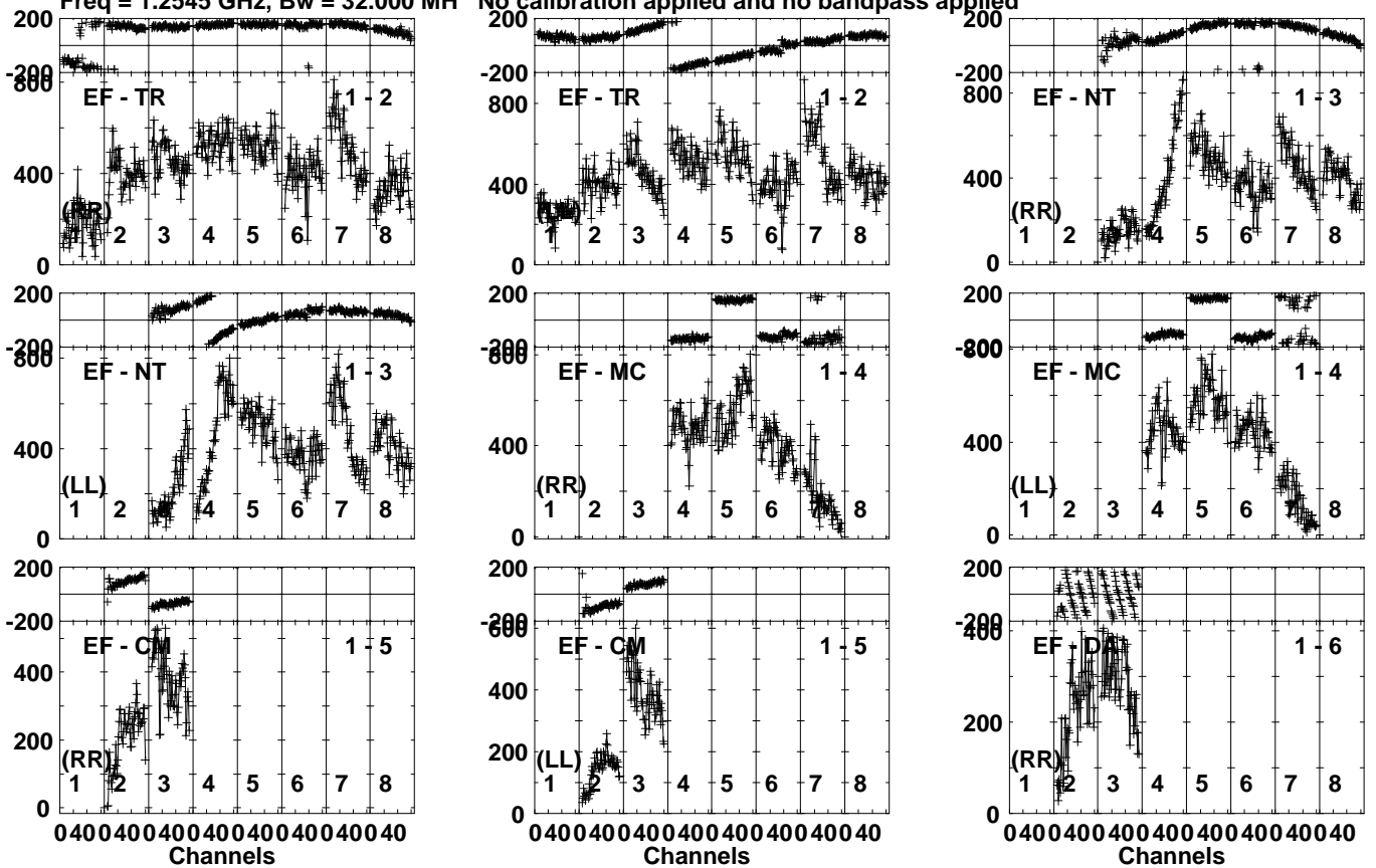
Lower frame: Micro Ampl Jy Top frame: Phas deg Vector averaged cross-power spectrum Several baselines displayed Timerange: 00/03:29:20 to 00/03:32:46
