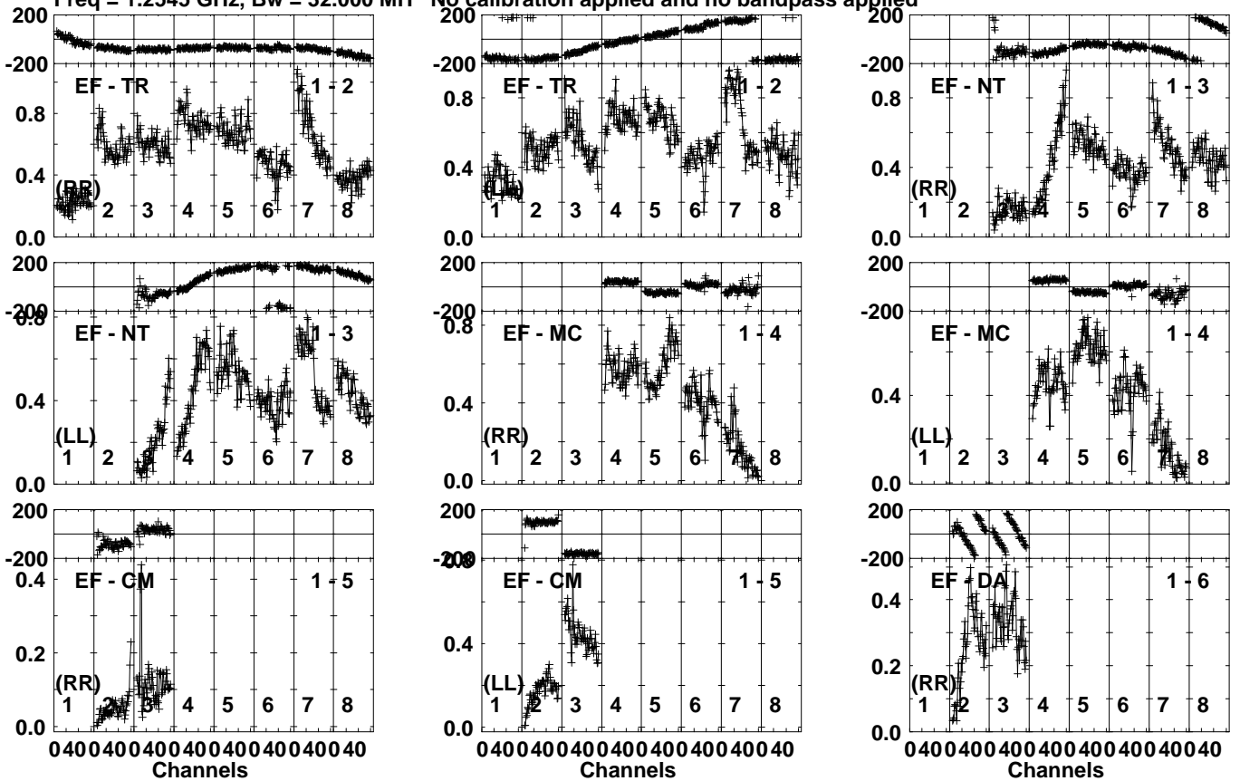
Lower frame: Milli Ampl Jy Top frame: Phas deg Vector averaged cross-power spectrum Several baselines displayed Timerange: 00/00:39:24 to 00/00:42:50
