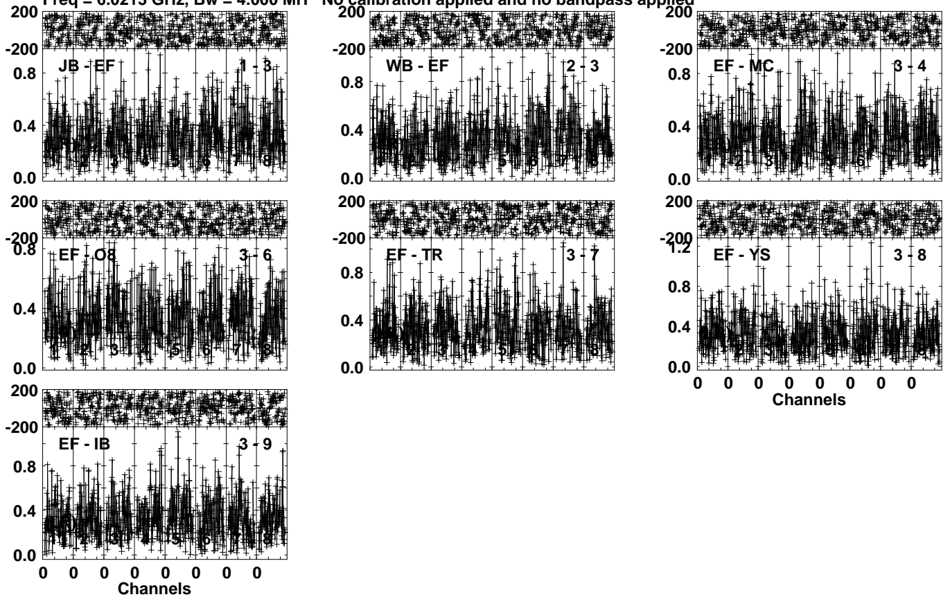
Lower frame: Milli Ampl Jy Top frame: Phas deg Vector averaged cross-power spectrum Several baselines displayed Timerange: 01/06:13:01 to 01/06:15:59
