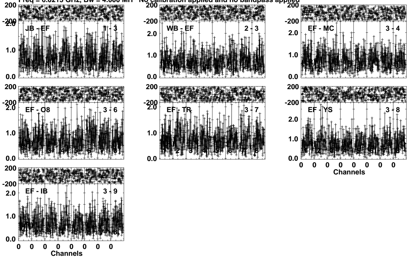
Lower frame: Milli Ampl Jy Top frame: Phas deg Vector averaged cross-power spectrum Several baselines displayed Timerange: 01/03:17:31 to 01/03:19:29
