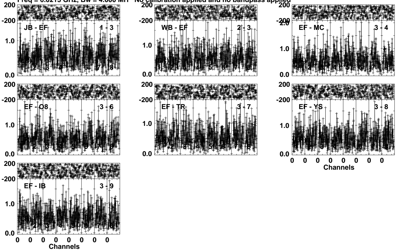
Lower frame: Milli Ampl Jy Top frame: Phas deg Vector averaged cross-power spectrum Several baselines displayed Timerange: 01/01:28:31 to 01/01:30:29
