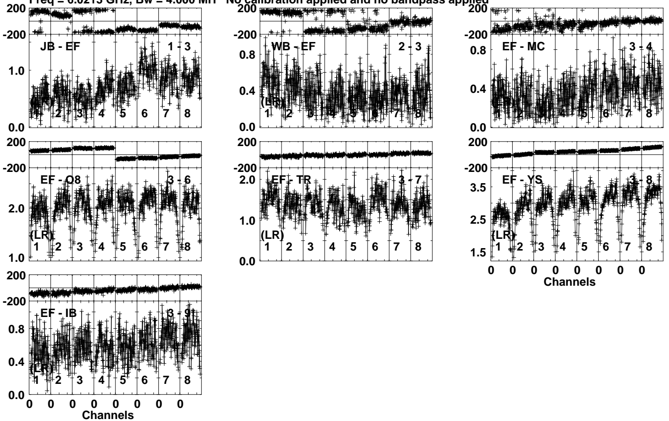
Lower frame: Milli Ampl Jy Top frame: Phas deg Vector averaged cross-power spectrum Several baselines displayed Timerange: 01/02:57:01 to 01/03:05:59
