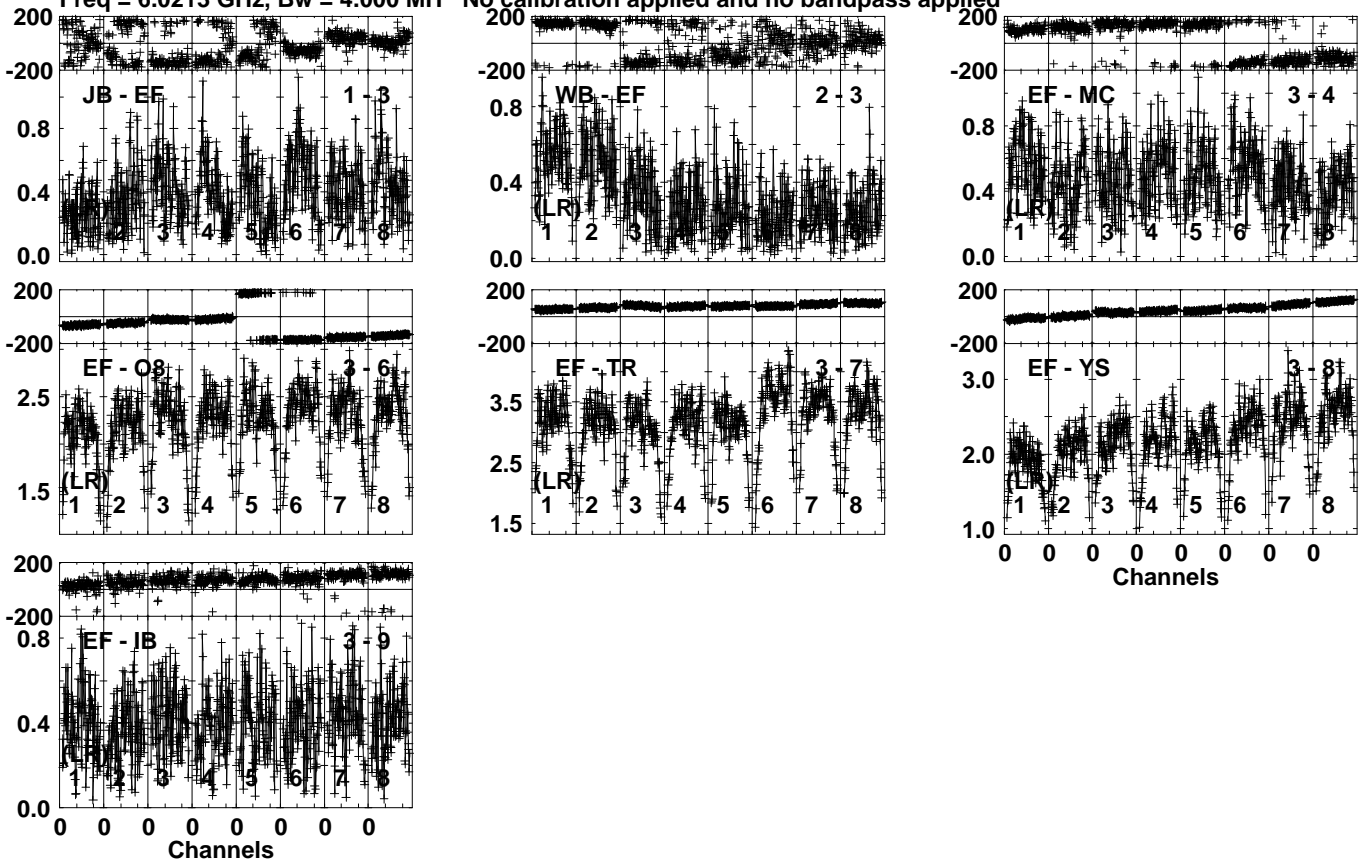
Lower frame: Milli Ampl Jy Top frame: Phas deg Vector averaged cross-power spectrum Several baselines displayed Timerange: 01/04:58:01 to 01/05:06:59
