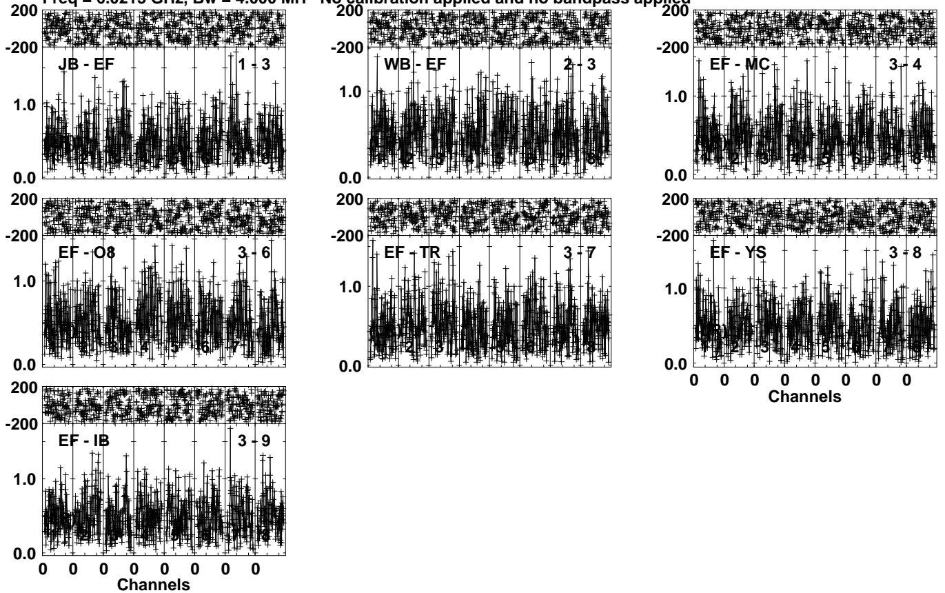
Lower frame: Milli Ampl Jy Top frame: Phas deg Vector averaged cross-power spectrum Several baselines displayed Timerange: 01/04:45:01 to 01/04:46:59
