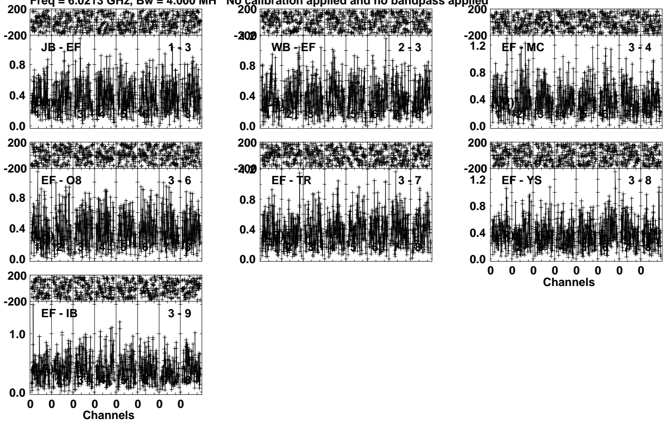
Lower frame: Milli Ampl Jy Top frame: Phas deg Vector averaged cross-power spectrum Several baselines displayed Timerange: 01/01:25:31 to 01/01:28:29
