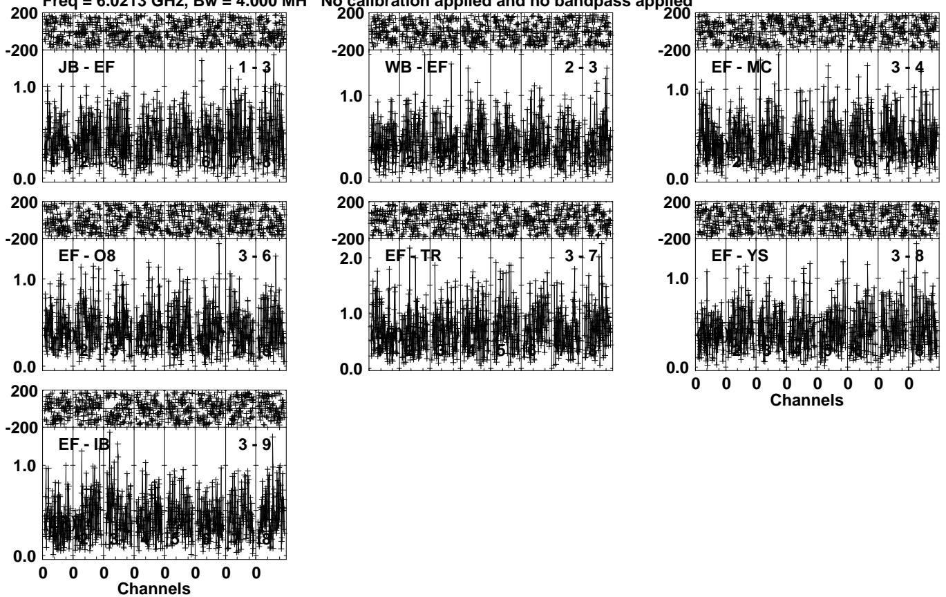
Lower frame: Milli Ampl Jy Top frame: Phas deg Vector averaged cross-power spectrum Several baselines displayed Timerange: 01/03:50:31 to 01/03:53:29
