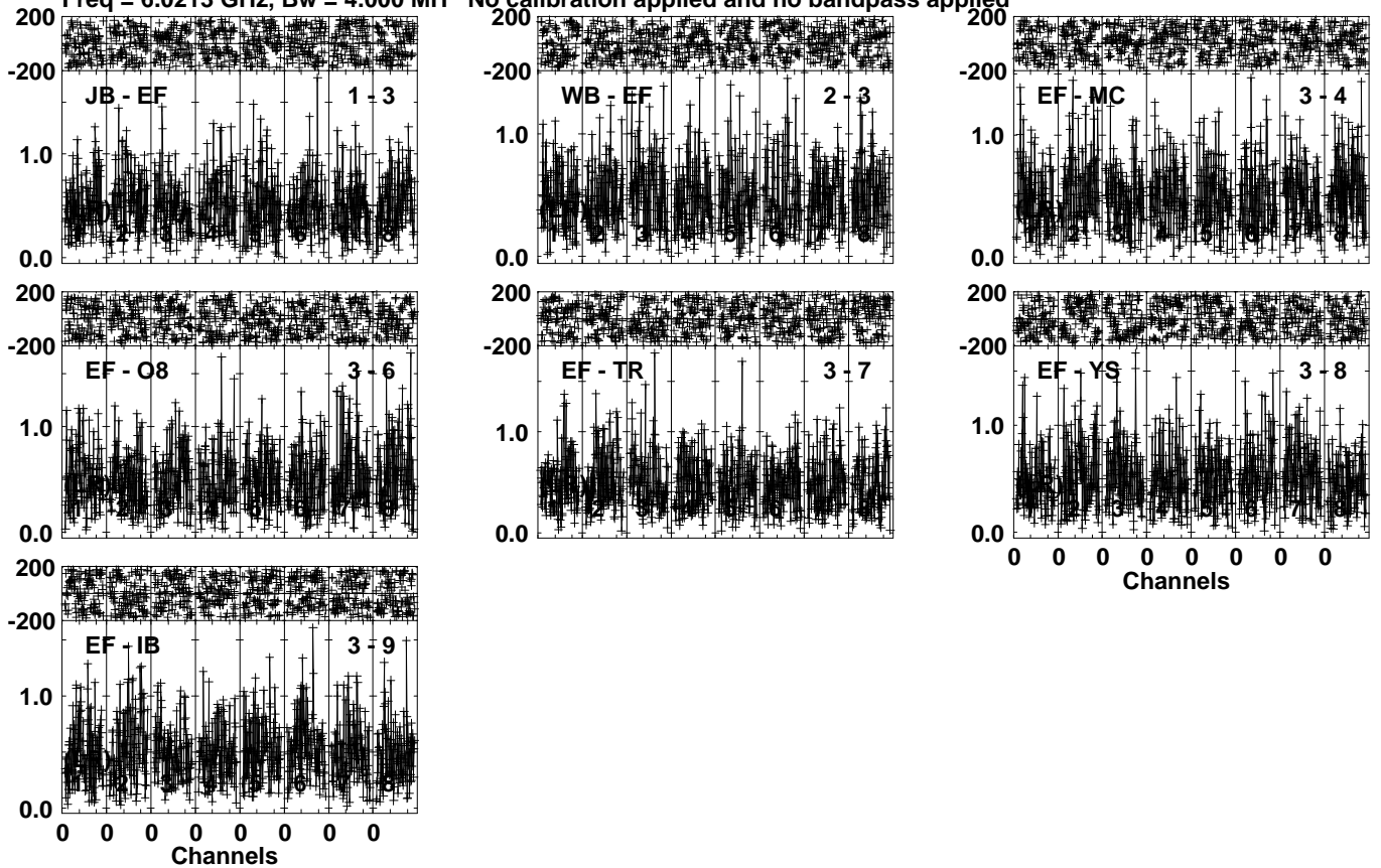
Lower frame: Milli Ampl Jy Top frame: Phas deg Vector averaged cross-power spectrum Several baselines displayed Timerange: 01/02:02:31 to 01/02:04:29
