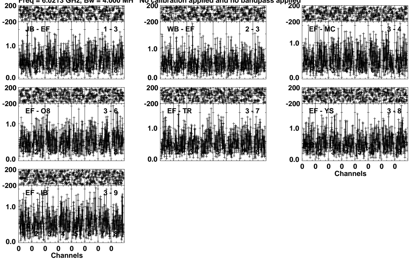
Lower frame: Milli Ampl Jy Top frame: Phas deg Vector averaged cross-power spectrum Several baselines displayed Timerange: 01/01:08:01 to 01/01:09:59
