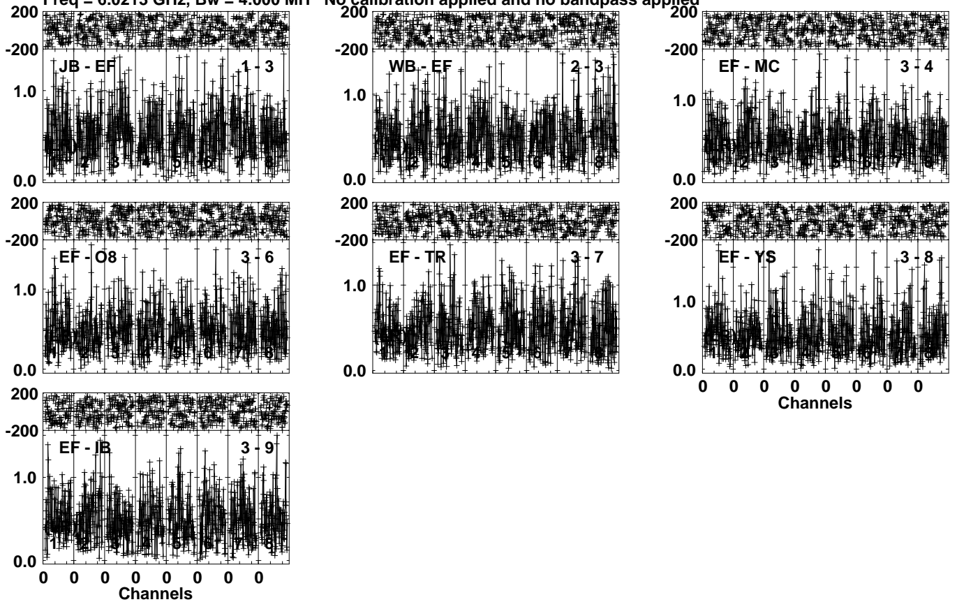
Lower frame: Milli Ampl Jy Top frame: Phas deg Vector averaged cross-power spectrum Several baselines displayed Timerange: 01/06:26:01 to 01/06:27:59
