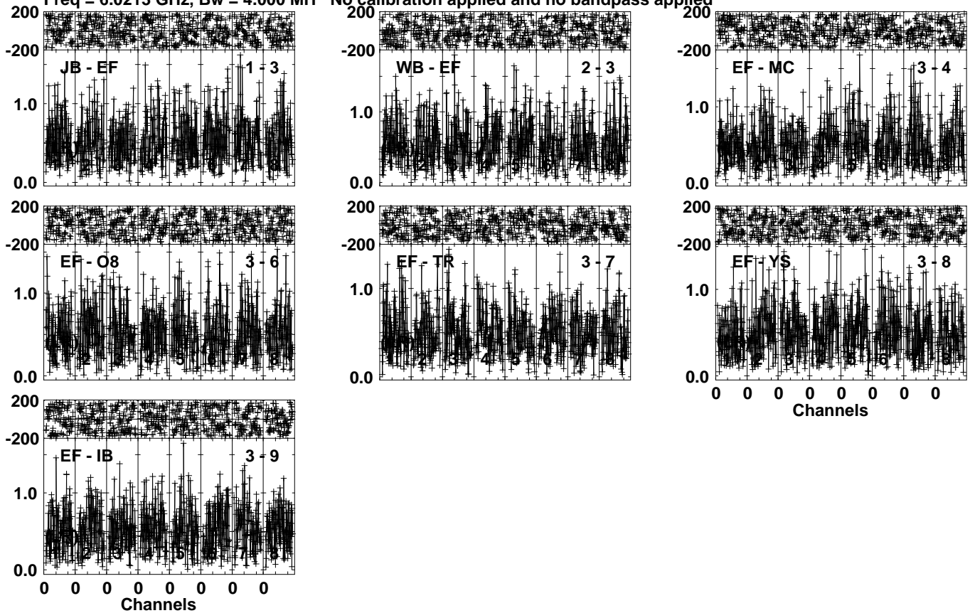
Lower frame: Milli Ampl Jy Top frame: Phas deg Vector averaged cross-power spectrum Several baselines displayed Timerange: 00/23:24:31 to 00/23:26:29
