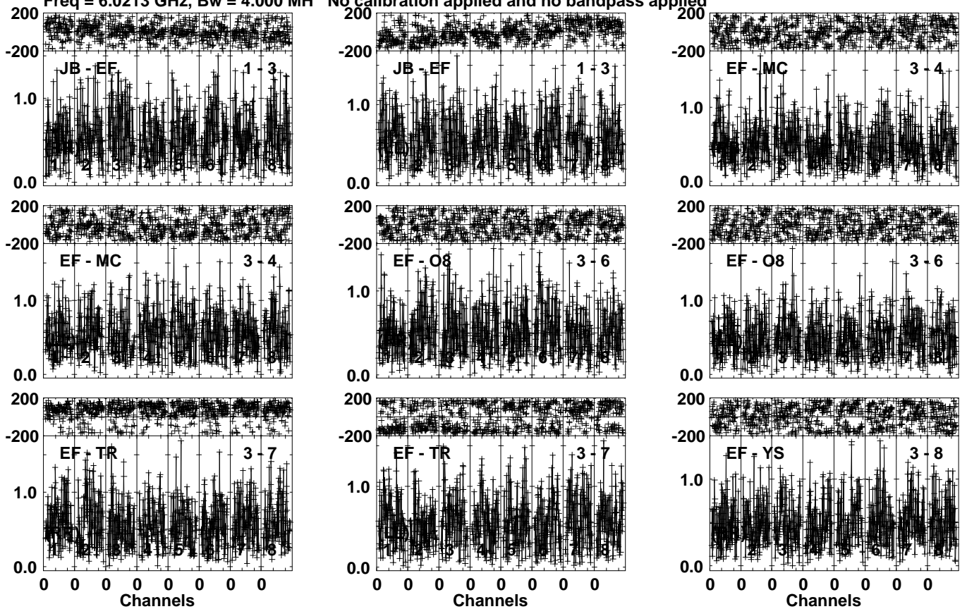
Lower frame: Milli Ampl Jy Top frame: Phas deg Vector averaged cross-power spectrum Several baselines displayed Timerange: 00/21:15:31 to 00/21:17:29
