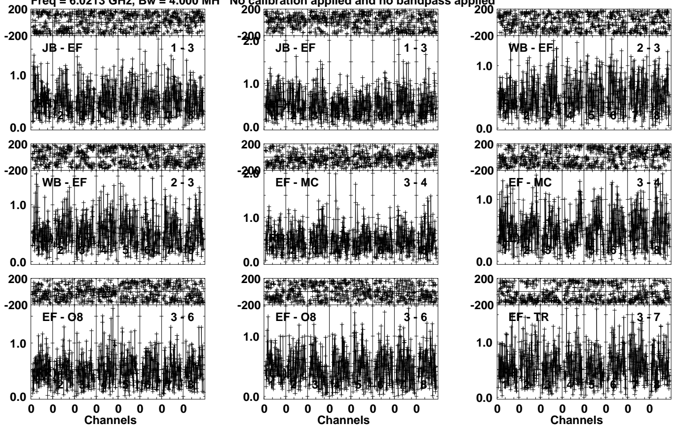
Lower frame: Milli Ampl Jy Top frame: Phas deg Vector averaged cross-power spectrum Several baselines displayed Timerange: 01/07:25:31 to 01/07:27:29
