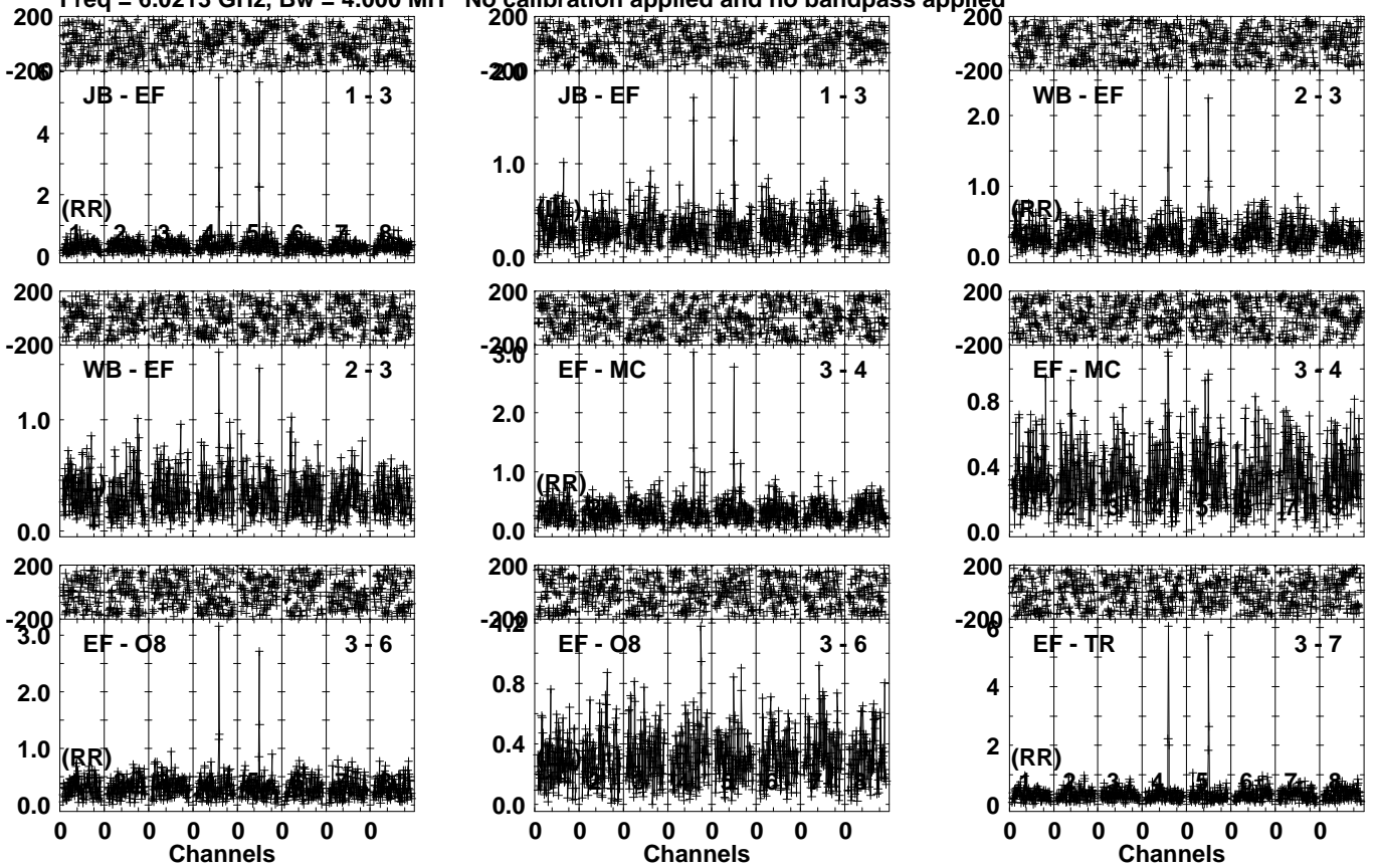
Lower frame: Milli Ampl Jy Top frame: Phas deg Vector averaged cross-power spectrum Several baselines displayed Timerange: 01/08:12:01 to 01/08:14:59
