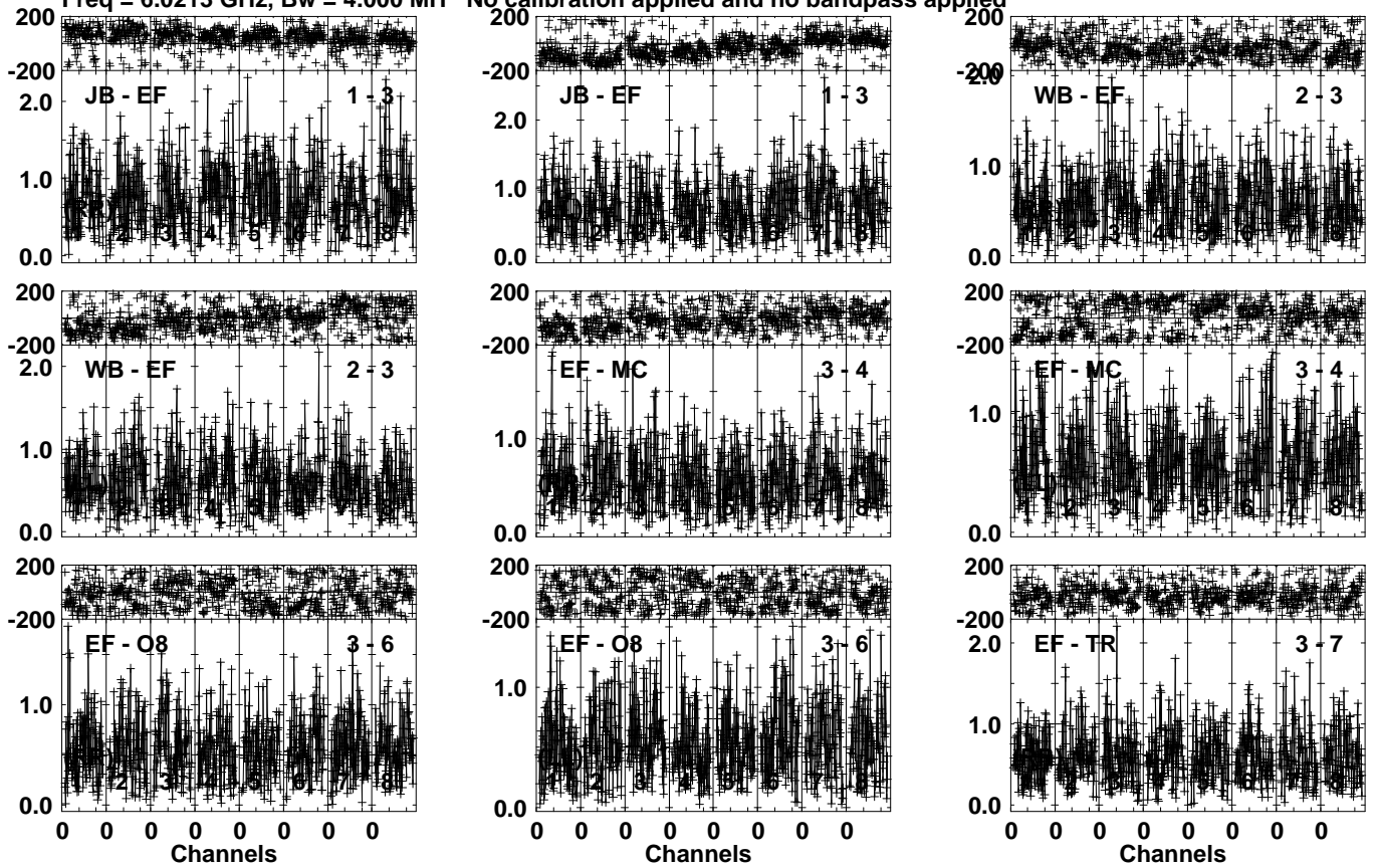
Lower frame: Milli Ampl Jy Top frame: Phas deg Vector averaged cross-power spectrum Several baselines displayed Timerange: 01/04:07:31 to 01/04:10:29
