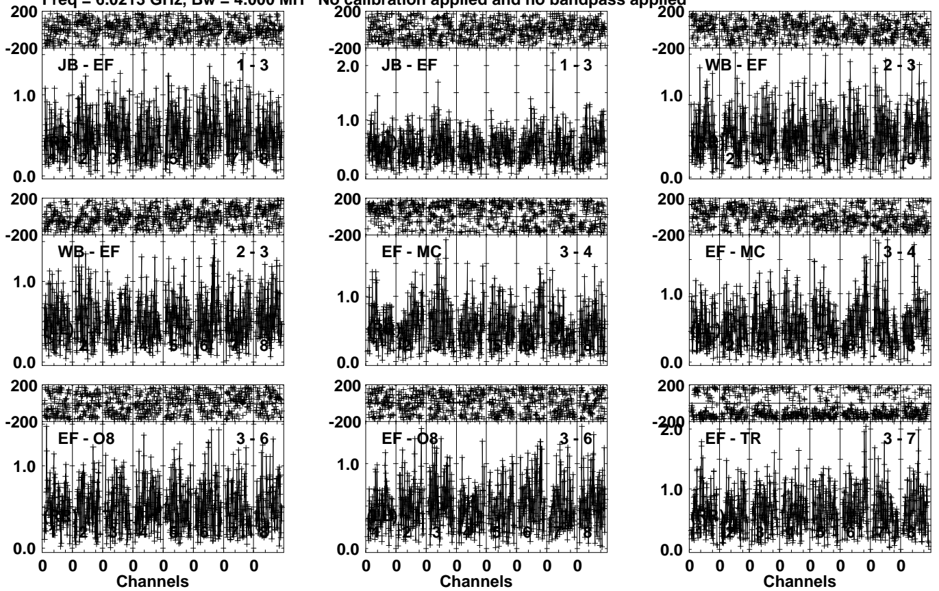
Lower frame: Milli Ampl Jy Top frame: Phas deg Vector averaged cross-power spectrum Several baselines displayed Timerange: 01/06:47:01 to 01/06:48:59
