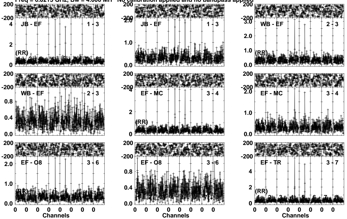
Lower frame: Milli Ampl Jy Top frame: Phas deg Vector averaged cross-power spectrum Several baselines displayed Timerange: 01/05:43:01 to 01/05:45:59
