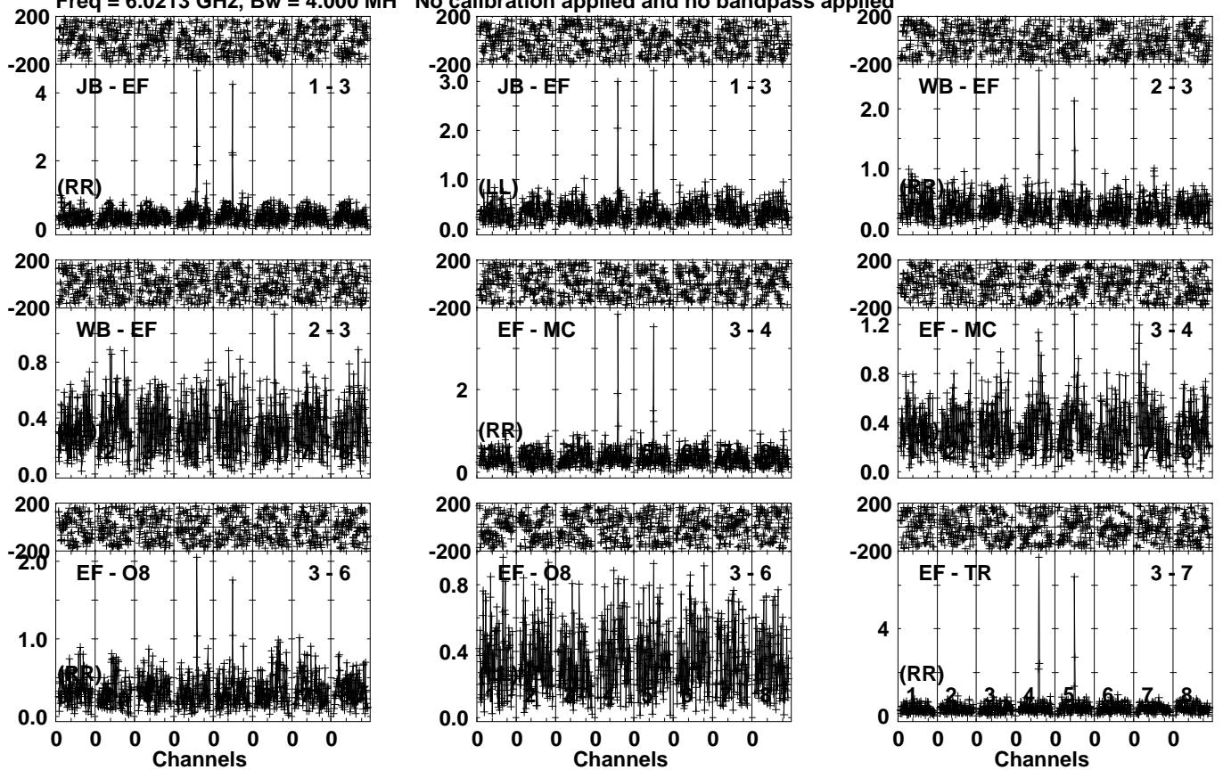
Lower frame: Milli Ampl Jy Top frame: Phas deg Vector averaged cross-power spectrum Several baselines displayed Timerange: 01/07:48:31 to 01/07:51:29
