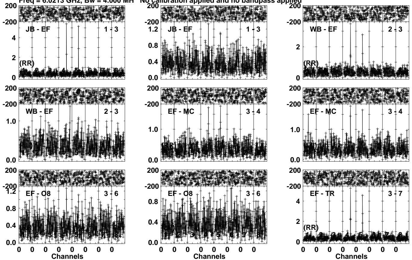
Lower frame: Milli Ampl Jy Top frame: Phas deg Vector averaged cross-power spectrum Several baselines displayed Timerange: 01/01:30:31 to 01/01:33:29
