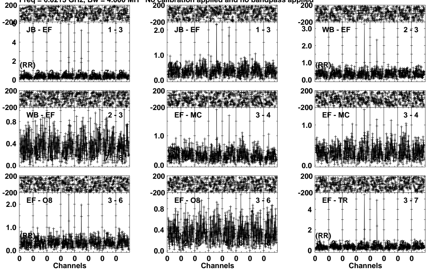
Lower frame: Milli Ampl Jy Top frame: Phas deg Vector averaged cross-power spectrum Several baselines displayed Timerange: 01/07:38:01 to 01/07:40:59
