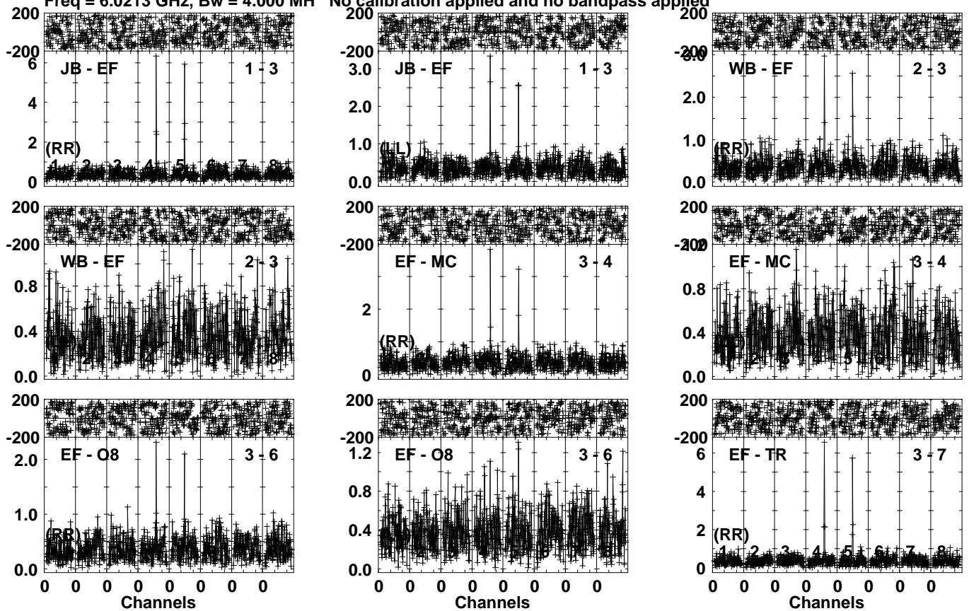
Lower frame: Milli Ampl Jy Top frame: Phas deg Vector averaged cross-power spectrum Several baselines displayed Timerange: 01/04:36:31 to 01/04:39:29
