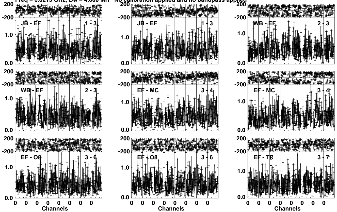
Lower frame: Milli Ampl Jy Top frame: Phas deg Vector averaged cross-power spectrum Several baselines displayed Timerange: 01/07:20:31 to 01/07:22:29
