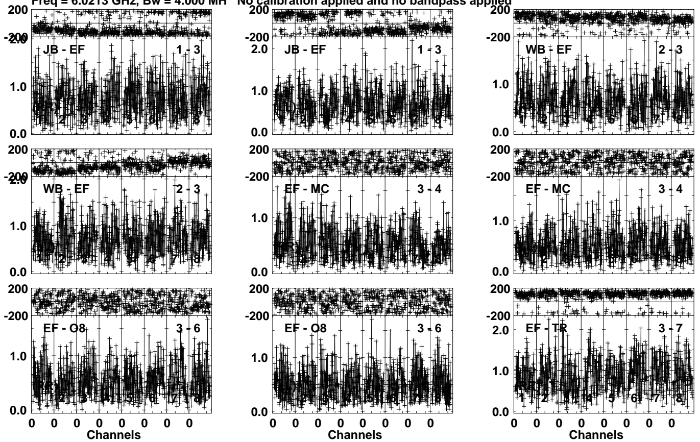
Lower frame: Milli Ampl Jy Top frame: Phas deg Vector averaged cross-power spectrum Several baselines displayed Timerange: 01/00:14:01 to 01/00:15:59
