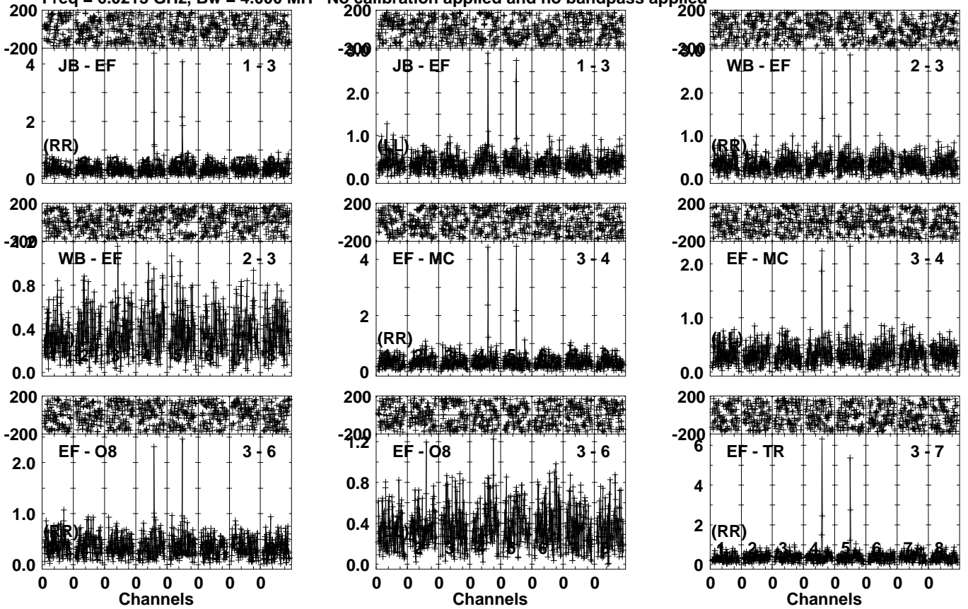
Lower frame: Milli Ampl Jy Top frame: Phas deg Vector averaged cross-power spectrum Several baselines displayed Timerange: 01/06:18:01 to 01/06:20:59
