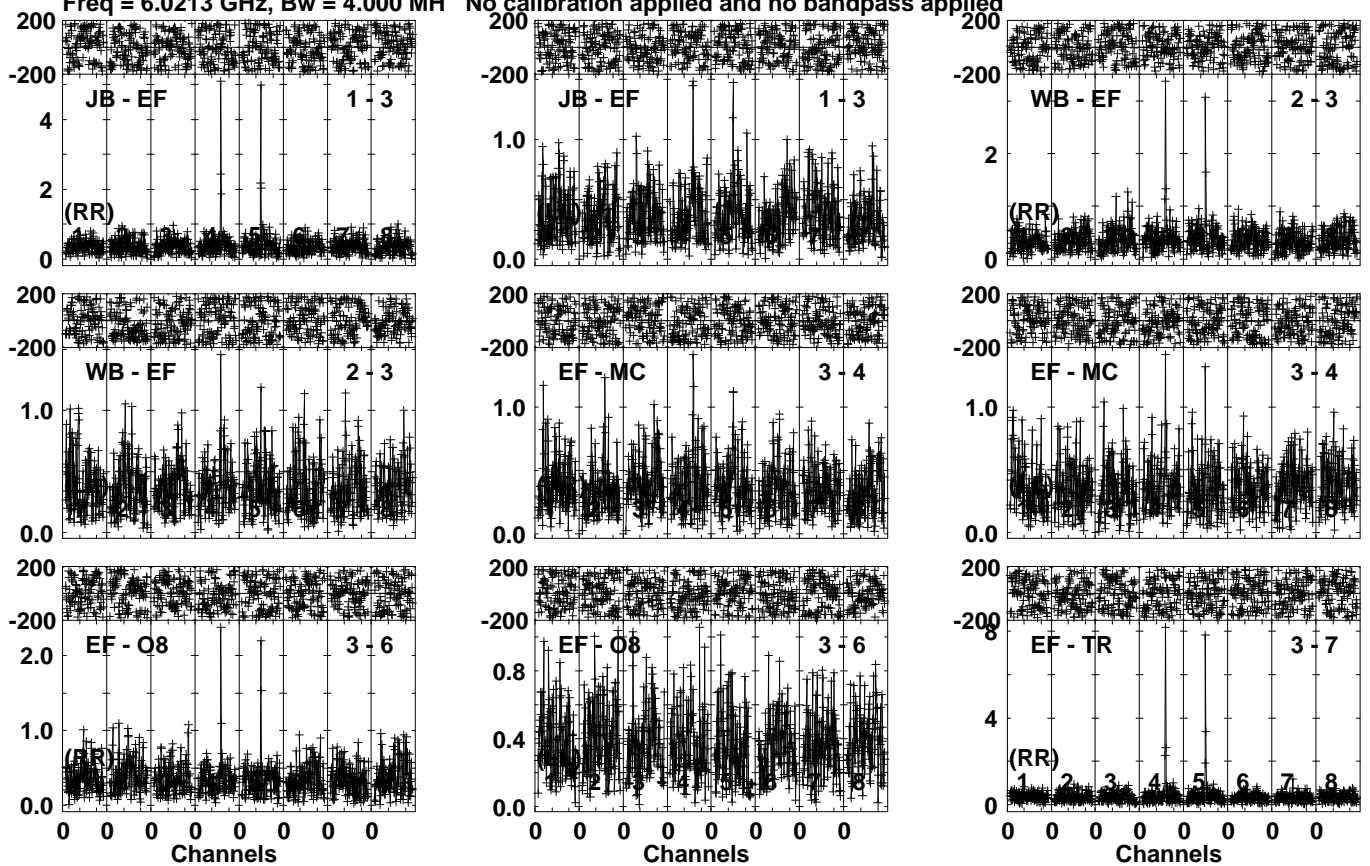
Lower frame: Milli Ampl Jy Top frame: Phas deg Vector averaged cross-power spectrum Several baselines displayed Timerange: 00/22:17:01 to 00/22:19:59
