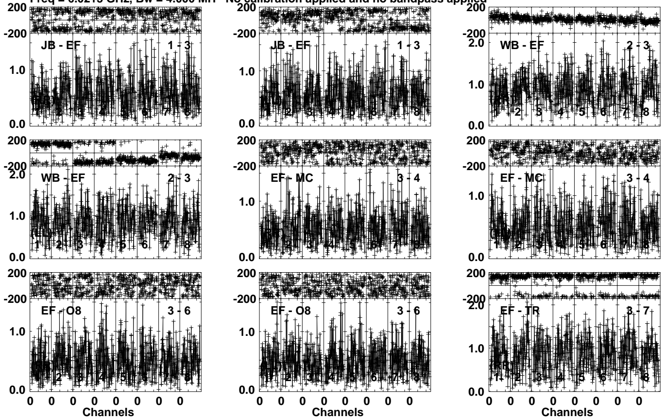
Lower frame: Milli Ampl Jy Top frame: Phas deg Vector averaged cross-power spectrum Several baselines displayed Timerange: 00/23:08:01 to 00/23:10:59
