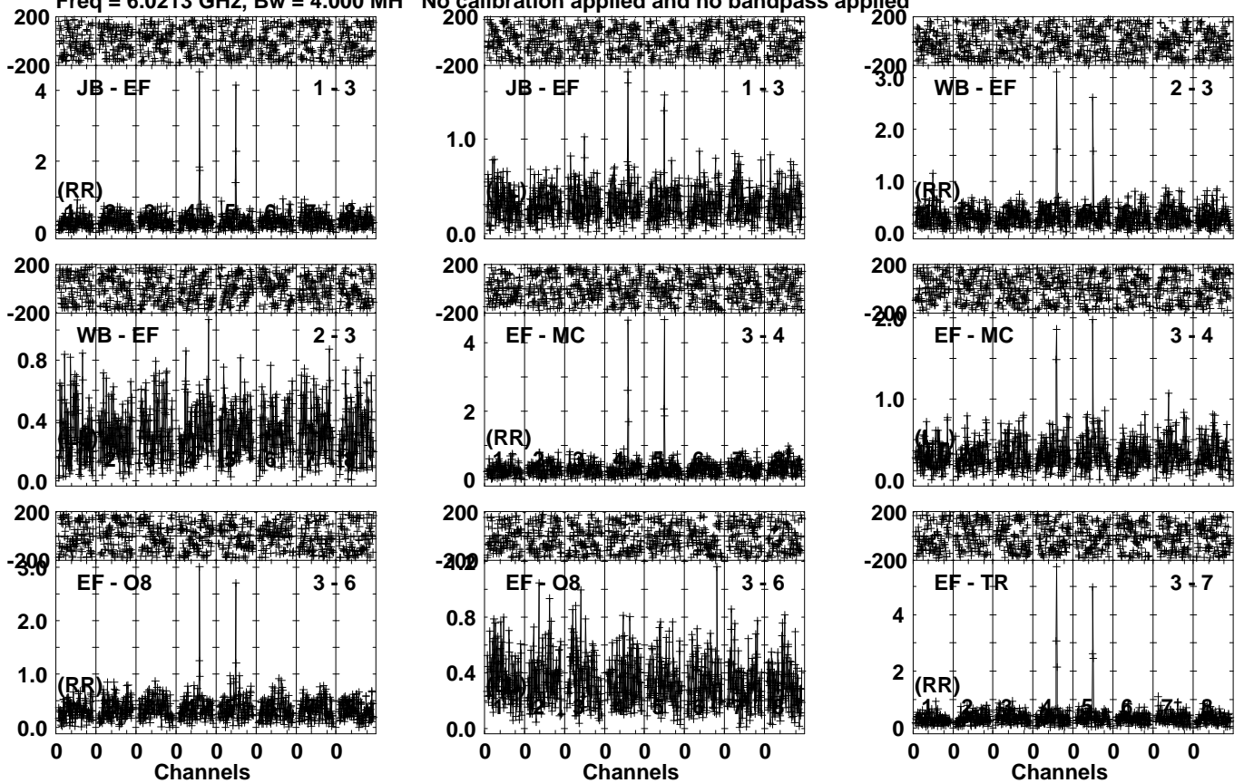
Lower frame: Milli Ampl Jy Top frame: Phas deg Vector averaged cross-power spectrum Several baselines displayed Timerange: 01/06:28:31 to 01/06:31:29
