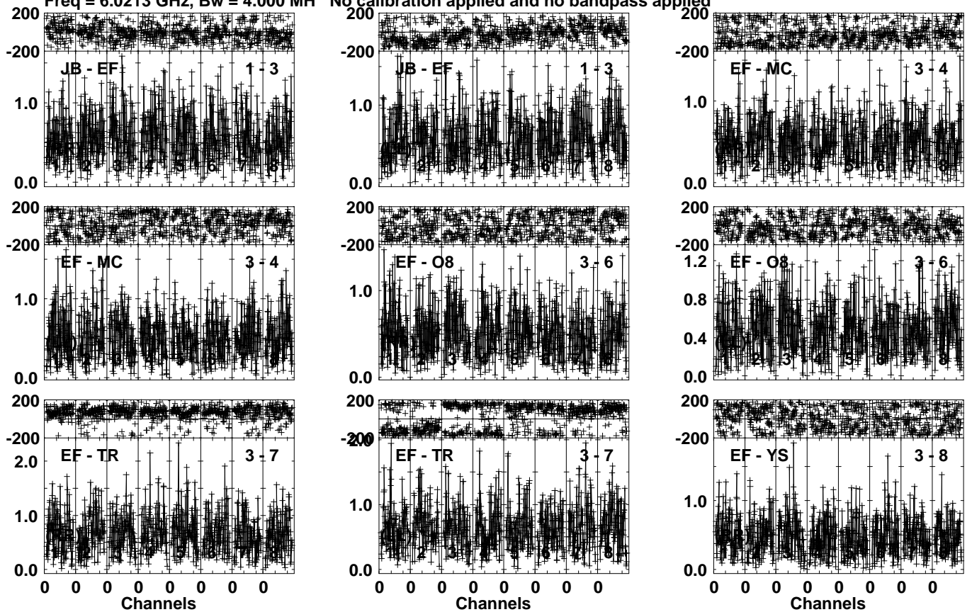
Lower frame: Milli Ampl Jy Top frame: Phas deg Vector averaged cross-power spectrum Several baselines displayed Timerange: 00/21:41:01 to 00/21:42:59
