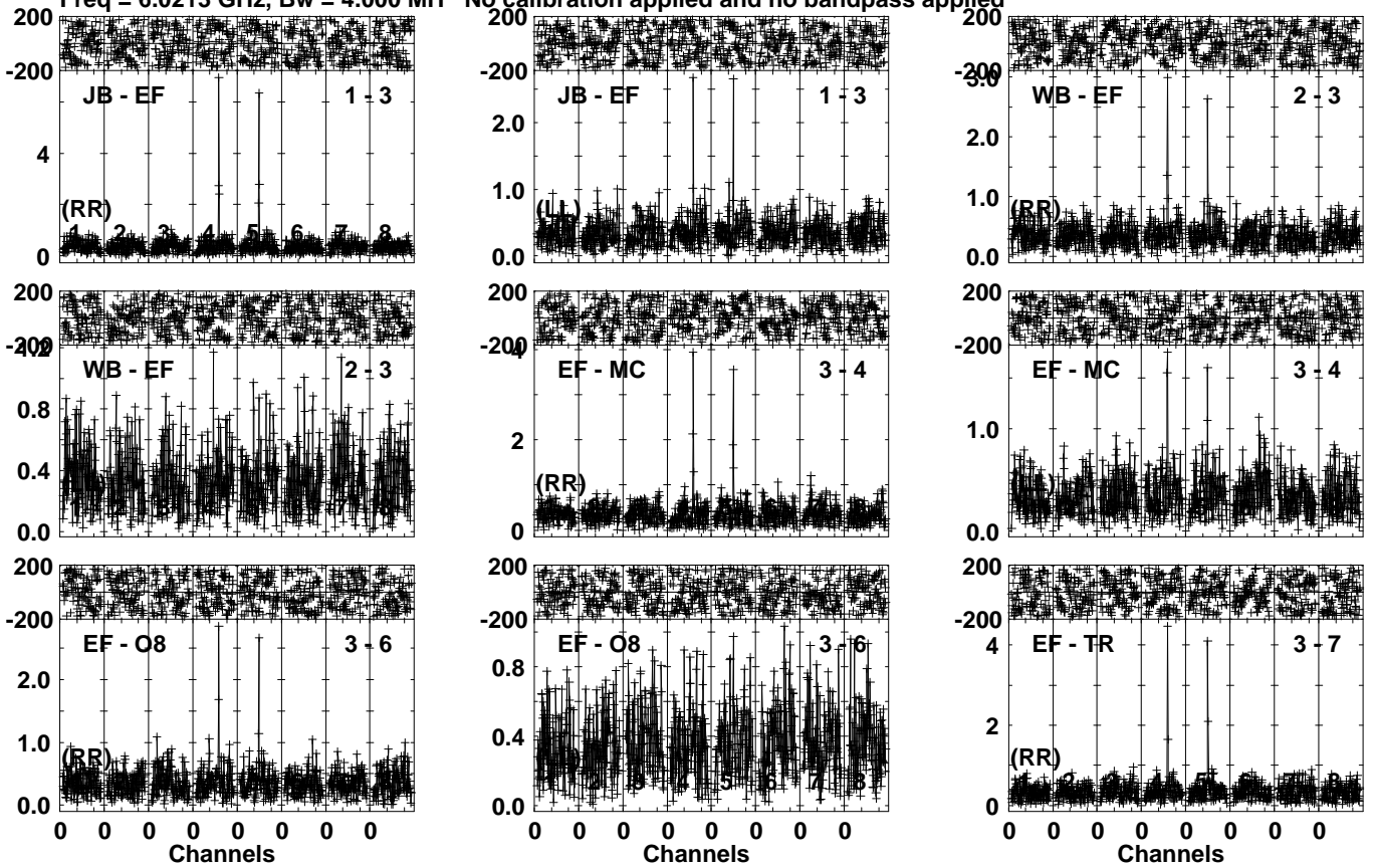
Lower frame: Milli Ampl Jy Top frame: Phas deg Vector averaged cross-power spectrum Several baselines displayed Timerange: 01/03:09:31 to 01/03:12:29
