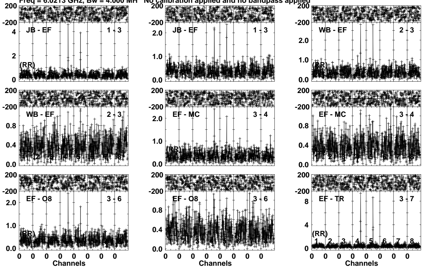
Lower frame: Milli Ampl Jy Top frame: Phas deg Vector averaged cross-power spectrum Several baselines displayed Timerange: 00/23:16:31 to 00/23:19:29
