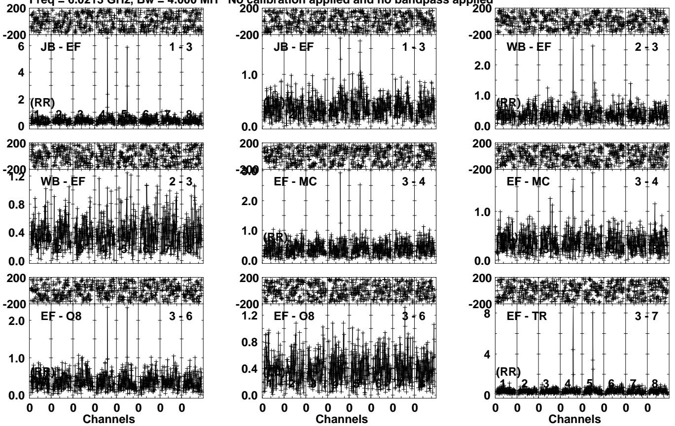
Lower frame: Milli Ampl Jy Top frame: Phas deg Vector averaged cross-power spectrum Several baselines displayed Timerange: 01/03:40:31 to 01/03:43:29
