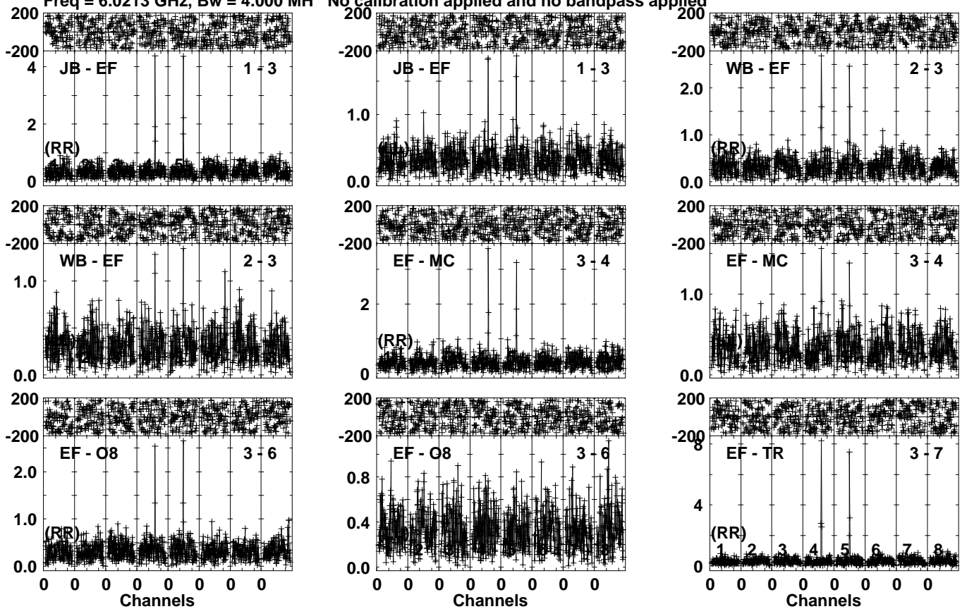
Lower frame: Milli Ampl Jy Top frame: Phas deg Vector averaged cross-power spectrum Several baselines displayed Timerange: 00/23:27:01 to 00/23:29:59
