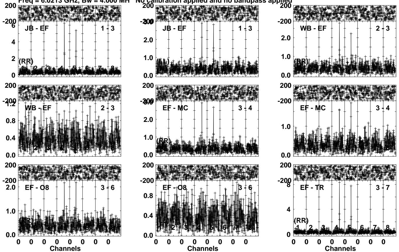
Lower frame: Milli Ampl Jy Top frame: Phas deg Vector averaged cross-power spectrum Several baselines displayed Timerange: 01/02:20:01 to 01/02:22:59
