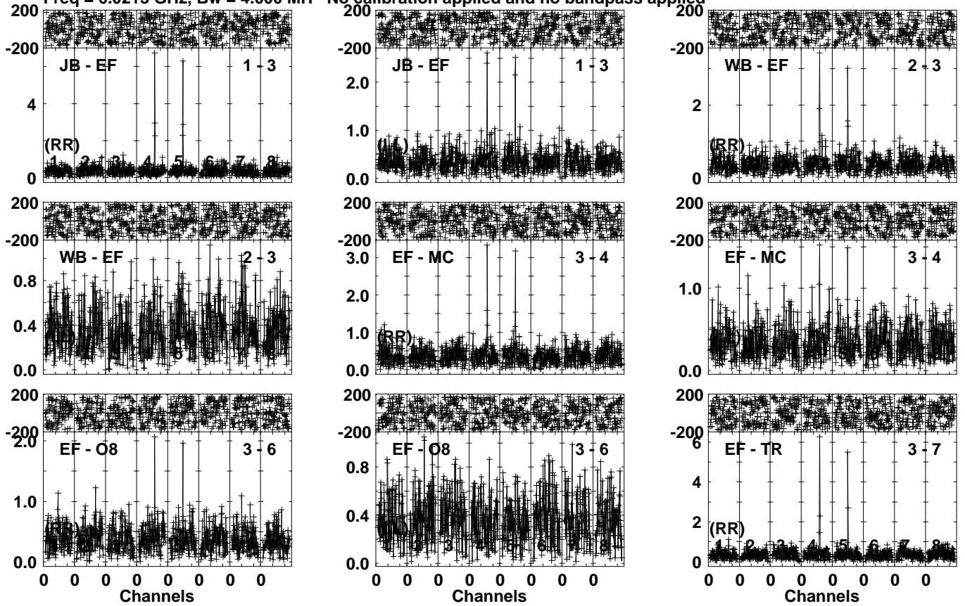
Lower frame: Milli Ampl Jy Top frame: Phas deg Vector averaged cross-power spectrum Several baselines displayed Timerange: 01/02:09:31 to 01/02:12:29
