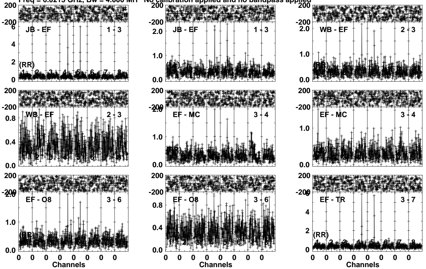
Lower frame: Milli Ampl Jy Top frame: Phas deg Vector averaged cross-power spectrum Several baselines displayed Timerange: 01/00:11:01 to 01/00:13:59
