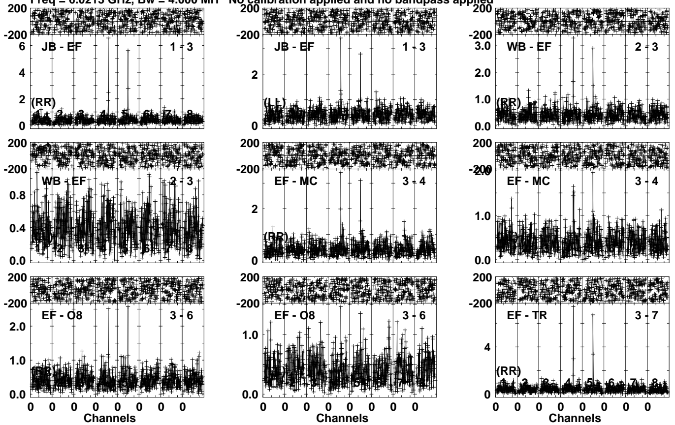
Lower frame: Milli Ampl Jy Top frame: Phas deg Vector averaged cross-power spectrum Several baselines displayed Timerange: 01/03:14:31 to 01/03:17:29
