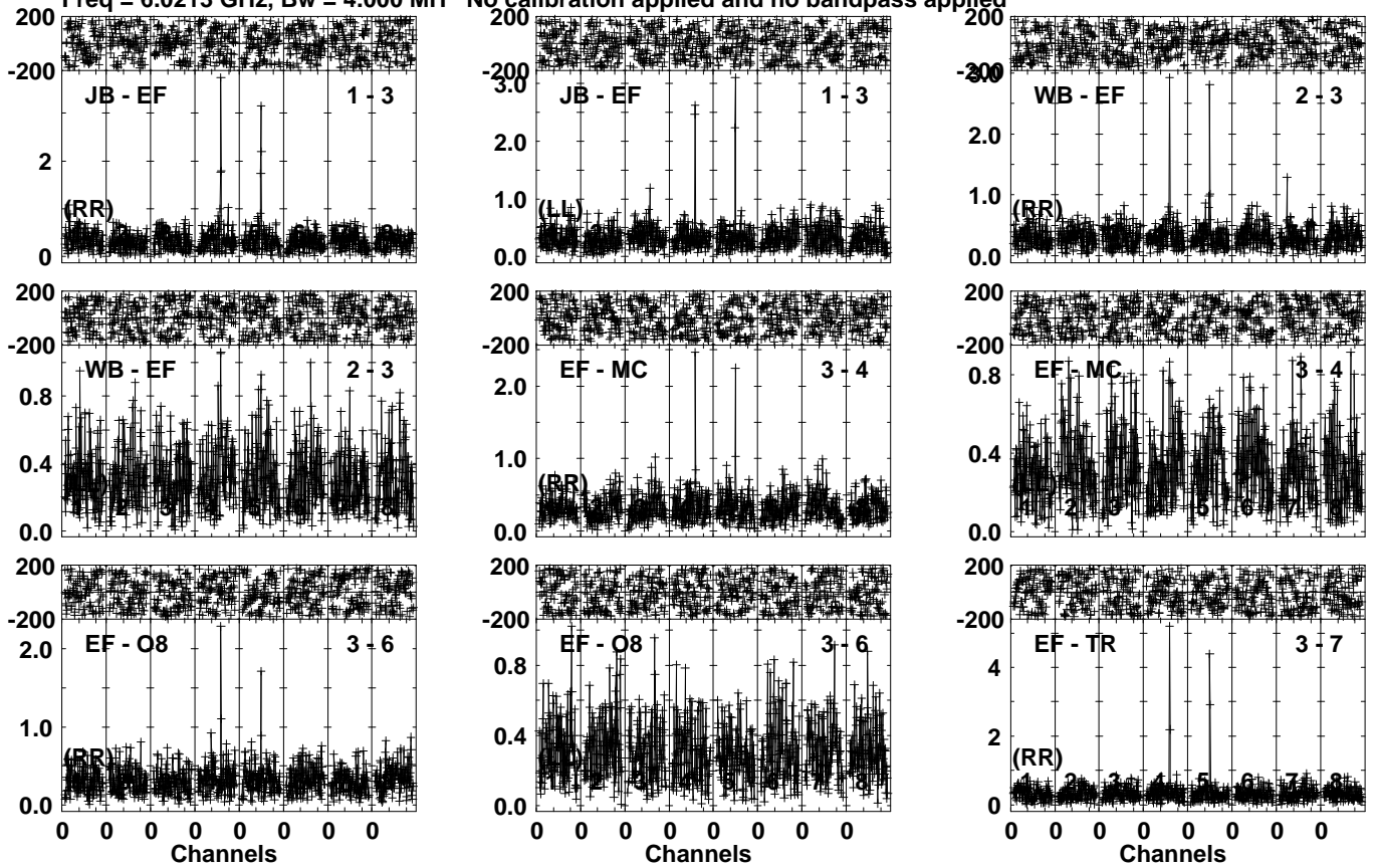
Lower frame: Milli Ampl Jy Top frame: Phas deg Vector averaged cross-power spectrum Several baselines displayed Timerange: 01/07:28:01 to 01/07:30:59
