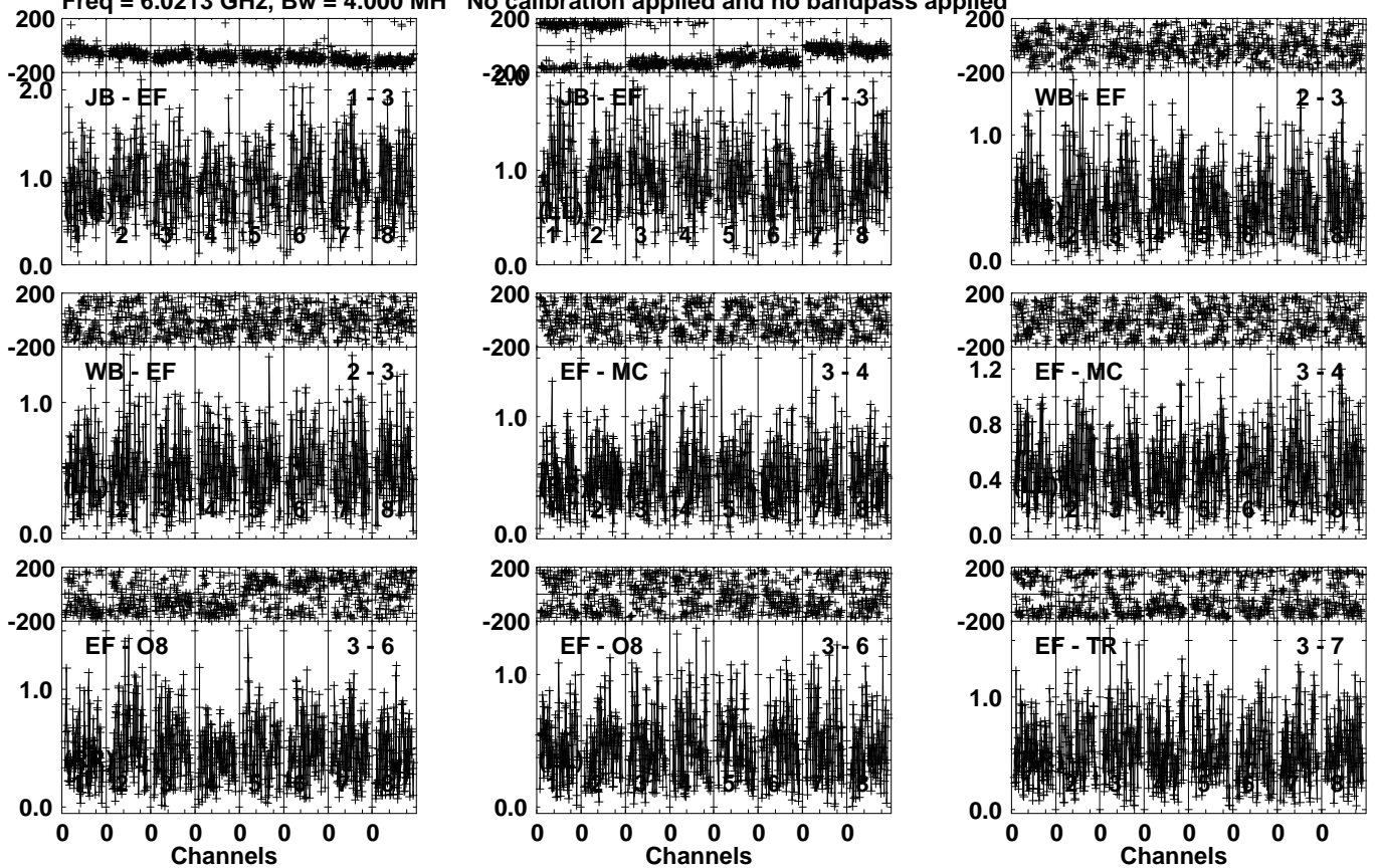
Lower frame: Milli Ampl Jy Top frame: Phas deg Vector averaged cross-power spectrum Several baselines displayed Timerange: 01/07:41:01 to 01/07:42:59
