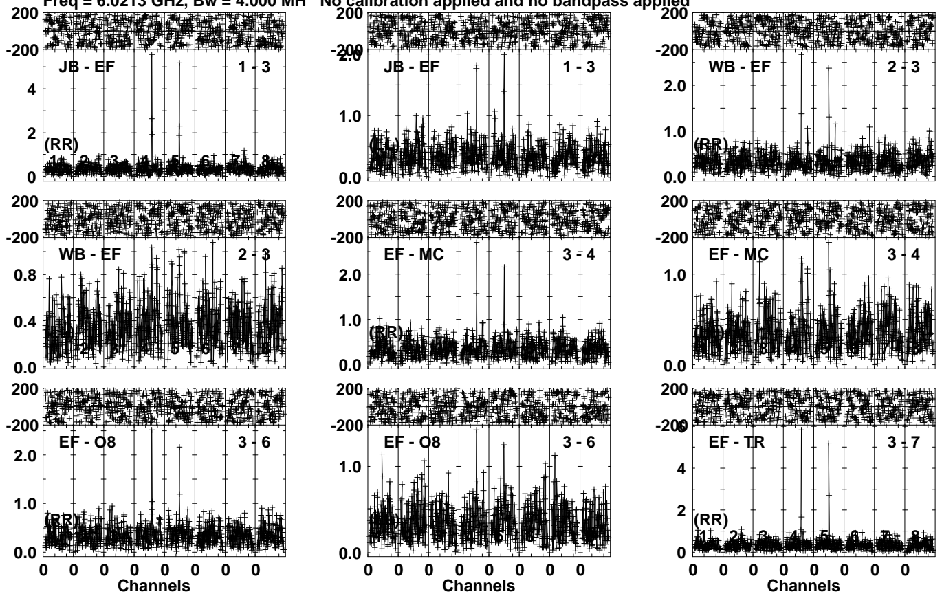
Lower frame: Milli Ampl Jy Top frame: Phas deg Vector averaged cross-power spectrum Several baselines displayed Timerange: 01/08:17:01 to 01/08:19:59
