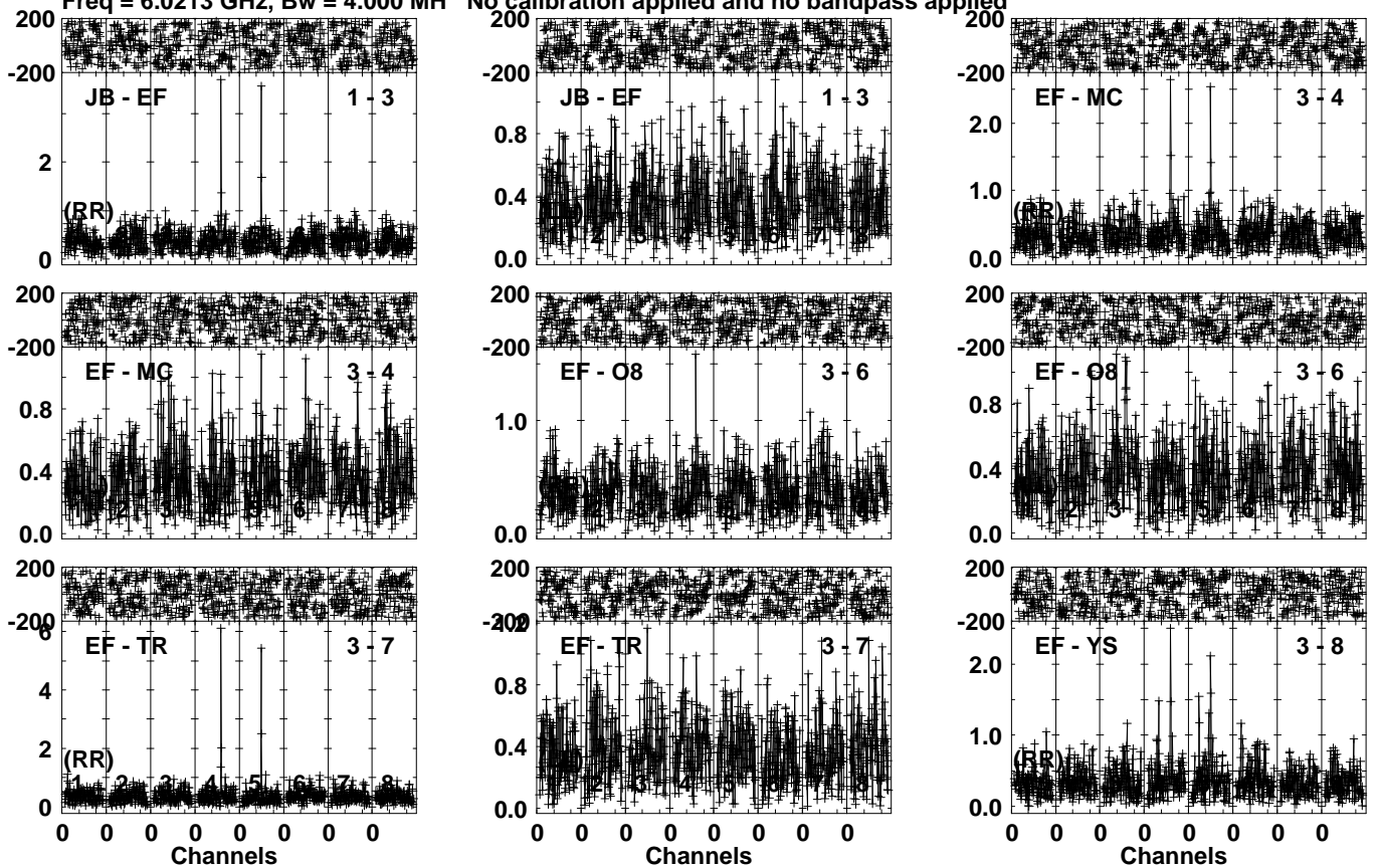
Lower frame: Milli Ampl Jy Top frame: Phas deg Vector averaged cross-power spectrum Several baselines displayed Timerange: 00/21:17:31 to 00/21:20:29
