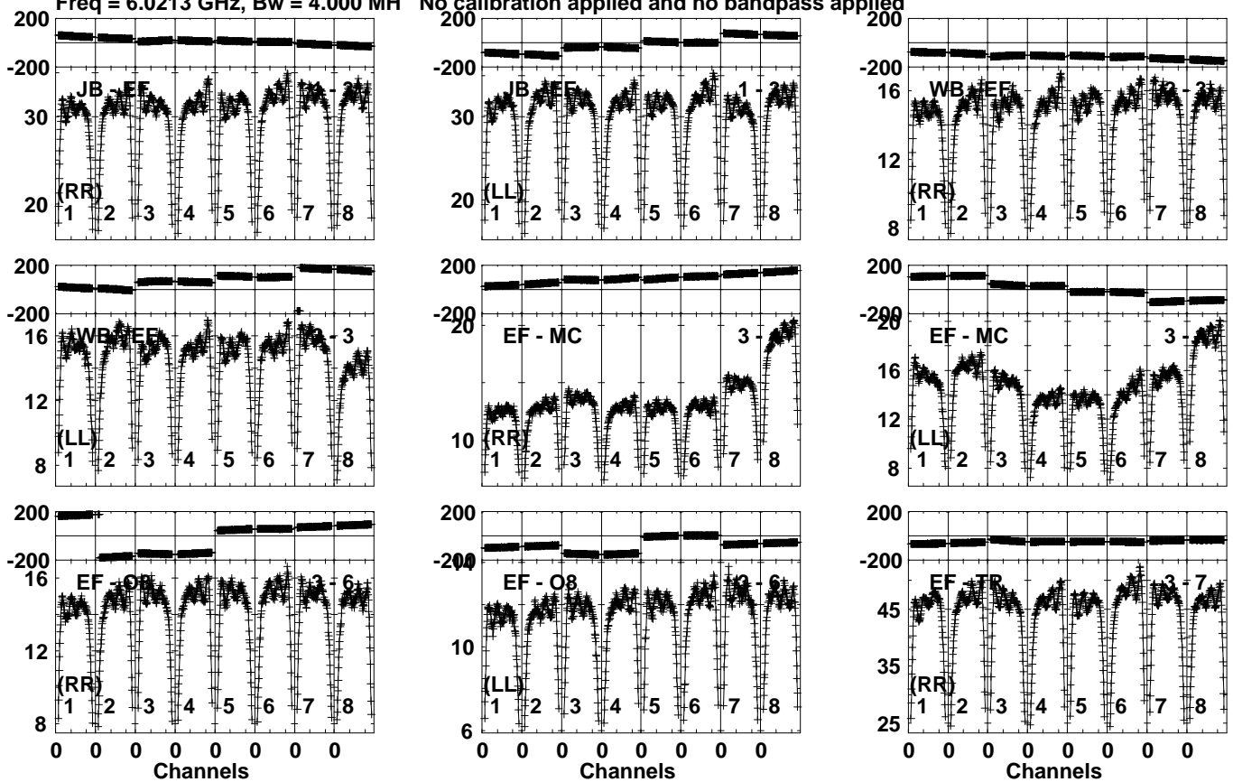
Lower frame: Milli Ampl Jy Top frame: Phas deg Vector averaged cross-power spectrum Several baselines displayed Timerange: 01/03:56:31 to 01/04:05:29
