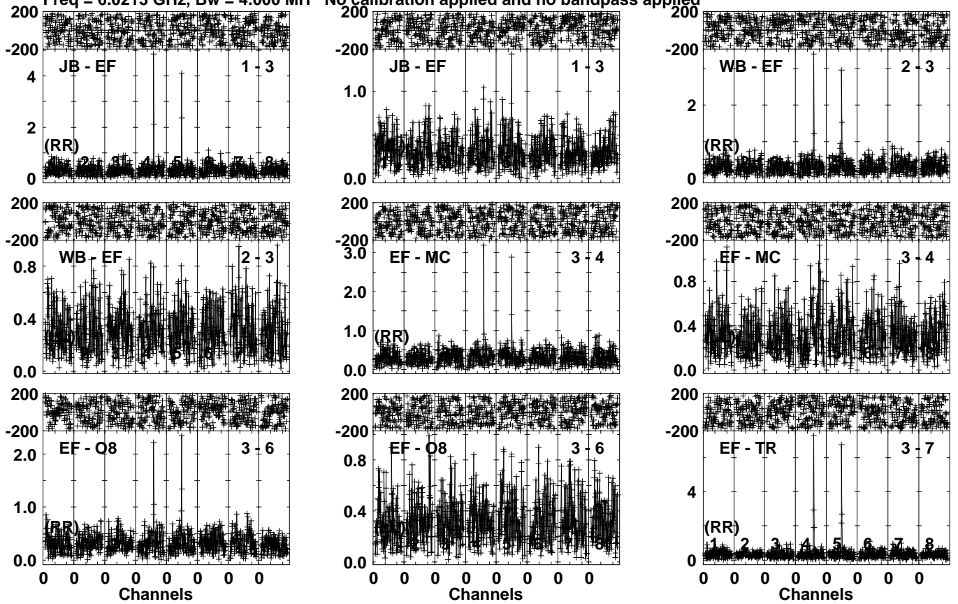
Lower frame: Milli Ampl Jy Top frame: Phas deg Vector averaged cross-power spectrum Several baselines displayed Timerange: 01/07:12:31 to 01/07:15:29
