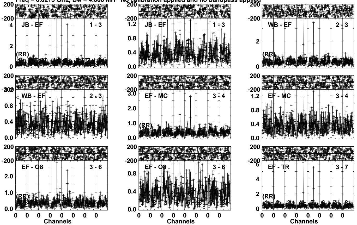
Lower frame: Milli Ampl Jy Top frame: Phas deg Vector averaged cross-power spectrum Several baselines displayed Timerange: 01/05:37:31 to 01/05:40:29
