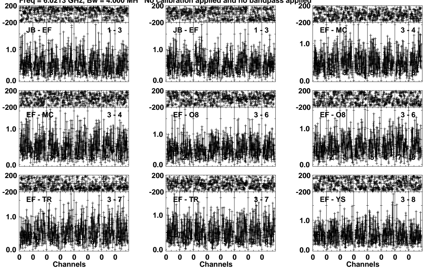
Lower frame: Milli Ampl Jy Top frame: Phas deg Vector averaged cross-power spectrum Several baselines displayed Timerange: 00/21:46:31 to 00/21:48:29
