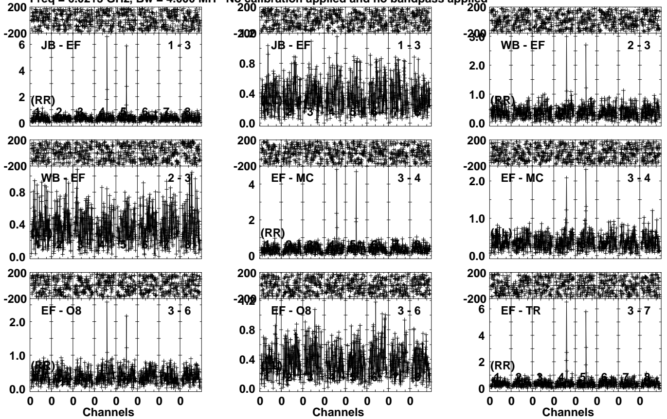
Lower frame: Milli Ampl Jy Top frame: Phas deg Vector averaged cross-power spectrum Several baselines displayed Timerange: 01/05:32:31 to 01/05:35:29
