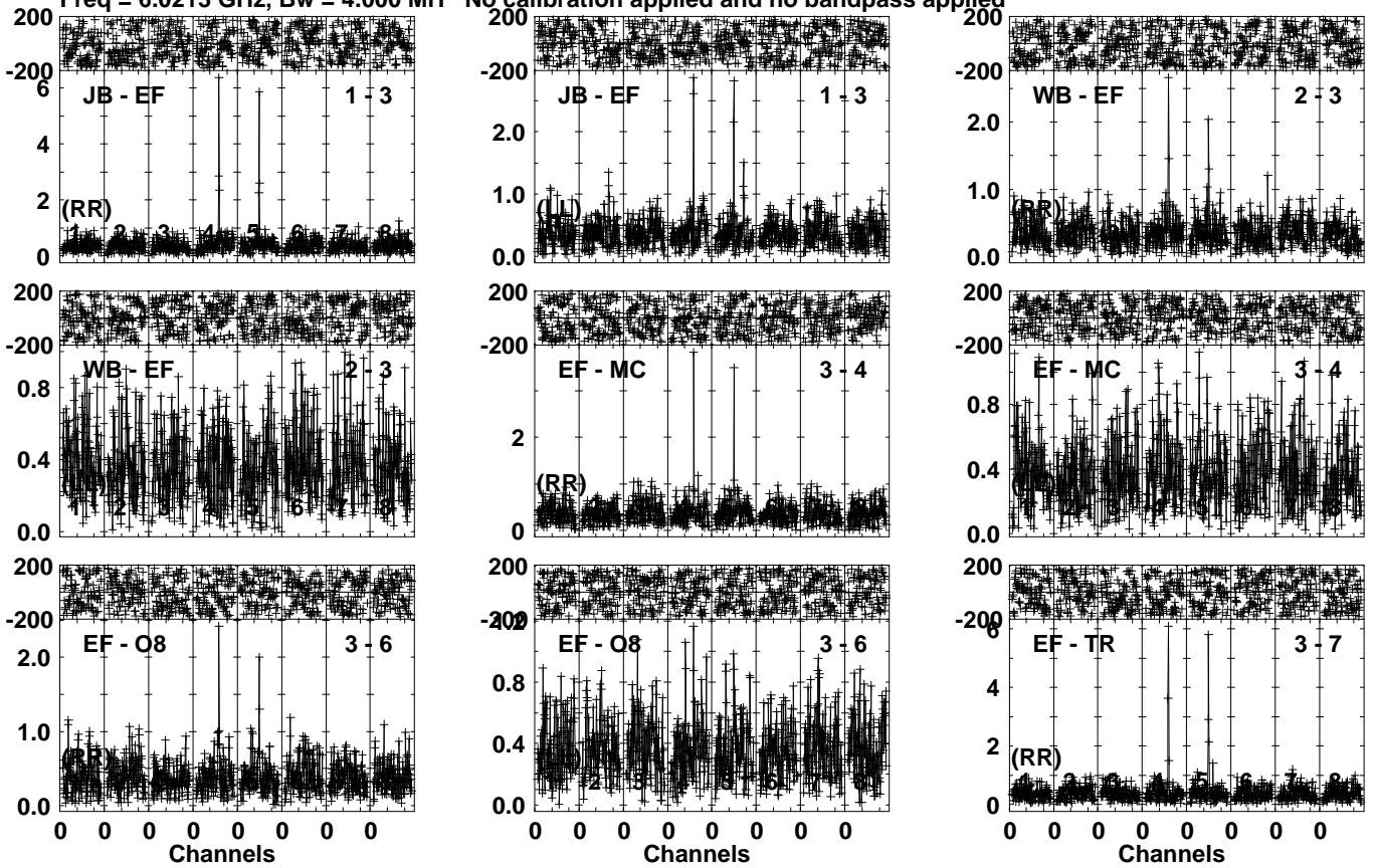
Lower frame: Milli Ampl Jy Top frame: Phas deg Vector averaged cross-power spectrum Several baselines displayed Timerange: 01/04:52:01 to 01/04:54:59
