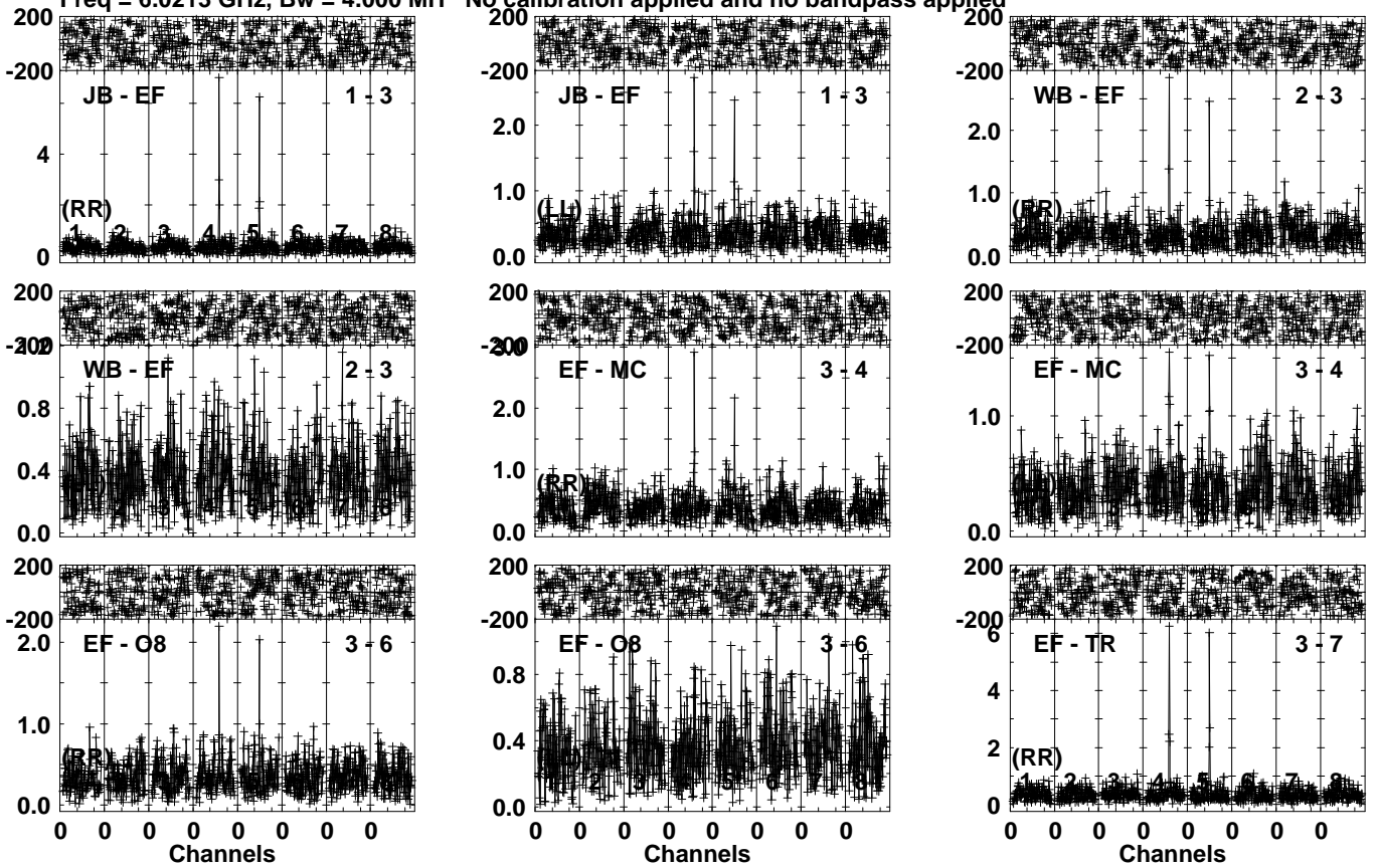
Lower frame: Milli Ampl Jy Top frame: Phas deg Vector averaged cross-power spectrum Several baselines displayed Timerange: 01/03:25:01 to 01/03:27:59
