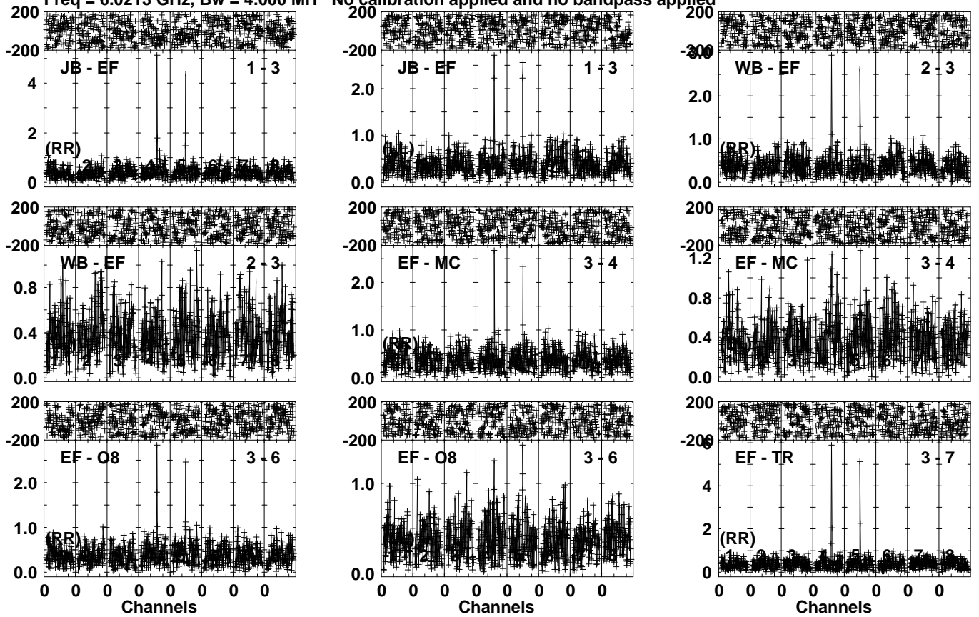
Lower frame: Milli Ampl Jy Top frame: Phas deg Vector averaged cross-power spectrum Several baselines displayed Timerange: 01/04:31:31 to 01/04:34:29
