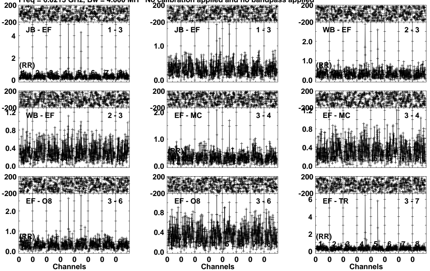
Lower frame: Milli Ampl Jy Top frame: Phas deg Vector averaged cross-power spectrum Several baselines displayed Timerange: 01/04:26:31 to 01/04:29:29
