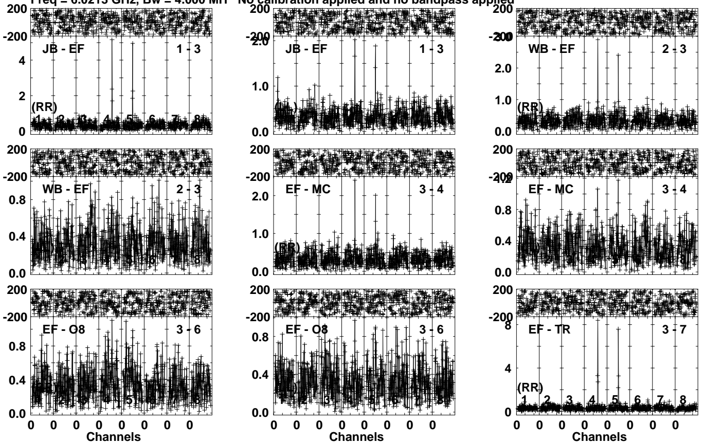
Lower frame: Milli Ampl Jy Top frame: Phas deg Vector averaged cross-power spectrum Several baselines displayed Timerange: 00/22:12:01 to 00/22:14:59
