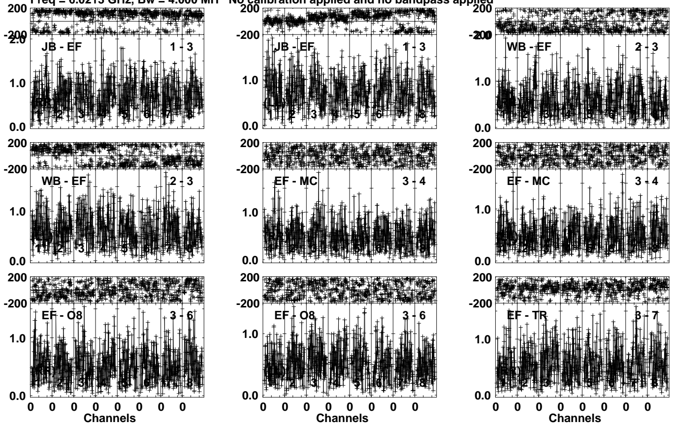
Lower frame: Milli Ampl Jy Top frame: Phas deg Vector averaged cross-power spectrum Several baselines displayed Timerange: 01/06:21:01 to 01/06:22:59
