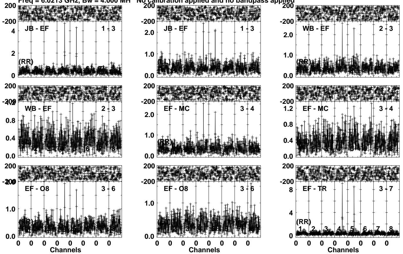
Lower frame: Milli Ampl Jy Top frame: Phas deg Vector averaged cross-power spectrum Several baselines displayed Timerange: 00/22:22:01 to 00/22:24:59
