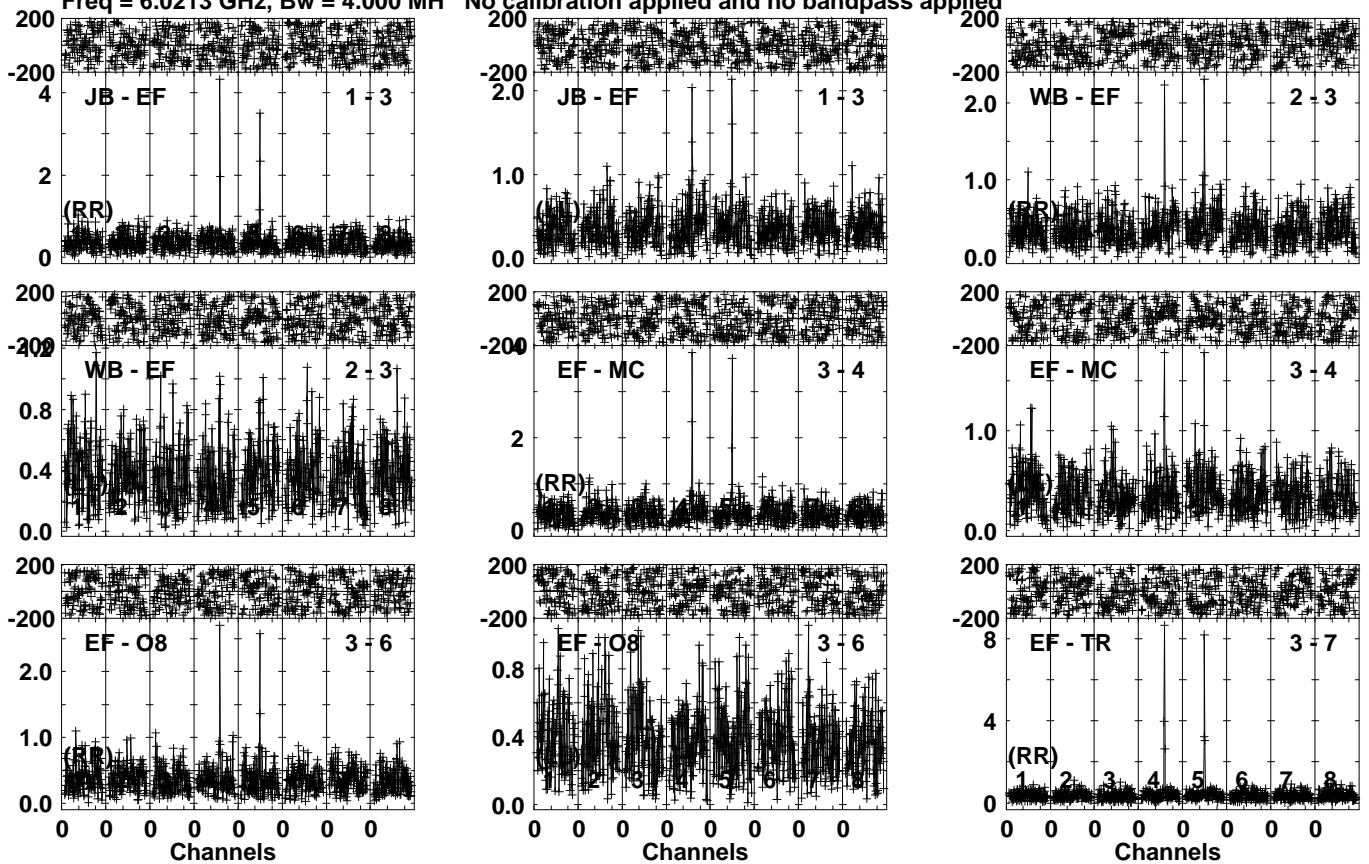
Lower frame: Milli Ampl Jy Top frame: Phas deg Vector averaged cross-power spectrum Several baselines displayed Timerange: 00/22:53:01 to 00/22:55:59
