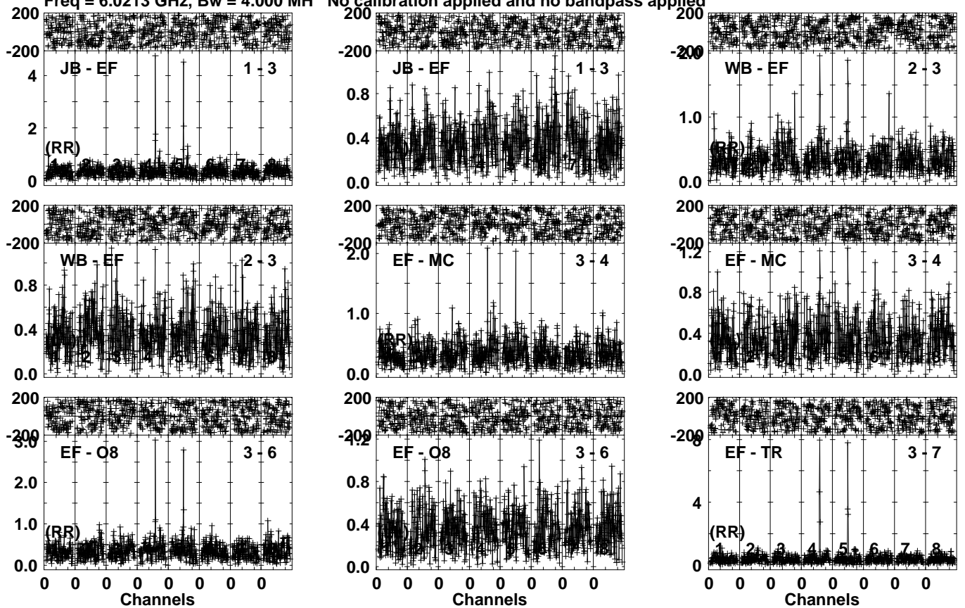
Lower frame: Milli Ampl Jy Top frame: Phas deg Vector averaged cross-power spectrum Several baselines displayed Timerange: 01/06:49:01 to 01/06:51:59
