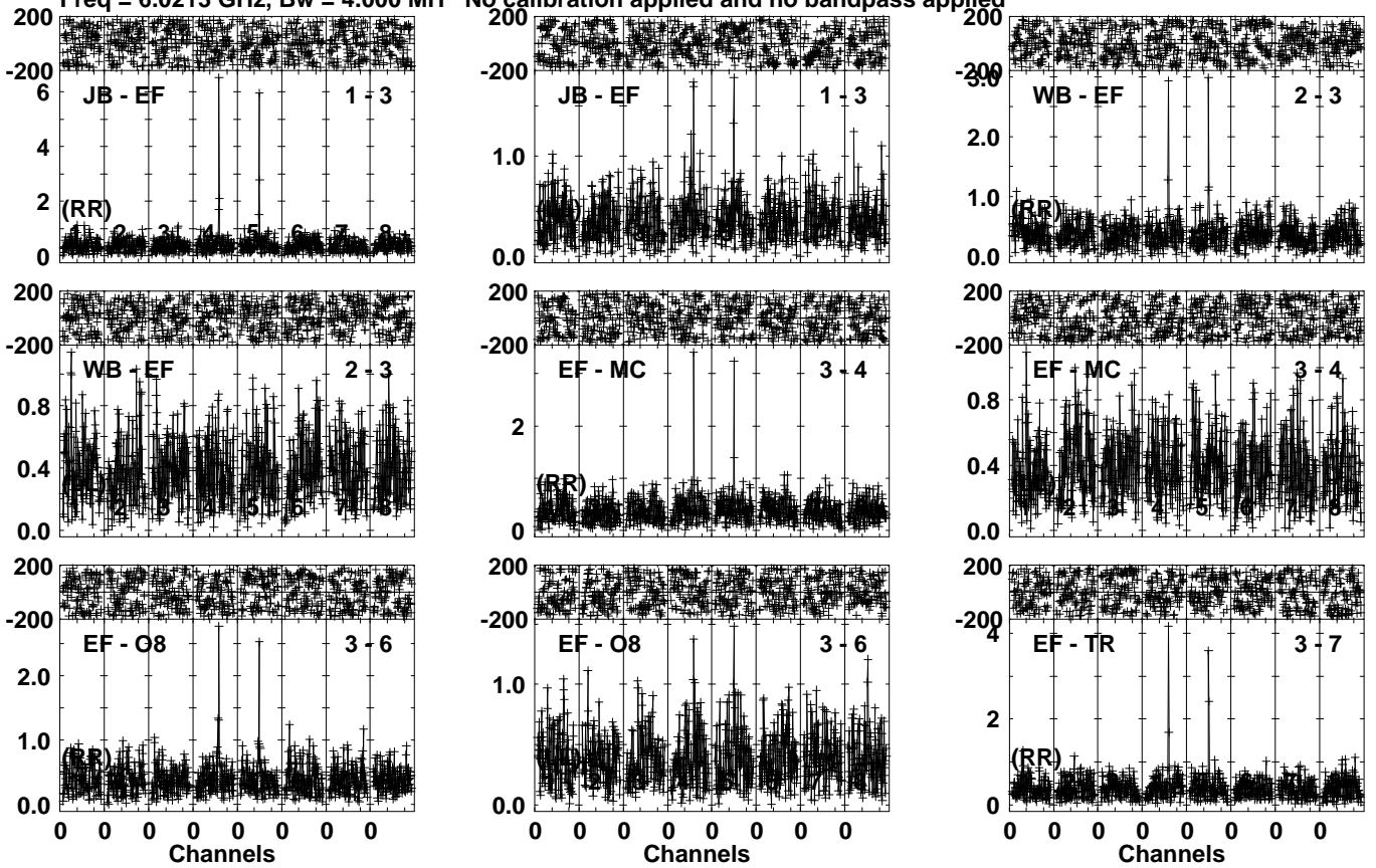
Lower frame: Milli Ampl Jy Top frame: Phas deg Vector averaged cross-power spectrum Several baselines displayed Timerange: 01/04:21:01 to 01/04:23:59
