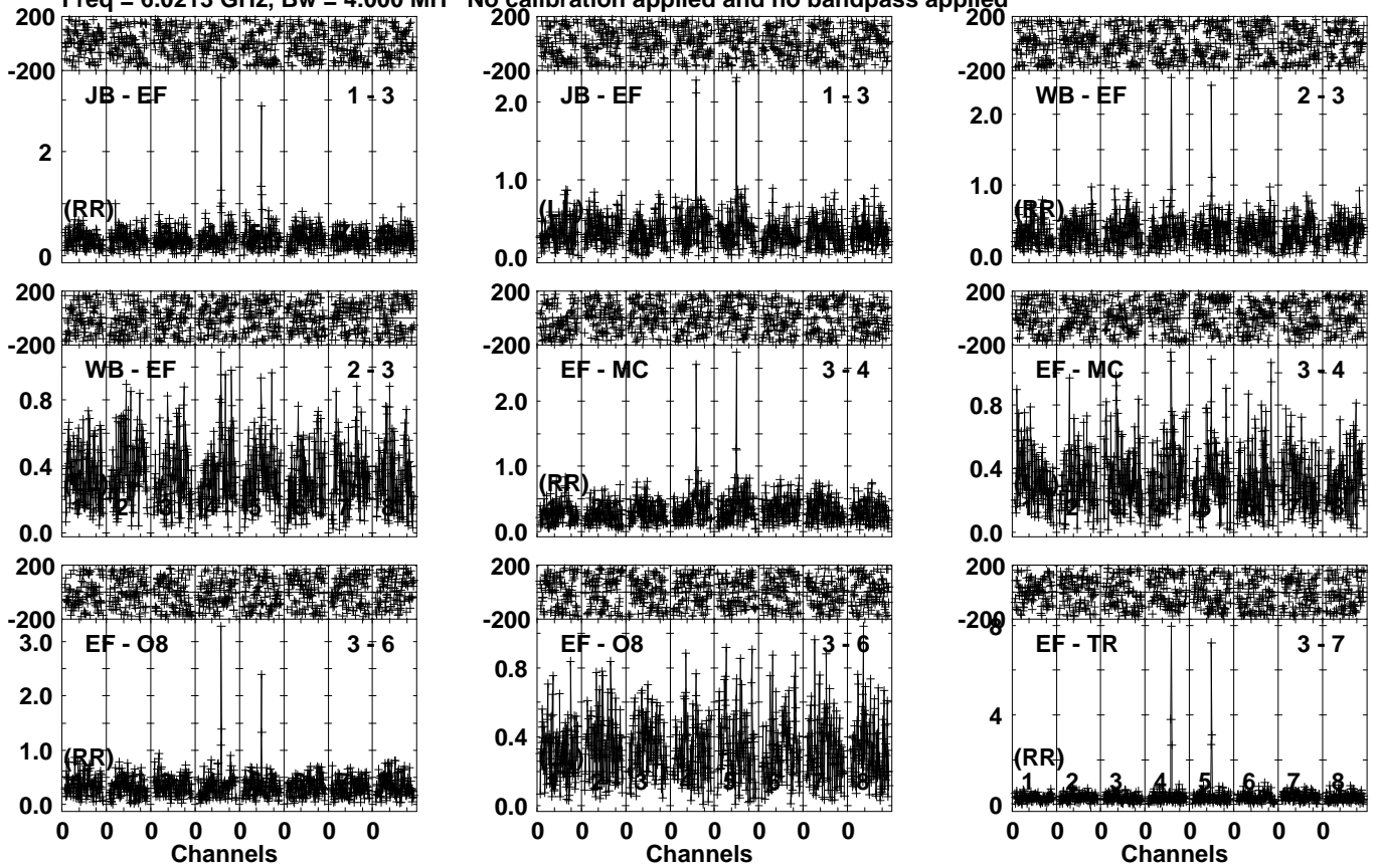
Lower frame: Milli Ampl Jy Top frame: Phas deg Vector averaged cross-power spectrum Several baselines displayed Timerange: 00/23:11:31 to 00/23:14:29
