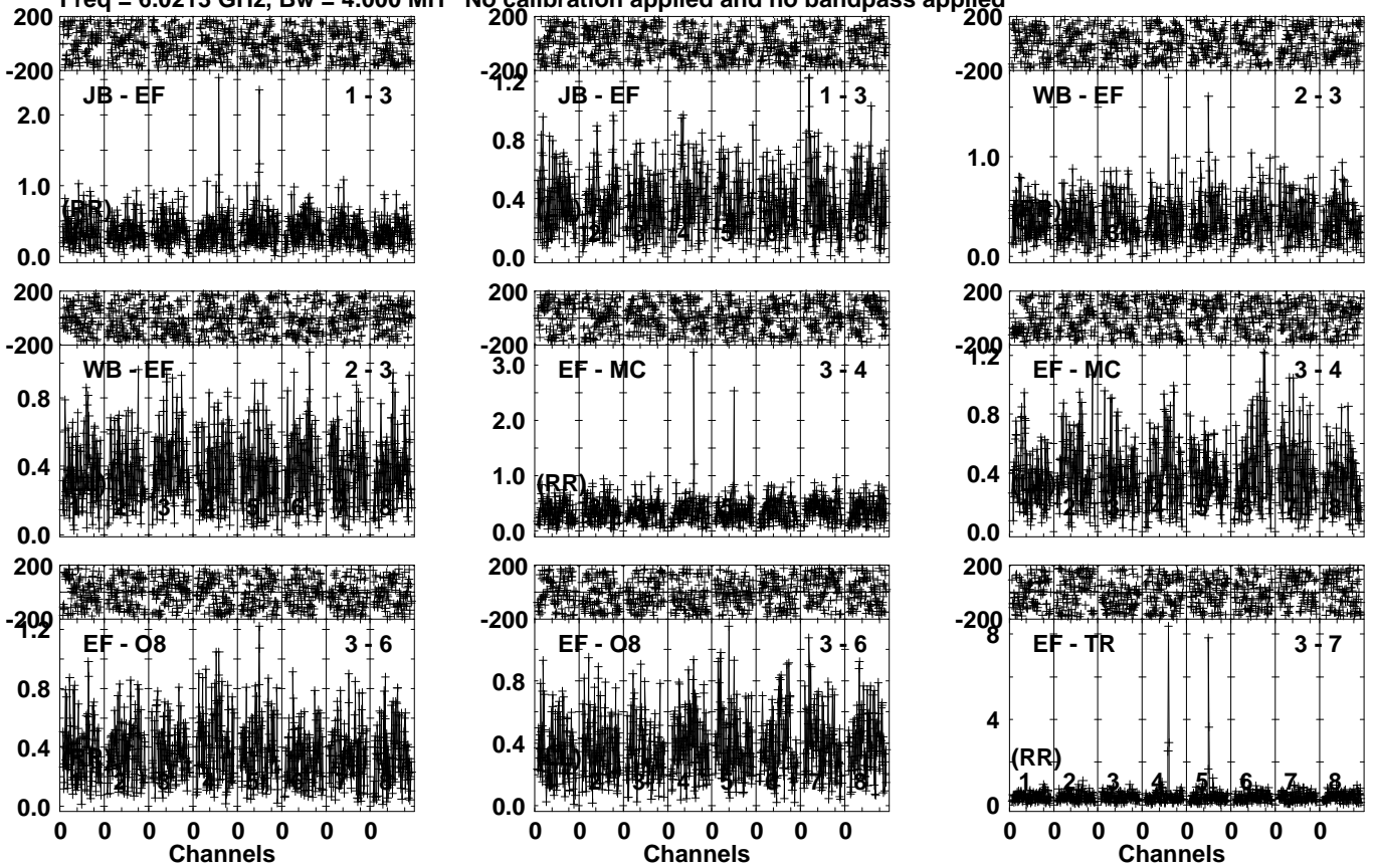
Lower frame: Milli Ampl Jy Top frame: Phas deg Vector averaged cross-power spectrum Several baselines displayed Timerange: 00/21:48:31 to 00/21:51:29
