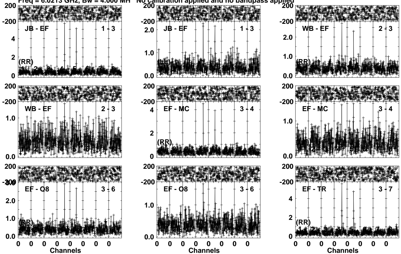
Lower frame: Milli Ampl Jy Top frame: Phas deg Vector averaged cross-power spectrum Several baselines displayed Timerange: 01/04:16:01 to 01/04:18:59
