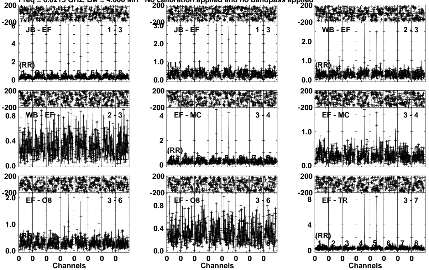
Lower frame: Milli Ampl Jy Top frame: Phas deg Vector averaged cross-power spectrum Several baselines displayed Timerange: 01/02:46:01 to 01/02:48:59
