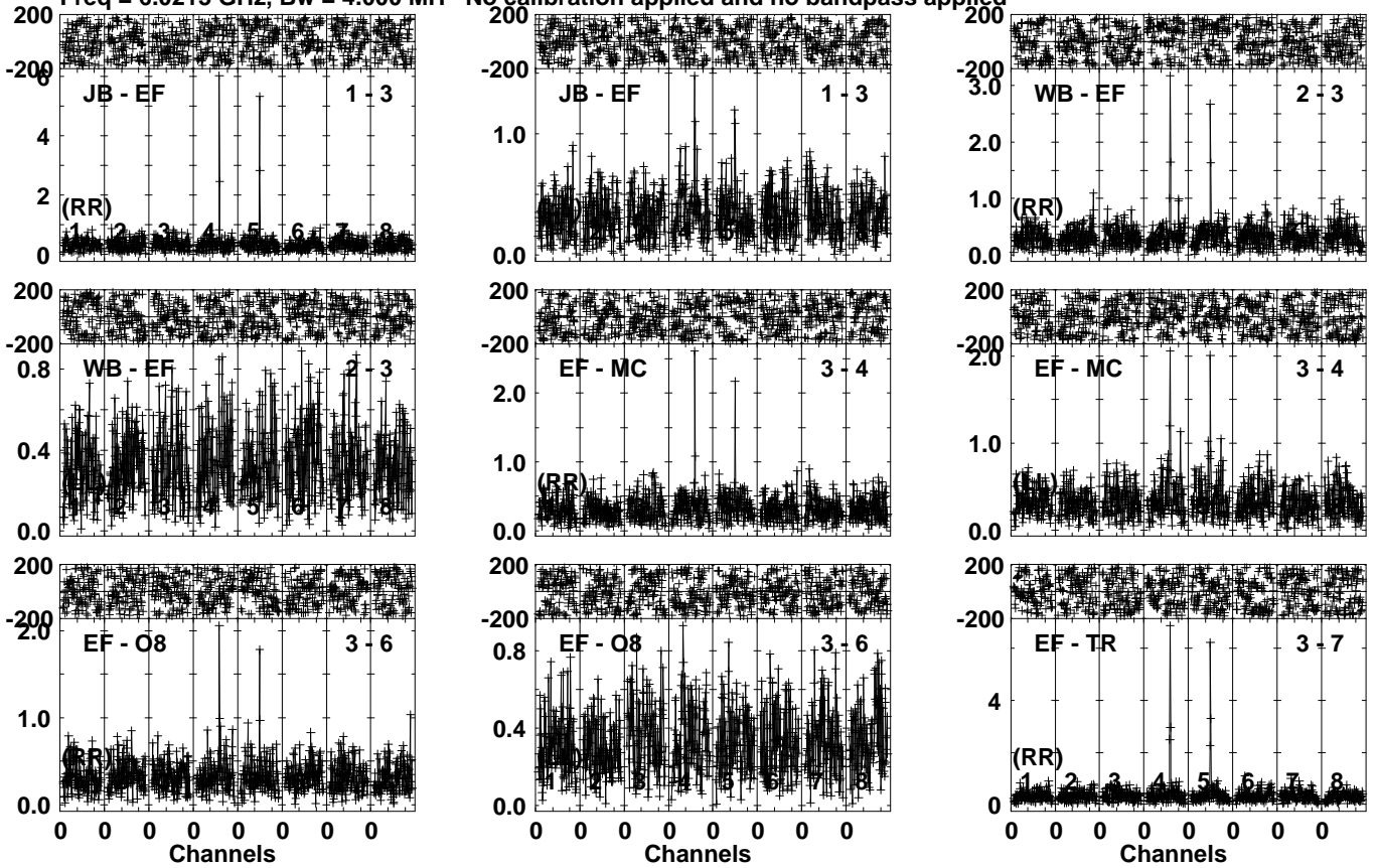
Lower frame: Milli Ampl Jy Top frame: Phas deg Vector averaged cross-power spectrum Several baselines displayed Timerange: 01/01:36:01 to 01/01:38:59
