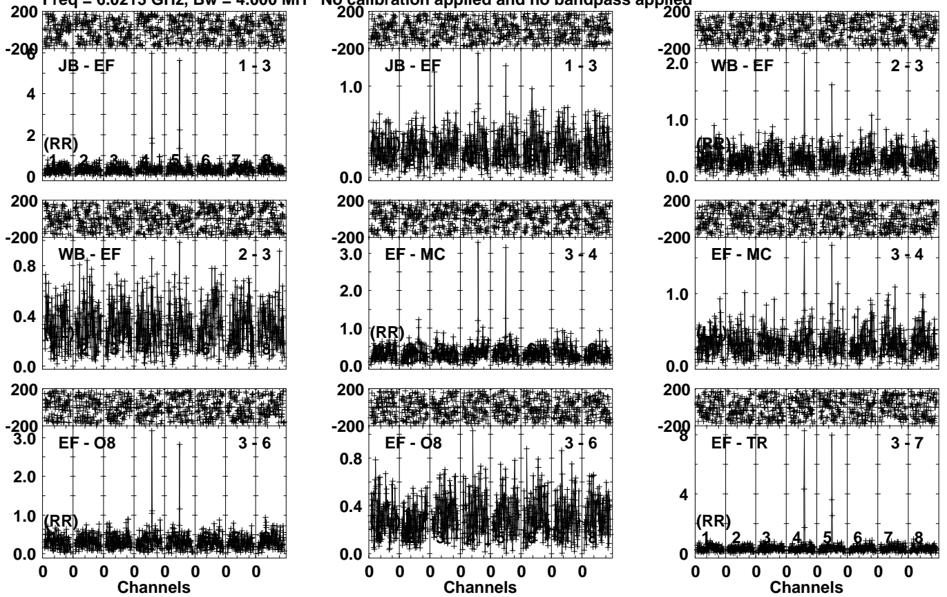
Lower frame: Milli Ampl Jy Top frame: Phas deg Vector averaged cross-power spectrum Several baselines displayed Timerange: 01/06:44:01 to 01/06:46:59
