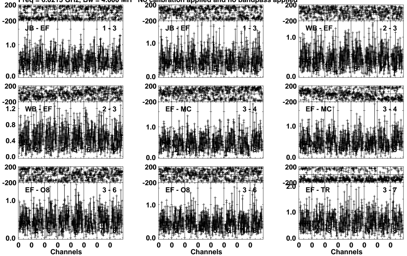
Lower frame: Milli Ampl Jy Top frame: Phas deg Vector averaged cross-power spectrum Several baselines displayed Timerange: 01/06:52:01 to 01/06:53:59
