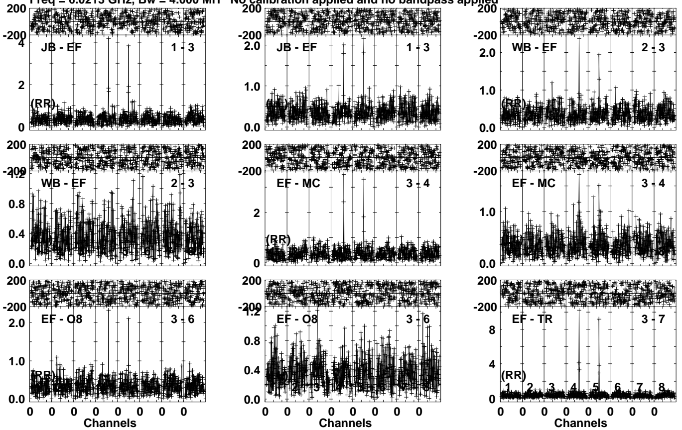
Lower frame: Milli Ampl Jy Top frame: Phas deg Vector averaged cross-power spectrum Several baselines displayed Timerange: 00/22:37:31 to 00/22:40:29
