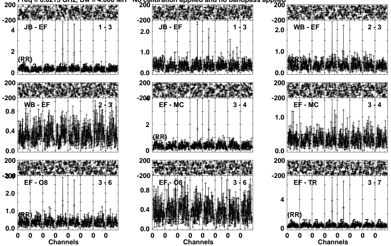
Lower frame: Milli Ampl Jy Top frame: Phas deg Vector averaged cross-power spectrum Several baselines displayed Timerange: 01/06:33:31 to 01/06:36:29
