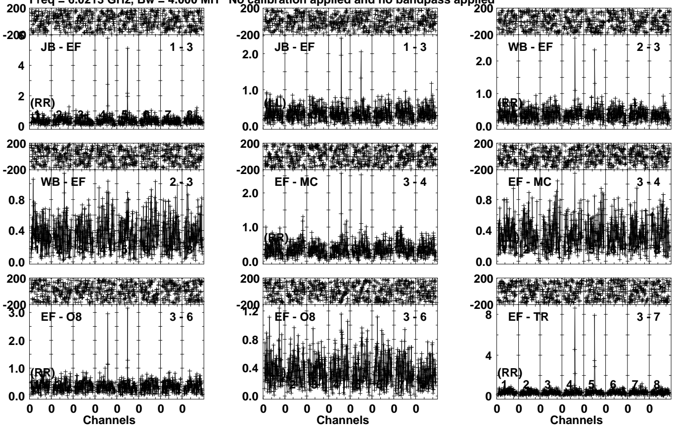
Lower frame: Milli Ampl Jy Top frame: Phas deg Vector averaged cross-power spectrum Several baselines displayed Timerange: 01/06:38:31 to 01/06:41:29
