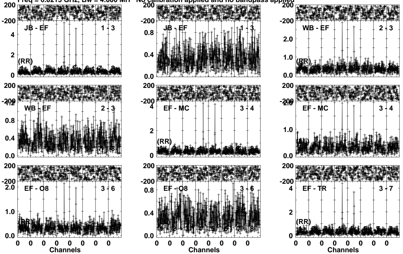
Lower frame: Milli Ampl Jy Top frame: Phas deg Vector averaged cross-power spectrum Several baselines displayed Timerange: 01/05:27:31 to 01/05:30:29
