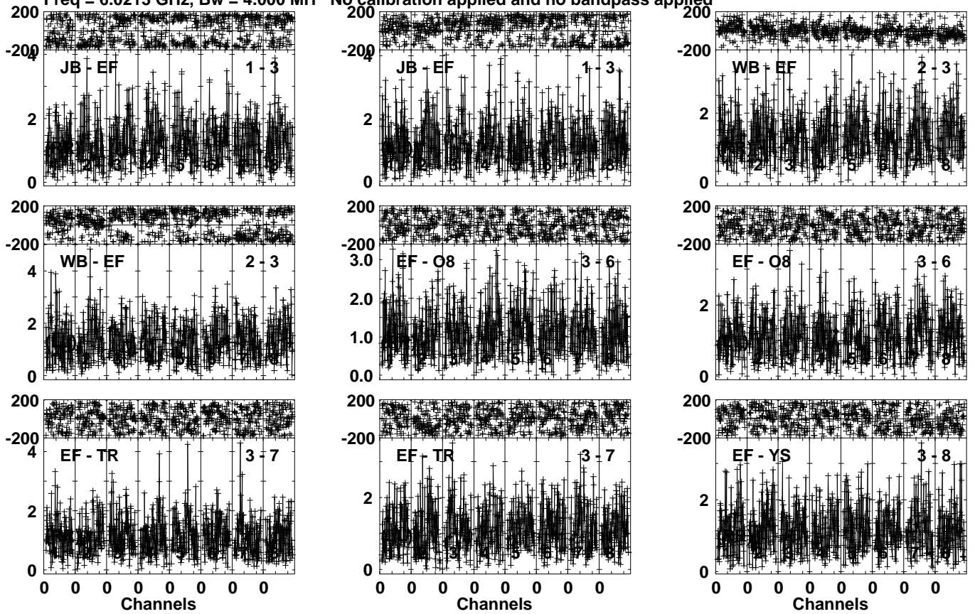
Lower frame: Milli Ampl Jy Top frame: Phas deg Vector averaged cross-power spectrum Several baselines displayed Timerange: 01/03:33:01 to 01/03:34:59
