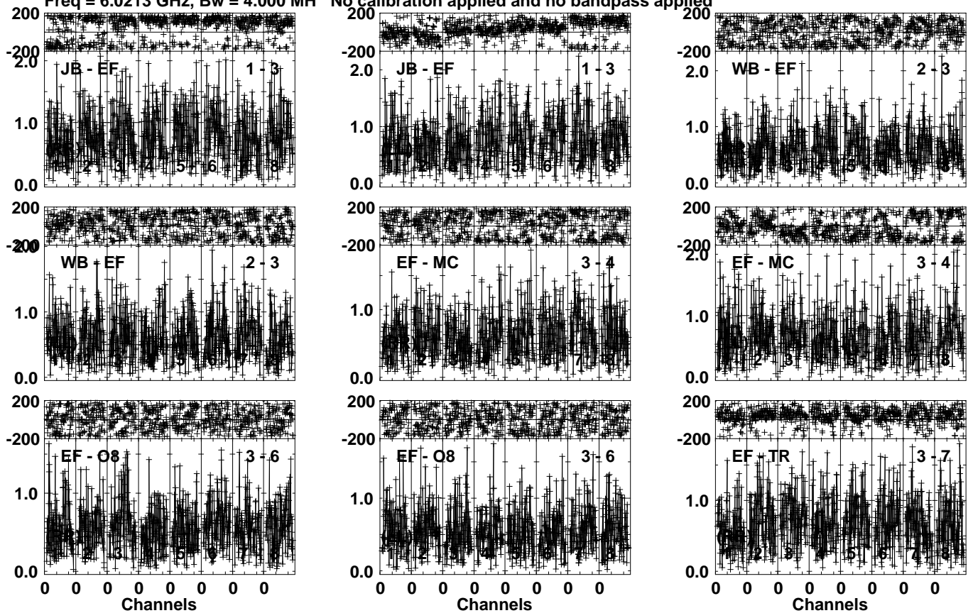
Lower frame: Milli Ampl Jy Top frame: Phas deg Vector averaged cross-power spectrum Several baselines displayed Timerange: 01/04:24:01 to 01/04:25:59
