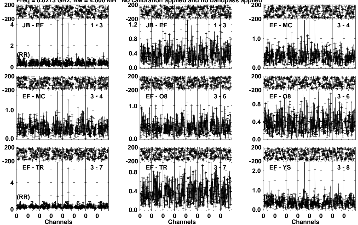
Lower frame: Milli Ampl Jy Top frame: Phas deg Vector averaged cross-power spectrum Several baselines displayed Timerange: 00/21:33:01 to 00/21:35:59
