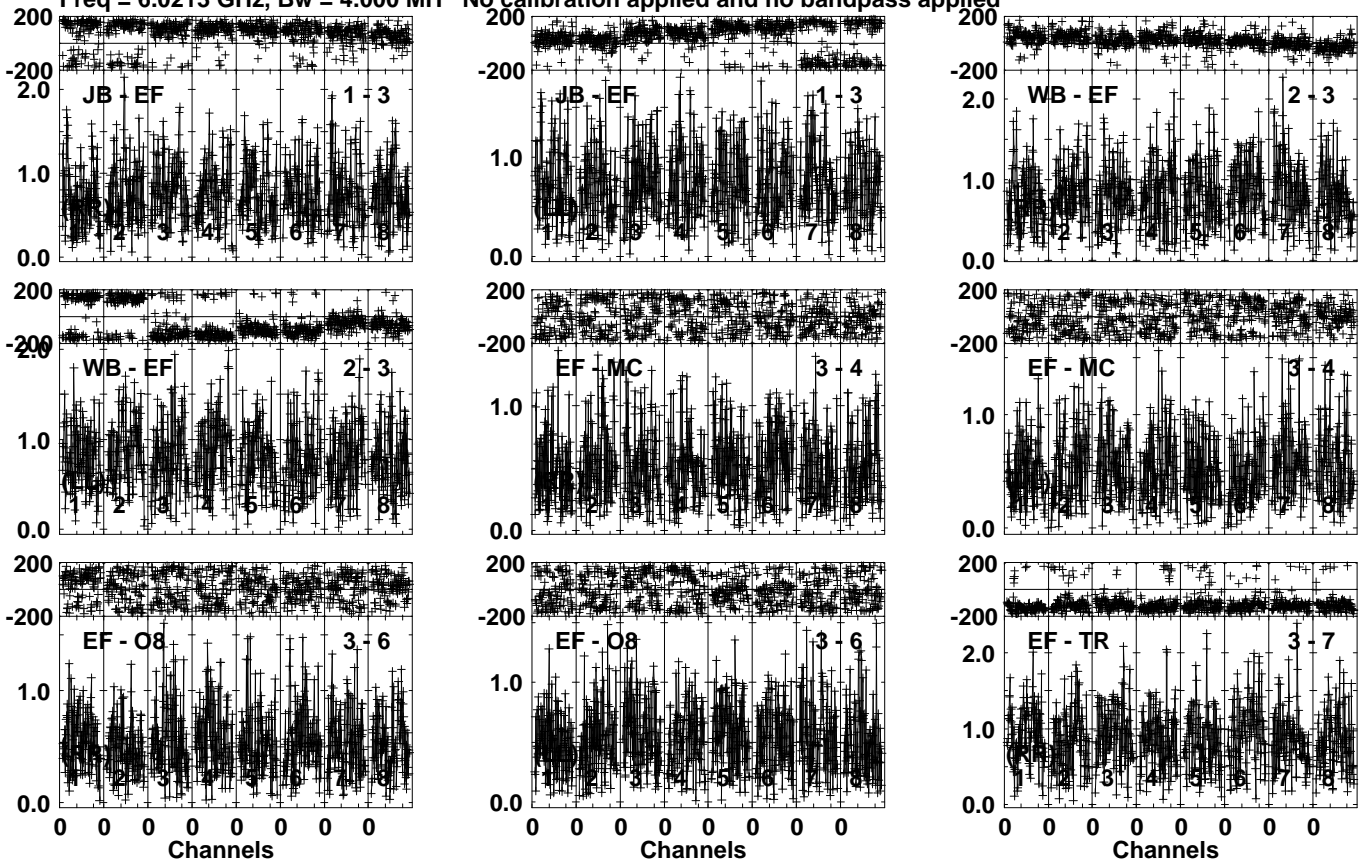
Lower frame: Milli Ampl Jy Top frame: Phas deg Vector averaged cross-power spectrum Several baselines displayed Timerange: 00/23:19:31 to 00/23:21:29
