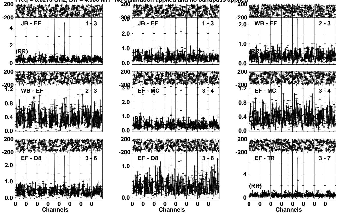
Lower frame: Milli Ampl Jy Top frame: Phas deg Vector averaged cross-power spectrum Several baselines displayed Timerange: 01/04:47:01 to 01/04:49:59
