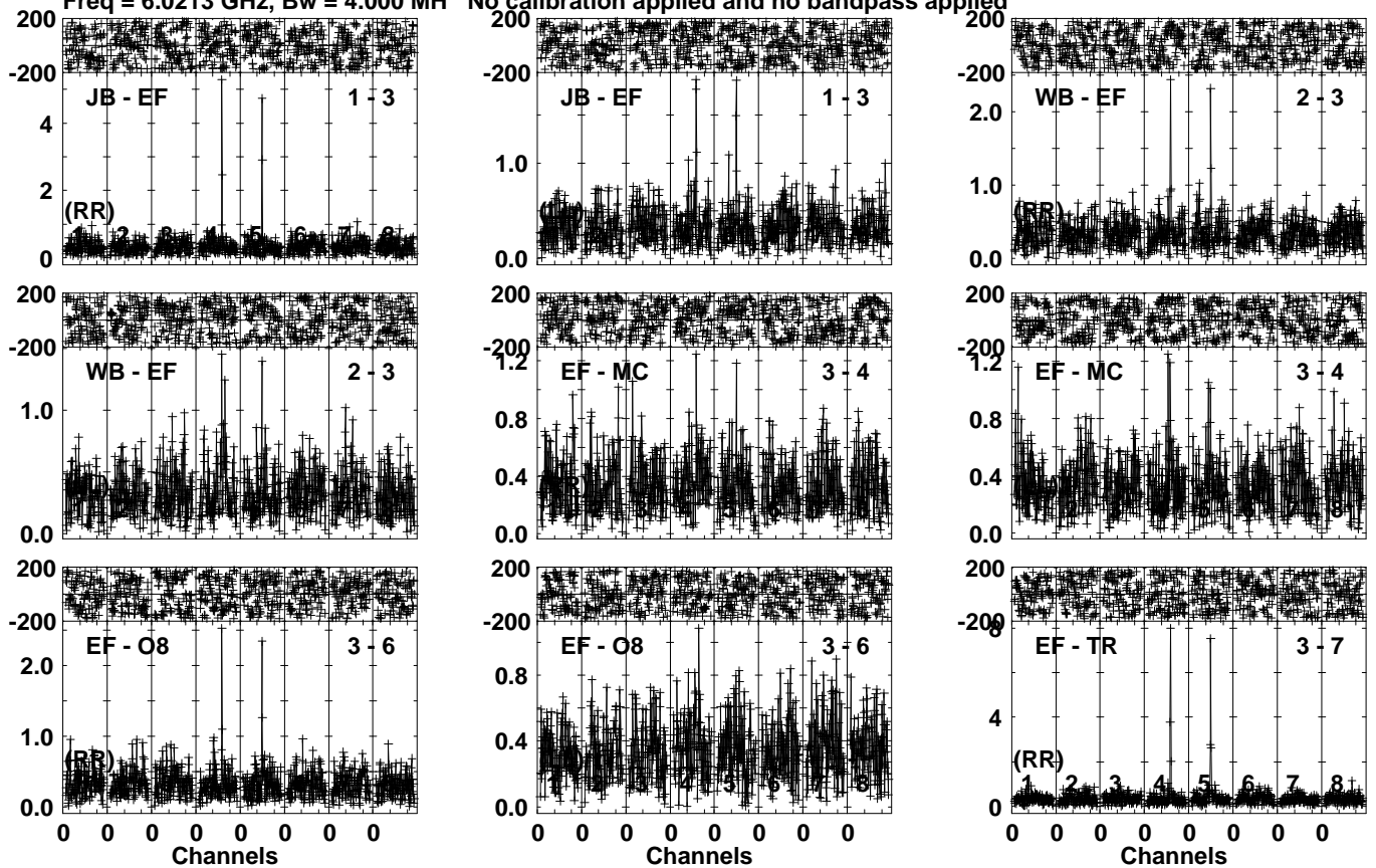
Lower frame: Milli Ampl Jy Top frame: Phas deg Vector averaged cross-power spectrum Several baselines displayed Timerange: 01/01:05:01 to 01/01:07:59
