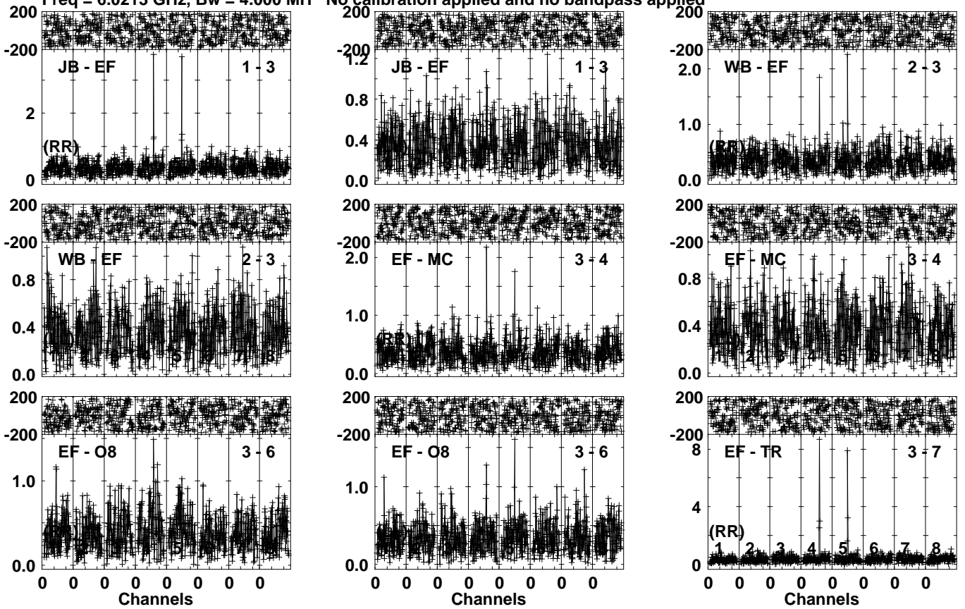
Lower frame: Milli Ampl Jy Top frame: Phas deg Vector averaged cross-power spectrum Several baselines displayed Timerange: 00/21:53:31 to 00/21:56:29
