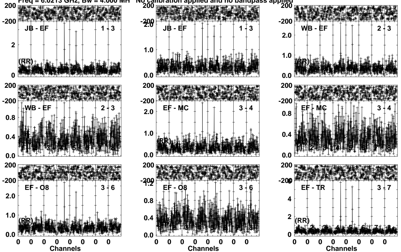
Lower frame: Milli Ampl Jy Top frame: Phas deg Vector averaged cross-power spectrum Several baselines displayed Timerange: 01/07:22:31 to 01/07:25:29
