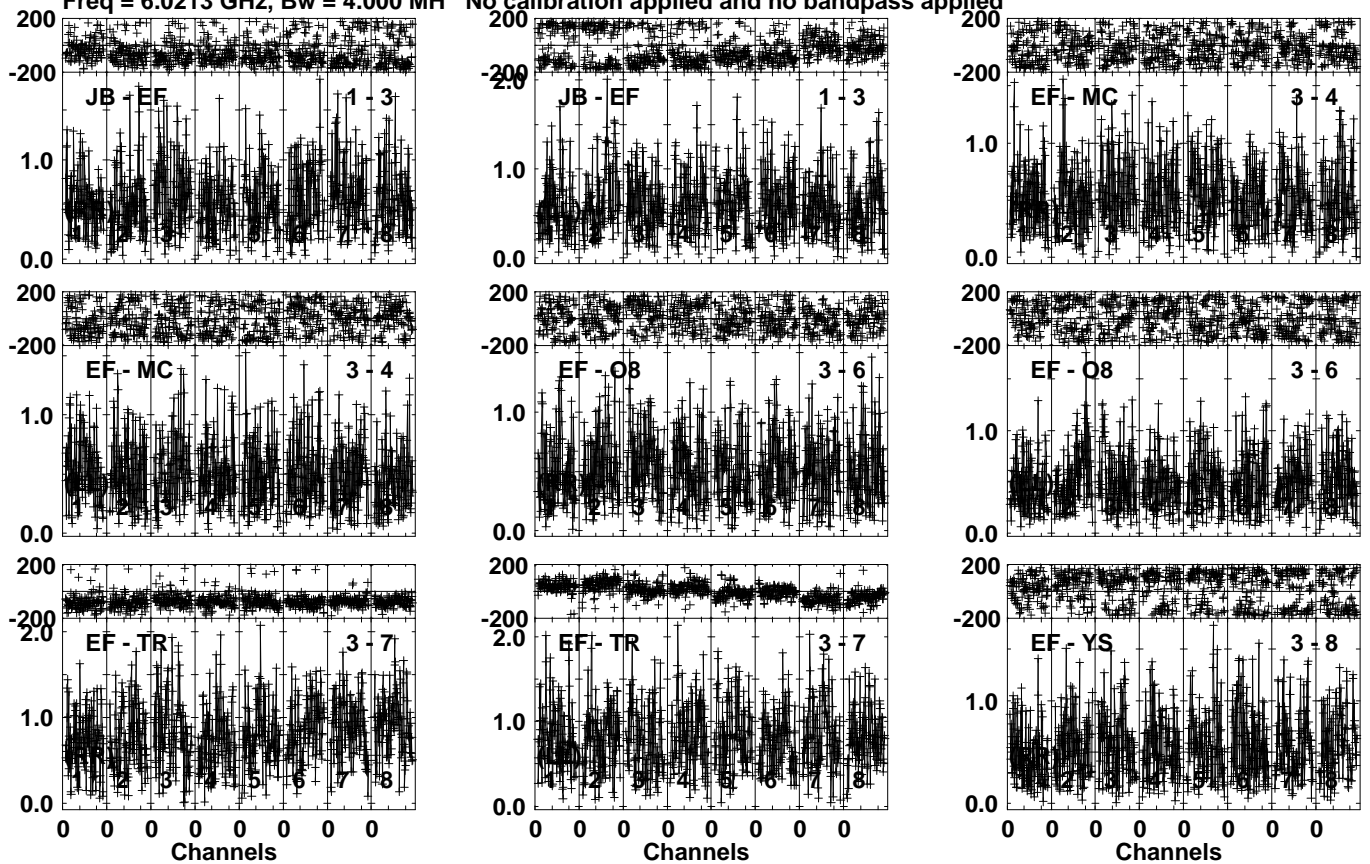
Lower frame: Milli Ampl Jy Top frame: Phas deg Vector averaged cross-power spectrum Several baselines displayed Timerange: 00/21:51:31 to 00/21:53:29
