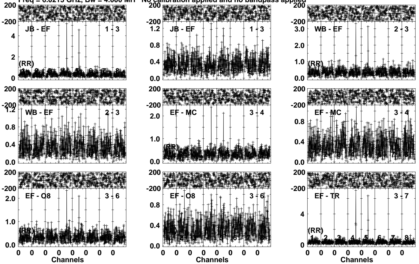
Lower frame: Milli Ampl Jy Top frame: Phas deg Vector averaged cross-power spectrum Several baselines displayed Timerange: 01/07:17:31 to 01/07:20:29
