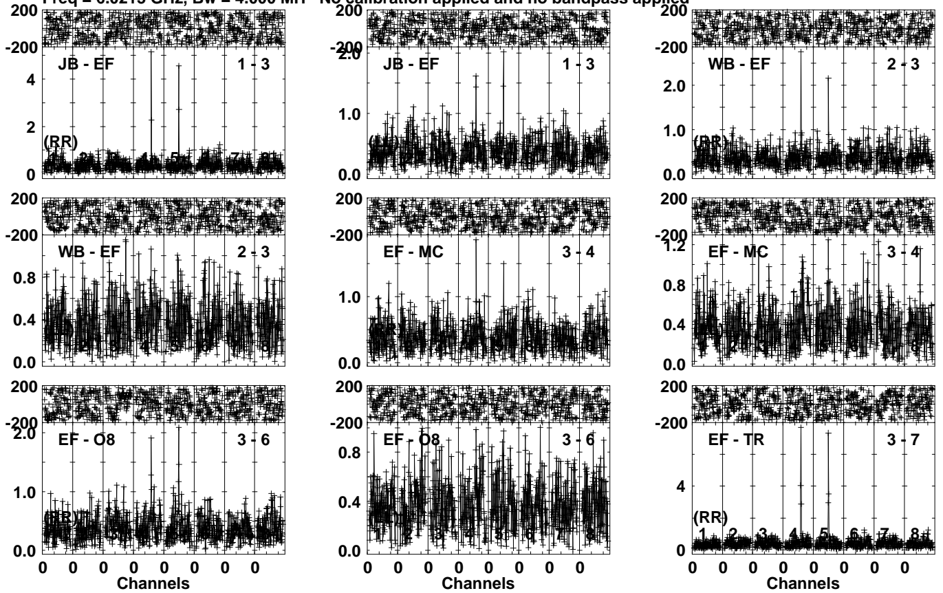
Lower frame: Milli Ampl Jy Top frame: Phas deg Vector averaged cross-power spectrum Several baselines displayed Timerange: 01/01:10:01 to 01/01:12:59
