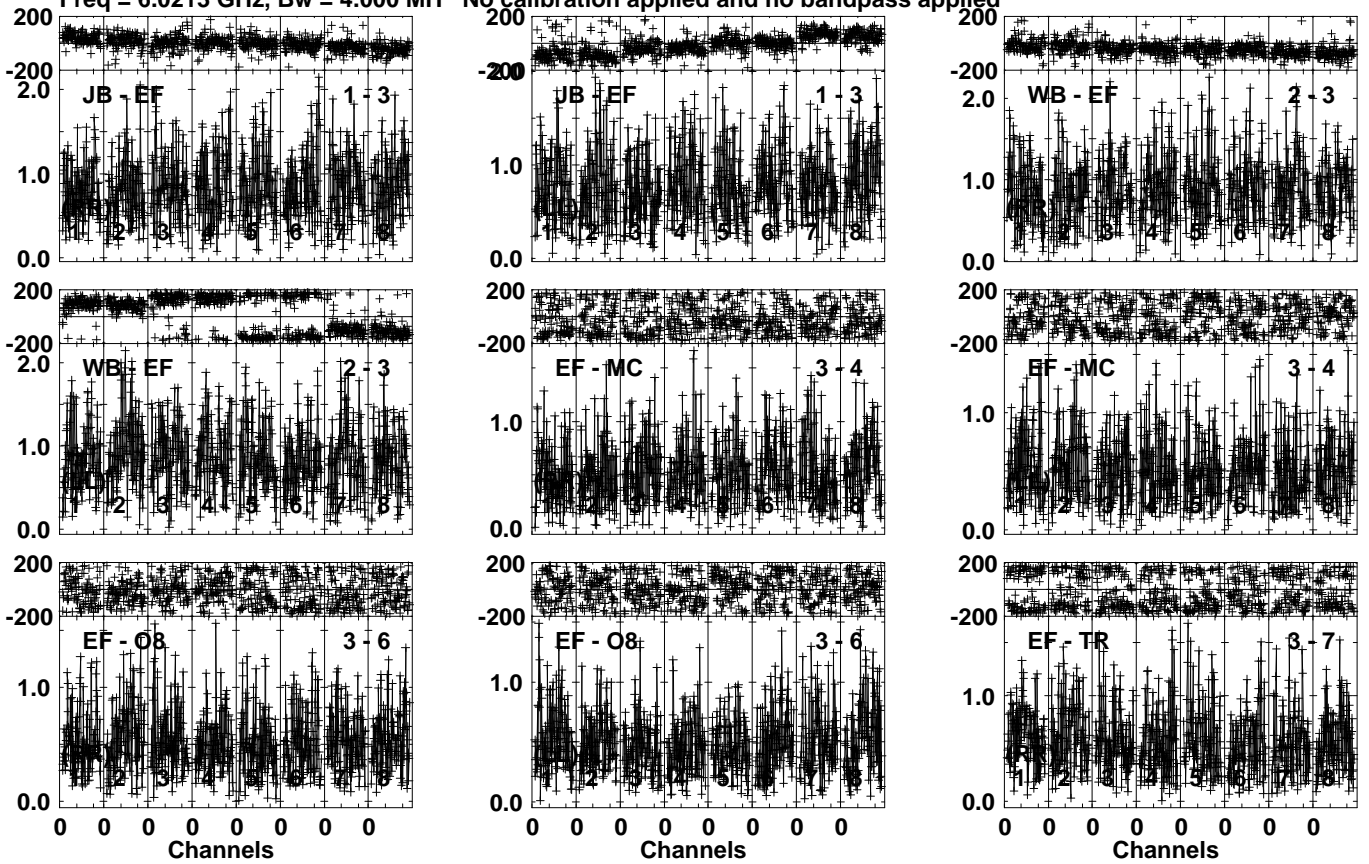
Lower frame: Milli Ampl Jy Top frame: Phas deg Vector averaged cross-power spectrum Several baselines displayed Timerange: 01/02:12:31 to 01/02:14:29
