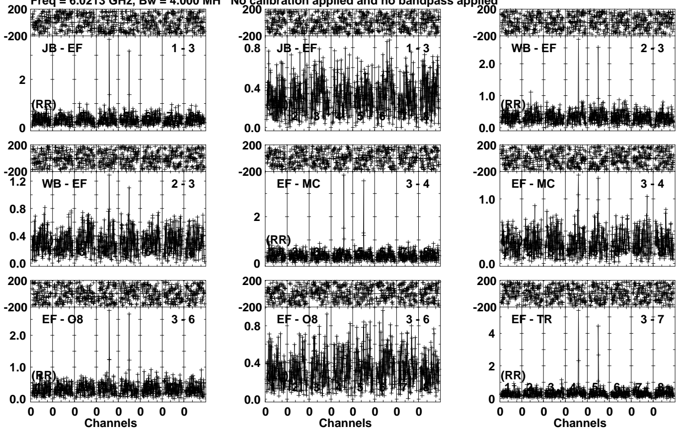
Lower frame: Milli Ampl Jy Top frame: Phas deg Vector averaged cross-power spectrum Several baselines displayed Timerange: 01/08:27:31 to 01/08:30:29
