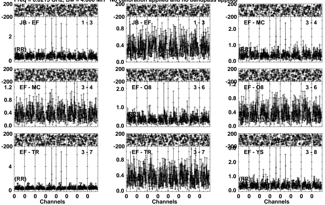
Lower frame: Milli Ampl Jy Top frame: Phas deg Vector averaged cross-power spectrum Several baselines displayed Timerange: 00/21:38:01 to 00/21:40:59
