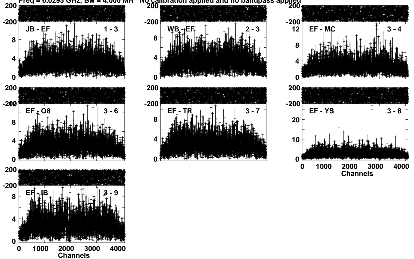
Lower frame: Milli Ampl Jy Top frame: Phas deg Vector averaged cross-power spectrum Several baselines displayed Timerange: 01/01:33:31 to 01/01:35:29
