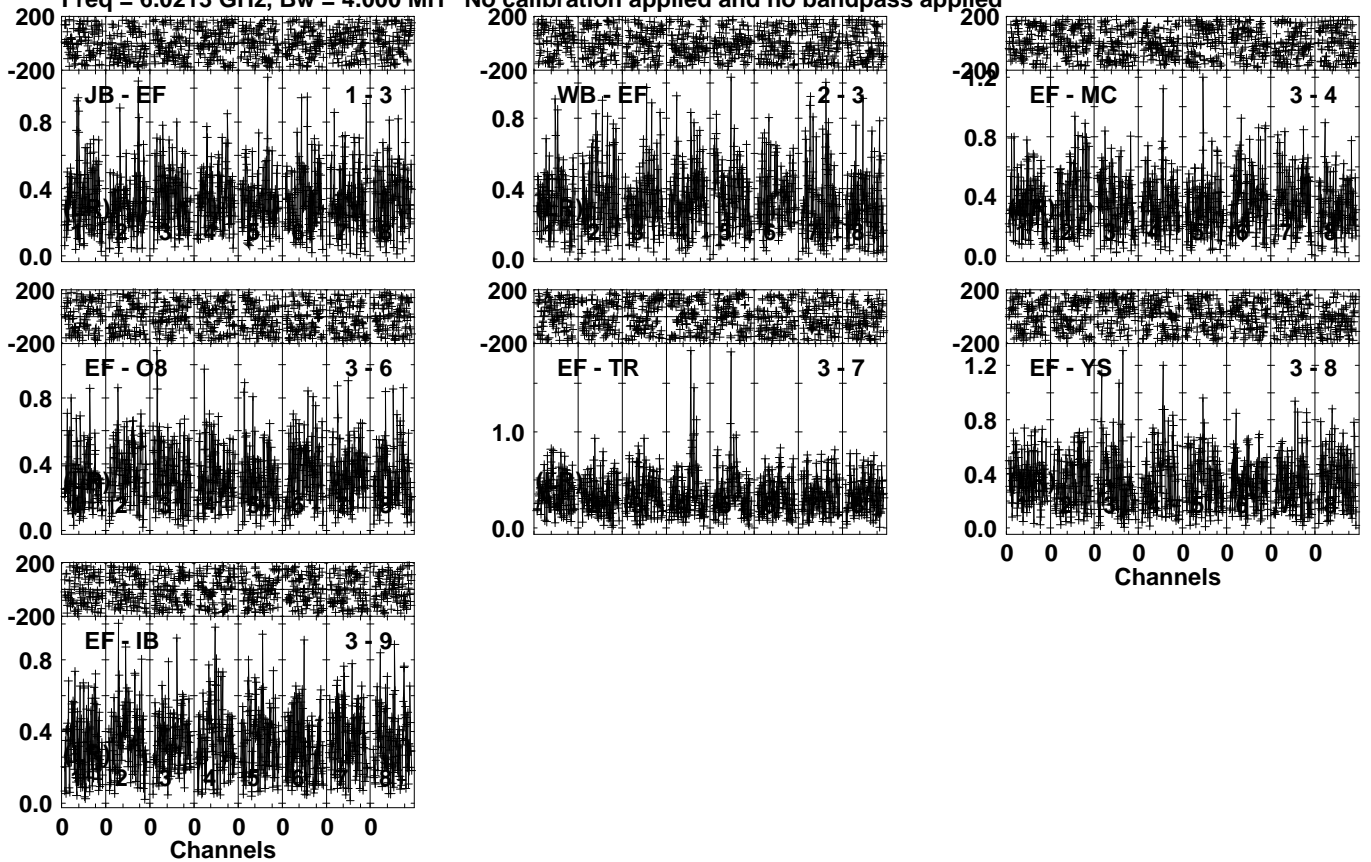
Lower frame: Milli Ampl Jy Top frame: Phas deg Vector averaged cross-power spectrum Several baselines displayed Timerange: 00/21:33:31 to 00/21:36:29
