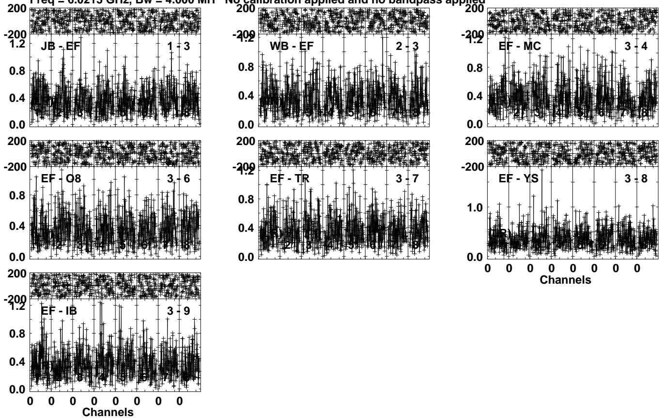
Lower frame: Milli Ampl Jy Top frame: Phas deg Vector averaged cross-power spectrum Several baselines displayed Timerange: 01/02:21:01 to 01/02:23:59
