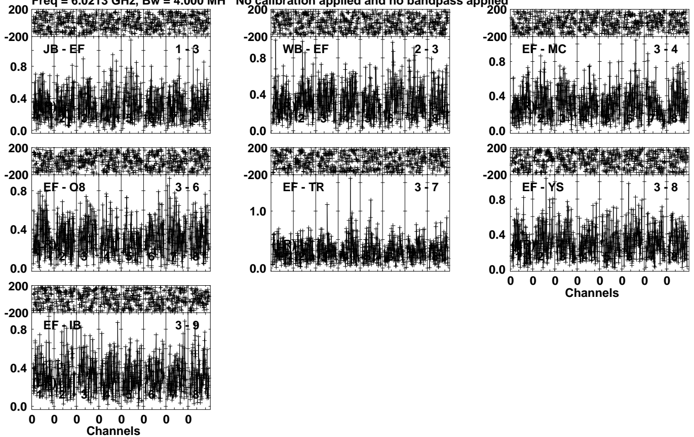
Lower frame: Milli Ampl Jy Top frame: Phas deg Vector averaged cross-power spectrum Several baselines displayed Timerange: 00/22:45:31 to 00/22:48:29
