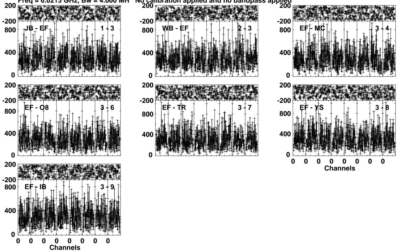
Lower frame: Micro Ampl Jy Top frame: Phas deg Vector averaged cross-power spectrum Several baselines displayed Timerange: 00/22:30:01 to 00/22:32:59
