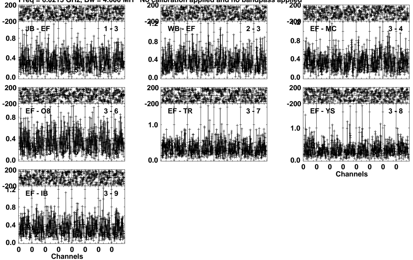
Lower frame: Milli Ampl Jy Top frame: Phas deg Vector averaged cross-power spectrum Several baselines displayed Timerange: 01/06:31:11 to 01/06:34:09
