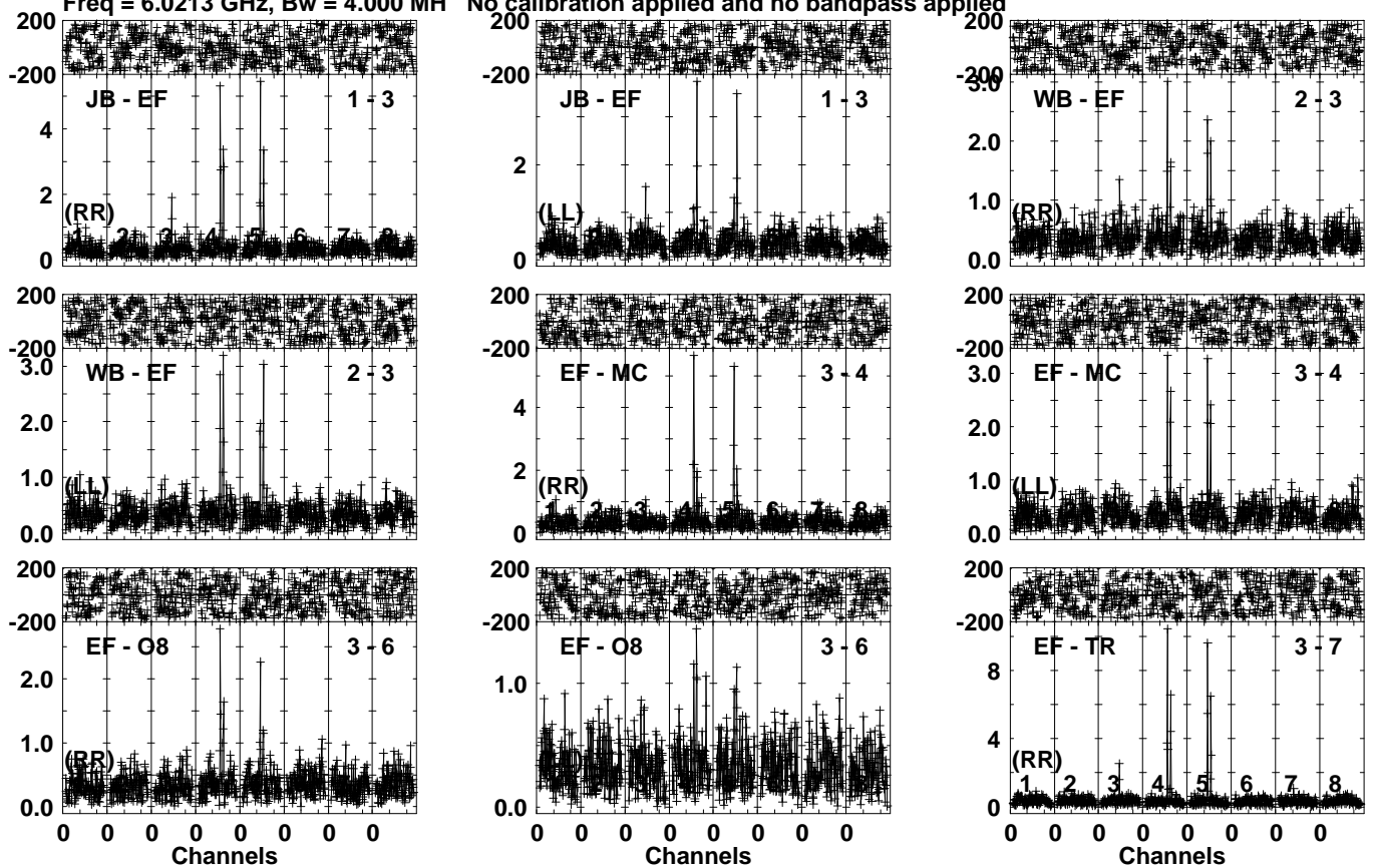
Lower frame: Milli Ampl Jy Top frame: Phas deg Vector averaged cross-power spectrum Several baselines displayed Timerange: 01/05:44:11 to 01/05:47:09
