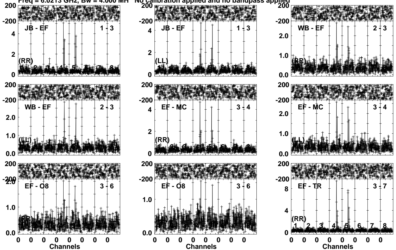
Lower frame: Milli Ampl Jy Top frame: Phas deg Vector averaged cross-power spectrum Several baselines displayed Timerange: 01/07:39:11 to 01/07:42:09
