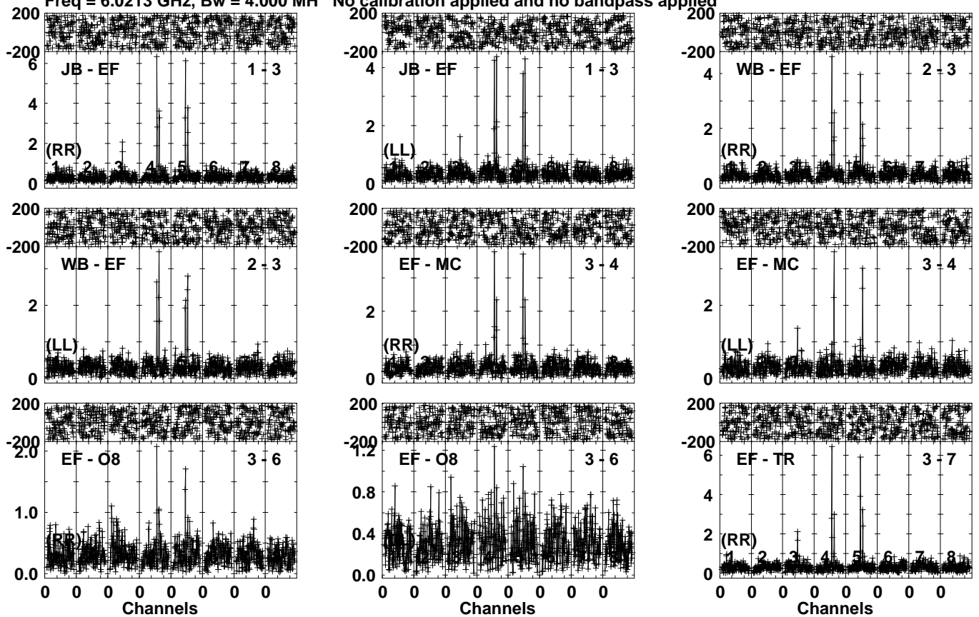
Lower frame: Milli Ampl Jy Top frame: Phas deg Vector averaged cross-power spectrum Several baselines displayed Timerange: 01/06:26:11 to 01/06:29:09
