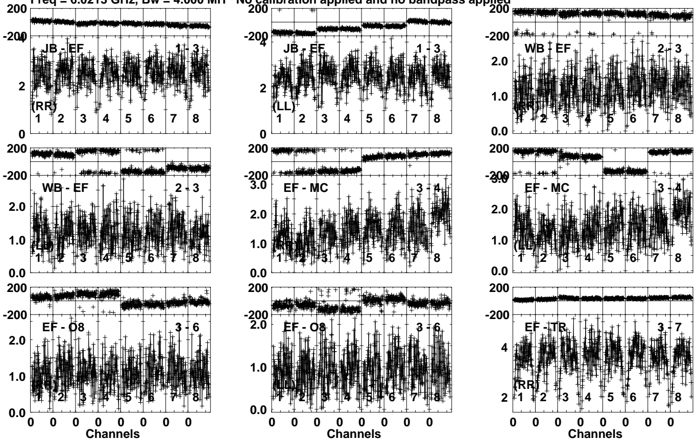
Lower frame: Milli Ampl Jy Top frame: Phas deg Vector averaged cross-power spectrum Several baselines displayed Timerange: 01/03:38:41 to 01/03:40:39
