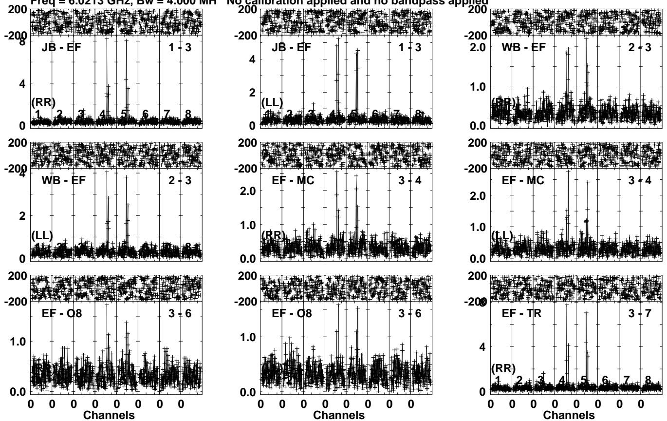
Lower frame: Milli Ampl Jy Top frame: Phas deg Vector averaged cross-power spectrum Several baselines displayed Timerange: 00/23:16:01 to 00/23:18:59
