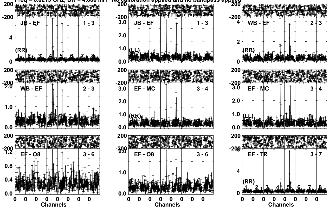
Lower frame: Milli Ampl Jy Top frame: Phas deg Vector averaged cross-power spectrum Several baselines displayed Timerange: 00/21:13:01 to 00/21:15:59
