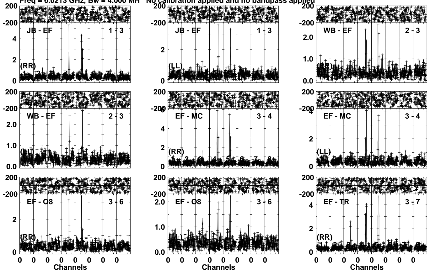
Lower frame: Milli Ampl Jy Top frame: Phas deg Vector averaged cross-power spectrum Several baselines displayed Timerange: 01/04:30:11 to 01/04:33:09
