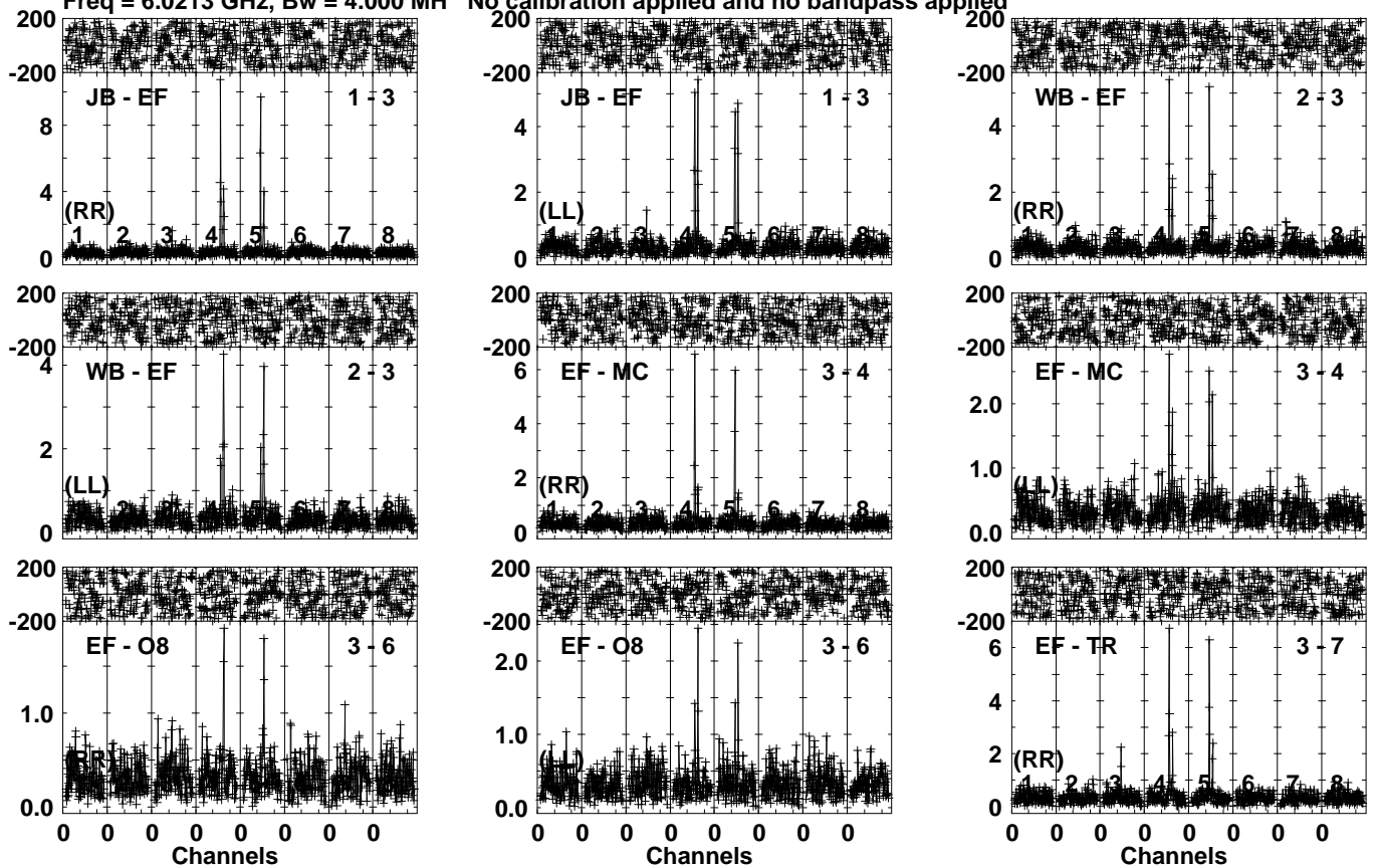
Lower frame: Milli Ampl Jy Top frame: Phas deg Vector averaged cross-power spectrum Several baselines displayed Timerange: 01/02:16:01 to 01/02:18:59
