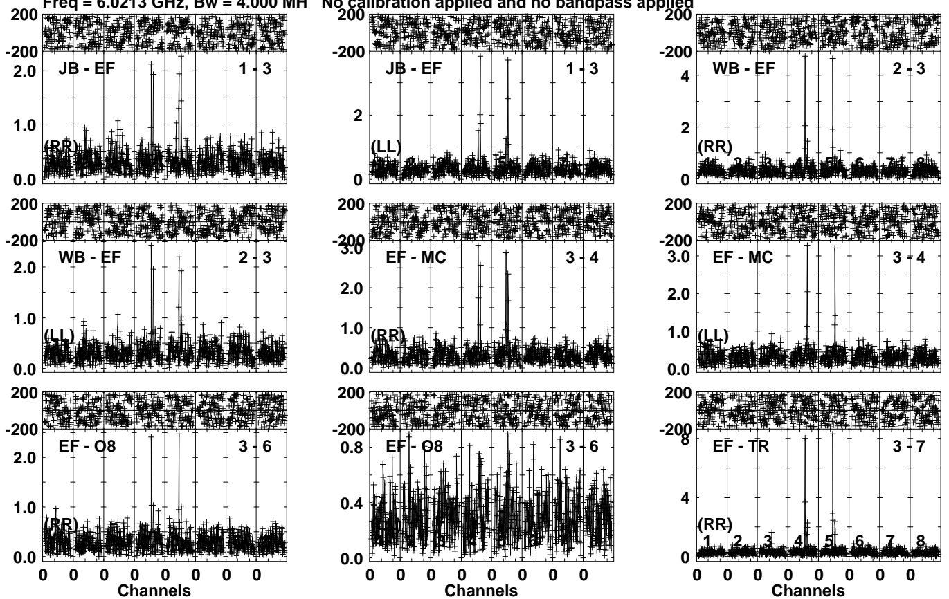
Lower frame: Milli Ampl Jy Top frame: Phas deg Vector averaged cross-power spectrum Several baselines displayed Timerange: 00/21:28:31 to 00/21:31:29
